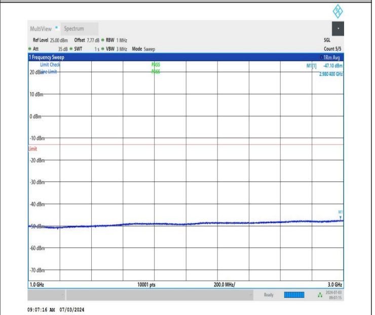
NTNV_DC_26A_n77A-3450-3550_PC2_30_5+40_M+M_TID2_N S_01_1000_3000_#1
