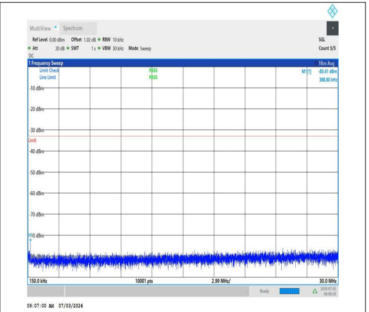
NTNV_DC_26A_n77A-3450-3550_PC2_30_5+40_M+M_TID2_N S_01_0.15_30_#1
