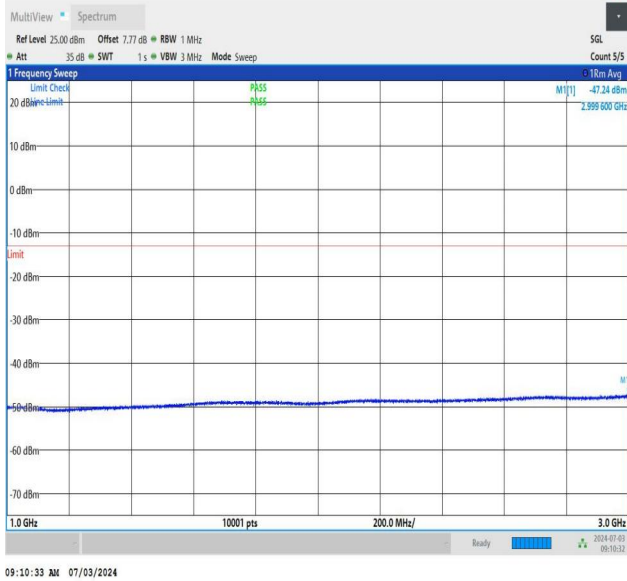
NTNV_DC_26A_n77A-3450-3550_PC2_30_5+40_M+H_TID1_N S_01_1000_3000_#1
