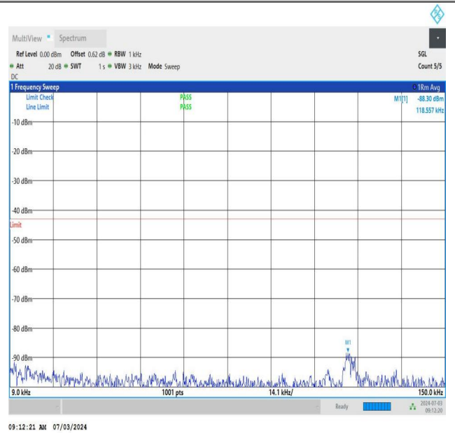
NTNV_DC_26A_n77A-3450-3550_PC2_30_5+40_M+H_TID4_N S_01_0.009_0.15_#1
