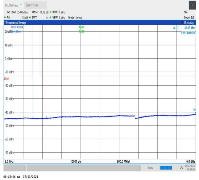
NTNV_DC_26A_n77A-3450-3550_PC2_30_5+50_M+L_TID1_NS_01_3000_6000_#1
