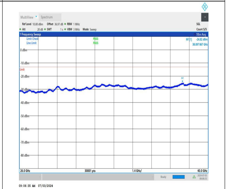
NTNV_DC_26A_n77A-3450-3550_PC2_30_5+40_M+M_TID1_N S_01_26000_40000_#1
