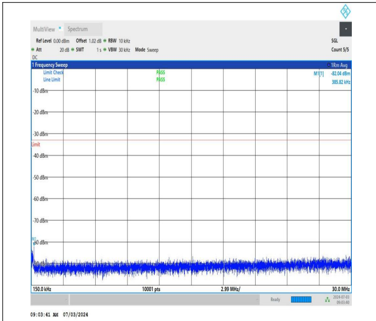
NTNV_DC_26A_n77A-3450-3550_PC2_30_5+40_M+L_TID4_NS_01_0.15_30_#1
