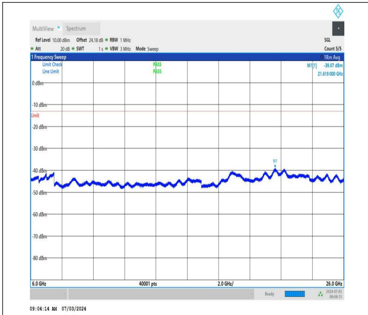
NTNV_DC_26A_n77A-3450-3550_PC2_30_5+40_M+L_TID4_NS_01_6000_26000_#1
