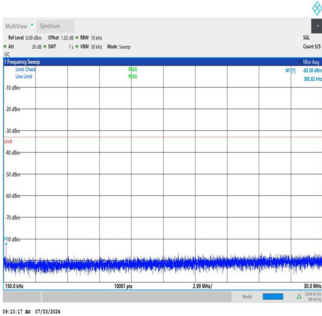
NTNV_DC_26A_n77A-3450-3550_PC2_30_5+40_M+H_TID1_N S_01_0.15_30_#1
