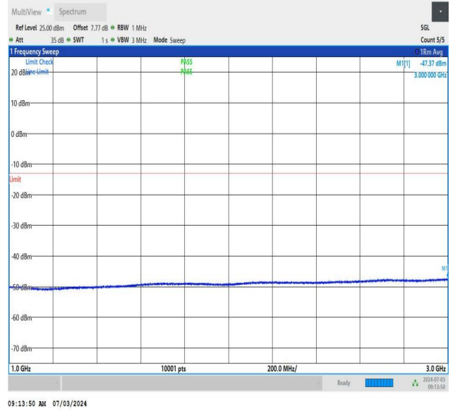
NTNV_DC_26A_n77A-3450-3550_PC2_30_5+40_M+H_TID5_N S_01_1000_3000_#1
