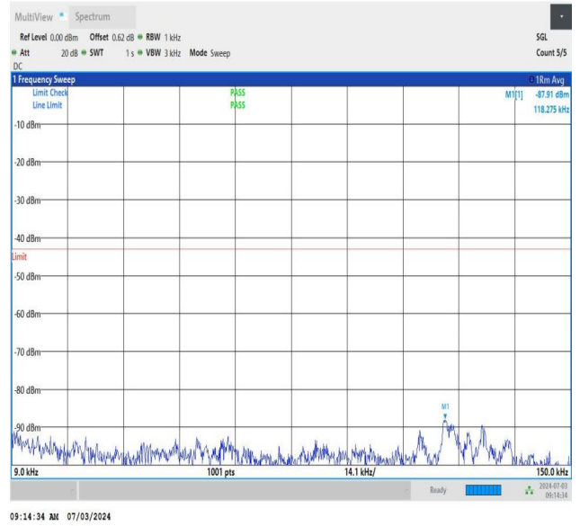
NTNV_DC_26A_n77A-3450-3550_PC2_30_5+50_M+L_TID1_NS _01_0.009_0.15_#1
