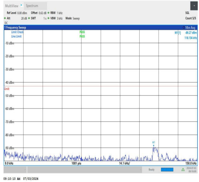
NTNV_DC_26A_n77A-3450-3550_PC2_30_5+40_M+H_TID1_N S_01_0.009_0.15_#1
