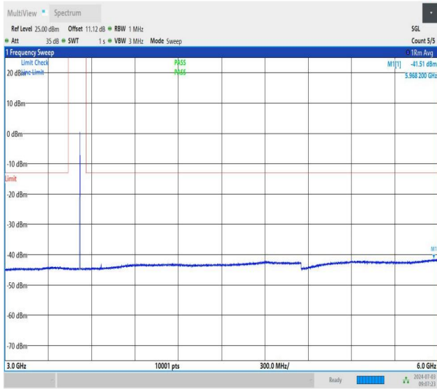
NTNV_DC_26A_n77A-3450-3550_PC2_30_5+40_M+M_TID2_N S_01_3000_6000_#1
