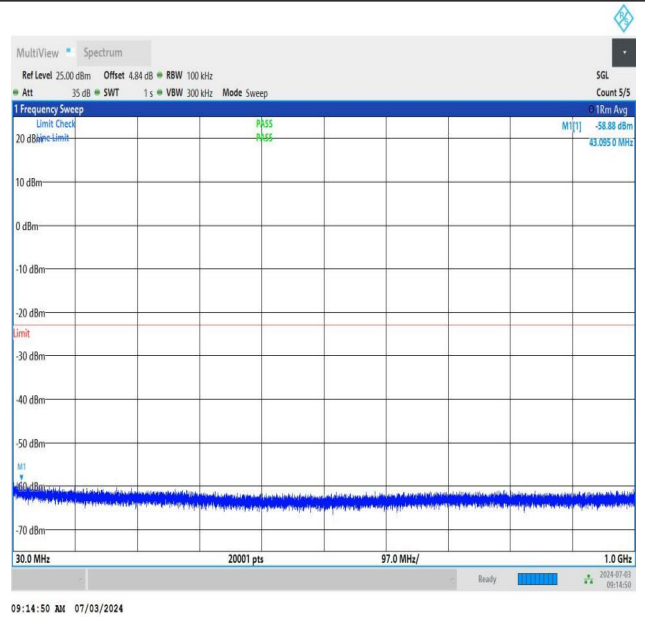
NTNV_DC_26A_n77A-3450-3550_PC2_30_5+50_M+L_TID1_NS _01_30_1000_#1
