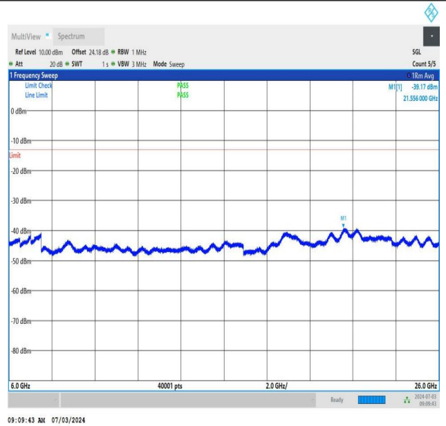
NTNV_DC_26A_n77A-3450-3550_PC2_30_5+40_M+M_TID5_N S_01_6000_26000_#1
