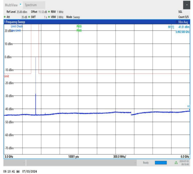
NTNV_DC_26A_n77A-3450-3550_PC2_30_5+40_M+H_TID1_N S_01_3000_6000_#1
