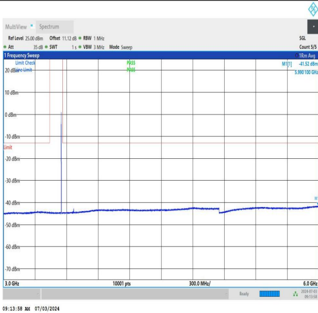
NTNV_DC_26A_n77A-3450-3550_PC2_30_5+40_M+H_TID5_N S_01_3000_6000_#1
