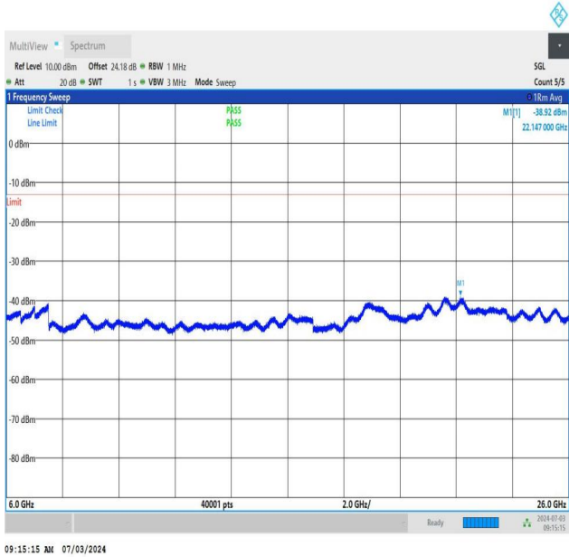
NTNV_DC_26A_n77A-3450-3550_PC2_30_5+50_M+L_TID1_NS_01_6000_26000_#1
