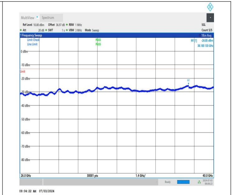
NTNV_DC_26A_n77A-3450-3550_PC2_30_5+40_M+L_TID4_NS_01_26000_40000_#1
