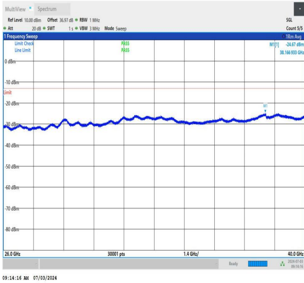
NTNV_DC_26A_n77A-3450-3550_PC2_30_5+40_M+H_TID5_N S_01_26000_40000_#1
