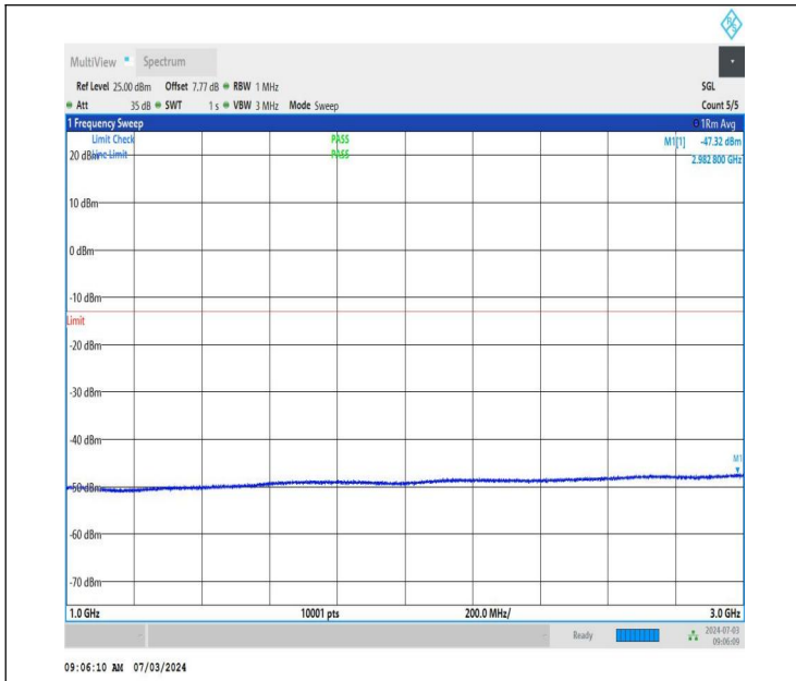
NTNV_DC_26A_n77A-3450-3550_PC2_30_5+40_M+M_TID1_N S_01_1000_3000_#1
