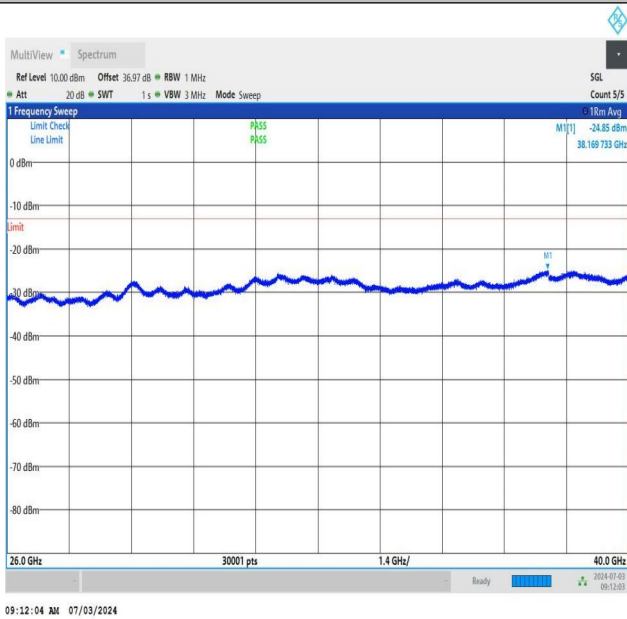
NTNV_DC_26A_n77A-3450-3550_PC2_30_5+40_M+H_TID2_N S_01_26000_40000_#1
