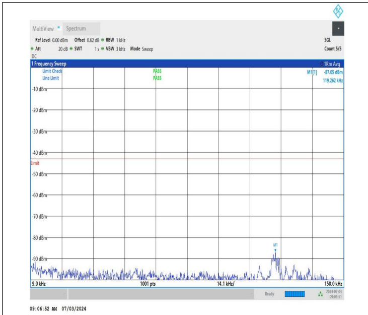
NTNV_DC_26A_n77A-3450-3550_PC2_30_5+40_M+M_TID2_N S_01_0.009_0.15_#1
