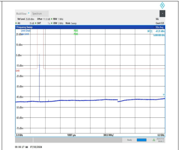
NTNV_DC_26A_n77A-3450-3550_PC2_30_5+40_M+M_TID1_N S_01_3000_6000_#1
