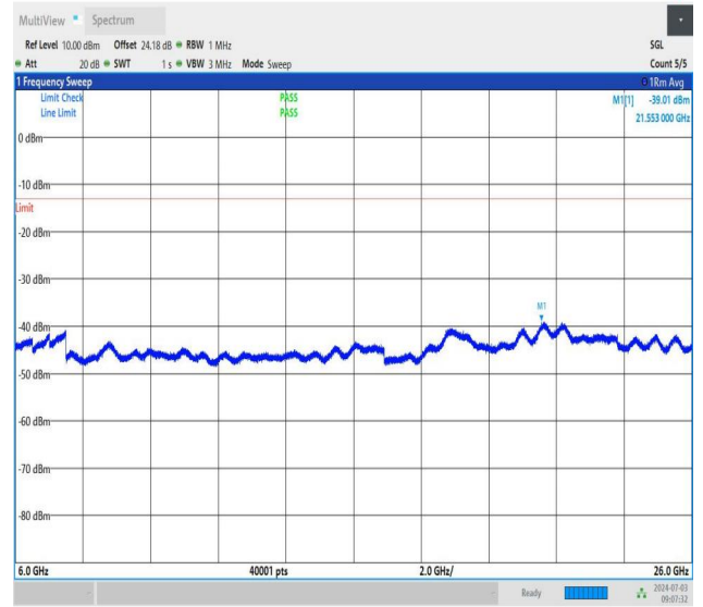
NTNV_DC_26A_n77A-3450-3550_PC2_30_5+40_M+M_TID2_N S_01_6000_26000_#1
