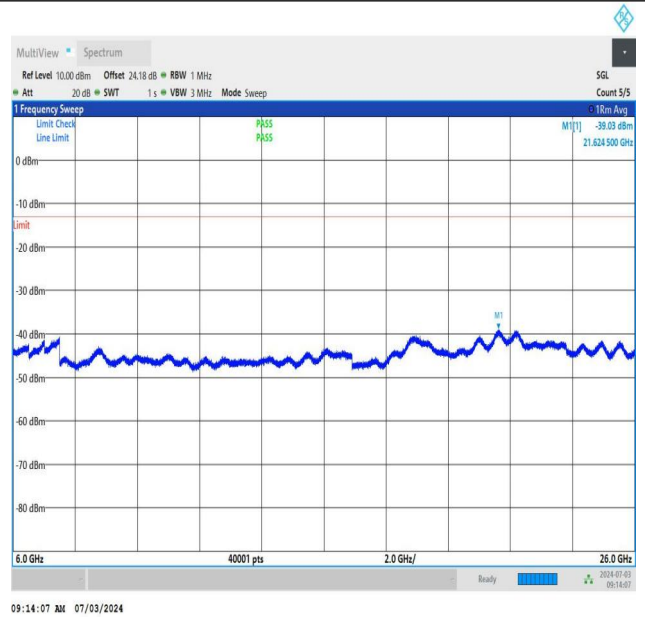
NTNV_DC_26A_n77A-3450-3550_PC2_30_5+40_M+H_TID5_N S_01_6000_26000_#1
