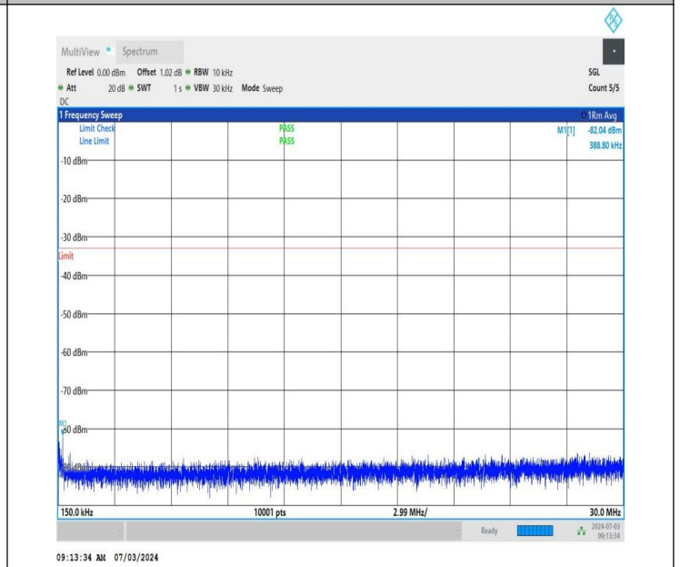
NTNV_DC_26A_n77A-3450-3550_PC2_30_5+40_M+H_TID5_N S_01_0.15_30_#1
