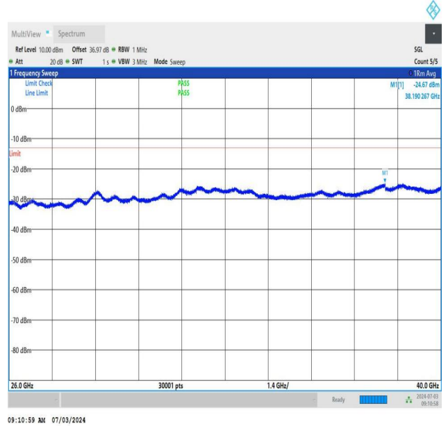
NTNV_DC_26A_n77A-3450-3550_PC2_30_5+40_M+H_TID1_N S_01_26000_40000_#1
