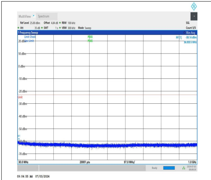
NTNV_DC_26A_n77A-3450-3550_PC2_30_5+40_M+L_TID5_NS_01_30_1000_#1
