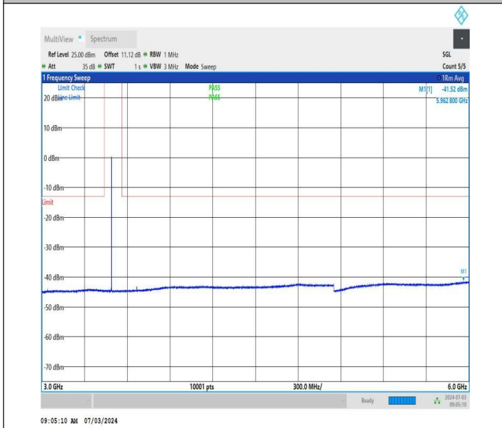
NTNV_DC_26A_n77A-3450-3550_PC2_30_5+40_M+L_TID5_NS_01_3000_6000_#1
