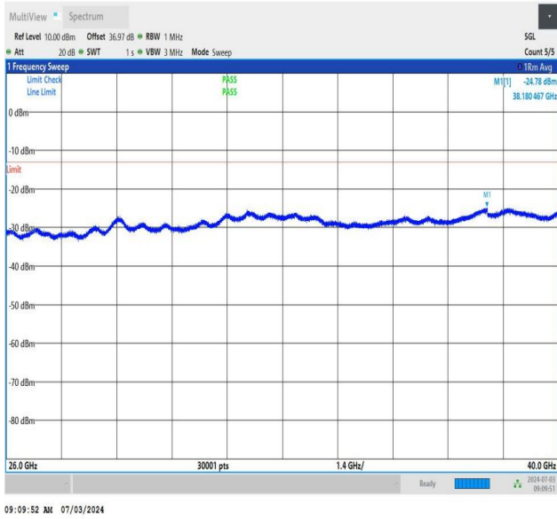
NTNV_DC_26A_n77A-3450-3550_PC2_30_5+40_M+M_TID5_N S_01_26000_40000_#1
