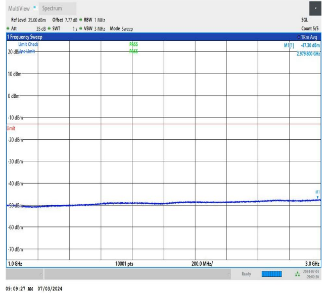
NTNV_DC_26A_n77A-3450-3550_PC2_30_5+40_M+M_TID5_N S_01_1000_3000_#1
