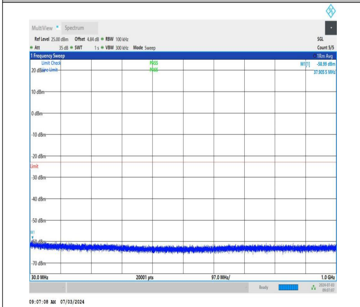
NTNV_DC_26A_n77A-3450-3550_PC2_30_5+40_M+M_TID2_N S_01_30_1000_#1
