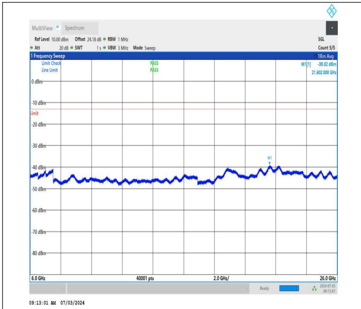
NTNV_DC_26A_n77A-3450-3550_PC2_30_5+40_M+H_TID4_N S_01_6000_26000_#1
