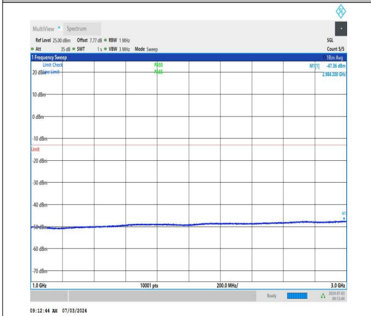
NTNV_DC_26A_n77A-3450-3550_PC2_30_5+40_M+H_TID4_N S_01_1000_3000_#1
