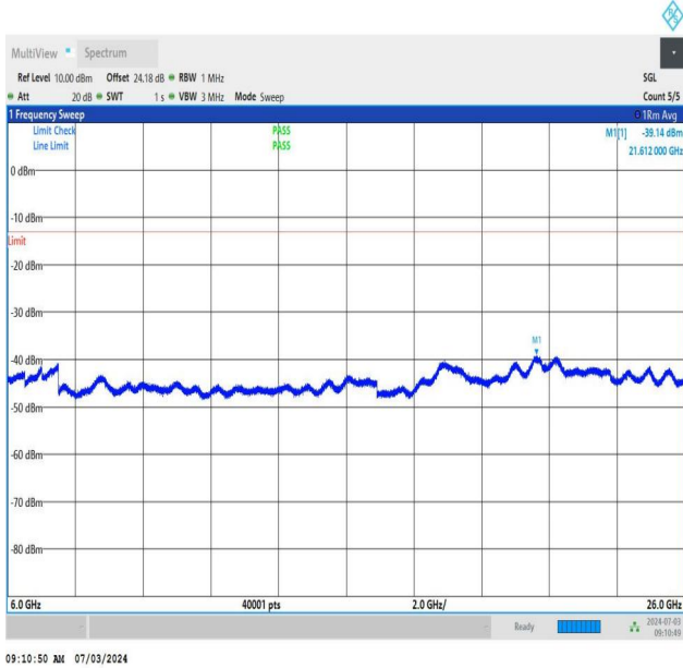
NTNV_DC_26A_n77A-3450-3550_PC2_30_5+40_M+H_TID1_N S_01_6000_26000_#1
