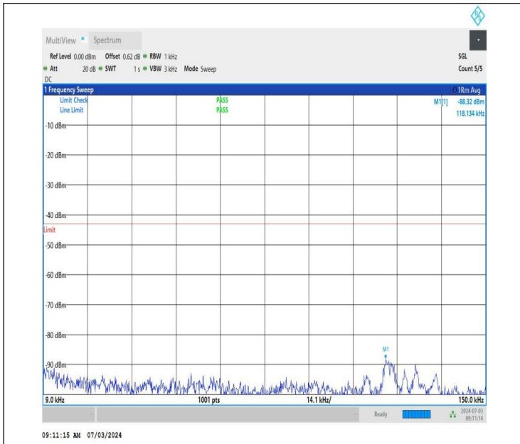
NTNV_DC_26A_n77A-3450-3550_PC2_30_5+40_M+H_TID2_N S_01_0.009_0.15_#1
