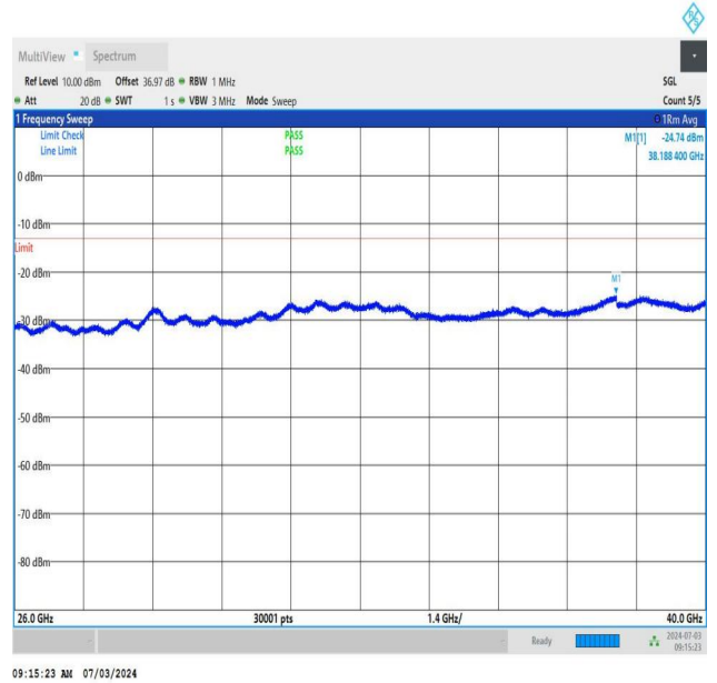
NTNV_DC_26A_n77A-3450-3550_PC2_30_5+50_M+L_TID1_NS_01_26000_40000_#1
