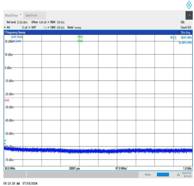
NTNV_DC_26A_n77A-3450-3550_PC2_30_5+40_M+H_TID1_N S_01_30_1000_#1
