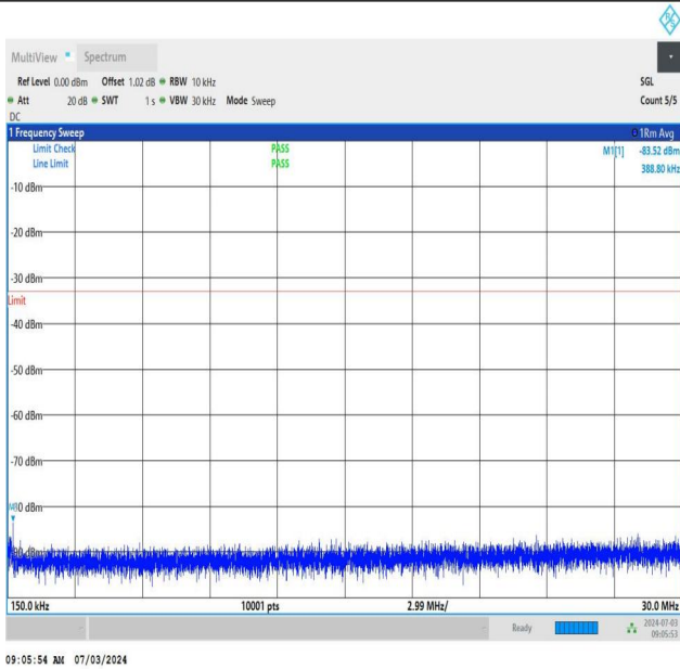
NTNV_DC_26A_n77A-3450-3550_PC2_30_5+40_M+M_TID1_N_S_01_0.15_30_#1
