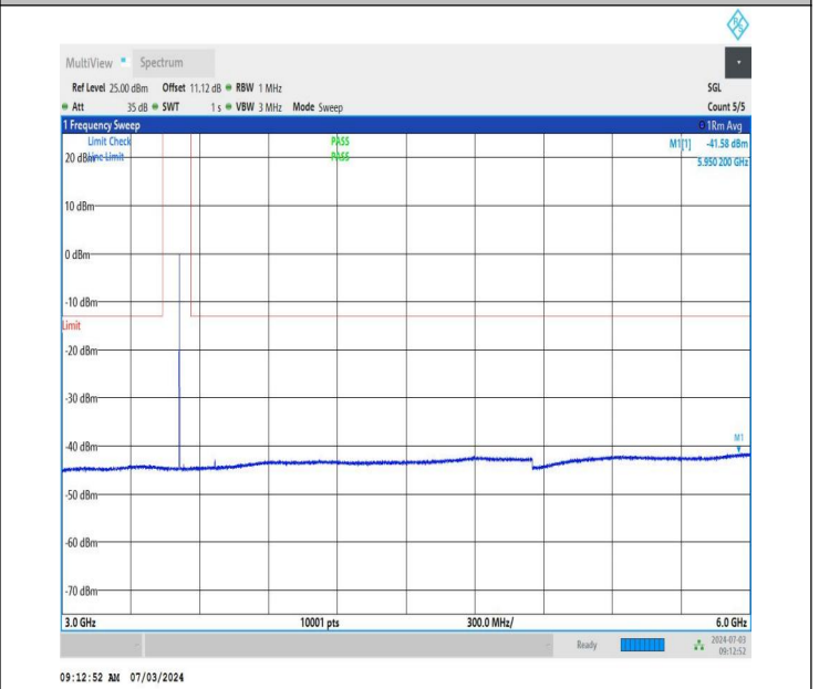
NTNV_DC_26A_n77A-3450-3550_PC2_30_5+40_M+H_TID4_N S_01_3000_6000_#1
