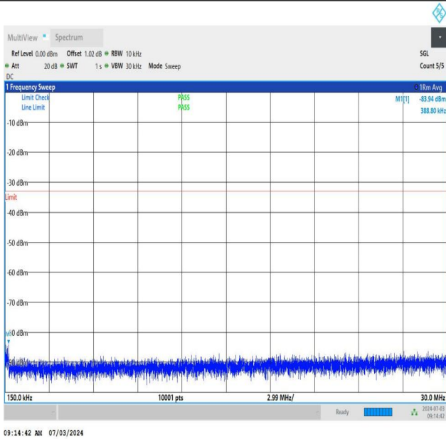
NTNV_DC_26A_n77A-3450-3550_PC2_30_5+50_M+L_TID1_NS _01_0.15_30_#1
