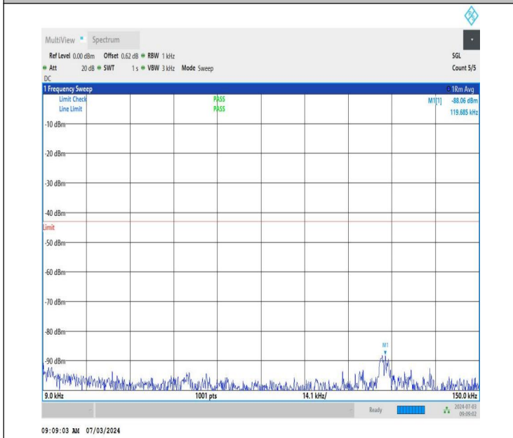
NTNV_DC_26A_n77A-3450-3550_PC2_30_5+40_M+M_TID5_N S_01_0.009_0.15_#1
