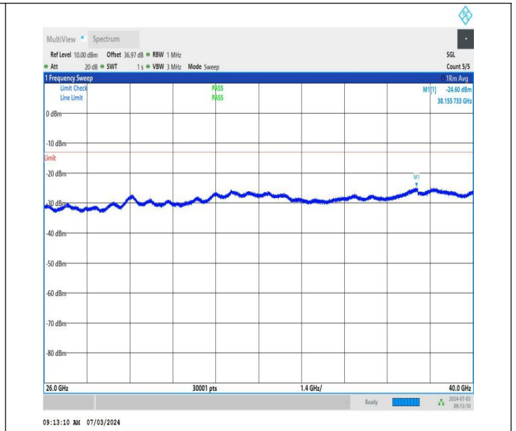
NTNV_DC_26A_n77A-3450-3550_PC2_30_5+40_M+H_TID4_N S_01_26000_40000_#1
