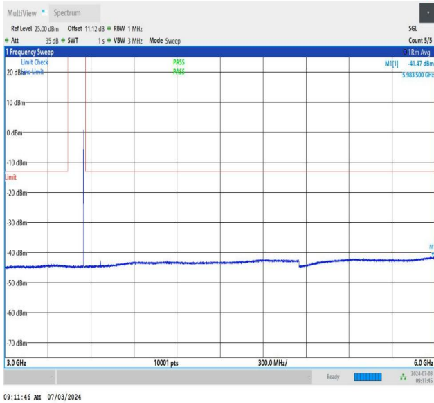
NTNV_DC_26A_n77A-3450-3550_PC2_30_5+40_M+H_TID2_N S_01_3000_6000_#1
