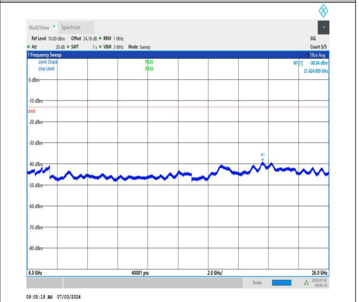
NTNV_DC_26A_n77A-3450-3550_PC2_30_5+40_M+L_TID5_NS_01_6000_26000_#1
