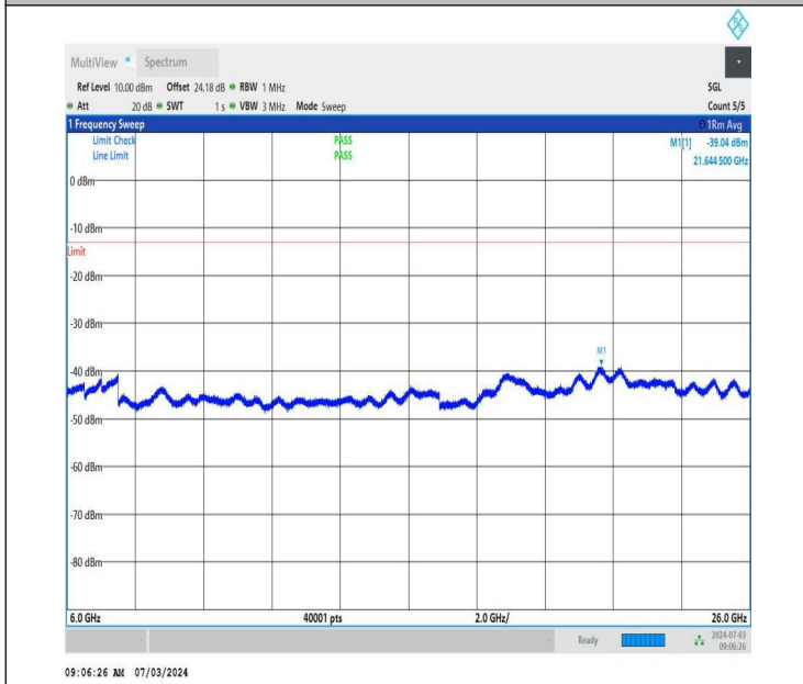
NTNV_DC_26A_n77A-3450-3550_PC2_30_5+40_M+M_TID1_N S_01_6000_26000_#1
