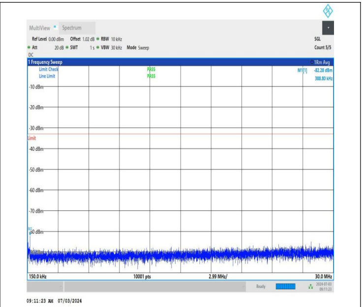
NTNV_DC_26A_n77A-3450-3550_PC2_30_5+40_M+H_TID2_N S_01_0.15_30_#1
