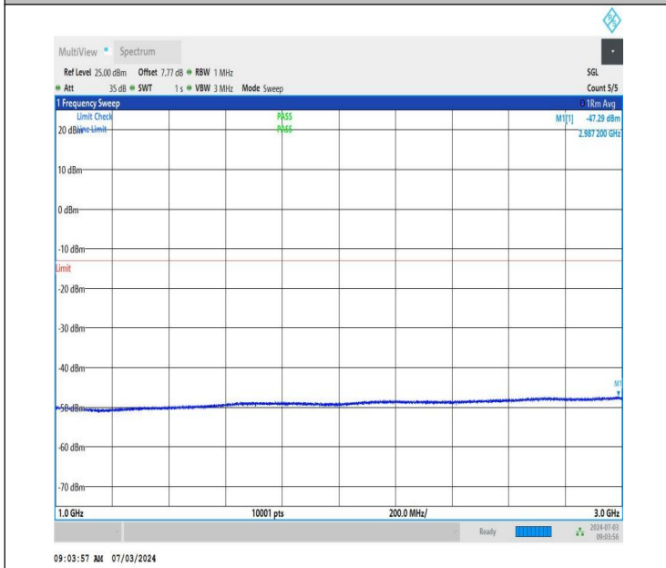
NTNV_DC_26A_n77A-3450-3550_PC2_30_5+40_M+L_TID4_NS_01_1000_3000_#1
