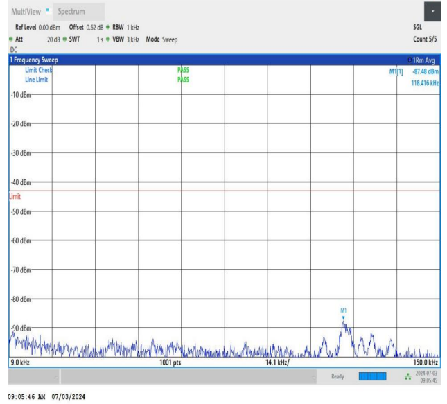
NTNV_DC_26A_n77A-3450-3550_PC2_30_5+40_M+M_TID1_N_S_01_0.009_0.15_#1
