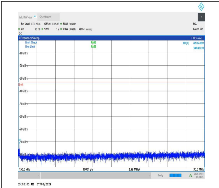
NTNV_DC_26A_n77A-3450-3550_PC2_30_5+40_M+M_TID4_N S_01_0.15_30_#1
