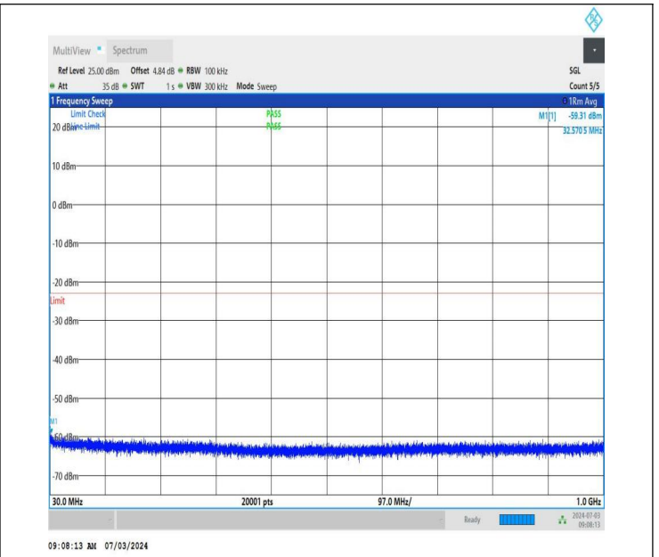
NTNV_DC_26A_n77A-3450-3550_PC2_30_5+40_M+M_TID4_N S_01_30_1000_#1
