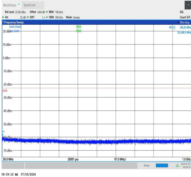
NTNV_DC_26A_n77A-3450-3550_PC2_30_5+40_M+M_TID5_N S_01_30_1000_#1
