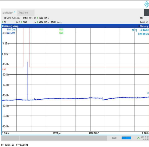
NTNV_DC_26A_n77A-3450-3550_PC2_30_5+40_M+M_TID5_N S_01_3000_6000_#1
