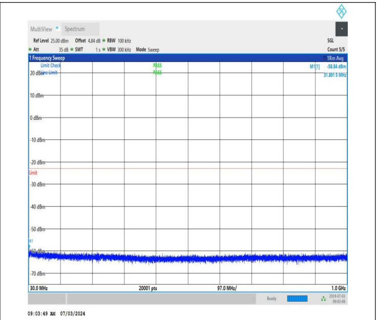
NTNV_DC_26A_n77A-3450-3550_PC2_30_5+40_M+L_TID4_NS_01_30_1000_#1
