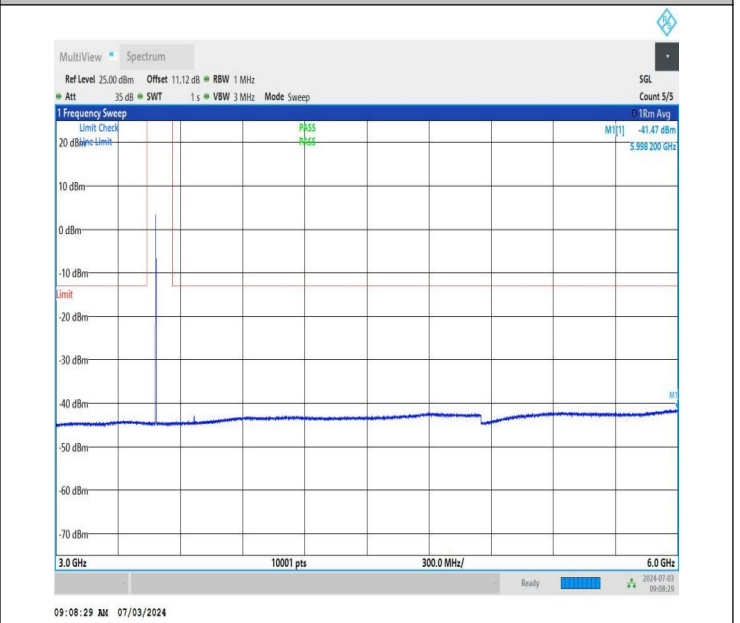
NTNV_DC_26A_n77A-3450-3550_PC2_30_5+40_M+M_TID4_N S_01_3000_6000_#1
