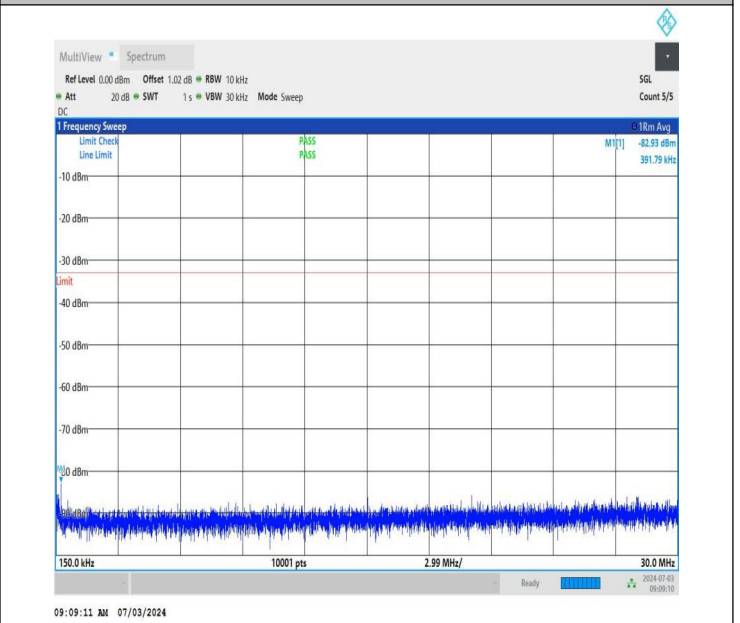
NTNV_DC_26A_n77A-3450-3550_PC2_30_5+40_M+M_TID5_N S_01_0.15_30_#1
