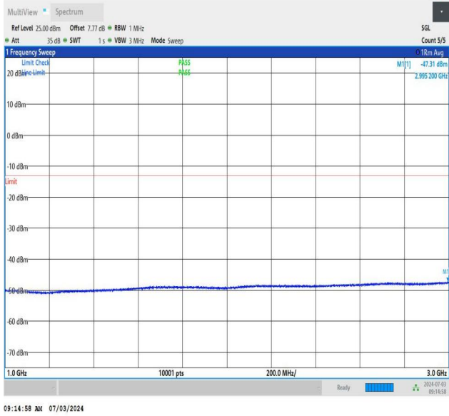
NTNV_DC_26A_n77A-3450-3550_PC2_30_5+50_M+L_TID1_NS_01_1000_3000_#1
