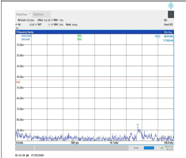
NTNV_DC_26A_n77A-3450-3550_PC2_30_5+40_M+H_TID5_N S_01_0.009_0.15_#1
