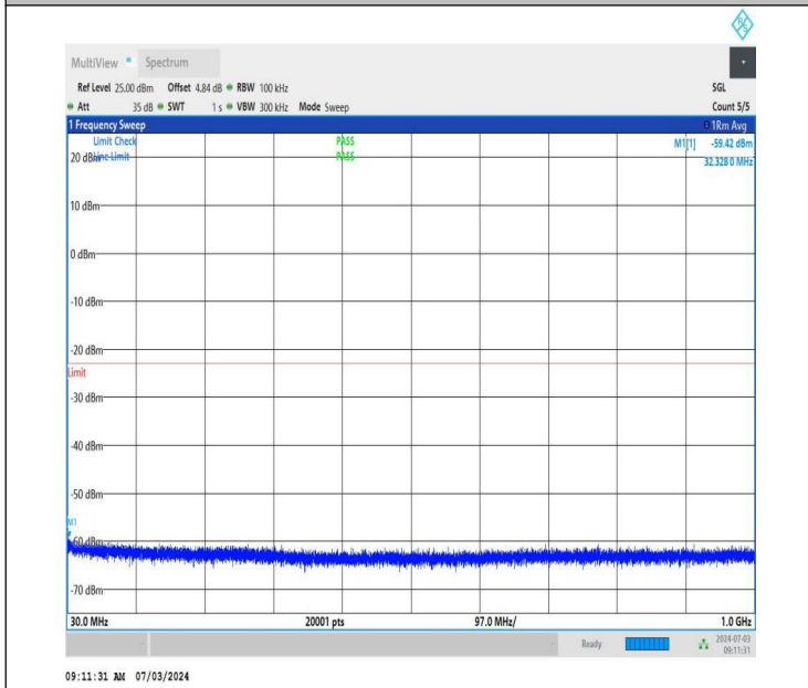
NTNV_DC_26A_n77A-3450-3550_PC2_30_5+40_M+H_TID2_N S_01_30_1000_#1
