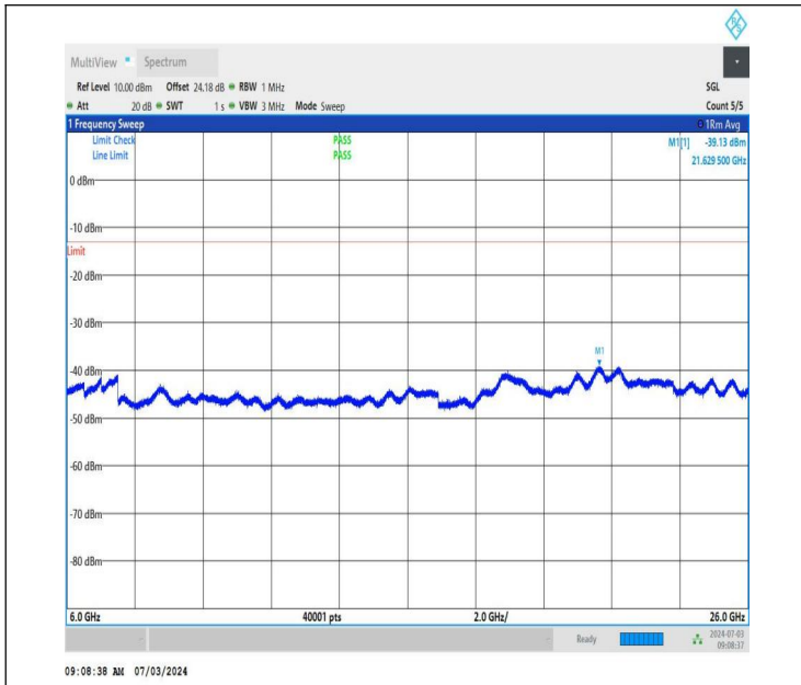
NTNV_DC_26A_n77A-3450-3550_PC2_30_5+40_M+M_TID4_N S_01_6000_26000_#1
