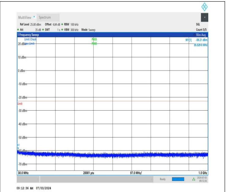
NTNV_DC_26A_n77A-3450-3550_PC2_30_5+40_M+H_TID4_N S_01_30_1000_#1
