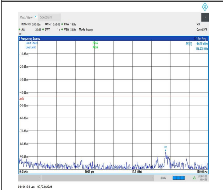
NTNV_DC_26A_n77A-3450-3550_PC2_30_5+40_M+L_TID5_NS_01_0.009_0.15_#1
