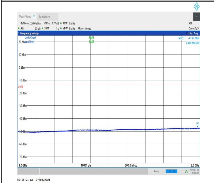
NTNV_DC_26A_n77A-3450-3550_PC2_30_5+40_M+M_TID4_N S_01_1000_3000_#1
