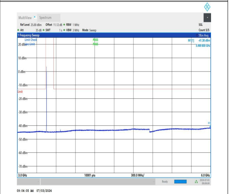
NTNV_DC_26A_n77A-3450-3550_PC2_30_5+40_M+L_TID4_NS_01_3000_6000_#1
