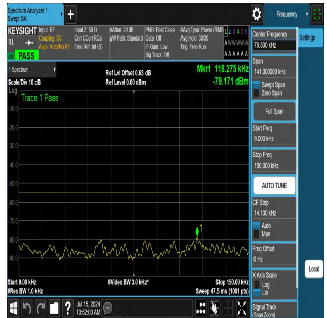
NTNV-N41-PC3-30-50-L-DFT-PI2BPSK-Edge_1RB_Left-0.009-0. 15-Ant1-PASS
