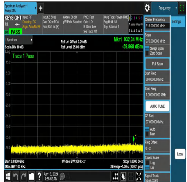
NTNV-N41-PC3-30-50-L-DFT-PI2BPSK-Edge_1RB_Left-30-1000-Ant1-PASS
