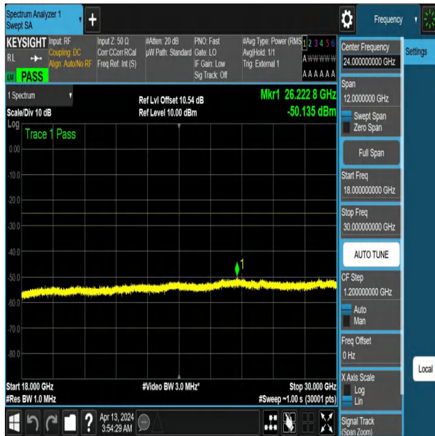
NTNV-N41-PC3-30-40-L-DFT-QPSK-Edge_1RB_Left-18000-3000 0-Ant1-PASS
