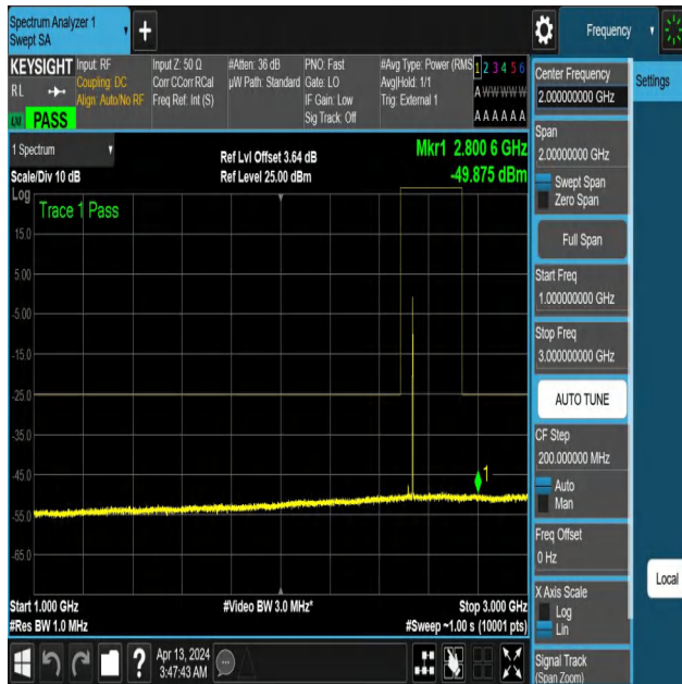
NTNV-N41-PC3-30-40-L-DFT-PI2BPSK-Edge_1RB_Right-1000-3 000-Ant1-PASS
