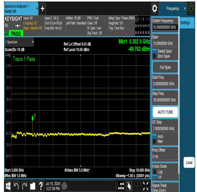
NTNV-N41-PC3-30-40-H-DFT-QPSK-Edge_1RB_Left-3000-1800 0-Ant1-PASS
