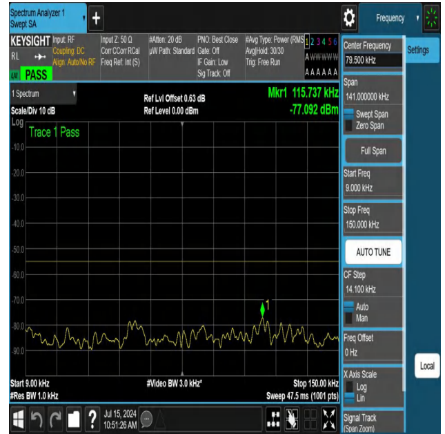
NTNV-N41-PC3-30-40-H-DFT-PI2BPSK-Edge_1RB_Right-0.009- 0.15-Ant1-PASS
