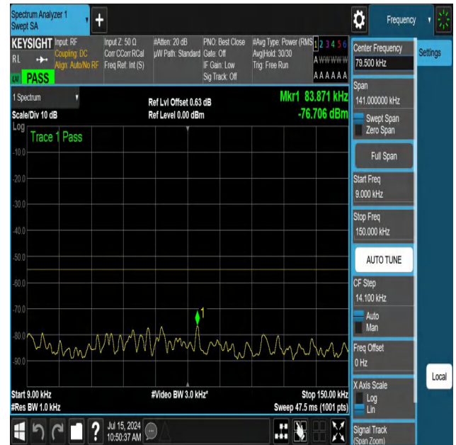
NTNV-N41-PC3-30-40-M-DFT-P12BPSK-Edge_1RB_Right-0.009 -0.15-Ant1-PASS
