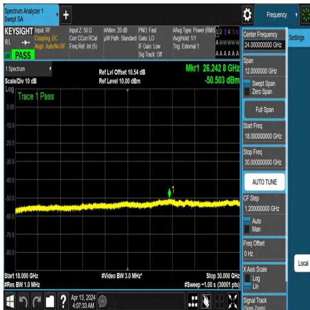
NTNV-N41-PC3-30-40-M-DFT-PI2BPSK-Edge_1RB_Right-18000-30000-Ant1-PASS
