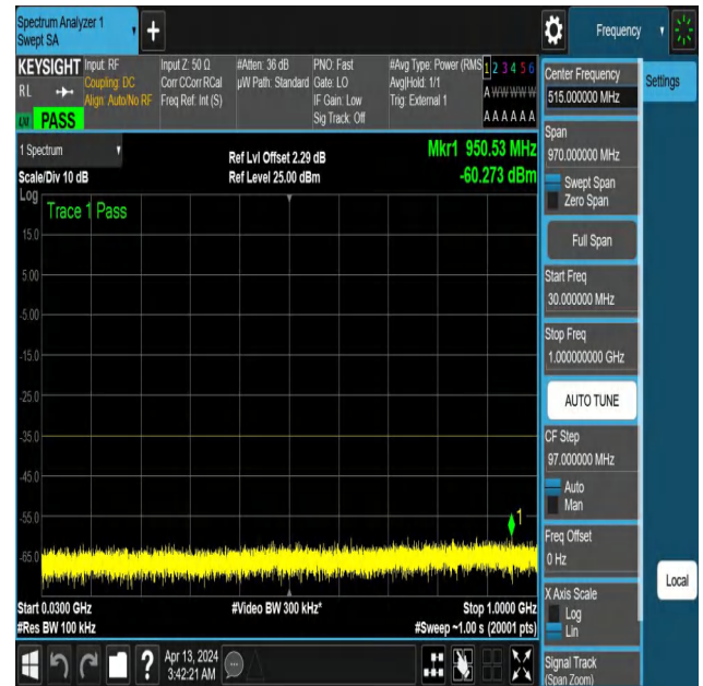
NTNV-N41-PC3-30-40-L-DFT-PI2BPSK-Edge_1RB_Left-30-1000 -Ant1-PASS
