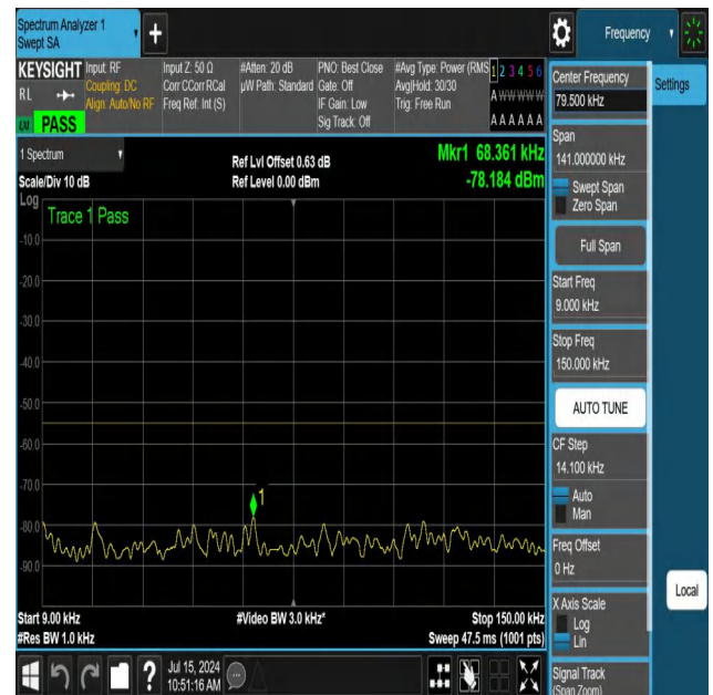
NTNV-N41-PC3-30-40-H-DFT-PI2BPSK-Edge_1RB_Left-0.009-0.15-Ant1-PASS
