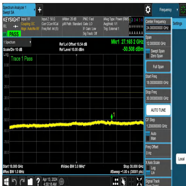
NTNV-N41-PC3-30-40-H-DFT-QPSK-Edge_1RB_Left-18000-3000 0-Ant1-PASS
