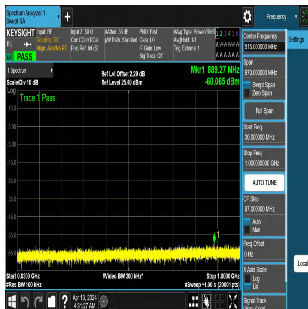
NTNV-N41-PC3-30-40-H-DFT-QPSK-Edge_1RB_Right-30-1000- Ant1-PASS
