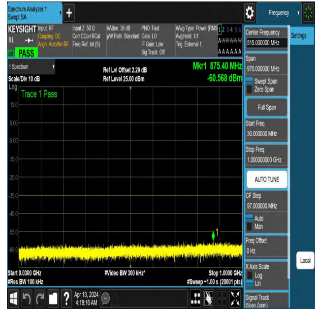
NTNV-N41-PC3-30-40-H-DFT-PI2BPSK-Edge_1RB_Left-30-100-0-Ant1-PASS
