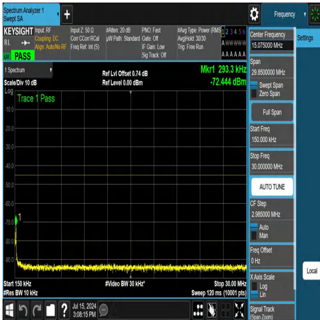
NTNV-N41-PC3-30-40-L-DFT-PI2BPSK-Edge_1RB_Right-0.15-30-Ant1-PASS
