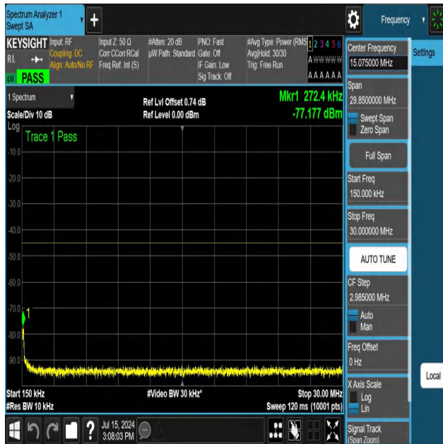
NTNV-N41-PC3-30-40-L-DFT-PI2BPSK-Edge_1RB_Left-0.15-30-Ant1-PASS
