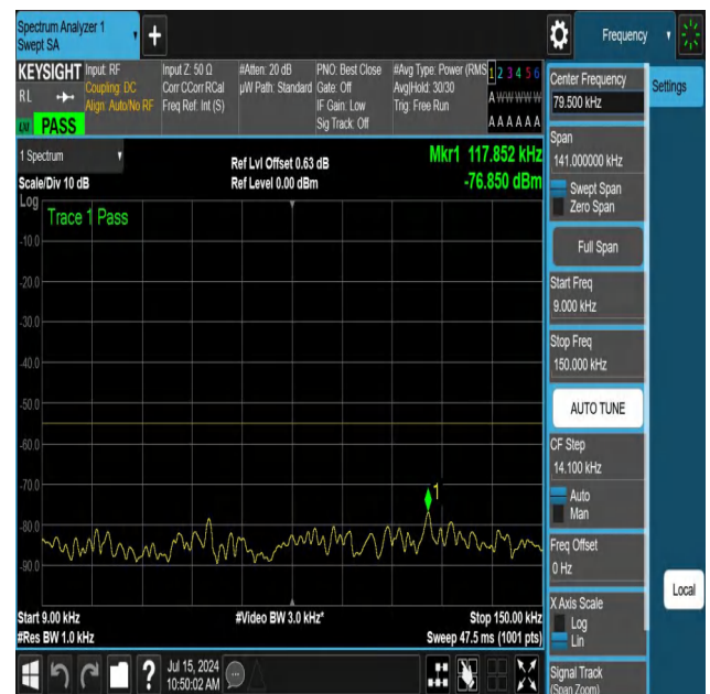
NTNV-N41-PC3-30-40-L-DFT-QPSK-Edge_1RB_Left-0.009-0.15- Ant1-PASS
