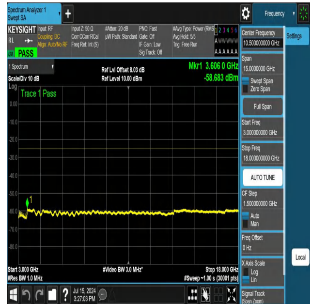
NTNV-N41-PC3-30-40-H-DFT-PI2BPSK-Edge_1RB_Left-3000-18000-Ant1-PASS
