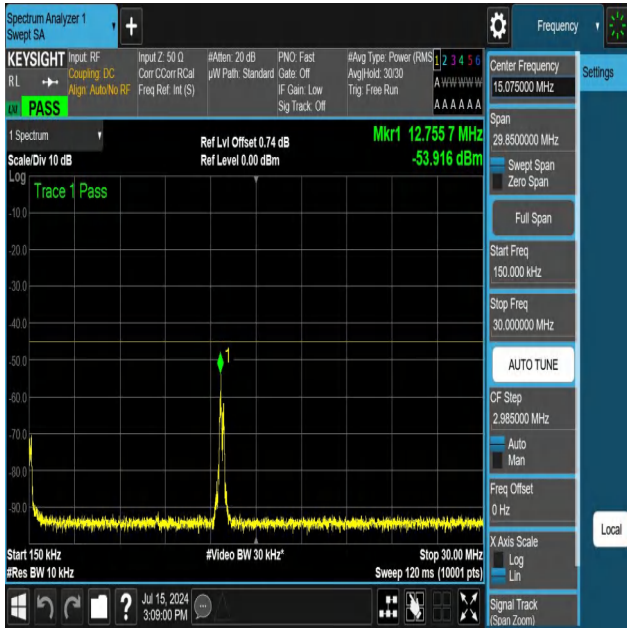
NTNV-N41-PC3-30-40-M-DFT-PI2BPSK-Edge_1RB_Left-0.15-30- Ant1-PASS
