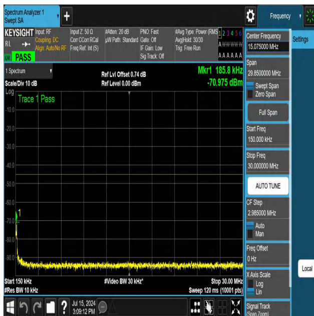
NTNV-N41-PC3-30-40-M-DFT-PI2BPSK-Edge_1RB_Right-0.15-3 0-Ant1-PASS
