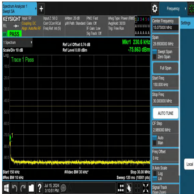
NTNV-N41-PC3-30-50-L-DFT-PI2BPSK-Edge_1RB_Left-0.15-30-Ant1-PASS
