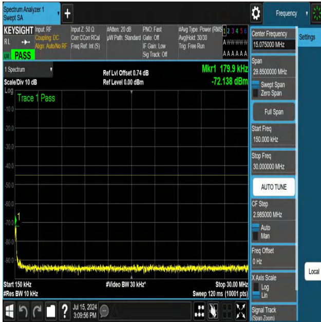
NTNV-N41-PC3-30-40-H-DFT-PI2BPSK-Edge_1RB_Left-0.15-30-Ant1-PASS
