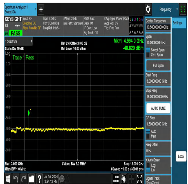
NTNV-N41-PC3-30-40-L-DFT-PI2BPSK-Edge_1RB_Left-3000-18 000-Ant1-PASS
