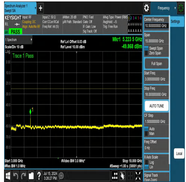
NTNV-IN41-PC3-30-40-M-DFT-QPSK-Edge_1RB_Right-3000-18 000-Ant1-PASS
