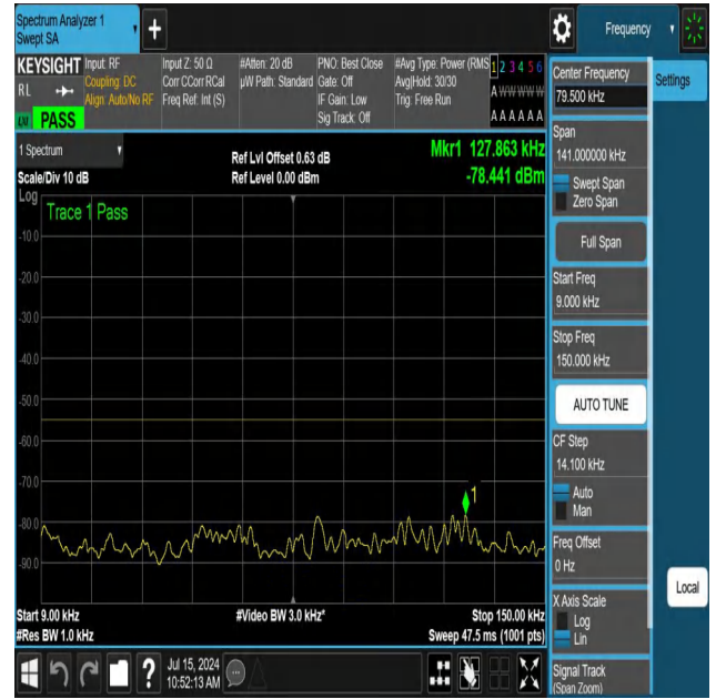
NTNV-N41-PC3-30-50-L-DFT-PI2BPSK-Edge_1RB_Right-0.009-0.15-Ant1-PASS
