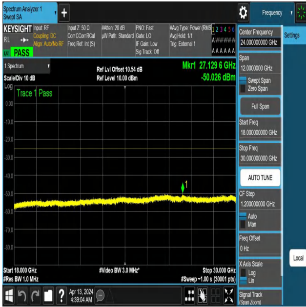
NTNV-N41-PC3-30-50-L-DFT-PI2BPSK-Edge_1RB_Left-18000-30000-Ant1-PASS
