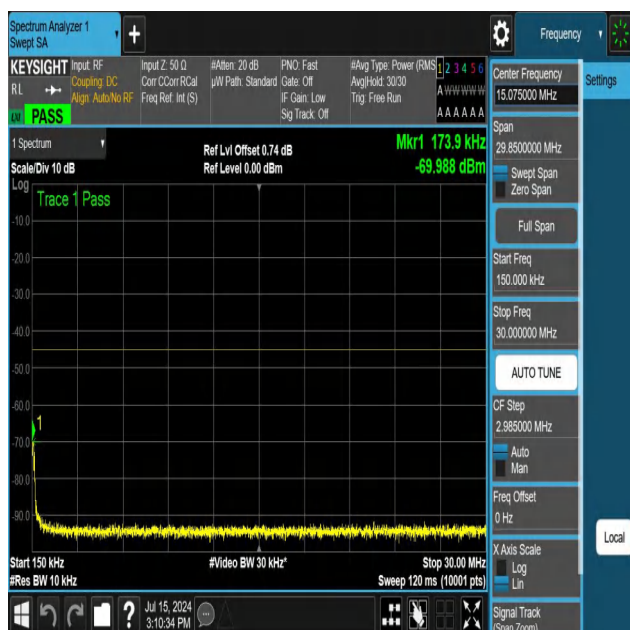
NTNV-N41-PC3-30-40-H-DFT-QPSK-Edge_1RB_Right-0.15-30-A nt1-PASS
