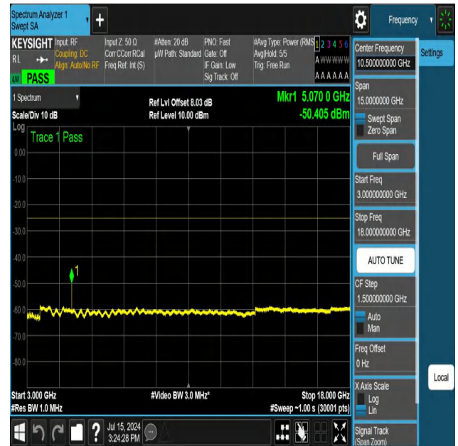
NTNV-N41-PC3-30-40-L-DFT-PI2BPSK-Edge_1RB_Right-3000-18000-Ant1-PASS
