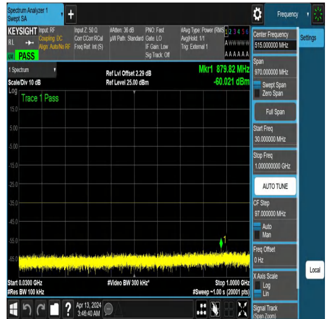
NTNV-N41-PC3-30-40-L-DFT-PI2BPSK-Edge_1RB_Right-30-1000-Ant1-PASS
