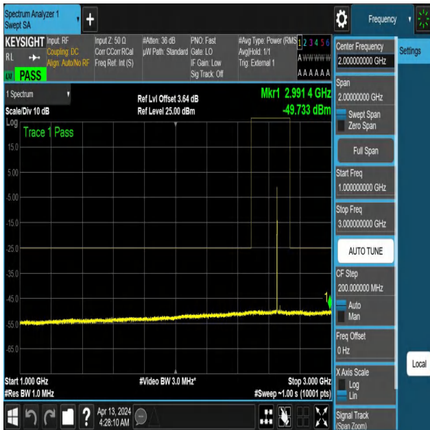
NTNV-N41-PC3-30-40-H-DFT-QPSK-Edge_1RB_Left-1000-3000- Ant1-PASS
