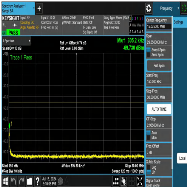
NTNV-N41-PC3-30-40-H-DFT-PI2BPSK-Edge_1RB_Right-0.15-3 0-Ant1-PASS
