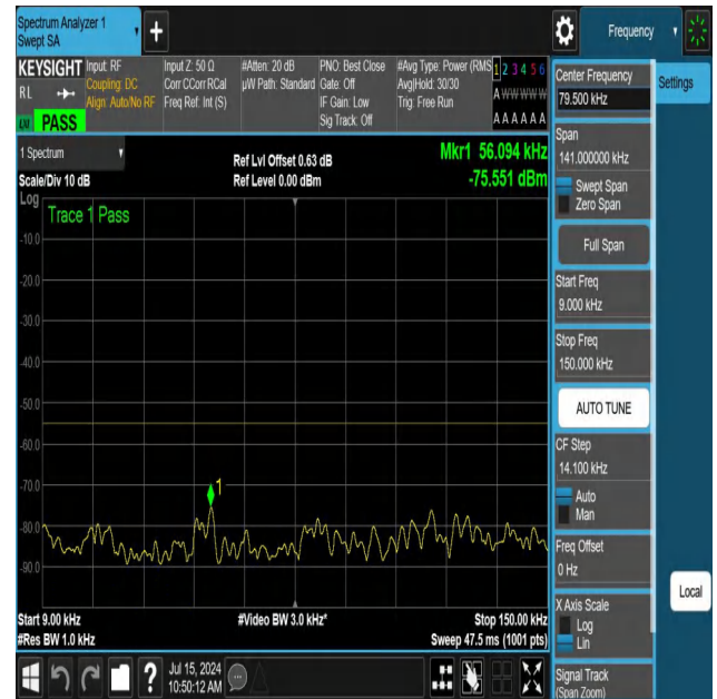
NTNV-N41-PC3-30-40-L-DFT-QPSK-Edge_1RB_Right-0.009-0.1 5-Ant1-PASS
