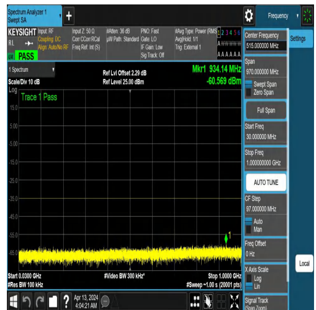
NTNV-N41-PC3-30-40-M-DFT-PI2BPSK-Edge_1RB_Right-30-10 00-Ant1-PASS
