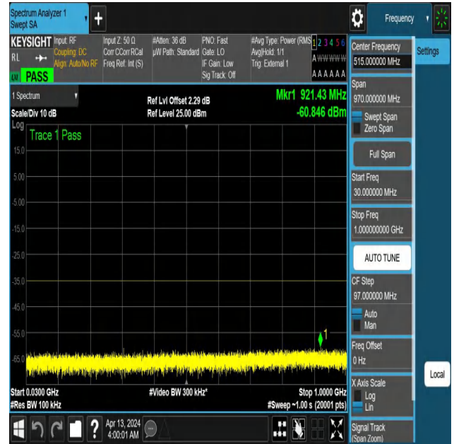
NTNV-N41-PC3-30-40-M-DFT-PI2BPSK-Edge_1RB_Left-30-100 0-Ant1-PASS
