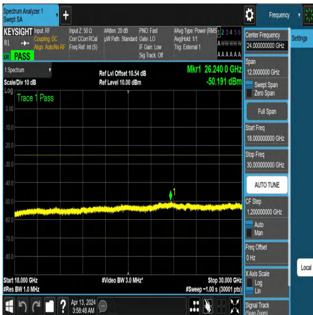
NTNV-N41-PC3-30-40-L-DFT-QPSK-Edge_1RB_Right-18000-300 00-Ant1-PASS
