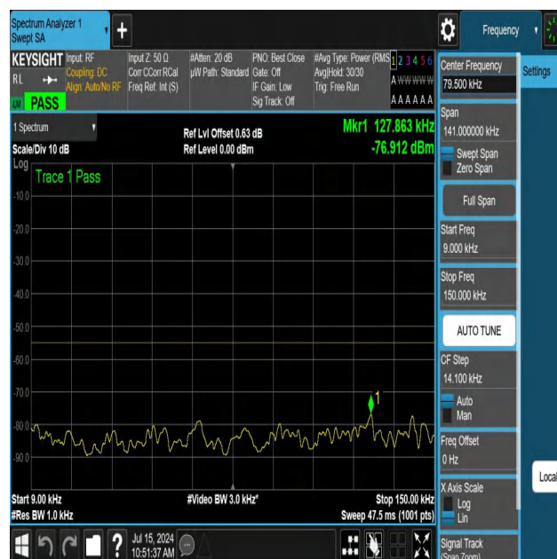
NTNV-N41-PC3-30-40-H-DFT-QPSK-Edge_1RB_Left-0.009-0.15 -Ant1-PASS
