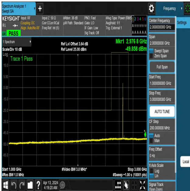
NTNV-N41-PC3-30-40-H-DFT-PI2BPSK-Edge_1RB_Left-1000-3000-Ant1-PASS
