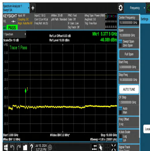
NTNV-N41-PC3-30-40-H-DFT-PI2BPSK-Edge_1RB_Right-3000-18000-Ant1-PASS
