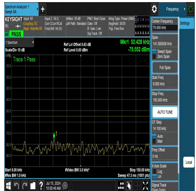
NTNV-N41-PC3-30-40-M-DFT-QPSK-Edge_1RB_Left-0.009-0.15 -Ant1-PASS
