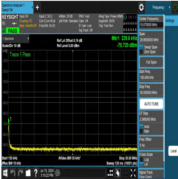
NTNV-N41-PC3-30-40-H-DFT-QPSK-Edge_1RB_Left-0.15-30-Ant 1-PASS
