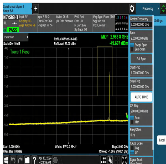
NTNV-N41-PC3-30-40-H-DFT-PI2BPSK-Edge_1RB_Right-1000-3 000-Ant1-PASS
