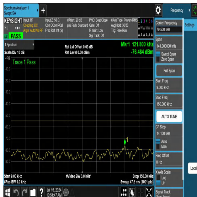
NTNV-N41-PC3-30-40-H-DFT-QPSK-Edge_1RB_Right-0.009-0.1 5-Ant1-PASS
