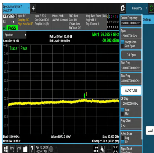
NTNV-N41-PC3-30-40-H-DFT-PI2BPSK-Edge_1RB_Right-18000-30000-Ant1-PASS
