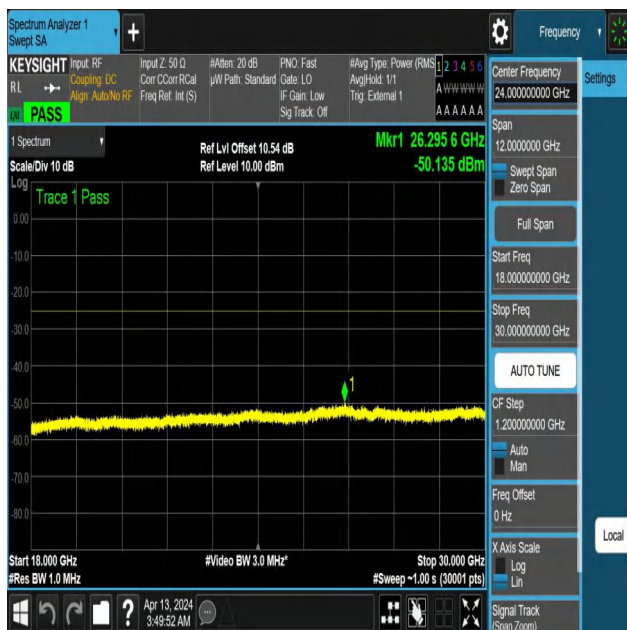
NTNV-N41-PC3-30-40-L-DFT-PI2BPSK-Edge_1RB_Right-18000-30000-Ant1-PASS
