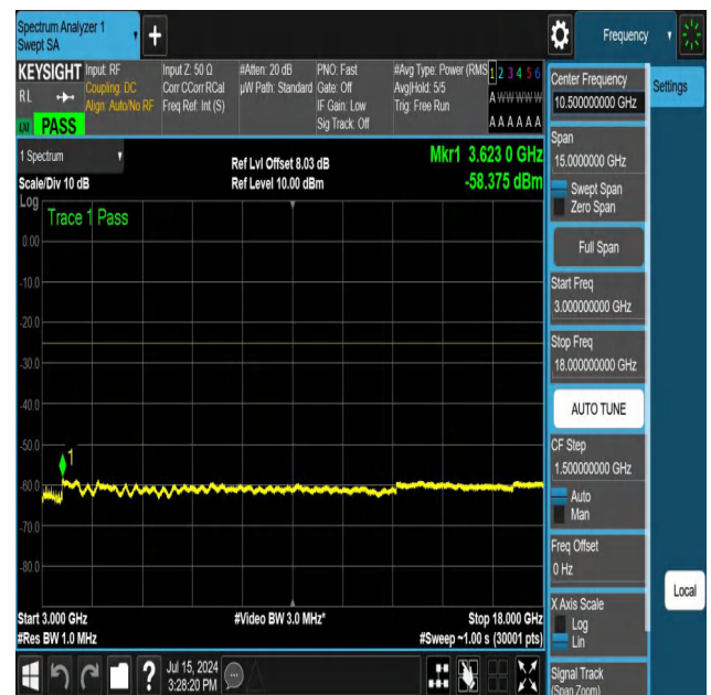
NTNV-N41-PC3-30-50-L-DFT-PI2BPSK-Edge_1RB_Left-3000-18000-Ant1-PASS
