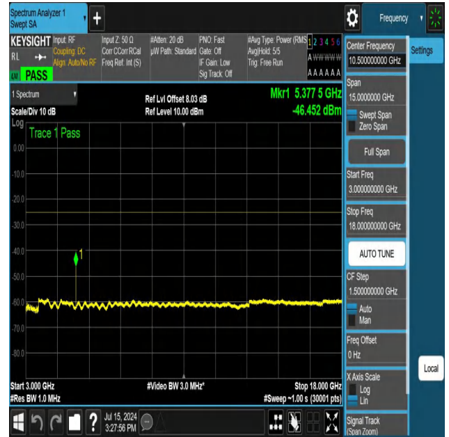
NTNV-N41-PC3-30-40-H-DFT-QPSK-Edge_1RB_Right-3000-180 00-Ant1-PASS
