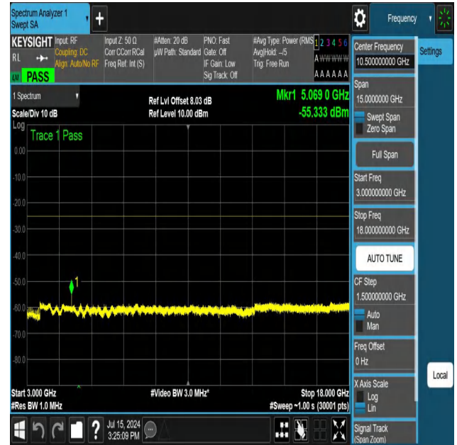
NTNV-N41-PC3-30-40-L-DFT-QPSK-Edge_1RB_Right-3000-180 00-Ant1-PASS
