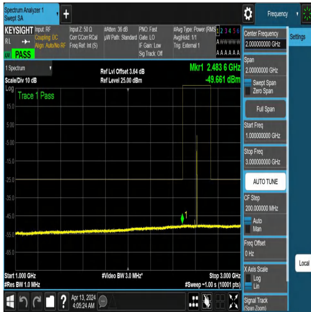
NTNV-N41-PC3-30-40-M-DFT-PI2BPSK-Edge_1RB_Right-1000-3 000-Ant1-PASS
