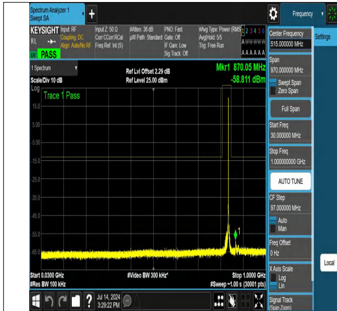
NTNV-N26-824-849-PC3-15-15-L-DFT-QPSK-Edge_1RB_Right-30-1000-Ant1-PASS
