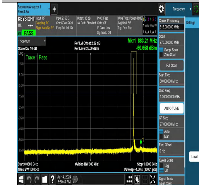
NTNV-N26-824-849-PC3-15-15-M-DFT-QPSK-Edge_1RB_Left-3 0-1000-Ant1-PASS
