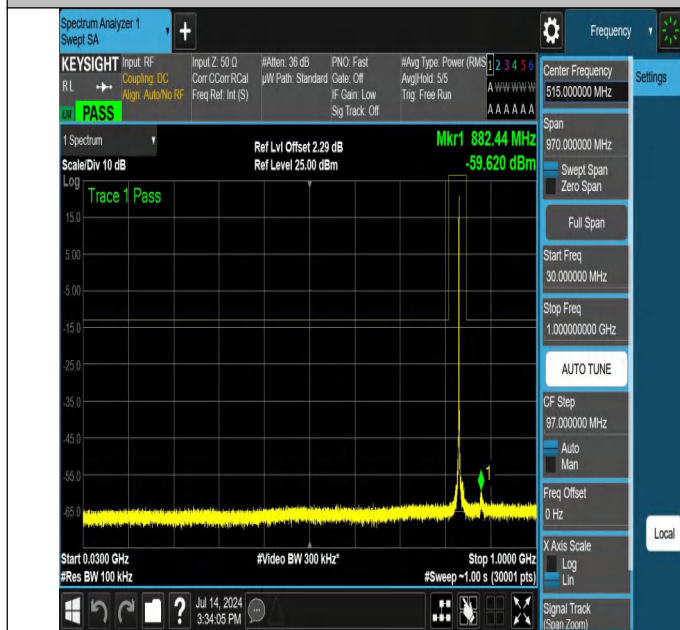
NTNV-N26-824-849-PC3-15-15-H-DFT-QPSK-Edge_1RB_Left-3
