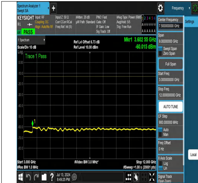
NTNV-N26-824-849-PC3-15-15-M-DFT-PI2BPSK-Edge_1RB_Lef t-3000-12000-Ant1-PASS
