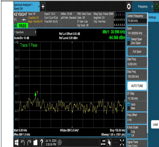
NTNV-N26-824-849-PC3-15-15-M-DFT-PI2BPSK-Edge_1RB_Rig ht-0.009-0.15-Ant1-PASS
