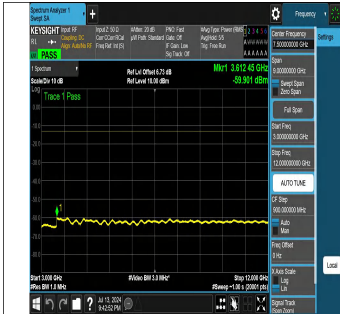
NTNV-N26-824-849-PC3-15-15-M-DFT-QPSK-Edge_1RB_Left-3 000-12000-Ant1-PASS
