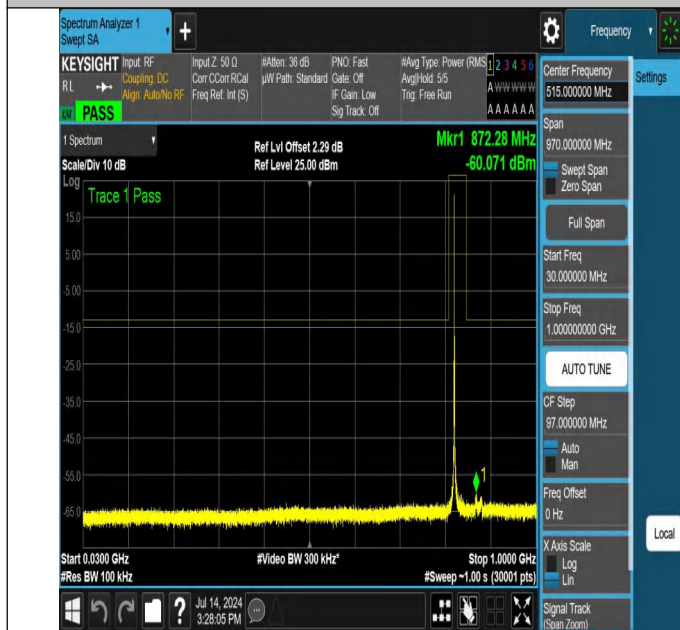
NTNV-N26-824-849-PC3-15-15-L-DFT-PI2BPSK-Edge_1RB_Left -30-1000-Ant1-PASS
