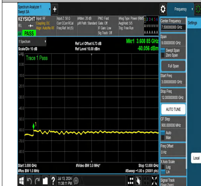
NTNV-N26-824-849-PC3-15-15-H-DFT-QPSK-Edge_1RB_Right-3000-12000-Ant1-PASS
