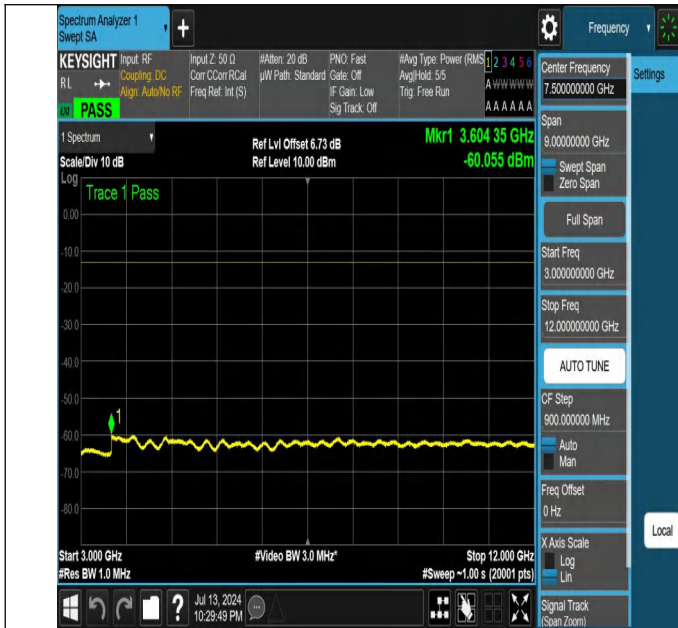
NTNV-N26-824-849-PC3-15-15-H-DFT-PI2BPSK-Edge_1RB_Lef t-3000-12000-Ant1-PASS
