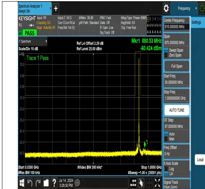
NTNV-N26-824-849-PC3-15-15-L-DFT-PI2BPSK-Edge_1RB_Rig ht-30-1000-Ant1-PASS
