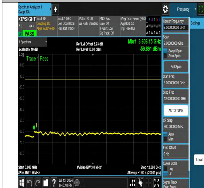
NTNV-N26-824-849-PC3-15-15-L-DFT-PI2BPSK-Edge_1RB_Rig ht-3000-12000-Ant1-PASS
