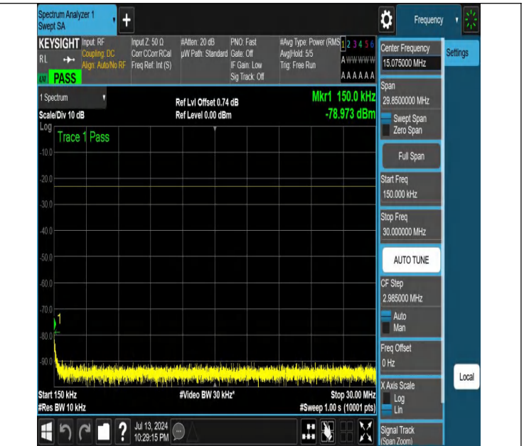
NTNV-N26-824-849-PC3-15-15-H-DFT-PI2BPSK-Edge_1RB_Left- 0.15-30-Ant1-PASS
