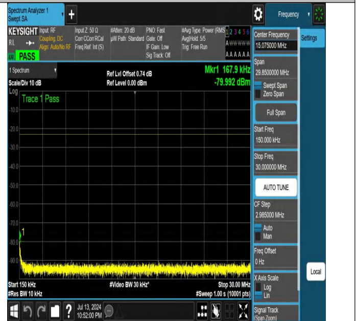
NTNV-N26-824-849-PC3-15-15-H-DFT-PI2BPSK-Edge_1RB_Rig ht-0.15-30-Ant1-PASS
