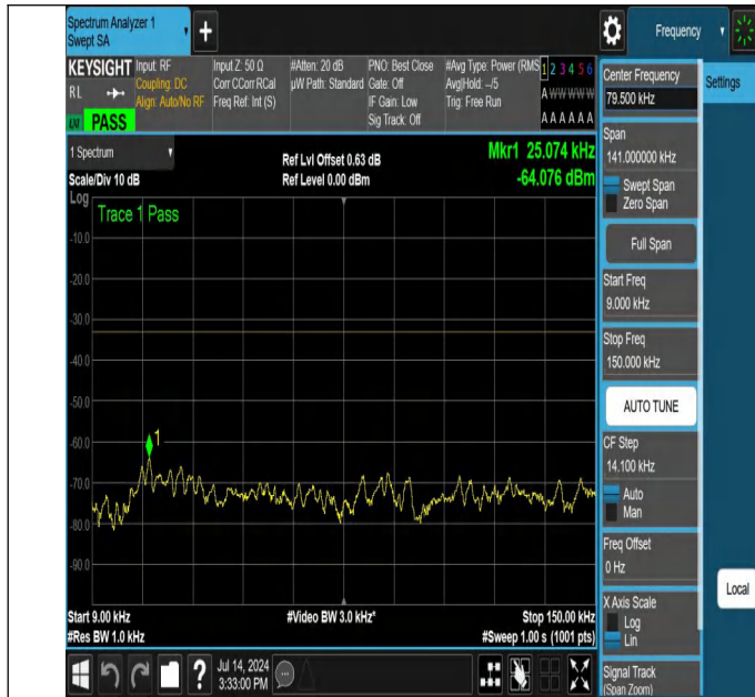
NTNV-N26-824-849-PC3-15-15-H-DFT-PI2BPSK-Edge_1RB_Lef t-0.009-0.15-Ant1-PASS
