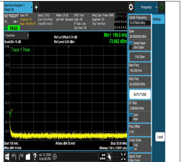
NTNV-N26-824-849-PC3-15-15-L-DFT-PI2BPSK-Edge_1RB_Left 0.15-30-Ant1-PASS
