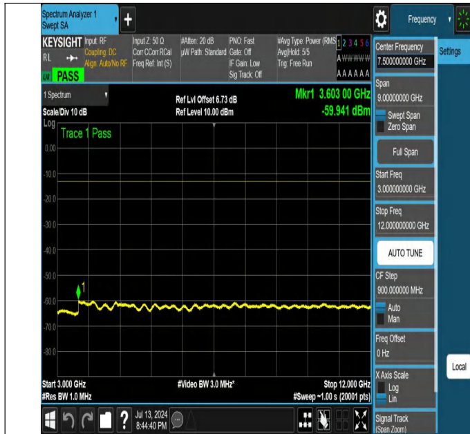
NTNV-N26-824-849-PC3-15-15-L-DFT-PI2BPSK-Edge_1RB_Left -3000-12000-Ant1-PASS
