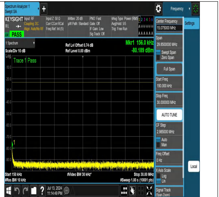
NTNV-N26-824-849-PC3-15-15-H-DFT-QPSK-Edge_1RB_Left-0.1
