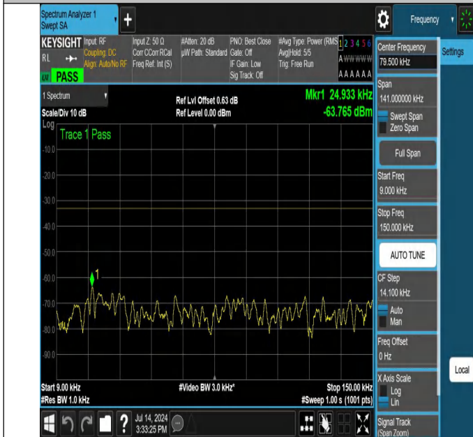
NTNV-N26-824-849-PC3-15-15-H-DFT-PI2BPSK-Edge_1RB_Rig ht-0.009-0.15-Ant1-PASS
