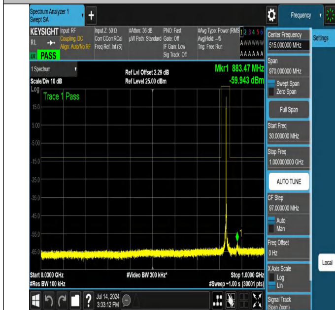
NTNV-N26-824-849-PC3-15-15-H-DFT-PI2BPSK-Edge_1RB_Lef t-30-1000-Ant1-PASS
