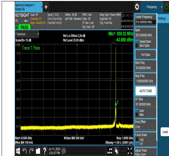
NTNV-N26-824-849-PC3-15-15-H-DFT-PI2BPSK-Edge_1RB_Rig ht-30-1000-Ant1-PASS
