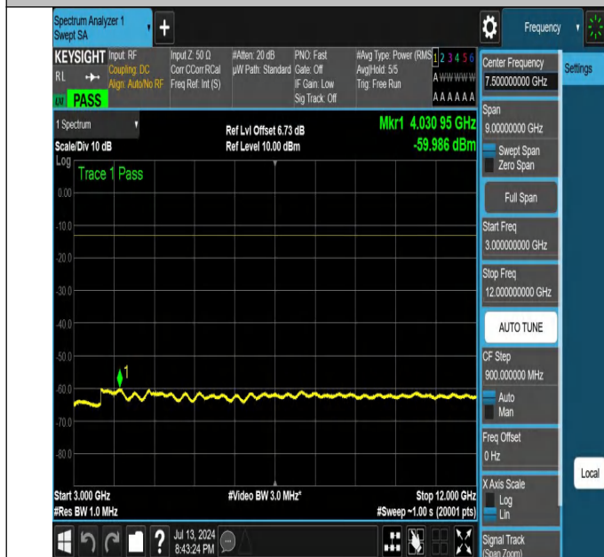
NTNV-N26-824-849-PC3-15-10-H-DFT-QPSK-Edge_1RB_Right-3000-12000-Ant1-PASS
