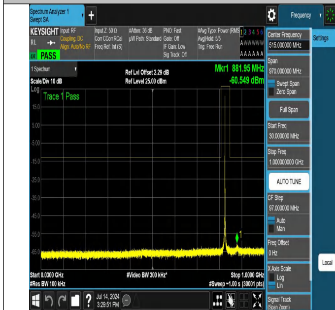
NTNV-N26-824-849-PC3-15-15-M-DFT-PI2BPSK-Edge_1RB_Lef t-30-1000-Ant1-PASS
