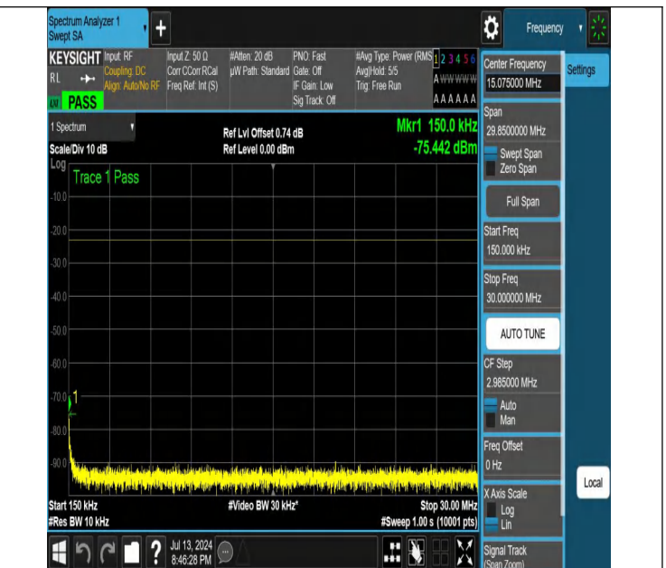
NTNV-N26-824-849-PC3-15-15-L-DFT-QPSK-Edge_1RB_Left-0.1 5-30-Ant1-PASS
