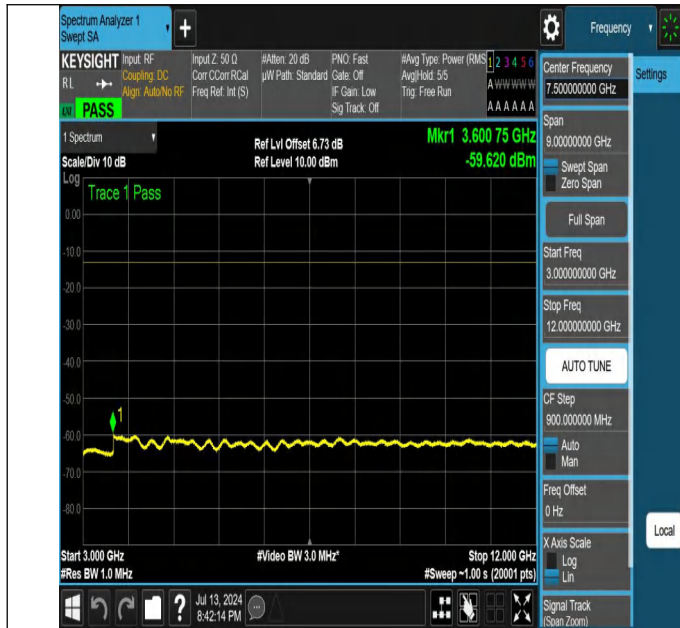
NTNV-N26-824-849-PC3-15-10-H-DFT-QPSK-Edge_1RB_Left-3 000-12000-Ant1-PASS
