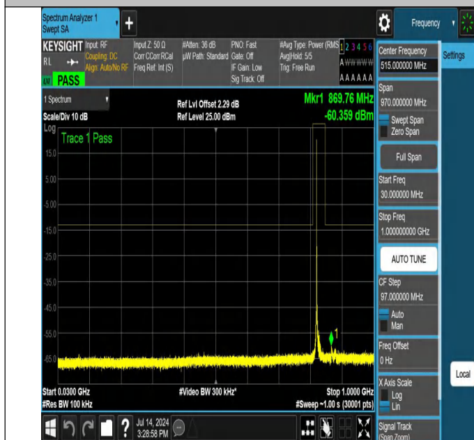
NTNV-N26-824-849-PC3-15-15-L-DFT-QPSK-Edge_1RB_Left-30 -1000-Ant1-PASS
