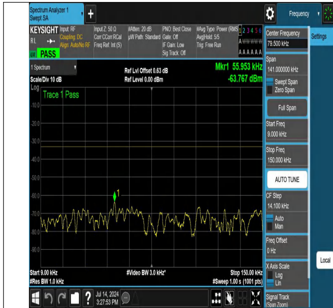
NTNV-N26-824-849-PC3-15-15-L-DFT-PI2BPSK-Edge_1RB_Left -0.009-0.15-Ant1-PASS
