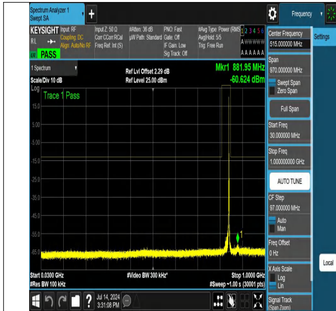
NTNV-N26-824-849-PC3-15-15-M-DFT-QPSK-Edge_1RB_Right-30-1000-Ant1-PASS
