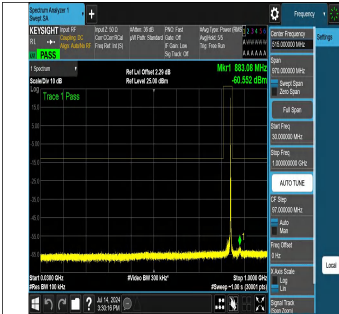
NTNV-N26-824-849-PC3-15-15-M-DFT-PI2BPSK-Edge_1RB_Rig ht-30-1000-Ant1-PASS
