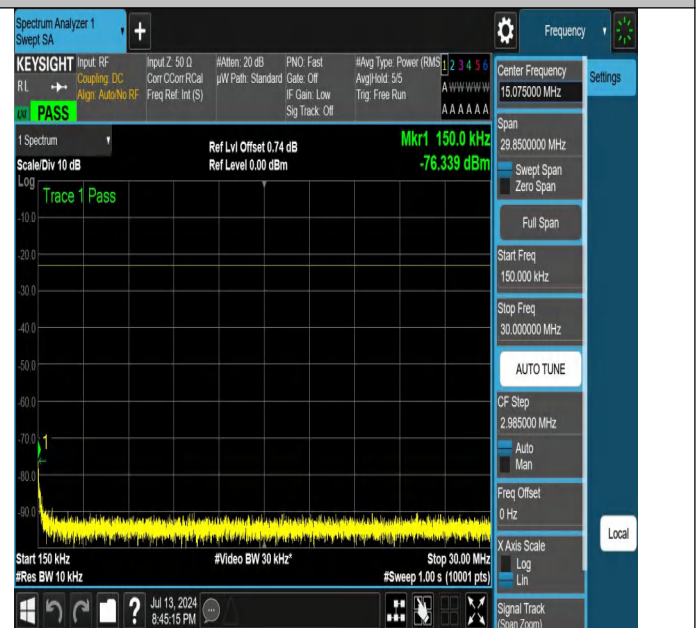
NTNV-N26-824-849-PC3-15-15-L-DFT-PI2BPSK-Edge_1RB_Righ t-0.15-30-Ant1-PASS
