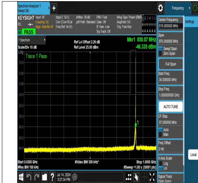
NTNV-N26-824-849-PC3-15-10-H-DFT-QPSK-Edge_1RB_Right-30-1000-Ant1-PASS
