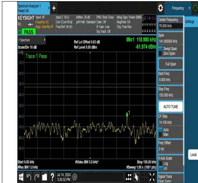
NTNV-N26-824-849-PC3-15-15-M-DFT-QPSK-Edge_1RB_Left-0. 009-0.15-Ant1-PASS
