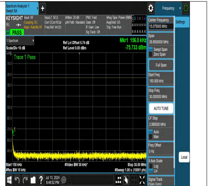
NTNV-N26-824-849-PC3-15-15-M-DFT-PI2BPSK-Edge_1RB_Left -0.15-30-Ant1-PASS
