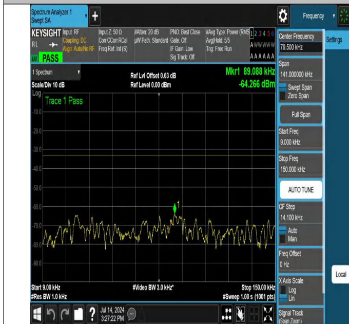
NTNV-N26-824-849-PC3-15-10-H-DFT-QPSK-Edge_1RB_Right- 0.009-0.15-Ant1-PASS
