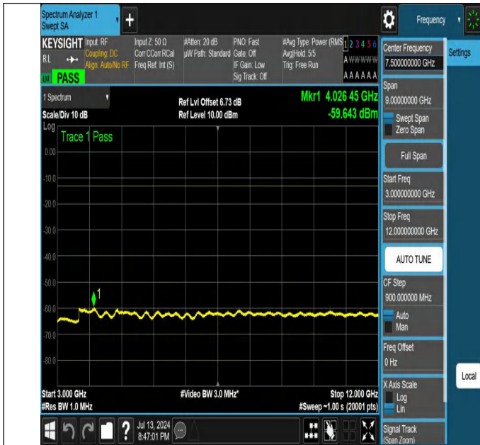
NTNV-N26-824-849-PC3-15-15-L-DFT-QPSK-Edge_1RB_Left-30 00-12000-Ant1-PASS
