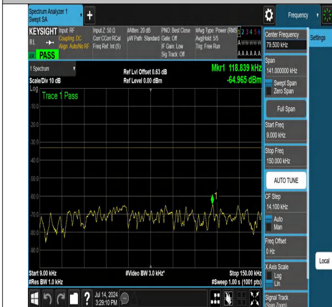
NTNV-N26-824-849-PC3-15-15-L-DFT-QPSK-Edge_1RB_Right- 0.009-0.15-Ant1-PASS
