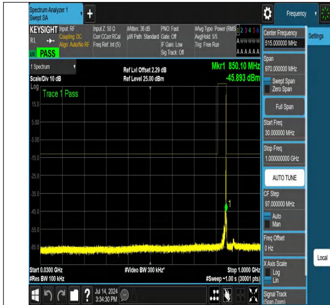
NTNV-N26-824-849-PC3-15-15-H-DFT-QPSK-Edge_1RB_Right-30-1000-Ant1-PASS
