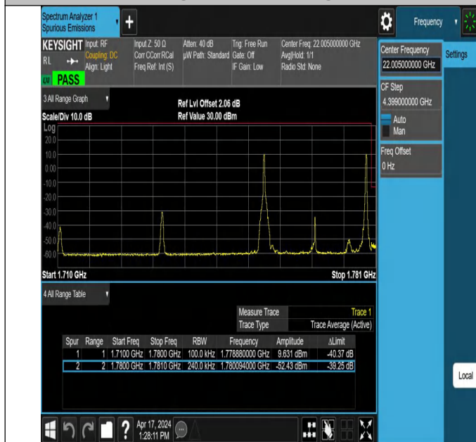
20MHz-5MHz_QPSK@QPSK-QPSK@QPSK_132522-132572_1 RB#0@100RB#0-1RB#24@25RB#0
