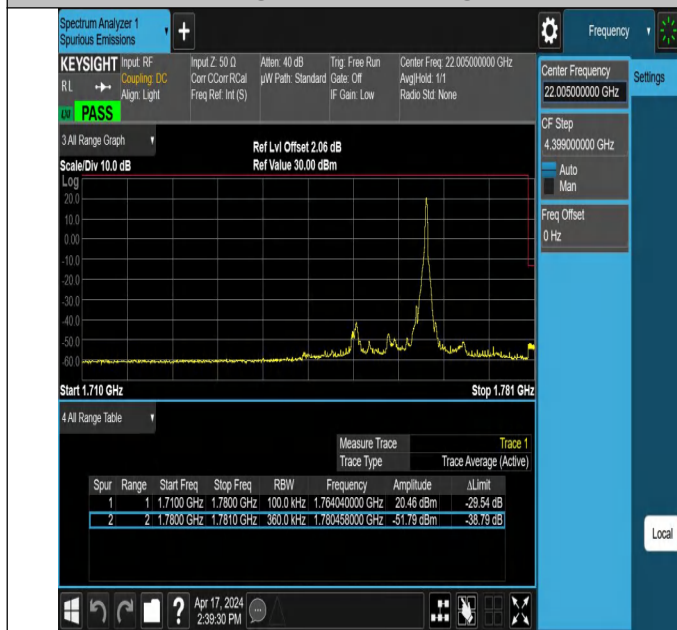
20MHz-15MHz_QPSK@QPSK-QPSK@QPSK_132423-132594_ 1RB#99@100RB#0-0RB#0@75RB#0
