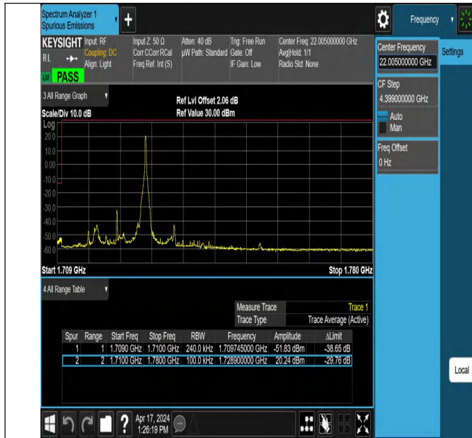
20MHz-5MHz_QPSK@QPSK-QPSK@QPSK_132072-132189_1 RB#99@100RB#0-0RB#0@25RB#0
