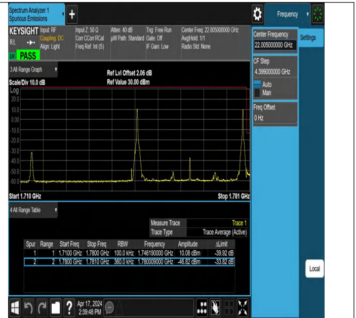
20MHz-15MHz_QPSK@QPSK-QPSK@QPSK_132423-132594_1 RB#0@100RB#0-1RB#74@75RB#0
