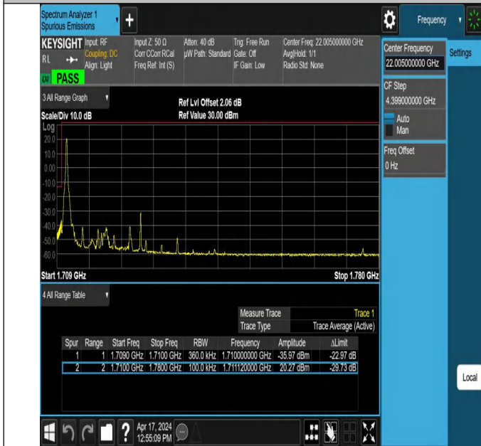
15MHz-20MHz_QPSK@QPSK-QPSK@QPSK_132050-132221_ 1RB#0@75RB#0-0RB#0@100RB#0
