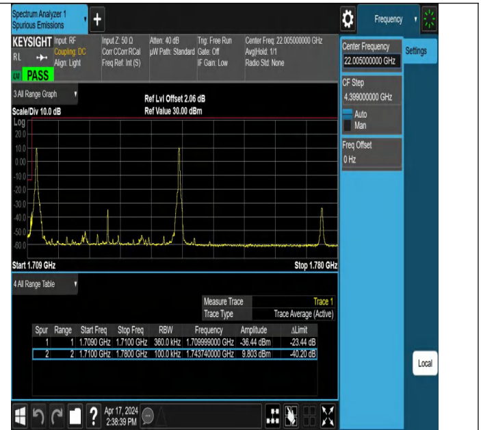
20MHz-15MHz_QPSK@QPSK-QPSK@QPSK_132072-132243_1RB#0@100RB#0-1RB#74@75RB#0
