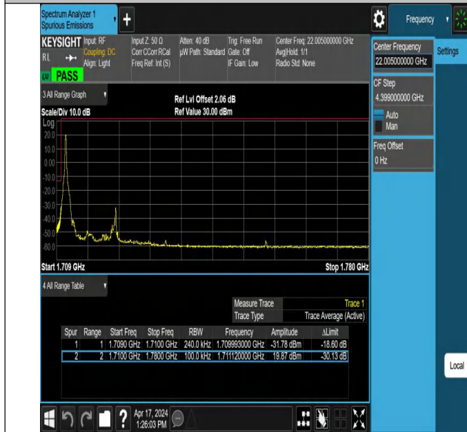
20MHz-5MHz_QPSK@QPSK-QPSK@QPSK_132072-132189_1 RB#0@100RB#0-0RB#0@25RB#0
