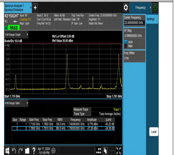
15MHz-20MHz_QPSK@QPSK-QPSK@QPSK_132401-132572_1RB#0@75RB#0-1RB#99@100RB#0
