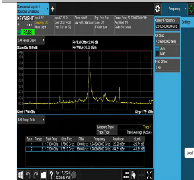
15MHz-20MHz_QPSK@QPSK-QPSK@QPSK_132401-132572_1RB#0@75RB#0-0RB#0@100RB#0
