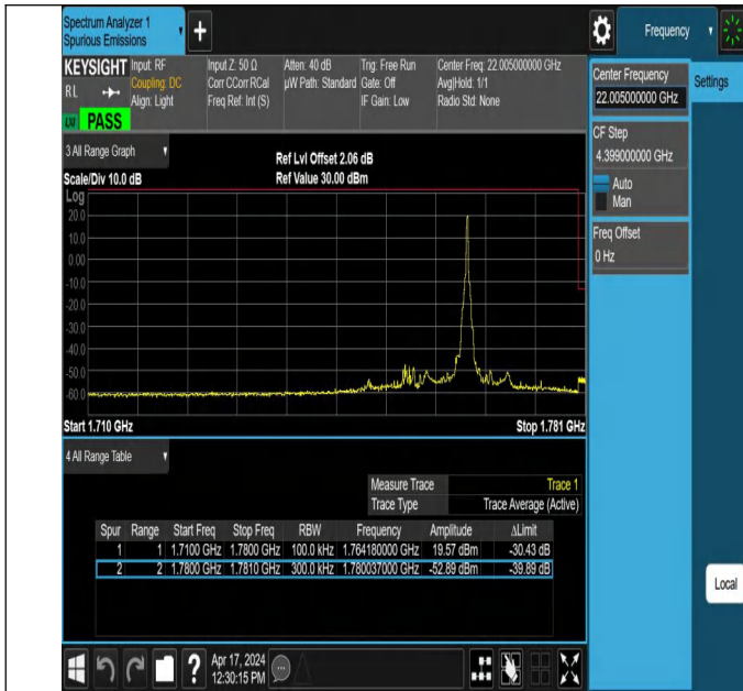
15MHz-15MHz_16QAM@16QAM-16QAM@16QAM_132447-13 2597_1RB#74@75RB#0-0RB#0@75RB#0
