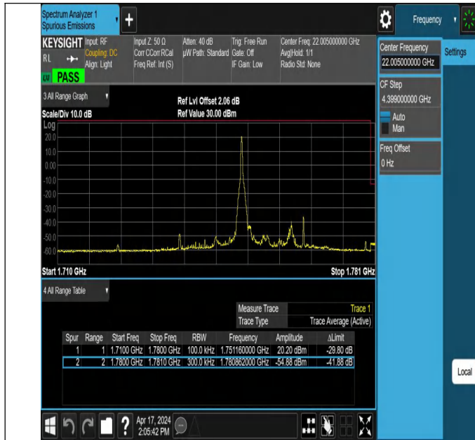
20MHz-10MHz_QPSK@QPSK-QPSK@QPSK_132473-132617_1RB#0@100RB#0-0RB#0@50RB#0
