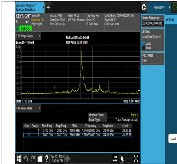
20MHz-15MHz_QPSK@QPSK-QPSK@QPSK_132423-132594_ 1RB#0@100RB#0-0RB#0@75RB#0
