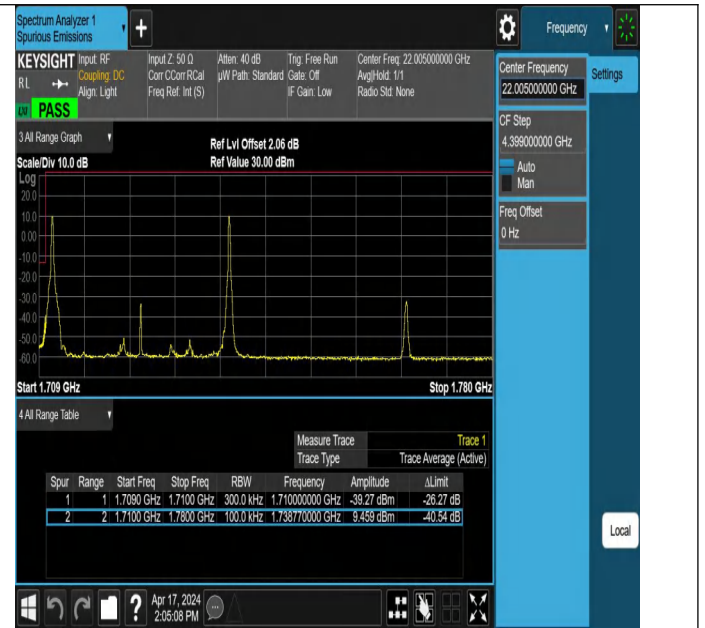
20MHz-10MHz_QPSK@QPSK-QPSK@QPSK_132072-132216_1 RB#0@100RB#0-1RB#49@50RB#0
