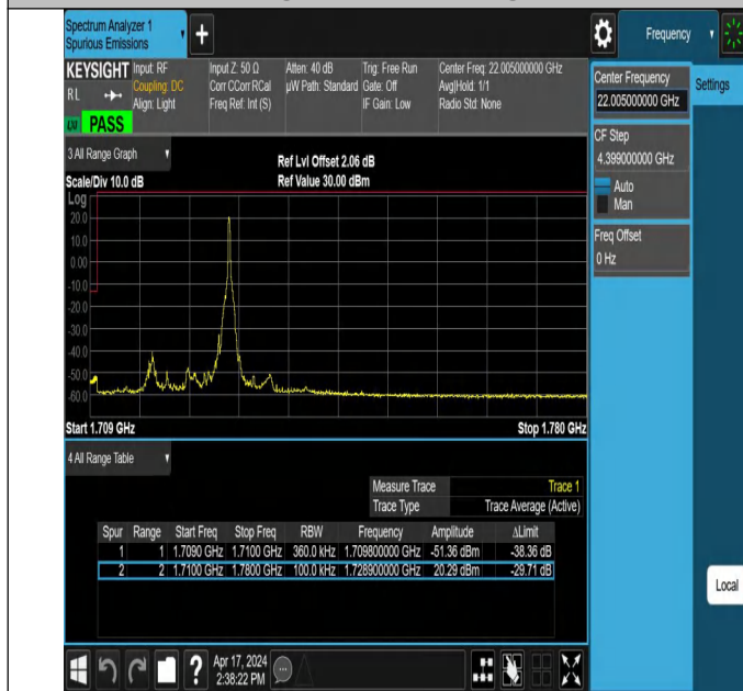
20MHz-15MHz_QPSK@QPSK-QPSK@QPSK_132072-132243_1RB#99@100RB#0-0RB#0@75RB#0
