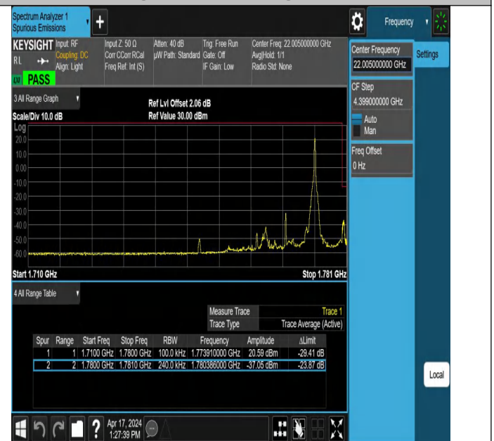
20MHz-5MHz_QPSK@QPSK-QPSK@QPSK_132522-132572_1R B#99@100RB#0-0RB#0@25RB#0
