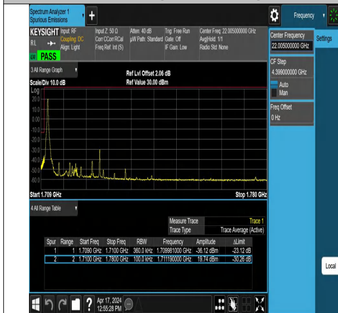
15MHz-20MHz_16QAM@16QAM-16QAM@16QAM_132050-13 2221_1RB#0@75RB#0-0RB#0@100RB#0
