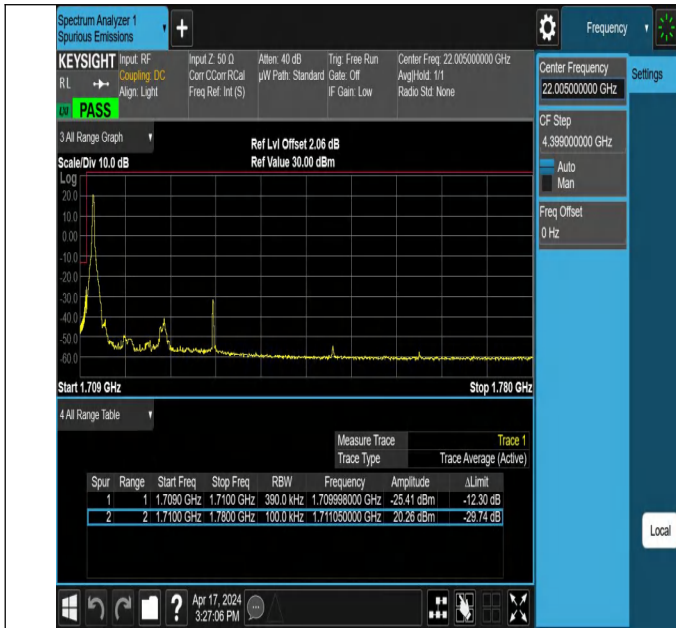
20MHz-20MHz_QPSK@QPSK-QPSK@QPSK_132072-132270_1RB#0@100RB#0-0RB#0@100RB#0
