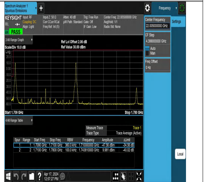
15MHz-20MHz_QPSK@QPSK-QPSK@QPSK_132050-132221_ 1RB#0@75RB#0-1RB#99@100RB#0
