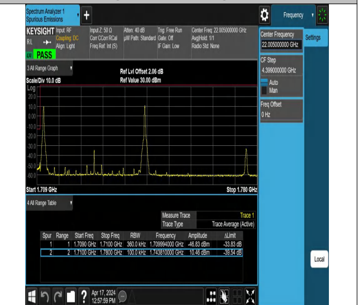
15MHz-20MHz_64QAM@64QAM-64QAM@64QAM_132050-132221_1RB#0@75RB#0-1RB#99@100RB#0
