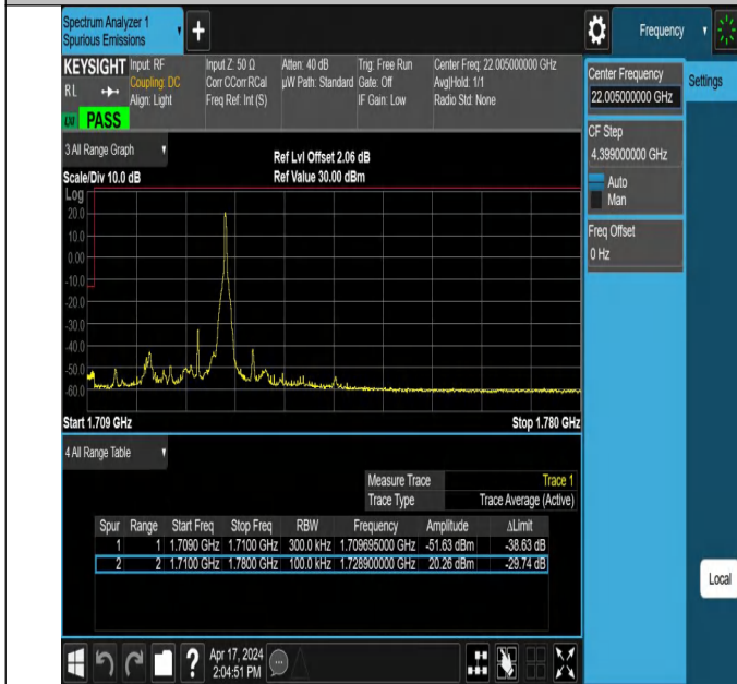
20MHz-10MHz_QPSK@QPSK-QPSK@QPSK_132072-132216_1 1RB#99@100RB#0-0RB#0@50RB#0
