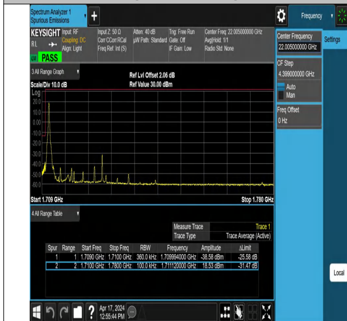
15MHz-20MHz_64QAM@64QAM-64QAM@64QAM_132050-132221_1RB#0@75RB#0-0RB#0@100RB#0
