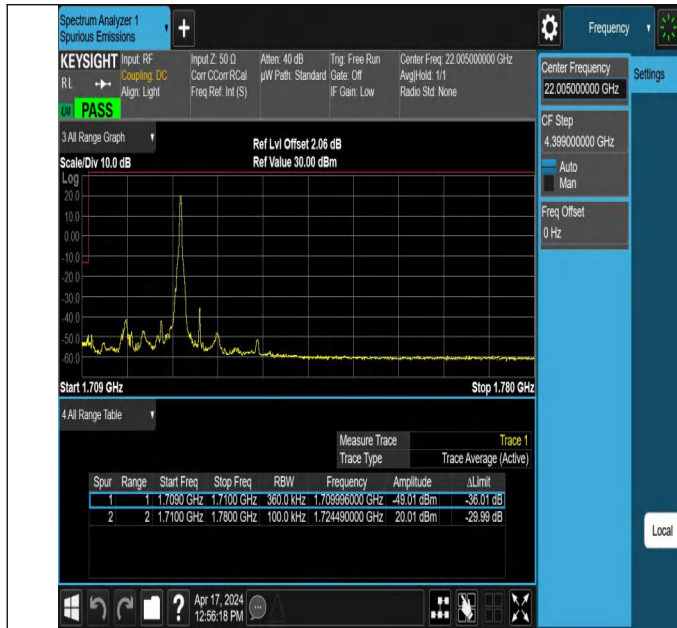
15MHz-20MHz_QPSK@QPSK-QPSK@QPSK_132050-132221_1RB#74@75RB#0-0RB#0@100RB#0
