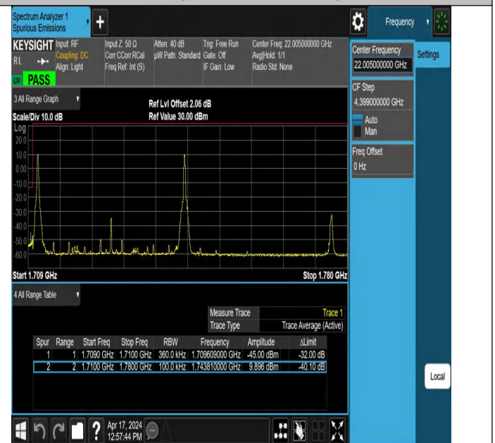
15MHz-20MHz_16QAM@16QAM-16QAM@16QAM_132050-1322 21_1RB#0@75RB#0-1RB#99@100RB#0
