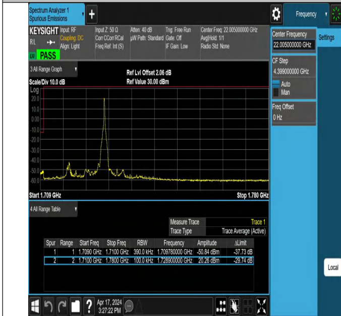
20MHz-20MHz_QPSK@QPSK-QPSK@QPSK_132072-132270_1RB#99@100RB#0-0RB#0@100RB#0
