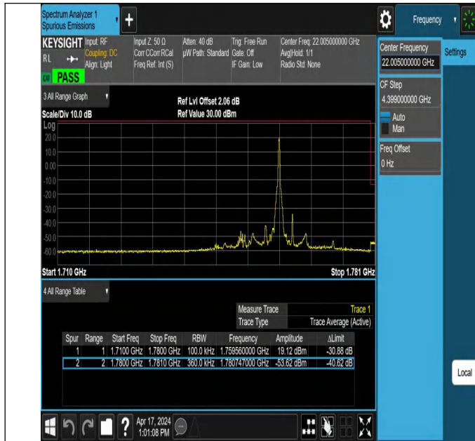
15MHz-20MHz_16QAM@16QAM-16QAM@16QAM_132401-13 2572_1RB#74@75RB#0-0RB#0@100RB#0
