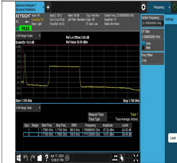
15MHz-20MHz_256QAM@256QAM-256QAM@256QAM_13205 0-132221_1RB#0@75RB#0-0RB#0@100RB#0
