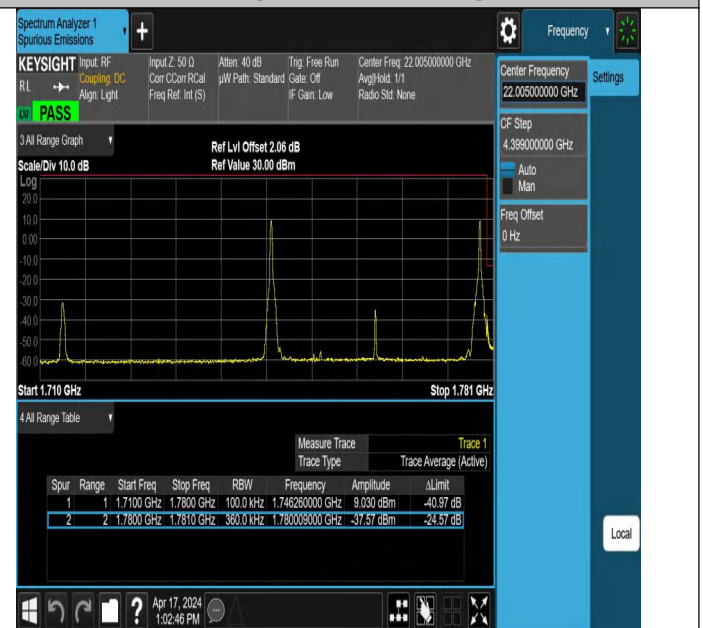
15MHz-20MHz_256QAM@256QAM-256QAM@256QAM_132401- 132572_1RB#0@75RB#0-1RB#99@100RB#0
