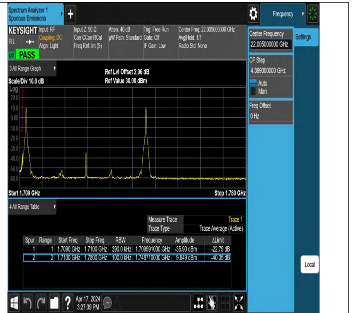
20MHz-20MHz_QPSK@QPSK-QPSK@QPSK_132072-132270_1RB#0@100RB#0-1RB#99@100RB#0
