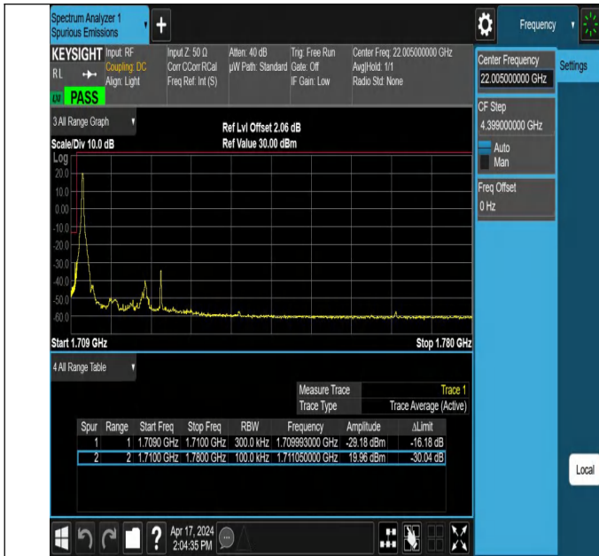
20MHz-10MHz_QPSK@QPSK-QPSK@QPSK_132072-132216_1 1RB#0@100RB#0-0RB#0@50RB#0
