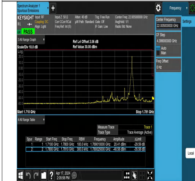
20MHz-10MHz_QPSK@QPSK-QPSK@QPSK_132473-132617_1RB#99@100RB#0-0RB#0@50RB#0
