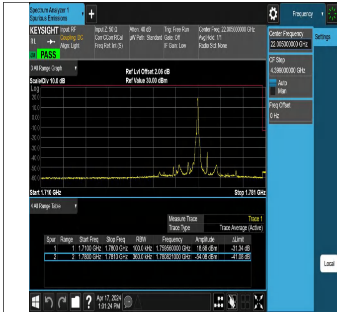
15MHz-20MHz_64QAM@64QAM-64QAM@64QAM_132401-13 2572_1RB#74@75RB#0-0RB#0@100RB#0
