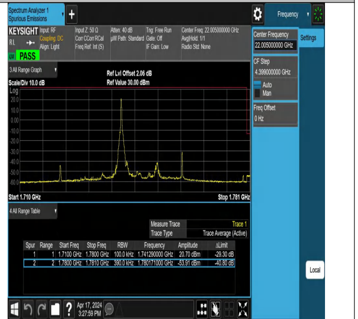
20MHz-20MHz_QPSK@QPSK-QPSK@QPSK_132374-132572_1RB#0@100RB#0-0RB#0@100RB#0
