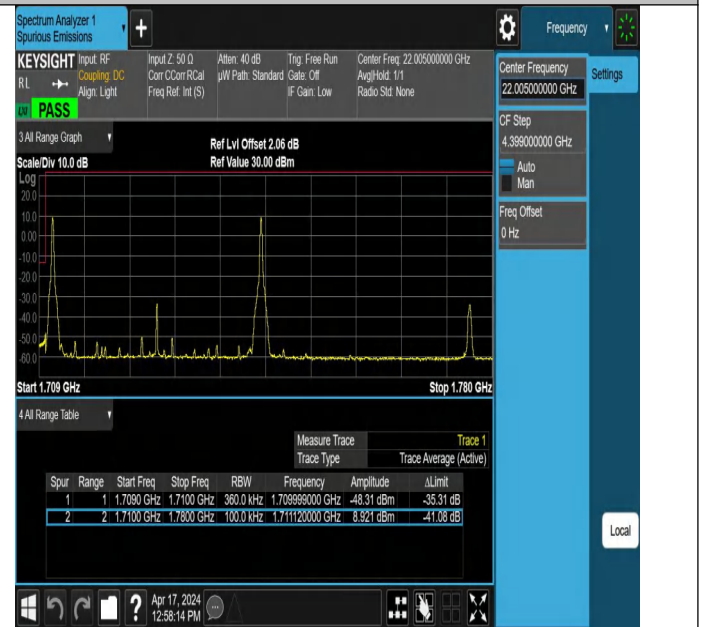
15MHz-20MHz_256QAM@256QAM-256QAM@256QAM_132050- 132221_1RB#0@75RB#0-1RB#99@100RB#0
