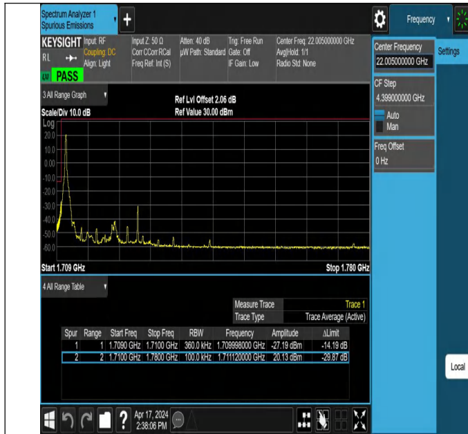
20MHz-15MHz_QPSK@QPSK-QPSK@QPSK_132072-132243_1RB#0@100RB#0-0RB#0@75RB#0
