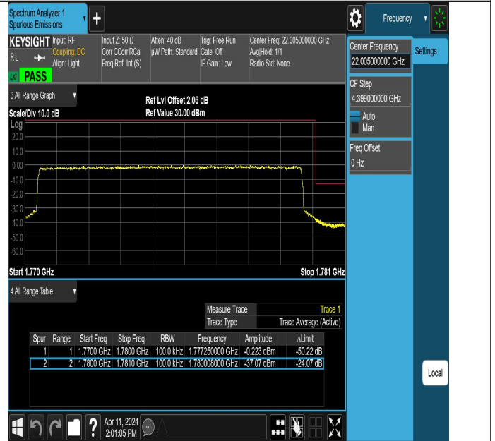
Band66_10MHz_QPSK_132622_50RB#0
