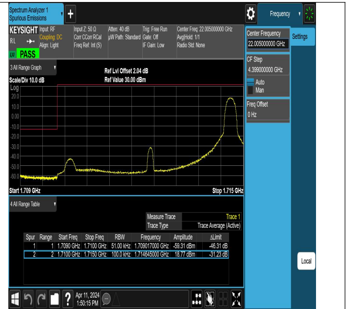
Band66_5MHz_QPSK_131997_1RB#24
