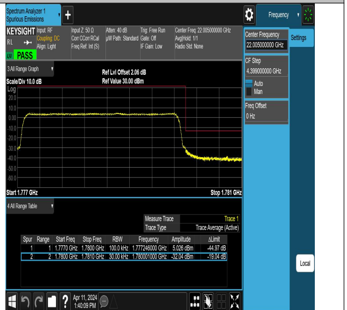
Band66_3MHz_QPSK_132657_15RB#0
