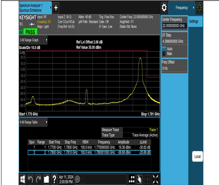
Band66_10MHz_QPSK_132622_1RB#49
