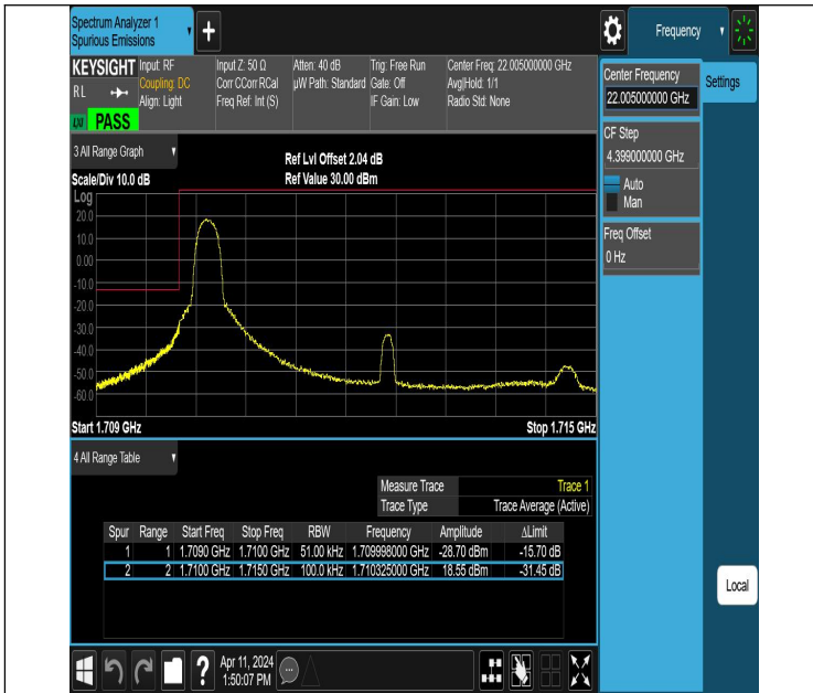
Band66_5MHz_QPSK_131997_1RB#0
