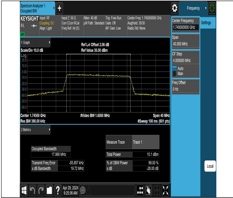
Band66-20MHz-QPSK-132322-100RB#0-PASS
