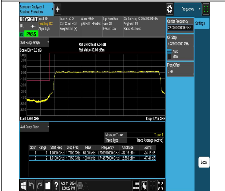
Band66_5MHz_QPSK_131997_25RB#0
