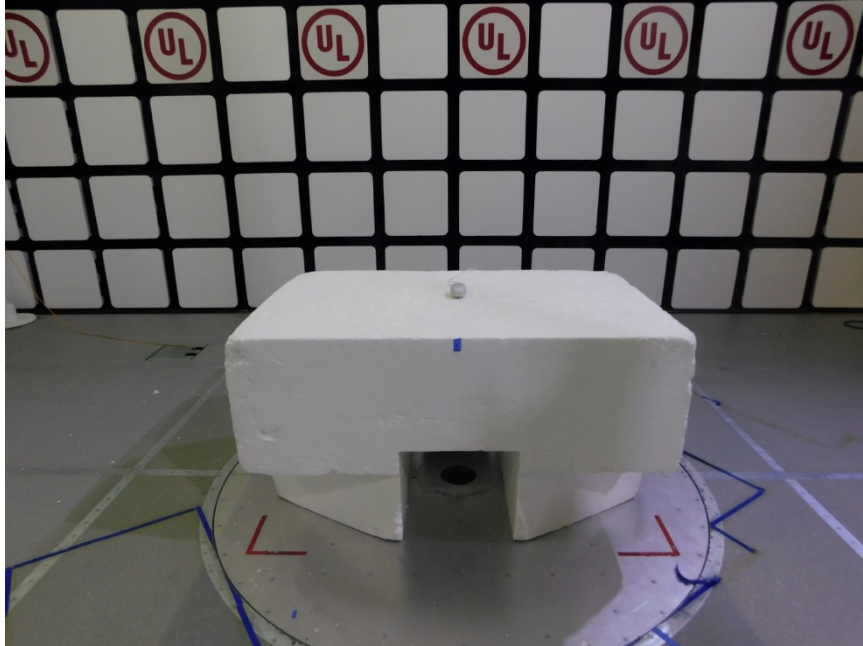
RADIATED EMISSIONS S-Chamber Photos (<30MHz)
