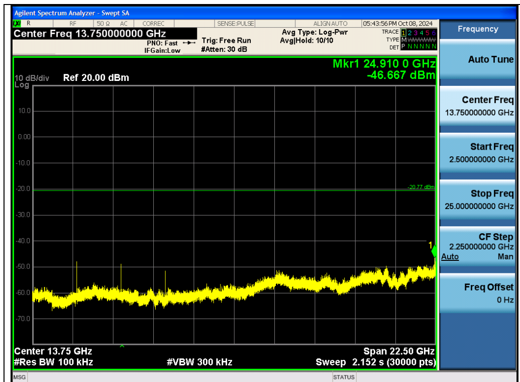
Test_Graph_2.4G_ANT1_2480_Higher Band Emissions
