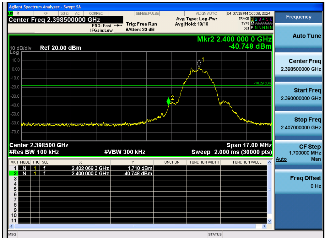
Test_Graph_2.4G_ANT2_2402_Lower Band Edge Emissions
