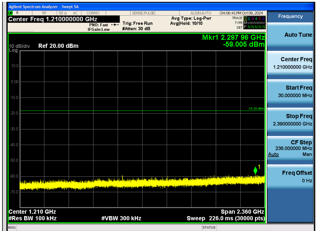
Test_Graph_2.4G_ANT2_2402_Lower Band Emissions
