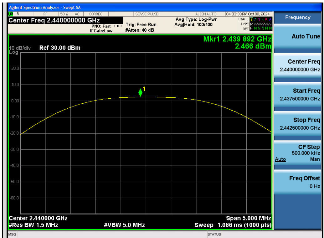
Test_Graph_2.4G_ANT2_2440_Peak Power
