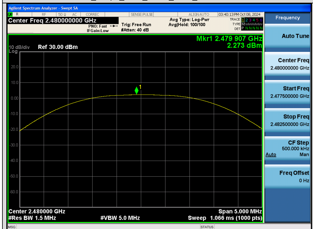
Test_Graph_2.4G_ANT2_2480_Peak Power
