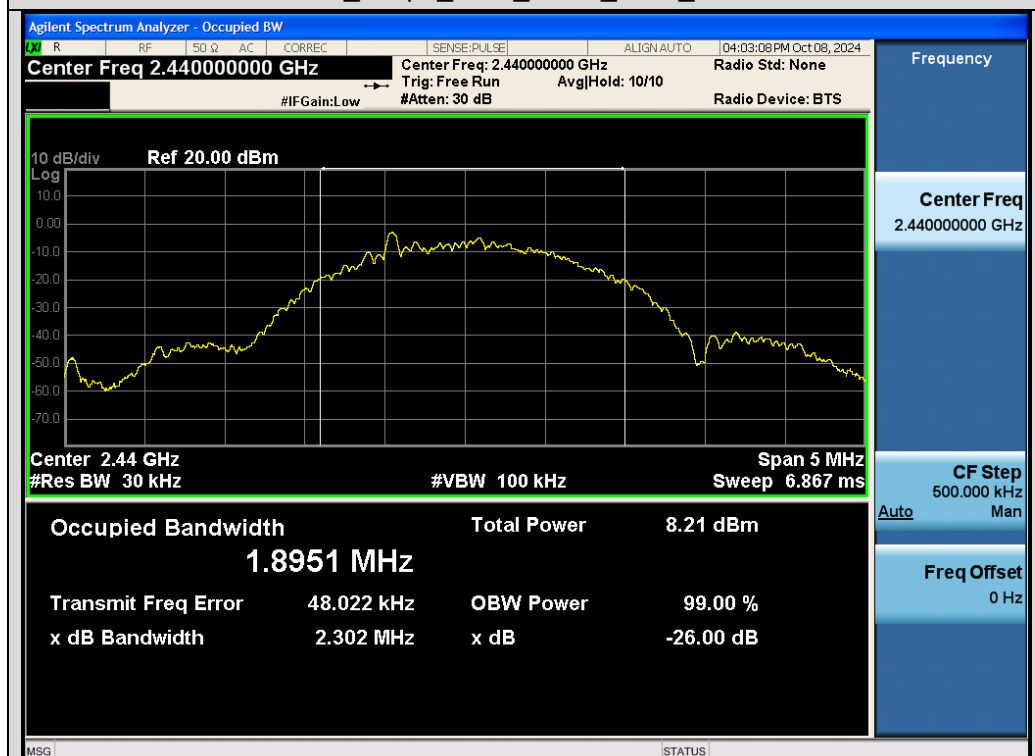
Test_Graph_2.4G_ANT2_2440_OBW
