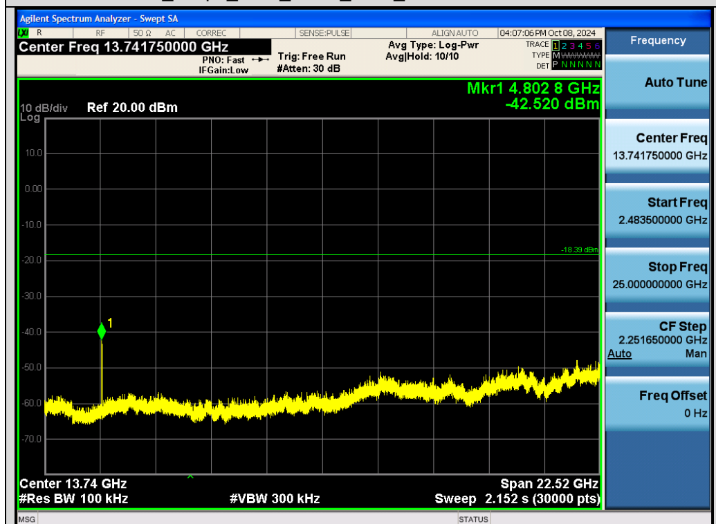
Test_Graph_2.4G_ANT2_2402_Higher Band Emissions
