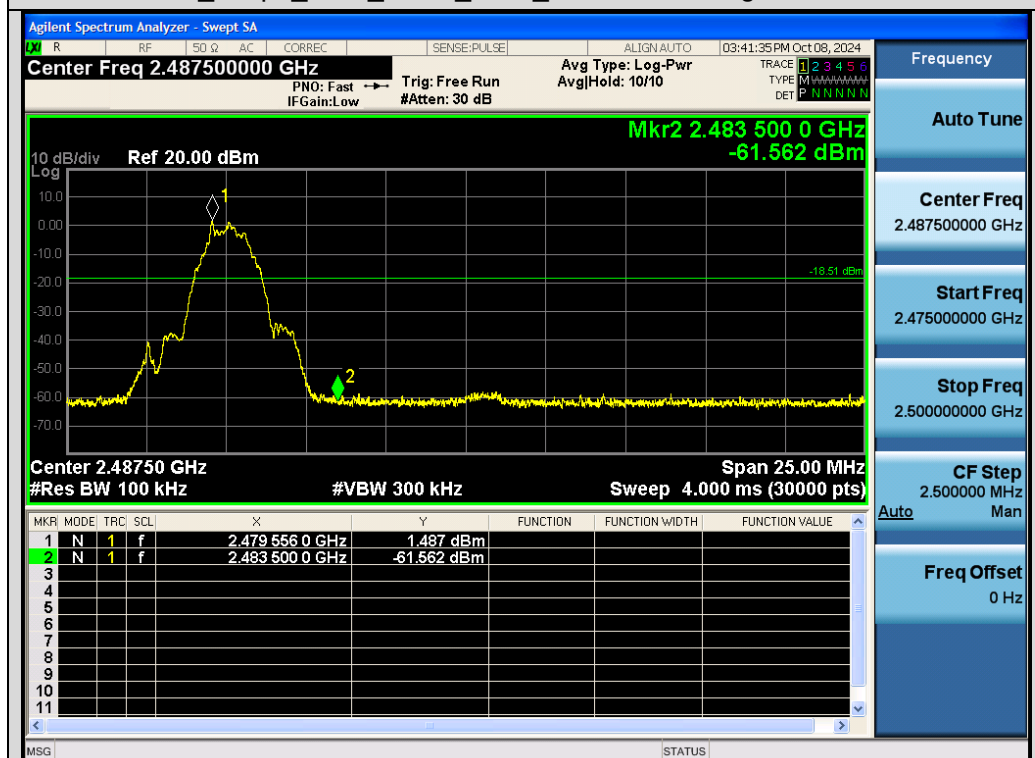
Test_Graph_2.4G_ANT2_2480_Higher Band Edge Emissions
