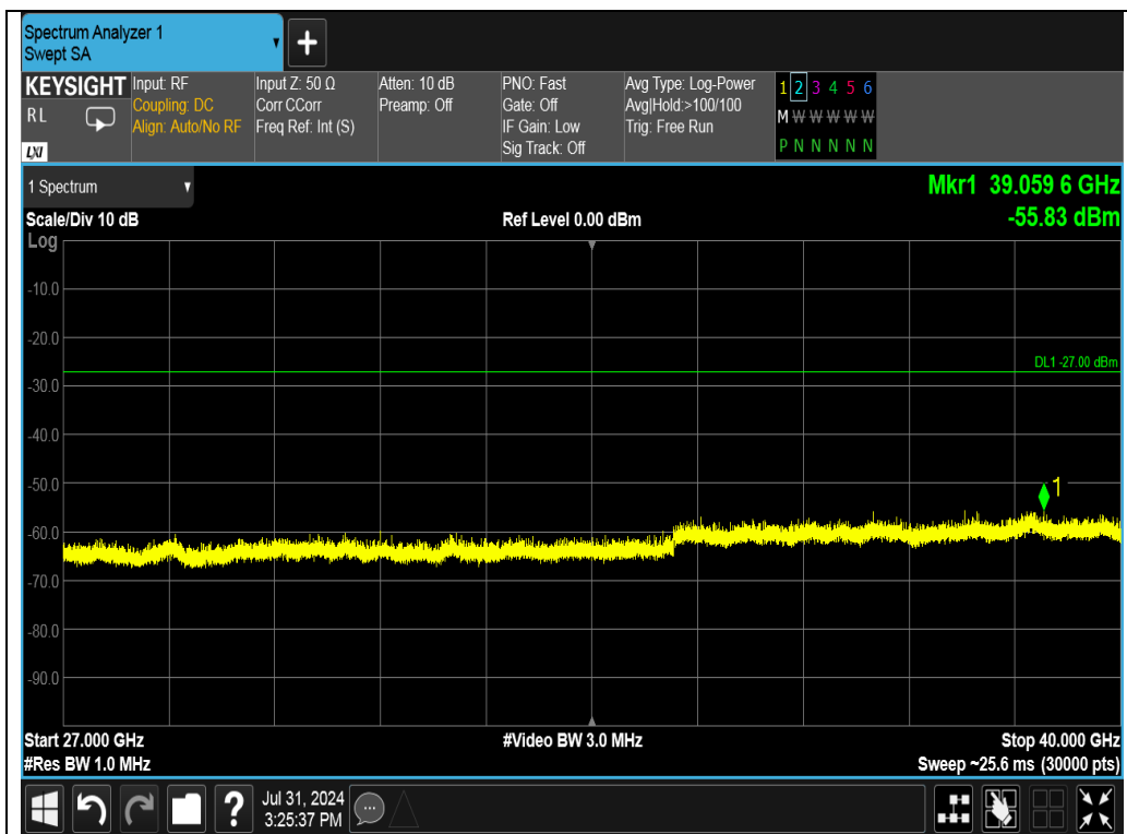
Test_Graph_802.11ac80_Chain B_5210_MCS0_Frequency Band 5
