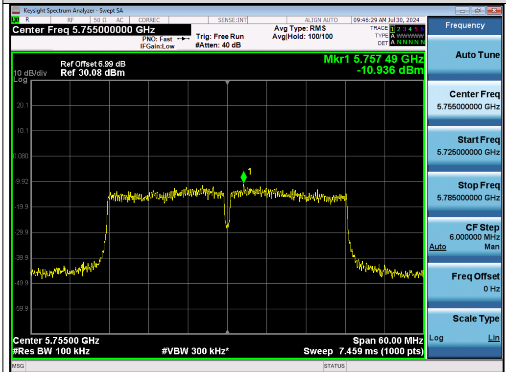
Test_Graph_802.11ac40_Chain B_5755_MCS0_PSD
