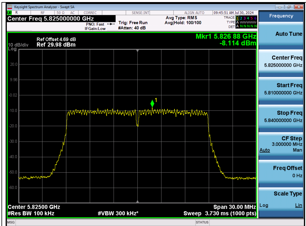
Test_Graph_802.11ac20_Chain B_5825_MCS0_PSD
