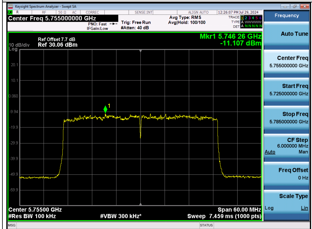
Test_Graph_802.11ax40_Chain A_5755_MCS0_PSD
