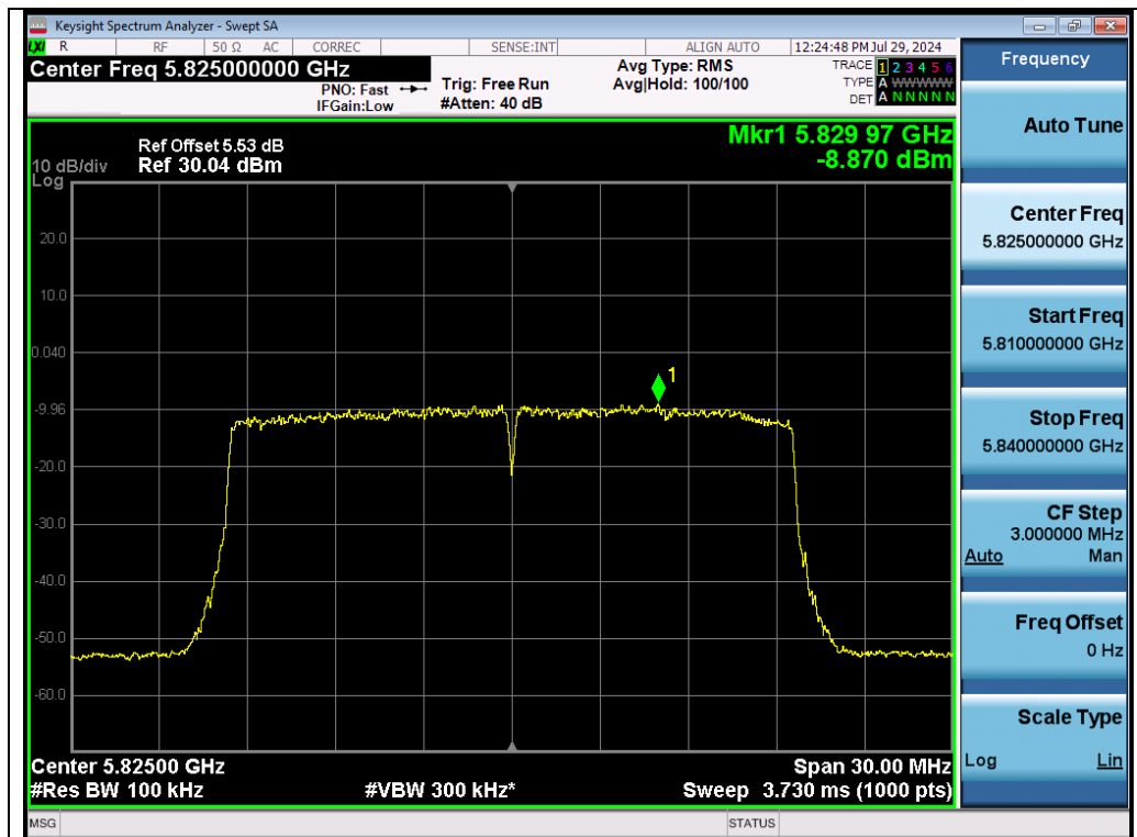
Test_Graph_802.11ax20_Chain A_5825_MCS0_PSD
