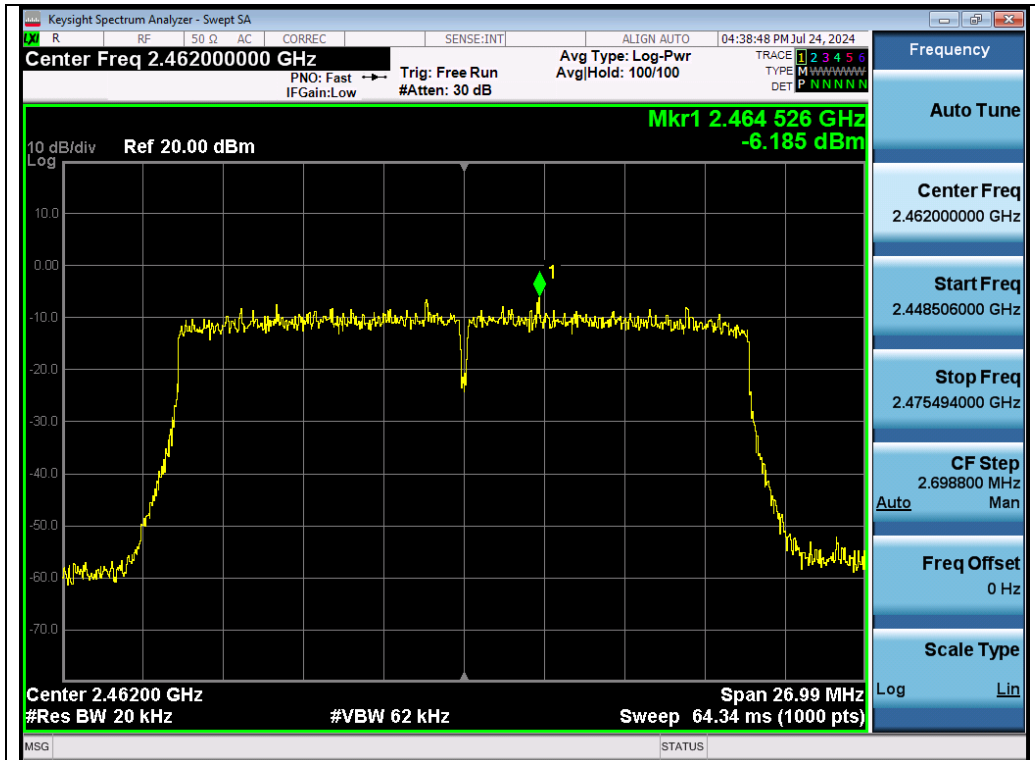
Test_Graph_802.11ax20_Chain B_2462_MCS0_PSD
