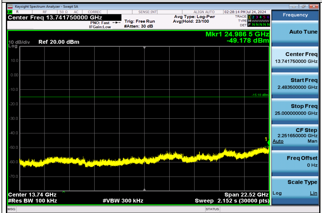
Test_Graph_802.11b_Chain A_2412_1Mbps_Higher Band Emissions
