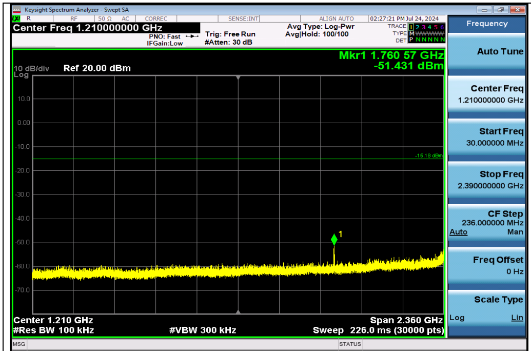
Test_Graph_802.11b_Chain A_2412_1Mbps_Lower Band Emissions
