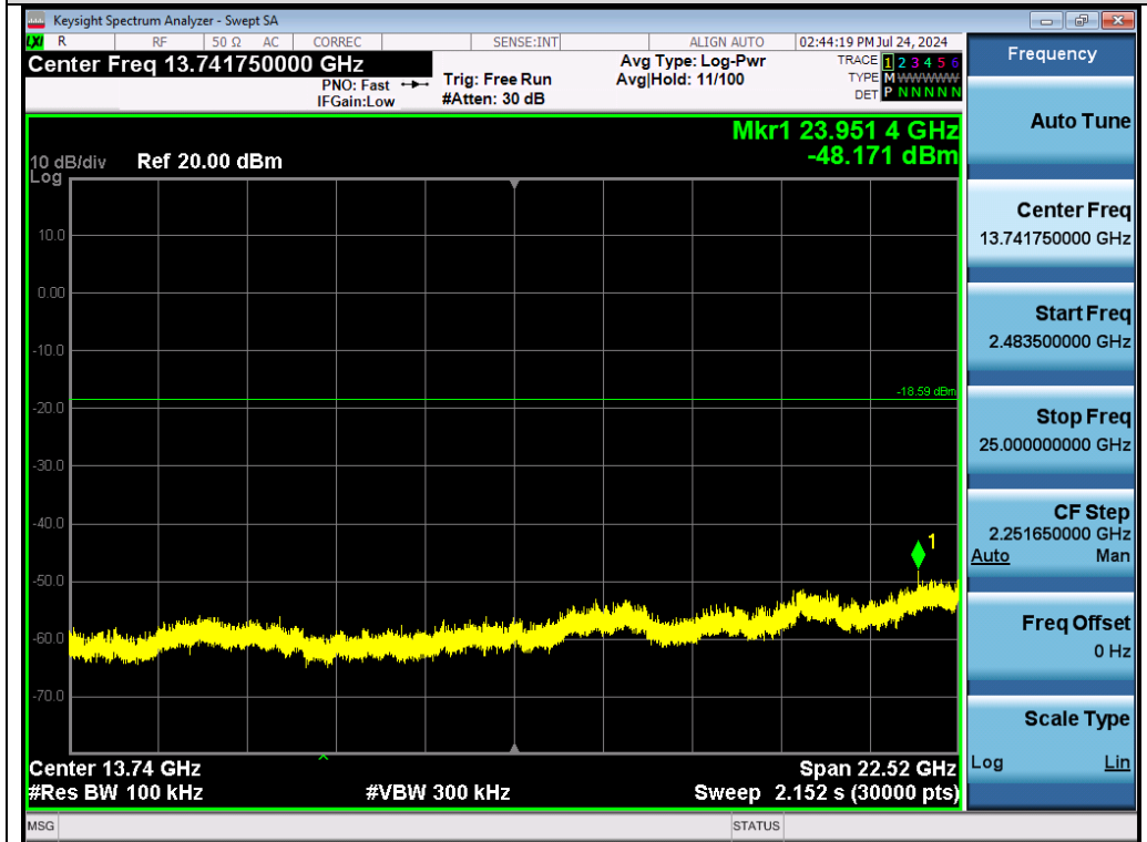
Test_Graph_802.11g_Chain A_2437_6Mbps_Higher Band Emissions
