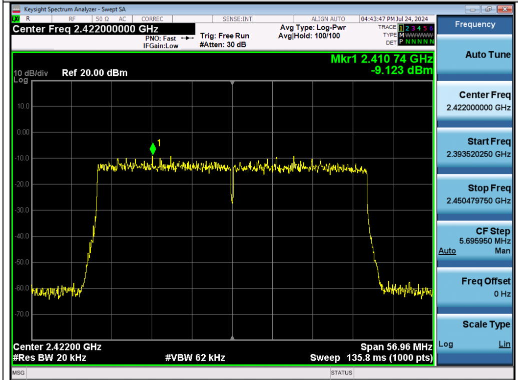
Test_Graph_802.11ax40_Chain B_2422_MCS0_PSD
