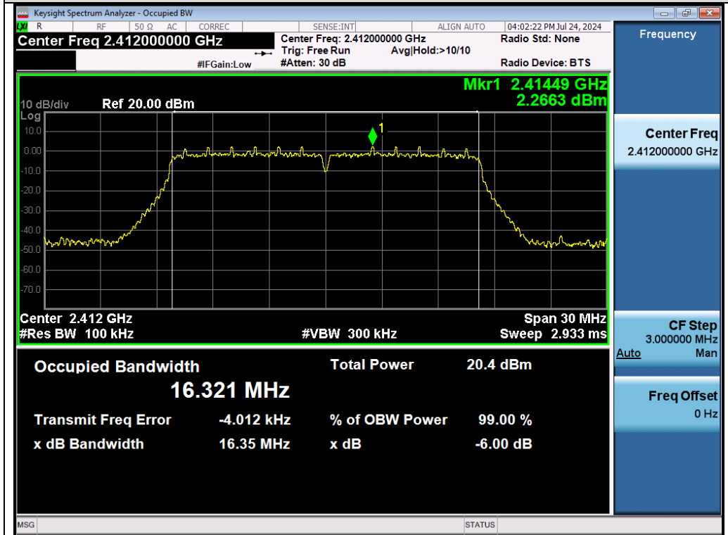
Test_Graph_802.11g_Chain B_2412_6Mbps_DTSSBW
