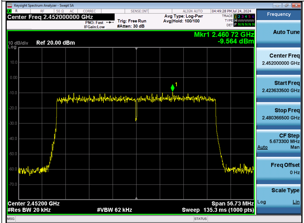
Test_Graph_802.11ax40_Chain B_2452_MCS0_PSD
