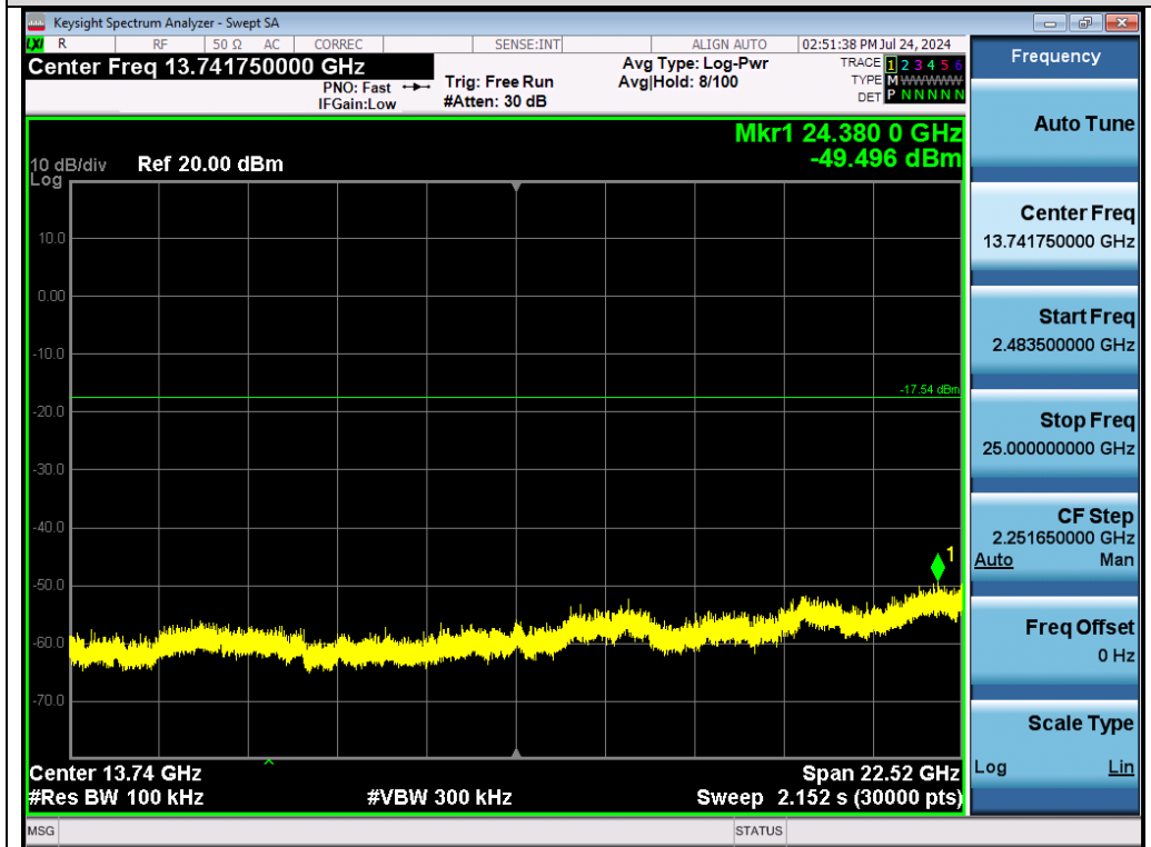
Test_Graph_802.11n20_Chain A_2412_MCS0_Higher Band Emissions
