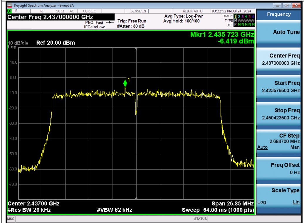
Test_Graph_802.11ax20_Chain A_2437_MCS0_PSD
