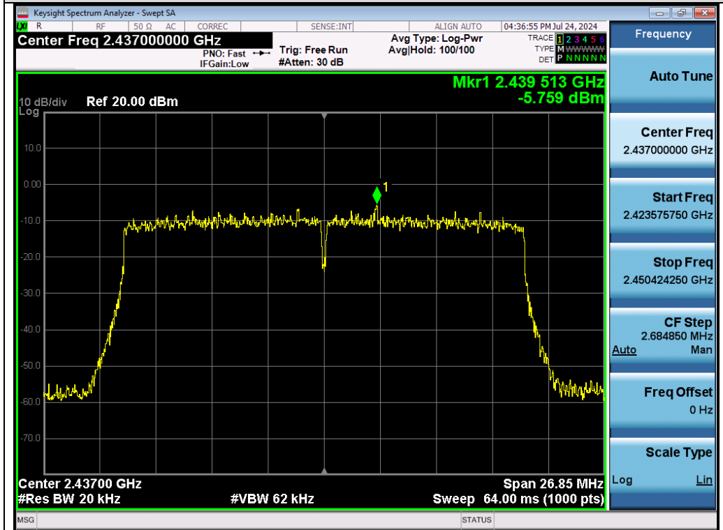
Test_Graph_802.11ax20_Chain B_2437_MCS0_PSD
