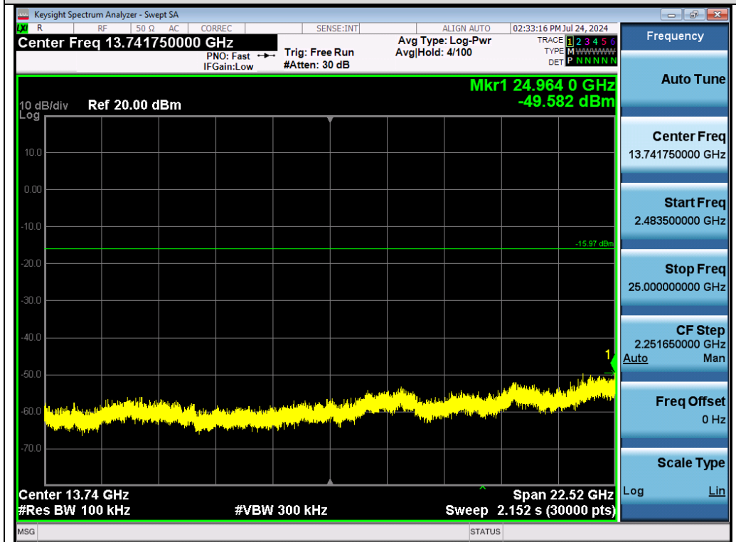
Test_Graph_802.11b_Chain A_2437_1Mbps_Higher Band Emissions
