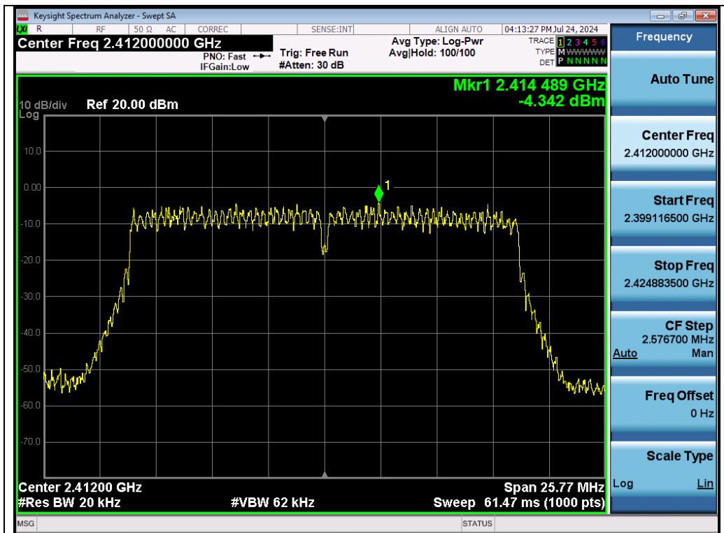
Test_Graph_802.11n20_Chain B_2412_MCS0_PSD
