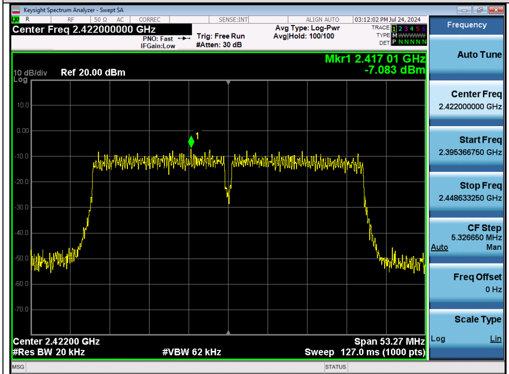
Test_Graph_802.11n40_Chain A_2422_MCS0_PSD
