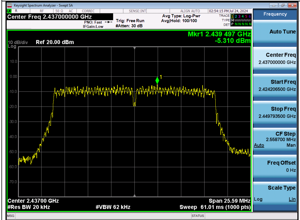
Test_Graph_802.11n20_Chain A_2437_MCS0_PSD
