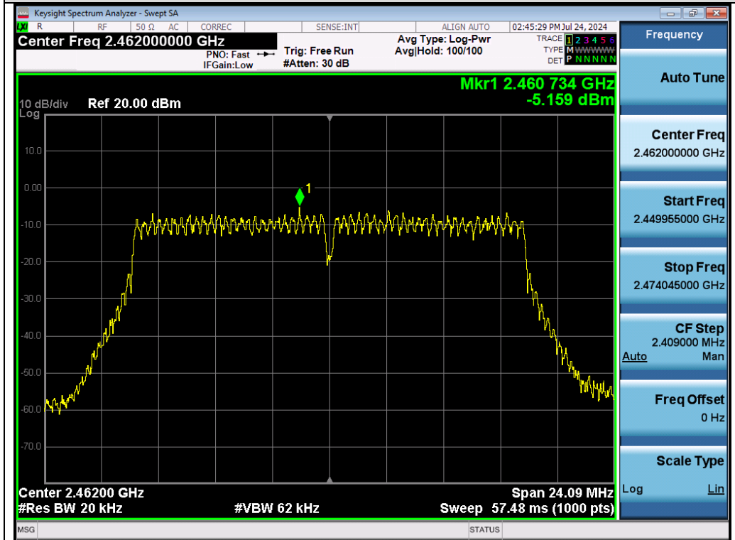
Test_Graph_802.11g_Chain A_2462_6Mbps_PSD
