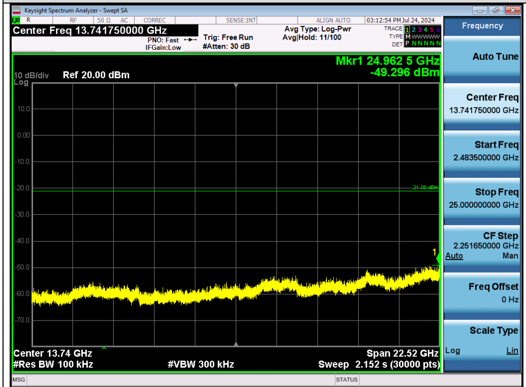
Test_Graph_802.11n40_Chain A_2422_MCS0_Higher Band Emissions
