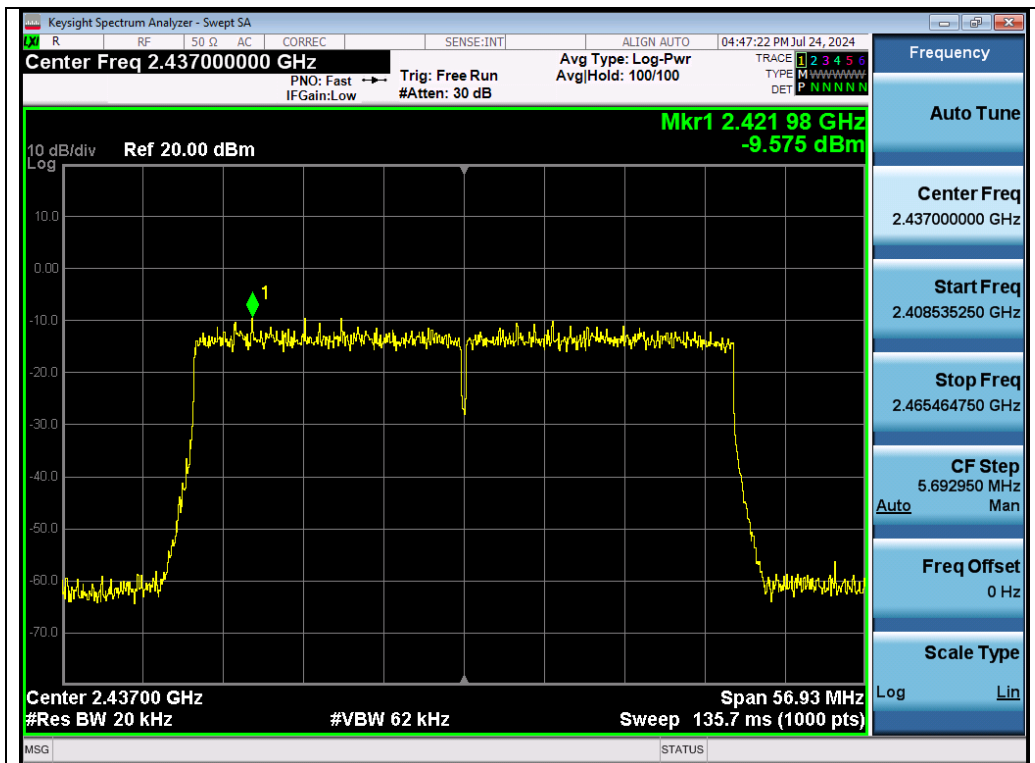
Test_Graph_802.11ax40_Chain B_2437_MCS0_PSD
