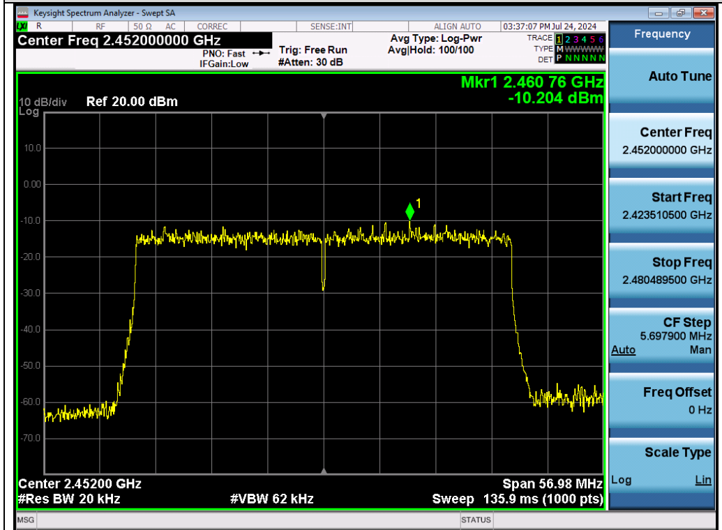
Test_Graph_802.11ax40_Chain A_2452_MCS0_PSD
