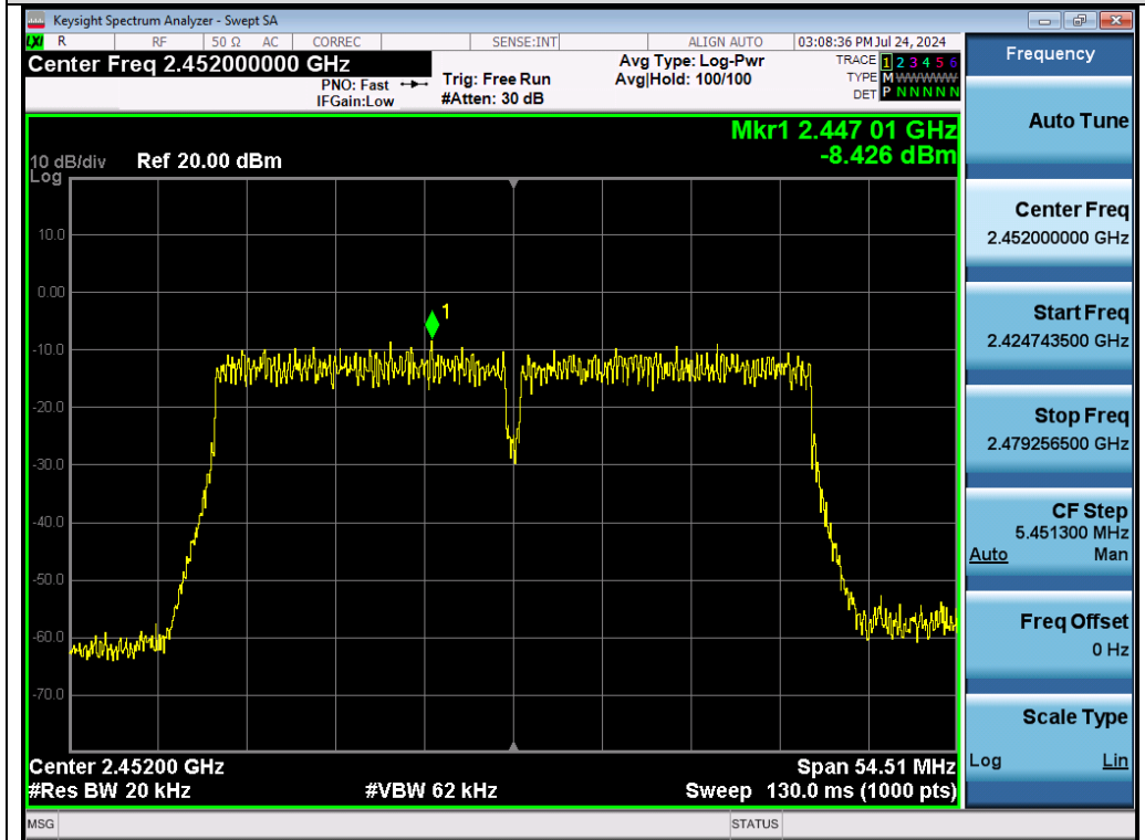
Test_Graph_802.11n40_Chain A_2452_MCS0_PSD
