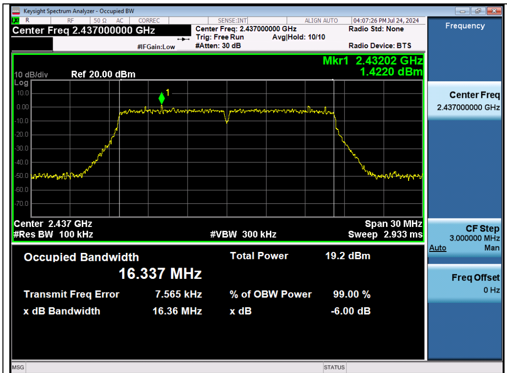
Test_Graph_802.11g_Chain B_2437_6Mbps_DTSBW
