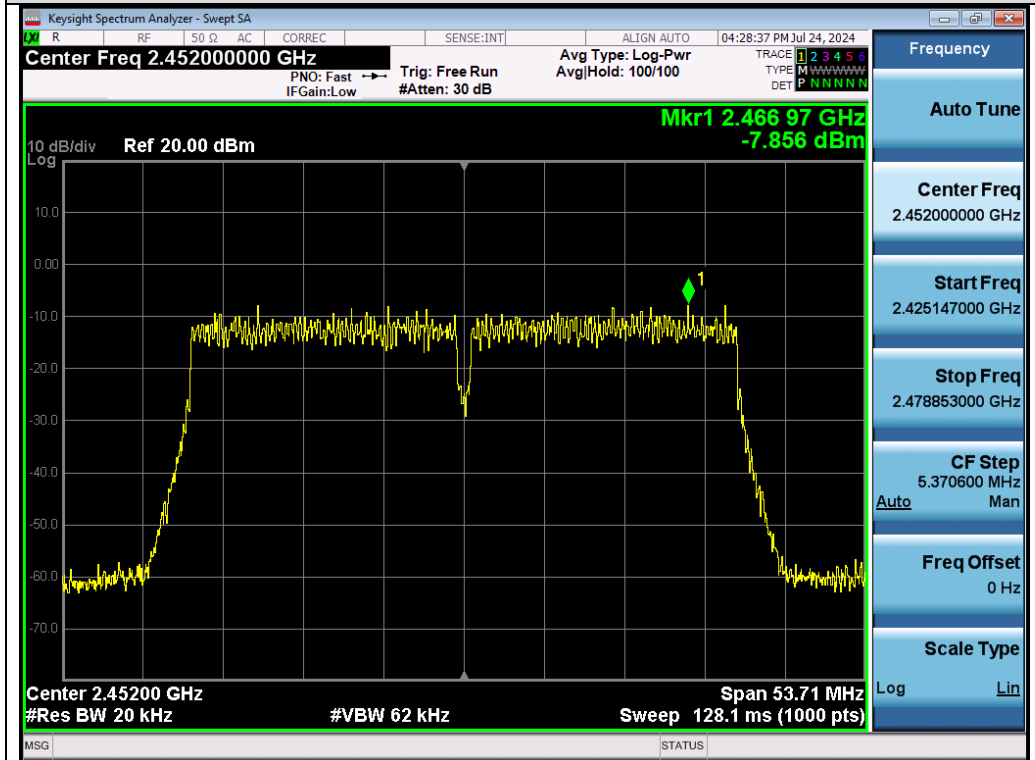
Test_Graph_802.11n40_Chain B_2452_MCS0_PSD
