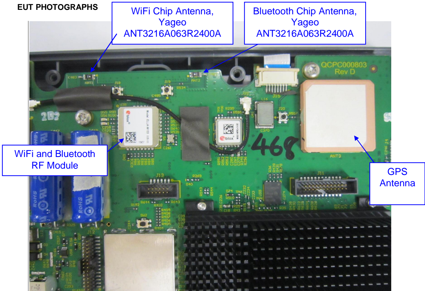
RF Module Circuit Close-up
