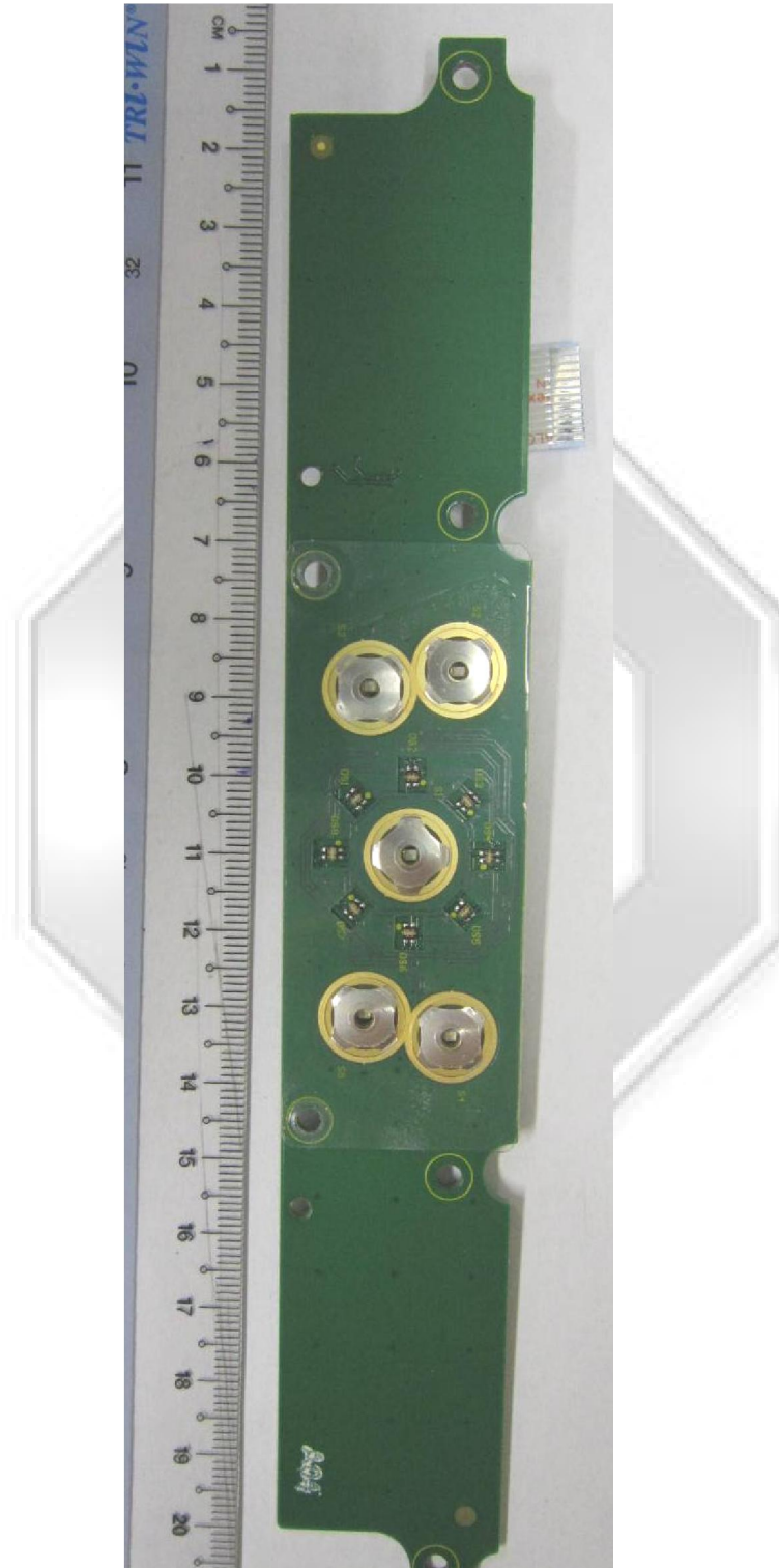
Sub-Board PCB Trace Side
