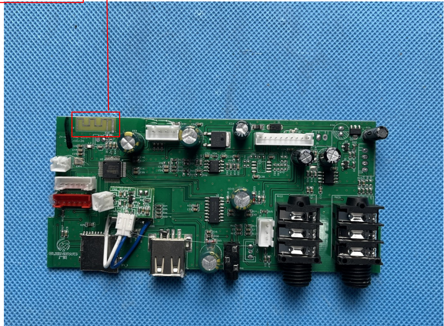
BT Antenna
