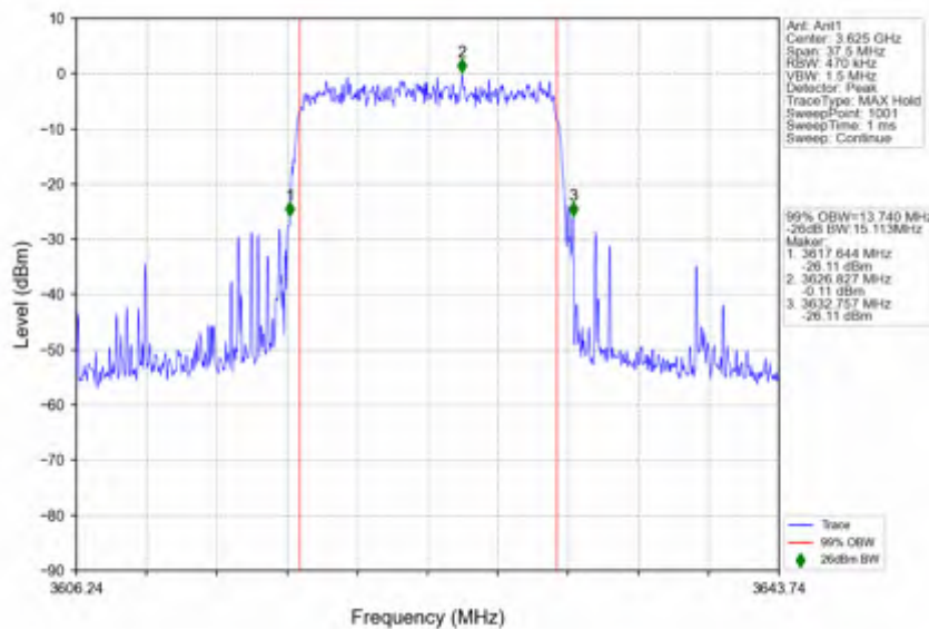
n78d_30kHz_SISO_NTV_15MHz_CP-OFDM 16 QAM_3624.99MHz_Outer_Full
