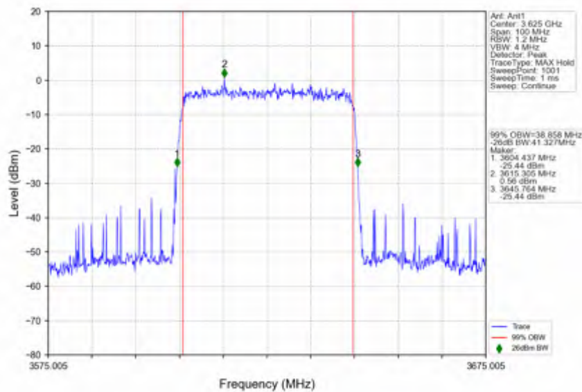
n78d_15kHz_SISO_NTNV_40MHz_DFT-s-OFDM PI/2 BPSK_3625.005MHz_Outer_Full
