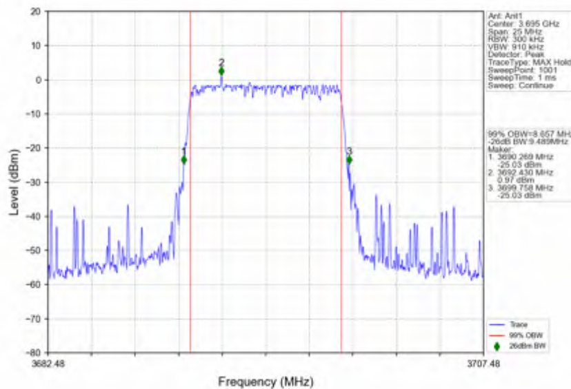
n78d_30kHz_SISO_NTNV_10MHz_DFT-s-OFDM_64_QAM_3694.98MHz_Outer_Full
