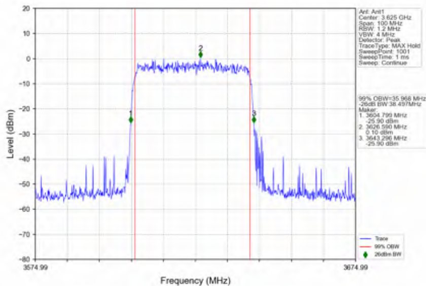
n78d_30kHz_SISO_NTNV_40MHz_DFT-s-OFDM 16 QAM_3624.99MHz_Outer_Full
