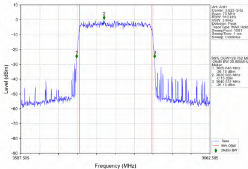
n78d_15kHz_SISO_NTNV_30MHz_DFT-s-OFDM 16 QAM_3625.005MHz_Outer_Full
