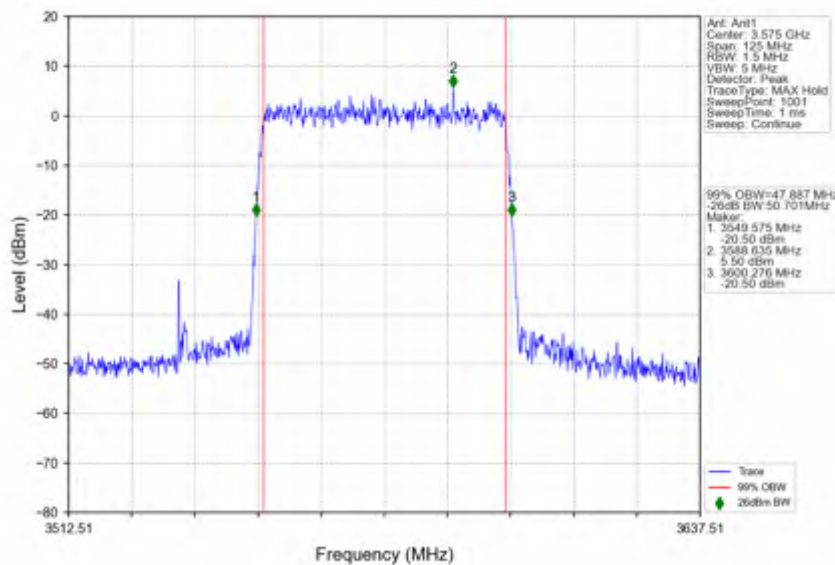
n78d_30kHz_SISO_NTNV_50MHz_CP-OFDM 64 QAM_3575.01MHz_Outer_Full
