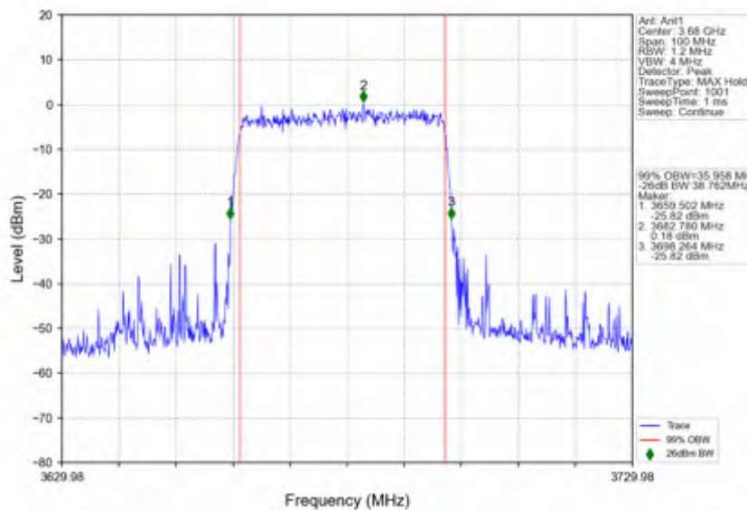
n78d_30kHz_SISO_NTNV_40MHz_DFT-s-OFDM QPSK_3679.98MHz_Outer_Full
