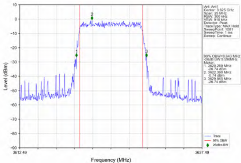
n78d_30kHz_SISO_NTNV_10MHz_CP-OFDM 16 QAM_3624.99MHz_Outer_Full
