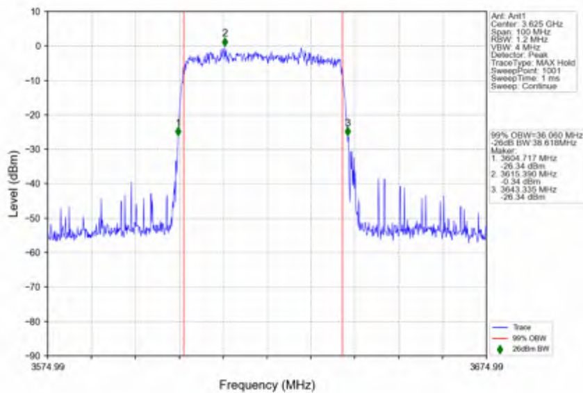
n78d_30kHz_SISO_NTNV_40MHz_DFT-s-OFDM PI/2 BPSK_3624.99MHz_Outer_Full
