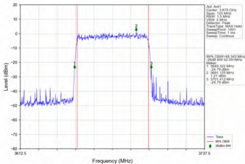
n78d_15kHz_SISO_NTNV_50MHz_CP-OFDM QPSK_3675MHz_Outer_Full
