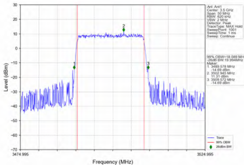
n78e_15kHz_SISO_NTNV_20MHz_DFT-s-OFDM_16_QAM_3499.995MHz_Outer_Full
