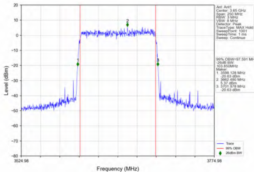
n78d_30kHz_SISO_NTNV_100MHz_CP-OFDM QPSK_3649.98MHz_Outer_Full
