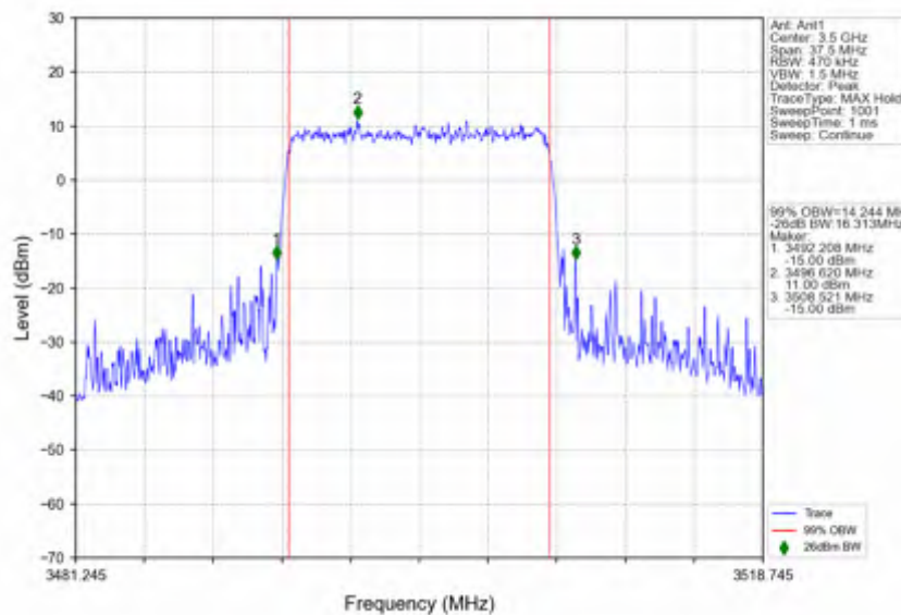
n78e_15kHz_SISO_NTNV_15MHz_CP-OFDM_16_QAM_3499.995MHz_Outer_Full
