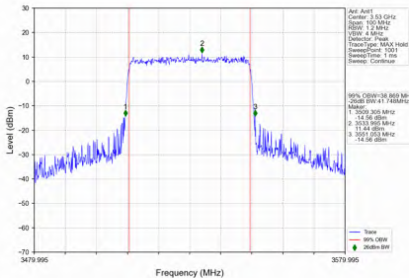
n78e_15kHz_SISO_NTNV_40MHz_CP-OFDM QPSK_3529.995MHz_Outer_Full
