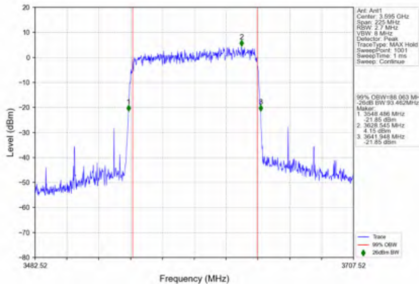
n78d_30kHz_SISO_NTNV_90MHz_CP-OFDM 64 QAM_3595.02MHz_Outer_Full
