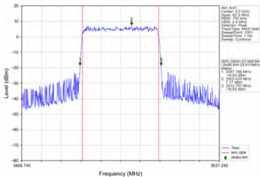
n78e 15kHz SISO NTNV 25MHz CP-OFDM 256 QAM 3499.995MHz Outer Full
