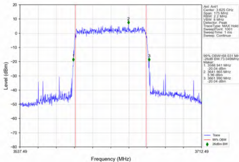
n78d_30kHz_SISO_NTNV_70MHz_CP-OFDM 16 QAM_3624.99MHz_Outer_Full
