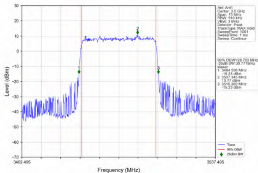
n78e_15kHz_SISO_NTNV_30MHz_DFT-s-OFDM_PI/2_BPSK_3499.995MHz_Outer_Full
