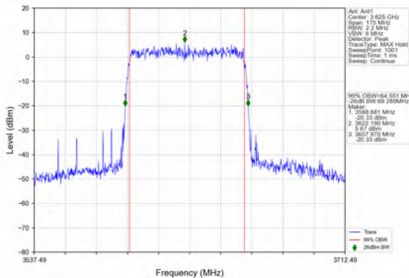
n78d_30kHz_SISO_NTNV_70MHz_DFT-s-OFDM 16 QAM_3624.99MHz_Outer_Full
