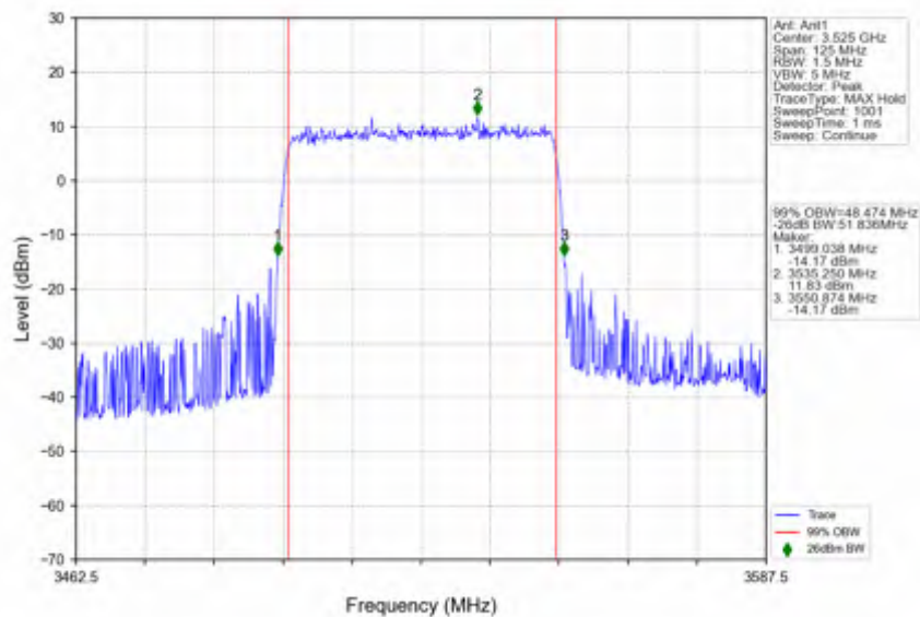
n78e_15kHz_SISO_NTNV_50MHz_DFT-s-OFDM QPSK_3525MHz_Outer_Full
