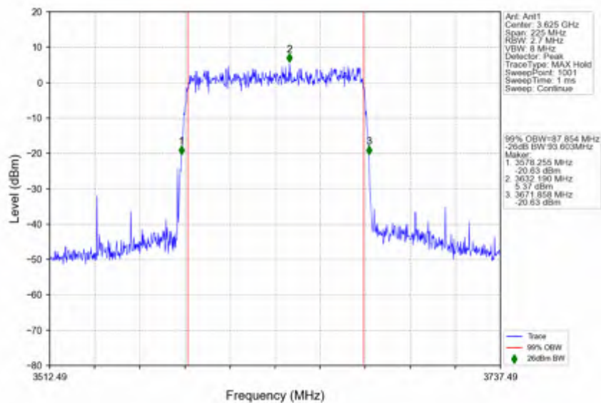
n78d_30kHz_SISO_NTNV_90MHz_CP-OFDM 16 QAM_3624.99MHz_Outer_Full
