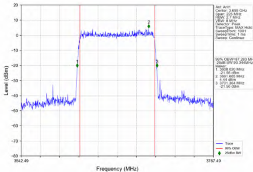
n78d 30kHz SISO NTNV 90MHz DFT-s-OFDM QPSK 3654.99MHz Outer Full
