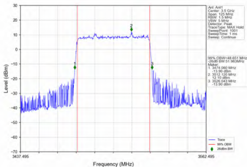
n78e_15kHz_SISO_NTNV_50MHz_DFT-s-OFDM_PI/2_BPSK_3499.995MHz_Outer_Full
