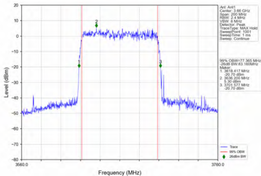
n78d_30kHz_SISO_NTNV_80MHz_CP-OFDM QPSK_3660MHz_Outer_Full
