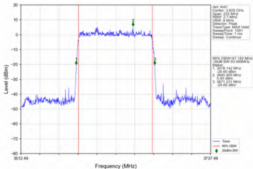
n78d_30kHz_SISO_NTNV_90MHz_DFT-s-OFDM PI/2 BPSK_3624.99MHz_Outer_Full
