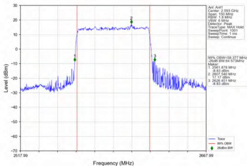
n41_30kHz_SISO_NTNV_60MHz_DFT-s-OFDM_PI/2_BPSK_2592.99MHz_Outer_Full
