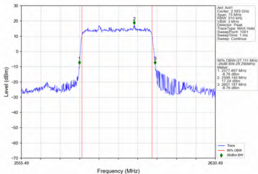
n41_30kHz_SISO_NTNV_30MHz_DFT-s-OFDM_PI/2_BPSK_2592.99MHz_Outer_Full
