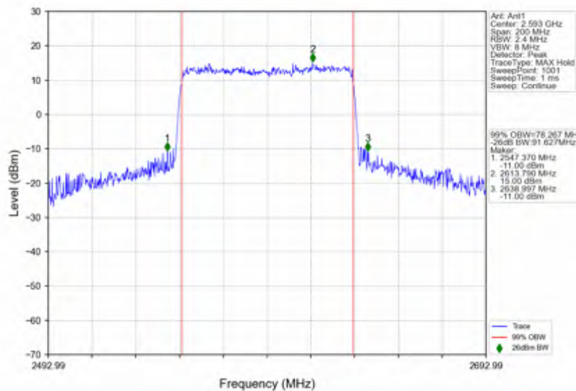
n41_30kHz_SISO_NTNV_80MHz_CP-OFDM_16_QAM_2592.99MHz_Outer_Full
