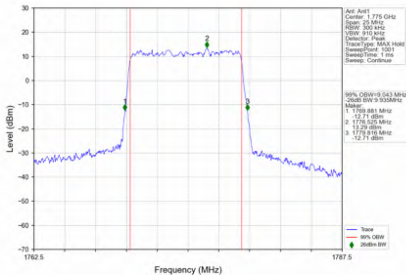
n66_15kHz_SISO_NTNV_10MHz_DFT-s-OFDM QPSK_1775MHz_Outer_Full
