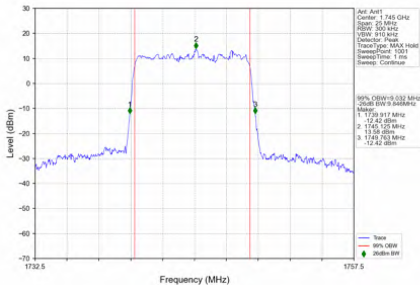
n66_15kHz_SISO_NTNV_10MHz_DFT-s-OFDM_16 QAM_1745MHz_Outer_Full
