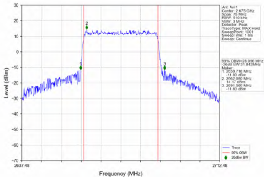
n41_30kHz_SISO_NTNV_30MHz_CP-OFDM_64_QAM_2674.98MHz_Outer_Full
