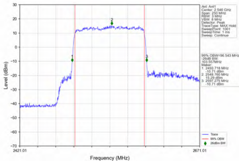
n41_30kHz_SISO_NTNV_100MHz_DFT-s-OFDM 64 QAM 2546.01MHz_Outer_Full
