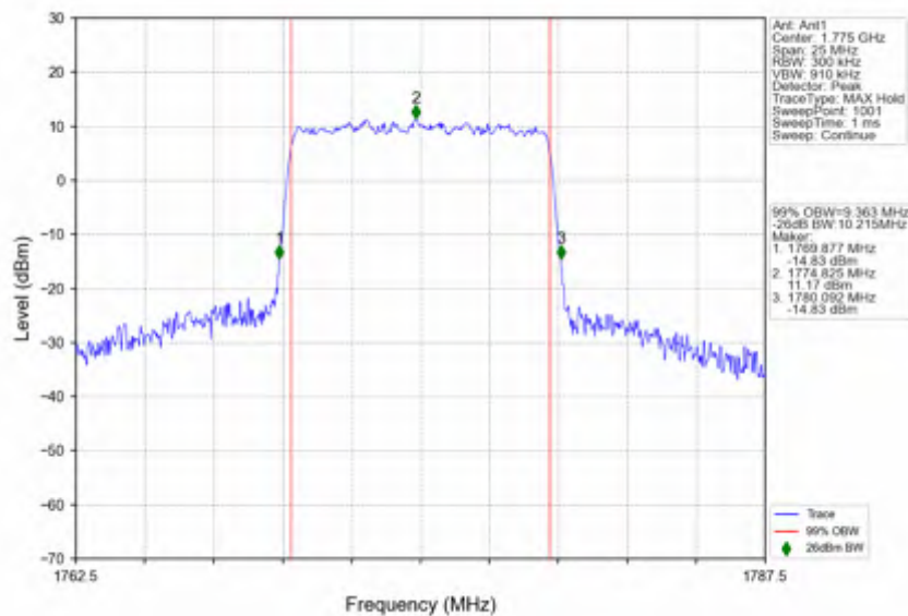
n66_15kHz_SISO_NTNV_10MHz_CP-OFDM_QPSK_1775MHz_Outer_Full
