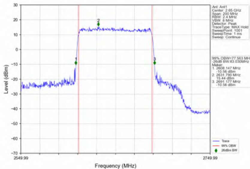
n41_30kHz_SISO_NTNV_80MHz_DFT-s-OFDM_64_QAM_2649.99MHz_Outer_Full
