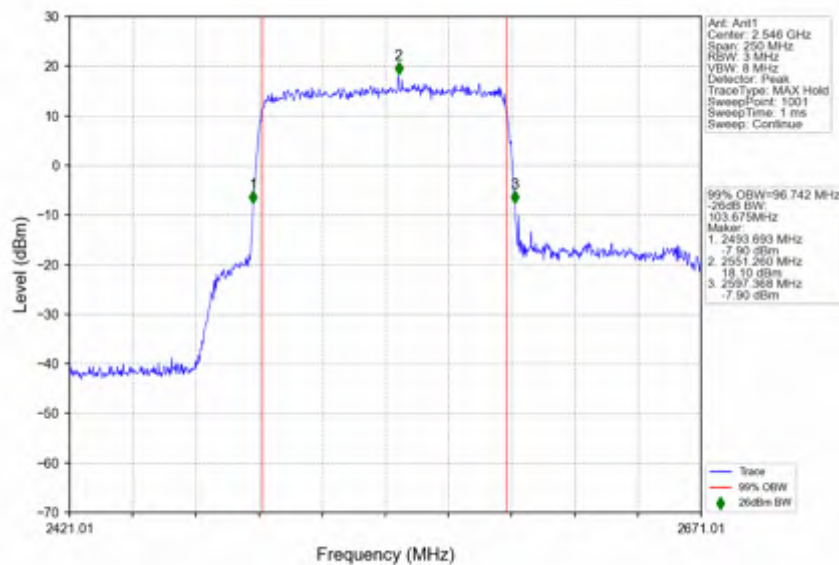
n41_30kHz_SISO_NTNV_100MHz_DFT-s-OFDM_QPSK_2546.01MHz_Outer_Full
