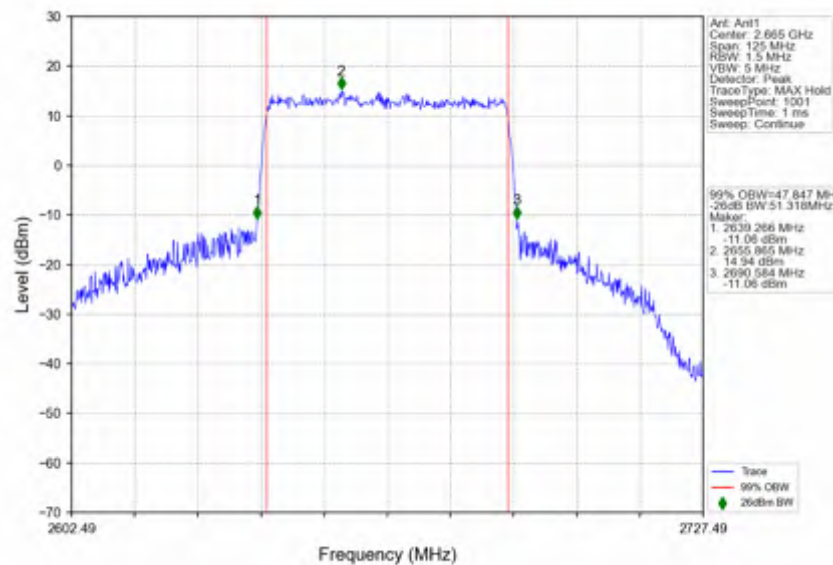
n41_30kHz_SISO_NTNV_50MHz_CP-OFDM QPSK_2664.99MHz_Outer_Full
