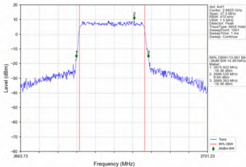
n41_30kHz_SISO_NTNV_15MHz_DFT-s-OFDM_64_QAM_2682.48MHz_Outer_Full
