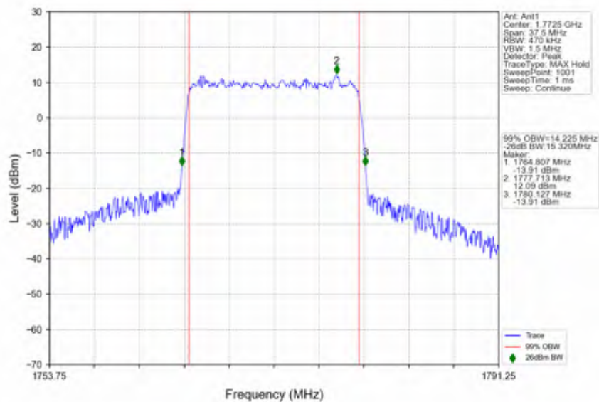
n66_15kHz_SISO_NTNV_15MHz_CP-OFDM_64_QAM_1772.5MHz_Outer_Full
