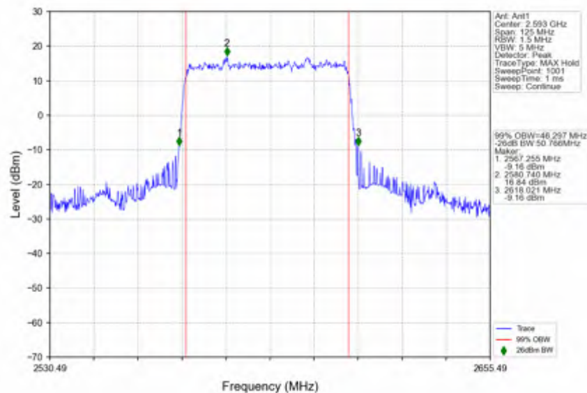
n41_30kHz_SISO_NTNV_50MHz_DFT-s-OFDM_PI/2_BPSK_2592.99MHz_Outer_Full
