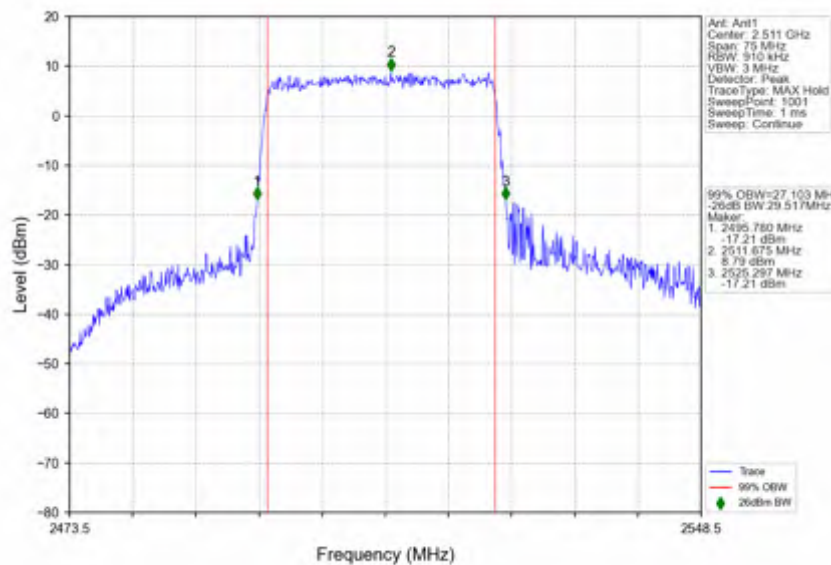
n41_30kHz_SISO_NTNV_30MHz_DFT-s-OFDM_64_QAM_2511MHz_Outer_Full
