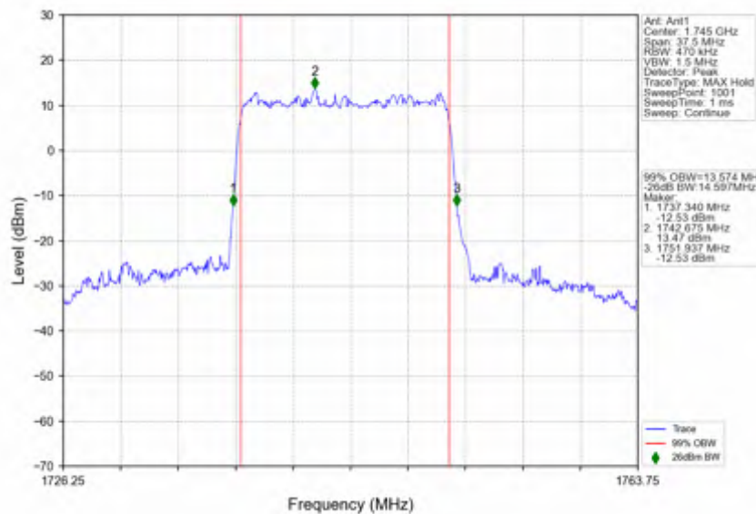
n66 15kHz SISO NTV 15MHz DFT-s-OFDM 16 QAM 1745MHz Outer Full
