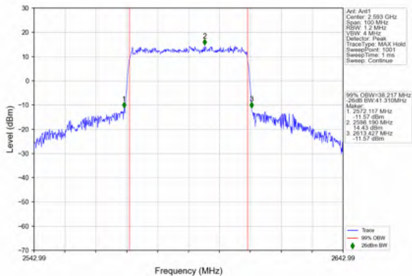
n41_30kHz_SISO_NTNV_40MHz_CP-OFDM_16_QAM_2592.99MHz_Outer_Full
