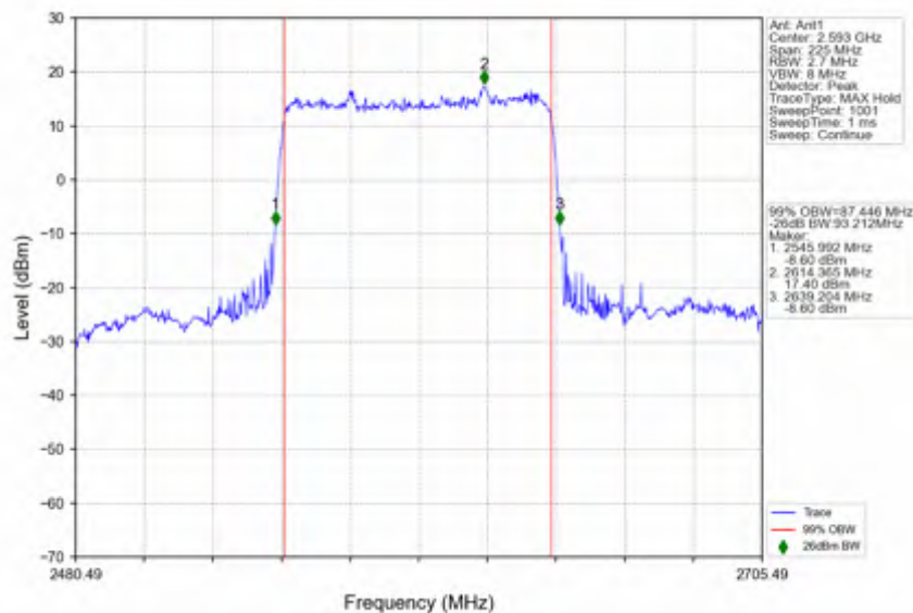
n41_30kHz_SISO_NTNV_90MHz_DFT-s-OFDM_PI/2_BPSK_2592.99MHz_Outer_Full
