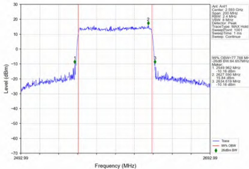
n41_30kHz_SISO_NTNV_80MHz_DFT-s-OFDM_16_QAM_2592.99MHz_Outer_Full
