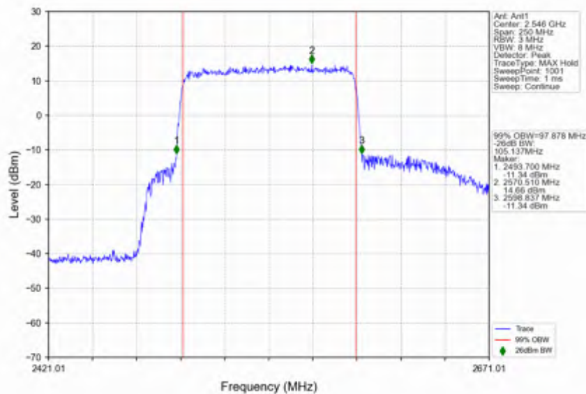
n41_30kHz_SISO_NTNV_100MHz_CP-OFDM_QPSK_2546.01MHz_Outer_Full
