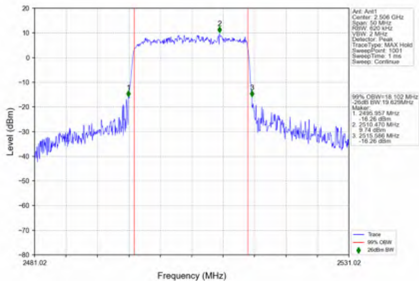
n41_30kHz_SISO_NTNV_20MHz_DFT-s-OFDM_64_QAM_2506.02MHz_Outer_Full
