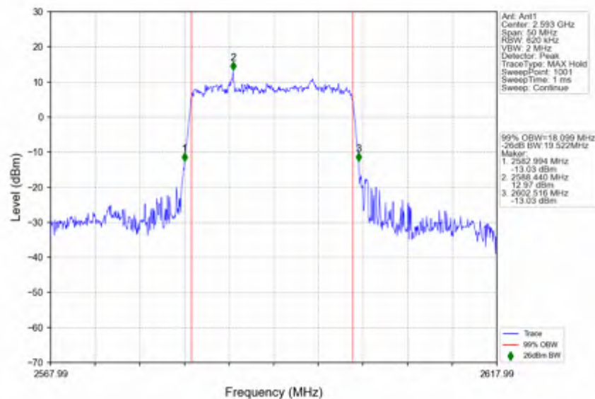
n41_30kHz_SISO_NTNV_20MHz_DFT-s-OFDM_PI/2_BPSK_2592.99MHz_Outer_Full
