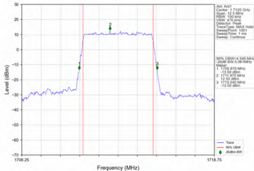
n66_15kHz_SISO_NTNV_5MHz_DFT-s-OFDM QPSK_1712.5MHz_Outer_Full
