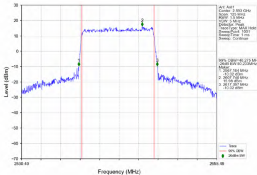
n41_30kHz_SISO_NTNV_50MHz_DFT-s-OFDM_16_QAM_2592.99MHz_Outer_Full
