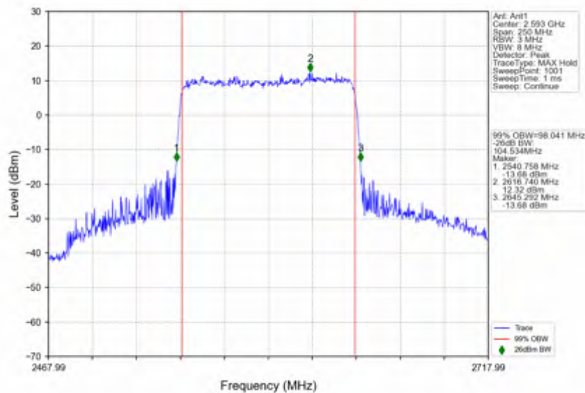
n41_30kHz_SISO_NTNV_100MHz_CP-OFDM_256_QAM_2592.99MHz_Outer_Full
