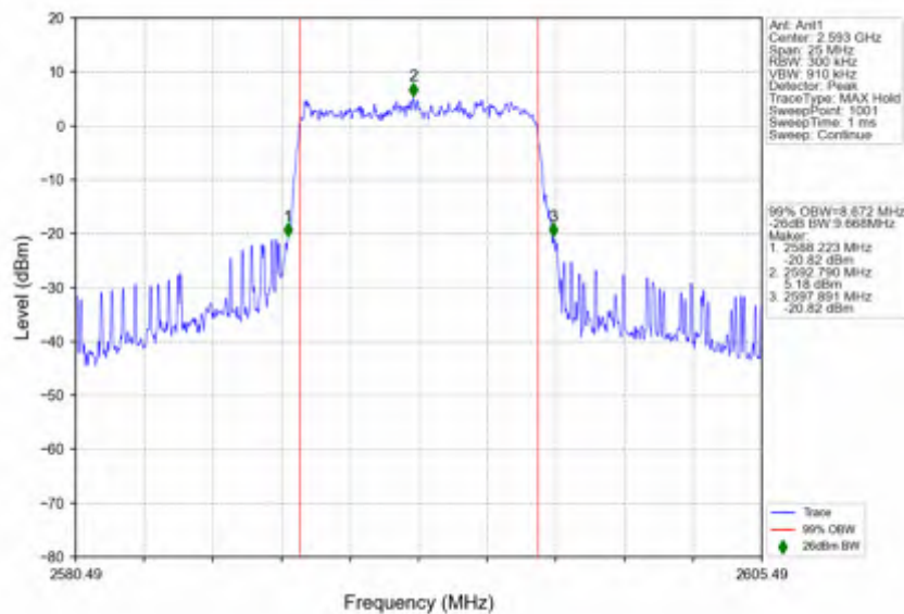
n41_30kHz_SISO_NTNV_10MHz_CP-OFDM 256 QAM_2592.99MHz_Outer_Full
