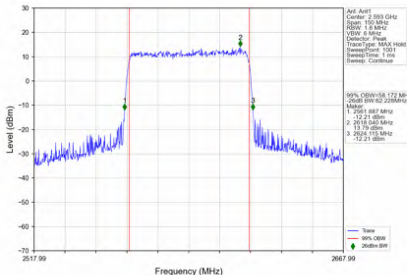
n41_30kHz_SISO_NTNV_60MHz_DFT-s-OFDM_256_QAM_2592.99MHz_Outer_Full
