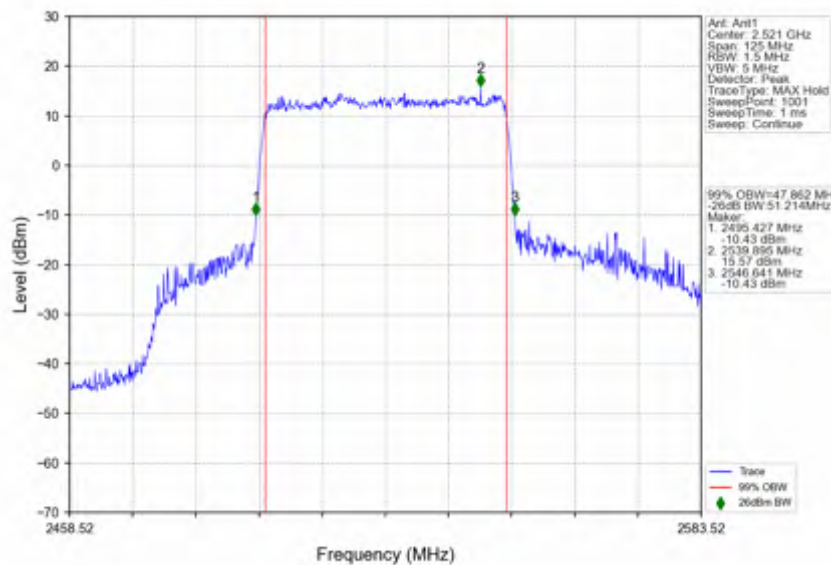
n41_30kHz_SISO_NTNV_50MHz_CP-OFDM QPSK_2521.02MHz_Outer_Full
