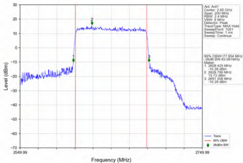
n41_30kHz_SISO_NTNV_80MHz_CP-OFDM_QPSK_2649.99MHz_Outer_Full
