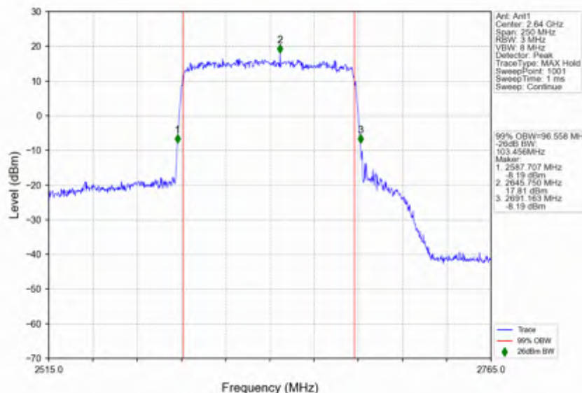
n41_30kHz_SISO_NTNV_100MHz_DFT-s-OFDM_QPSK_2640MHz_Outer_Full
