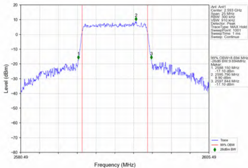
n41_30kHz_SISO_NTNV_10MHz_CP-OFDM_16_QAM_2592.99MHz_Outer_Full
