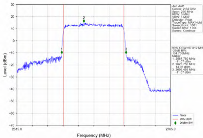
n41_30kHz_SISO_NTNV_100MHz_CP-OFDM QPSK_2640MHz_Outer_Full
