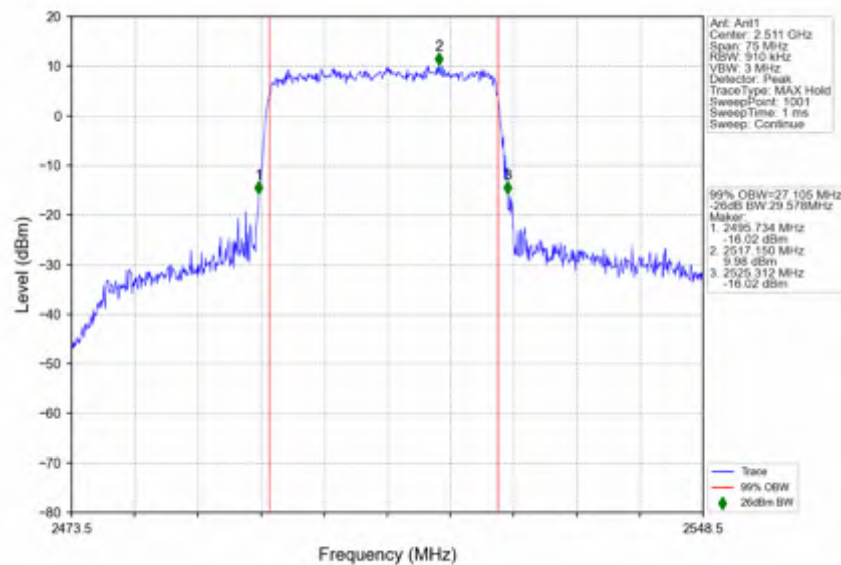
n41_30kHz_SISO_NTNV_30MHz_DFT-s-OFDM QPSK_2511MHz_Outer_Full
