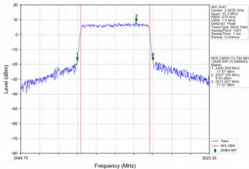
n41_30kHz_SISO_NTNV_15MHz_CP-OFDM QPSK_2503.5MHz_Outer_Full
