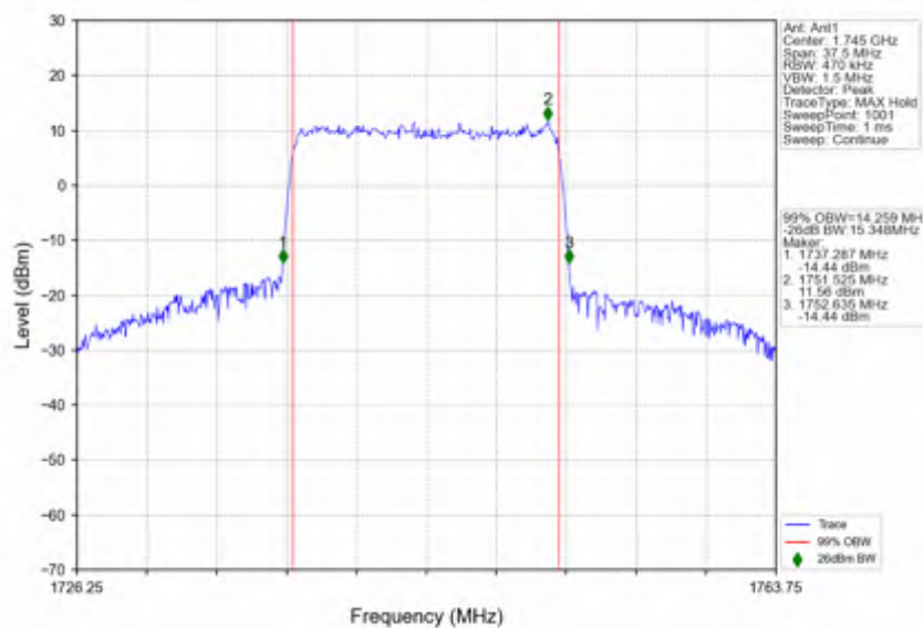
n66_15kHz_SISO_NTNV_15MHz_CP-OFDM_16 QAM_1745MHz_Outer_Full
