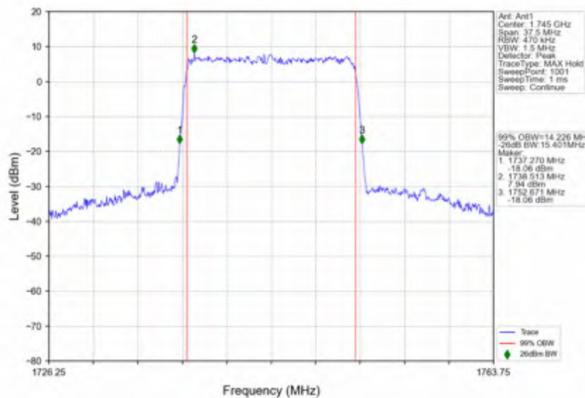
n66_15kHz_SISO_NTNV_15MHz_CP-OFDM_256_QAM_1745MHz_Outer_Full
