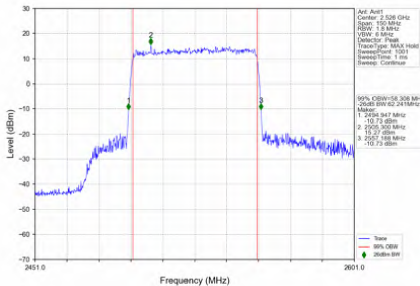
n41_30kHz_SISO_NTNV_60MHz_DFT-s-OFDM_64_QAM_2526MHz_Outer_Full
