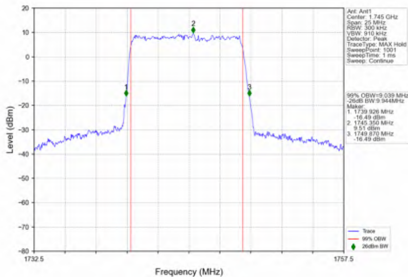
n66_15kHz_SISO_NTNV_10MHz_DFT-s-OFDM_256_QAM_1745MHz_Outer_Full
