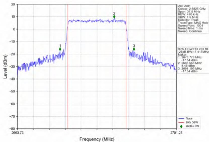
n41_30kHz_SISO_NTNV_15MHz_CP-OFDM QPSK_2682.48MHz_Outer_Full
