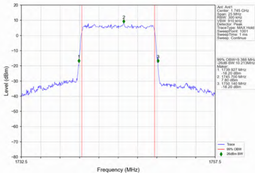
n66_15kHz_SISO_NTNV_10MHz_CP-OFDM 256 QAM_1745MHz_Outer_Full
