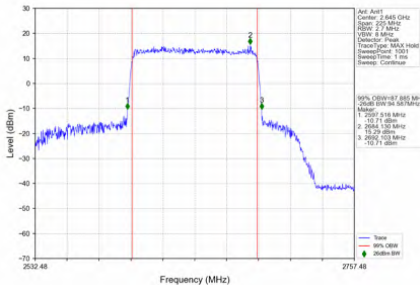
n41_30kHz_SISO_NTNV_90MHz_CP-OFDM QPSK_2644.98MHz_Outer_Full
