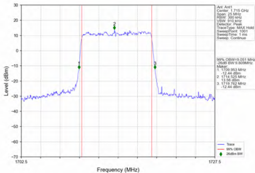
n66_15kHz_SISO_NTNV_10MHz_DFT-s-OFDM_QPSK_1715MHz_Outer_Full
