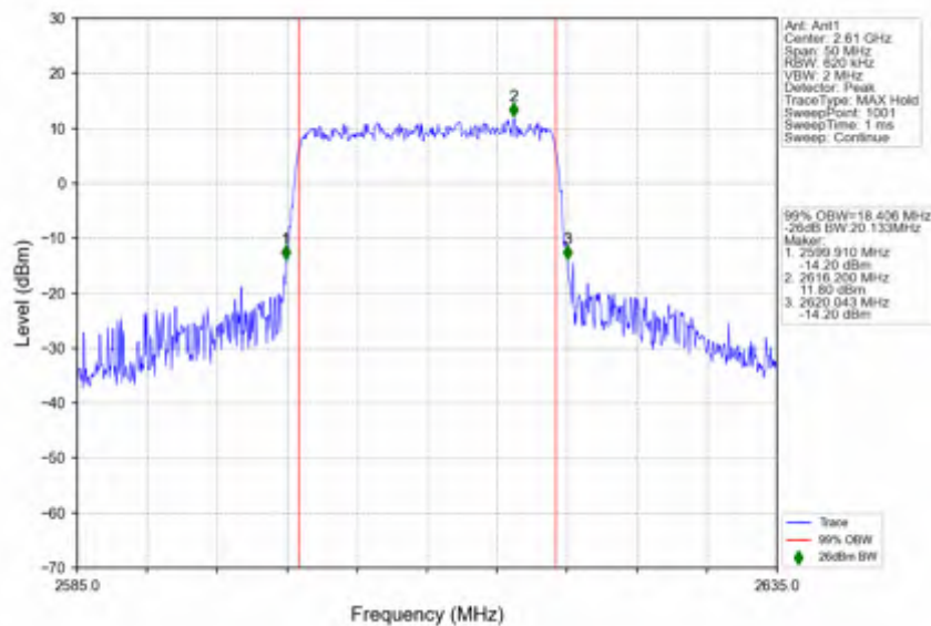
n38_30kHz_SISO_NTNV_20MHz_CP-OFDM QPSK_2610MHz_Outer_Full
