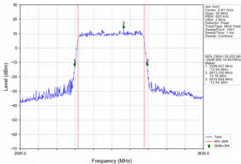
n38_30kHz_SISO_NTNV_20MHz_DFT-s-OFDM_64_QAM_2610MHz_Outer_Full
