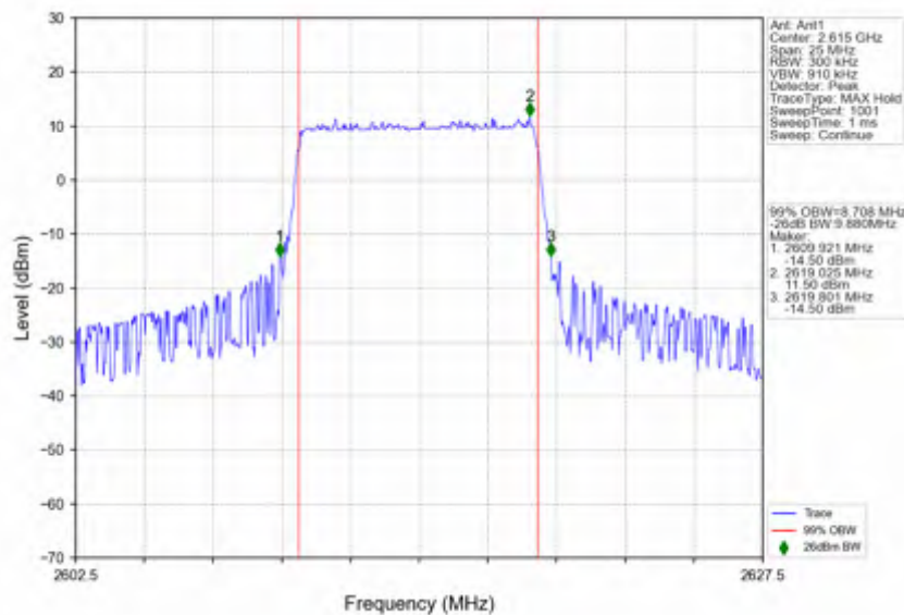
n38_30kHz_SISO_NTNV_10MHz_DFT-s-OFDM_64_QAM_2615MHz_Outer_Full
