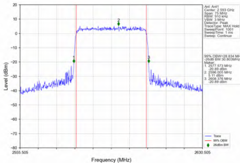
n41_15kHz_SISO_NTNV_30MHz_CP-OFDM 256 QAM_2593.005MHz_Outer_Full
