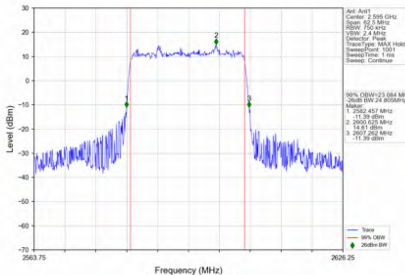
n38_30kHz_SISO_NTNV_25MHz_DFT-s-OFDM PI/2 BPSK_2595MHz_Outer_Full
