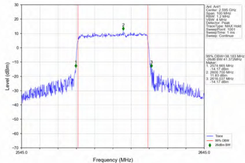
n38_30kHz_SISO_NTNV_40MHz_CP-OFDM 64 QAM_2600MHz_Outer_Full
