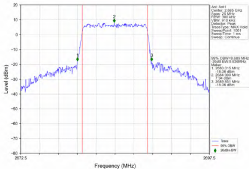
n41_30kHz_SISO_NTNV_10MHz_CP-OFDM QPSK_2685MHz_Outer_Full
