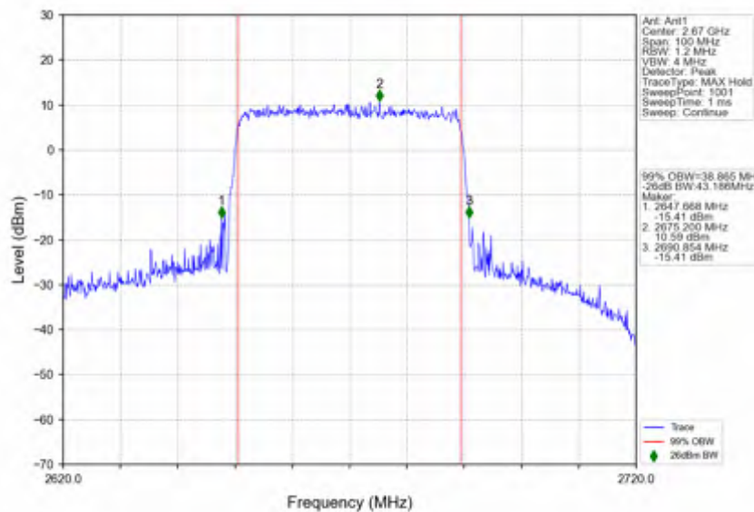
n41_15kHz_SISO_NTNV_40MHz_DFT-s-OFDM QPSK_2670MHz_Outer_Full
