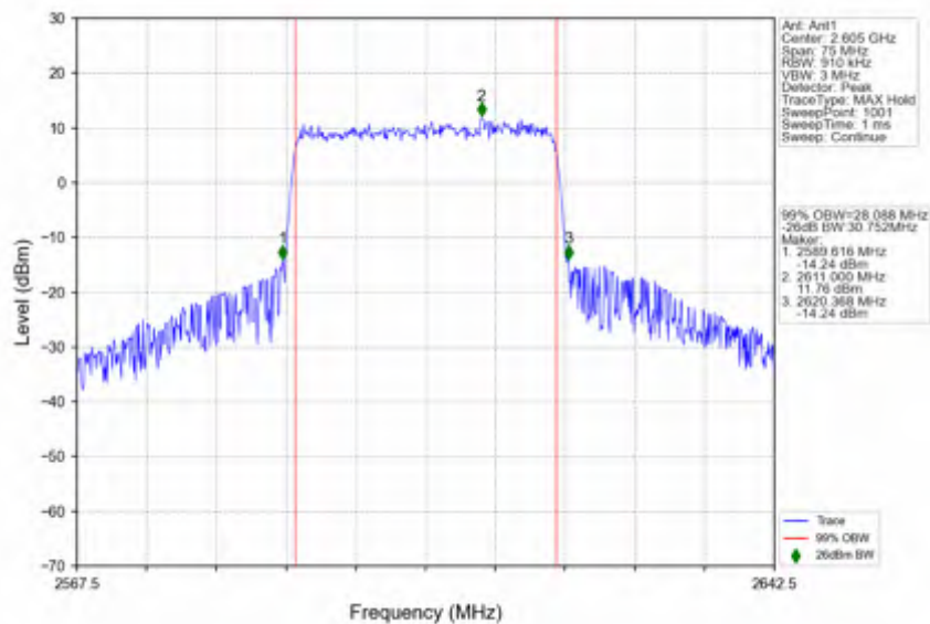
n38_30kHz_SISO_NTNV_30MHz_CP-OFDM QPSK_2605MHz_Outer_Full
