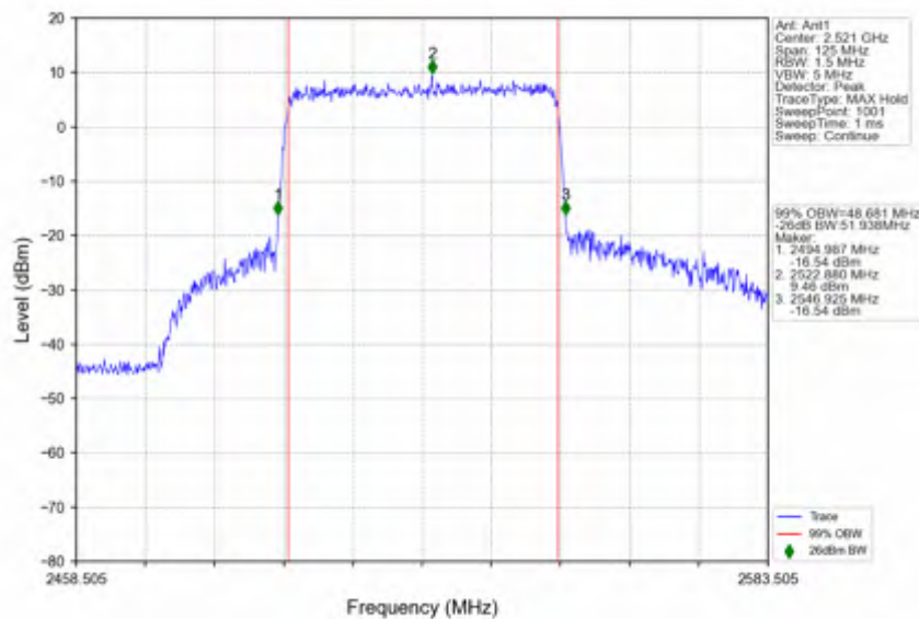
n41_15kHz_SISO_NTNV_50MHz_CP-OFDM QPSK_2521.005MHz_Outer_Full
