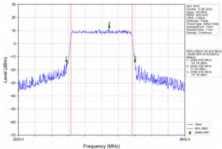
n38 30kHz SISO NTN 20MHz CP-OFDM 64 QAM 2580MHz Outer Full
