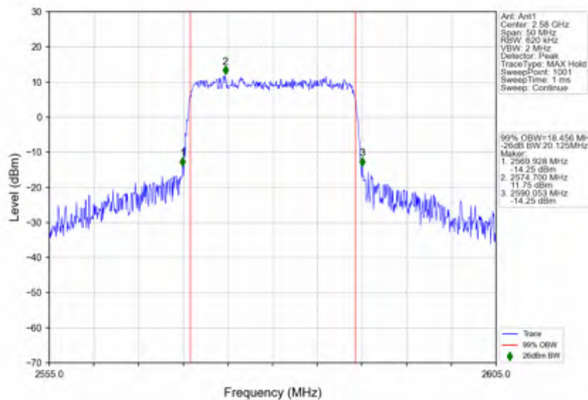
n38_30kHz_SISO_NTNV_20MHz_CP-OFDM QPSK_2580MHz_Outer_Full
