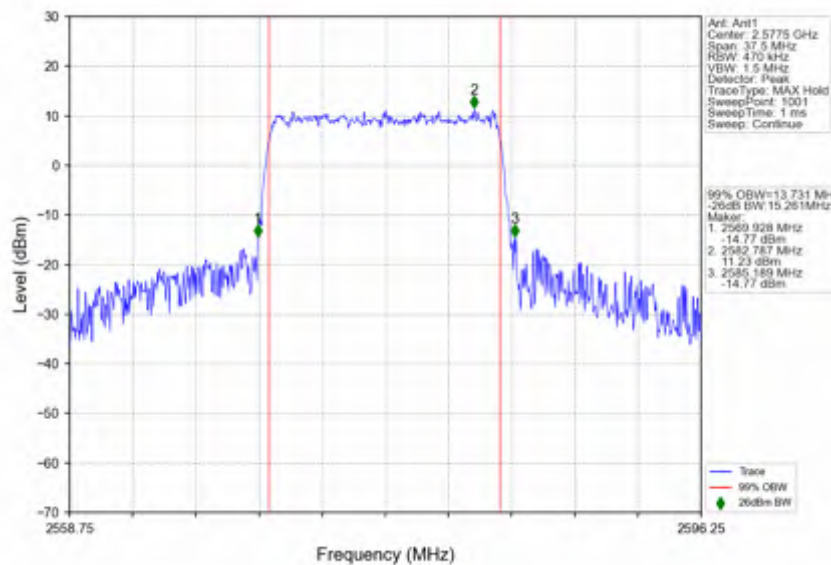
n38_30kHz_SISO_NTNV_15MHz_CP-OFDM_QPSK_2577.5MHz_Outer_Full
