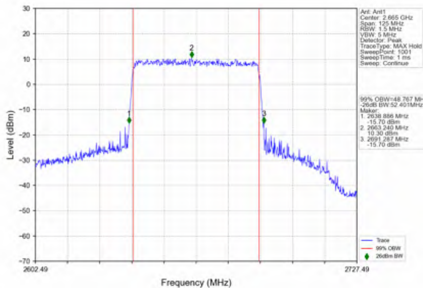
n41_15kHz_SISO_NTNV_50MHz_DFT-s-OFDM QPSK_2664.99MHz_Outer_Full
