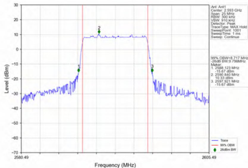
n41_30kHz_SISO_NTNV_10MHz_DFT-s-OFDM PI/2 BPSK_2592.99MHz_Outer_Full
