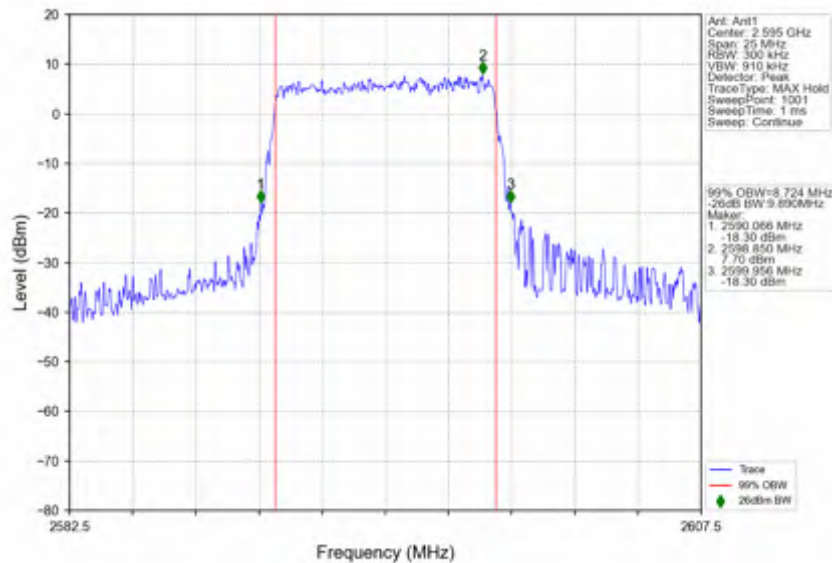
n38_30kHz_SISO_NTNV_10MHz_CP-OFDM_256 QAM_2595MHz_Outer_Full
