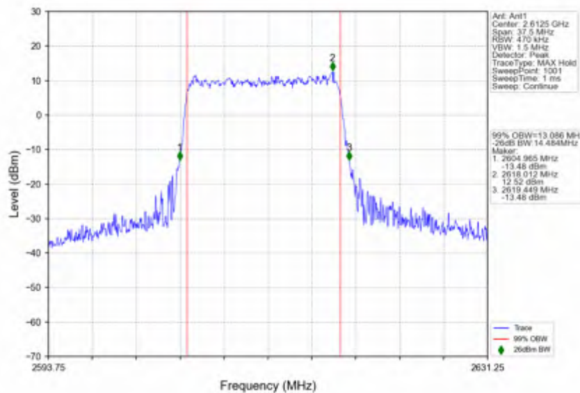
n38_30kHz_SISO_NTNV_15MHz_DFT-s-OFDM_64_QAM_2612.5MHz_Outer_Full
