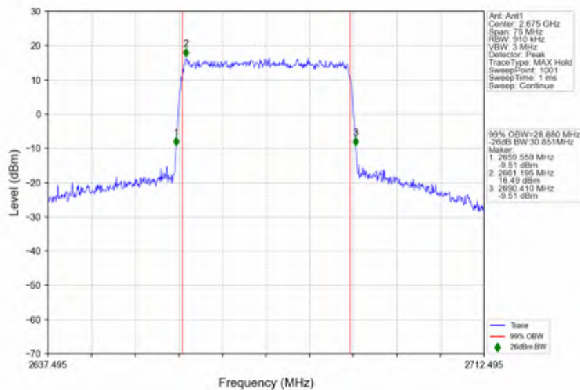
n41_15kHz_SISO_NTNV_30MHz_DFT-s-OFDM_QPSK_2674.995MHz_Outer_Full
