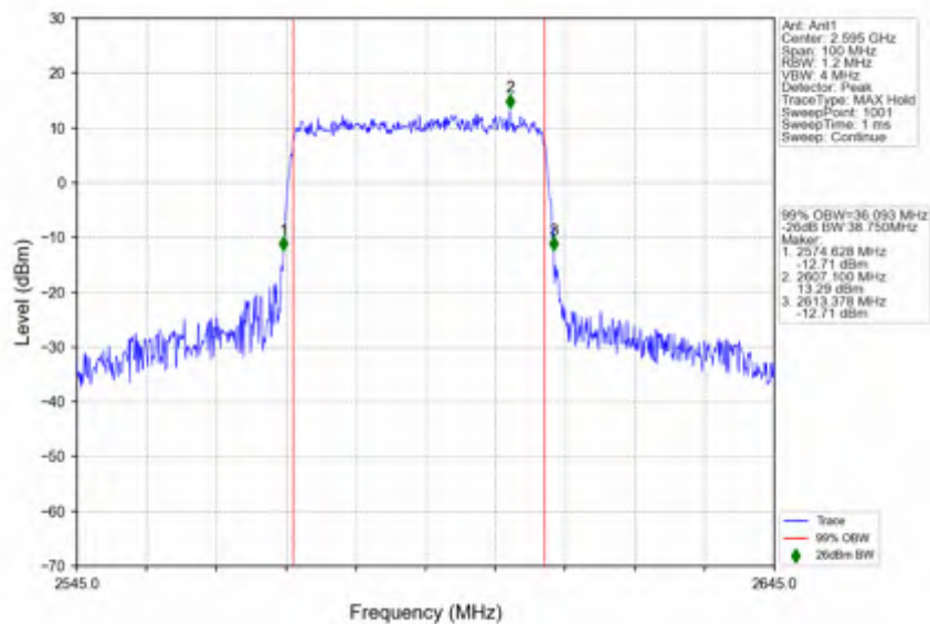
n38_30kHz_SISO_NTNV_40MHz_DFT-s-OFDM_16_QAM_2595MHz_Outer_Full
