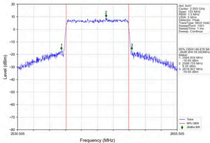
n41_15kHz_SISO_NTNV_50MHz_CP-OFDM 16 QAM 2593.005MHz_Outer_Full
