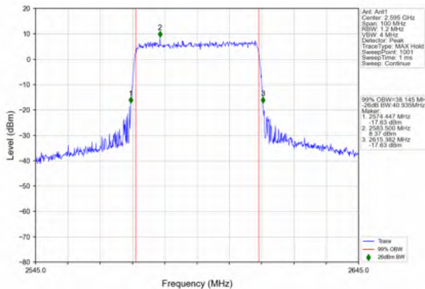
n38_30kHz_SISO_NTNV_40MHz_CP-OFDM_256 QAM_2595MHz_Outer_Full
