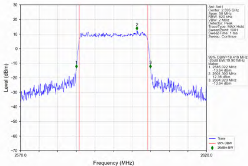
n38_30kHz_SISO_NTNV_20MHz_CP-OFDM_16_QAM_2595MHz_Outer_Full
