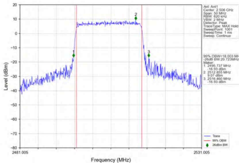
n41_15kHz_SISO_NTNV_20MHz_DFT-s-OFDM 64 QAM_2506.005MHz_Outer_Full
