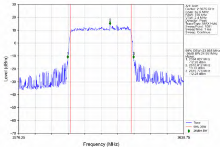
n38_30kHz_SISO_NTNV_25MHz_DFT-s-OFDM QPSK_2607.5MHz_Outer_Full
