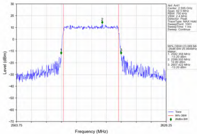
n38_30kHz_SISO_NTNV_25MHz_DFT-s-OFDM_16_QAM_2595MHz_Outer_Full
