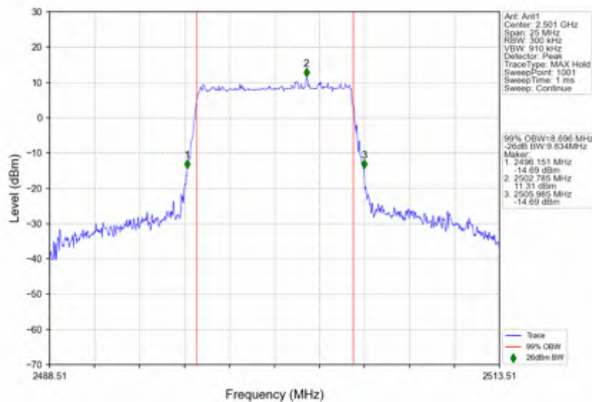
n41_30kHz_SISO_NTNV_10MHz_DFT-s-OFDM QPSK_2501.01MHz_Outer_Full
