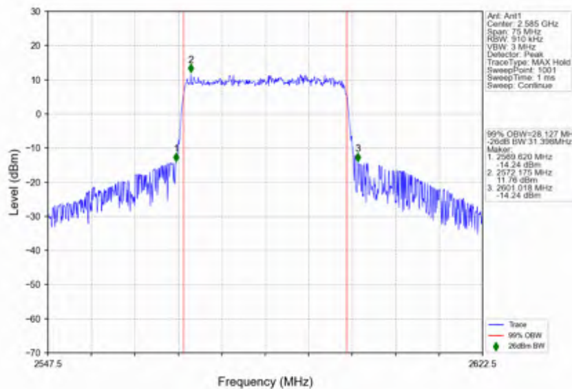
n38_30kHz_SISO_NTNV_30MHz_CP-OFDM QPSK 2585MHz_Outer_Full
