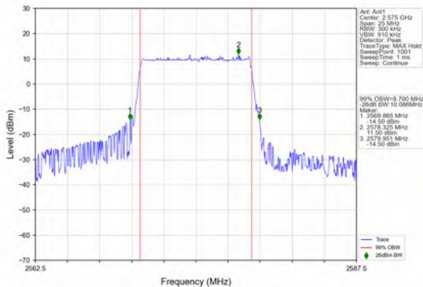
n38_30kHz_SISO_NTNV_10MHz_DFT-s-OFDM_64_QAM_2575MHz_Outer_Full
