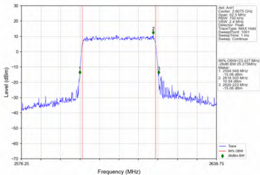
n38 30kHz SISO NTNV 25MHz CP-OFDM 64 QAM 2607.5MHz Outer Full
