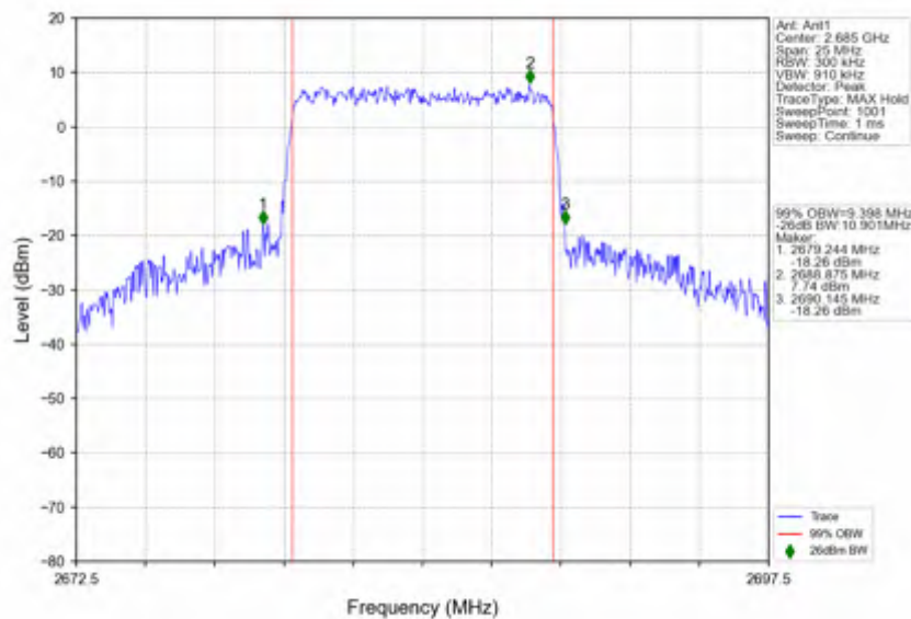
n41 15kHz SISO NTN 10MHz CP-OFDM 64 QAM 2685MHz Outer Full
