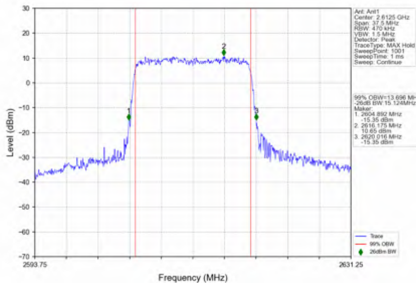
n38_30kHz_SISO_NTNV_15MHz_CP-OFDM 64 QAM_2612.5MHz_Outer_Full
