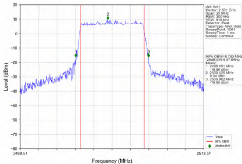
n41_30kHz_SISO_NTNV_10MHz_DFT-s-OFDM_64_QAM_2501.01MHz_Outer_Full
