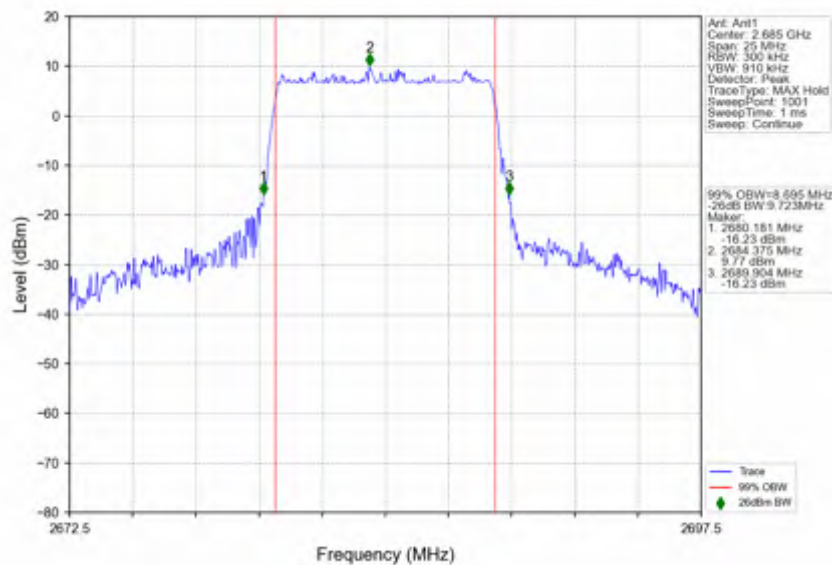
n41_30kHz_SISO_NTNV_10MHz_DFT-s-OFDM 64 QAM_2685MHz_Outer_Full
