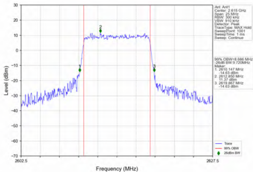
n38_30kHz_SISO_NTNV_10MHz_CP-OFDM QPSK_2615MHz_Outer_Full
