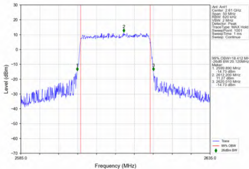
n38_30kHz_SISO_NTNV_20MHz_CP-OFDM 64 QAM_2610MHz_Outer_Full
