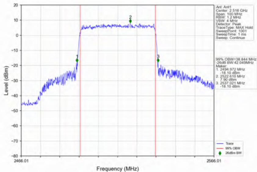
n41_15kHz_SISO_NTNV_40MHz_CP-OFDM 64 QAM_2516.01MHz_Outer_Full
