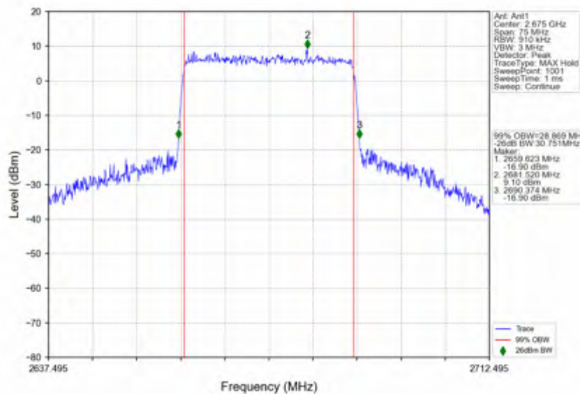
n41_15kHz_SISO_NTNV_30MHz_CP-OFDM 64 QAM_2674.995MHz_Outer_Full
