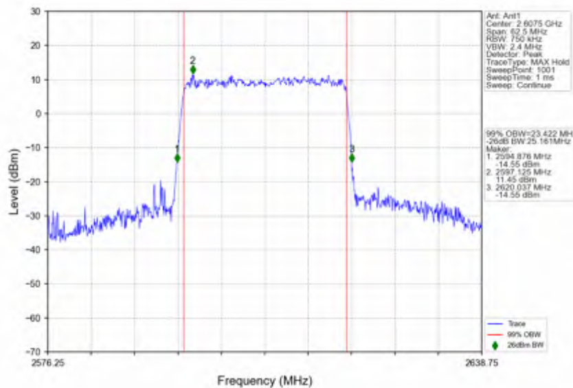
n38_30kHz_SISO_NTNV_25MHz_CP-OFDM QPSK_2607.5MHz_Outer_Full
