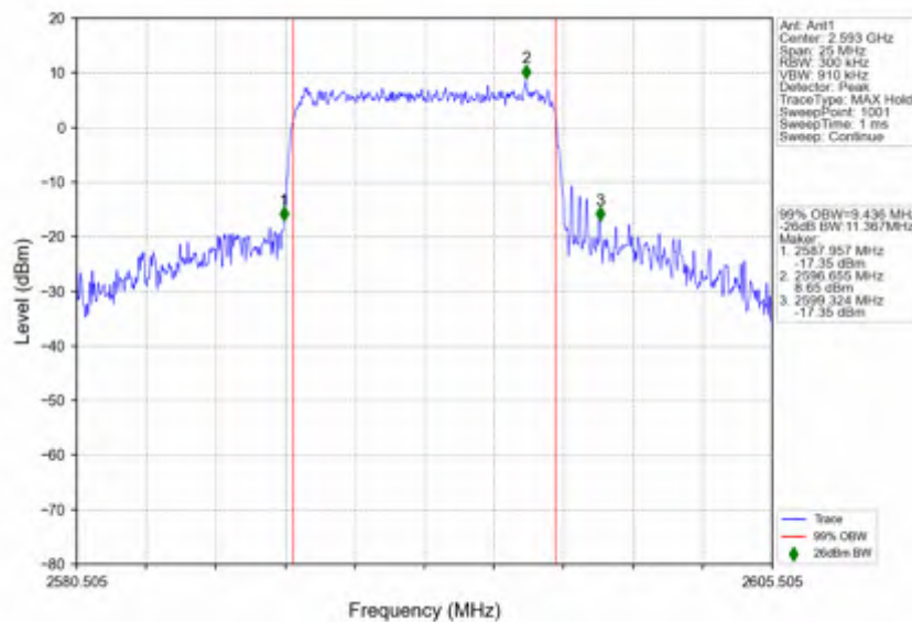
n41_15kHz_SISO_NTNV_10MHz_CP-OFDM_16 QAM_2593.005MHz_Outer_Full
