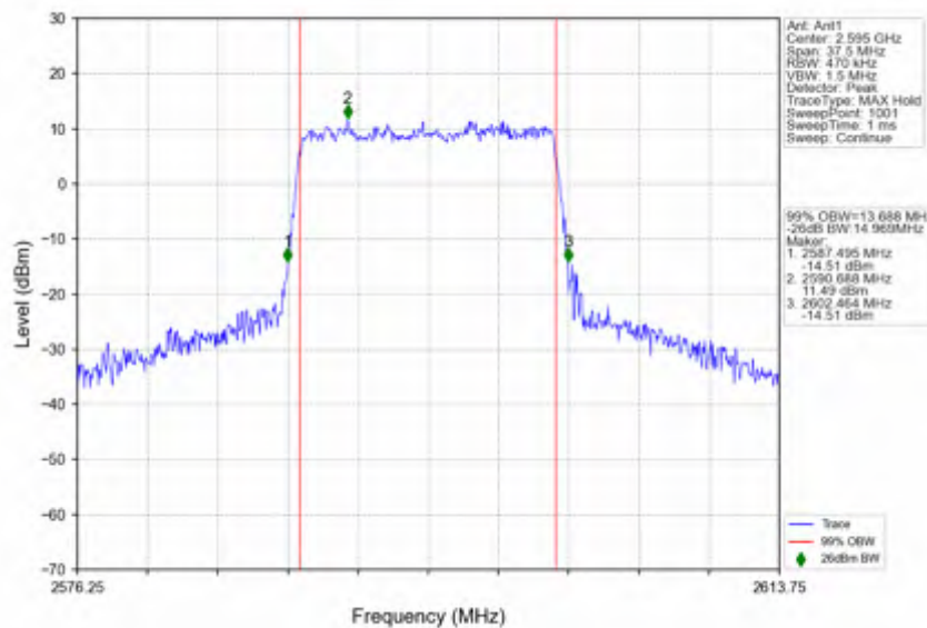
n38_30kHz_SISO_NTNV_15MHz_CP-OFDM_16_QAM_2595MHz_Outer_Full
