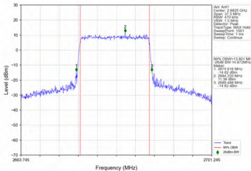
n41 15kHz SISO NTNV 15MHz DFT-s-OFDM QPSK 2682.495MHz Outer Full
