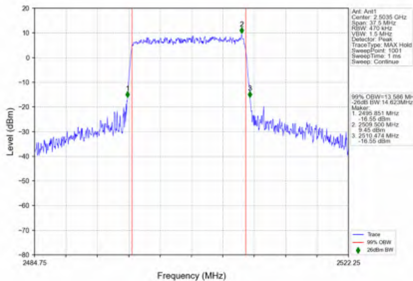
n41_15kHz_SISO_NTNV_15MHz_DFT-s-OFDM 64 QAM_2503.5MHz_Outer_Full
