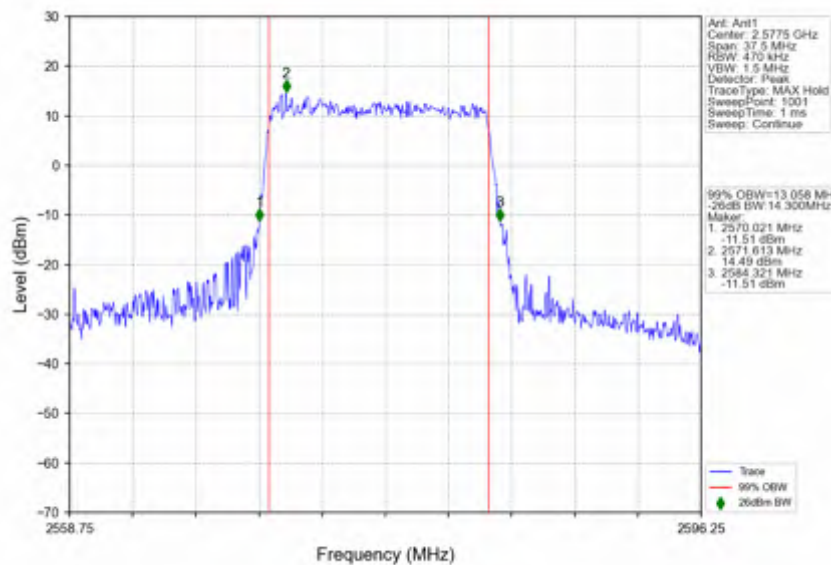
n38_30kHz_SISO_NTNV_15MHz_DFT-s-OFDM QPSK_2577.5MHz_Outer_Full
