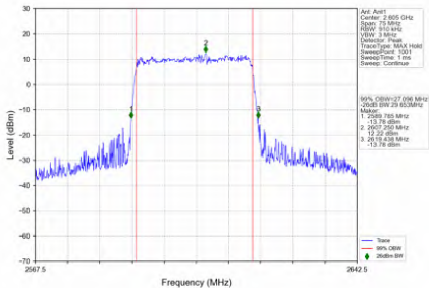
n38_30kHz_SISO_NTNV_30MHz_DFT-s-OFDM_64_QAM_2605MHz_Outer_Full
