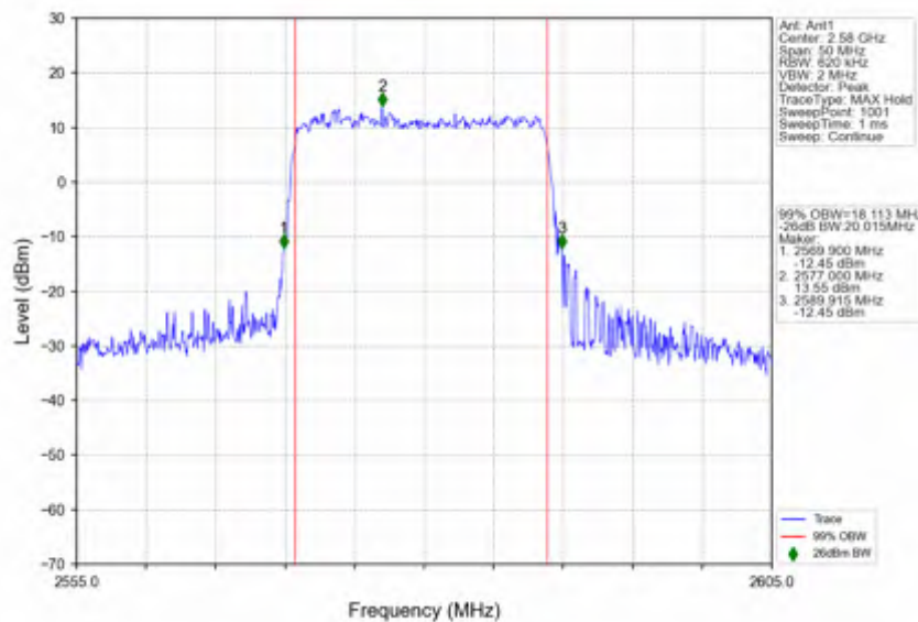
n38_30kHz_SISO_NTNV_20MHz_DFT-s-OFDM QPSK_2580MHz_Outer_Full
