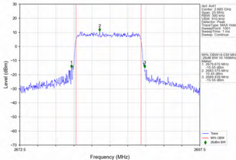
n41_15kHz_SISO_NTNV_10MHz_DFT-s-OFDM QPSK_2685MHz_Outer_Full
