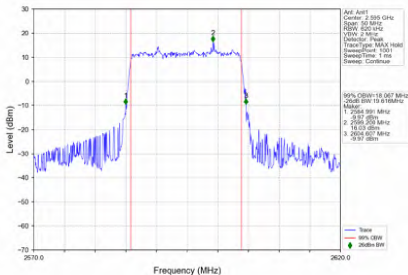
n38_30kHz_SISO_NTNV_20MHz_DFT-s-OFDM_PI/2_BPSK_2595MHz_Outer_Full
