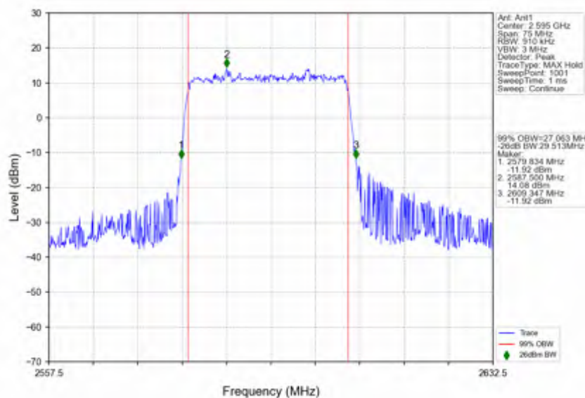
n38_30kHz_SISO_NTNV_30MHz_DFT-s-OFDM_PI/2_BPSK_2595MHz_Outer_Full
