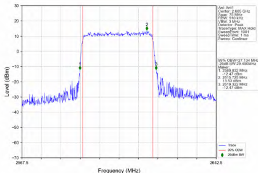
n38_30kHz_SISO_NTNV_30MHz_DFT-s-OFDM QPSK_2605MHz_Outer_Full
