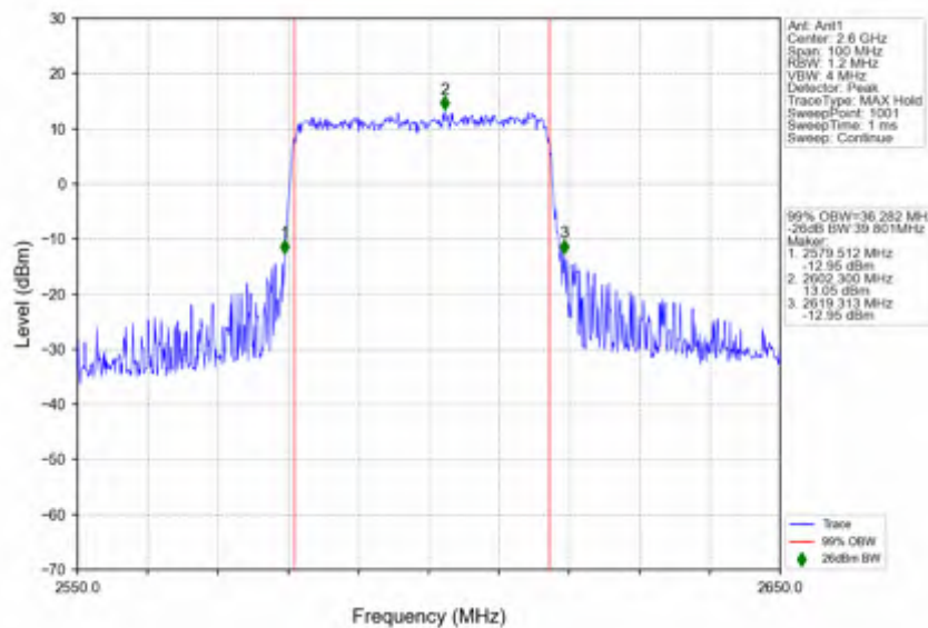
n38_30kHz_SISO_NTNV_40MHz_DFT-s-OFDM_QPSK_2600MHz_Outer_Full
