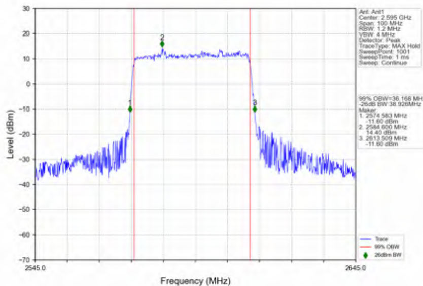
n38_30kHz_SISO_NTNV_40MHz_DFT-s-OFDM_PI/2_BPSK_2595MHz_Outer_Full
