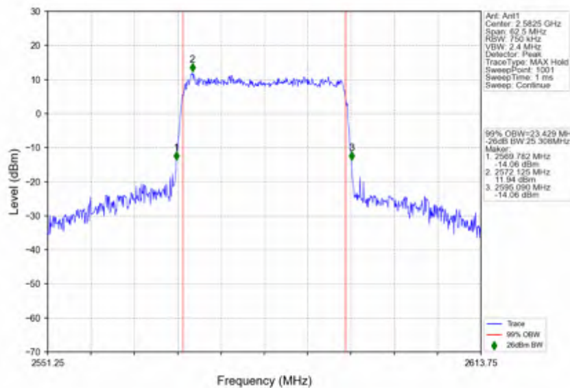
n38_30kHz_SISO_NTNV_25MHz_CP-OFDM_QPSK_2582.5MHz_Outer_Full
