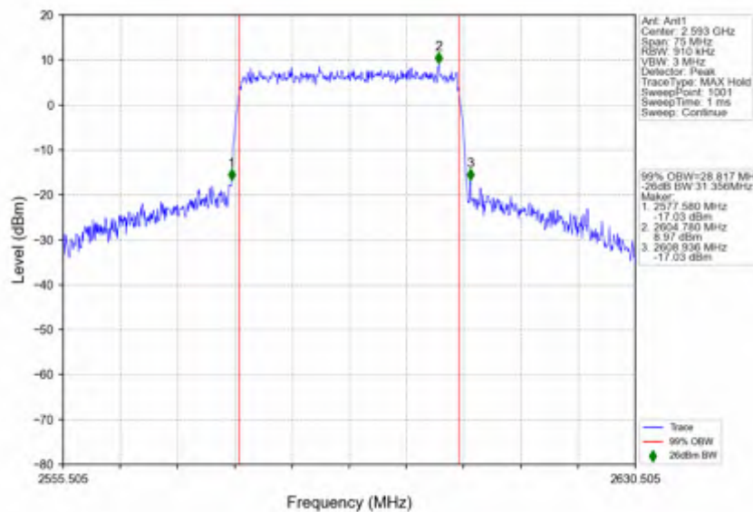
n41_15kHz_SISO_NTNV_30MHz_CP-OFDM 16 QAM_2593.005MHz_Outer_Full
