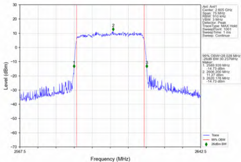
n38_30kHz_SISO_NTNV_30MHz_CP-OFDM 64 QAM_2605MHz_Outer_Full
