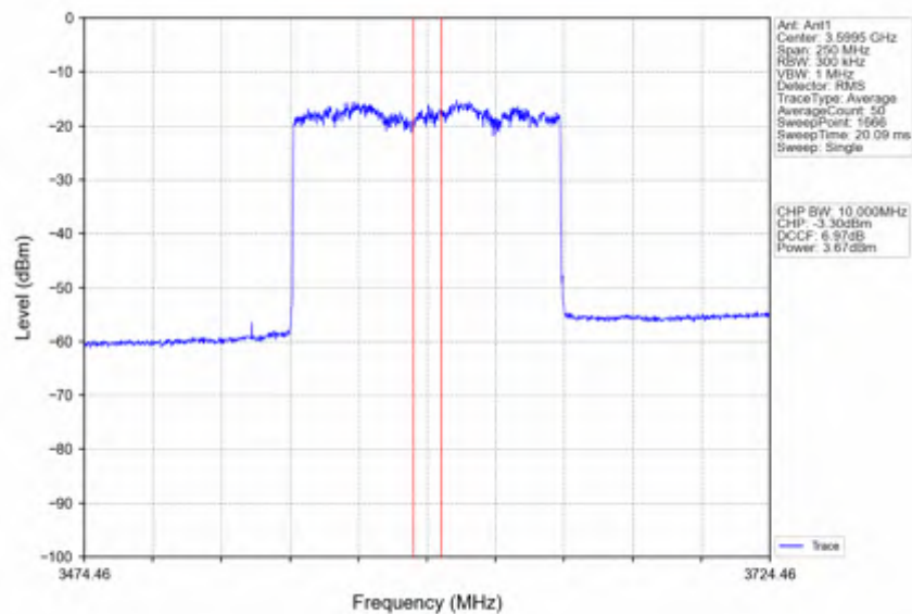
n78d_30kHz_SISO_NTNV_100MHz_DFT-s-OFDM_16_QAM_3600MHz_Inner_Full
