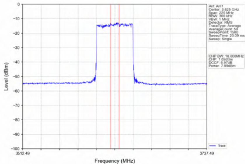
n78d_30kHz_SISO_NTNV_90MHz_CP-OFDM 64 QAM_3624.99MHz_Inner_Full
