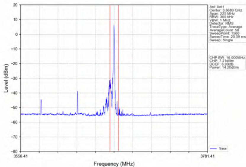
n78d_30kHz_SISO_NTNV_90MHz_CP-OFDM 256 QAM_3624.99MHz_Edge_1RB_Right
