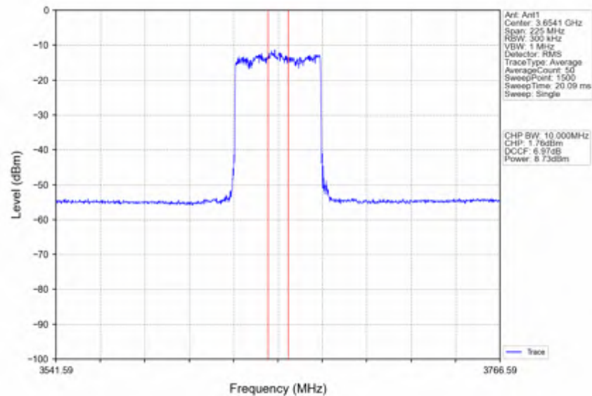
n78d_30kHz_SISO_NTNV_90MHz_DFT-s-OFDM_256_QAM_3654.99MHz_Inner_Full
