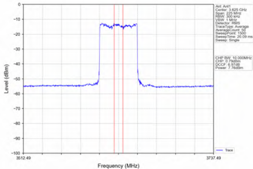
n78d_30kHz_SISO_NTNV_90MHz_CP-OFDM 256 QAM_3624.99MHz_Inner_Full
