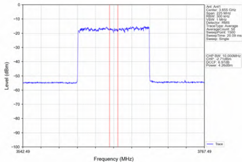
n78d 30kHz SISO NTNV 90MHz CP-OFDM 256 QAM 3654.99MHz Inner Full
