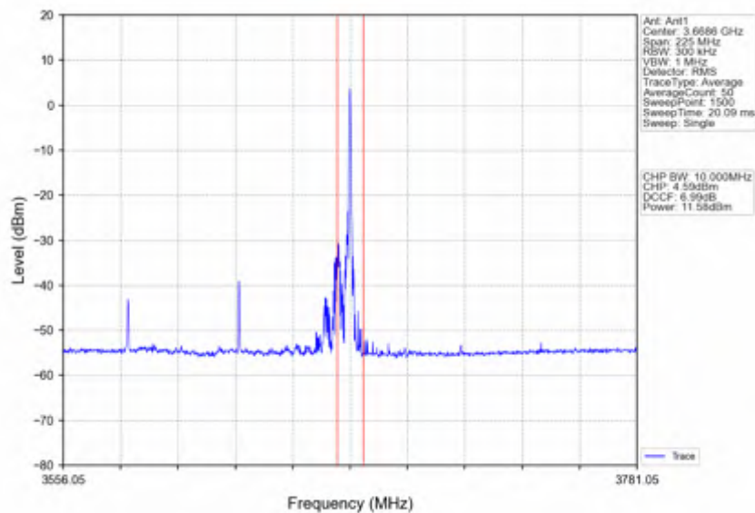
n78d_30kHz_SISO_NTV_90MHz_CP-OFDM QPSK_3624.99MHz_Inner_1RB_Right
