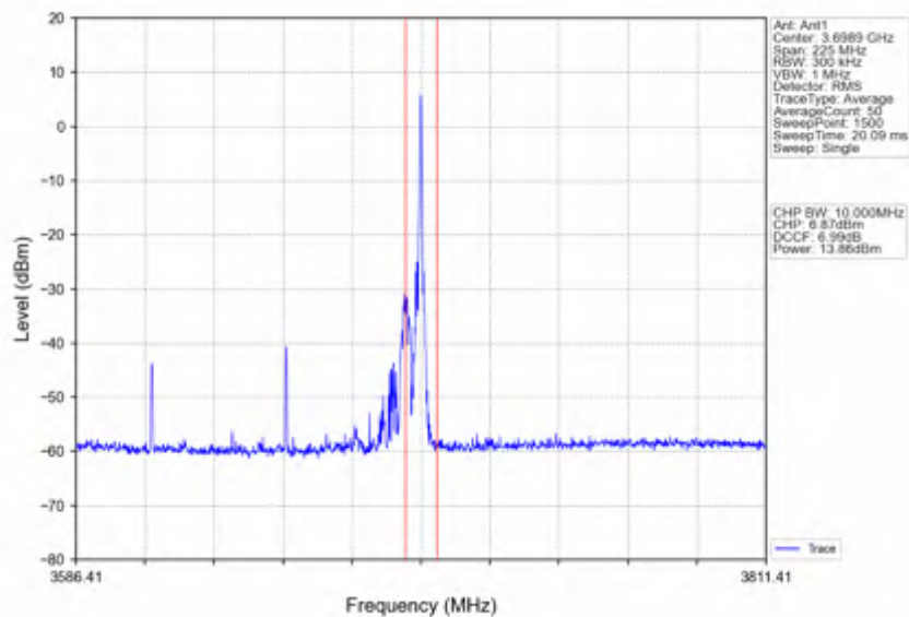
n78d_30kHz_SISO_NTNV_90MHz_CP-OFDM 64 QAM_3654.99MHz_Edge_1RB_Right
