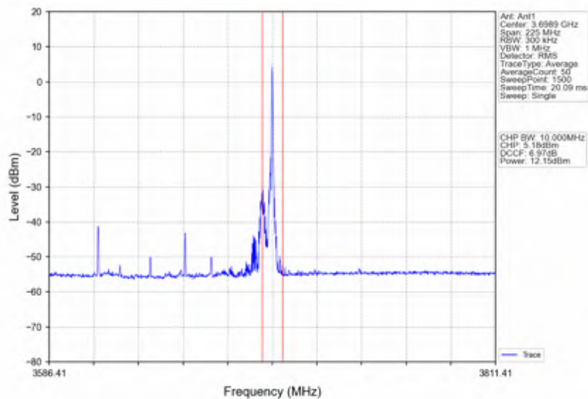
n78d_30kHz_SISO_NTNV_90MHz_DFT-s-OFDM_QPSK_3654.99MHz_Edge_1RB_Right
