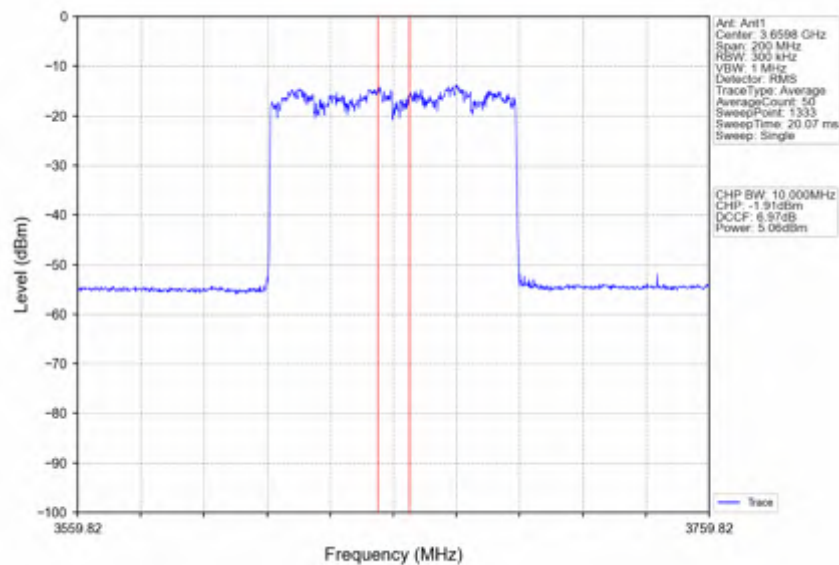
n78d_30kHz_SISO_NTNV_80MHz_DFT-s-OFDM_256_QAM_3660MHz_Inner_Full
