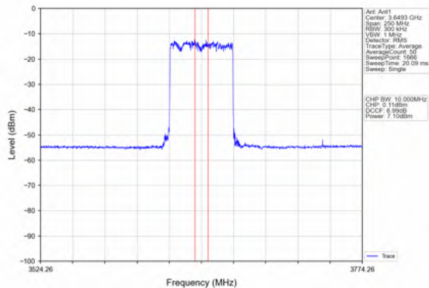
n78d_30kHz_SISO_NTNV_100MHz_DFT-s-OFDM_16_QAM_3649.98MHz_Inner_Full
