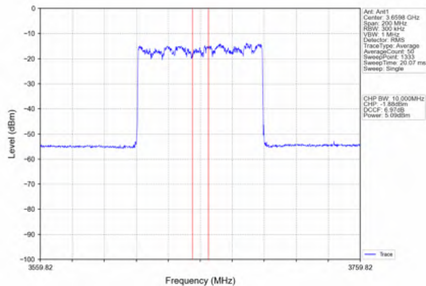
n78d_30kHz_SISO_NTNV_80MHz_DFT-s-OFDM 16 QAM_3660MHz_Inner_Full
