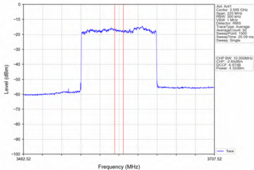
n78d_30kHz_SISO_NTNV_90MHz_CP-OFDM 64 QAM_3595.02MHz_Inner_Full
