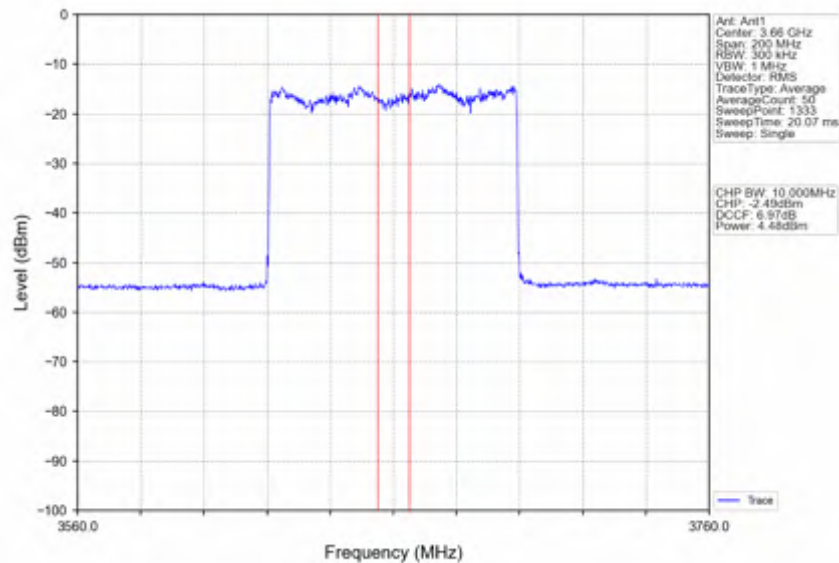
n78d_30kHz_SISO_NTNV_80MHz_CP-OFDM_256_QAM_3660MHz_Inner_Full
