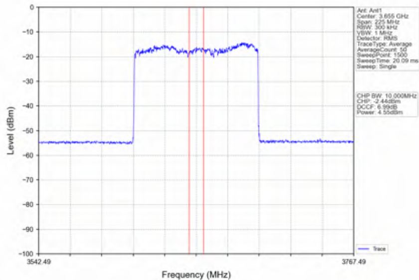
n78d_30kHz_SISO_NTNV_90MHz_CP-OFDM 64 QAM_3654.99MHz_Inner_Full
