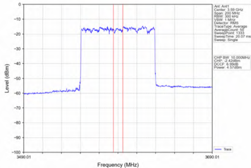
n78d_30kHz_SISO_NTNV_80MHz_CP-OFDM 16 QAM 3590.01MHz_Inner_Full
