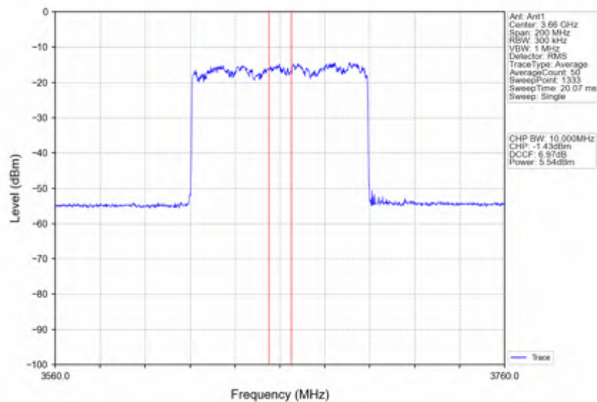
n78d 30kHz SISO NTV 80MHz CP-OFDM QPSK 3660MHz Inner Full
