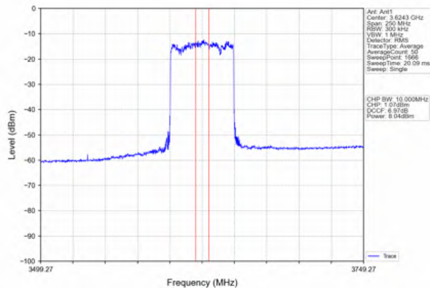
n78d 30kHz SISO NTNV 100MHz DFT-s-OFDM QPSK 3624.99MHz Inner Full
