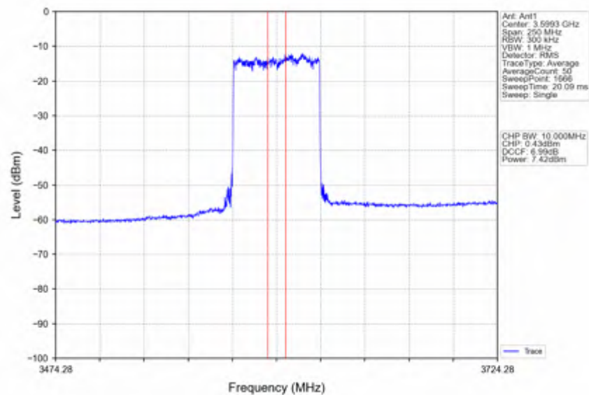
n78d_30kHz_SISO_NTNV_100MHz_DFT-s-OFDM_64_QAM_3600MHz_Inner_Full
