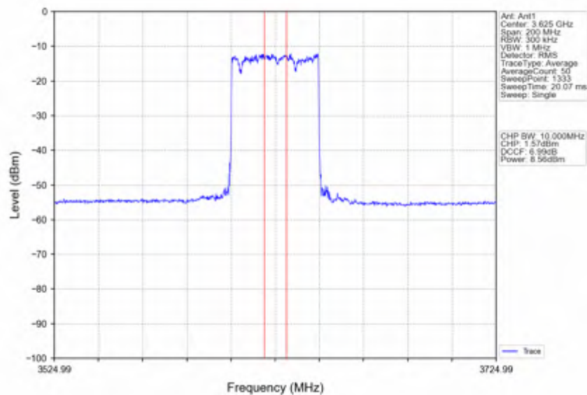
n78d_30kHz_SISO_NTNV_80MHz_CP-OFDM_256_QAM_3624.99MHz_Inner_Full
