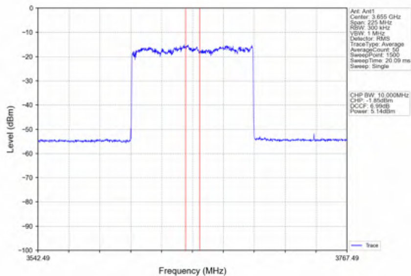
n78d_30kHz_SISO_NTNV_90MHz_CP-OFDM QPSK_3654.99MHz_Inner_Full
