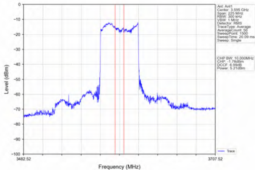
n78d_30kHz_SISO_NTNV_90MHz_CP-OFDM_256_QAM_3595.02MHz_Inner_Full
