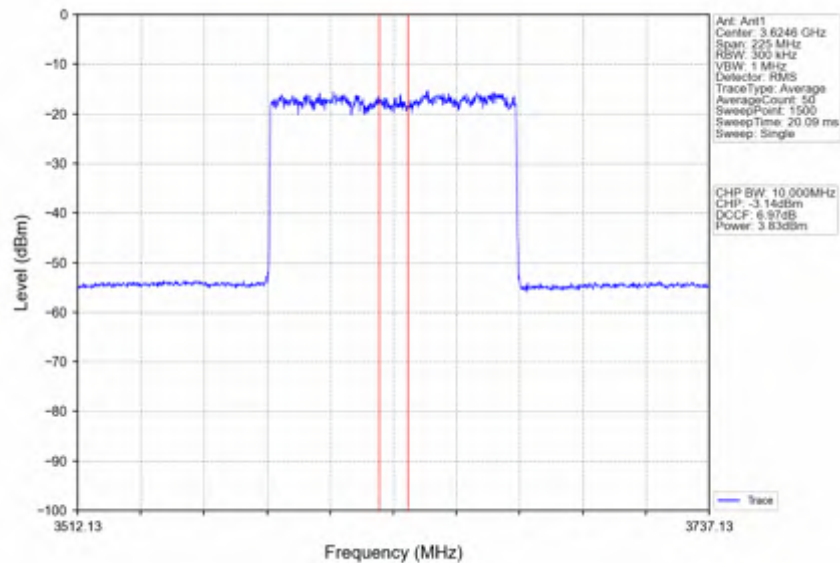
n78d_30kHz_SISO_NTNV_90MHz_DFT-s-OFDM_QPSK_3624.99MHz_Inner_Full
