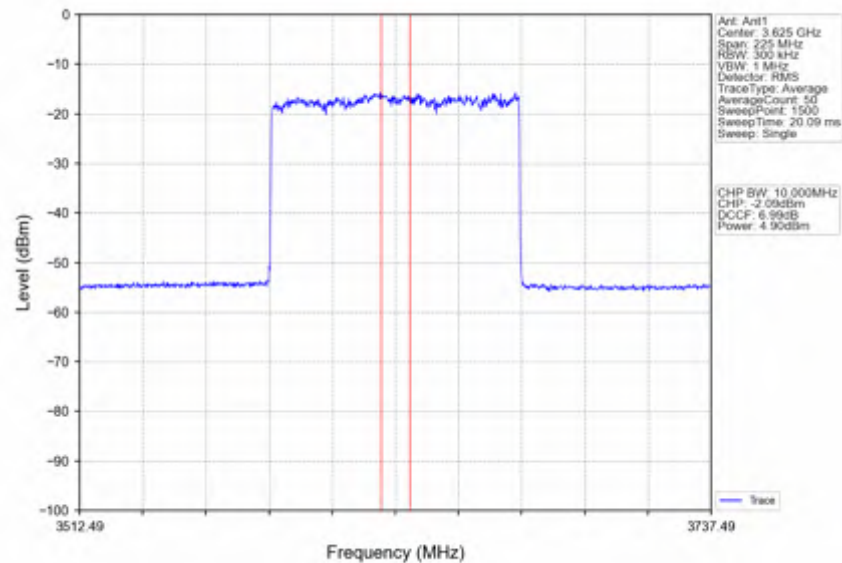
n78d_30kHz_SISO_NTNV_90MHz_CP-OFDM 16 QAM 3624.99MHz_Inner_Full
