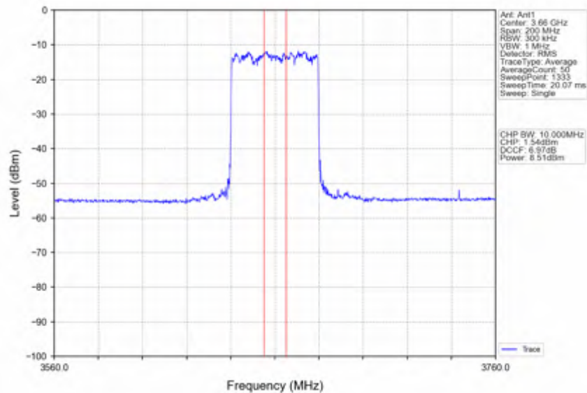
n78d_30kHz_SISO_NTNV_80MHz_CP-OFDM 16 QAM_3660MHz_Inner_Full
