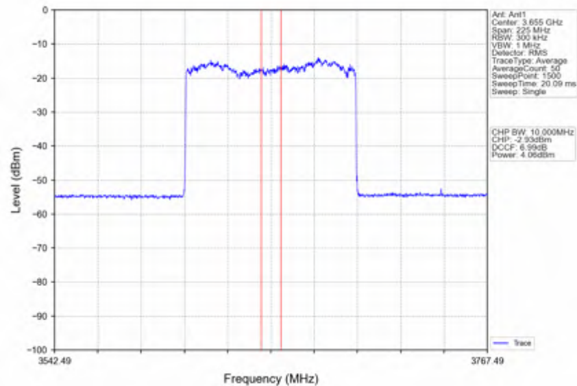
n78d_30kHz_SISO_NTNV_90MHz_CP-OFDM 16 QAM 3654.99MHz_Inner_Full
