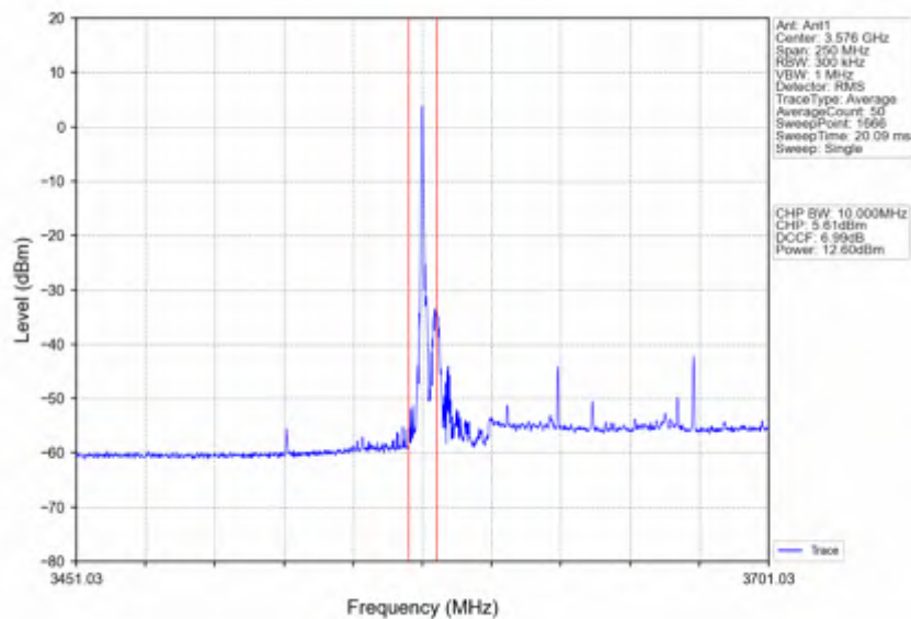
n78d_30kHz_SISO_NTNV_100MHz_DFT-s-OFDM QPSK_3624.99MHz_Edge_1RB_Right
