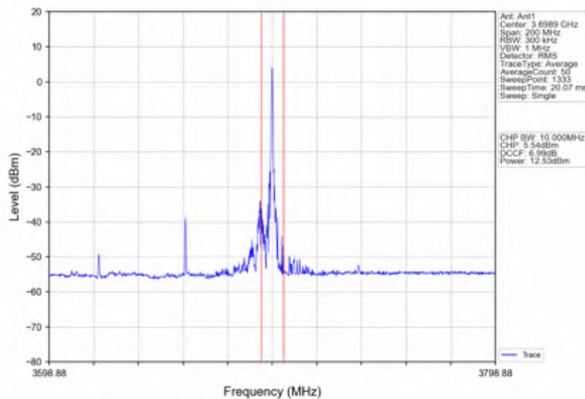
n78d_30kHz_SISO_NTNV_80MHz_CP-OFDM 256 QAM_3660MHz_Edge_1RB_Right
