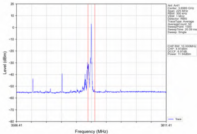
n78d_30kHz_SISO_NTNV_90MHz_CP-OFDM 16 QAM_3654.99MHz_Edge_1RB_Right
