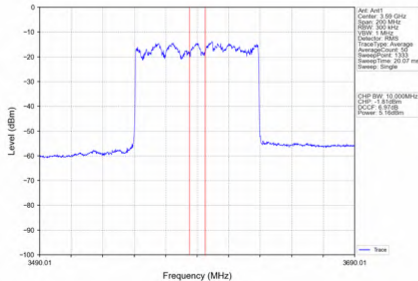
n78d_30kHz_SISO_NTNV_80MHz_CP-OFDM_256_QAM_3590.01MHz_Inner_Full
