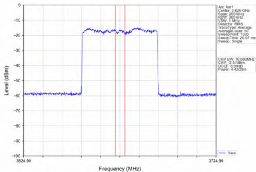
n78d_30kHz_SISO_NTNV_80MHz_CP-OFDM 16 QAM 3624.99MHz_Inner_Full
