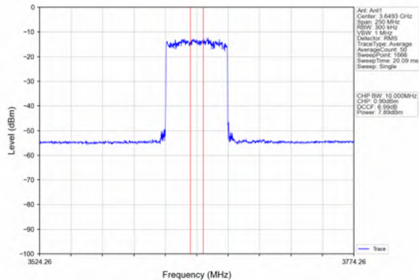
n78d_30kHz_SISO_NTNV_100MHz_DFT-s-OFDM QPSK_3649.98MHz_Inner_Full
