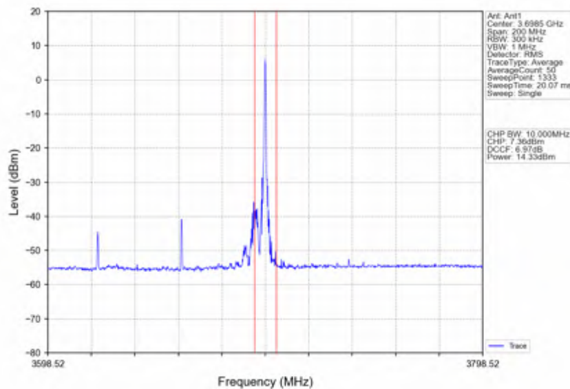
n78d_30kHz_SISO_NTNV_80MHz_CP-OFDM_QPSK_3660MHz_Inner_1RB_Right
