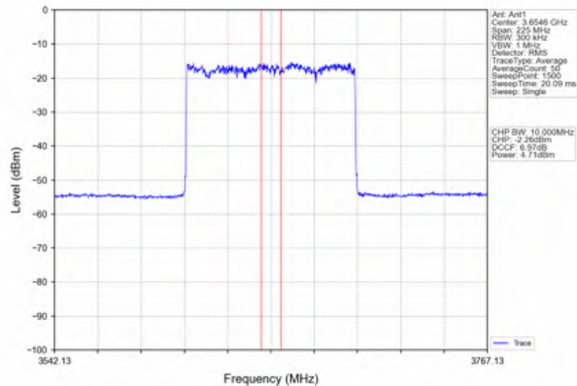
n78d_30kHz_SISO_NTNV_90MHz_DFT-s-OFDM PI/2 BPSK_3654.99MHz_Inner_Full
