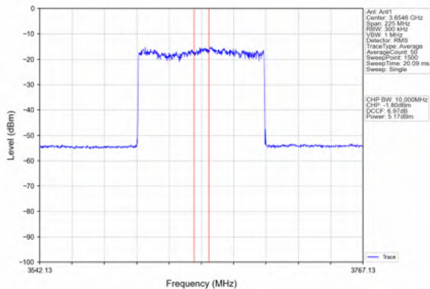
n78d_30kHz_SISO_NTNV_90MHz_DFT-s-OFDM QPSK_3654.99MHz_Inner_Full
