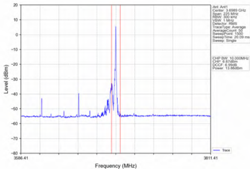
n78d_30kHz_SISO_NTNV_90MHz_DFT-s-OFDM_64_QAM_3654.99MHz_Edge_1RB_Right
