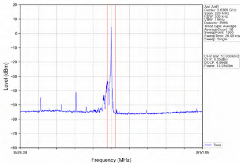
n78d_30kHz_SISO_NTNV_90MHz_DFT-s-OFDM 16 QAM_3595.02MHz_Inner_1RB_Right
