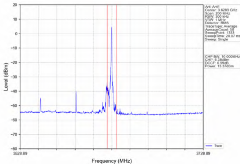
n78d_30kHz_SISO_NTNV_80MHz_DFT-s-OFDM 64 QAM_3590.01MHz_Edge_1RB_Right
