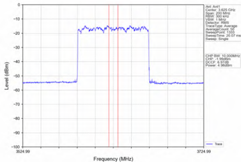
n78d_30kHz_SISO_NTNV_80MHz_CP-OFDM QPSK_3624.99MHz_Inner_Full
