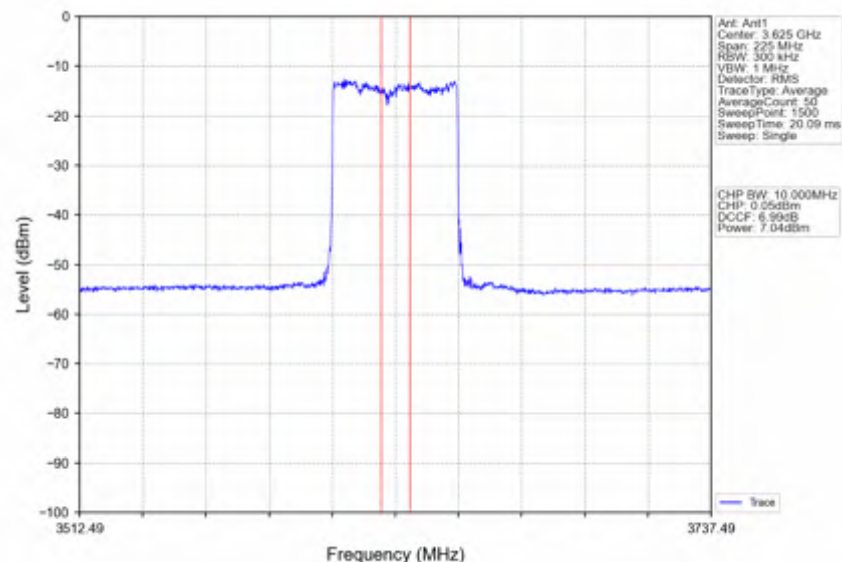
n78d 30kHz SISO NTNV 90MHz CP-OFDM QPSK 3624.99MHz Inner Full
