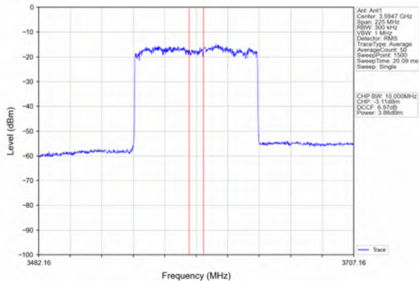
n78d_30kHz_SISO_NTNV_90MHz_DFT-s-OFDM_QPSK_3595.02MHz_Inner_Full
