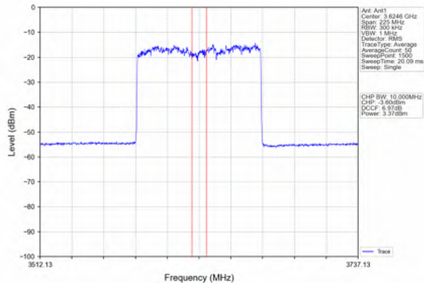
n78d_30kHz_SISO_NTNV_90MHz_DFT-s-OFDM_256_QAM_3624.99MHz_Inner_Full
