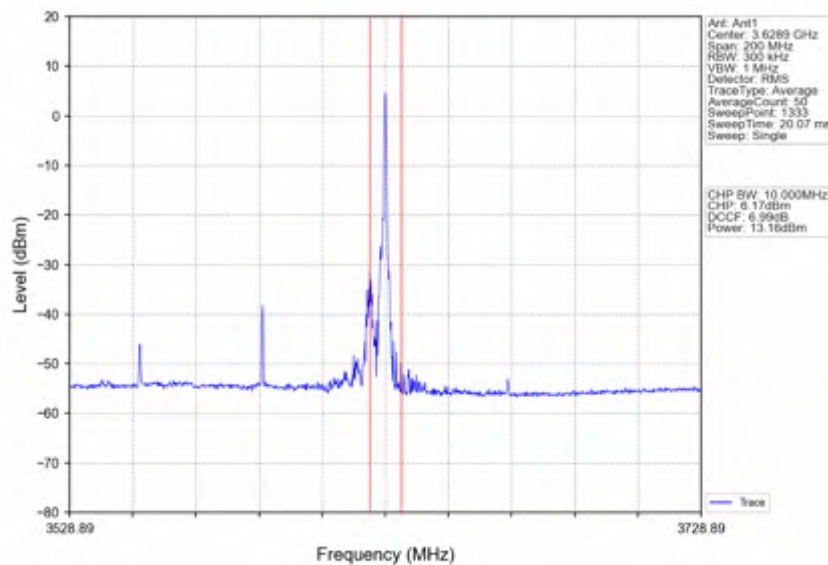
n78d_30kHz_SISO_NTNV_80MHz_CP-OFDM_64_QAM_3590.01MHz_Edge_1RB_Right
