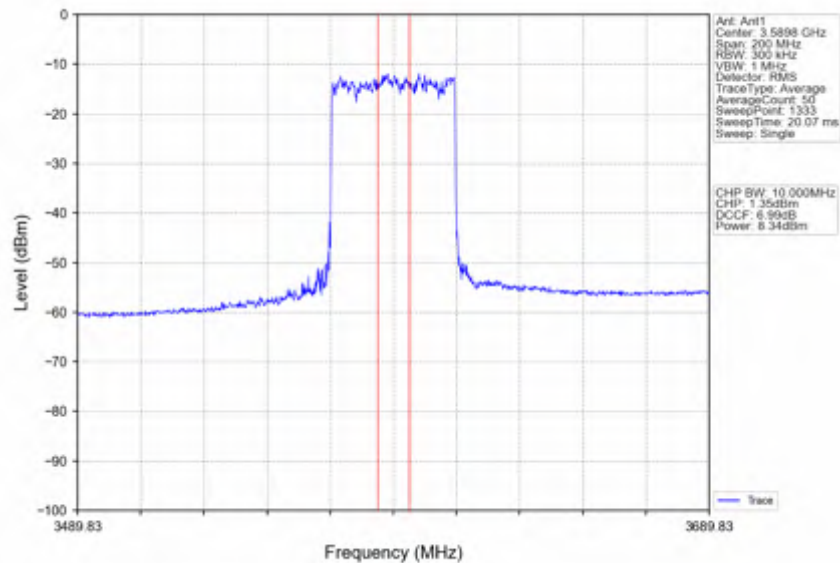
n78d_30kHz_SISO_NTNV_80MHz_DFT-s-OFDM_QPSK_3590.01MHz_Inner_Full
