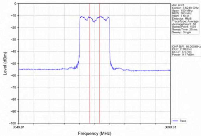
n78d_30kHz_SISO_NTNV_60MHz_CP-OFDM 16 QAM 3624.99MHz_Inner_Full
