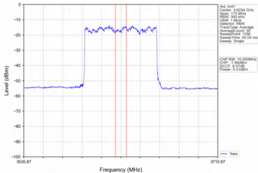
n78d_30kHz_SISO_NTNV_70MHz_DFT-s-OFDM_QPSK_3624.99MHz_Inner_Full
