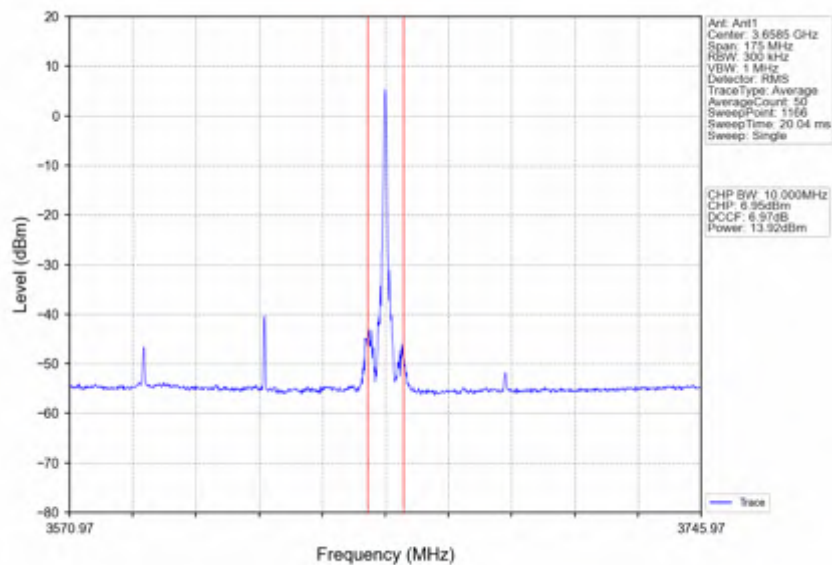
n78d_30kHz_SISO_NTNV_70MHz_CP-OFDM 16 QAM_3624.99MHz_Inner_1RB_Right
