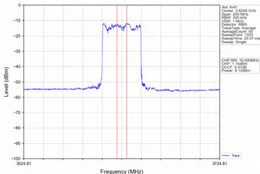
n78d 30kHz SISO NTNV 80MHz DFT-s-OFDM QPSK 3624.99MHz Inner Full
