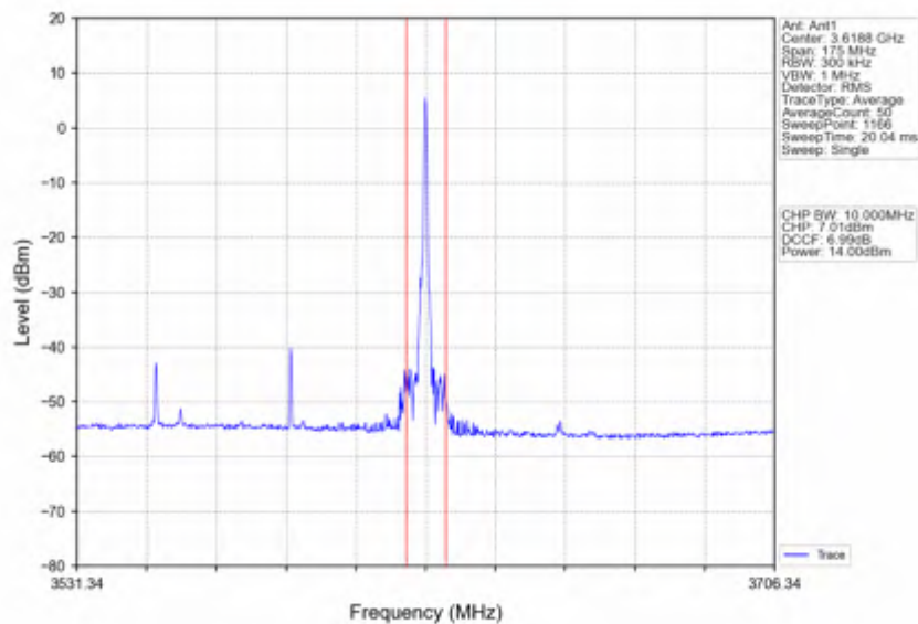
n78d_30kHz_SISO_NTNV_70MHz_DFT-s-OFDM_16_QAM_3585MHz_Edge_1RB_Right
