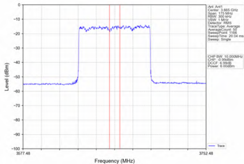
n78d 30kHz SISO NTNV 70MHz CP-OFDM 256 QAM 3664.98MHz Inner Full
