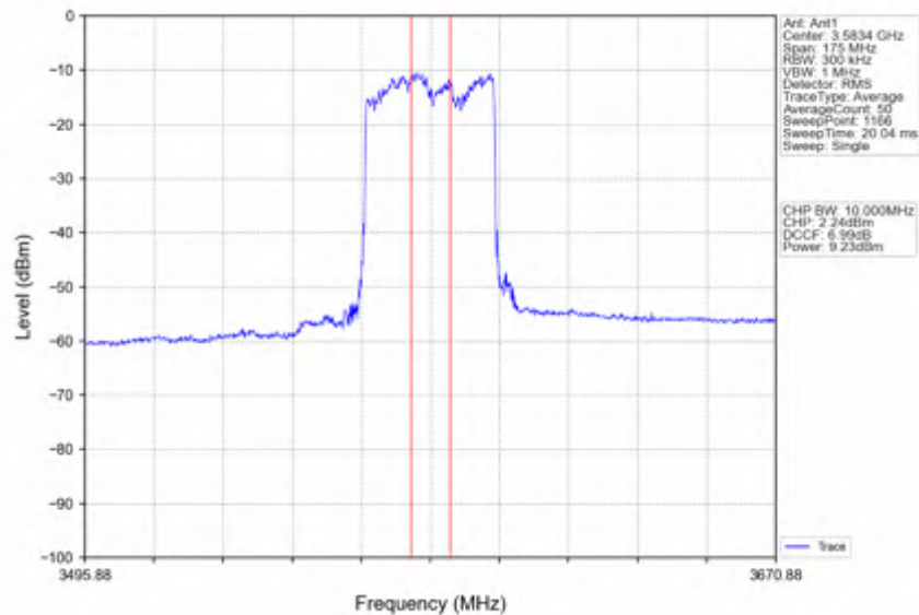
n78d_30kHz_SISO_NTNV_70MHz_DFT-s-OFDM_256_QAM_3585MHz_Inner_Full
