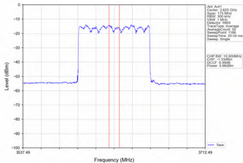
n78d_30kHz_SISO_NTNV_70MHz_CP-OFDM 16 QAM 3624.99MHz_Inner_Full
