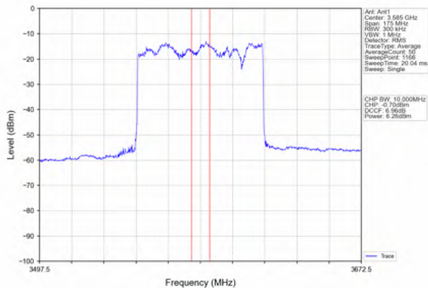
n78d 30kHz SISO NTN 70MHz CP-OFDM 256 QAM 3585MHz Inner Full
