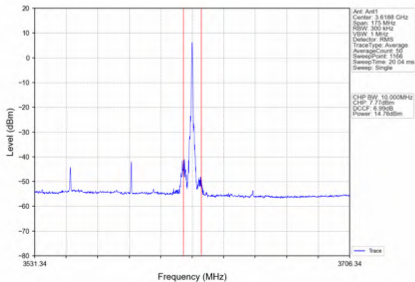
n78d_30kHz_SISO_NTNV_70MHz_CP-OFDM QPSK_3585MHz_Edge_1RB_Right
