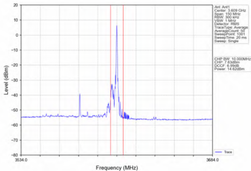
n78d_30kHz_SISO_NTNV_60MHz_DFT-s-OFDM_256_QAM_3580.02MHz_Edge_1RB_Right
