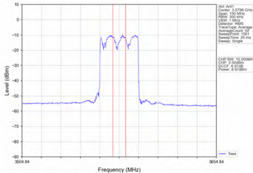
n78d_30kHz_SISO_NTNV_60MHz_CP-OFDM 64 QAM_3580.02MHz_Inner_Full
