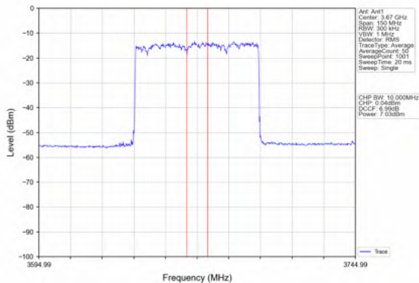
n78d_30kHz_SISO_NTNV_60MHz_CP-OFDM_256_QAM_3669.99MHz_Inner_Full
