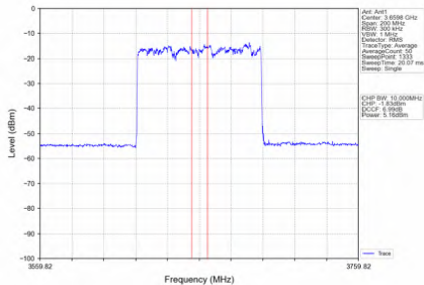
n78d_30kHz_SISO_NTNV_80MHz_DFT-s-OFDM QPSK_3660MHz_Inner_Full
