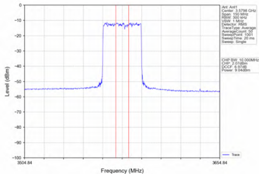
n78d_30kHz_SISO_NTNV_60MHz_DFT-s-OFDM_256_QAM_3580.02MHz_Inner_Full
