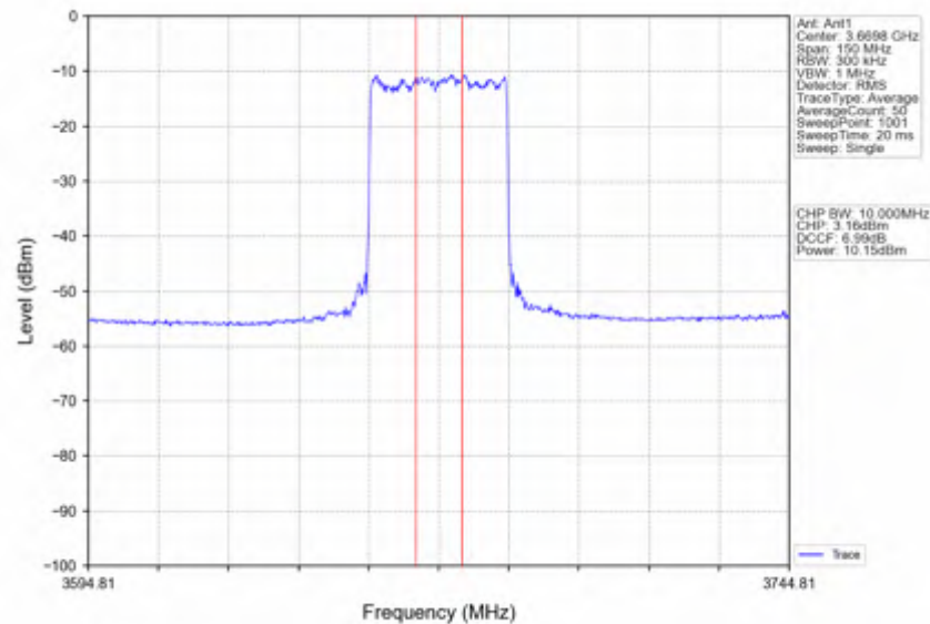
n78d_30kHz_SISO_NTNV_60MHz_CP-OFDM 64 QAM_3669.99MHz_Inner_Full
