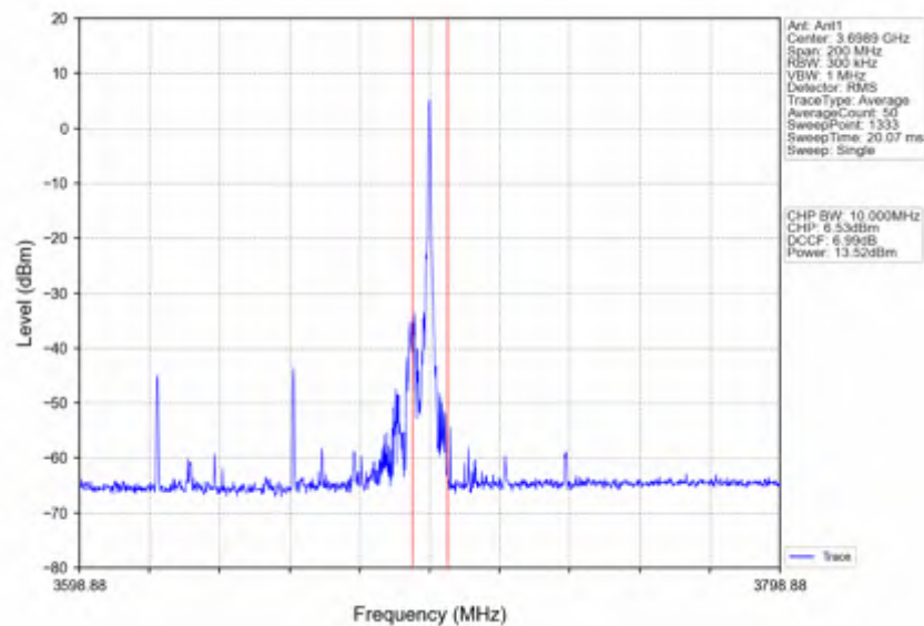
n78d_30kHz_SISO_NTNV_80MHz_DFT-s-OFDM PI/2 BPSK_3660MHz_Edge_1RB_Right
