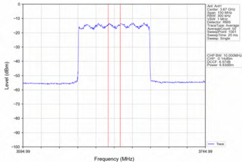
n78d_30kHz_SISO_NTNV_60MHz_CP-OFDM 16 QAM 3669.99MHz_Inner_Full
