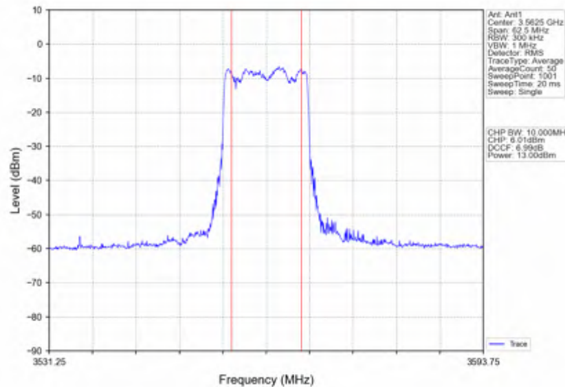
n78d_30kHz_SISO_NTNV_25MHz_CP-OFDM_16_QAM_3562.5MHz_Inner_Full
