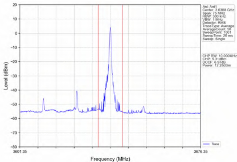
n78d_30kHz_SISO_NTNV_30MHz_CP-OFDM QPSK_3624.99MHz_Edge_1RB_Right
