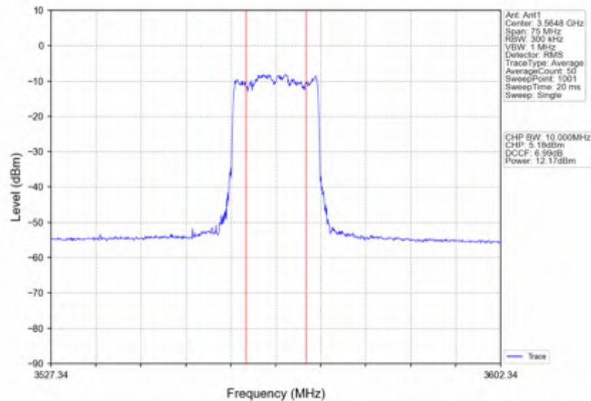
n78d_30kHz_SISO_NTNV_30MHz_CP-OFDM QPSK_3565.02MHz_Inner_Full
