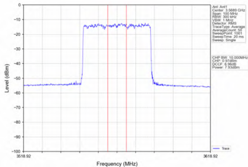
n78d_30kHz_SISO_NTNV_40MHz_DFT-s-OFDM QPSK_3570MHz_Inner_Full
