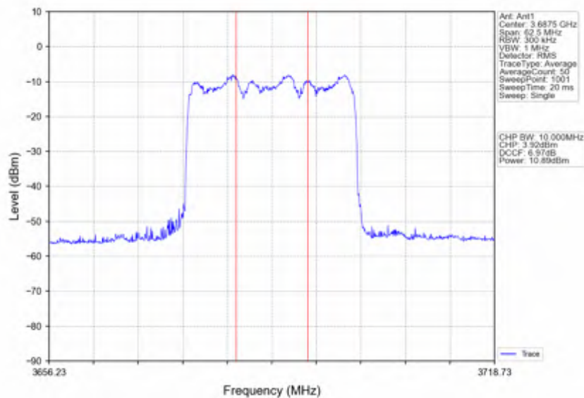
n78d_30kHz_SISO_NTNV_25MHz_CP-OFDM QPSK_3687.48MHz_Inner_Full
