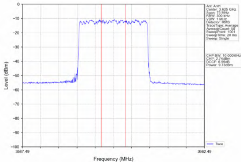
n78d_30kHz_SISO_NTNV_30MHz_CP-OFDM_256_QAM_3624.99MHz_Inner_Full
