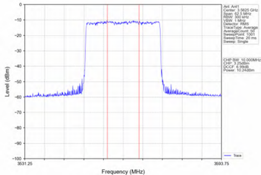
n78d_30kHz_SISO_NTNV_25MHz_CP-OFDM_16_QAM_3562.5MHz_Inner_Full
