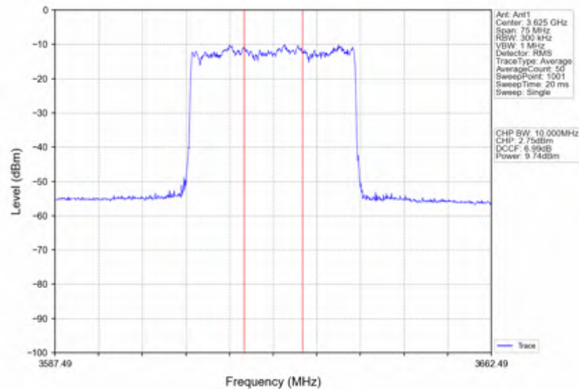
n78d_30kHz_SISO_NTNV_30MHz_CP-OFDM 64 QAM_3624.99MHz_Inner_Full
