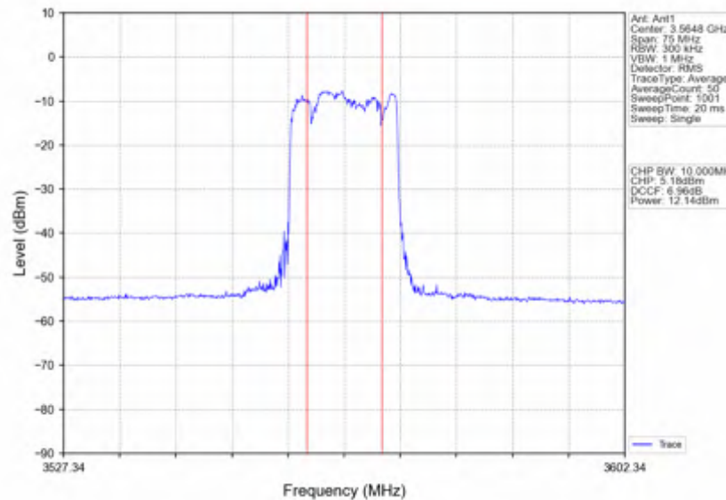
n78d_30kHz_SISO_NTNV_30MHz_CP-OFDM 16 QAM_3565.02MHz_Inner_Full
