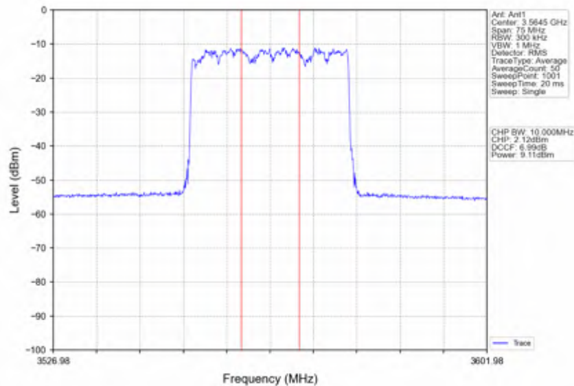
n78d_30kHz_SISO_NTNV_30MHz_DFT-s-OFDM_QPSK_3565.02MHz_Inner_Full
