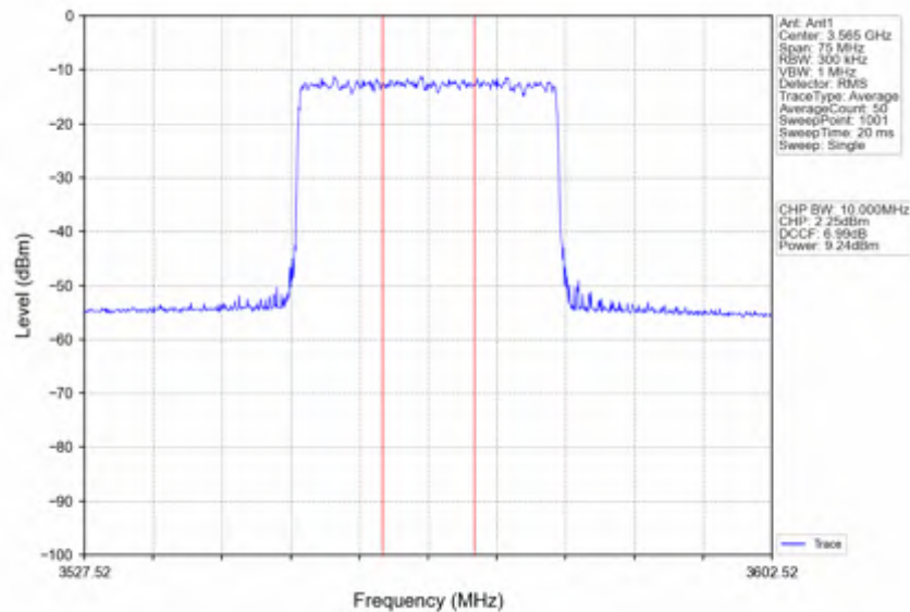
n78d_30kHz_SISO_NTNV_30MHz_CP-OFDM QPSK_3565.02MHz_Inner_Full
