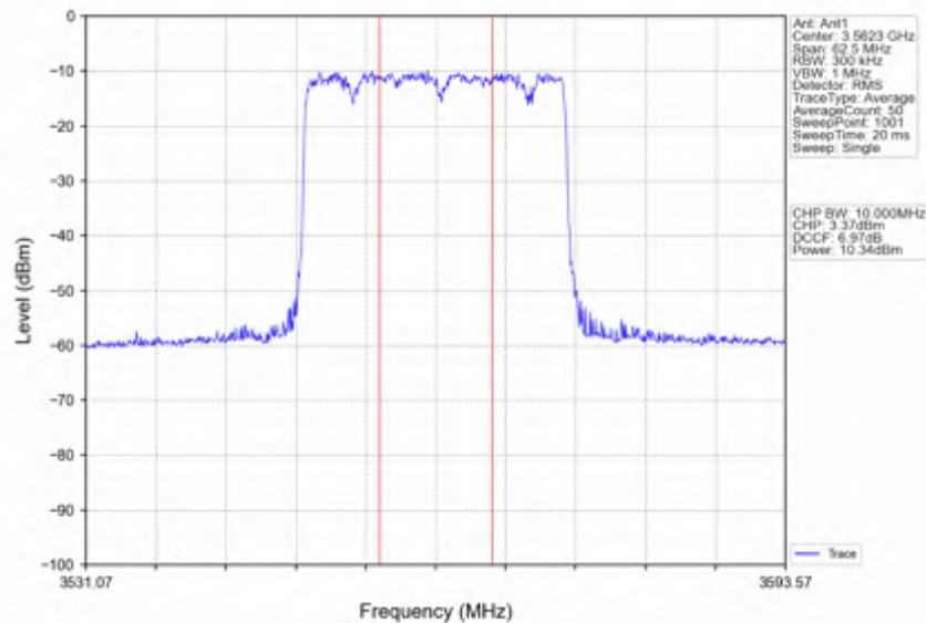
n78d_30kHz_SISO_NTNV_25MHz_DFT-s-OFDM 64 QAM_3562.5MHz_Inner_Full
