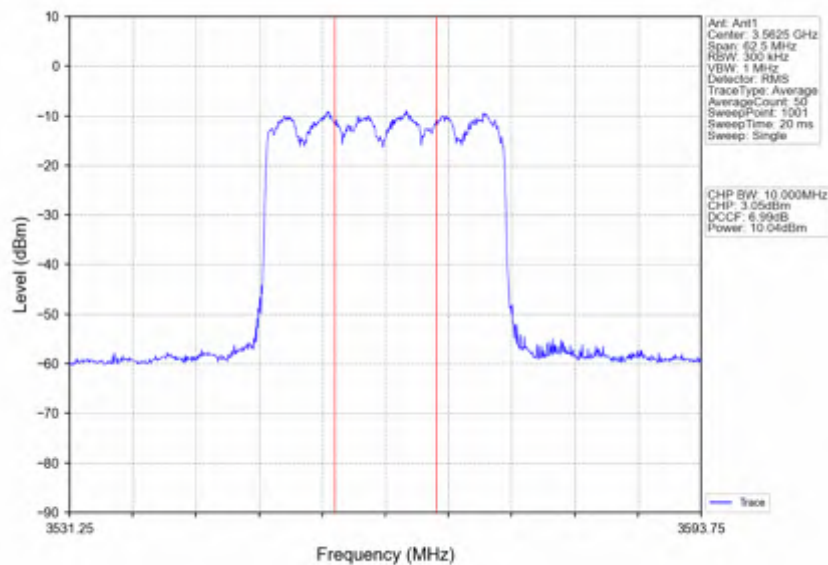
n78d_30kHz_SISO_NTNV_25MHz_CP-OFDM 64 QAM_3562.5MHz_Inner_Full
