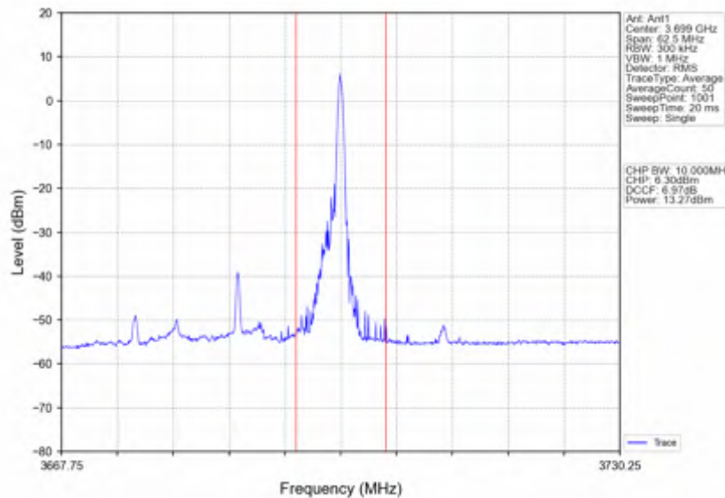
n78d_30kHz_SISO_NTNV_25MHz_CP-OFDM QPSK_3687.48MHz_Edge_1RB_Right
