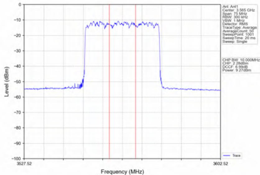
n78d_30kHz_SISO_NTNV_30MHz_CP-OFDM_256_QAM_3565.02MHz_Inner_Full
