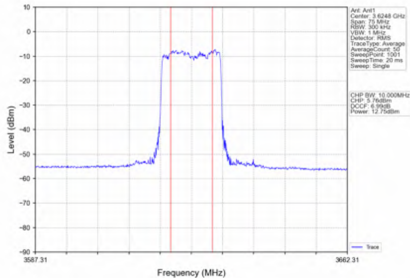
n78d_30kHz_SISO_NTNV_30MHz_CP-OFDM 64 QAM_3624.99MHz_Inner_Full
