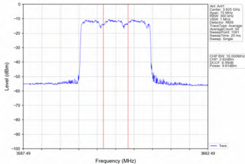
n78d_30kHz_SISO_NTNV_30MHz_CP-OFDM_QPSK_3624.99MHz_Inner_Full
