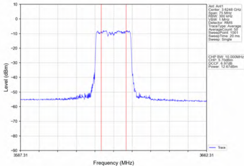
n78d_30kHz_SISO_NTNV_30MHz_CP-OFDM_256_QAM_3624.99MHz_Inner_Full
