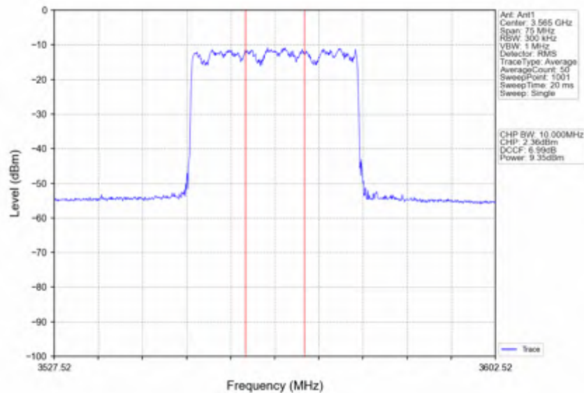
n78d_30kHz_SISO_NTNV_30MHz_CP-OFDM 16 QAM_3565.02MHz_Inner_Full
