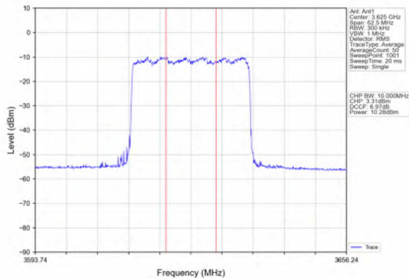
n78d_30kHz_SISO_NTNV_25MHz_CP-OFDM 256 QAM_3624.99MHz_Inner_Full
