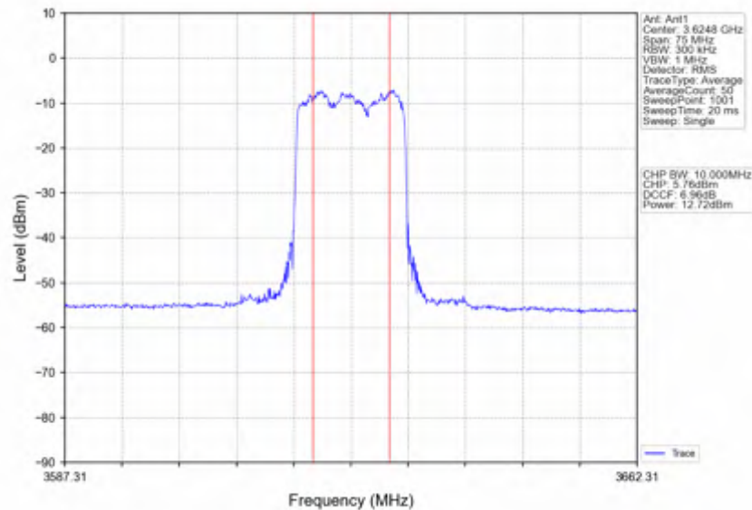
n78d_30kHz_SISO_NTNV_30MHz_CP-OFDM_QPSK_3624.99MHz_Inner_Full
