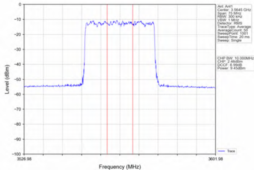
n78d_30kHz_SISO_NTNV_30MHz_DFT-s-OFDM_256_QAM_3565.02MHz_Inner_Full
