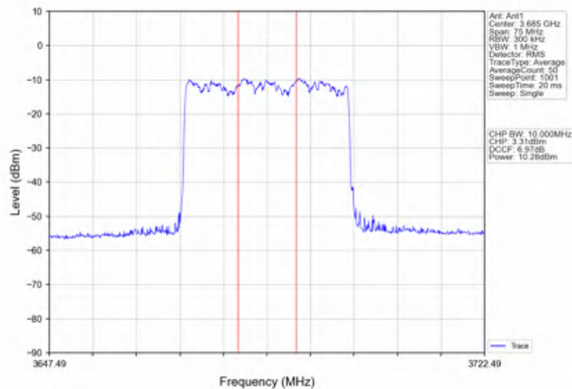
n78d_30kHz_SISO_NTNV_30MHz_CP-OFDM QPSK_3684.99MHz_Inner_Full
