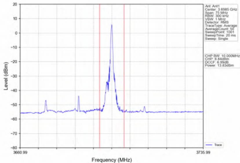
n78d_30kHz_SISO_NTNV_30MHz_CP-OFDM 16 QAM_3684.99MHz_Inner_1RB_Right
