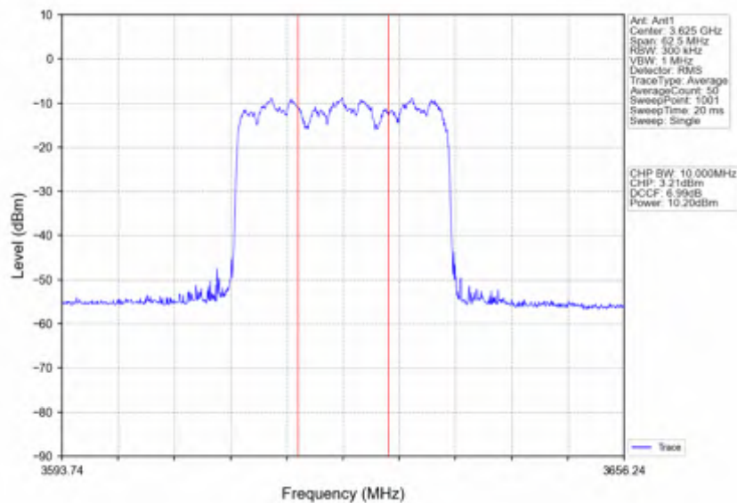
n78d_30kHz_SISO_NTNV_25MHz_CP-OFDM QPSK_3624.99MHz_Inner_Full
