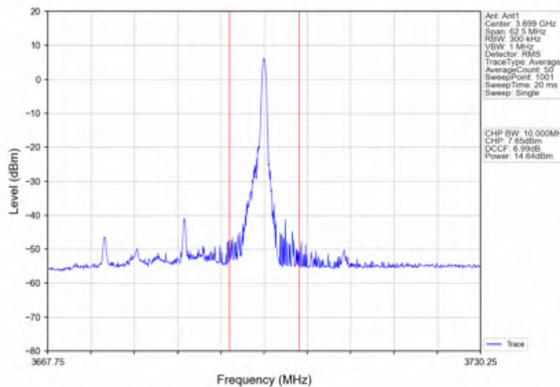
n78d_30kHz_SISO_NTNV_25MHz_CP-OFDM 64 QAM_3687.48MHz_Edge_1RB_Right
