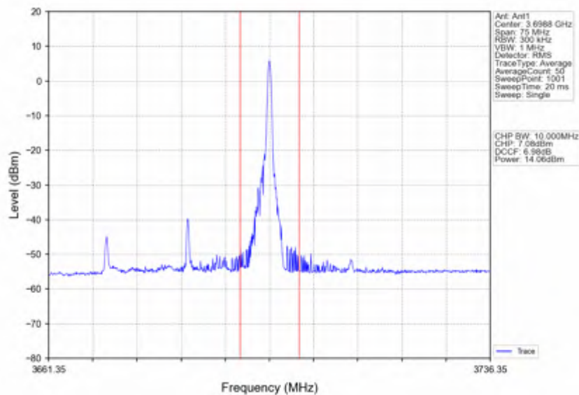
n78d_30kHz_SISO_NTNV_30MHz_CP-OFDM_64_QAM_3684.99MHz_Edge_1RB_Right
