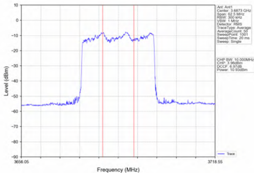
n78d_30kHz_SISO_NTNV_25MHz_DFT-s-OFDM_QPSK_3687.48MHz_Inner_Full
