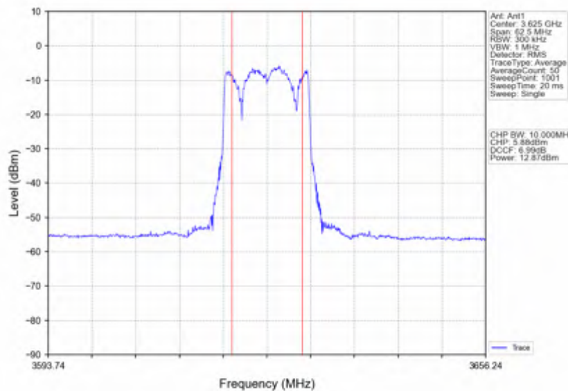
n78d_30kHz_SISO_NTNV_25MHz_CP-OFDM QPSK_3624.99MHz_Inner_Full
