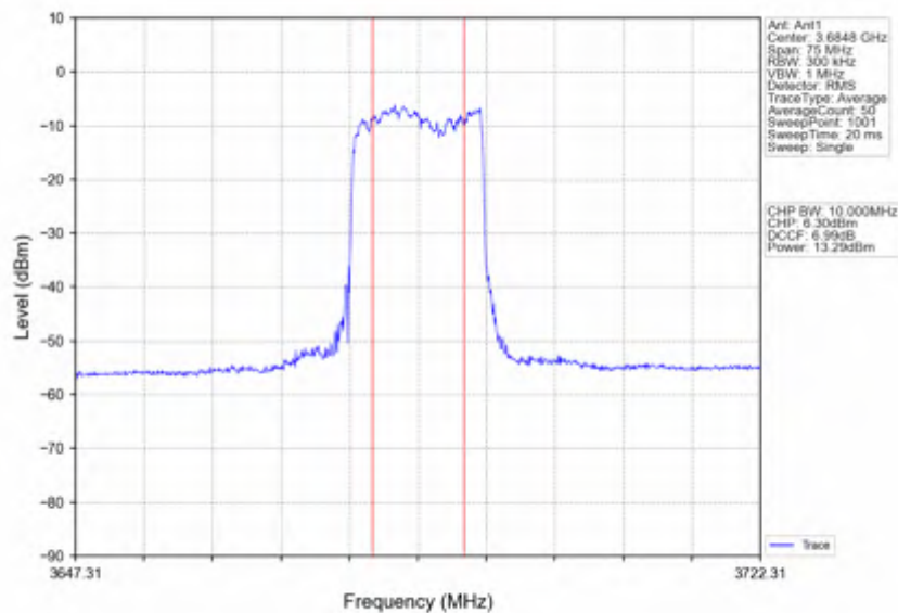
n78d_30kHz_SISO_NTNV_30MHz_CP-OFDM 16 QAM_3684.99MHz_Inner_Full
