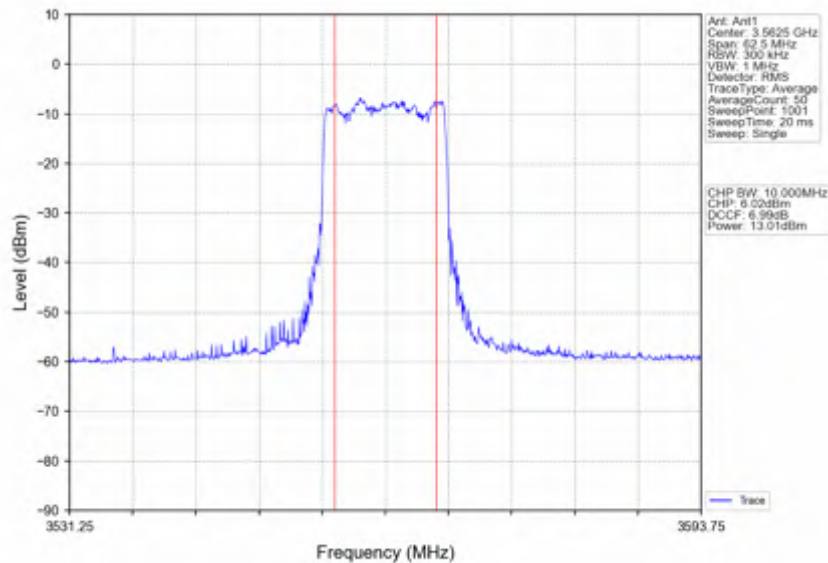
n78d_30kHz_SISO_NTNV_25MHz_CP-OFDM 256 QAM_3562.5MHz_Inner_Full
