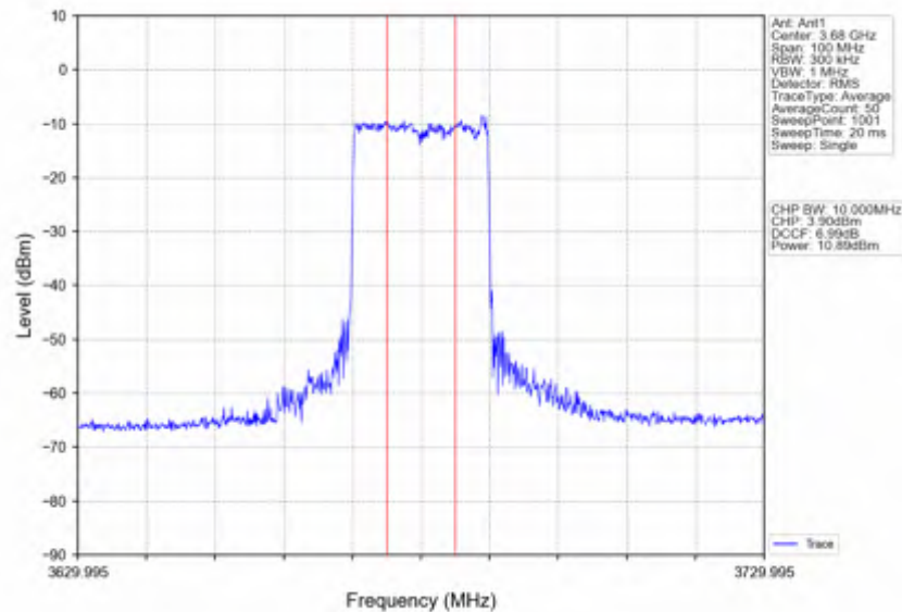
n78d_15kHz_SISO_NTNV_40MHz_DFT-s-OFDM QPSK 3679.995MHz_Inner_Full
