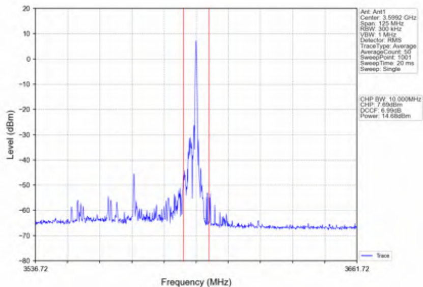
n78d_15kHz_SISO_NTNV_50MHz_DFT-s-OFDM PI/2 BPSK_3575.01MHz_Edge_1RB_Right
