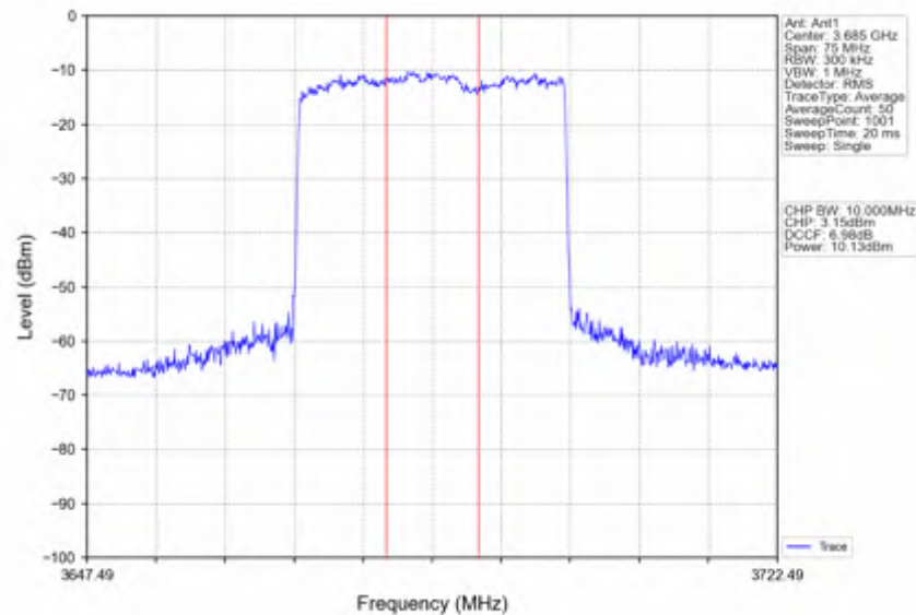
n78d_15kHz_SISO_NTNV_30MHz_CP-OFDM 64 QAM_3684.99MHz_Inner_Full
