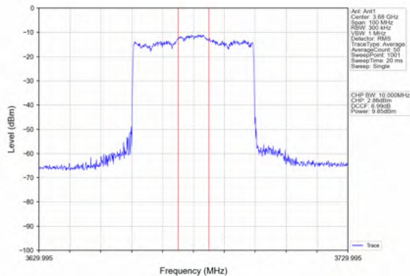
n78d_15kHz_SISO_NTNV_40MHz_CP-OFDM QPSK_3679.995MHz_Inner_Full
