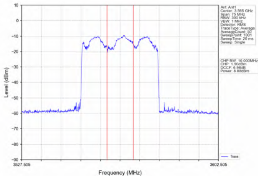
n78d_15kHz_SISO_NTNV_30MHz_CP-OFDM 256 QAM_3565.005MHz_Inner_Full
