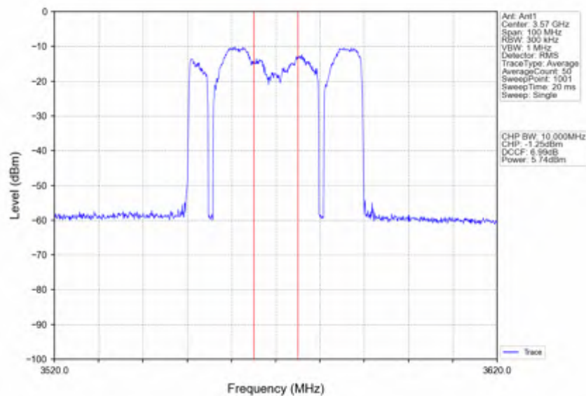
n78d 15kHz SISO NTV 40MHz CP-OFDM QPSK 3570MHz Inner Full
