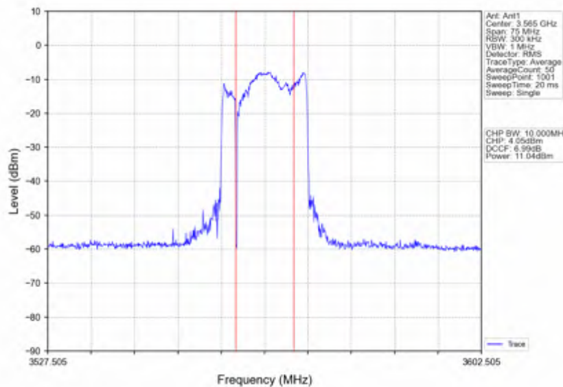
n78d 15kHz SISO NTNV 30MHz CP-OFDM 16 QAM 3565.005MHz Inner Full
