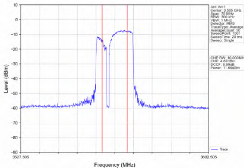
n78d_15kHz_SISO_NTNV_30MHz_CP-OFDM 256 QAM_3565.005MHz_Inner_Full
