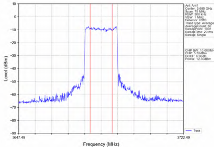
n78d_15kHz_SISO_NTNV_30MHz_CP-OFDM_QPSK_3684.99MHz_Inner_Full
