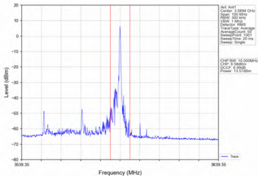
n78d_15kHz_SISO_NTNV_40MHz_CP-OFDM 64 QAM_3570MHz_Edge_1RB_Right
