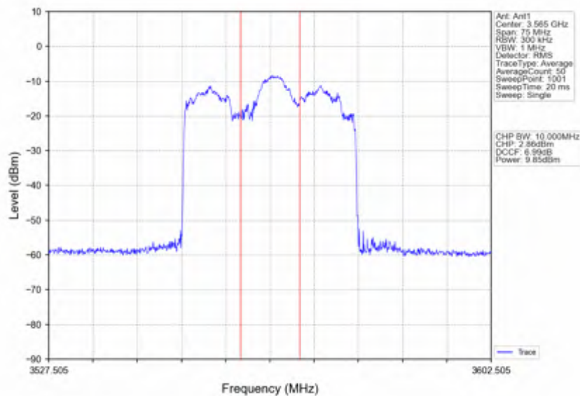
n78d 15kHz SISO NTNV 30MHz CP-OFDM 16 QAM 3565.005MHz Inner Full
