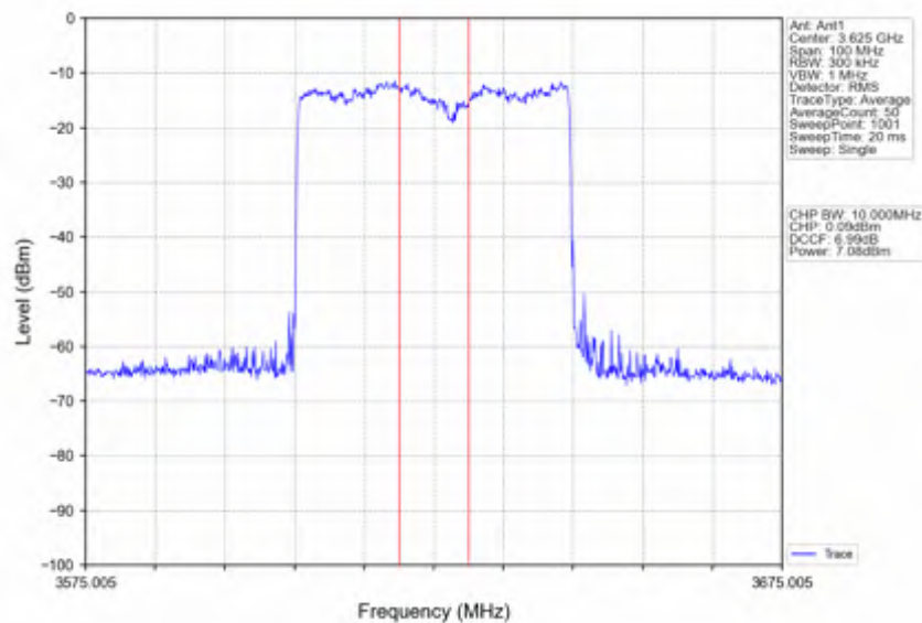
n78d_15kHz_SISO_NTNV_40MHz_CP-OFDM 64 QAM_3625.005MHz_Inner_Full
