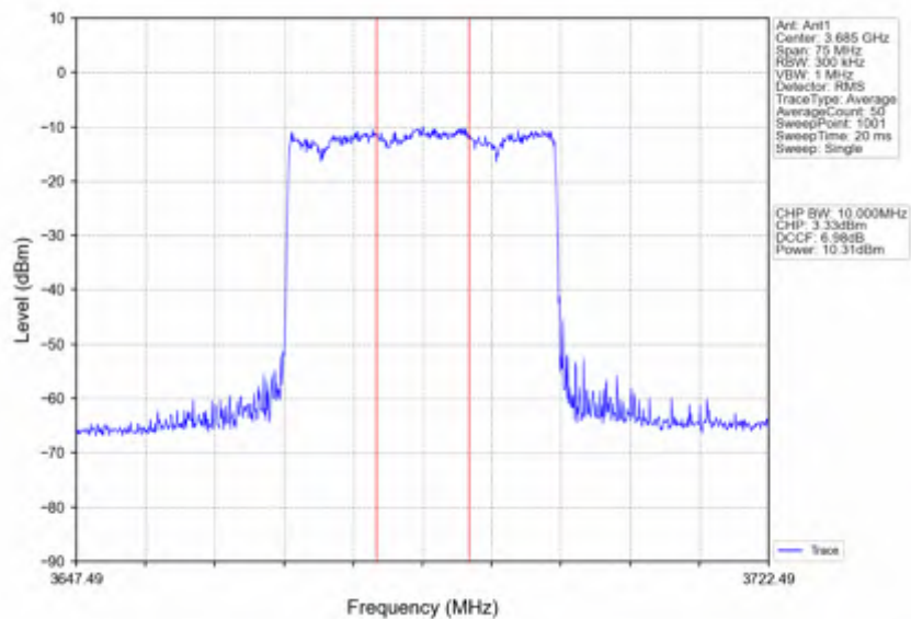
n78d_15kHz_SISO_NTNV_30MHz_DFT-s-OFDM_16 QAM_3684.99MHz_Inner_Full
