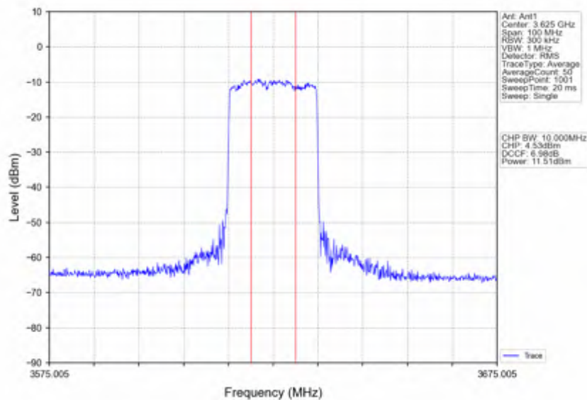
n78d_15kHz_SISO_NTNV_40MHz_CP-OFDM 64 QAM_3625.005MHz_Inner_Full
