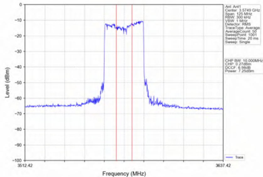
n78d_15kHz_SISO_NTNV_50MHz_DFT-s-OFDM PI/2 BPSK_3575.01MHz_Inner_Full
