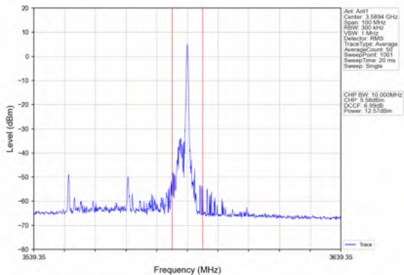
n78d_15kHz_SISO_NTNV_40MHz_DFT-s-OFDM QPSK_3570MHz_Edge_1RB_Right
