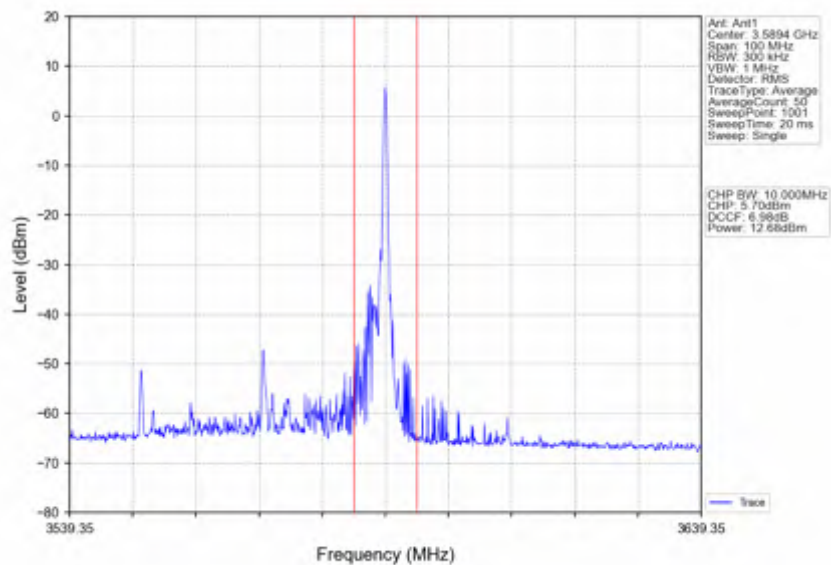
n78d_15kHz_SISO_NTNV_40MHz_DFT-s-OFDM_256_QAM_3570MHz_Edge_1RB_Right
