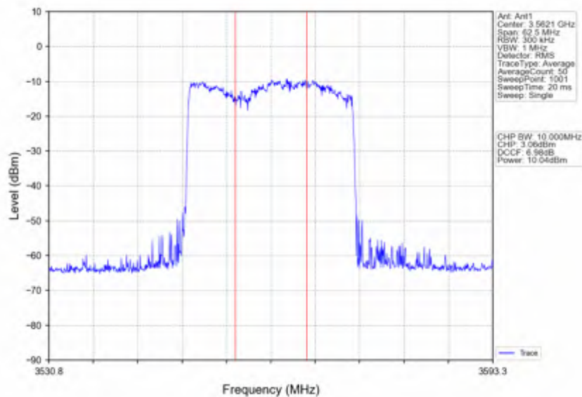
n78d_15kHz_SISO_NTNV_25MHz_DFT-s-OFDM 64 QAM_3562.5MHz_Inner_Full
