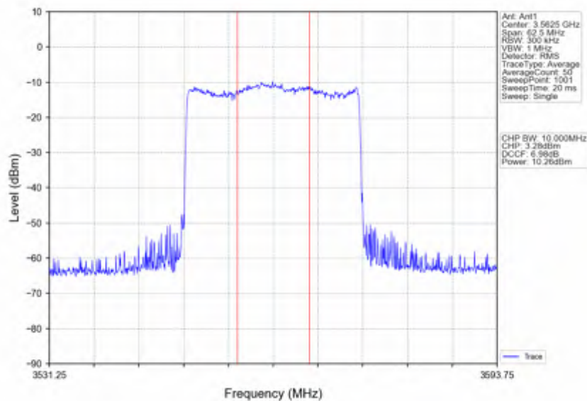
n78d_15kHz_SISO_NTNV_25MHz_CP-OFDM 64 QAM_3562.5MHz_Inner_Full
