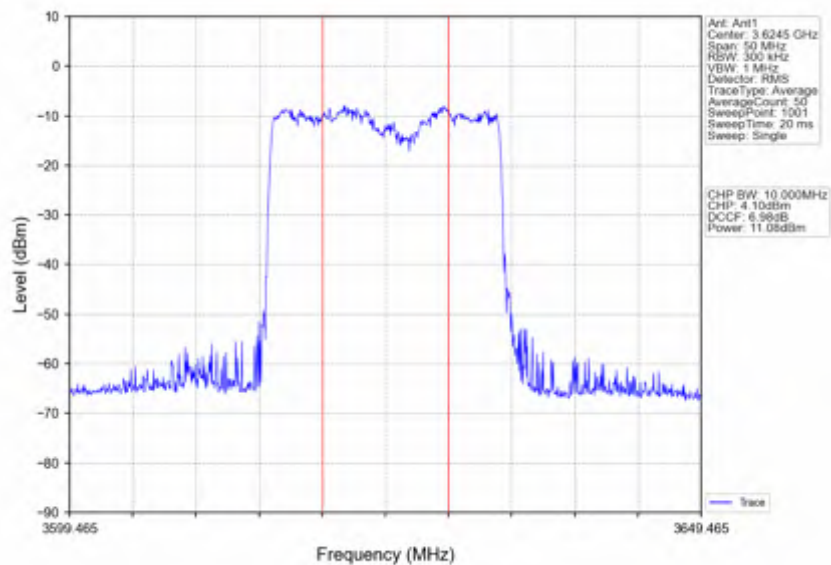
n78d_15kHz_SISO_NTNV_20MHz_DFT-s-OFDM 64 QAM_3625.005MHz_Inner_Full
