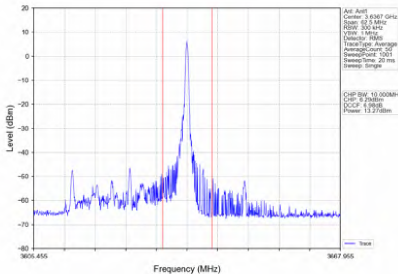
n78d_15kHz_SISO_NTNV_25MHz_DFT-s-OFDM_QPSK_3625.005MHz_Inner_1RB_Right
