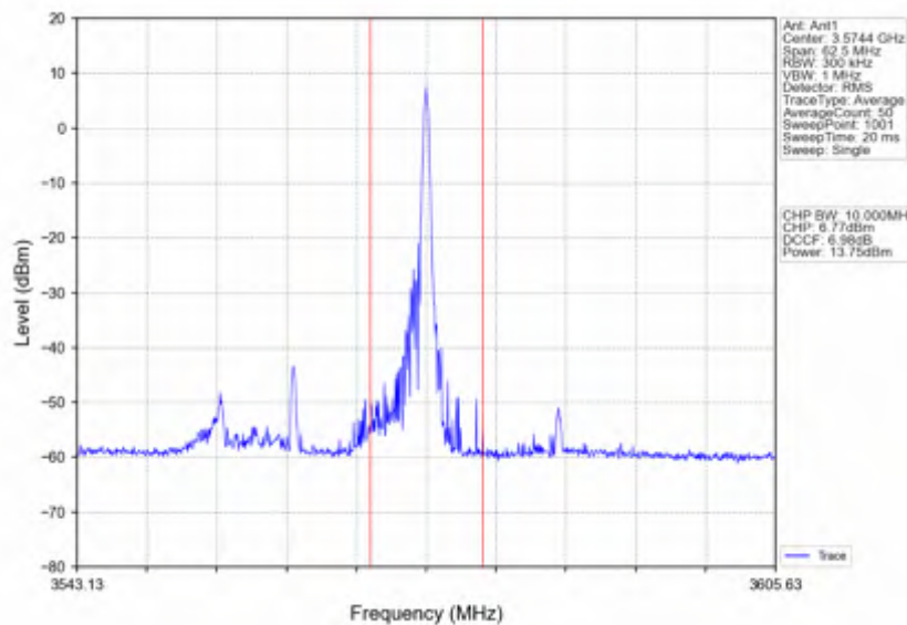
n78d_15kHz_SISO_NTNV_25MHz_CP-OFDM_16_QAM_3562.5MHz_Edge_1RB_Right
