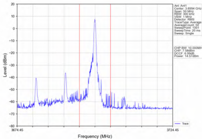
n78d_15kHz_SISO_NTNV_20MHz_DFT-s-OFDM 64 QAM_3690MHz_Edge_1RB_Right
