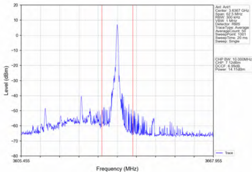
n78d_15kHz_SISO_NTNV_25MHz_CP-OFDM_256_QAM_3625.005MHz_Inner_1RB_Right
