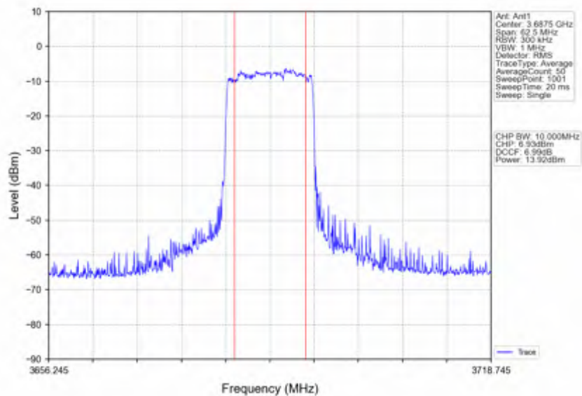
n78d_15kHz_SISO_NTNV_25MHz_CP-OFDM 64 QAM_3687.495MHz_Inner_Full
