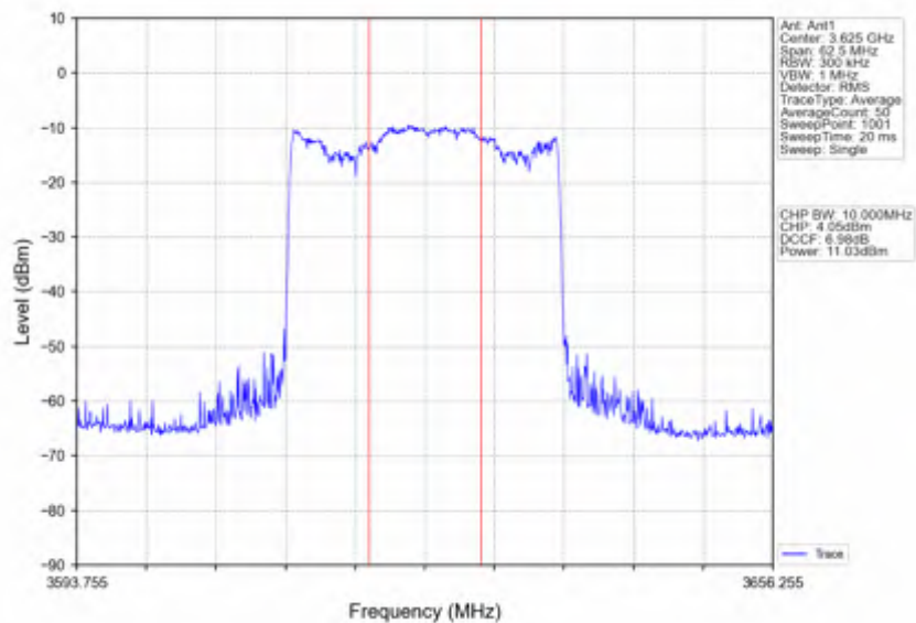
n78d_15kHz_SISO_NTNV_25MHz_CP-OFDM QPSK_3625.005MHz_Inner_Full
