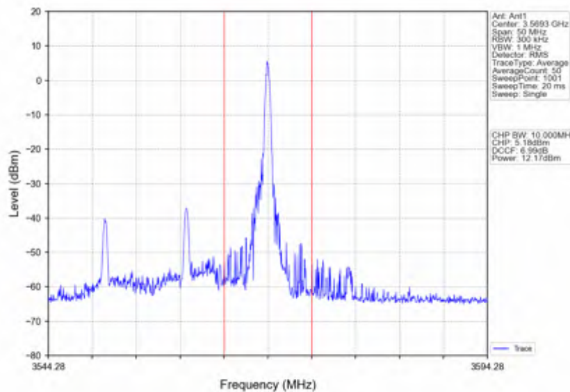
n78d_15kHz_SISO_NTNV_20MHz_CP-OFDM_16_QAM_3560.01MHz_Inner_1RB_Right
