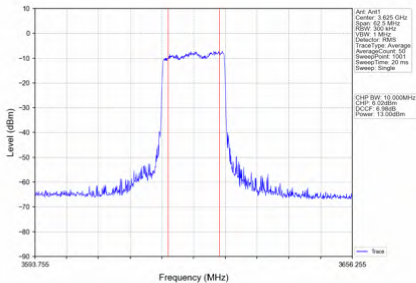
n78d_15kHz_SISO_NTNV_25MHz_CP-OFDM_16_QAM_3625.005MHz_Inner_Full
