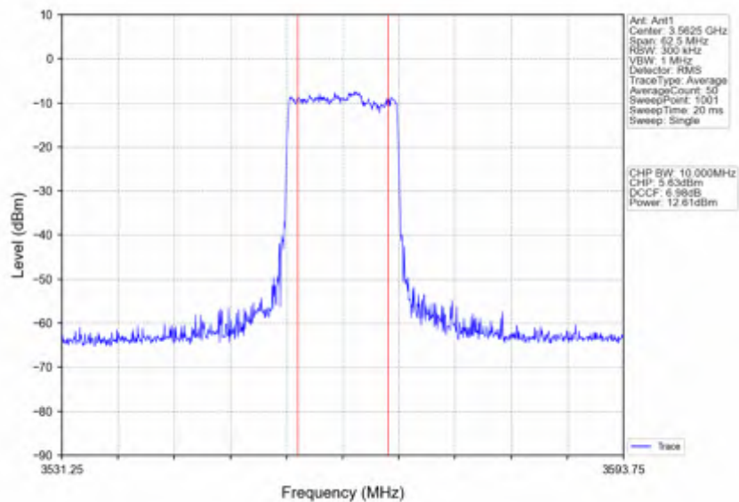
n78d_15kHz_SISO_NTNV_25MHz_CP-OFDM 256 QAM_3562.5MHz_Inner_Full
