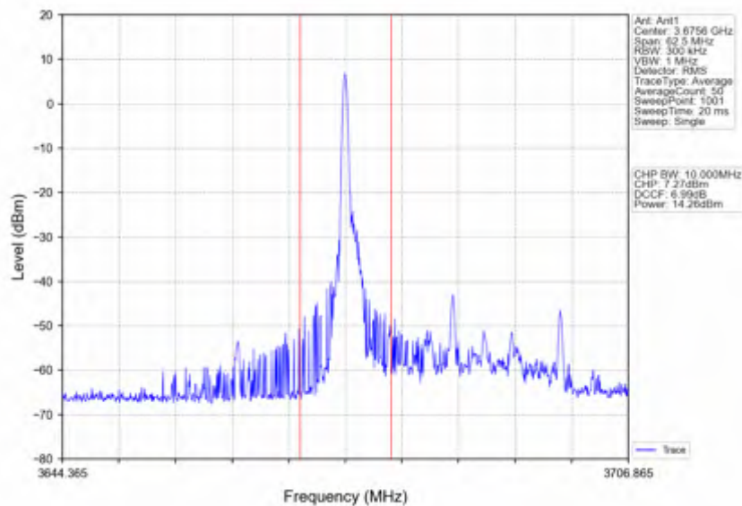
n78d_15kHz_SISO_NTNV_25MHz_DFT-s-OFDM_QPSK_3687.495MHz_Edge_1RB_Right
