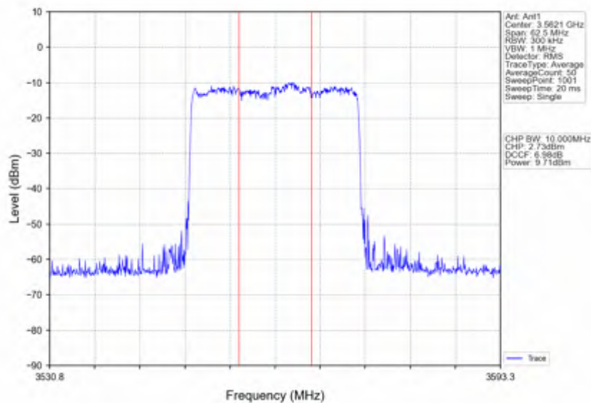
n78d_15kHz_SISO_NTNV_25MHz_DFT-s-OFDM QPSK_3562.5MHz_Inner_Full
