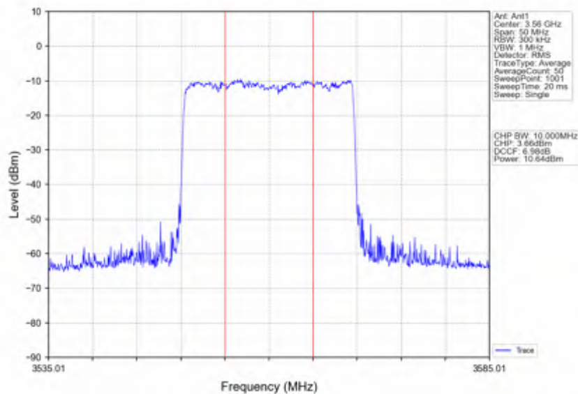
n78d_15kHz_SISO_NTNV_20MHz_CP-OFDM 16 QAM_3560.01MHz_Inner_Full
