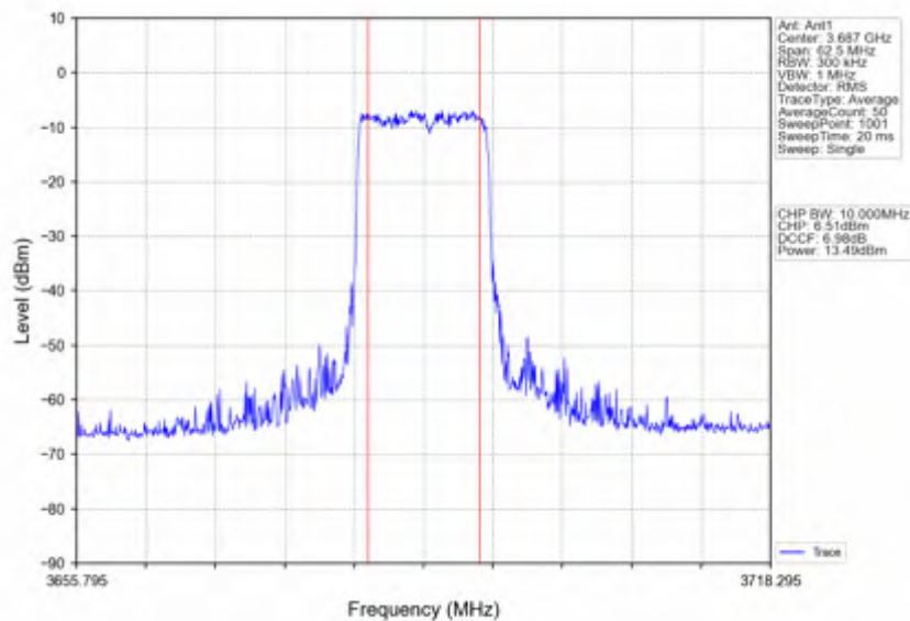
n78d_15kHz_SISO_NTNV_25MHz_DFT-s-OFDM QPSK_3687.495MHz_Inner_Full
