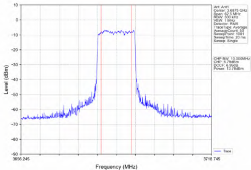
n78d_15kHz_SISO_NTNV_25MHz_CP-OFDM_16_QAM_3687.495MHz_Inner_Full
