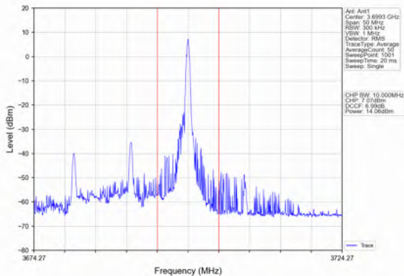
n78d_15kHz_SISO_NTNV_20MHz_CP-OFDM_QPSK_3690MHz_Inner_1RB_Right
