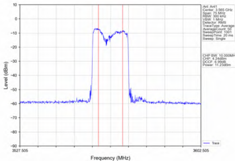
n78d_15kHz_SISO_NTNV_30MHz_DFT-s-OFDM QPSK_3565.005MHz_Inner_Full
