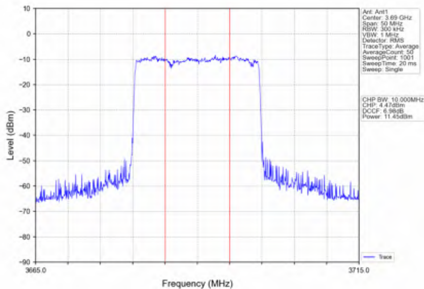
n78d_15kHz_SISO_NTNV_20MHz_CP-OFDM 256 QAM_3690MHz_Inner_Full
