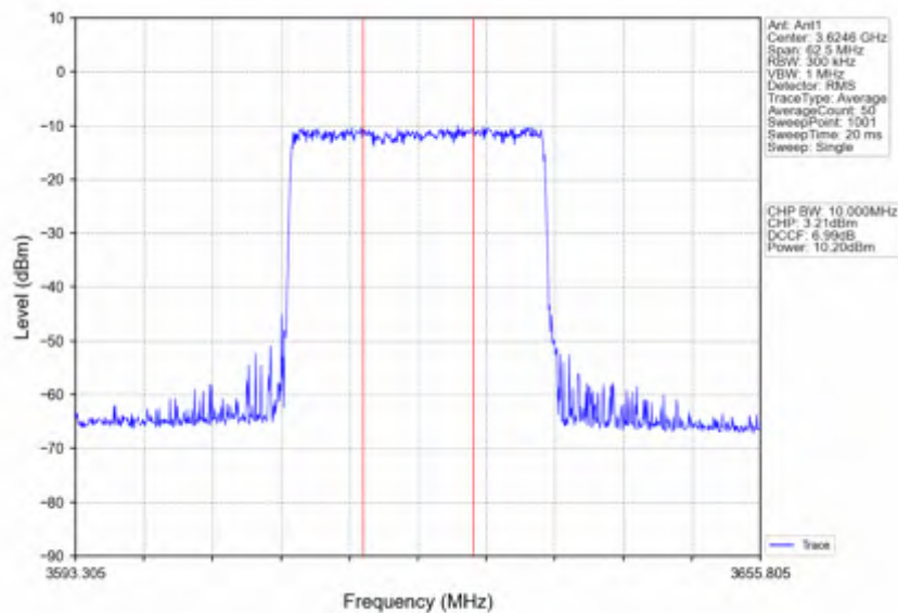
n78d_15kHz_SISO_NTNV_25MHz_DFT-s-OFDM 64 QAM_3625.005MHz_Inner_Full
