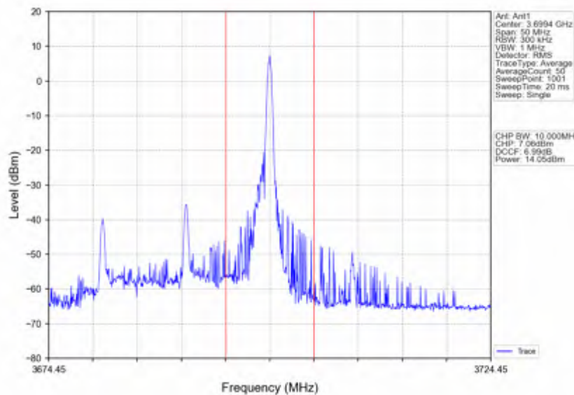
n78d_15kHz_SISO_NTNV_20MHz_CP-OFDM QPSK_3690MHz_Edge_1RB_Right
