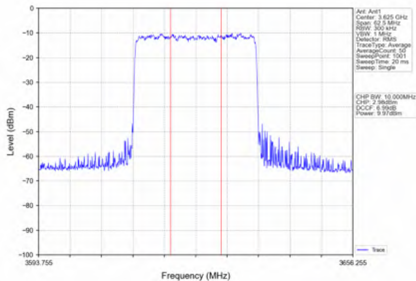
n78d_15kHz_SISO_NTNV_25MHz_CP-OFDM 256 QAM_3625.005MHz_Inner_Full
