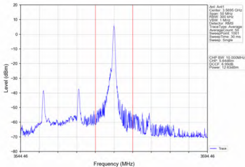
n78d_15kHz_SISO_NTNV_20MHz_DFT-s-OFDM_64_QAM_3560.01MHz_Edge_1RB_Right
