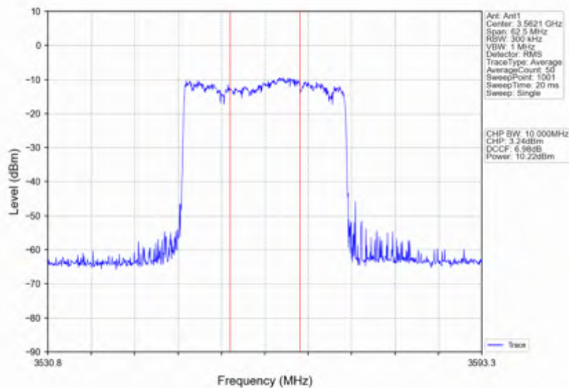
n78d_15kHz_SISO_NTNV_25MHz_DFT-s-OFDM_16_QAM_3562.5MHz_Inner_Full
