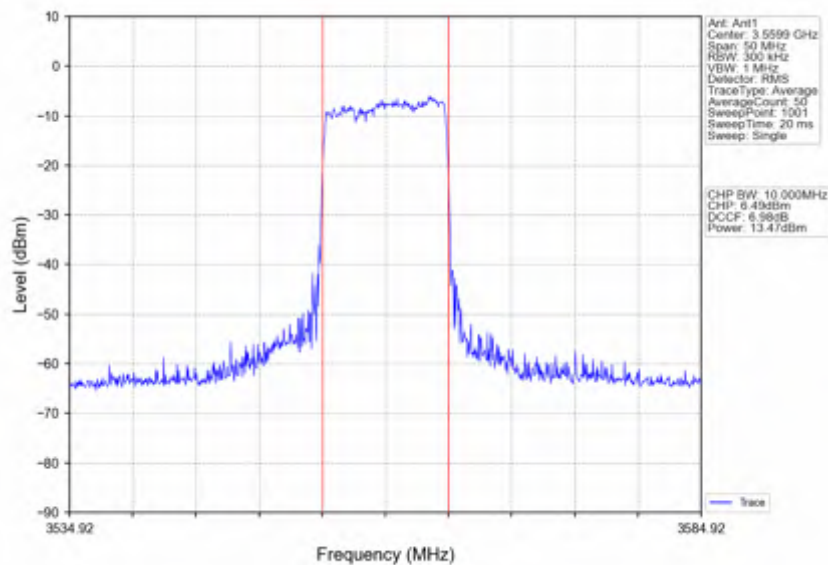
n78d_15kHz_SISO_NTNV_20MHz_CP-OFDM_256_QAM_3560.01MHz_Inner_Full
