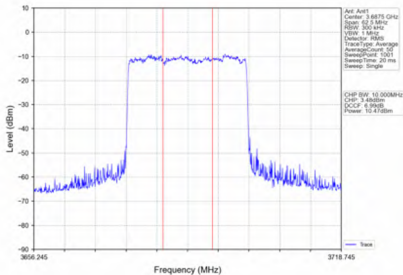
n78d_15kHz_SISO_NTNV_25MHz_CP-OFDM 256 QAM 3687.495MHz_Inner_Full
