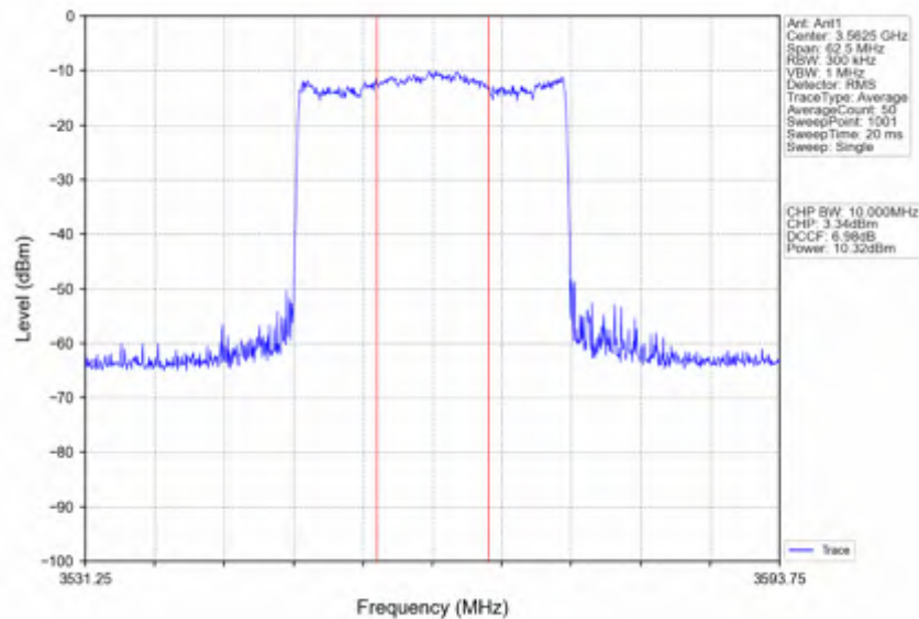
n78d_15kHz_SISO_NTNV_25MHz_CP-OFDM 16 QAM_3562.5MHz_Inner_Full
