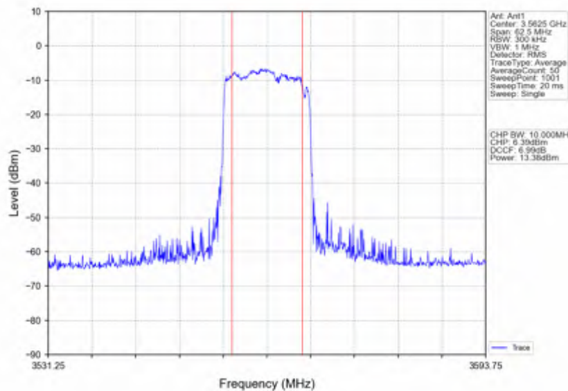
n78d_15kHz_SISO_NTNV_25MHz_CP-OFDM 64 QAM_3562.5MHz_Inner_Full
