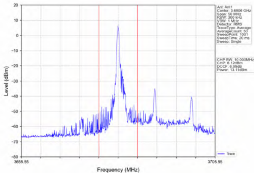
n78d_15kHz_SISO_NTNV_20MHz_CP-OFDM 64 QAM_3690MHz_Edge_1RB_Right
