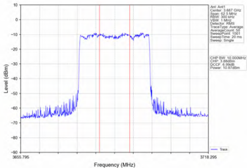
n78d_15kHz_SISO_NTNV_25MHz_DFT-s-OFDM 256 QAM_3687.495MHz_Inner_Full
