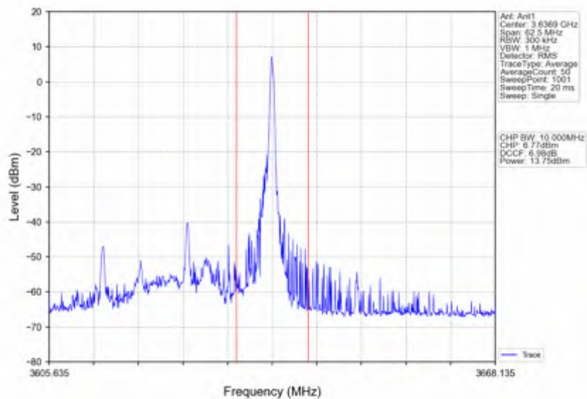
n78d_15kHz_SISO_NTNV_25MHz_CP-OFDM_256_QAM_3625.005MHz_Edge_1RB_Right
