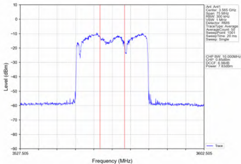
n78d_15kHz_SISO_NTNV_30MHz_DFT-s-OFDM QPSK_3565.005MHz_Inner_Full
