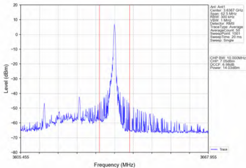
n78d_15kHz_SISO_NTNV_25MHz_CP-OFDM QPSK_3625.005MHz_Inner_1RB_Right
