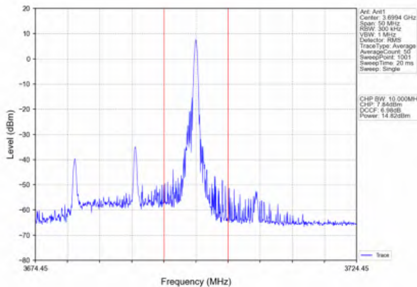
n78d_15kHz_SISO_NTNV_20MHz_CP-OFDM 64 QAM_3690MHz_Edge_1RB_Right
