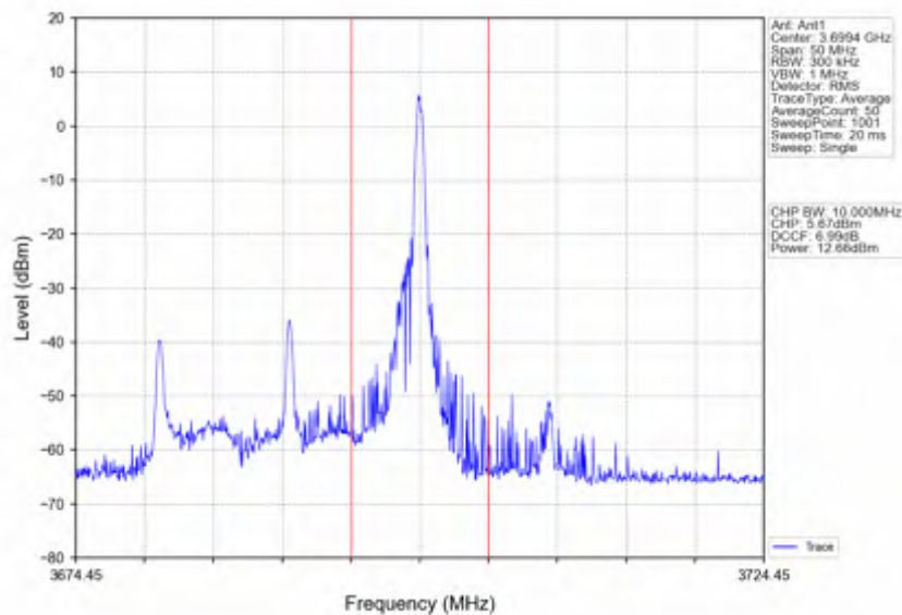
n78d_15kHz_SISO_NTNV_20MHz_CP-OFDM 16 QAM_3690MHz_Edge_1RB_Right
