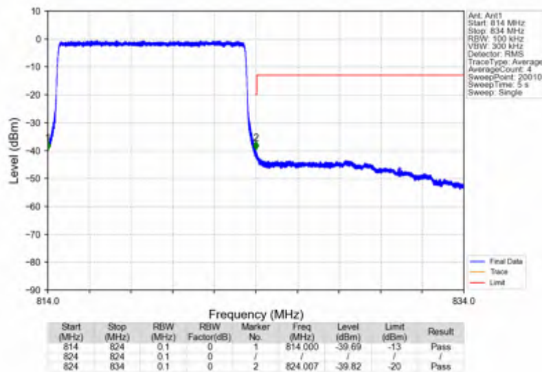
Band26a_10MHz_256QAM_HCH_819MHz_RB_50_0_NTNV
