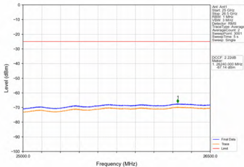
Band38_15MHz_16QAM_LCH_2577.5MHz_RB_75_0_NTNV
