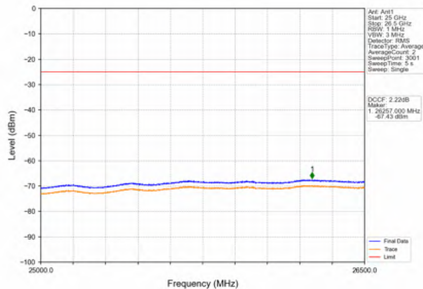
Band38_5MHz_256QAM_LCH_2572.5MHz_RB_25_0_NTNV
