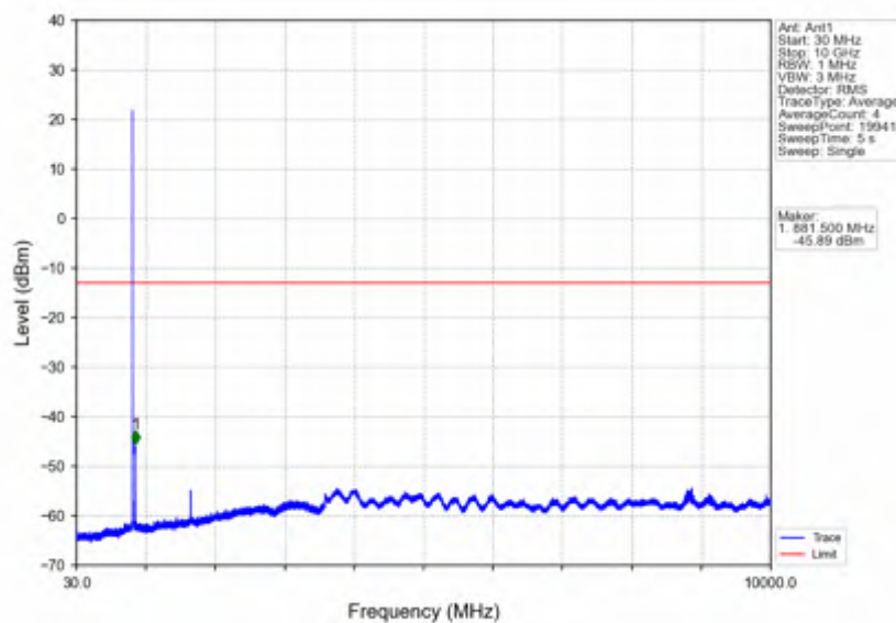
Band26b 5MHz 64QAM MCH 836.5MHz RB 1 0 NTNV
