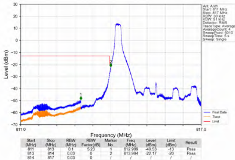
Band26a_3MHz_16QAM_LCH_815.5MHz_RB_1_0_NTNV
