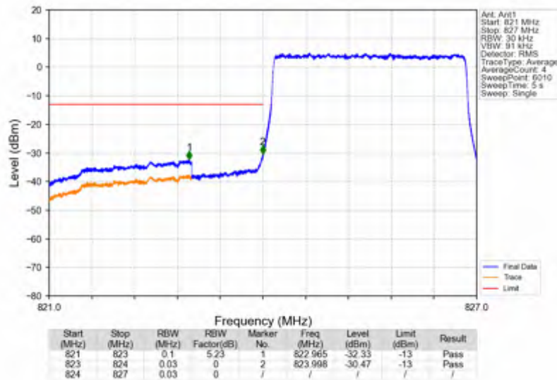
Band26b 3MHz QPSK LCH 825.5MHz RB 15 0 NTNV
