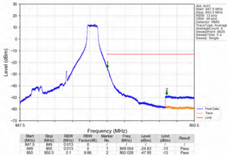
Band26b_1.4MHz_64QAM_HCH_848.3MHz_RB_1_5_NTNV
