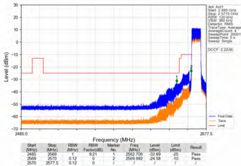
Band38_5MHz_16QAM_LCH_2572.5MHz_RB_25_0_NTNV
