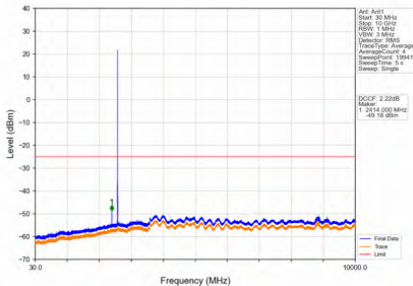
Band38_5MHz_16QAM_MCH_2595MHz_RB_1_0_NTNV
