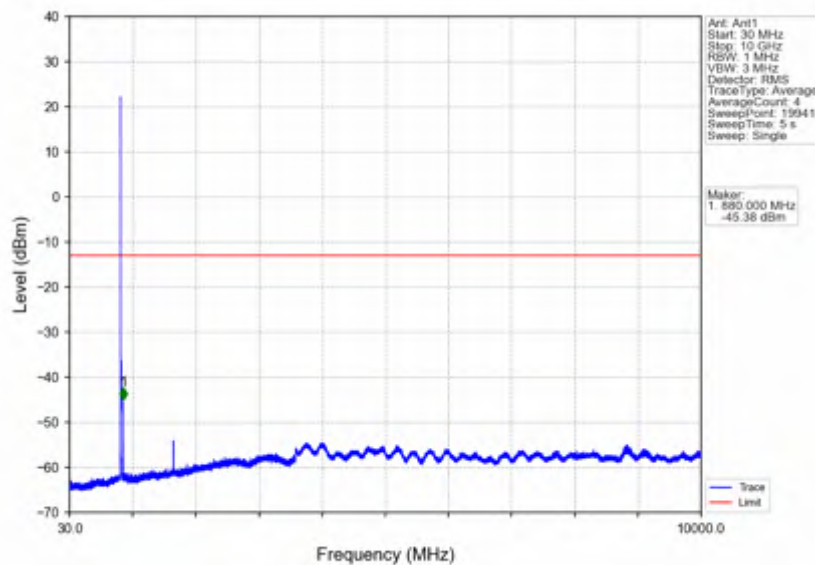
Band26b_5MHz_16QAM_HCH_846.5MHz_RB_1_0_NTNV
