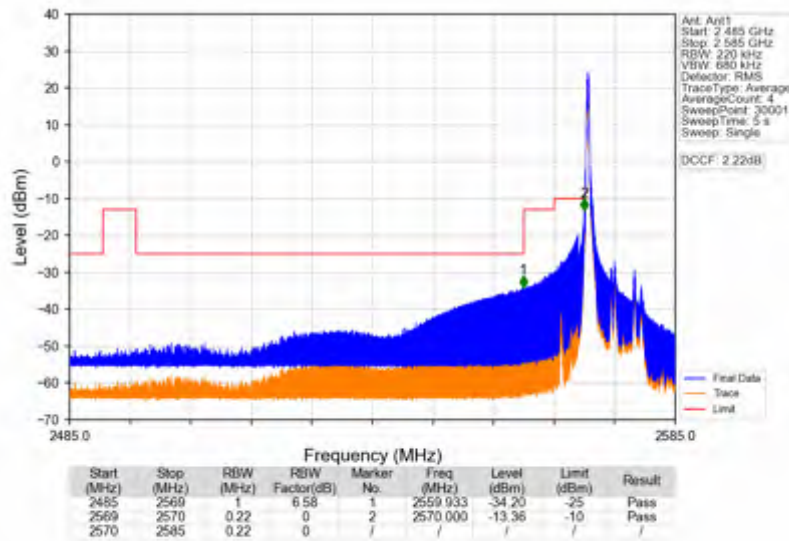
Band38_10MHz_64QAM_LCH_2575MHz_RB_1_0_NTNV
