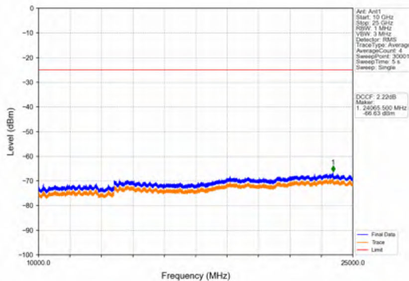
Band38_5MHz_QPSK_HCH_2617.5MHz_RB_1_0_NTNV
