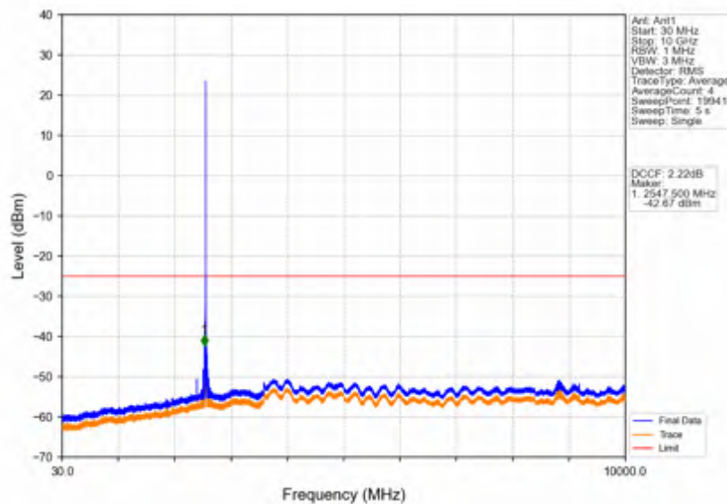
Band38_10MHz_16QAM_LCH_2575MHz_RB_1_0_NTNV
