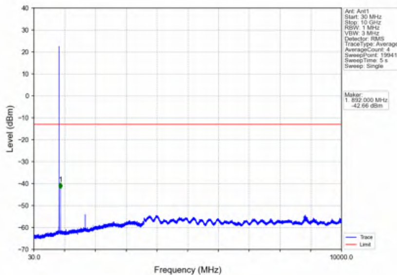
Band26b_3MHz_16QAM_HCH_847.5MHz_RB_1_0_NTNV
