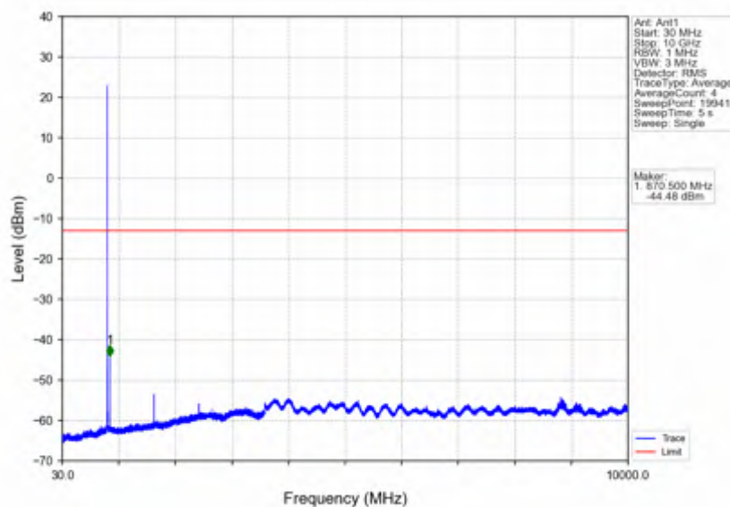
Band26b_3MHz_QPSK_LCH_825.5MHz_RB_1_0_NTNV
