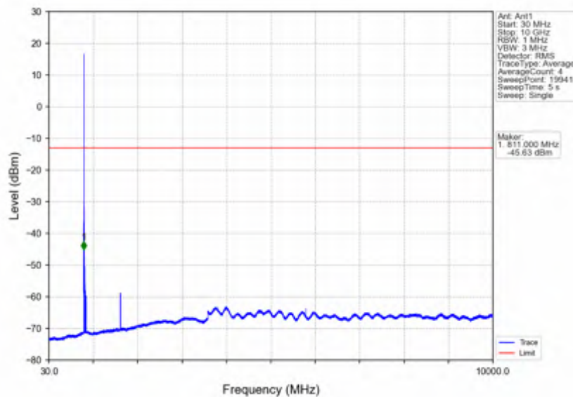
Band26a_3MHz_256QAM_HCH_822.5MHz_RB_1_0_NTNV
