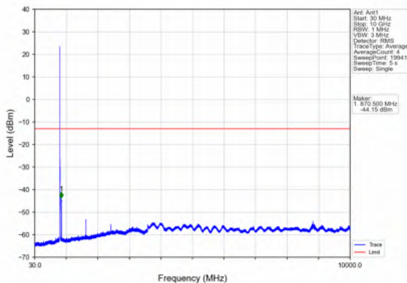
Band26b_10MHz_QPSK_LCH_829MHz_RB_1_0_NTNV
