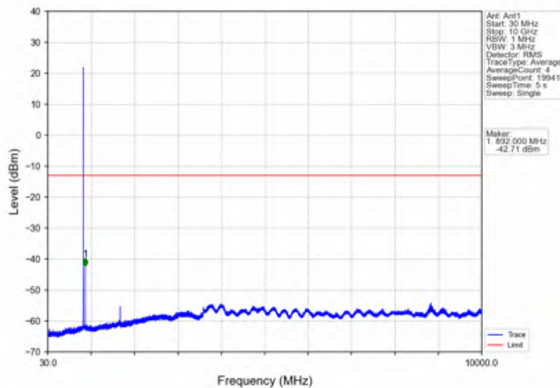
Band26b_3MHz_64QAM_HCH_847.5MHz_RB_1_14_NTNV
