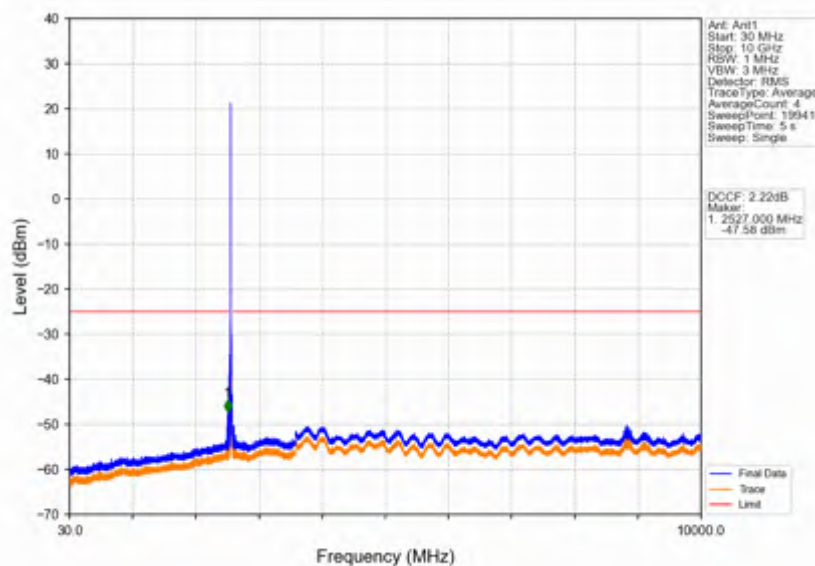
Band38_15MHz_QPSK_LCH_2577.5MHz_RB_1_0_NTNV
