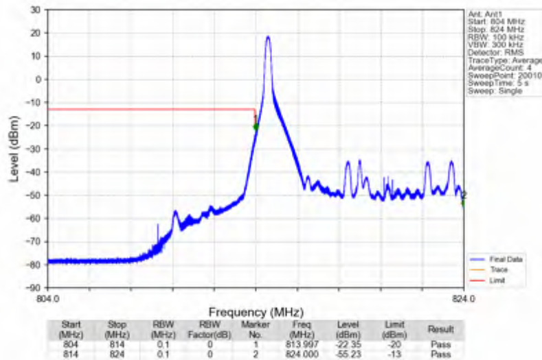
Band26a_10MHz_64QAM_LCH_819MHz_RB_50_0_NTNV
