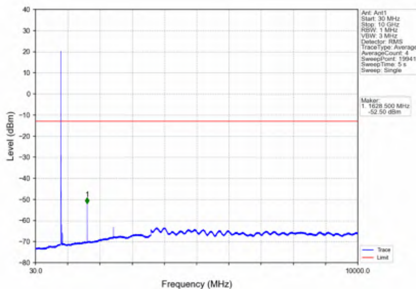
Band26a_5MHz_QPSK_LCH_816.5MHz_RB_1_0_NTNV
