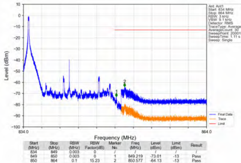
Band26c_15MHz_64QAM_HCH_841.5MHz_RB_1_74_NTNV
