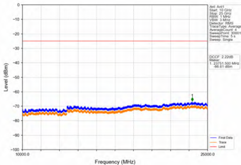
Band38_10MHz_64QAM_HCH_2615MHz_RB_1_0_NTNV
