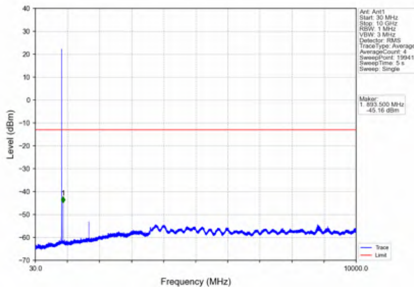
Band26b_1.4MHz_64QAM_HCH_848.3MHz_RB_1_5_NTNV
