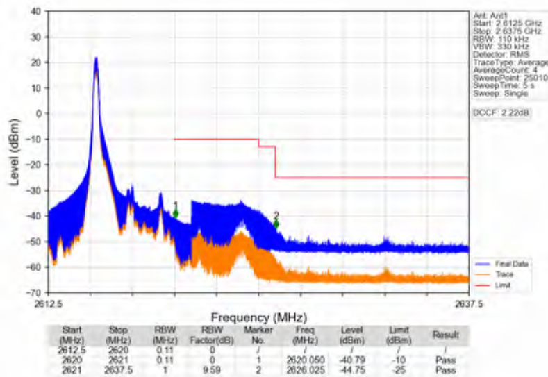
Band38_5MHz_16QAM_HCH_2617.5MHz_RB_25_0_NTNV
