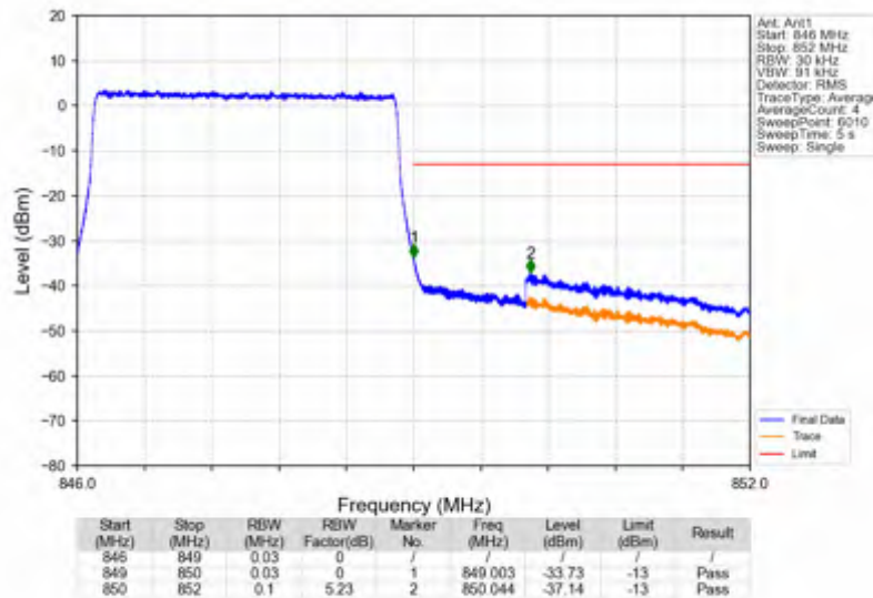
Band26b_3MHz_64QAM_HCH_847.5MHz_RB_15_0_NTNV
