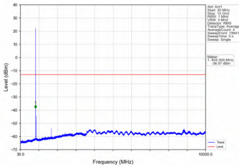
Band26b 1.4MHz QPSK HCH 848.3MHz RB_1_5 NTN
