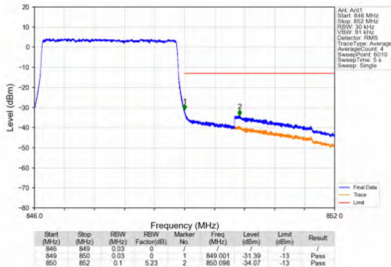
Band26b_3MHz_16QAM_HCH_847.5MHz_RB_15_0_NTNV
