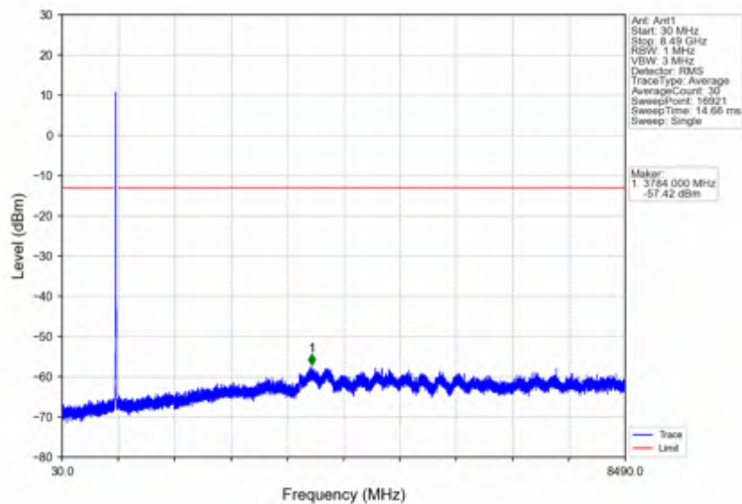
Band26c_15MHz_256QAM_HCH_841.5MHz_RB_1_0_NTNV
