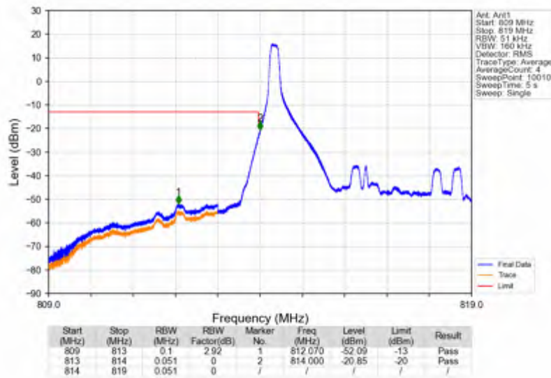
Band26a_5MHz_QPSK_LCH_816.5MHz_RB_1_0_NTNV
