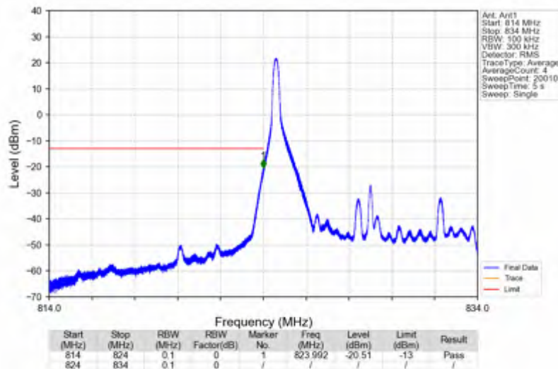
Band26b_10MHz_QPSK_LCH_829MHz_RB_1_0_NTNV
