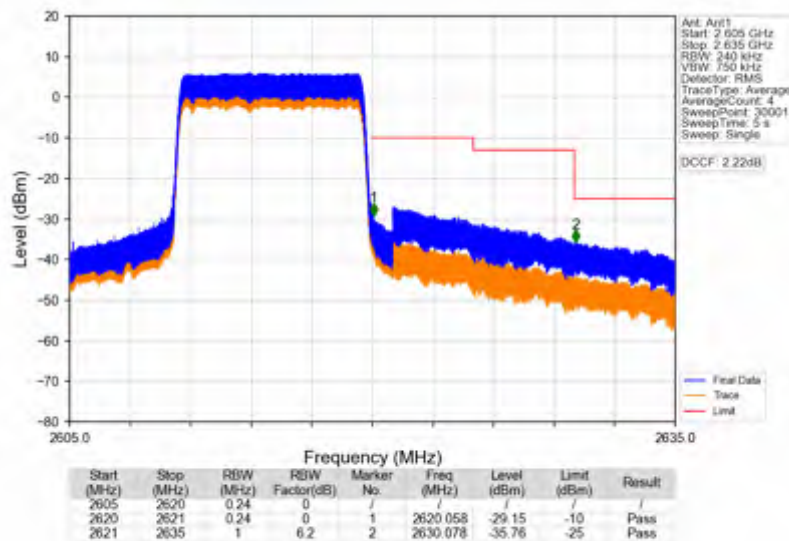
Band38_10MHz_256QAM_HCH_2615MHz_RB_50_0_NTNV
