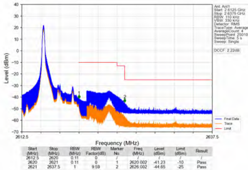
Band38_5MHz_16QAM_HCH_2617.5MHz_RB_1_24_NTNV
