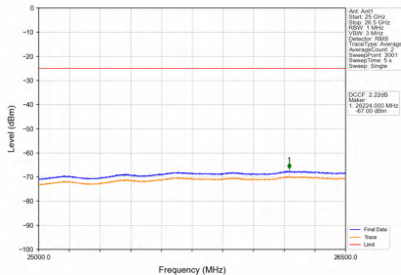
Band38_5MHz_64QAM_MCH_2595MHz_RB_1_0_NTNV
