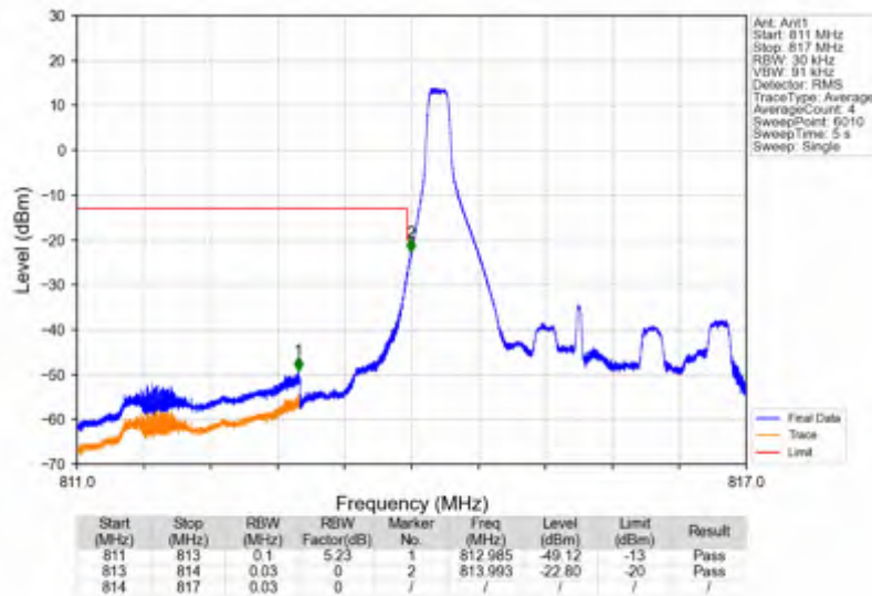
Band26a 3MHz QPSK LCH 815.5MHz RB 15 0 NTNV
