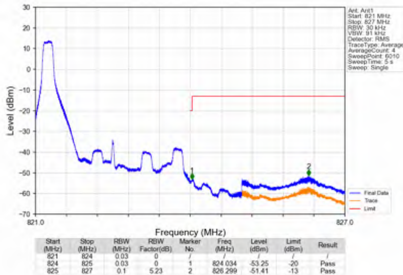
Band26a_3MHz_16QAM_HCH_822.5MHz_RB_1_14_NTNV
