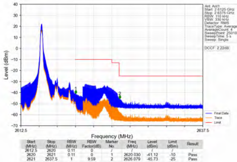
Band38_5MHz_64QAM_HCH_2617.5MHz_RB_25_0_NTNV
