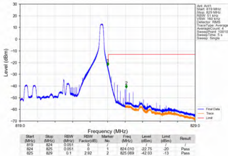
Band26a_5MHz_256QAM_HCH_821.5MHz_RB_1_24_NTNV
