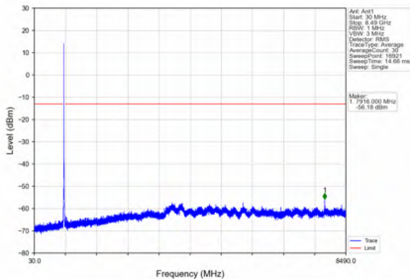
Band26c 15MHz 64QAM MCH 836.5MHz RB 1 0 NTNV
