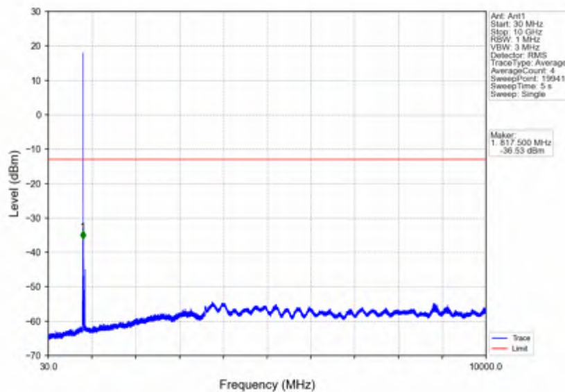
Band26b_3MHz_256QAM_LCH_825.5MHz_RB_15_0_NTNV
