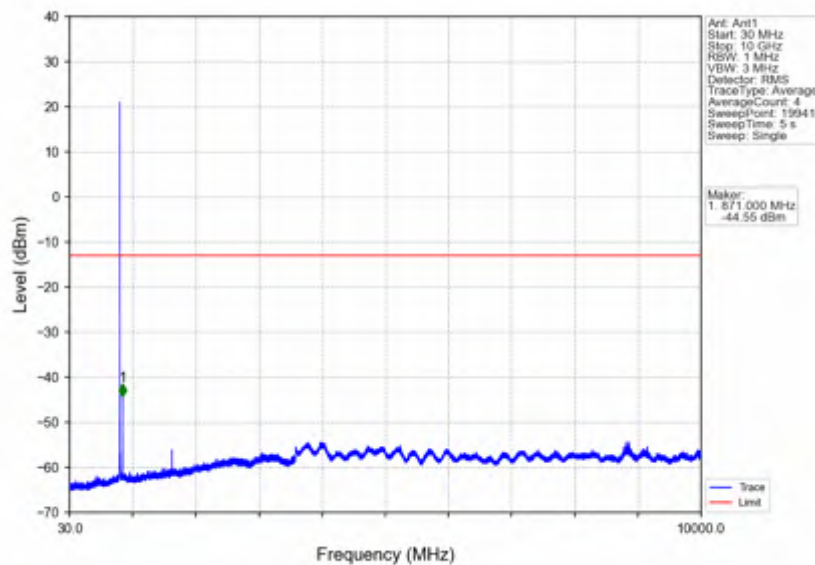
Band26b 3MHz 64QAM LCH 825.5MHz RB 1 0 NTNV
