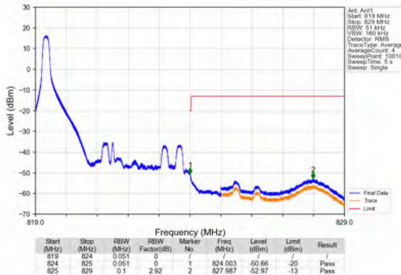
Band26a_5MHz_QPSK_HCH_821.5MHz_RB_25_0_NTNV
