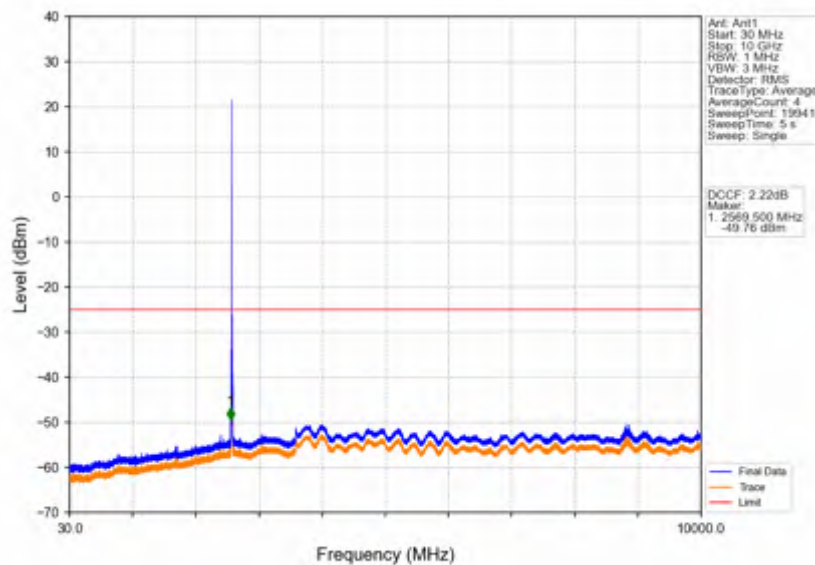
Band38_10MHz_16QAM_MCH_2595MHz_RB_1_0_NTNV
