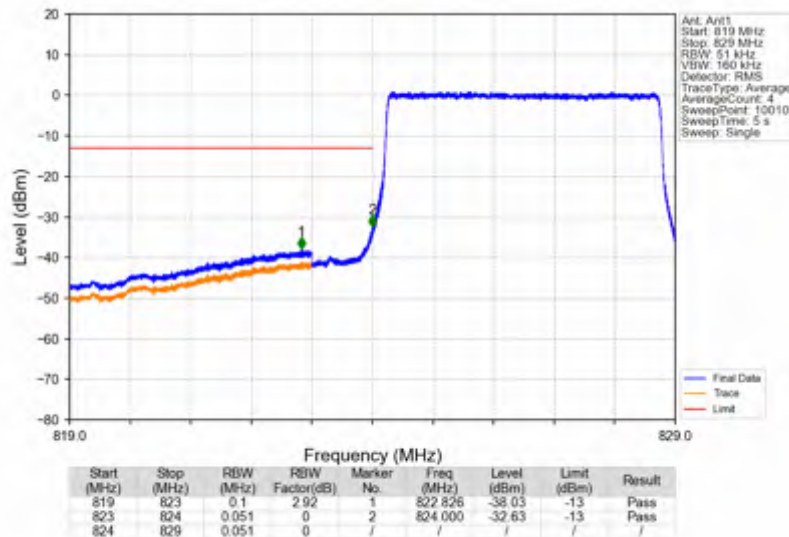
Band26b_5MHz_256QAM_LCH_826.5MHz_RB_25_0_NTNV
