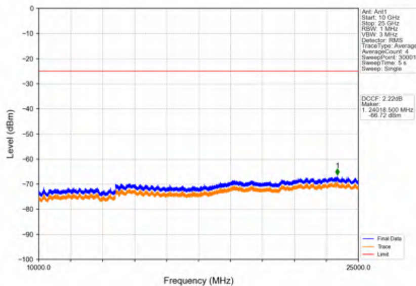
Band38_10MHz_256QAM_LCH_2575MHz_RB_1_0_NTNV
