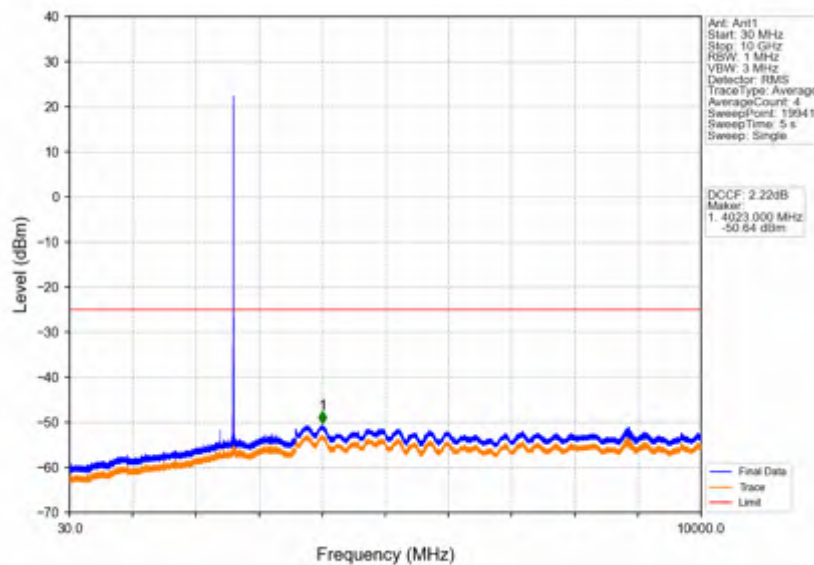
Band38_5MHz_QPSK_HCH_2617.5MHz_RB_1_0_NTNV
