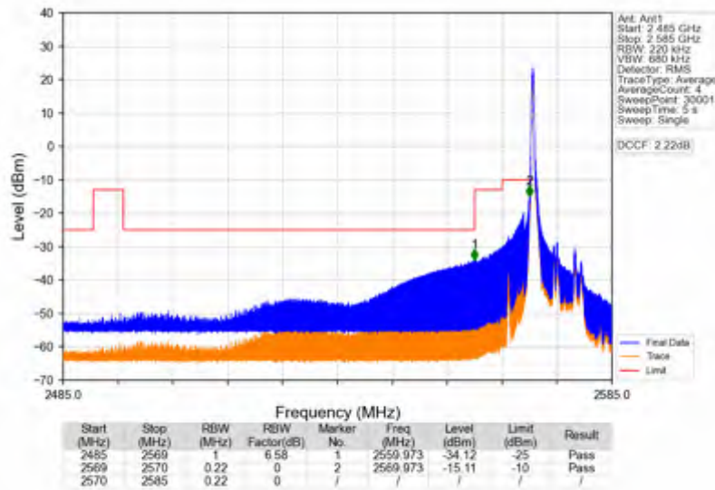
Band38_10MHz_64QAM_LCH_2575MHz_RB_50_0_NTNV
