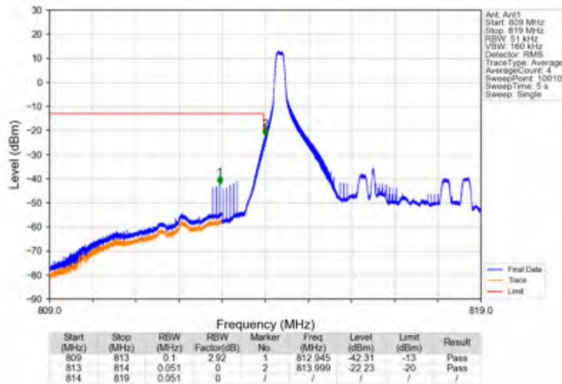
Band26a_5MHz_256QAM_LCH_816.5MHz_RB_1_0_NTNV
