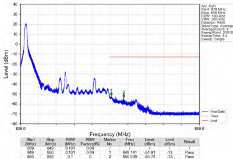
Band26b_10MHz_QPSK_HCH_844MHz_RB_50_0_NTNV
