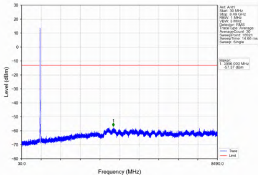
Band26c_15MHz_16QAM_LCH_831.5MHz_RB_75_0_NTNV
