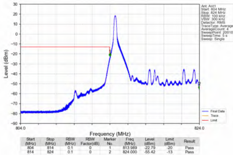
Band26a_10MHz_16QAM_LCH_819MHz_RB_50_0_NTNV
