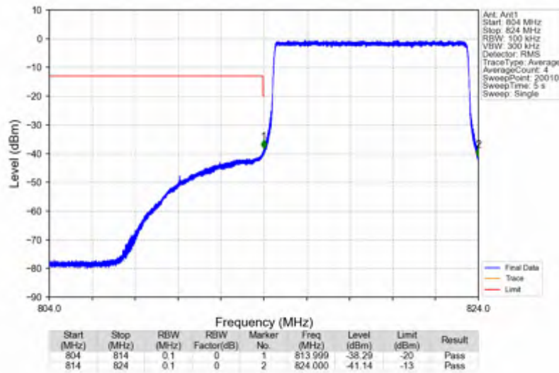
Band26a_10MHz_256QAM_LCH_819MHz_RB_50_0_NTNV
