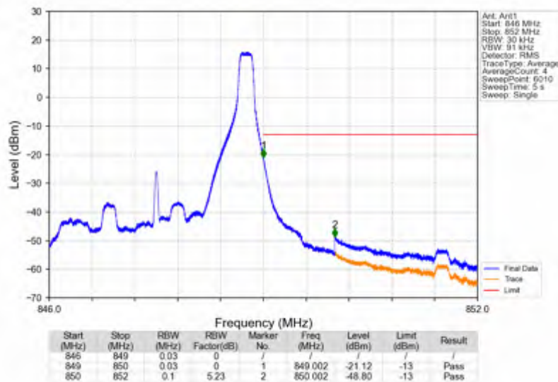
Band26b_3MHz_64QAM_HCH_847.5MHz_RB_1_14_NTNV
