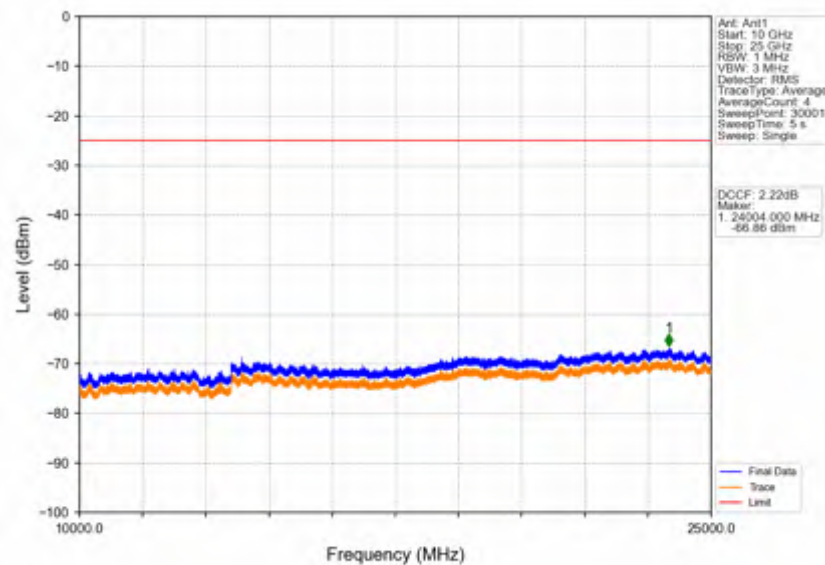
Band38_10MHz_256QAM_HCH_2615MHz_RB_1_0_NTNV
