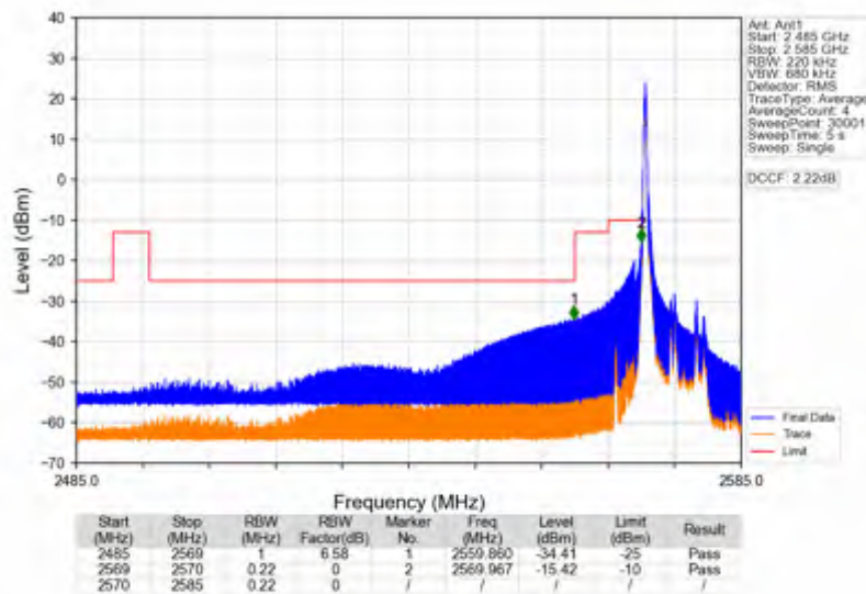
Band38_10MHz_16QAM_LCH_2575MHz_RB_1_0_NTNV
