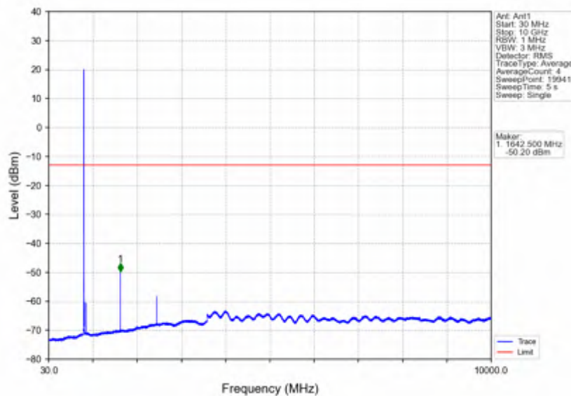
Band26a_3MHz_64QAM_HCH_822.5MHz_RB_1_14_NTNV
