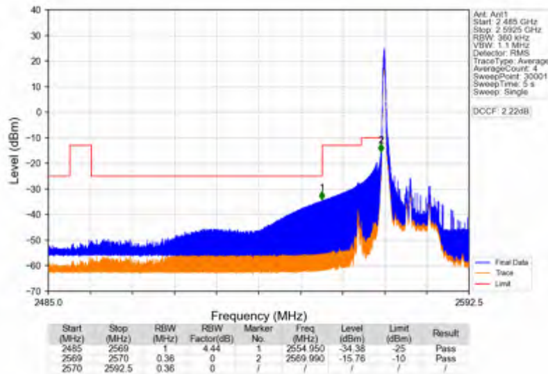
Band38_15MHz_QPSK_LCH_2577.5MHz_RB_75_0_NTNV
