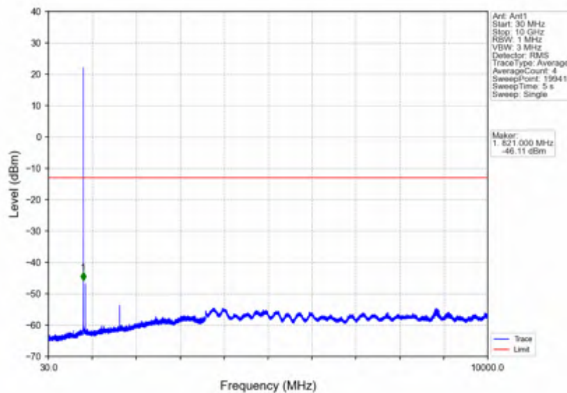
Band26b_1.4MHz_16QAM_LCH_824.7MHz_RB_6_0_NTNV
