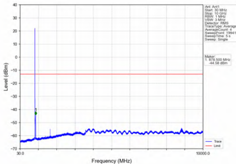
Band26b_10MHz_QPSK_MCH_836.5MHz_RB_1_0_NTNV
