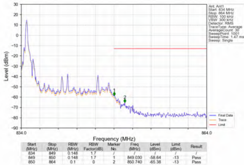
Band26c_15MHz_64QAM_HCH_841.5MHz_RB_75_0_NTNV
