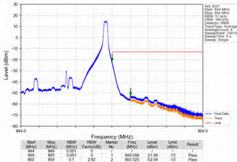
Band26b_5MHz_256QAM_HCH_846.5MHz_RB_1_24_NTNV
