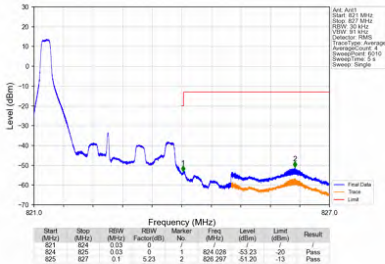
Band26a_3MHz_64QAM_HCH_822.5MHz_RB_15_0_NTNV
