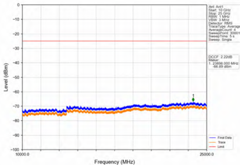
Band38_5MHz_16QAM_LCH_2572.5MHz_RB_1_0_NTNV
