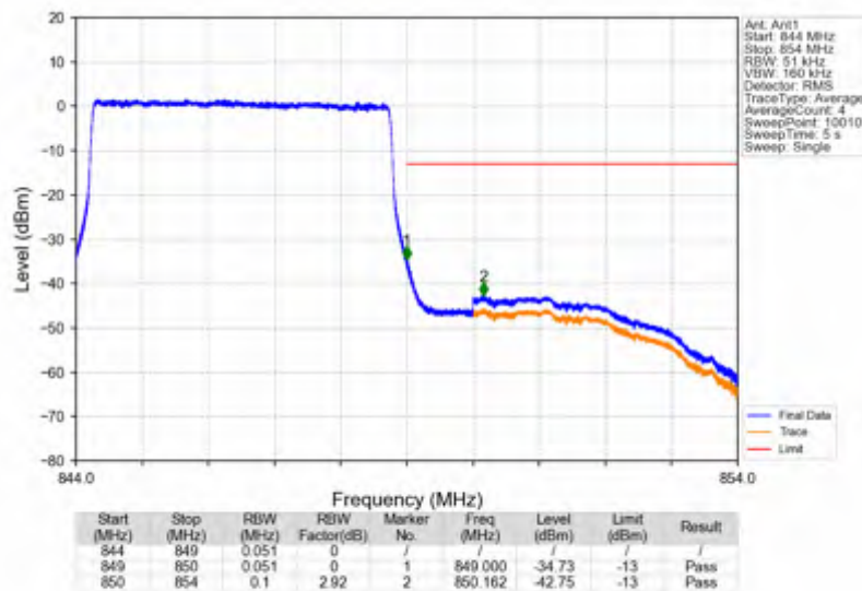
Band26b_5MHz_256QAM_HCH_846.5MHz_RB_25_0_NTNV
