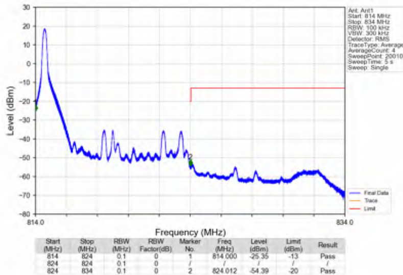
Band26a_10MHz_16QAM_HCH_819MHz_RB_50_0_NTNV
