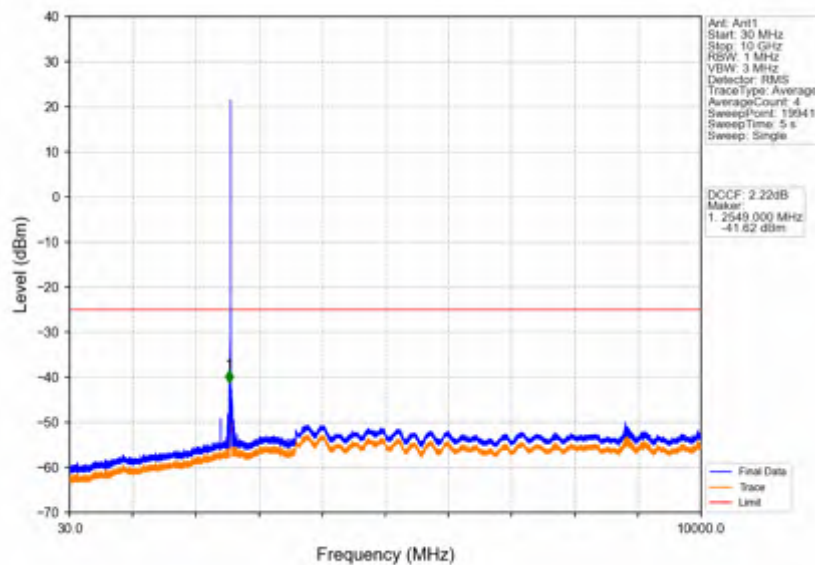
Band38_10MHz_64QAM_LCH_2575MHz_RB_1_0_NTNV
