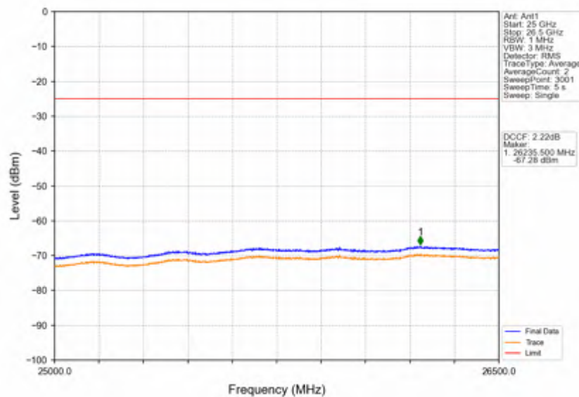
Band38_10MHz_16QAM_HCH_2615MHz_RB_1_0_NTNV
