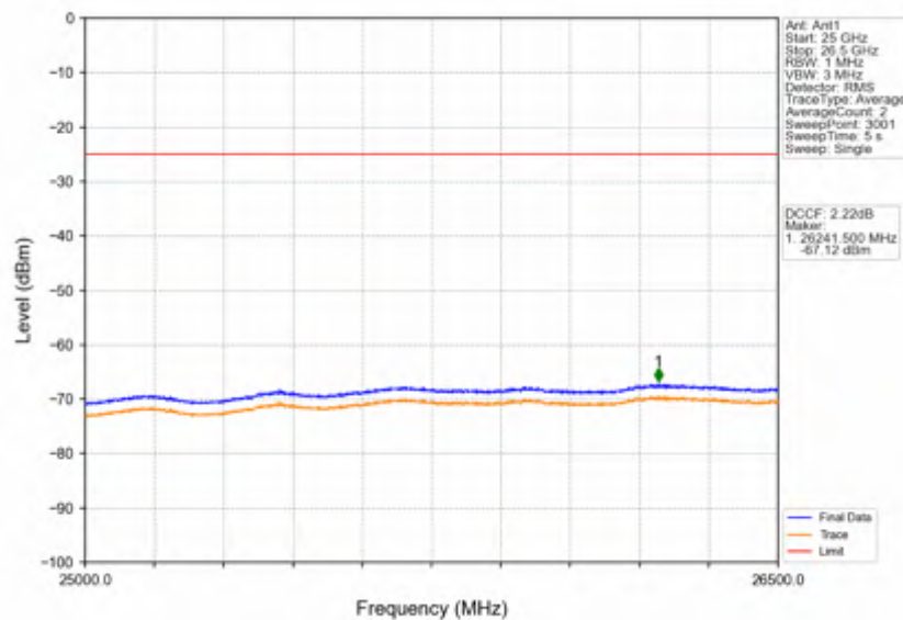
Band38_15MHz_QPSK_HCH_2612.5MHz_RB_1_74_NTNV
