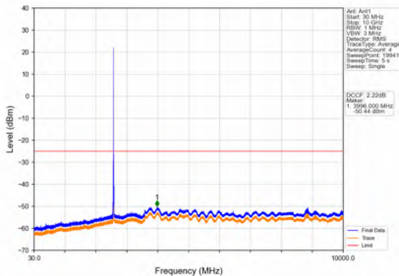
Band38_10MHz_64QAM_MCH_2595MHz_RB_1_0_NTNV
