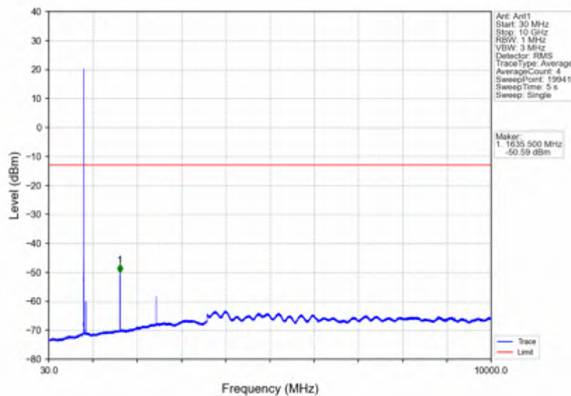
Band26a 3MHz QPSK MCH 819MHz RB 1 0 NTNV
