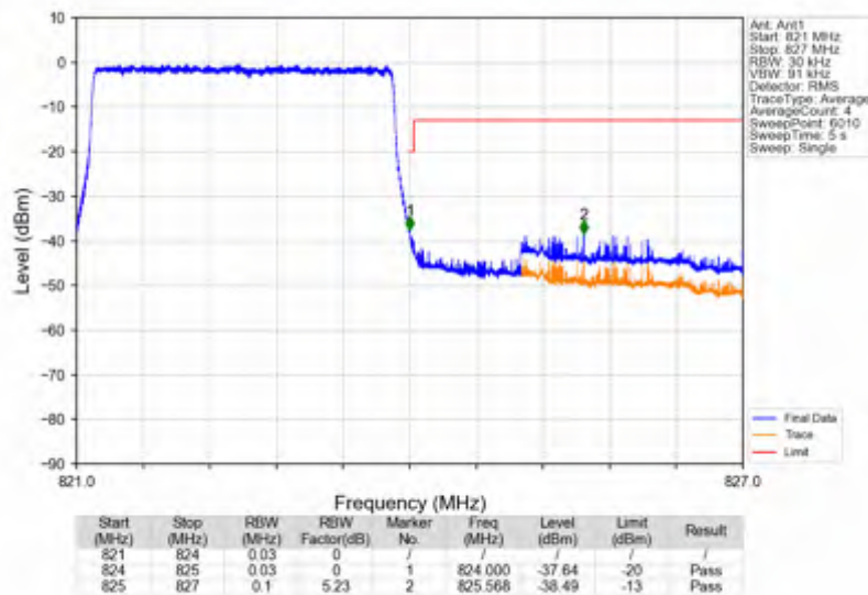
Band26a_3MHz_256QAM_HCH_822.5MHz_RB_15_0_NTNV
