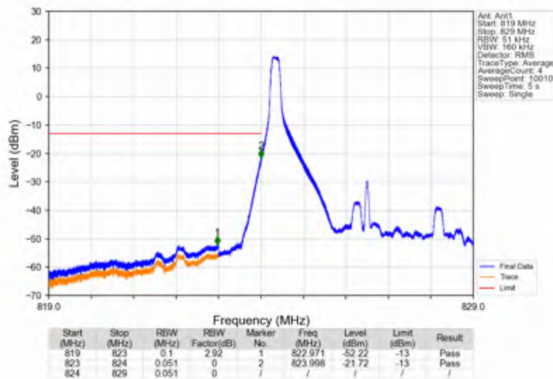
Band26b_5MHz_256QAM_LCH_826.5MHz_RB_1_0_NTNV
