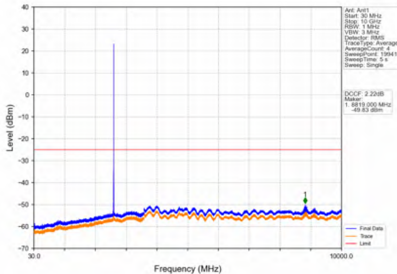
Band38_5MHz_16QAM_HCH_2617.5MHz_RB_1_0_NTNV
