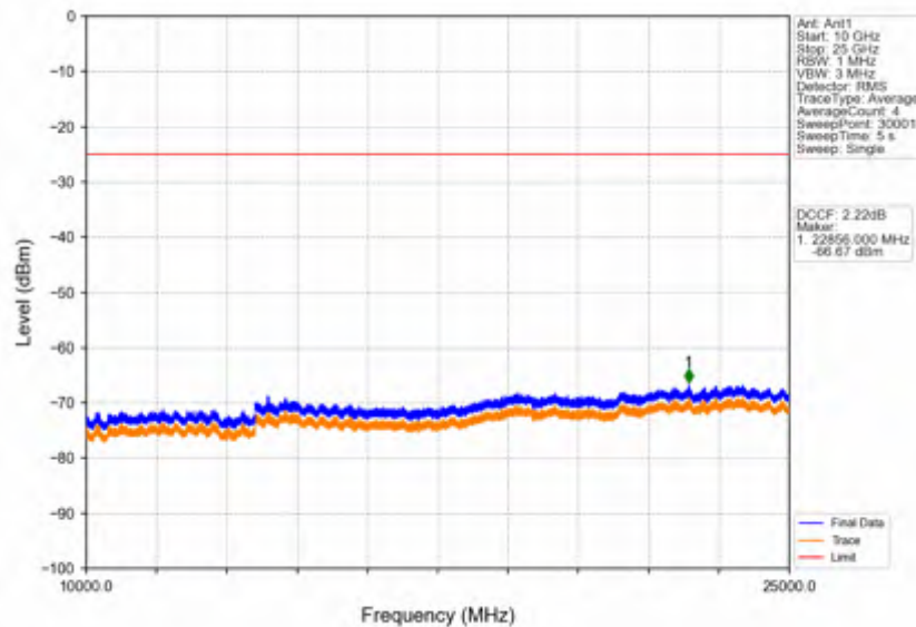
Band38_15MHz_16QAM_HCH_2612.5MHz_RB_1_0_NTNV
