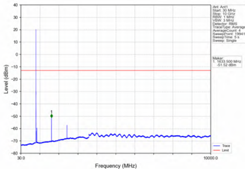
Band26a 5MHz 64QAM MCH 819MHz RB 1 0 NTNV
