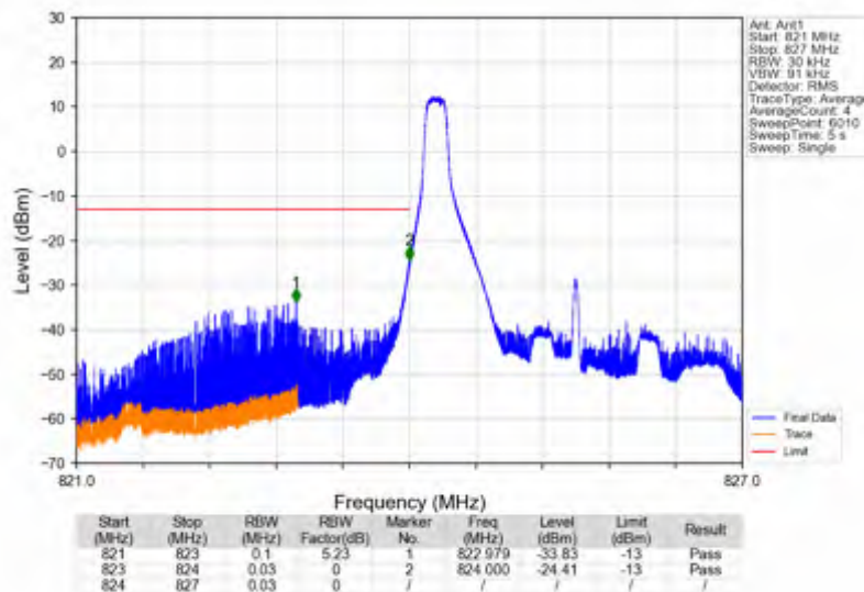
Band26b_3MHz_256QAM_LCH_825.5MHz_RB_1_0_NTNV
