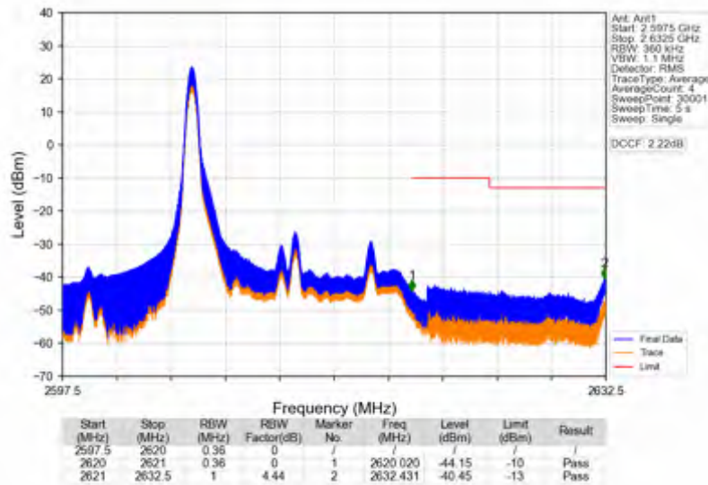
Band38_15MHz_QPSK_HCH_2612.5MHz_RB_75_0_NTNV
