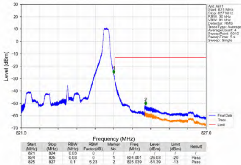
Band26a_3MHz_256QAM_HCH_822.5MHz_RB_1_14_NTNV
