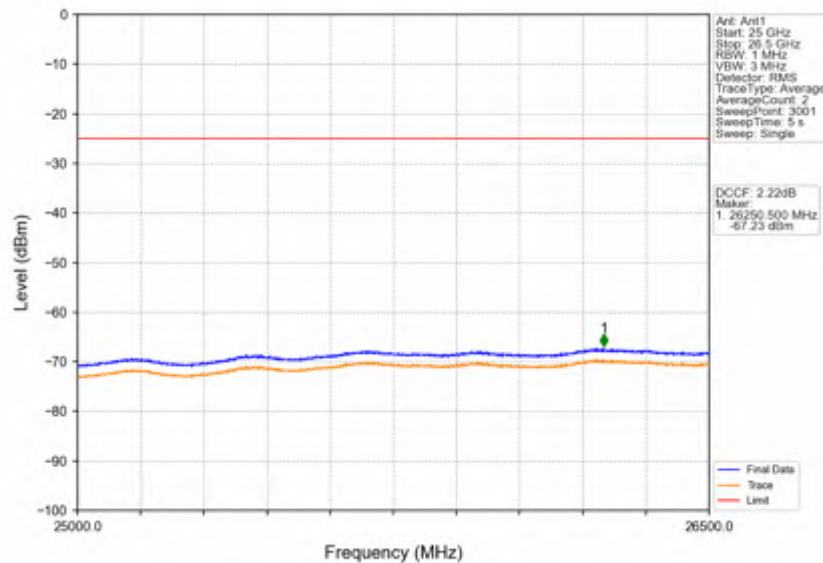
Band38_10MHz_64QAM_HCH_2615MHz_RB_1_49_NTNV
