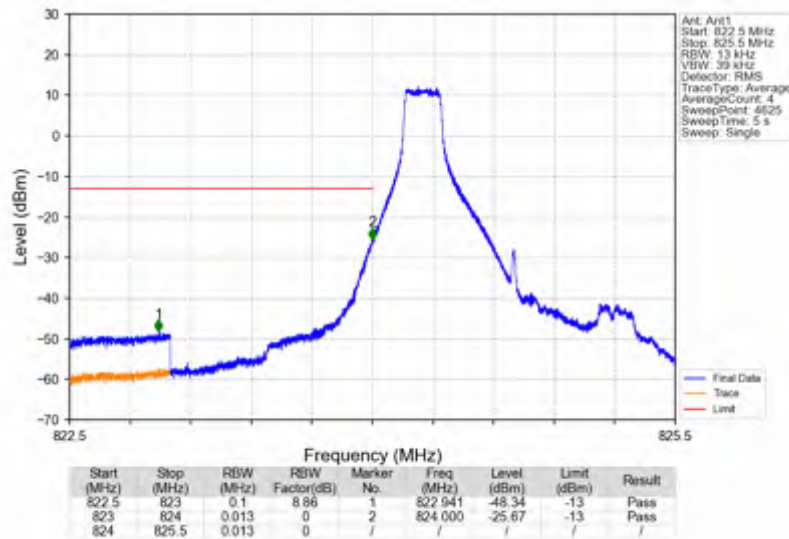
Band26b_1.4MHz_64QAM_LCH_824.7MHz_RB_1_0_NTNV
