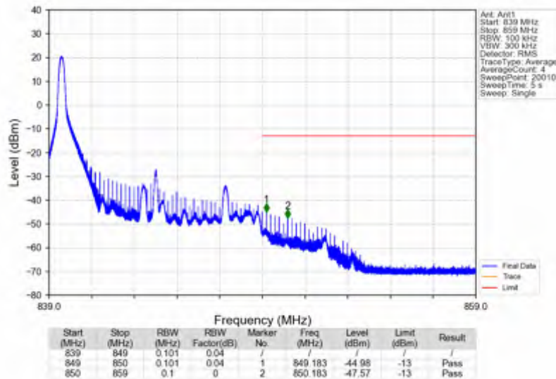
Band26b_10MHz_16QAM_HCH_844MHz_RB_1_49_NTNV
