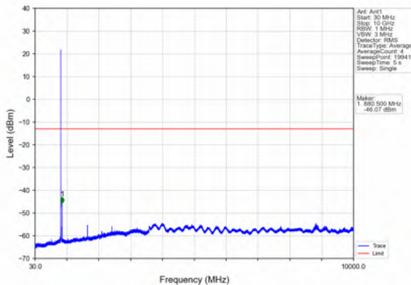
Band26b_5MHz_QPSK_MCH_836.5MHz_RB_1_0_NTNV
