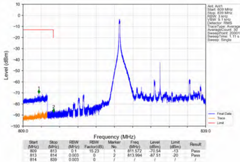
Band26c_15MHz_256QAM_LCH_831.5MHz_RB_1_0_NTNV
