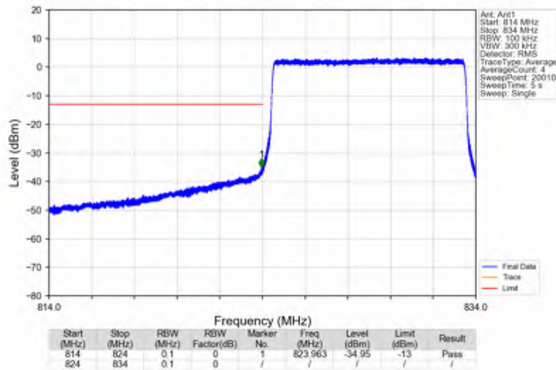
Band26b_10MHz_64QAM_LCH_829MHz_RB_50_0_NTNV
