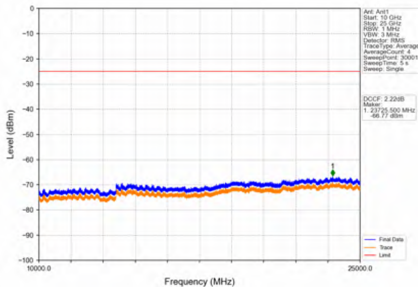
Band38_15MHz_16QAM_LCH_2577.5MHz_RB_1_0_NTNV
