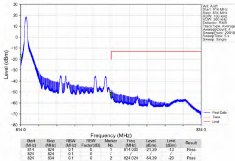
Band26a_10MHz_QPSK_HCH_819MHz_RB_50_0_NTNV
