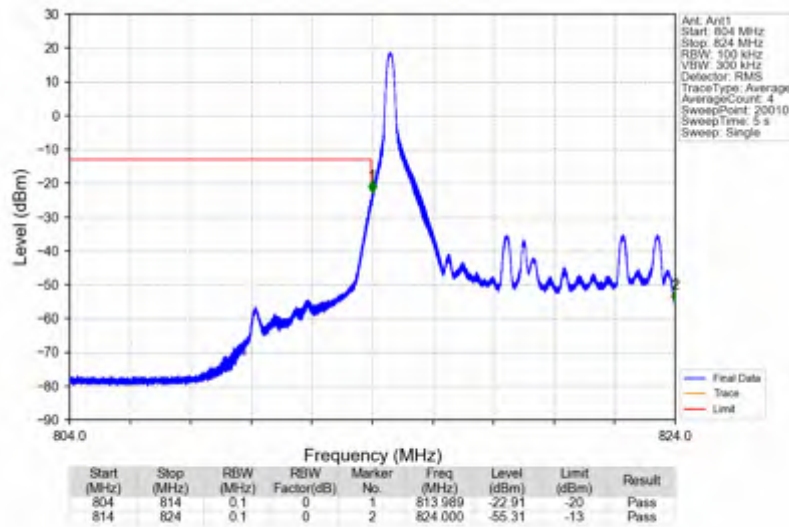
Band26a_10MHz_16QAM_LCH_819MHz_RB_1_0_NTNV
