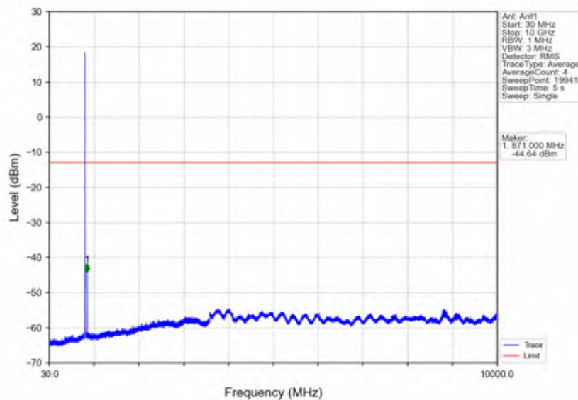
Band26b_5MHz_256QAM_LCH_826.5MHz_RB_25_0_NTNV
