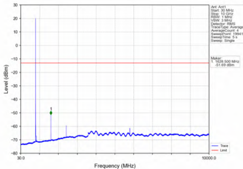
Band26a_3MHz_16QAM_LCH_815.5MHz_RB_15_0_NTNV
