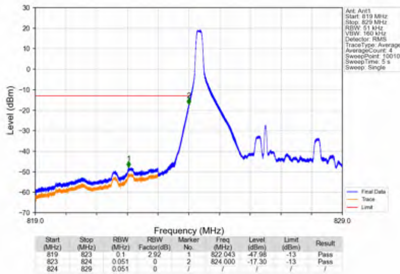
Band26b_5MHz_QPSK_LCH_826.5MHz_RB_1_0_NTNV
