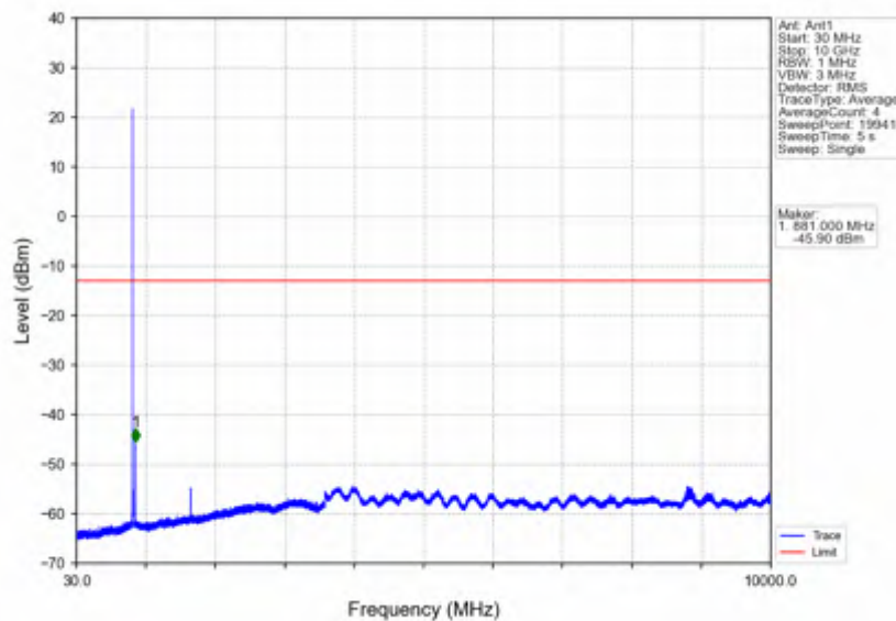
Band26b 3MHz 64QAM MCH 836.5MHz RB 1 0 NTNv
