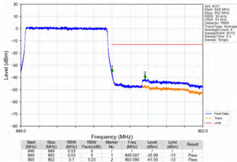
Band26b_3MHz_256QAM_HCH_847.5MHz_RB_15_0_NTNV
