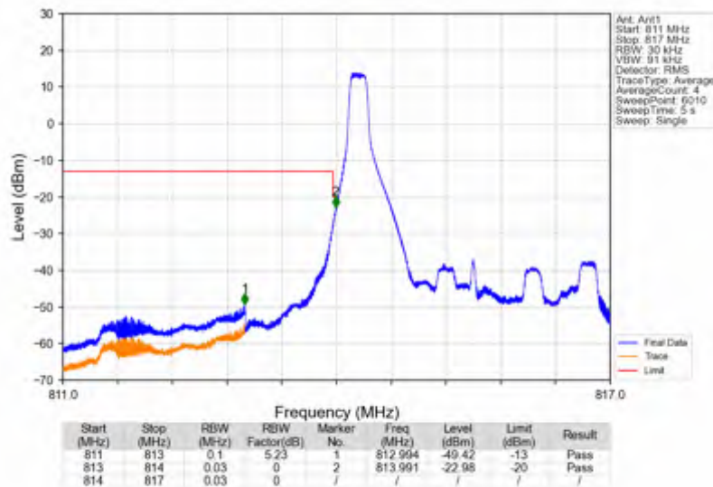
Band26a_3MHz_QPSK_LCH_815.5MHz_RB_1_0_NTNV
