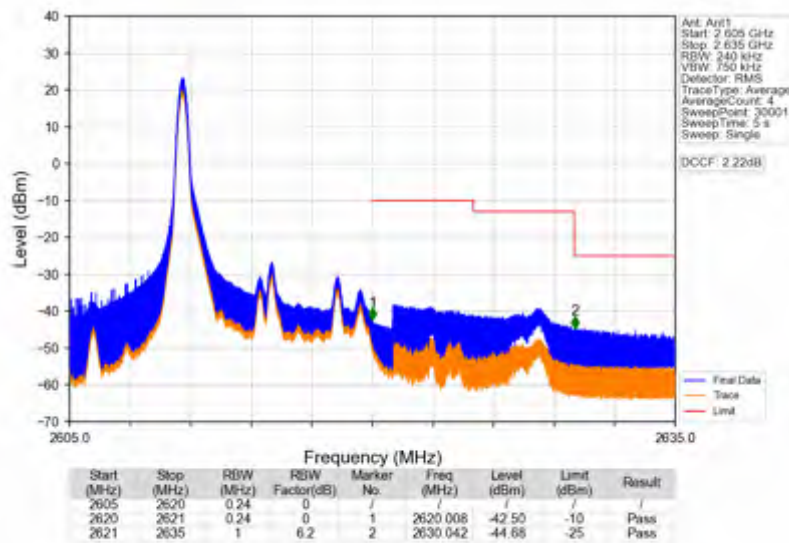
Band38_10MHz_16QAM_HCH_2615MHz_RB_50_0_NTNV
