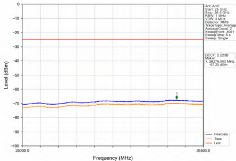
Band38_5MHz_16QAM_LCH_2572.5MHz_RB_25_0_NTNV
