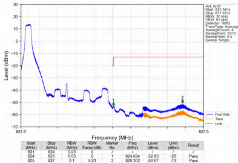
Band26a_3MHz_64QAM_HCH_822.5MHz_RB_1_14_NTNV
