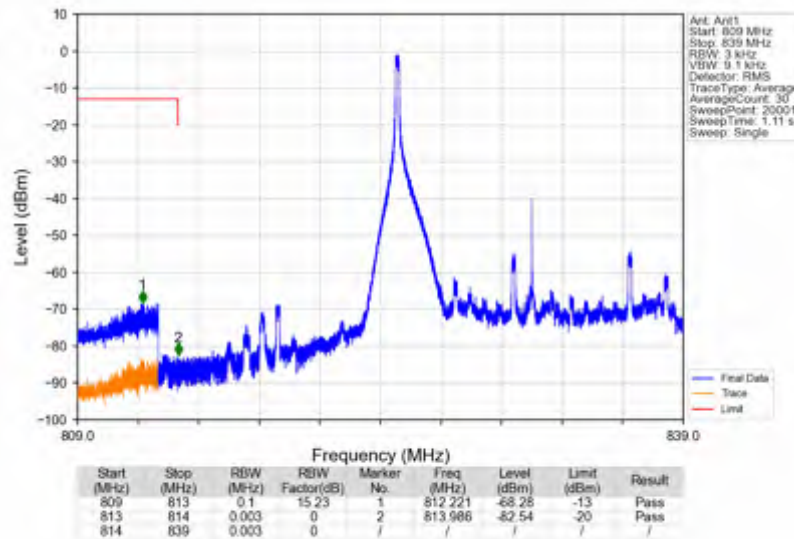
Band26c_15MHz_64QAM_LCH_831.5MHz_RB_1_0_NTNV
