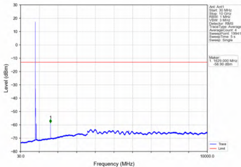
Band26a_10MHz_256QAM_HCH_819MHz_RB_1_0_NTNV
