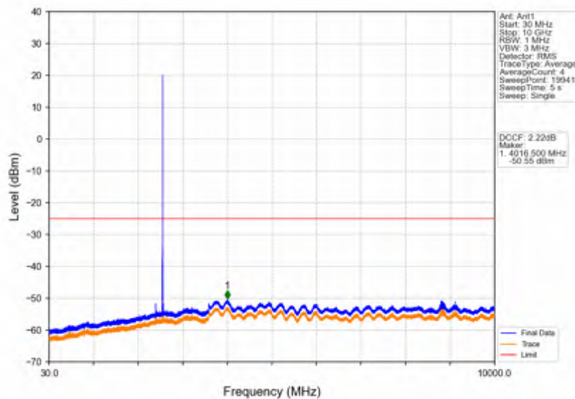
Band38_5MHz_256QAM_LCH_2572.5MHz_RB_1_0_NTNV
