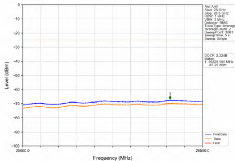
Band38_10MHz_64QAM_MCH_2595MHz_RB_1_0_NTNV
