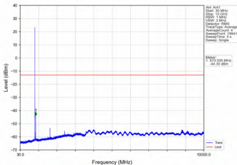
Band26b_5MHz_QPSK_LCH_826.5MHz_RB_1_0_NTNV
