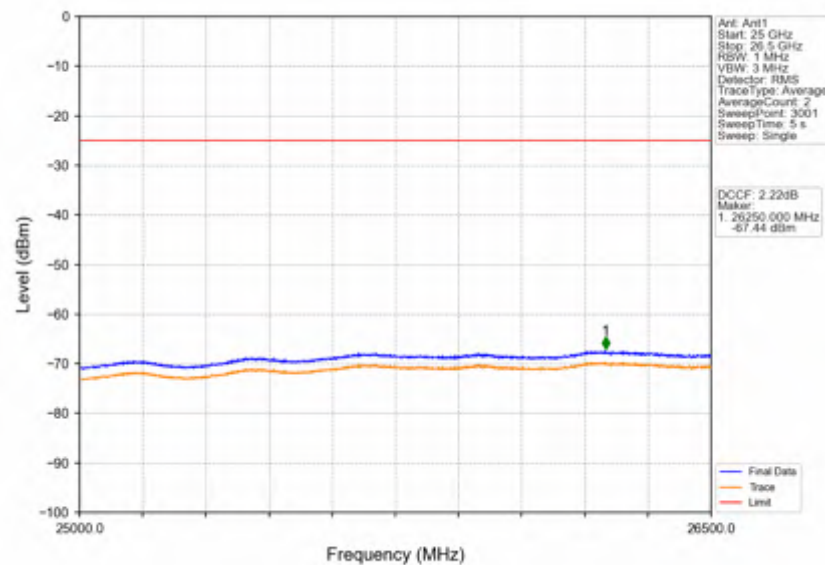
Band38_5MHz_64QAM_HCH_2617.5MHz_RB_1_24_NTNV
