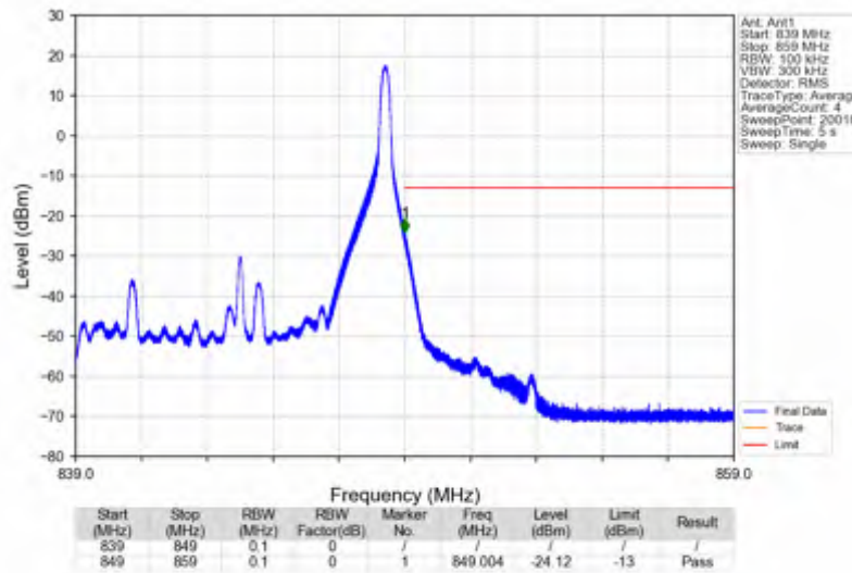
Band26b_10MHz_256QAM_HCH_844MHz_RB_1_49_NTNV
