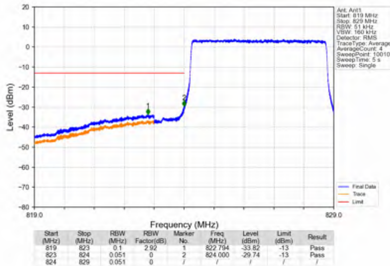
Band26b_5MHz_16QAM_LCH_826.5MHz_RB_25_0_NTNV
