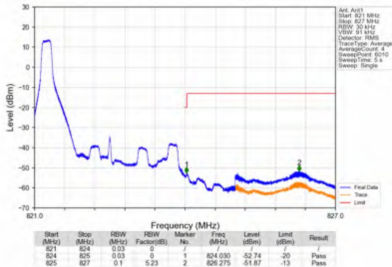
Band26a_3MHz_QPSK_HCH_822.5MHz_RB_1_14_NTNV
