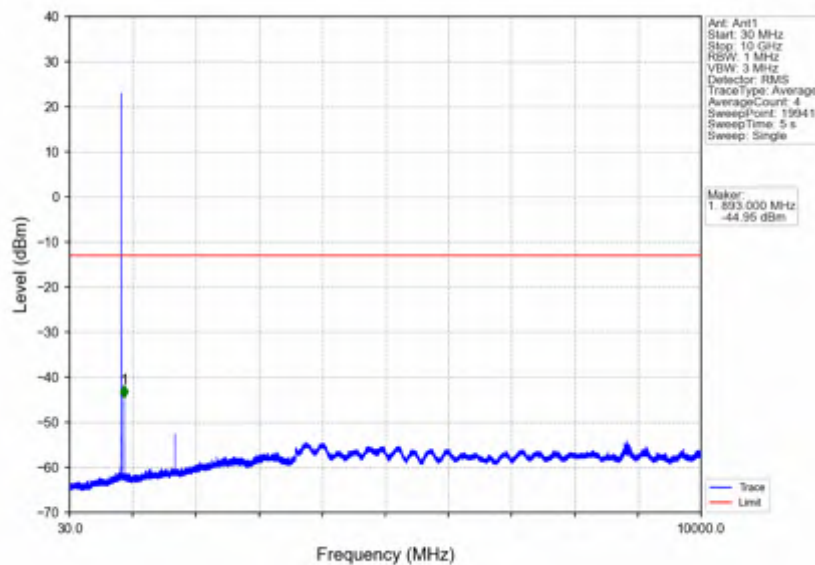
Band26b_1.4MHz_16QAM_HCH_848.3MHz_RB_1_0_NTNV
