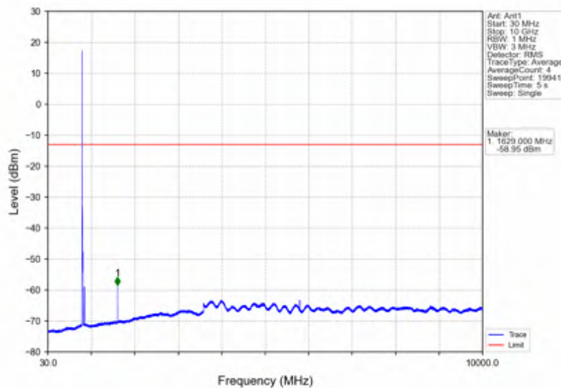
Band26a_10MHz_256QAM_LCH_819MHz_RB_50_0_NTNV
