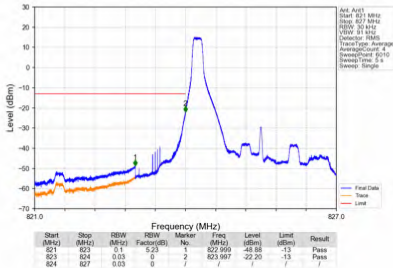
Band26b 3MHz 64QAM LCH 825.5MHz RB 1 0 NTNV
