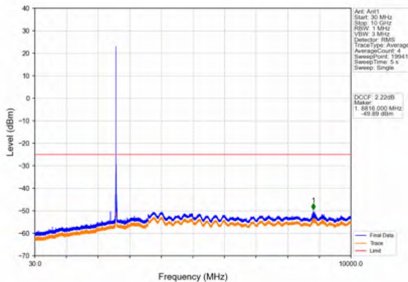
Band38_15MHz_16QAM_MCH_2595MHz_RB_1_0_NTNV
