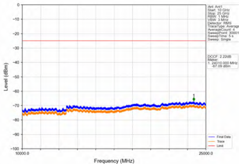
Band38_5MHz_64QAM_HCH_2617.5MHz_RB_1_0_NTNV
