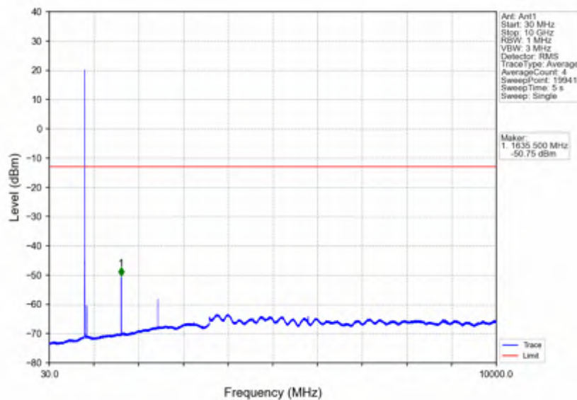
Band26a_3MHz_64QAM_MCH_819MHz_RB_1_0_NTNV
