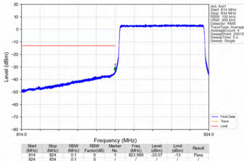
Band26b_10MHz_16QAM_LCH_829MHz_RB_50_0_NTNV
