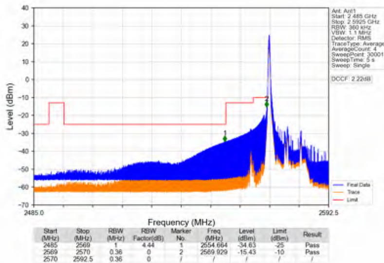
Band38_15MHz_16QAM_LCH_2577.5MHz_RB_1_0_NTNV
