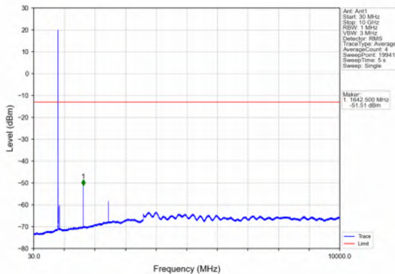
Band26a_3MHz_16QAM_HCH_822.5MHz_RB_1_0_NTNV
