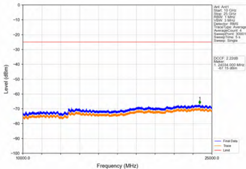
Band38_5MHz_256QAM_MCH_2595MHz_RB_1_0_NTNV
