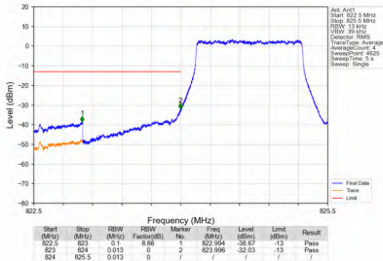
Band26b_1.4MHz_64QAM_LCH_824.7MHz_RB_6_0_NTNV
