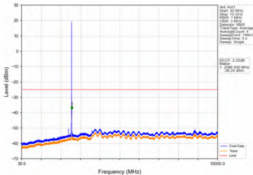
Band38_5MHz_16QAM_LCH_2572.5MHz_RB_1_0_NTNV
