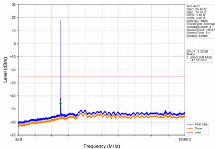
Band38_10MHz_256QAM_LCH_2575MHz_RB_1_0_NTNV
