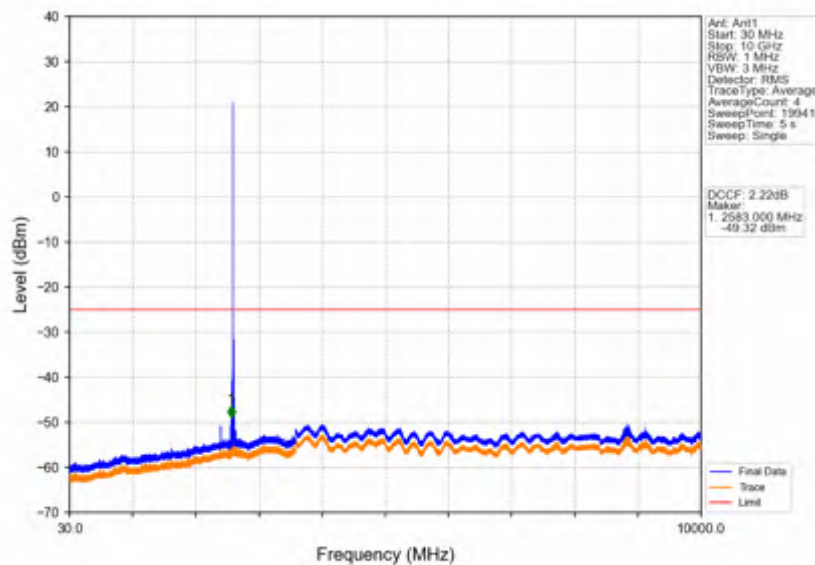
Band38_10MHz_256QAM_HCH_2615MHz_RB_1_0_NTNV
