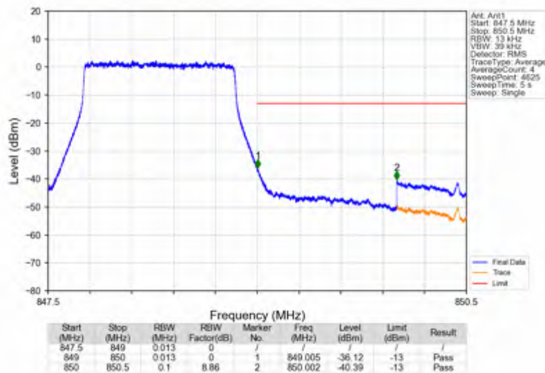
Band26b_1.4MHz_256QAM_HCH_848.3MHz_RB_6_0_NTNV
