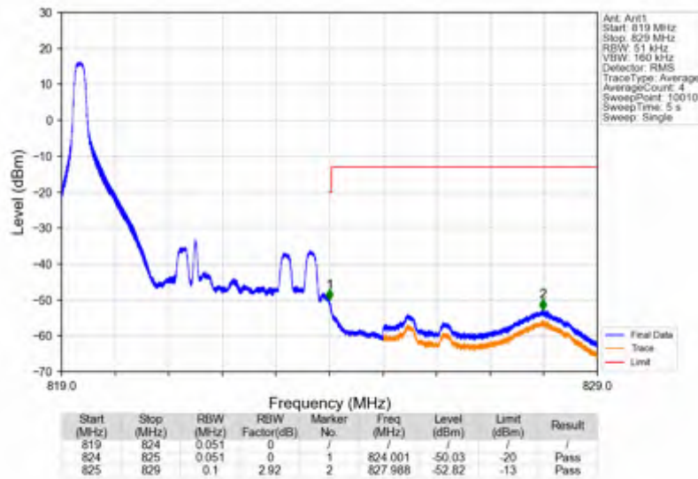
Band26a_5MHz_16QAM_HCH_821.5MHz_RB_1_24_NTNV
