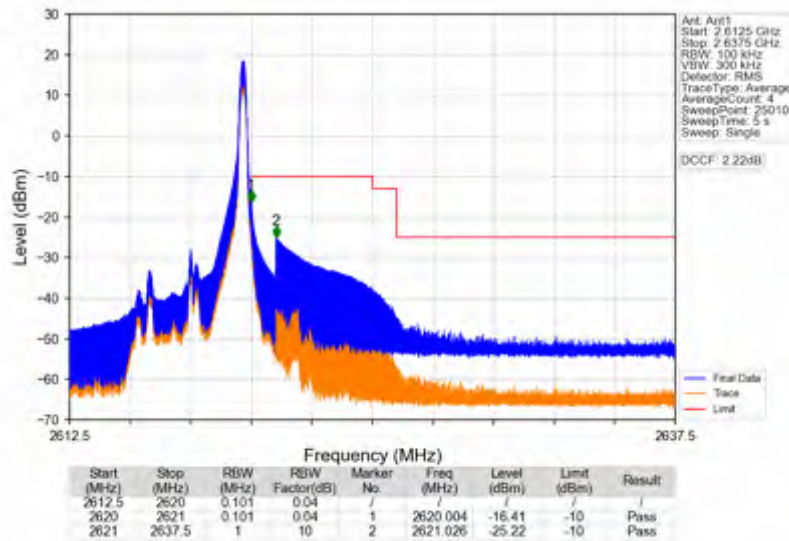
Band38_5MHz_256QAM_HCH_2617.5MHz_RB_1_24_NTNV
