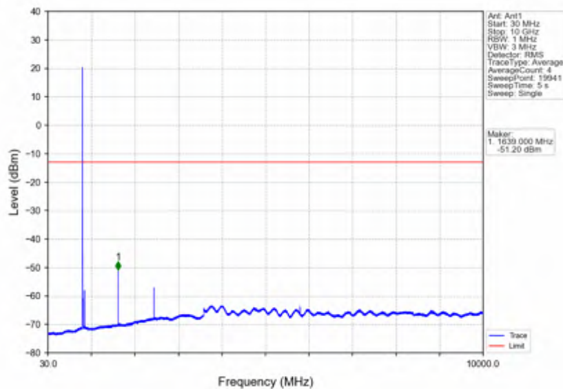
Band26a_5MHz_QPSK_HCH_821.5MHz_RB_1_24_NTNV
