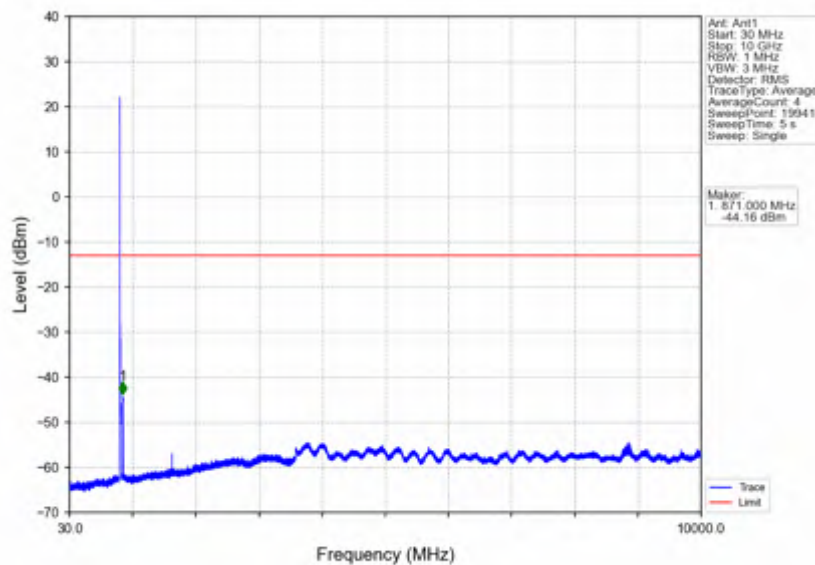
Band26b_10MHz_64QAM_LCH_829MHz_RB_1_0_NTNV
