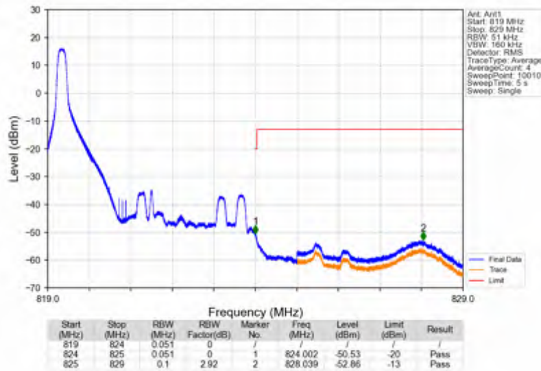
Band26a_5MHz_64QAM_HCH_821.5MHz_RB_25_0_NTNV
