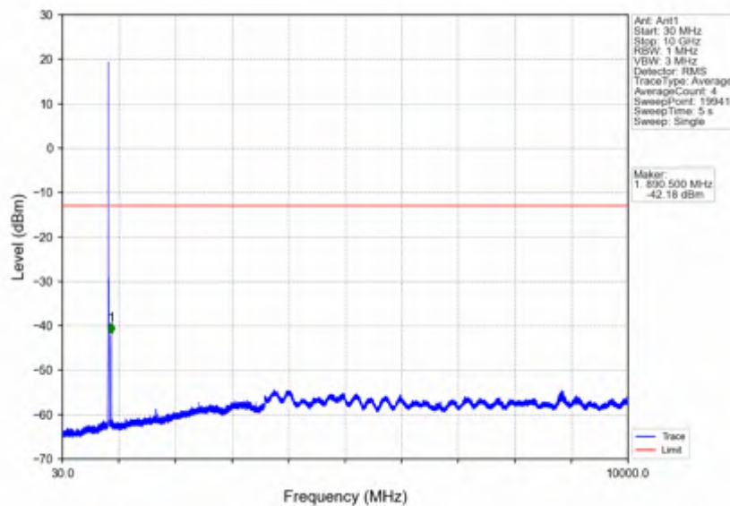
Band26b_10MHz_256QAM_HCH_844MHz_RB_1_0_NTNV
