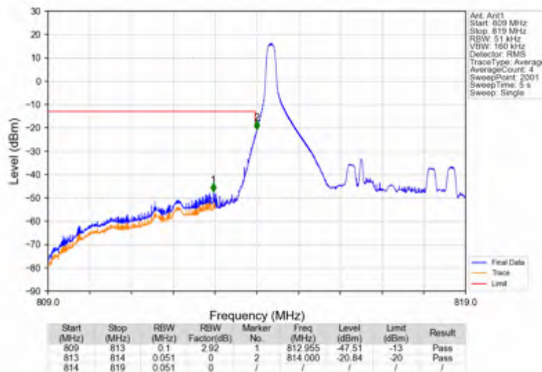
Band26a_5MHz_16QAM_LCH_816.5MHz_RB_1_0_NTNV
