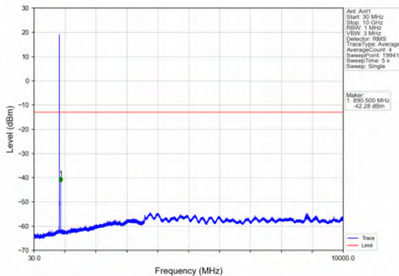
Band26b_5MHz_256QAM_HCH_846.5MHz_RB_1_0_NTNV
