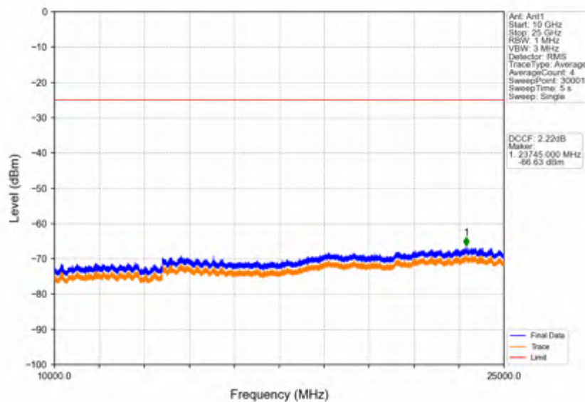
Band38_15MHz_16QAM_MCH_2595MHz_RB_1_0_NTNV
