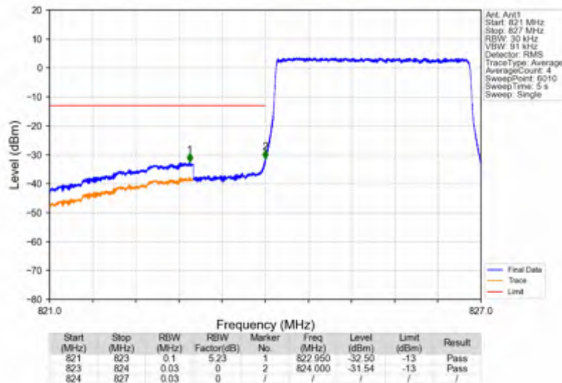
Band26b_3MHz_16QAM_LCH_825.5MHz_RB_15_0_NTNV
