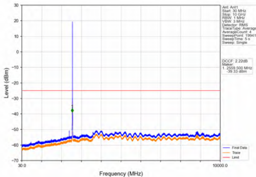
Band38_5MHz_64QAM_LCH_2572.5MHz_RB_1_0_NTNV
