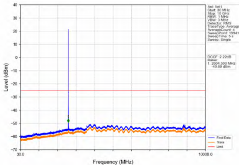
Band38_5MHz_64QAM_HCH_2617.5MHz_RB_1_0_NTNV
