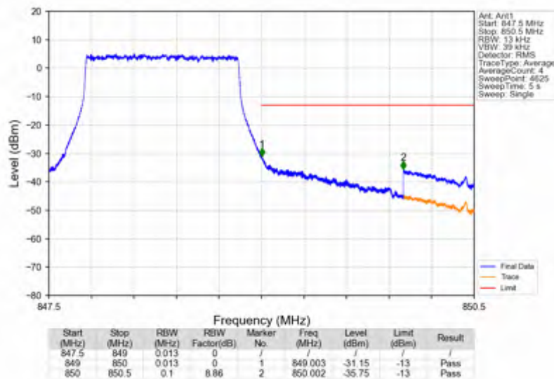
Band26b_1.4MHz_16QAM_HCH_848.3MHz_RB_6_0_NTNV
