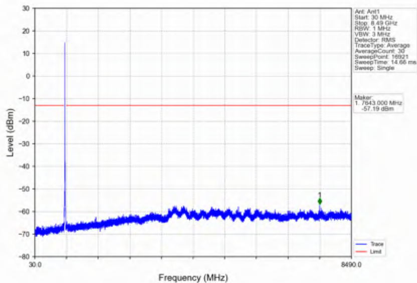
Band26c_15MHz_QPSK_MCH_836.5MHz_RB_1_0_NTNV
