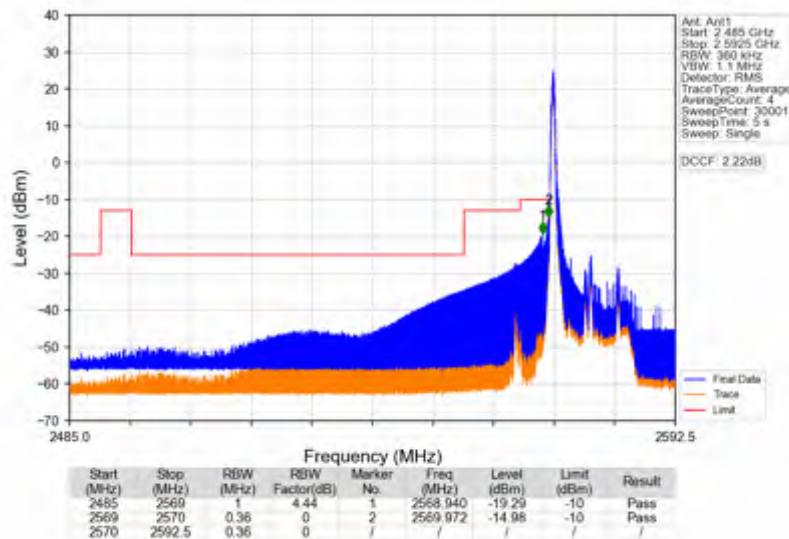
Band38_15MHz_QPSK_LCH_2577.5MHz_RB_1_0_NTNV
