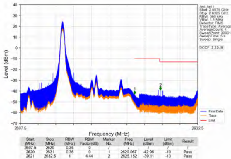
Band38_15MHz_QPSK_HCH_2612.5MHz_RB_1_74_NTNV
