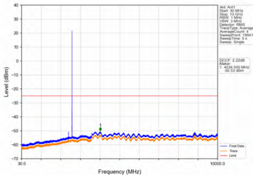
Band38_5MHz_64QAM_MCH_2595MHz_RB_1_0_NTNV
