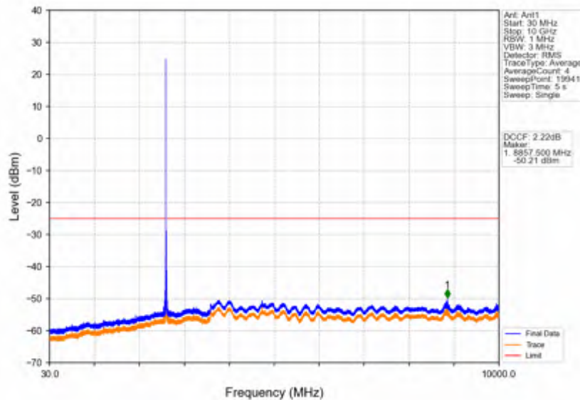
Band38_10MHz_16QAM_HCH_2615MHz_RB_1_0_NTNV
