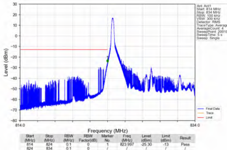
Band26b_10MHz_256QAM_LCH_829MHz_RB_1_0_NTNV
