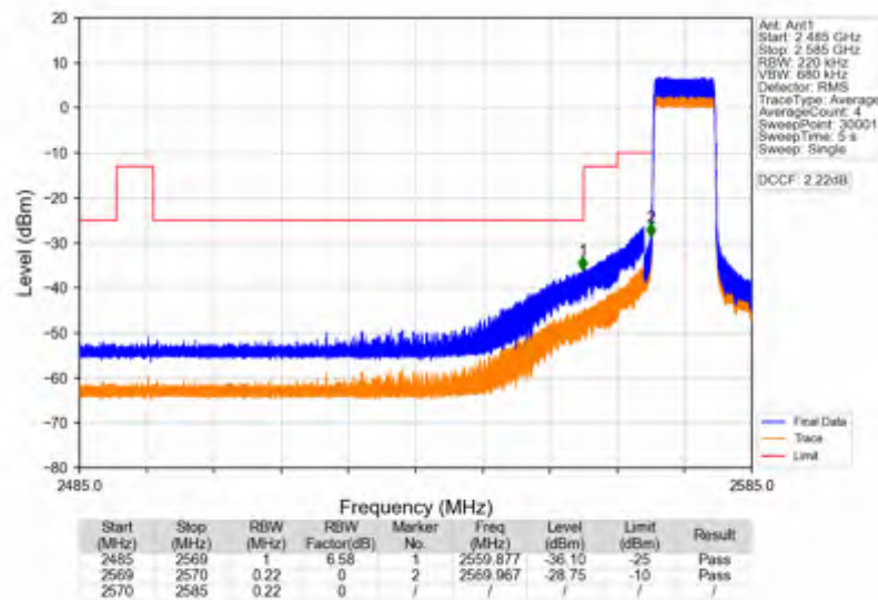
Band38_10MHz_256QAM_LCH_2575MHz_RB_50_0_NTNV
