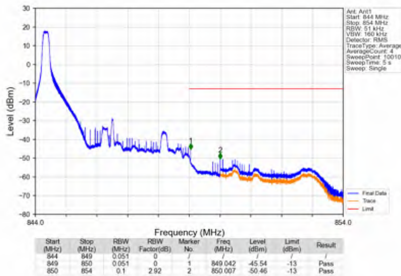
Band26b_5MHz_16QAM_HCH_846.5MHz_RB_25_0_NTNV
