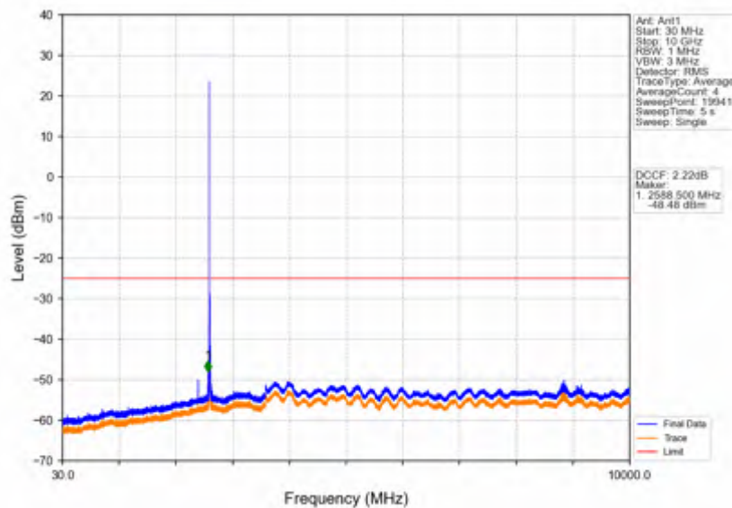
Band38_10MHz_64QAM_HCH_2615MHz_RB_1_0_NTNV
