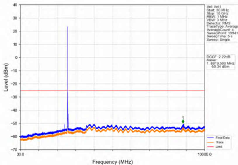
Band38_15MHz_QPSK_MCH_2595MHz_RB_1_0_NTNV
