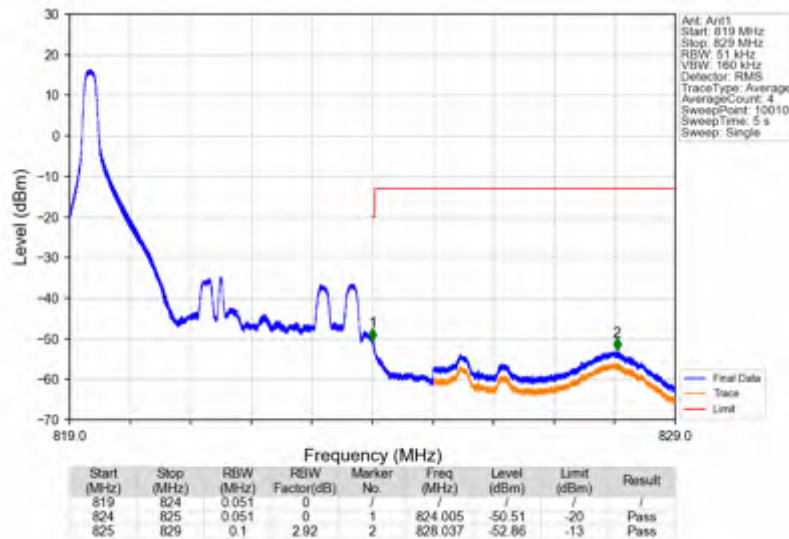
Band26a_5MHz_64QAM_HCH_821.5MHz_RB_1_24_NTNV
