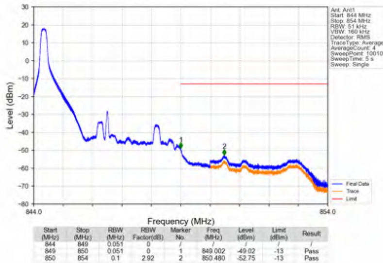
Band26b_5MHz_16QAM_HCH_846.5MHz_RB_1_24_NTNV
