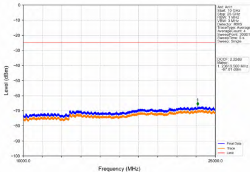
Band38_10MHz_256QAM_MCH_2595MHz_RB_1_0_NTNV
