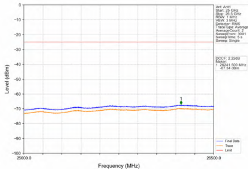
Band38_10MHz_256QAM_LCH_2575MHz_RB_50_0_NTNV
