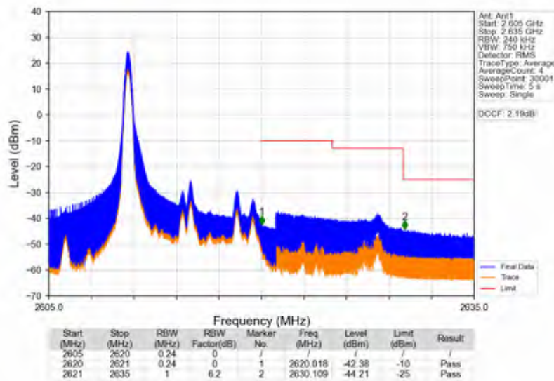
Band38_10MHz_64QAM_HCH_2615MHz_RB_1_49_NTNV
