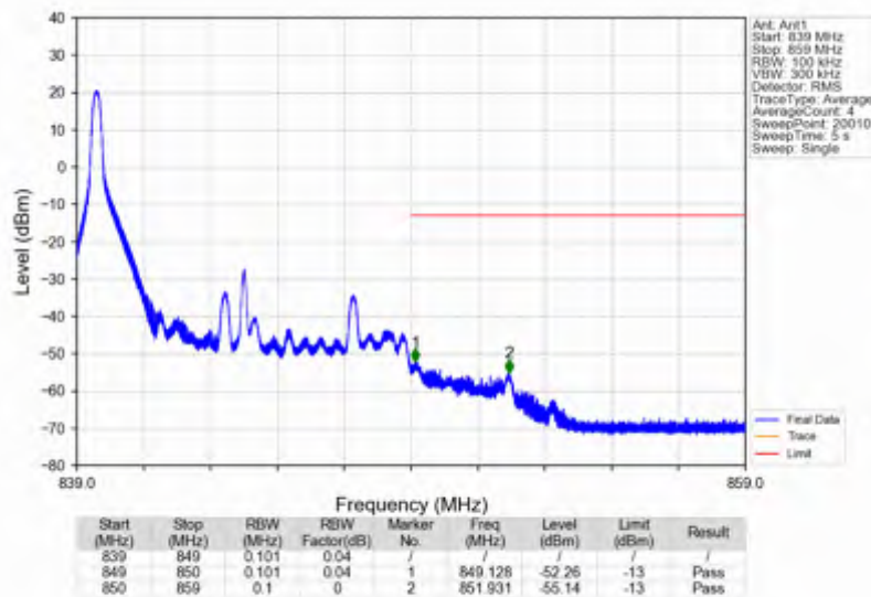
Band26b_10MHz_16QAM_HCH_844MHz_RB_50_0_NTNV
