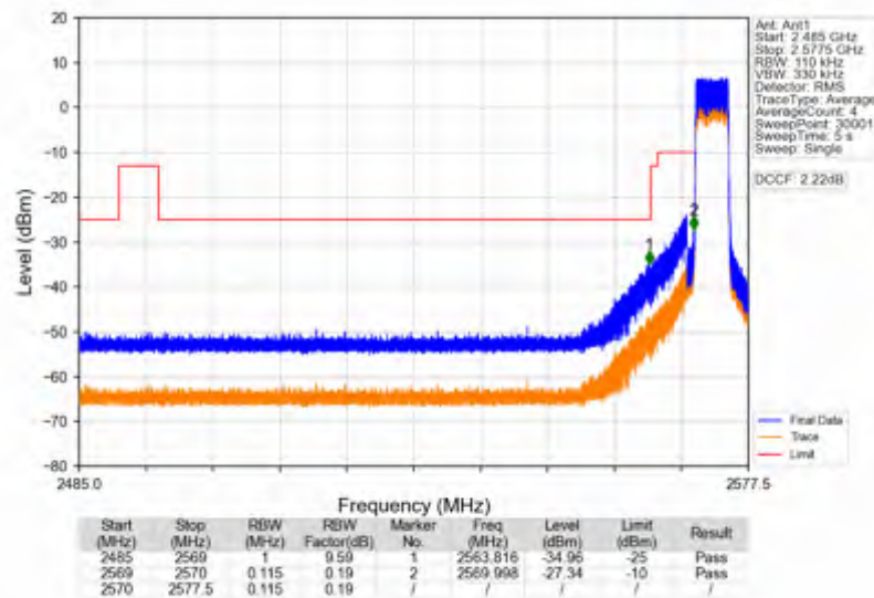
Band38_5MHz_256QAM_LCH_2572.5MHz_RB_25_0_NTNV
