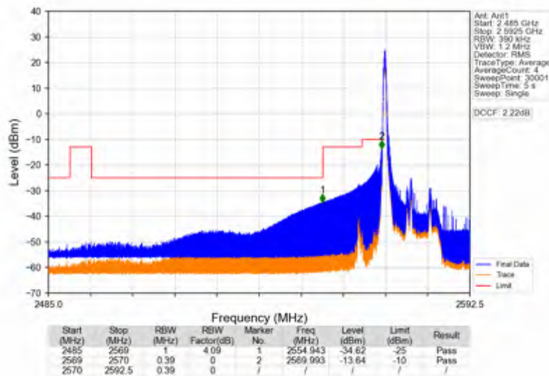
Band38_15MHz_16QAM_LCH_2577.5MHz_RB_75_0_NTNV
