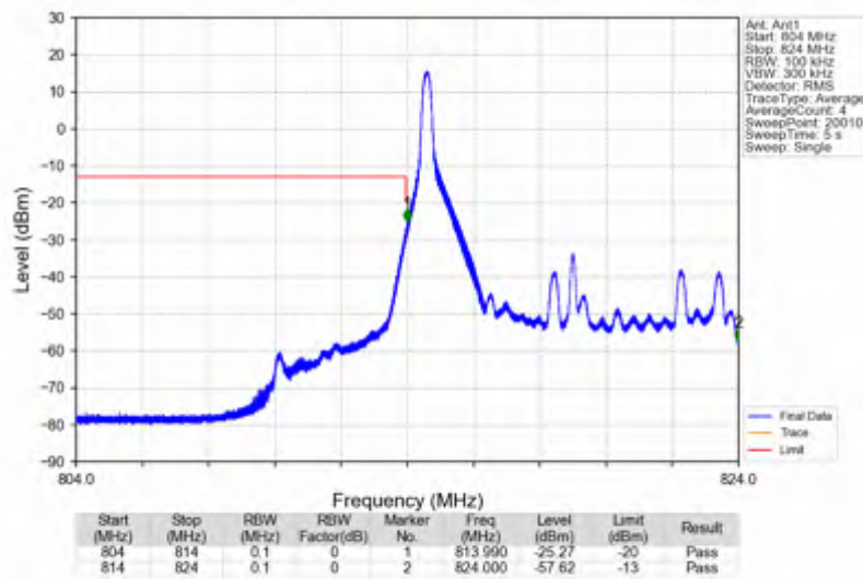
Band26a_10MHz_256QAM_LCH_819MHz_RB_1_0_NTNV
