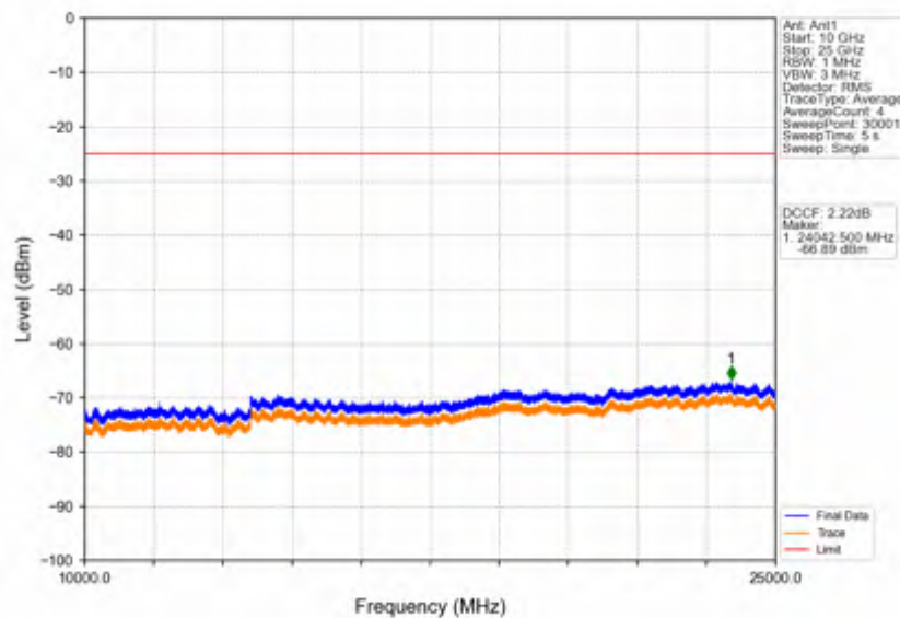
Band38_5MHz_256QAM_HCH_2617.5MHz_RB_1_0_NTNV
