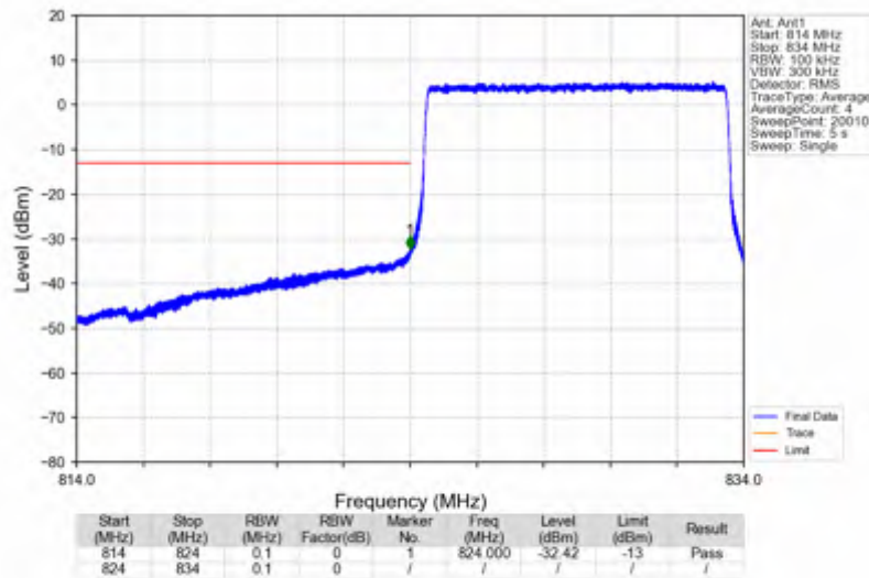
Band26b_10MHz_QPSK_LCH_829MHz_RB_50_0_NTNV
