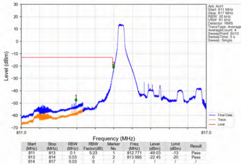
Band26a_3MHz_16QAM_LCH_815.5MHz_RB_15_0_NTNV
