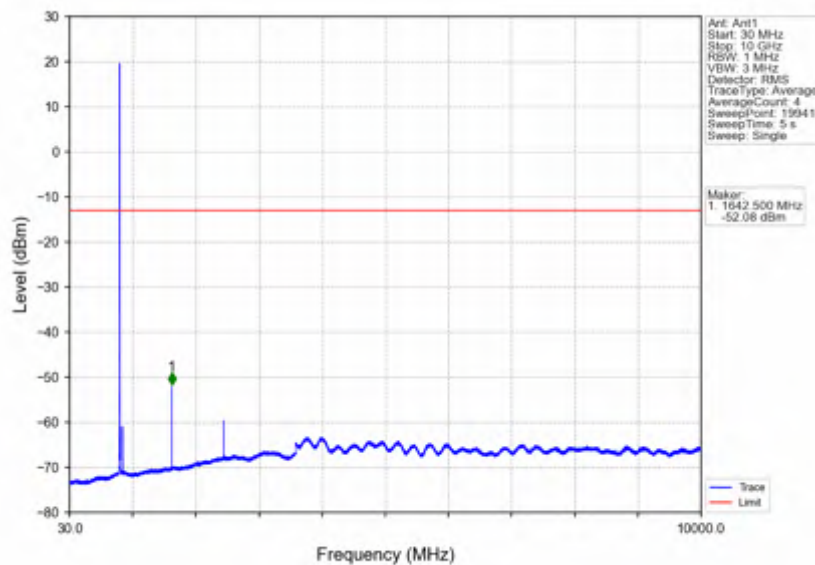
Band26a_3MHz_QPSK_HCH_822.5MHz_RB_1_14_NTNV
