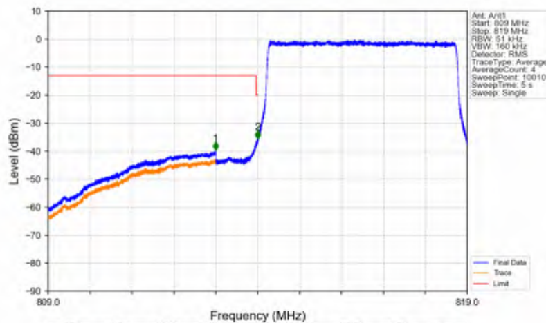
Band26a_5MHz_256QAM_LCH_816.5MHz_RB_25_0_NTNV
