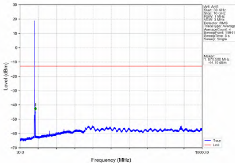
Band26b_10MHz_256QAM_LCH_829MHz_RB_50_0_NTNV
