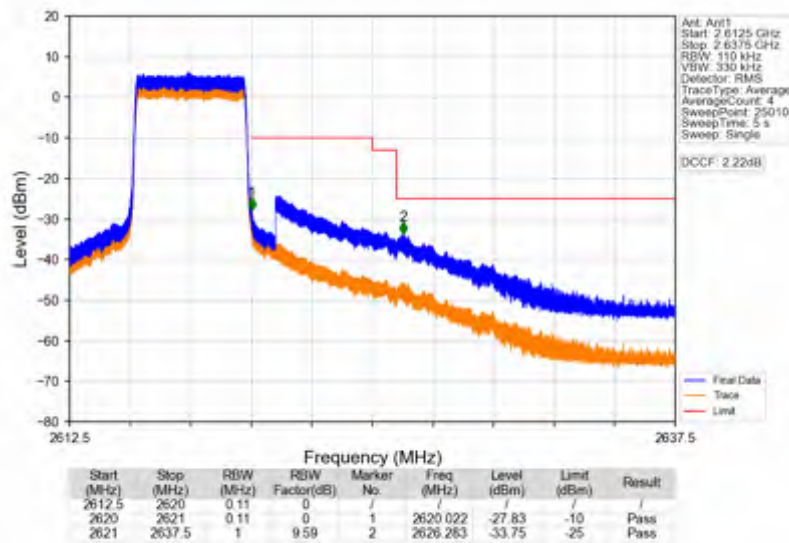
Band38_5MHz_256QAM_HCH_2617.5MHz_RB_25_0_NTNV
