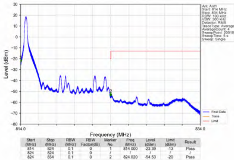
Band26a_10MHz_16QAM_HCH_819MHz_RB_1_49_NTNV
