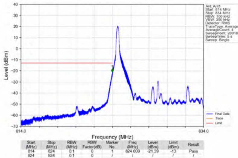
Band26b 10MHz 64QAM LCH 829MHz RB 1 0 NTNV
