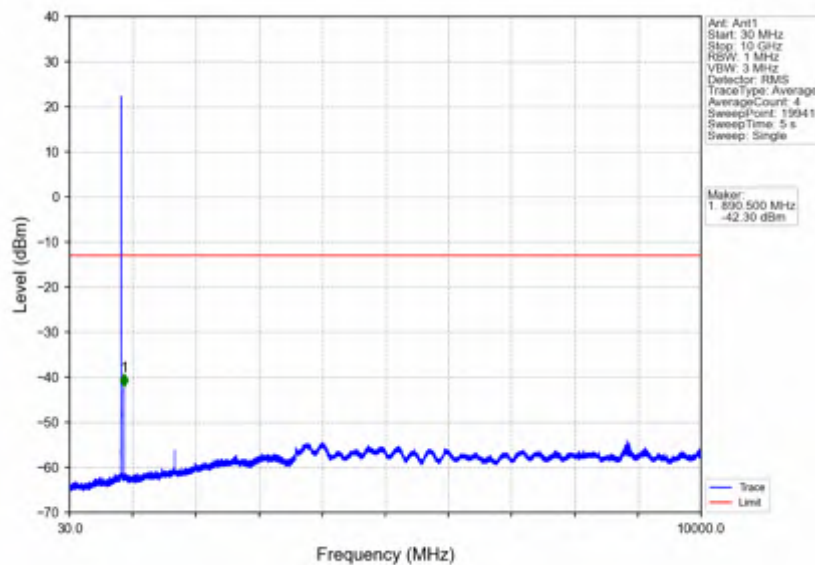
Band26b_5MHz_64QAM_HCH_846.5MHz_RB_1_24_NTNV
