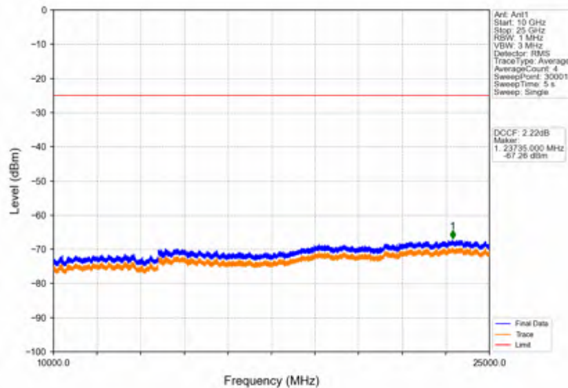
Band38_5MHz_64QAM_LCH_2572.5MHz_RB_1_0_NTNV
