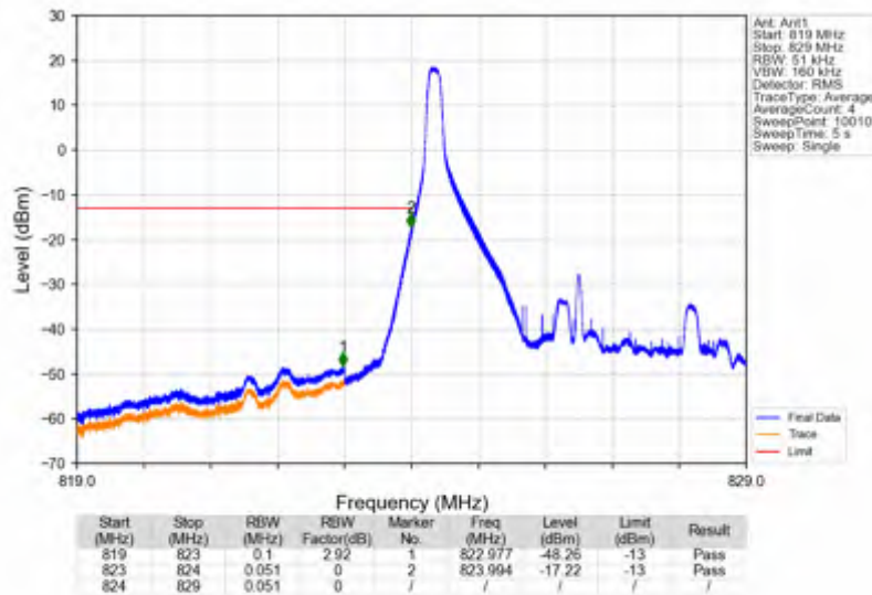
Band26b_5MHz_16QAM_LCH_826.5MHz_RB_1_0_NTNV
