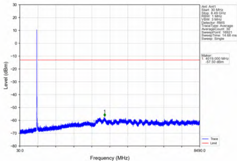
Band26c_15MHz_256QAM_LCH_831.5MHz_RB_75_0_NTNV
