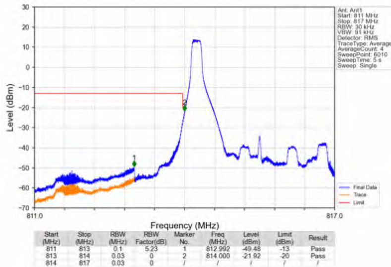
Band26a_3MHz_64QAM_LCH_815.5MHz_RB_15_0_NTNV
