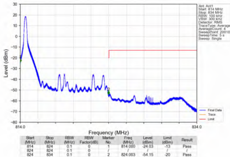
Band26a_10MHz_64QAM_HCH_819MHz_RB_1_49_NTNV
