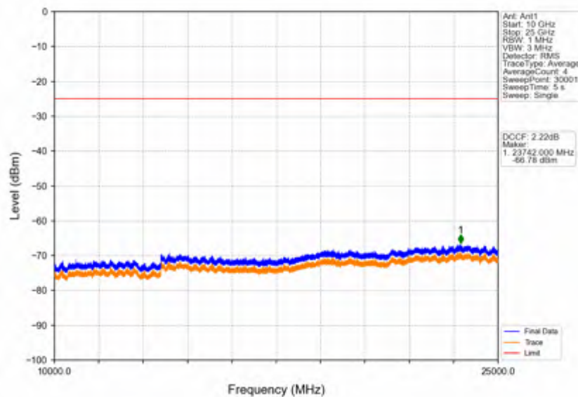
Band38_15MHz_QPSK_LCH_2577.5MHz_RB_1_0_NTNV
