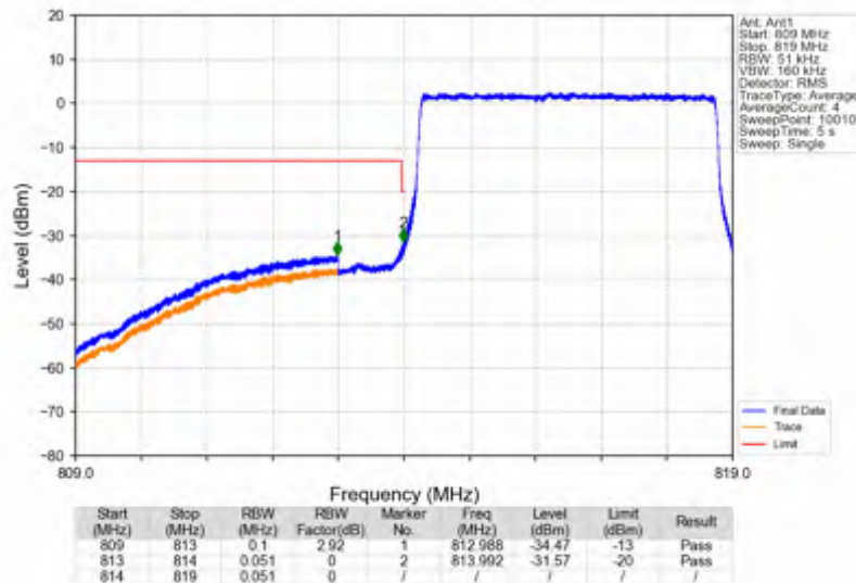
Band26a_5MHz_16QAM_LCH_816.5MHz_RB_25_0_NTNV
