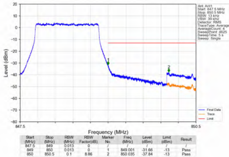
Band26b_1.4MHz_64QAM_HCH_848.3MHz_RB_6_0_NTNV
