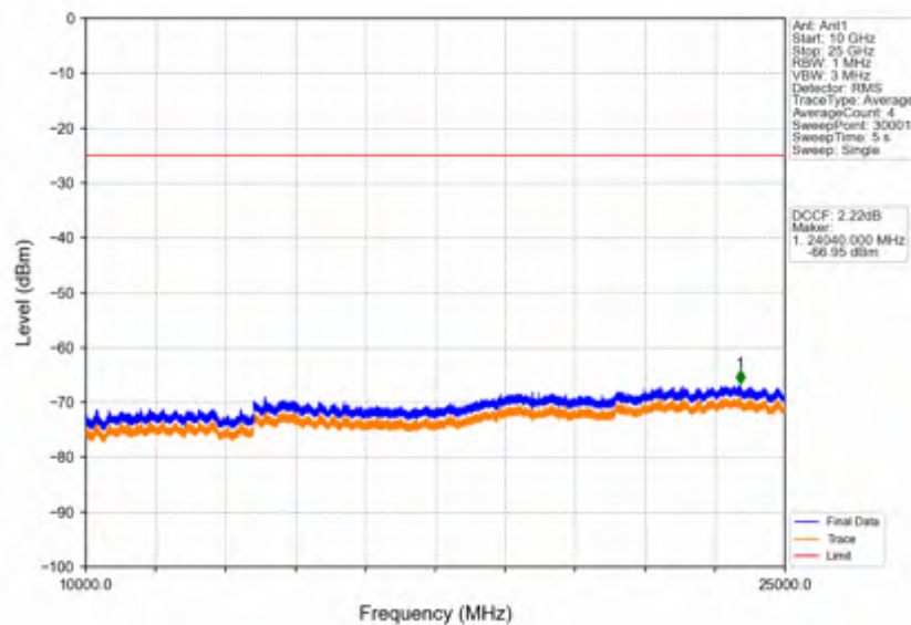
Band38_15MHz_QPSK_MCH_2595MHz_RB_1_0_NTNV
