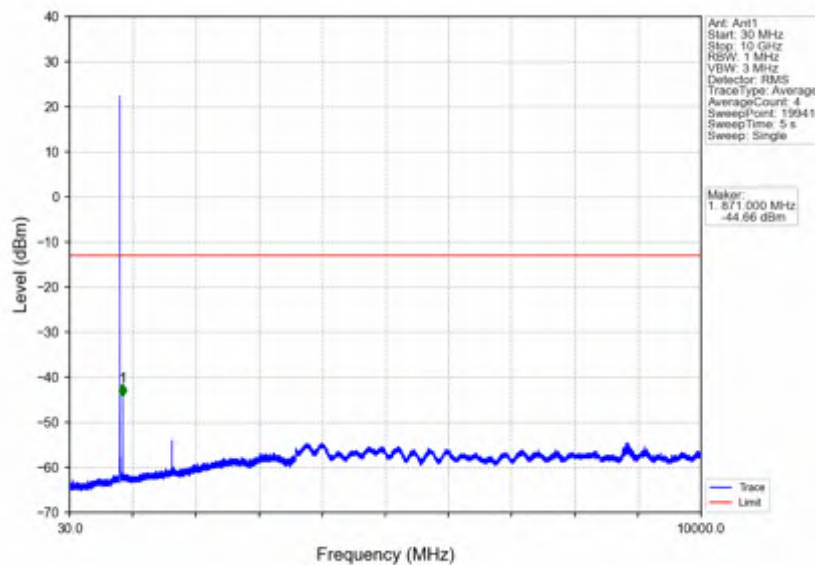
Band26b_3MHz_16QAM_LCH_825.5MHz_RB_15_0_NTNV
