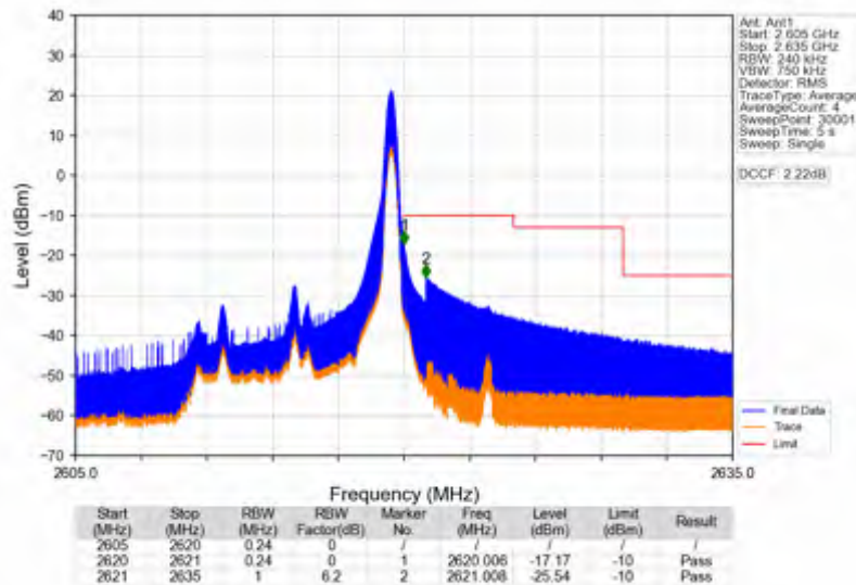
Band38_10MHz_256QAM_HCH_2615MHz_RB_1_49_NTNV
