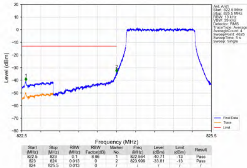
Band26b_1.4MHz_256QAM_LCH_824.7MHz_RB_6_0_NTNV
