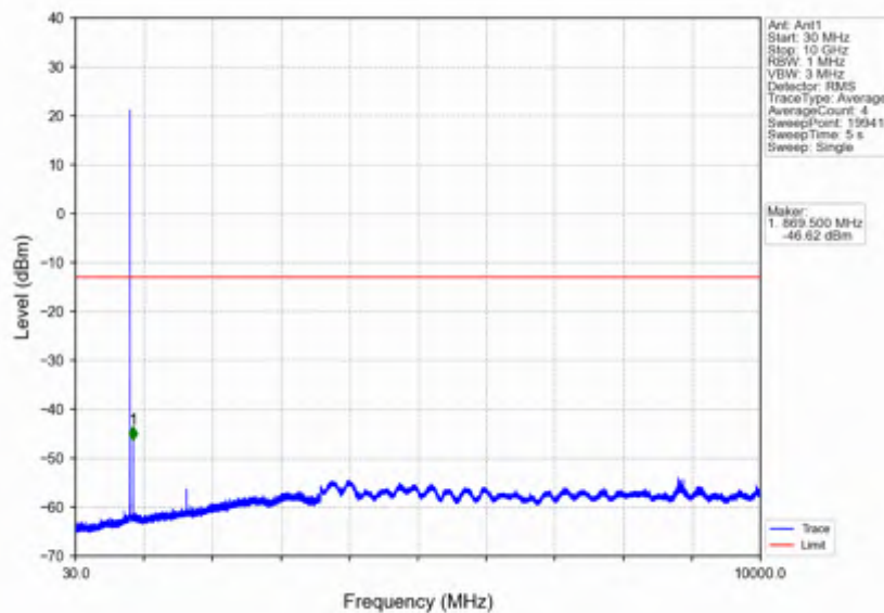
Band26b_1.4MHz_64QAM_LCH_824.7MHz_RB_1_0_NTNV
