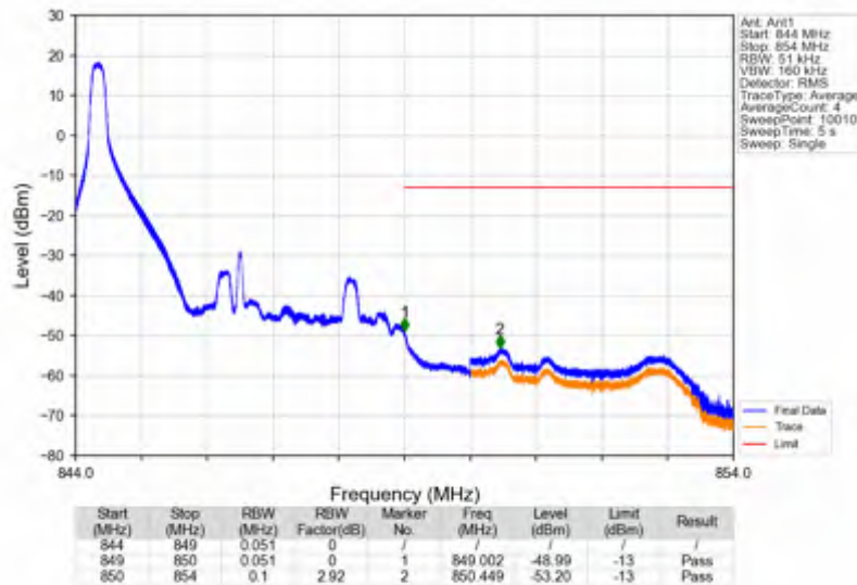
Band26b_5MHz_64QAM_HCH_846.5MHz_RB_1_24_NTNV
