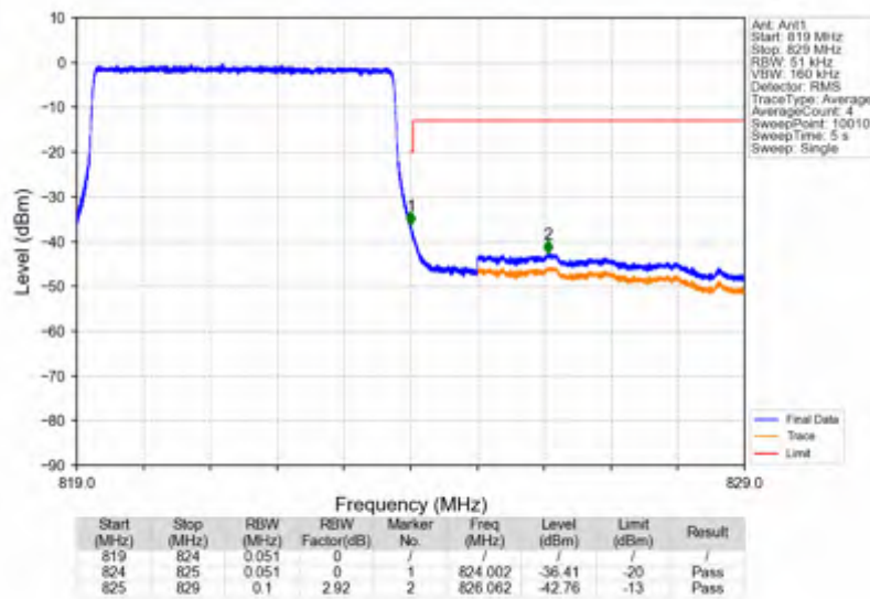
Band26a_5MHz_256QAM_HCH_821.5MHz_RB_25_0_NTNV
