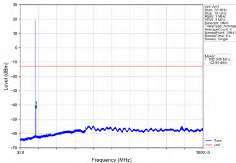
Band26b_3MHz_256QAM_HCH_847.5MHz_RB_1_0_NTNV
