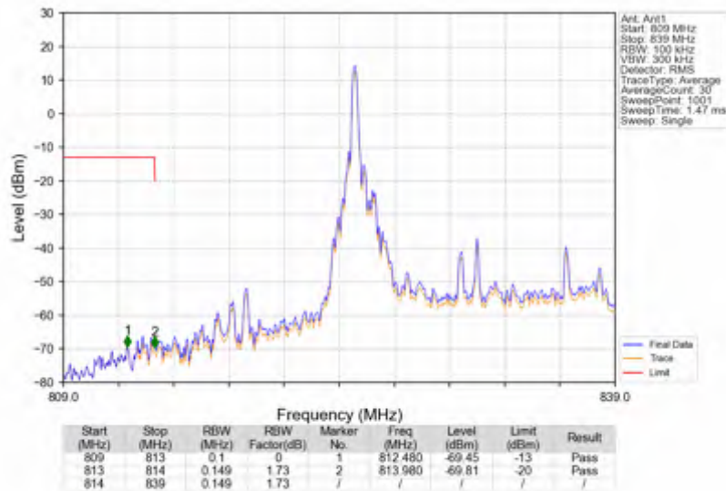
Band26c_15MHz_16QAM_LCH_831.5MHz_RB_75_0_NTNV
