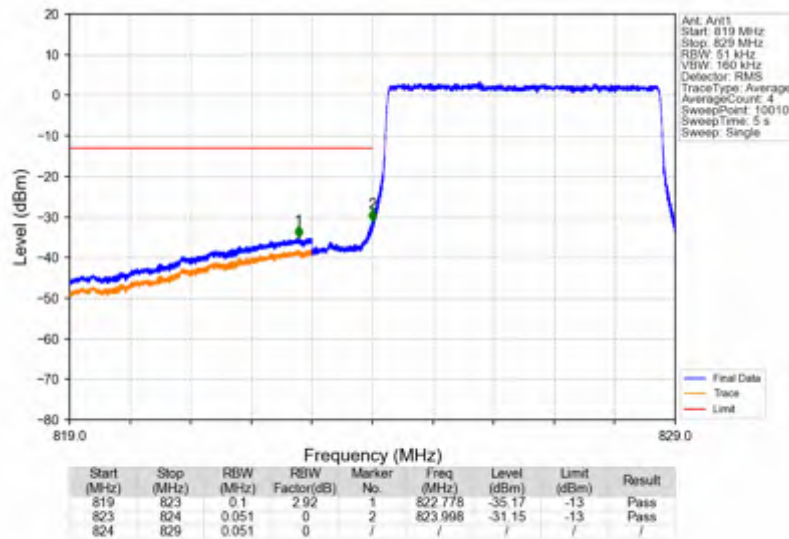
Band26b 5MHz 64QAM LCH 826.5MHz RB 25 0 NTNv
