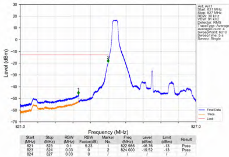
Band26b_3MHz_QPSK_LCH_825.5MHz_RB_1_0_NTNV
