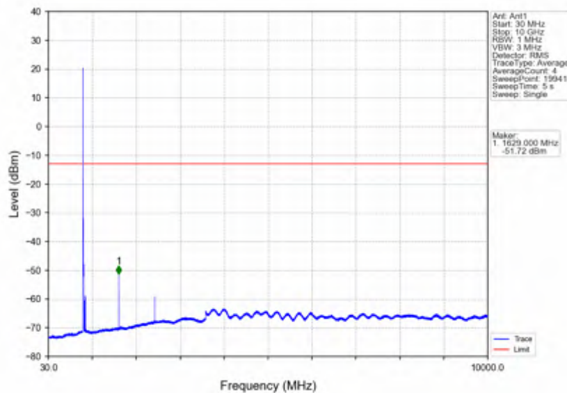
Band26a_10MHz_64QAM_HCH_819MHz_RB_1_49_NTNV
