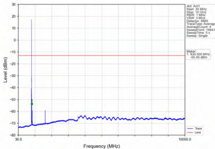
Band26a_5MHz_256QAM_HCH_821.5MHz_RB_1_0_NTNV
