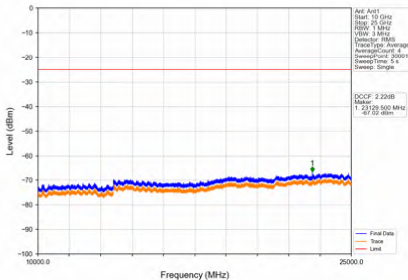
Band38_5MHz_256QAM_LCH_2572.5MHz_RB_1_0_NTNV
