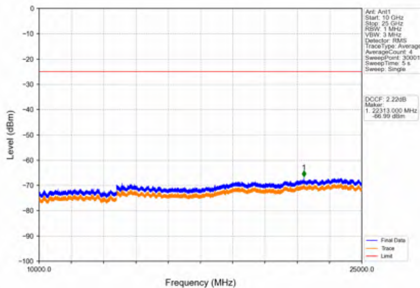
Band38_10MHz_16QAM_MCH_2595MHz_RB_1_0_NTNV
