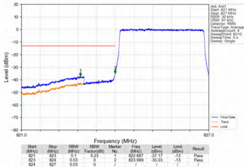
Band26b_3MHz_256QAM_LCH_825.5MHz_RB_15_0_NTNV
