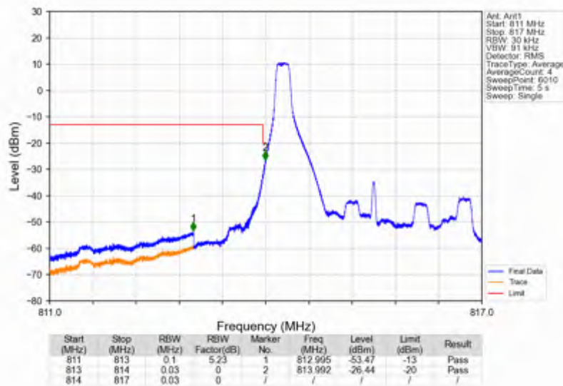
Band26a_3MHz_256QAM_LCH_815.5MHz_RB_1_0_NTNV
