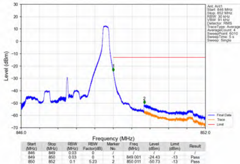
Band26b_3MHz_256QAM_HCH_847.5MHz_RB_1_14_NTNV
