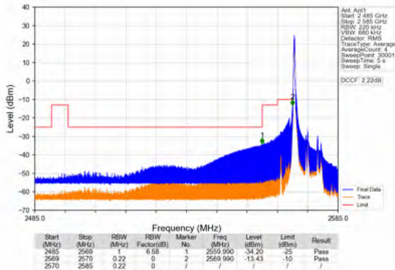
Band38_10MHz_16QAM_LCH_2575MHz_RB_50_0_NTNV
