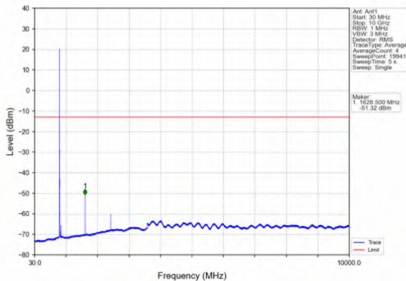
Band26a_5MHz_16QAM_LCH_816.5MHz_RB_25_0_NTNV
