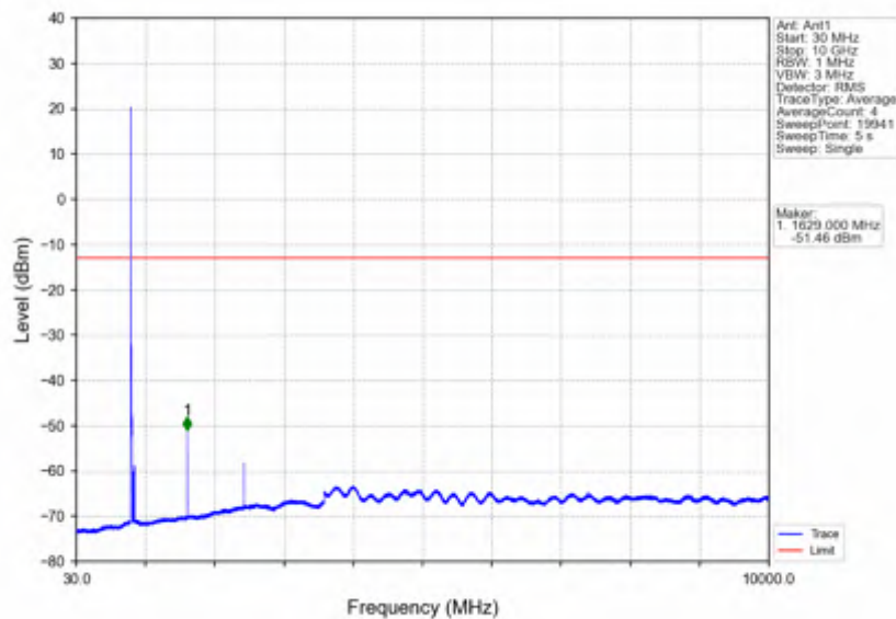
Band26a_10MHz_16QAM_LCH_819MHz_RB_50_0_NTNV
