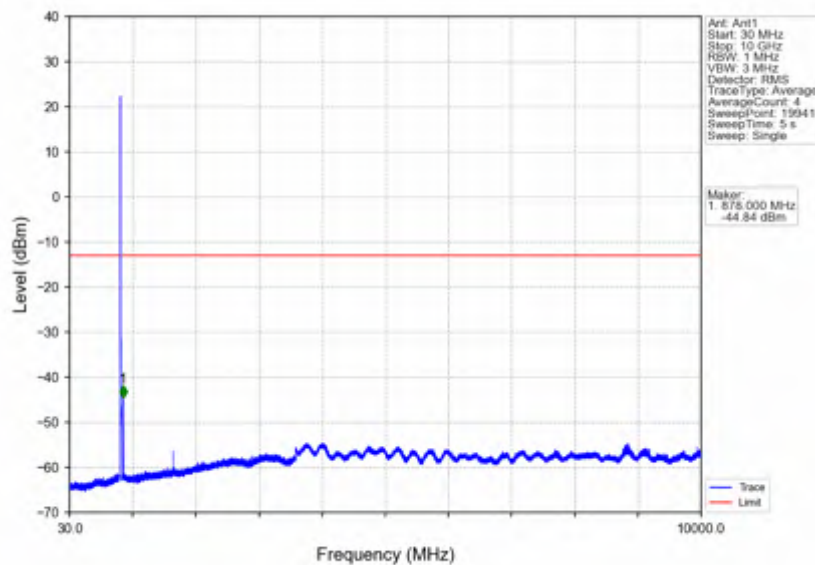
Band26b_10MHz_16QAM_HCH_844MHz_RB_1_0_NTNV
