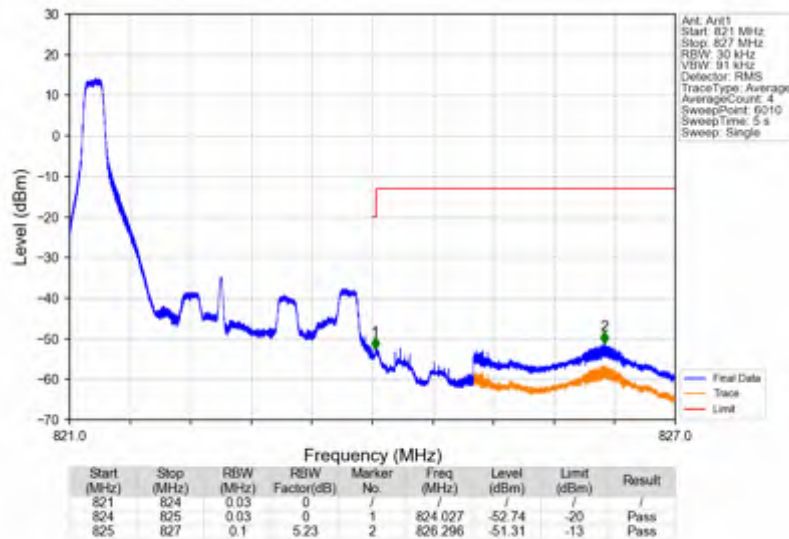
Band26a_3MHz_16QAM_HCH_822.5MHz_RB_15_0_NTNV
