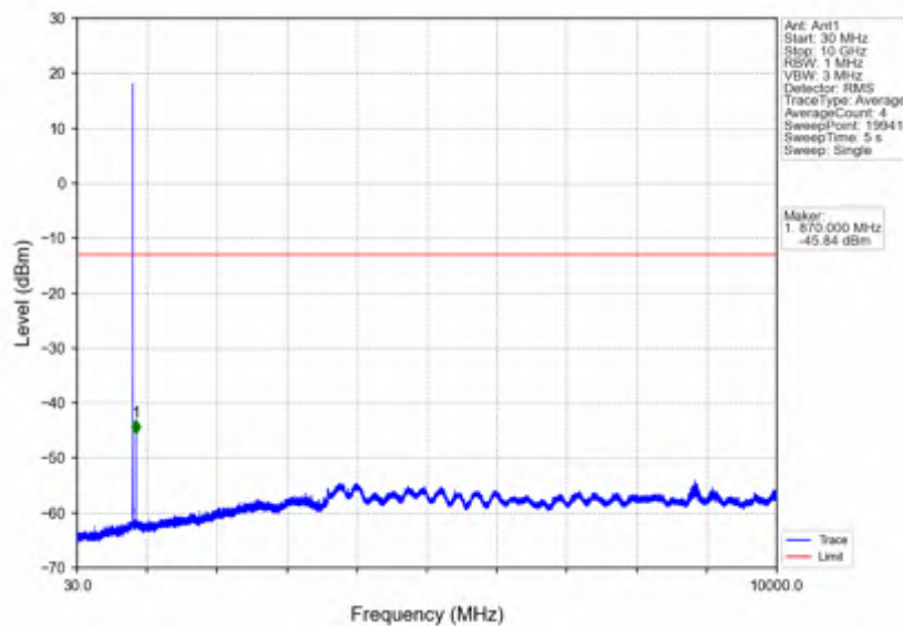
Band26b_1.4MHz_256QAM_LCH_824.7MHz_RB_6_0_NTNV
