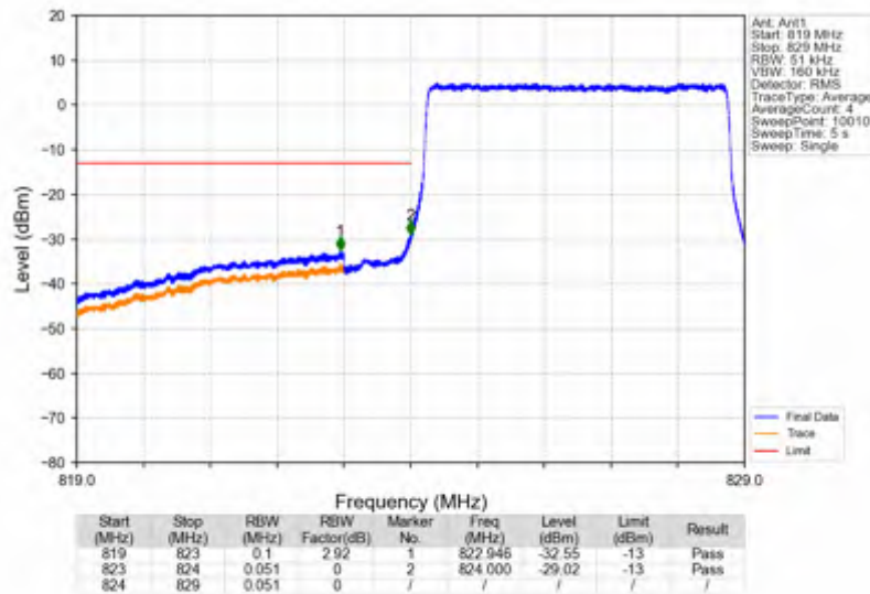
Band26b_5MHz_QPSK_LCH_826.5MHz_RB_25_0_NTNV
