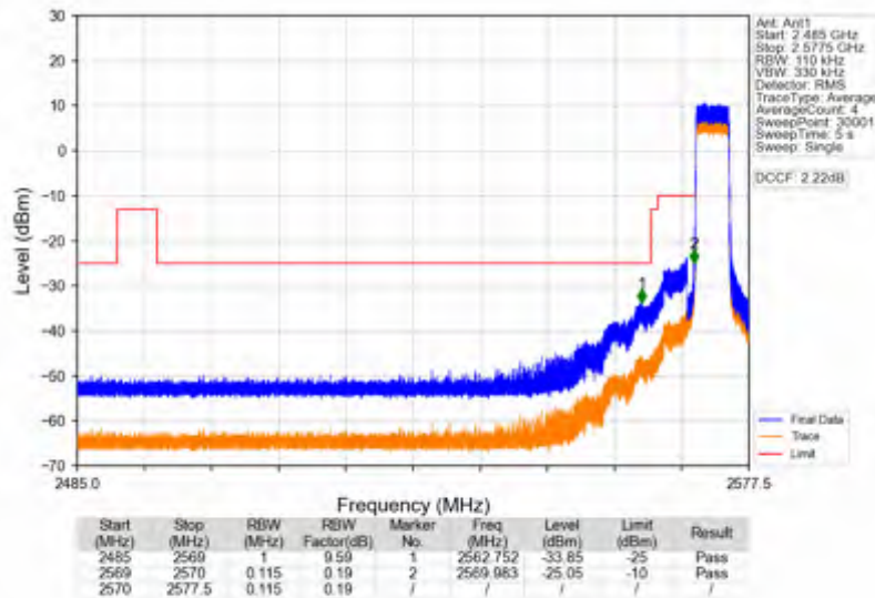
Band38_5MHz_64QAM_LCH_2572.5MHz_RB_25_0_NTNV
