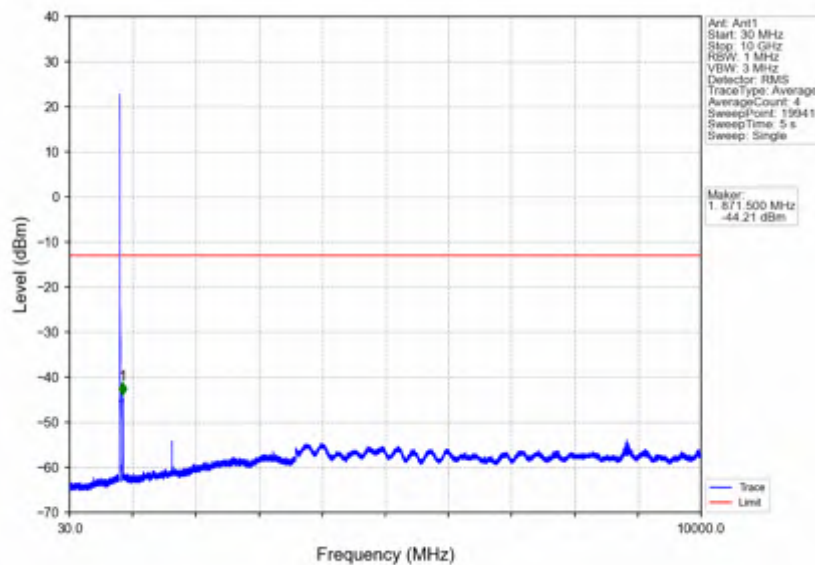
Band26b_10MHz_16QAM_LCH_829MHz_RB_50_0_NTNV
