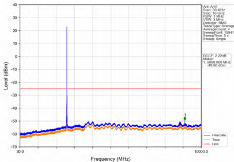
Band38_15MHz_QPSK_HCH_2612.5MHz_RB_1_0_NTNV
