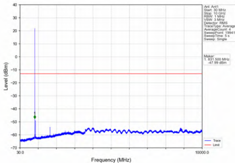
Band26b_1.4MHz_64QAM_MCH_836.5MHz_RB_1_0_NTNV
