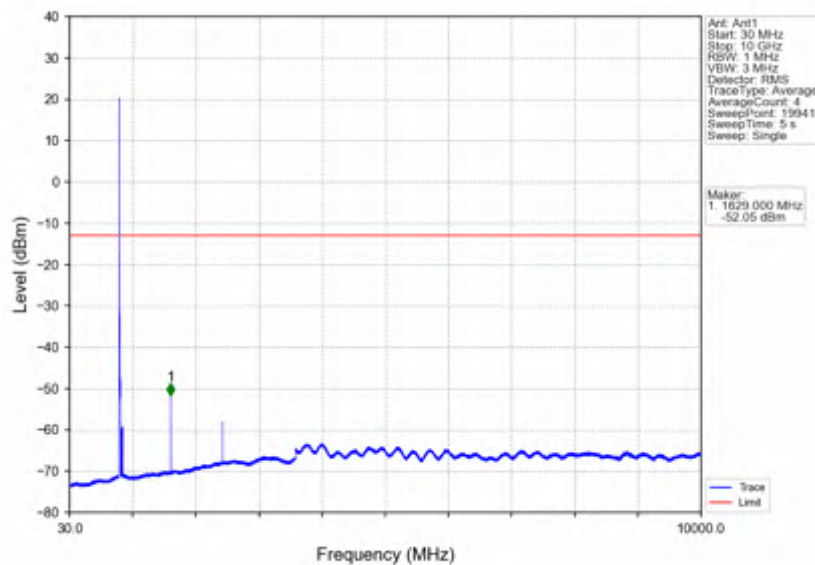
Band26a_10MHz_64QAM_LCH_819MHz_RB_1_0_NTNV
