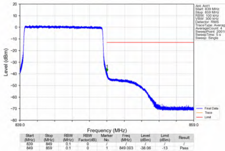
Band26b_10MHz_256QAM_HCH_844MHz_RB_50_0_NTNV
