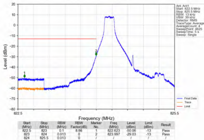
Band26b_1.4MHz_256QAM_LCH_824.7MHz_RB_1_0_NTNV
