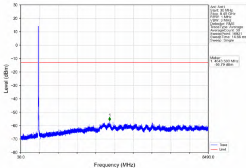
Band26c_15MHz_64QAM_LCH_831.5MHz_RB_1_0_NTNV
