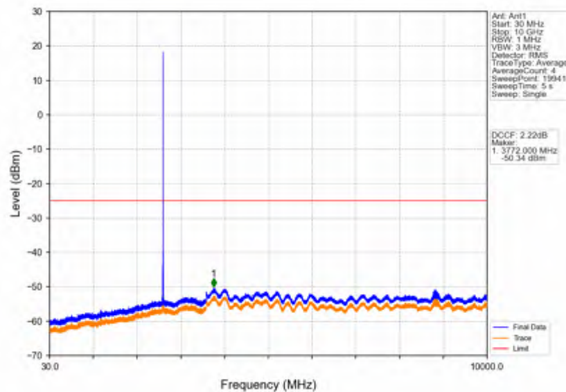
Band38 5MHz 256QAM HCH 2617.5MHz RB 1 0 NTNV
