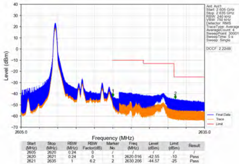
Band38_10MHz_16QAM_HCH_2615MHz_RB_1_49_NTNV
