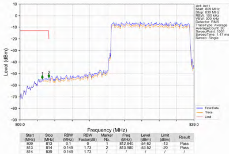
Band26c_15MHz_256QAM_LCH_831.5MHz_RB_75_0_NTNV
