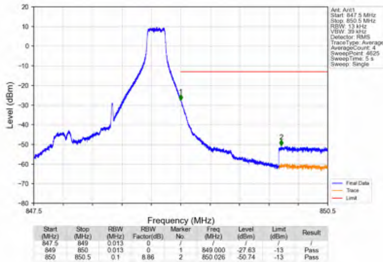
Band26b_1.4MHz_256QAM_HCH_848.3MHz_RB_1_5_NTNV
