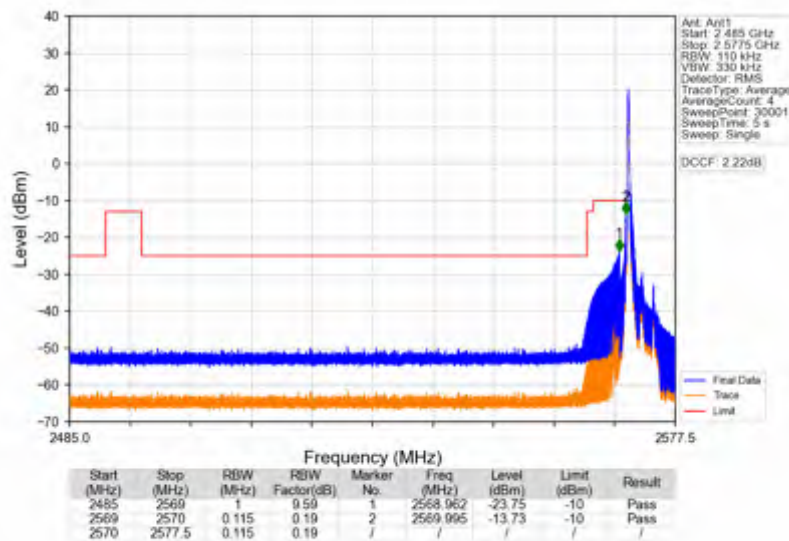
Band38_5MHz_256QAM_LCH_2572.5MHz_RB_1_0_NTNV
