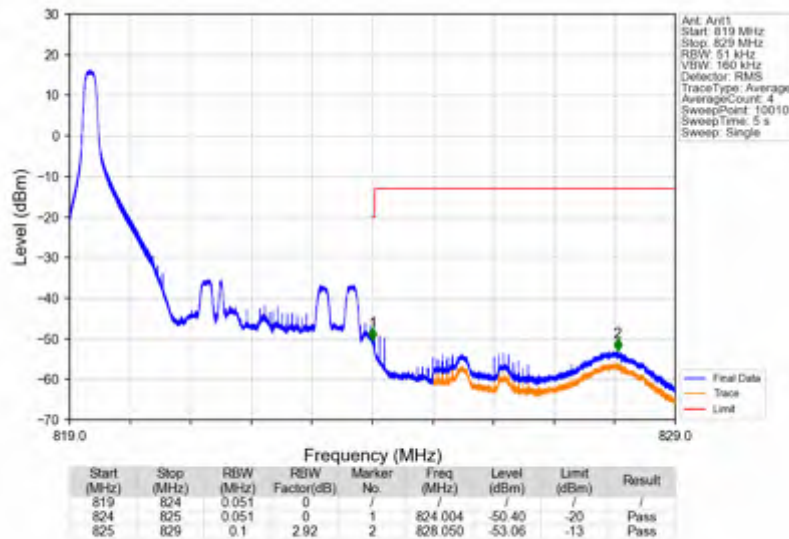
Band26a_5MHz_QPSK_HCH_821.5MHz_RB_1_24_NTNV
