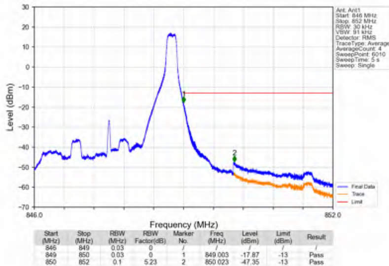
Band26b_3MHz_16QAM_HCH_847.5MHz_RB_1_14_NTNV
