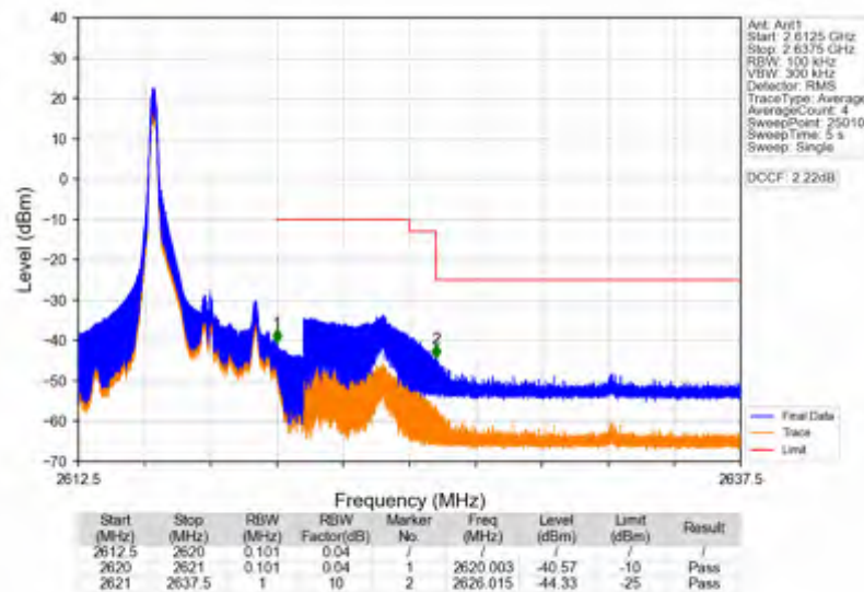
Band38_5MHz_64QAM_HCH_2617.5MHz_RB_1_24_NTNV
