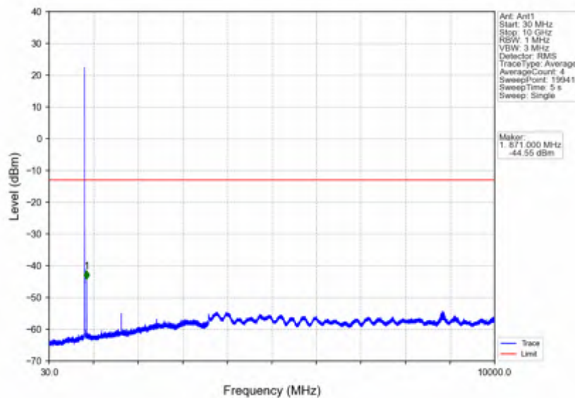
Band26b_5MHz_16QAM_LCH_826.5MHz_RB_25_0_NTNV
