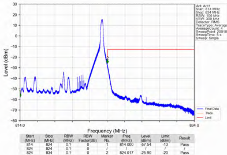
Band26a_10MHz_256QAM_HCH_819MHz_RB_1_49_NTNV
