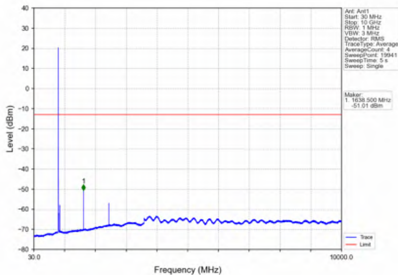
Band26a_5MHz_64QAM_HCH_821.5MHz_RB_1_24_NTNV
