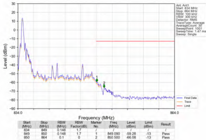
Band26c_15MHz_16QAM_HCH_841.5MHz_RB_75_0_NTNV
