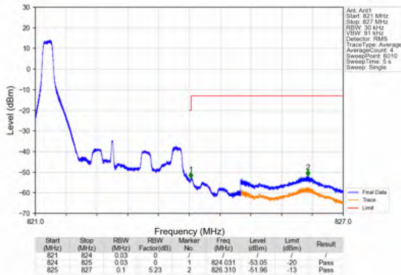
Band26a_3MHz_QPSK_HCH_822.5MHz_RB_15_0_NTNV
