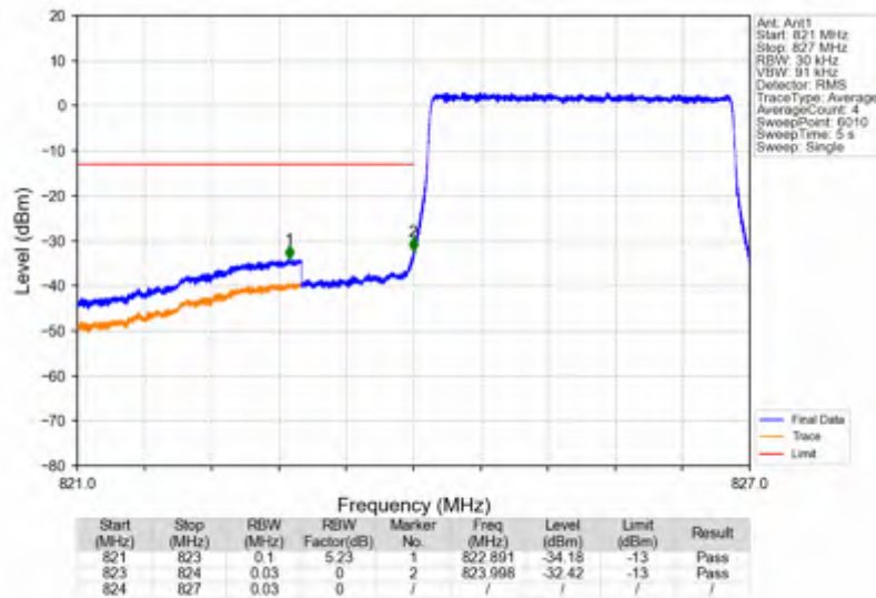
Band26b 3MHz 64QAM LCH 825.5MHz RB 15 0 NTNV
