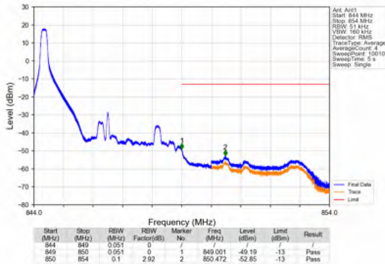
Band26b_5MHz_64QAM_HCH_846.5MHz_RB_25_0_NTNV
