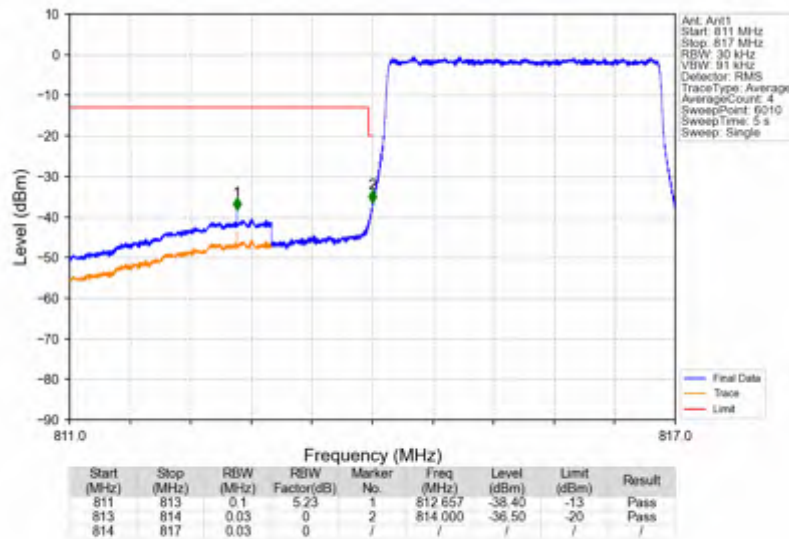
Band26a_3MHz_256QAM_LCH_815.5MHz_RB_15_0_NTNV
