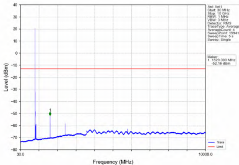
Band26a_10MHz_64QAM_MCH_819MHz_RB_1_0_NTNV
