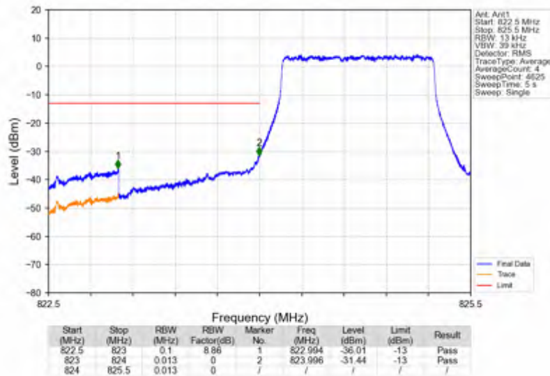
Band26b_1.4MHz_16QAM_LCH_824.7MHz_RB_6_0_NTNV
