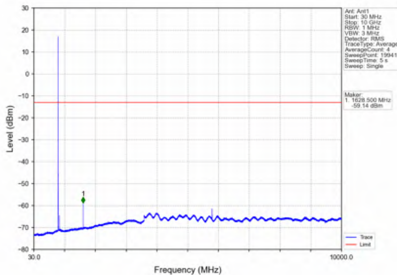
Band26a_3MHz_256QAM_LCH_815.5MHz_RB_15_0_NTNV
