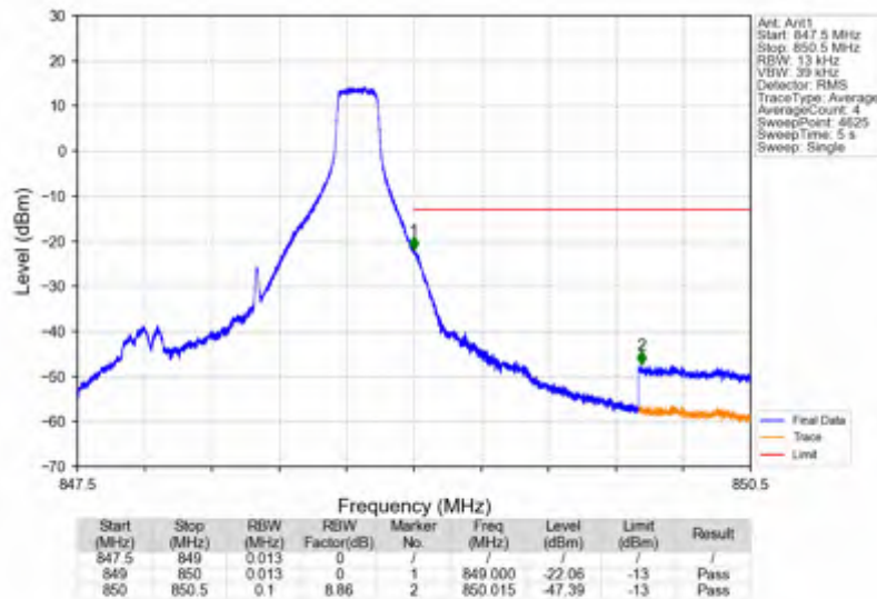
Band26b 1.4MHz QPSK HCH 848.3MHz RB_1_5 NTN
