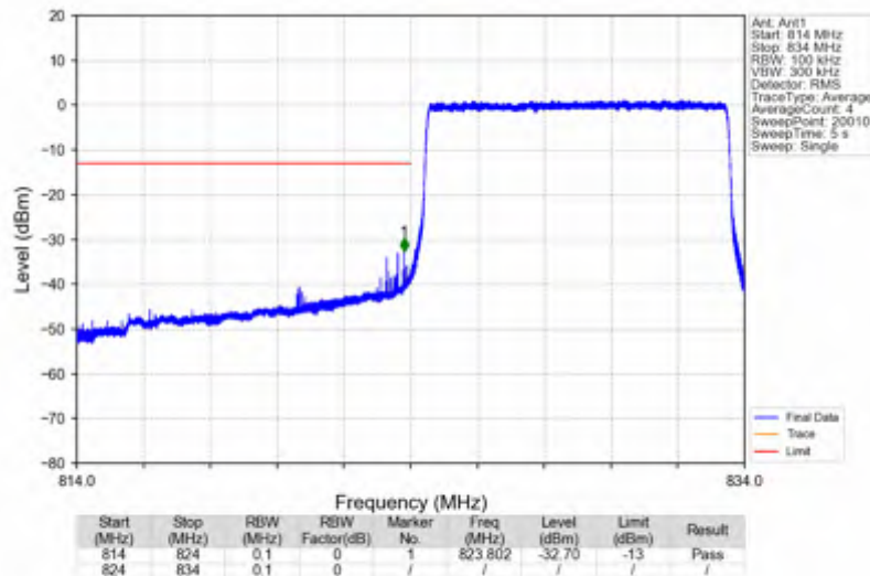
Band26b_10MHz_256QAM_LCH_829MHz_RB_50_0_NTNV
