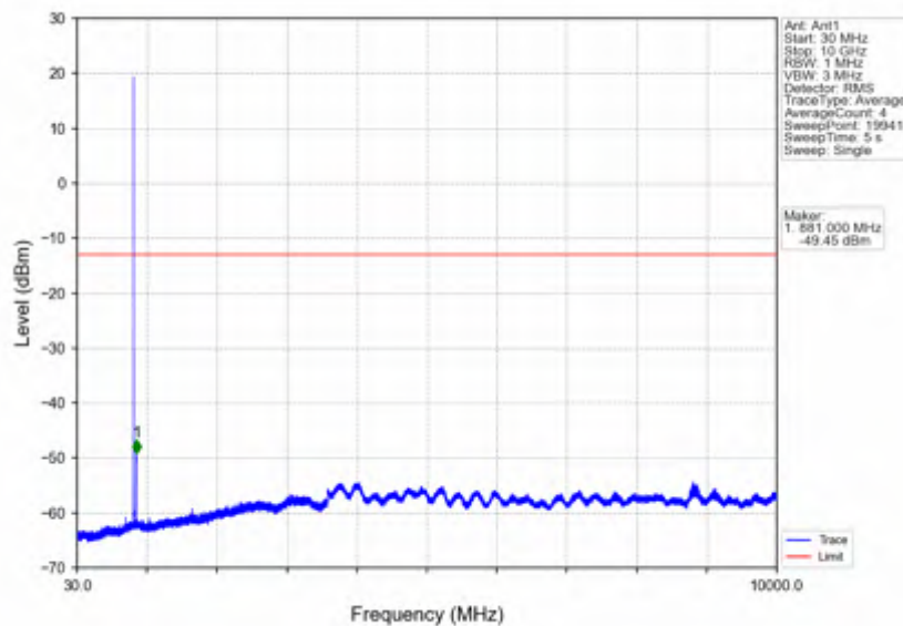
Band26b_1.4MHz_256QAM_HCH_848.3MHz_RB_1_0_NTNV
