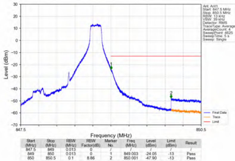
Band26b_1.4MHz_16QAM_HCH_848.3MHz_RB_1_5_NTNV
