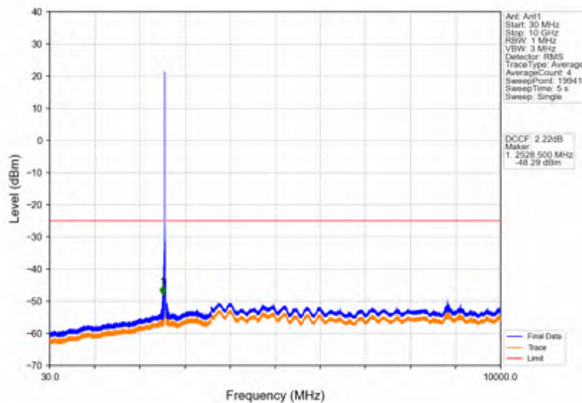
Band38_15MHz_16QAM_LCH_2577.5MHz_RB_1_0_NTNV
