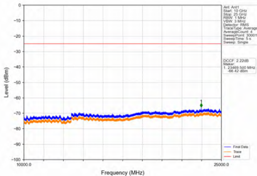
Band38_10MHz_16QAM_LCH_2575MHz_RB_1_0_NTNV
