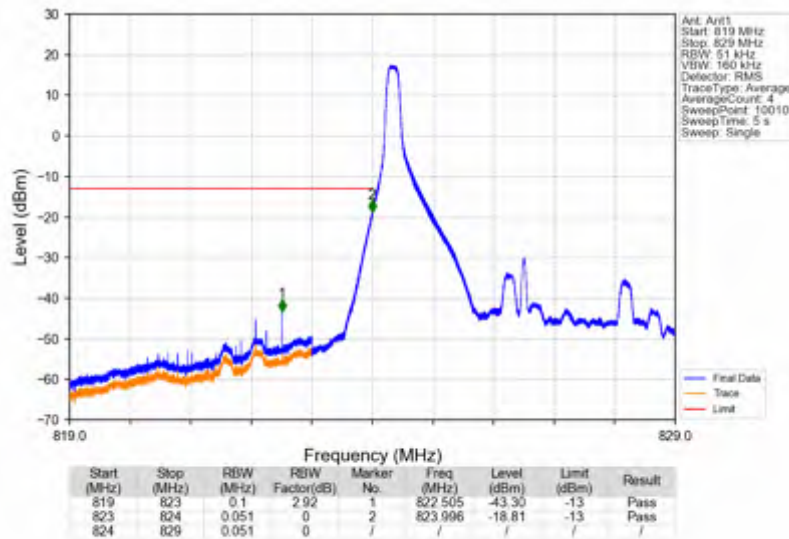
Band26b 5MHz 64QAM LCH 826.5MHz RB 1 0 NTNV
