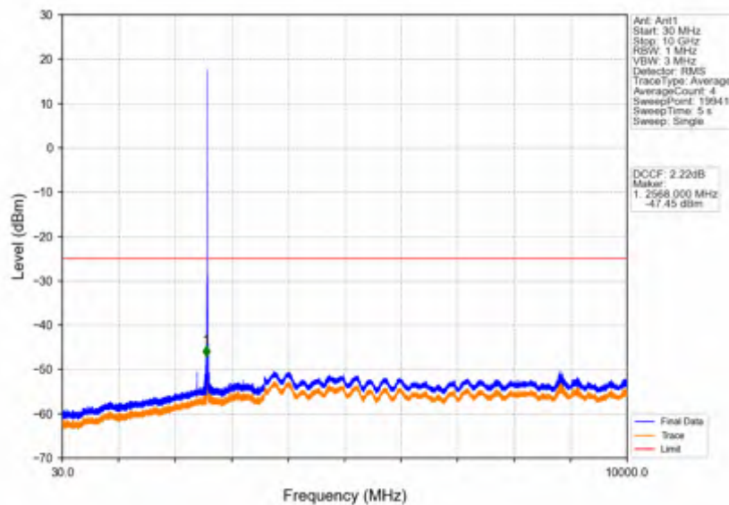
Band38_10MHz_256QAM_MCH_2595MHz_RB_1_0_NTNV
