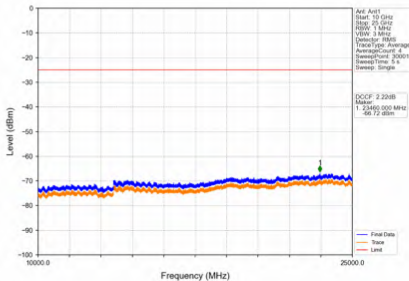
Band38_5MHz_16QAM_MCH_2595MHz_RB_1_0_NTNV
