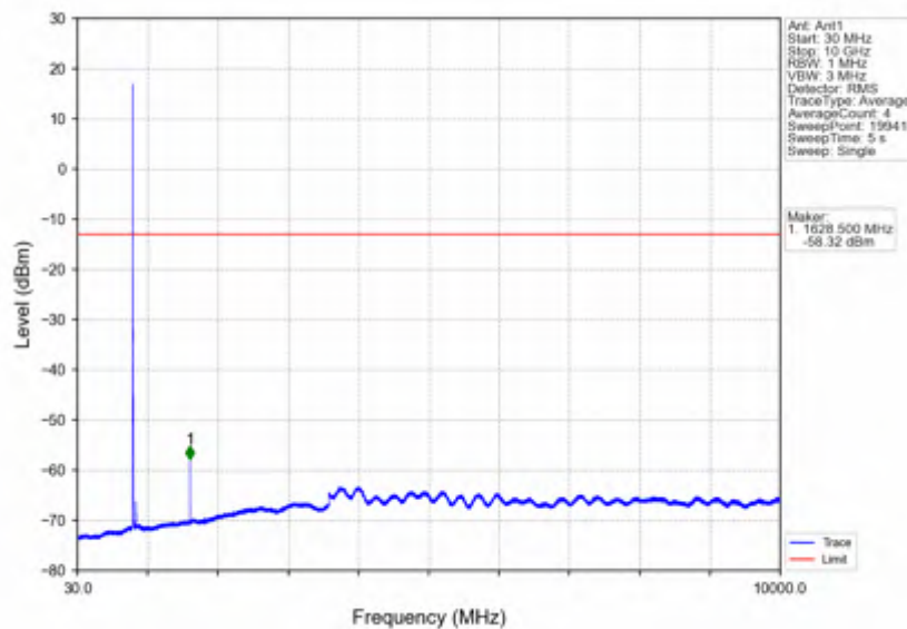
Band26a_5MHz_256QAM_LCH_816.5MHz_RB_25_0_NTNV
