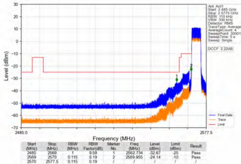
Band38_5MHz_64QAM_LCH_2572.5MHz_RB_1_0_NTNV
