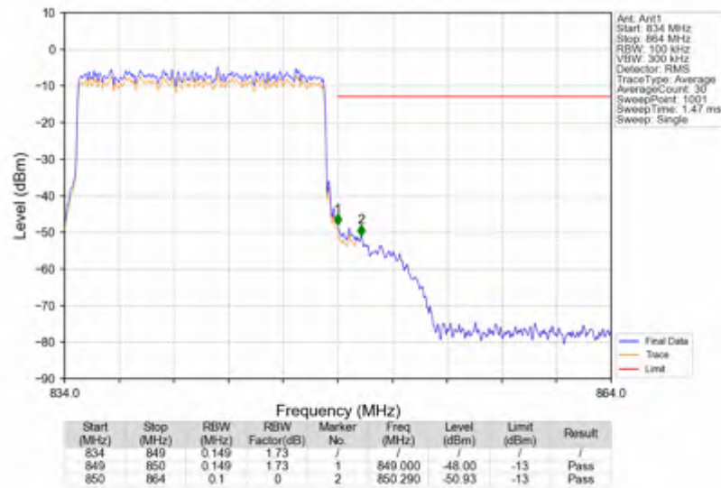
Band26c_15MHz_256QAM_HCH_841.5MHz_RB_75_0_NTNV
