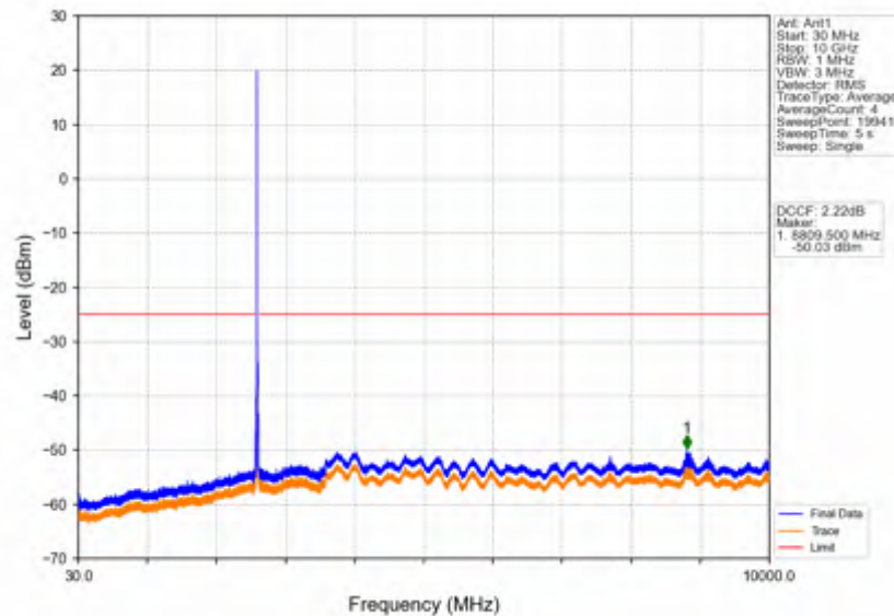
Band38_15MHz_16QAM_HCH_2612.5MHz_RB_1_0_NTNV
