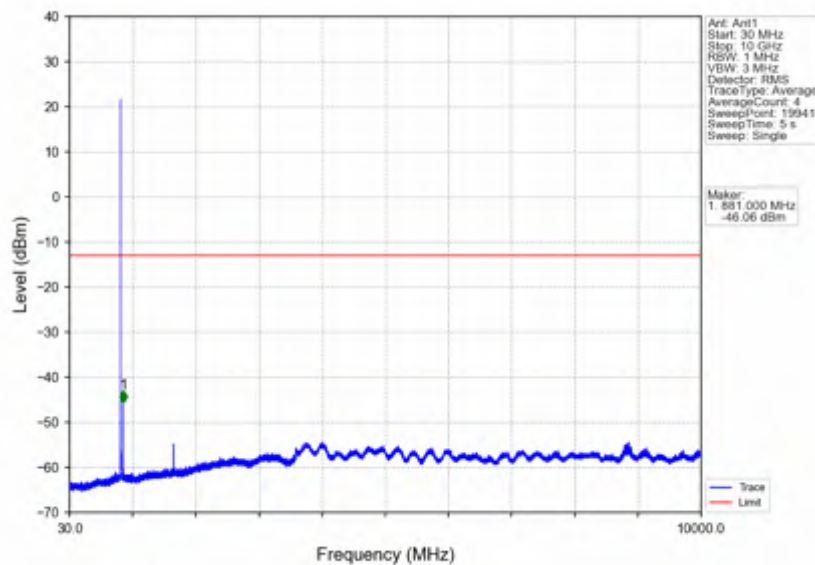
Band26b_3MHz_QPSK_MCH_836.5MHz_RB_1_0_NTNV
