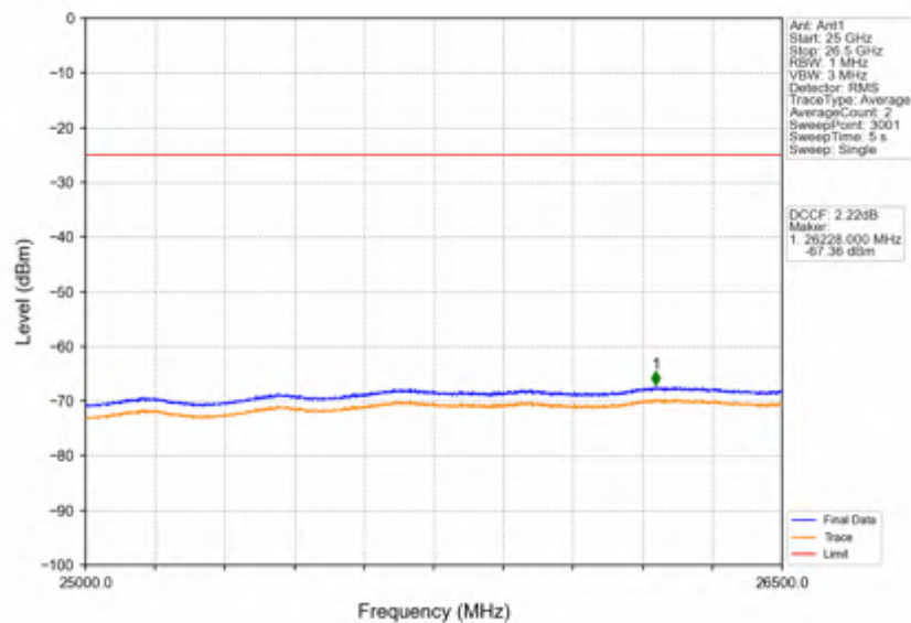
Band38_10MHz_16QAM_LCH_2575MHz_RB_50_0_NTNV
