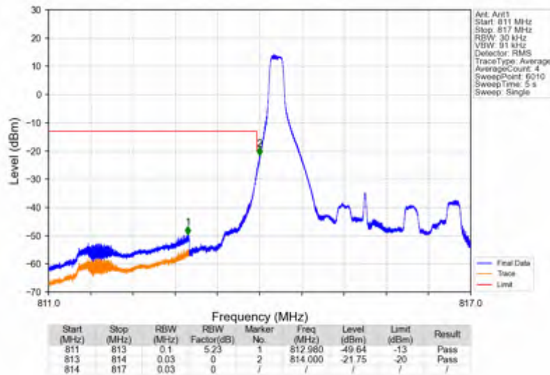
Band26a_3MHz_64QAM_LCH_815.5MHz_RB_1_0_NTNV
