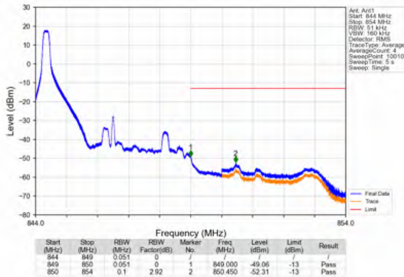
Band26b_5MHz_QPSK_HCH_846.5MHz_RB_25_0_NTNV
