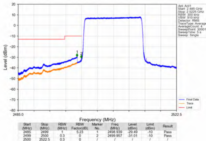
Band7_15MHz_16QAM_LCH_2507.5MHz_RB_75_0_NTNV
