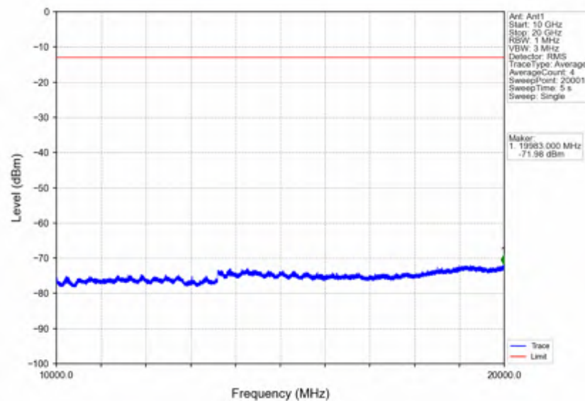
Band25_15MHz_256QAM_LCH_1857.5MHz_RB_75_0_NTNV
