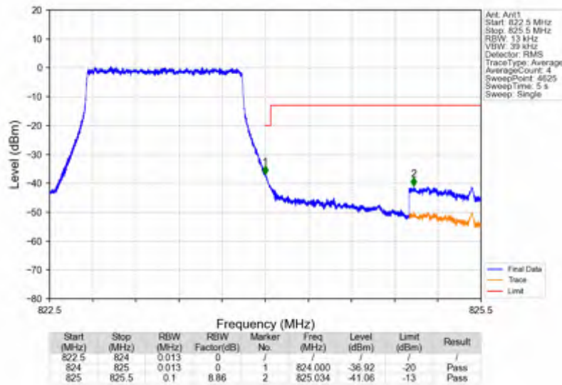
Band26a_1.4MHz_256QAM_HCH_823.3MHz_RB_6_0_NTNV
