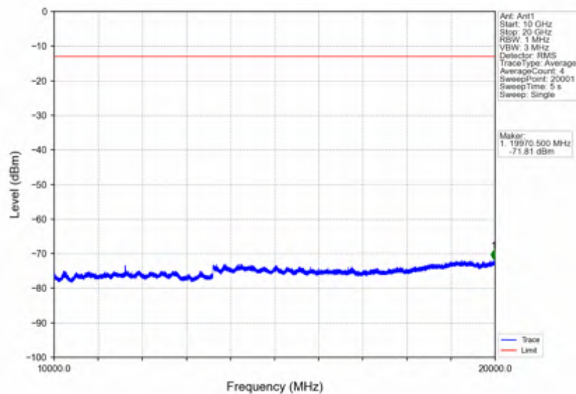
Band25 10MHz 16QAM LCH 1855MHz RB 50 0 NTNV
