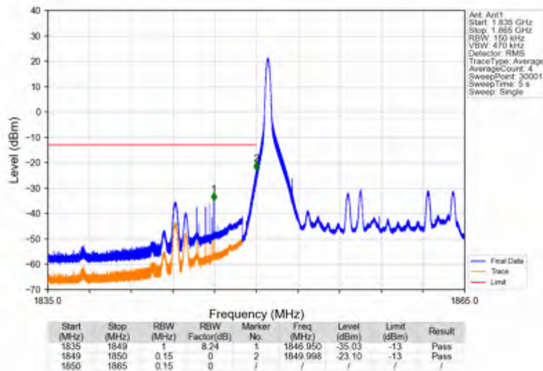
Band25_15MHz_QPSK_LCH_1857.5MHz_RB_1_0_NTNV
