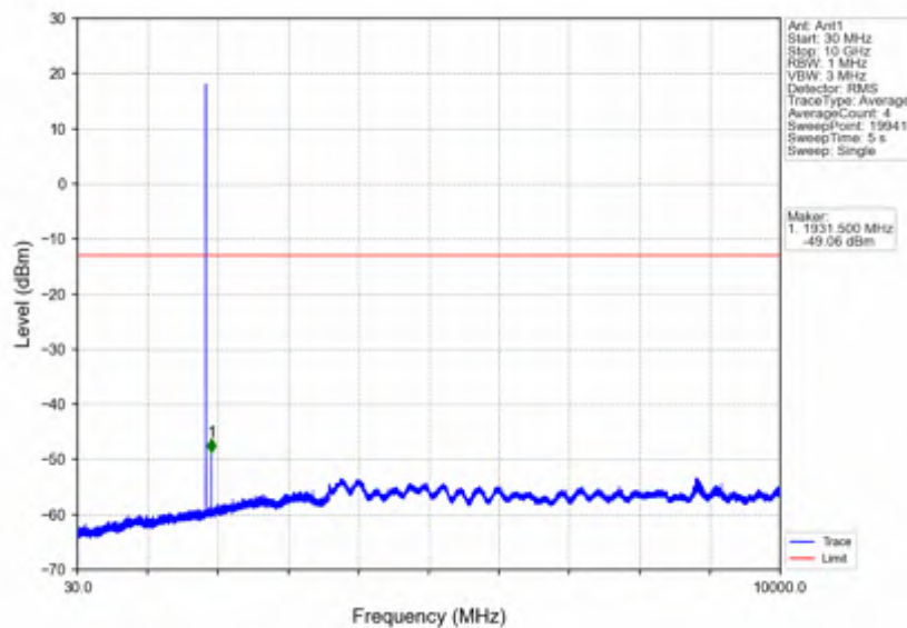
Band25_3MHz_256QAM_LCH_1851.5MHz_RB_1_0_NTNV
