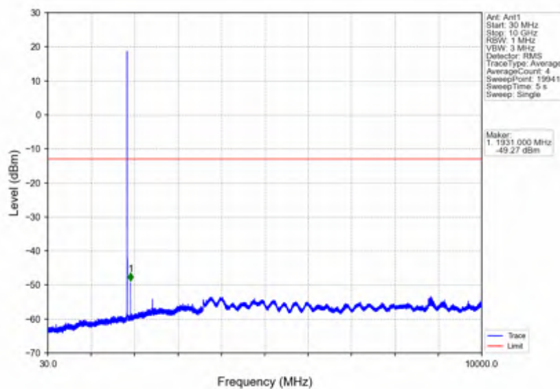
Band25 5MHz 256QAM LCH 1852.5MHz RB 1 0 NTNV
