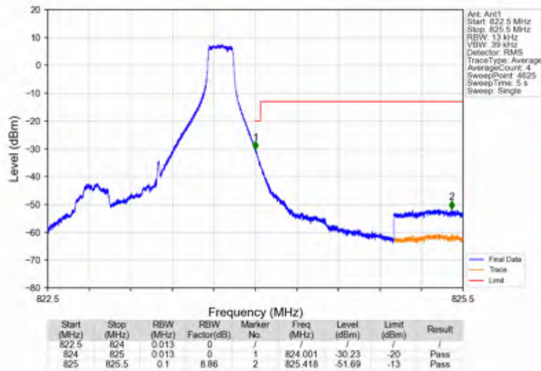
Band26a_1.4MHz_256QAM_HCH_823.3MHz_RB_1_5_NTNV
