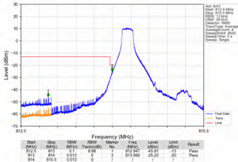
Band26a_1.4MHz_64QAM_LCH_814.7MHz_RB_6_0_NTNV
