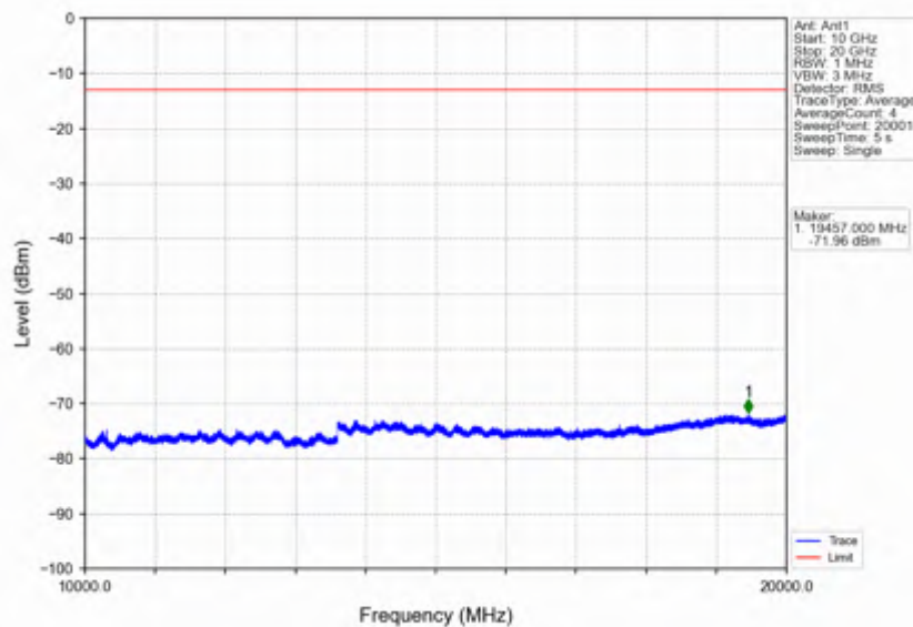
Band25_20MHz_64QAM_HCH_1905MHz_RB_1_0_NTV
