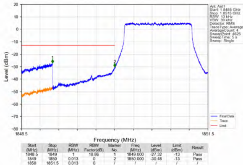
Band25_1.4MHz_QPSK_LCH_1850.7MHz_RB_6_0_NTNV
