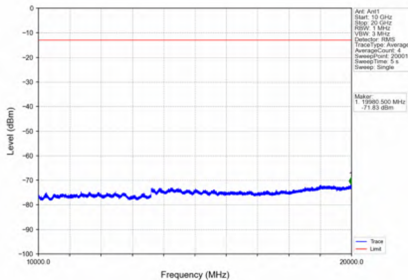
Band25 1.4MHz 16QAM LCH 1850.7MHz RB 6 0 NTN
