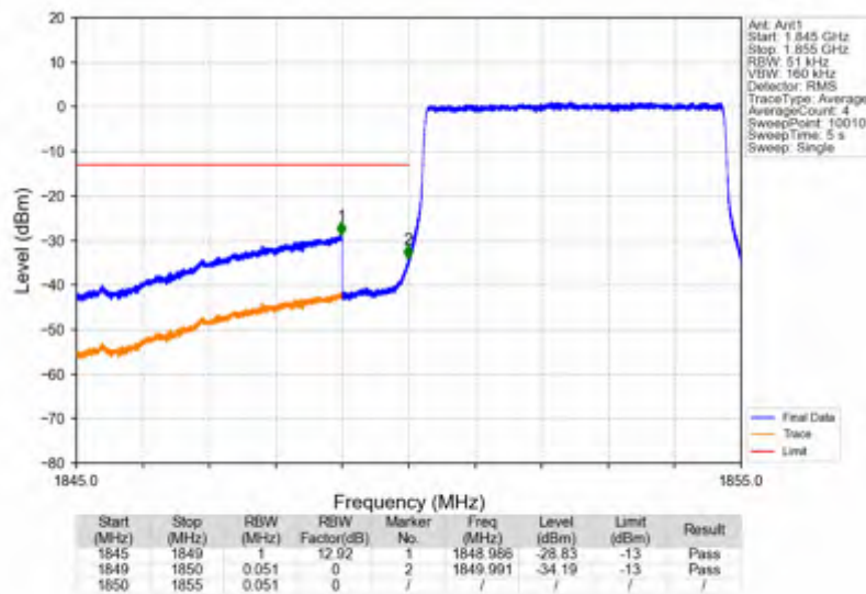
Band25_5MHz_256QAM_LCH_1852.5MHz_RB_25_0_NTNV
