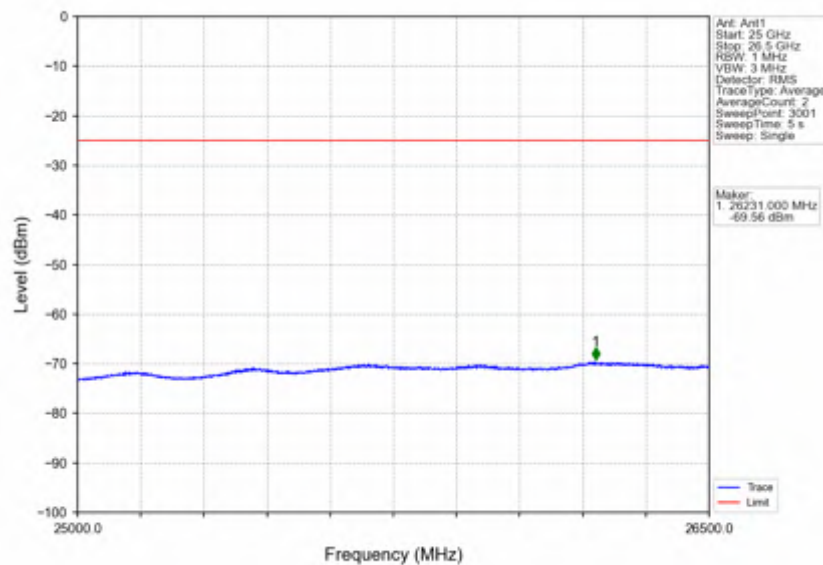
Band7_15MHz_16QAM_LCH_2507.5MHz_RB_75_0_NTNV
