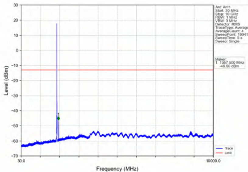
Band25_15MHz_256QAM_MCH_1882.5MHz_RB_1_0_NTNV
