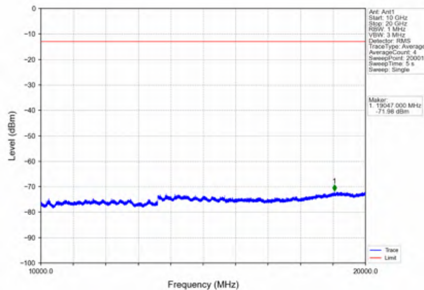
Band25 1.4MHz 64QAM LCH 1850.7MHz RB 6 0 NTNV
