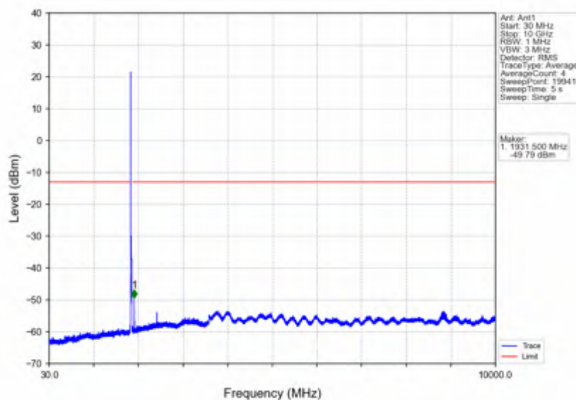
Band25_15MHz_QPSK_LCH_1857.5MHz_RB_1_0_NTNV
