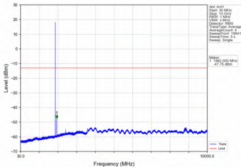
Band25_3MHz_256QAM_MCH_1882.5MHz_RB_1_0_NTNV
