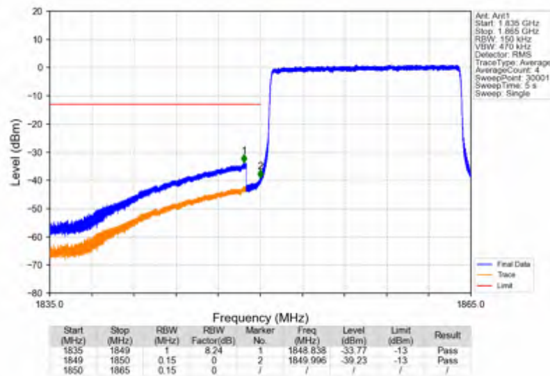
Band25_15MHz_256QAM_LCH_1857.5MHz_RB_75_0_NTNV
