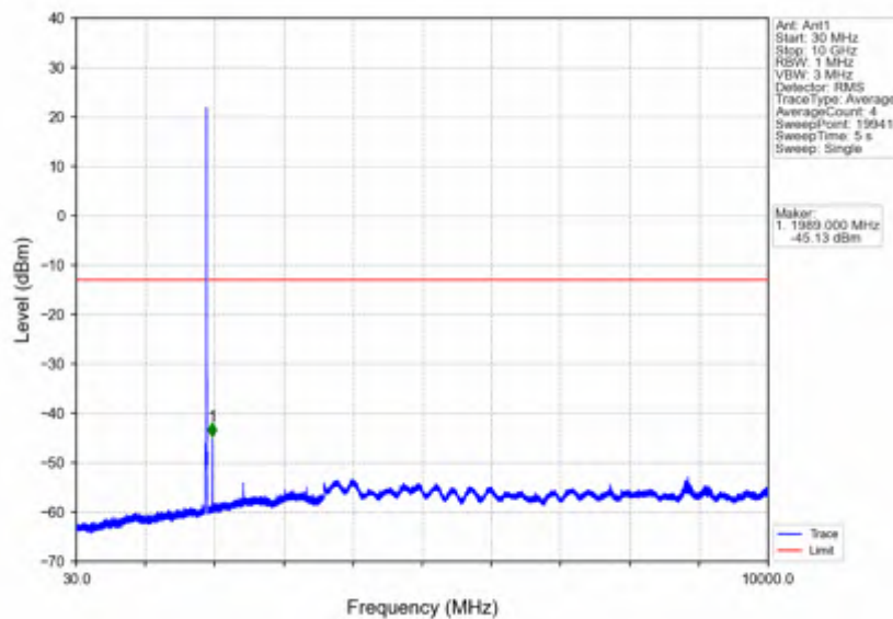
Band25_10MHz_16QAM_HCH_1910MHz_RB_1_0_NTV
