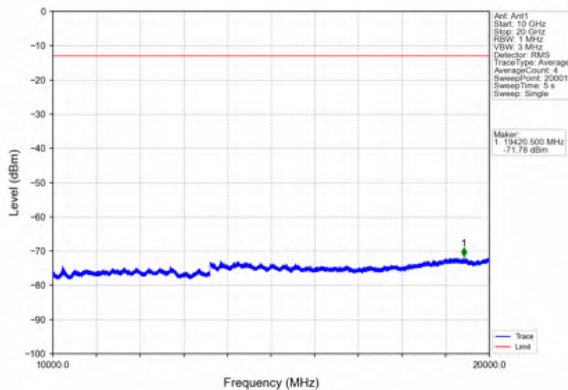
Band25_5MHz_256QAM_MCH_1882.5MHz_RB_1_0_NTNV
