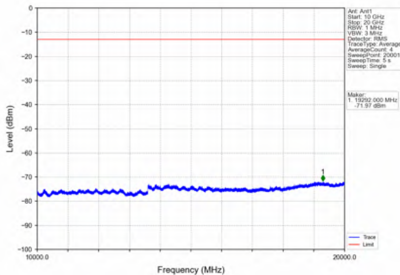
Band25_15MHz_256QAM_HCH_1907.5MHz_RB_1_0_NTNV
