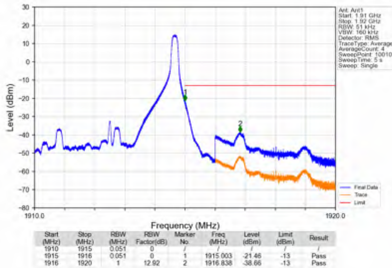
Band25_5MHz_256QAM_HCH_1912.5MHz_RB_1_24_NTNV
