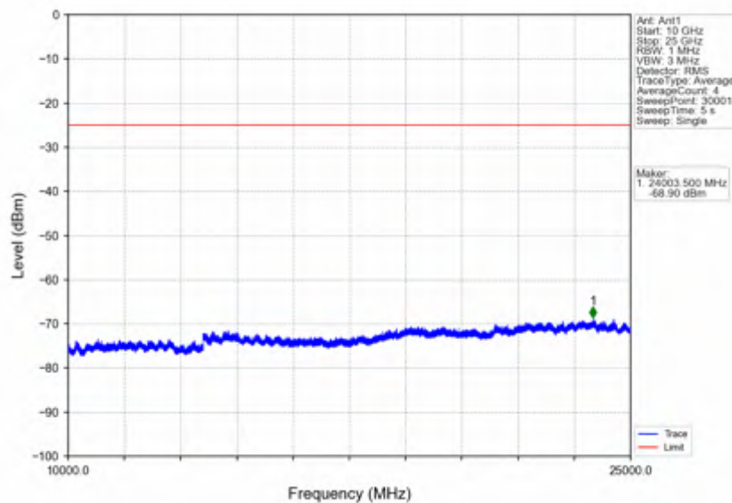
Band7_15MHz_256QAM_MCH_2535MHz_RB_1_0_NTNV
