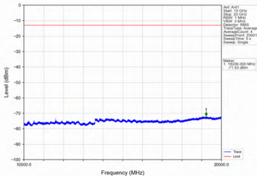
Band25_20MHz_256QAM_HCH_1905MHz_RB_1_0_NTNV
