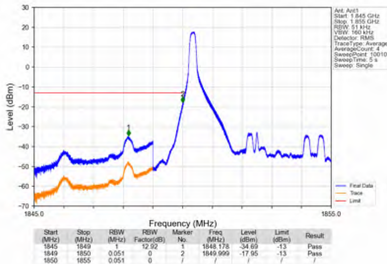
Band25_5MHz_QPSK_LCH_1852.5MHz_RB_1_0_NTNV
