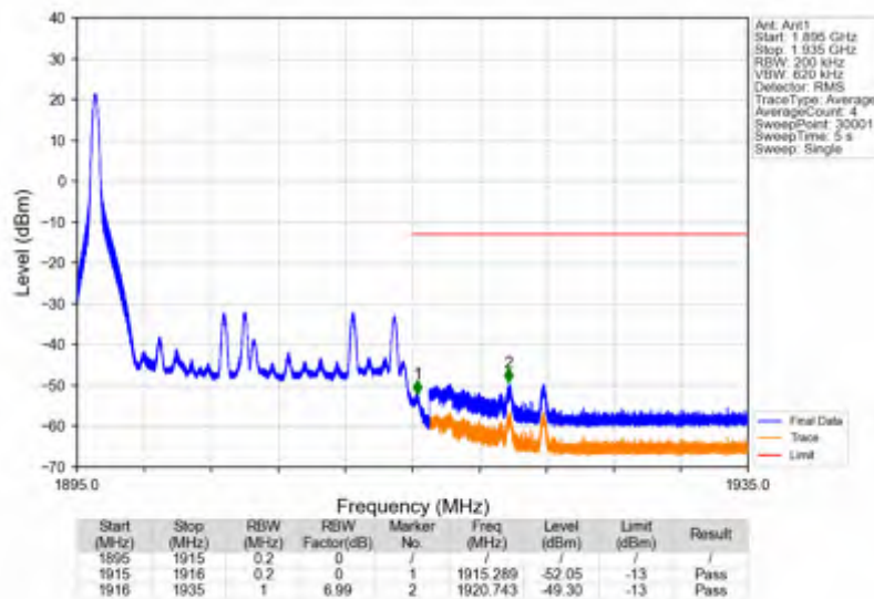
Band25_20MHz_16QAM_HCH_1905MHz_RB_100_0_NTNV
