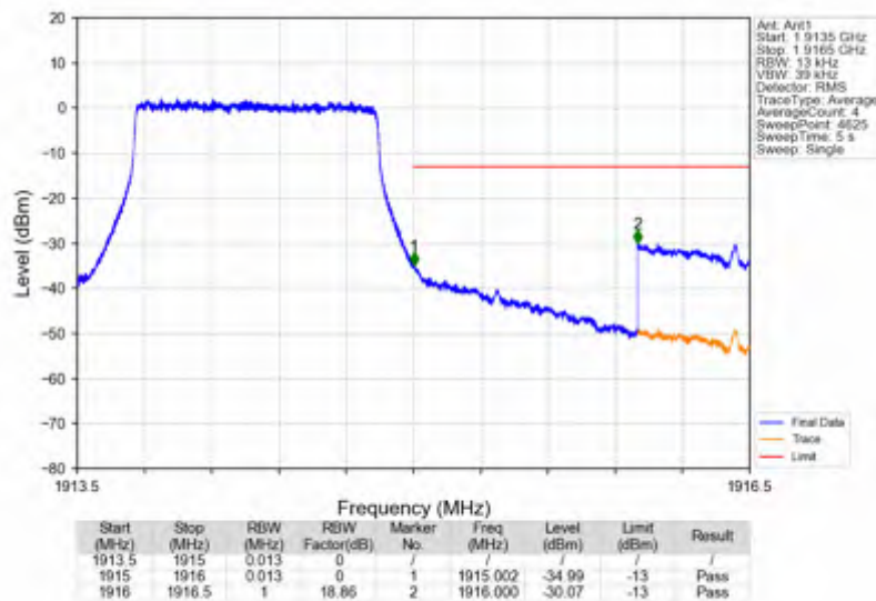
Band25_1.4MHz_256QAM_HCH_1914.3MHz_RB_6_0_NTNV
