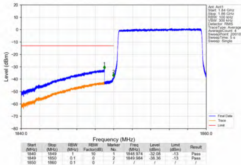
Band25_10MHz_256QAM_LCH_1855MHz_RB_50_0_NTNV
