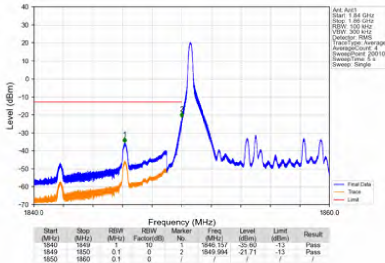
Band25_10MHz_16QAM_LCH_1855MHz_RB_1_0_NTV
