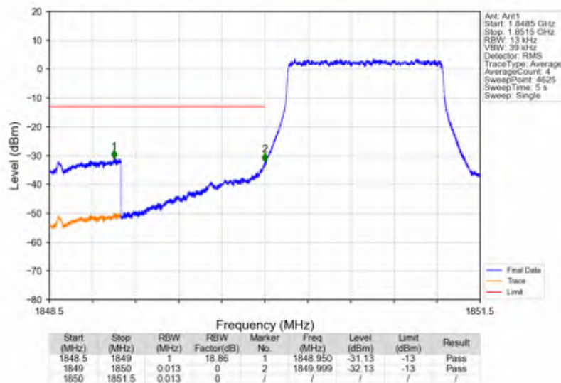
Band25 1.4MHz 64QAM LCH 1850.7MHz RB 6 0 NTNV
