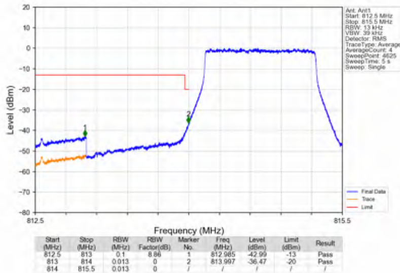
Band26a_1.4MHz_256QAM_LCH_814.7MHz_RB_6_0_NTNV
