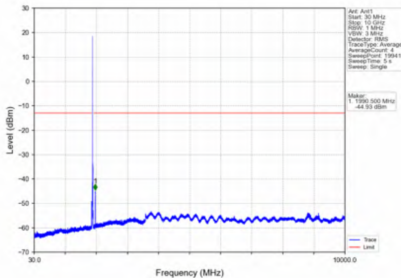
Band25_15MHz_256QAM_HCH_1907.5MHz_RB_1_0_NTNV
