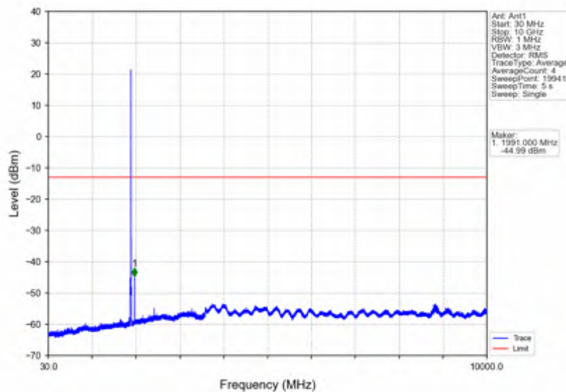
Band25_10MHz_64QAM_HCH_1910MHz_RB_1_0_NTNV
