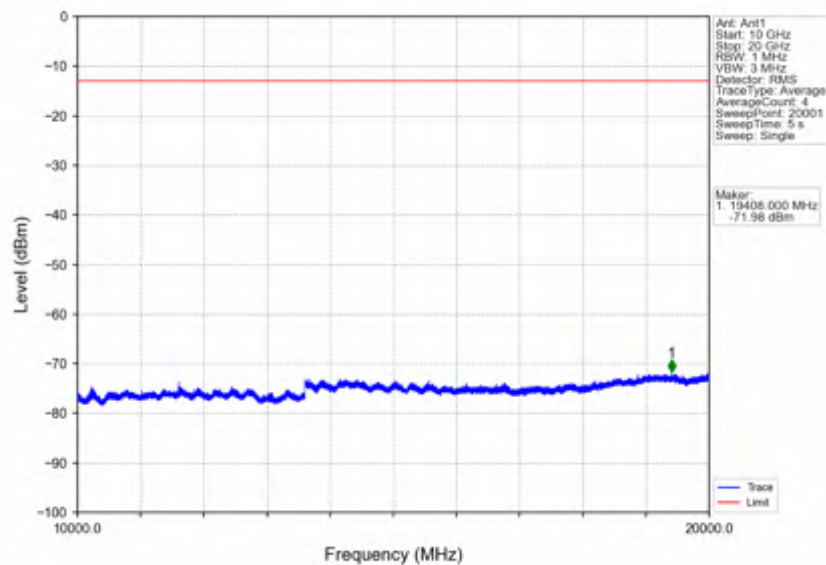
Band25_3MHz_64QAM_LCH_1851.5MHz_RB_15_0_NTNV
