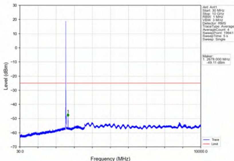
Band7_15MHz_256QAM_HCH_2562.5MHz_RB_1_0_NTNV
