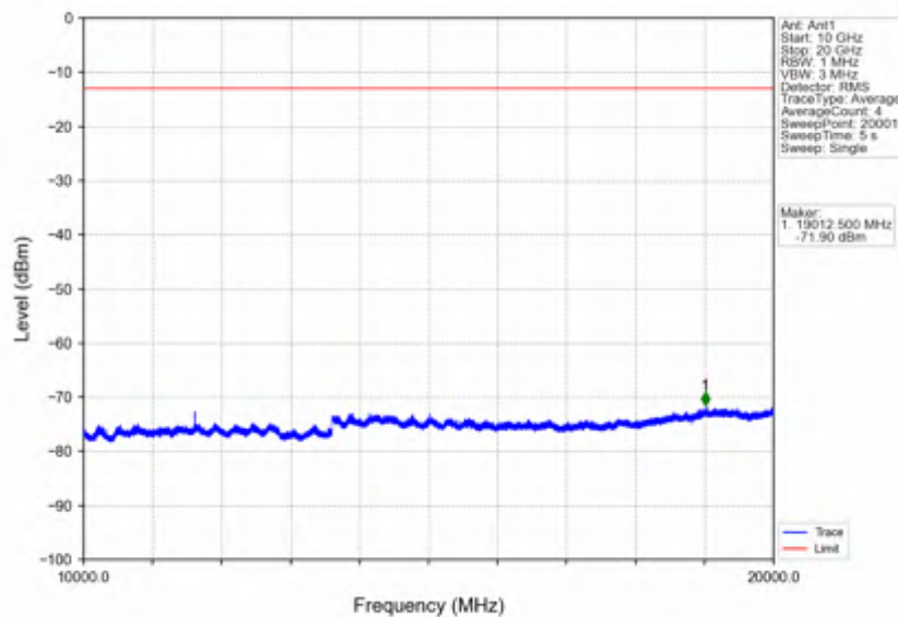
Band25_5MHz_256QAM_HCH_1912.5MHz_RB_1_0_NTNV
