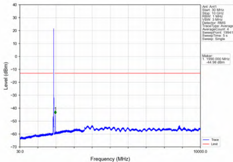
Band25_20MHz_64QAM_HCH_1905MHz_RB_1_0_NTV
