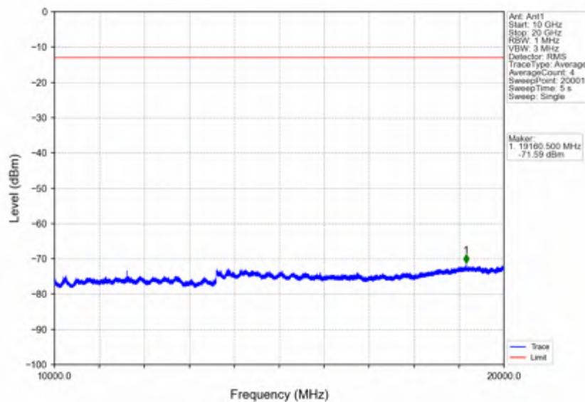
Band25_10MHz_256QAM_HCH_1910MHz_RB_1_0_NTNV
