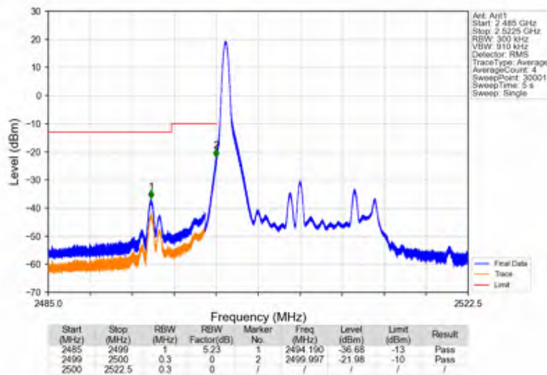
Band7_15MHz_256QAM_LCH_2507.5MHz_RB_75_0_NTNV
