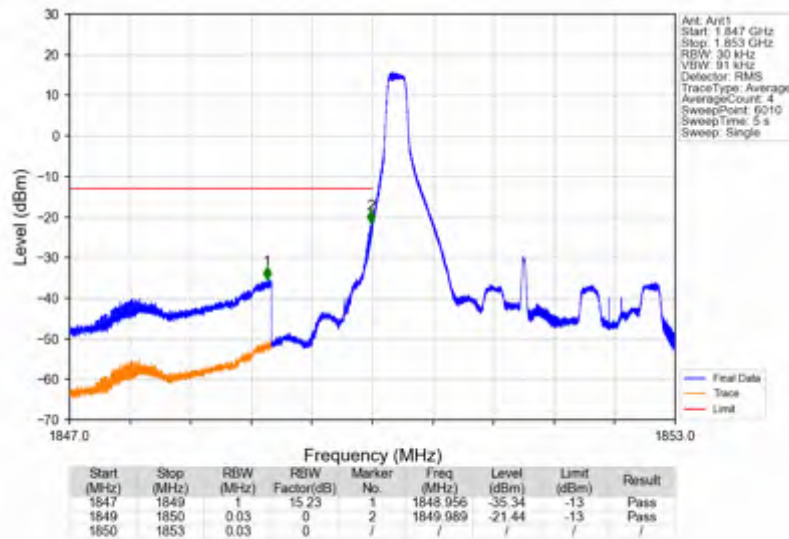
Band25 3MHz 64QAM LCH 1851.5MHz RB 1 0 NTNV
