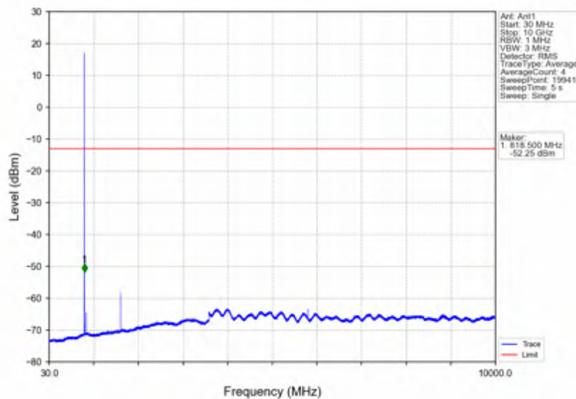
Band26a_1.4MHz_256QAM_LCH_814.7MHz_RB_6_0_NTNV
