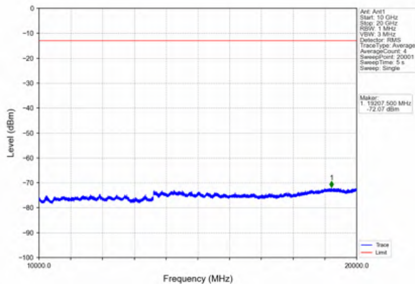
Band25_3MHz_256QAM_LCH_1851.5MHz_RB_15_0_NTNV
