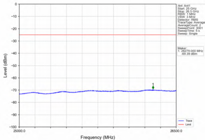
Band7_15MHz_256QAM_HCH_2562.5MHz_RB_1_0_NTNV
