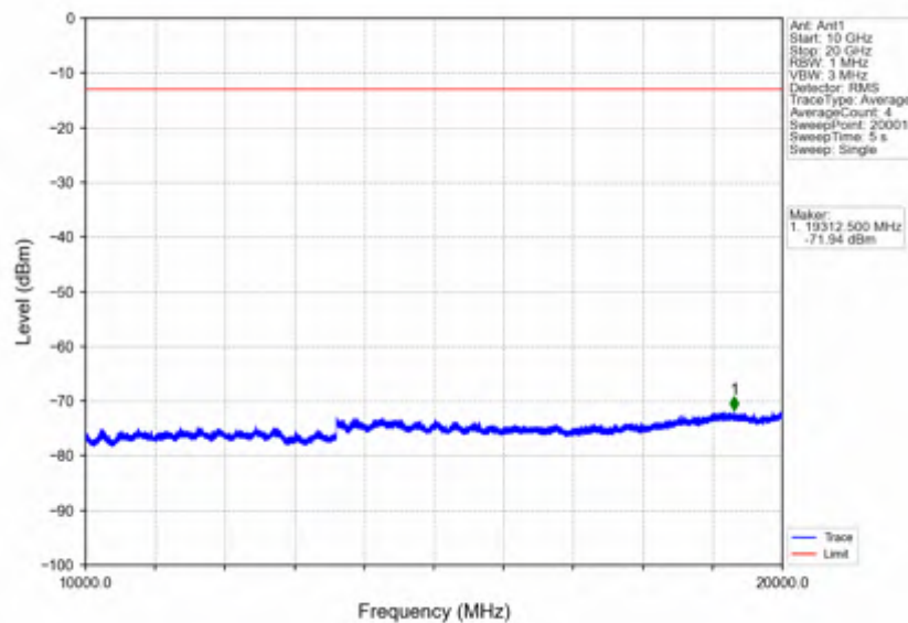
Band25 1.4MHz 64QAM HCH 1914.3MHz RB 1 0 NTNV
