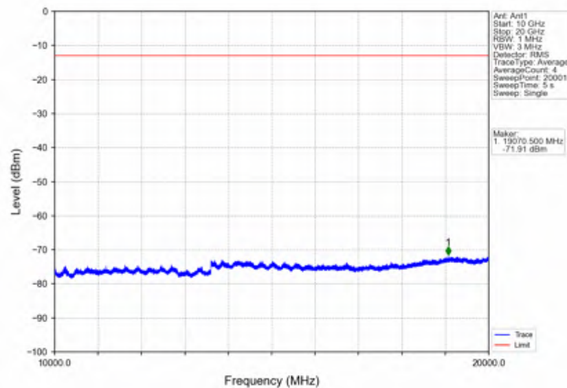
Band25_1.4MHz_256QAM_LCH_1850.7MHz_RB_6_0_NTNV
