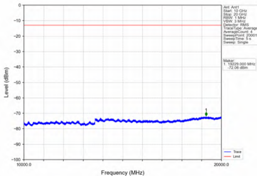
Band25_1.4MHz_256QAM_MCH_1882.5MHz_RB_1_0_NTNV
