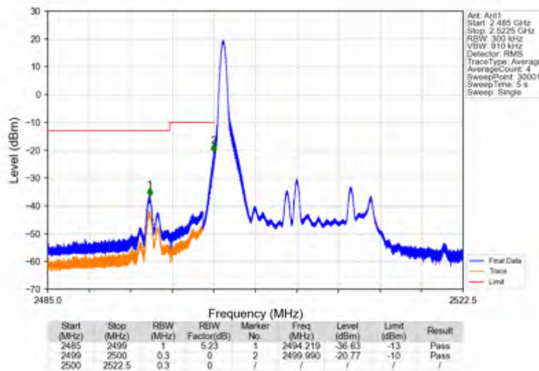
Band7_15MHz_256QAM_LCH_2507.5MHz_RB_1_0_NTNV
