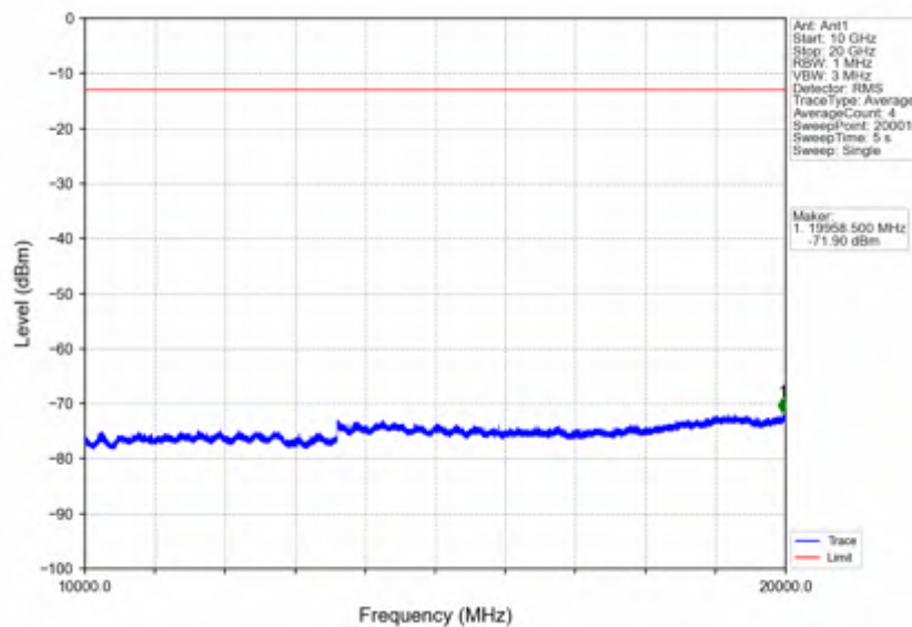
Band25_20MHz_256QAM_MCH_1882.5MHz_RB_1_0_NTNV
