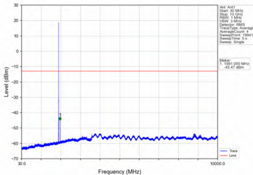
Band25_5MHz_256QAM_HCH_1912.5MHz_RB_1_0_NTNV
