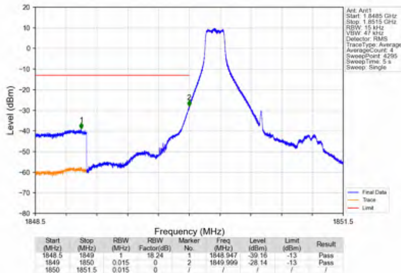
Band25 1.4MHz 256QAM LCH 1850.7MHz RB 1 0 NTNV
