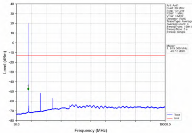
Band26a_1.4MHz_QPSK_HCH_823.3MHz_RB_1_5_NTNV
