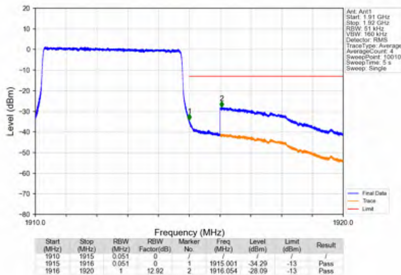
Band25_5MHz_256QAM_HCH_1912.5MHz_RB_25_0_NTNV
