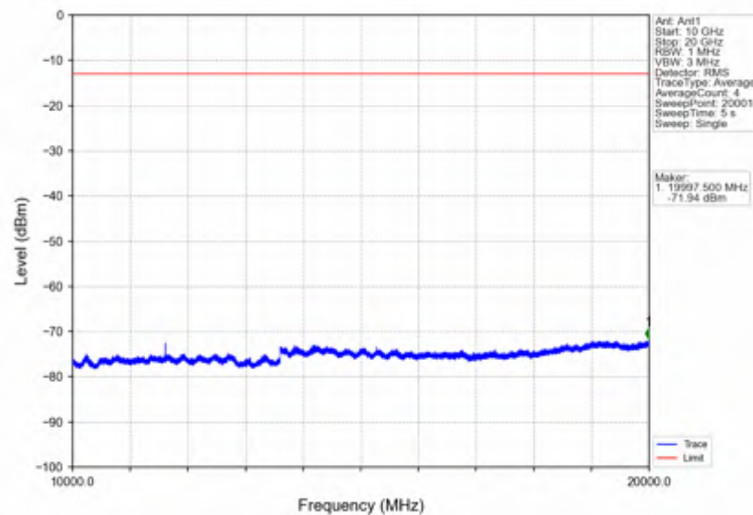
Band25_5MHz_256QAM_LCH_1852.5MHz_RB_25_0_NTNV
