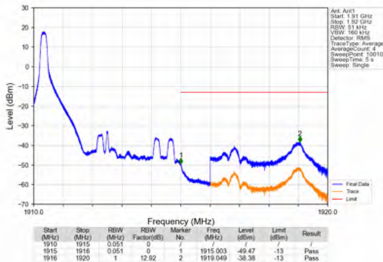
Band25 5MHz 16QAM HCH 1912.5MHz RB 25 0 NTV
