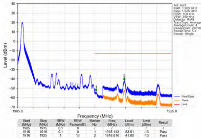
Band25_10MHz_16QAM_HCH_1910MHz_RB_50_0_NTNV
