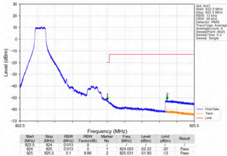
Band26a_1.4MHz_64QAM_HCH_823.3MHz_RB_6_0_NTNV
