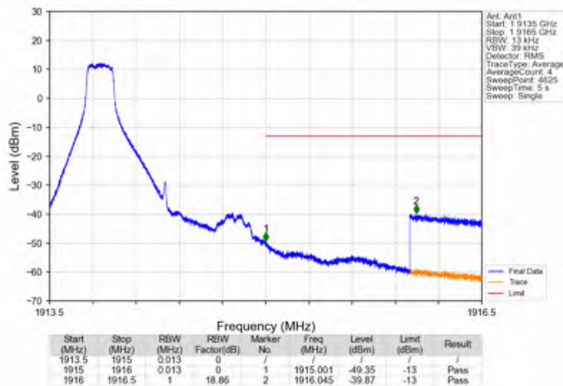
Band25_1.4MHz_64QAM_HCH_1914.3MHz_RB_6_0_NTNV
