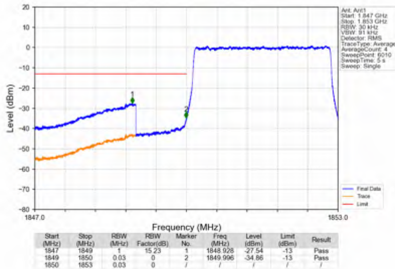
Band25_3MHz_256QAM_LCH_1851.5MHz_RB_15_0_NTNV
