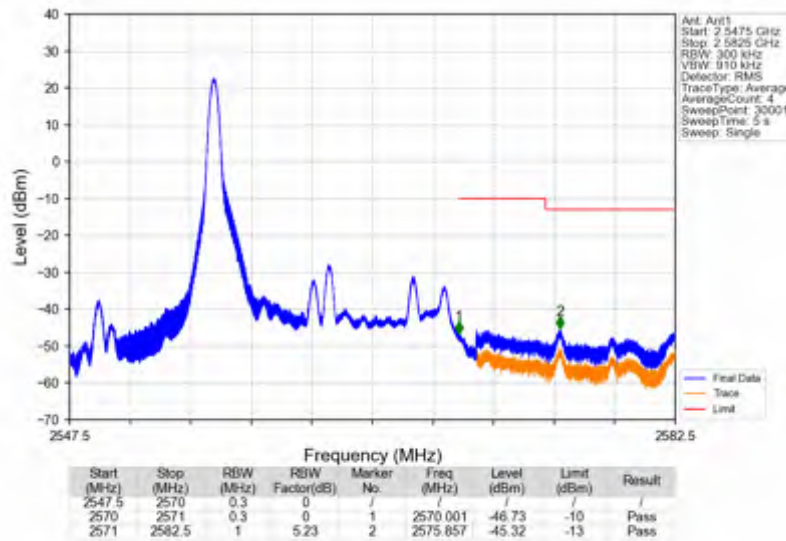
Band7_15MHz_64QAM_HCH_2562.5MHz_RB_75_0_NTNV
