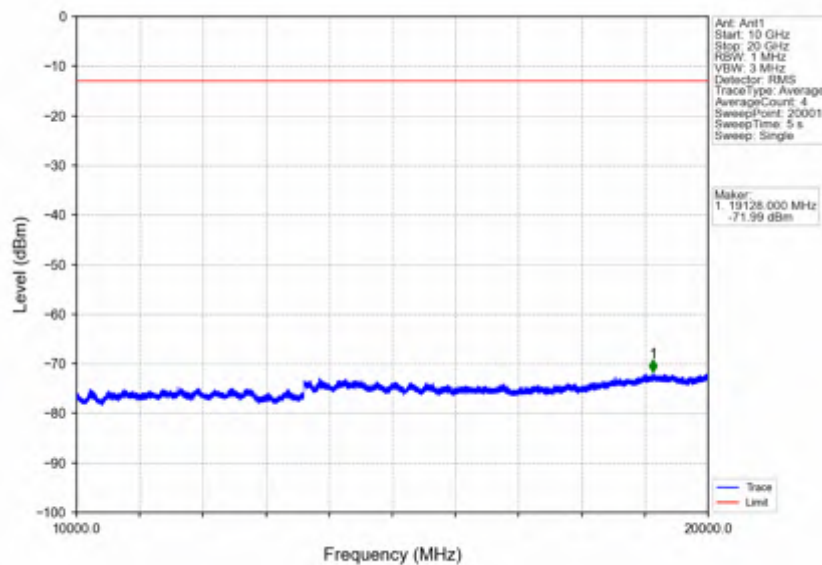
Band25_1.4MHz_256QAM_HCH_1914.3MHz_RB_1_0_NTNV
