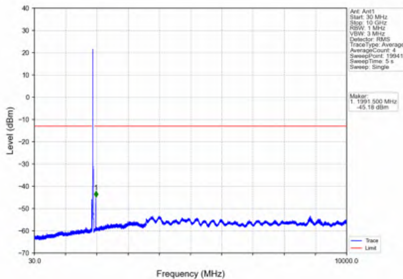
Band25_20MHz_16QAM_HCH_1905MHz_RB_1_0_NTV
