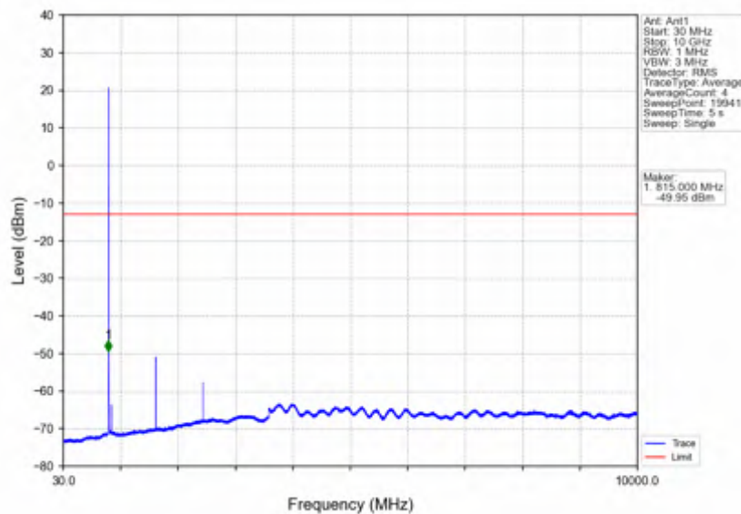
Band26a_1.4MHz_64QAM_MCH_819MHz_RB_1_0_NTNV
