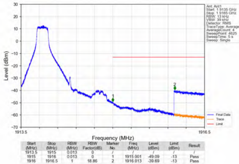
Band25_1.4MHz_16QAM_HCH_1914.3MHz_RB_6_0_NTNV
