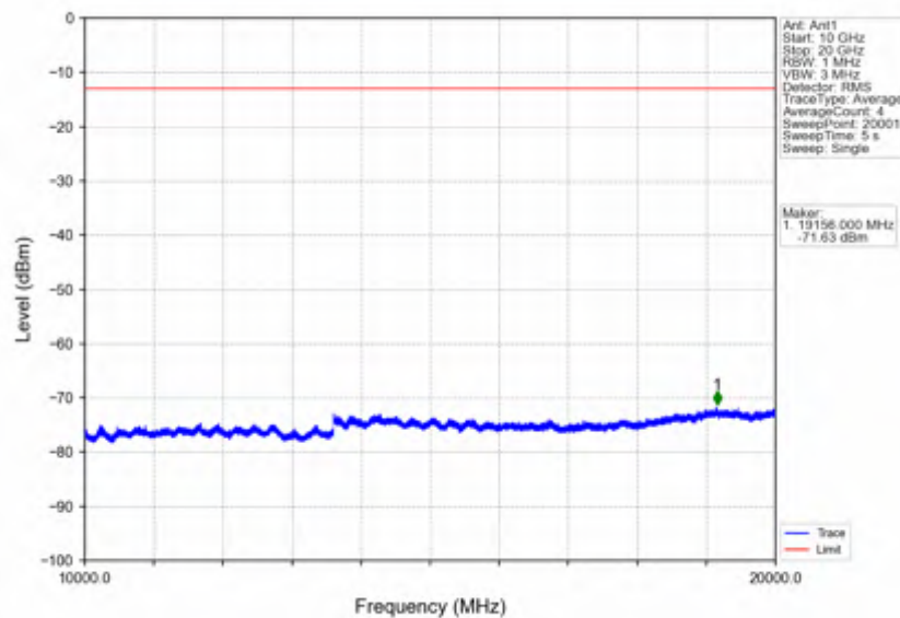
Band25_15MHz_QPSK_HCH_1907.5MHz_RB_1_0_NTNV
