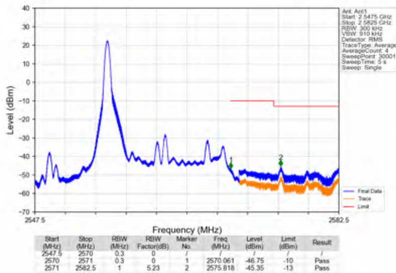
Band7_15MHz_16QAM_HCH_2562.5MHz_RB_75_0_NTNV
