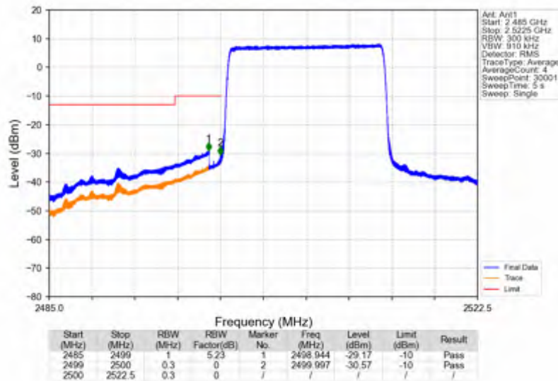
Band7_15MHz_64QAM_LCH_2507.5MHz_RB_1_0_NTNV
