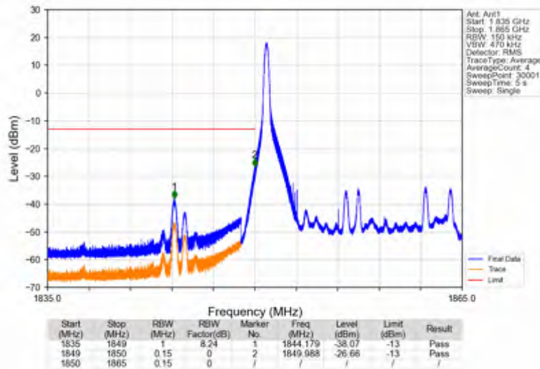
Band25 15MHz 256QAM LCH 1857.5MHz RB 1 0 NTNV
