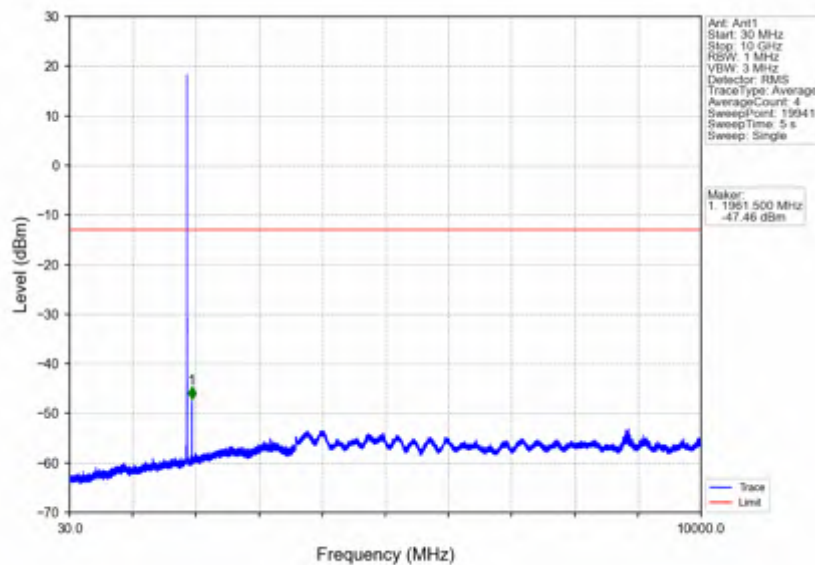
Band25_5MHz_256QAM_MCH_1882.5MHz_RB_1_0_NTNV
