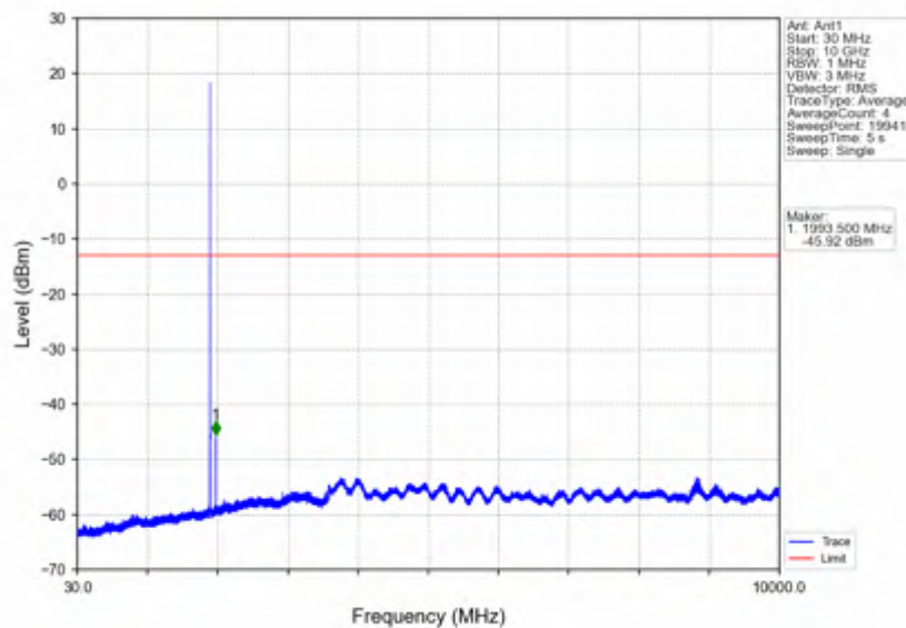
Band25_3MHz_256QAM_HCH_1913.5MHz_RB_1_0_NTNV
