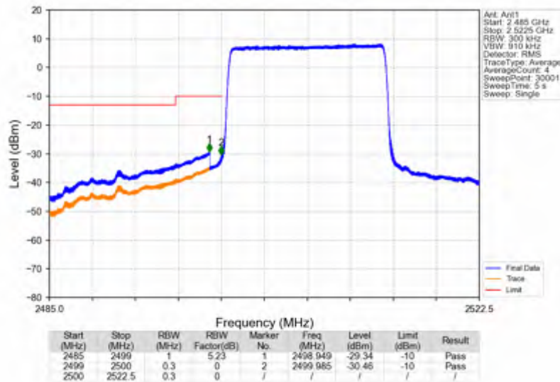
Band7_15MHz_64QAM_LCH_2507.5MHz_RB_75_0_NTNV
