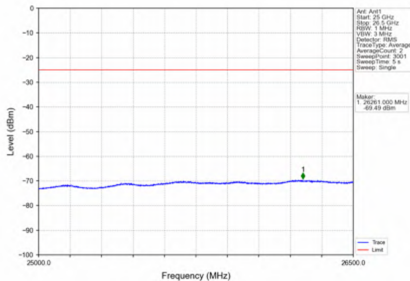
Band7_15MHz_256QAM_LCH_2507.5MHz_RB_75_0_NTNV
