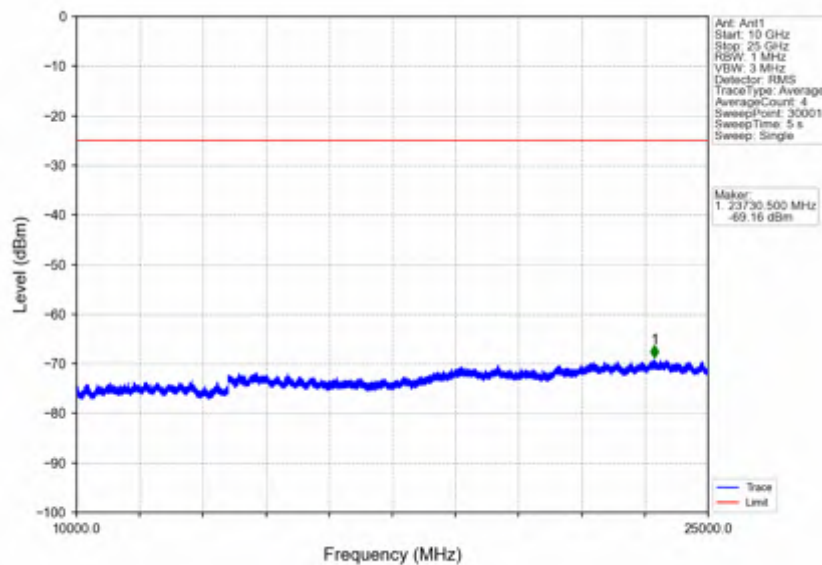
Band7_15MHz_256QAM_LCH_2507.5MHz_RB_1_0_NTNV
