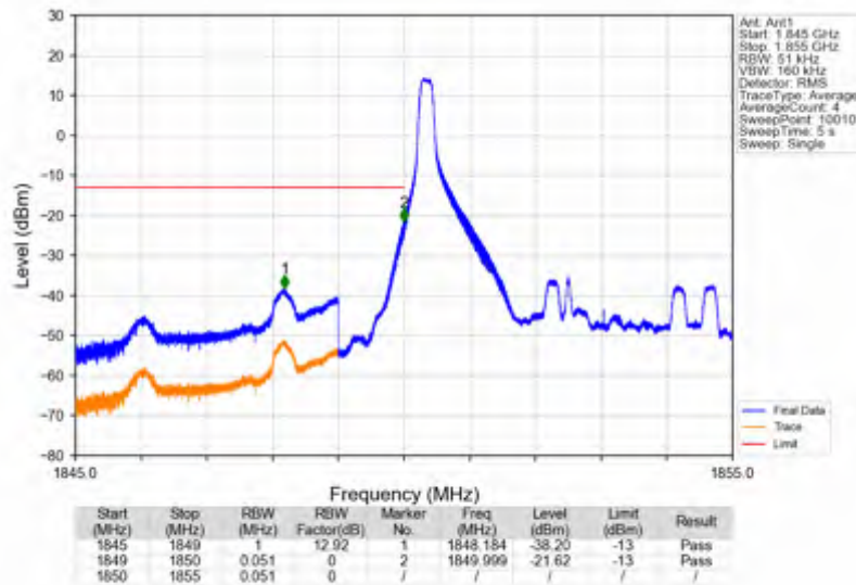
Band25 5MHz 256QAM LCH 1852.5MHz RB 1 0 NTNV
