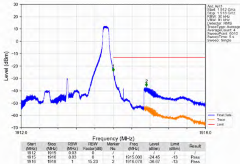
Band25_3MHz_256QAM_HCH_1913.5MHz_RB_1_14_NTNV
