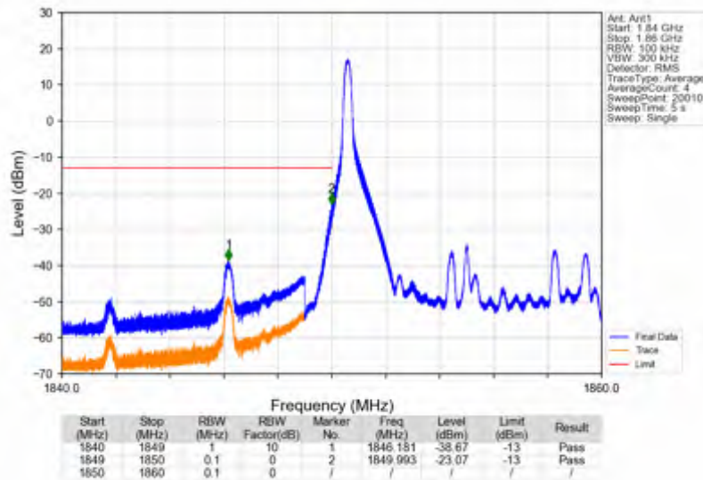
Band25_10MHz_256QAM_LCH_1855MHz_RB_1_0_NTNV
