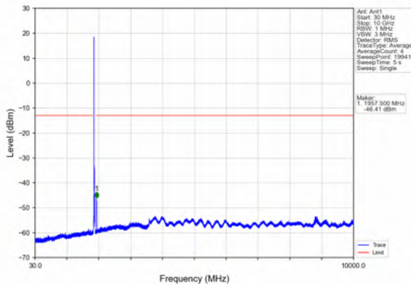
Band25_20MHz_256QAM_MCH_1882.5MHz_RB_1_0_NTNV
