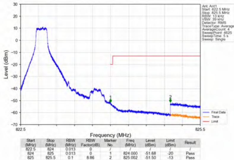
Band26a_1.4MHz_QPSK_HCH_823.3MHz_RB_1_5_NTNV
