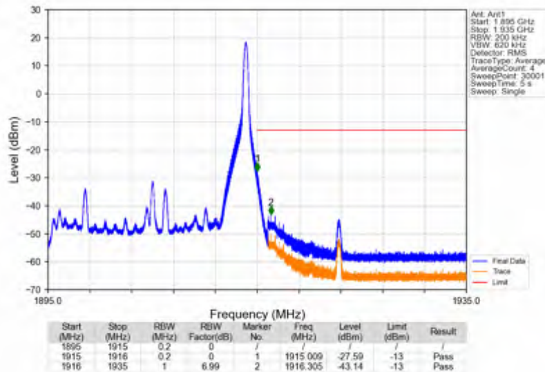
Band25_20MHz_256QAM_HCH_1905MHz_RB_1_99_NTNV
