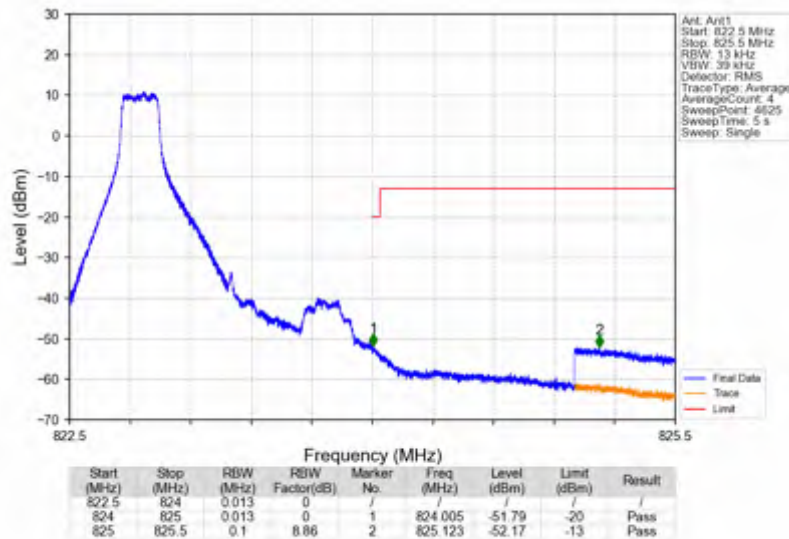
Band26a_1.4MHz_64QAM_HCH_823.3MHz_RB_1_5_NTNV
