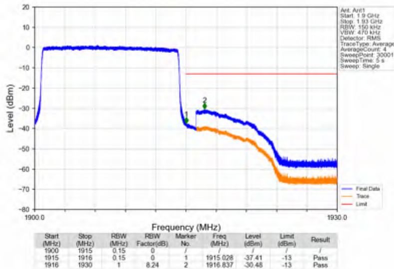
Band25_15MHz_256QAM_HCH_1907.5MHz_RB_75_0_NTNV
