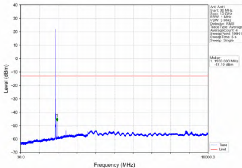
Band25 10MHz 16QAM MCH 1882.5MHz RB 1 0 NTNv
