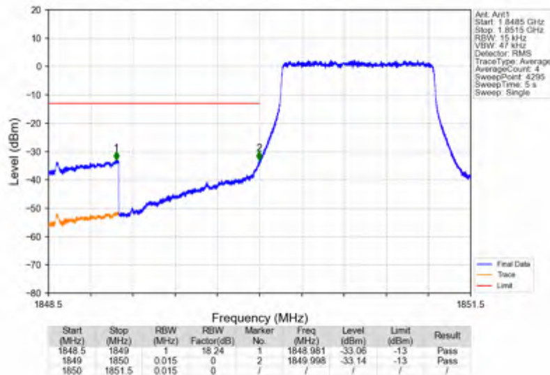
Band25_1.4MHz_256QAM_LCH_1850.7MHz_RB_6_0_NTNV
