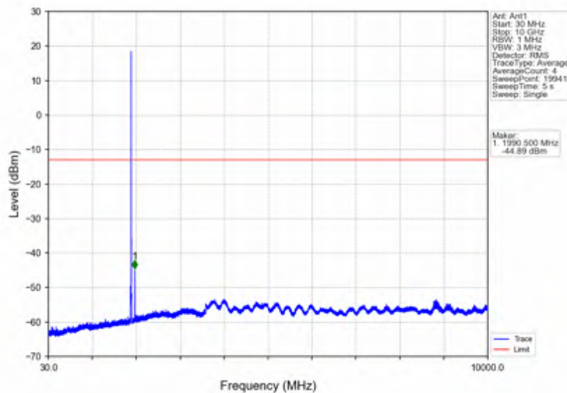
Band25_10MHz_256QAM_HCH_1910MHz_RB_1_0_NTNV
