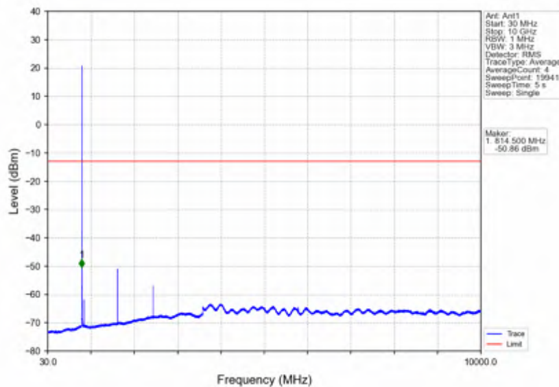
Band26a_1.4MHz_16QAM_HCH_823.3MHz_RB_1_0_NTNV
