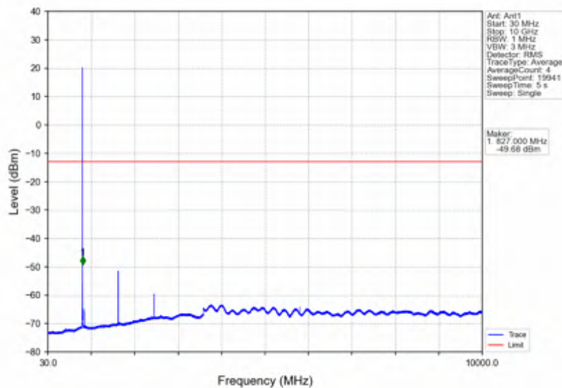
Band26a_1.4MHz_64QAM_HCH_823.3MHz_RB_1_5_NTNV
