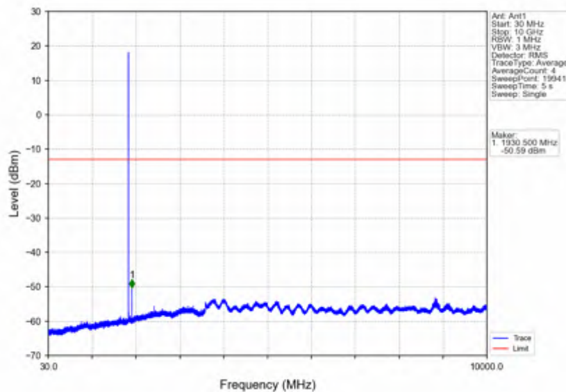
Band25 1.4MHz 256QAM LCH 1850.7MHz RB 1 0 NTV
