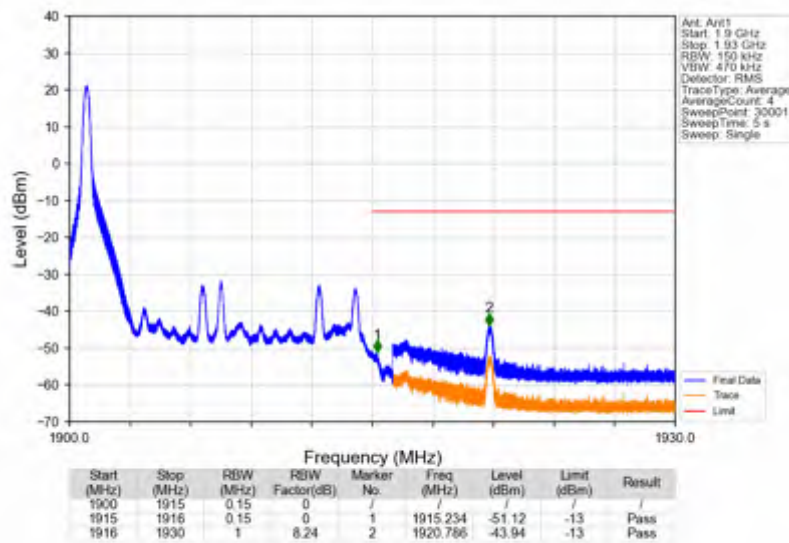
Band25_15MHz_16QAM_HCH_1907.5MHz_RB_75_0_NTNV
