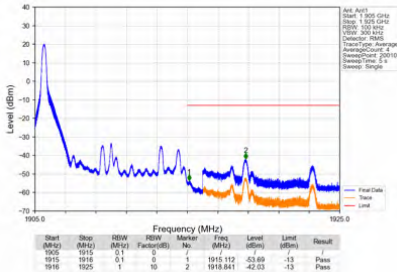
Band25_10MHz_16QAM_HCH_1910MHz_RB_1_49_NTNV
