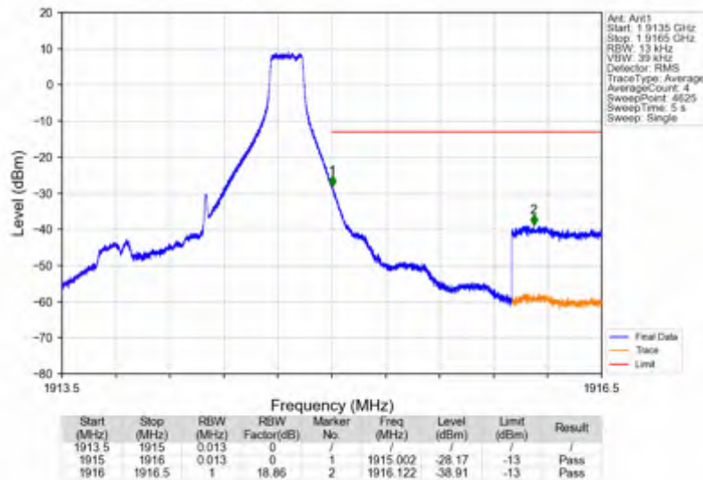
Band25_1.4MHz_256QAM_HCH_1914.3MHz_RB_1_5_NTNV
