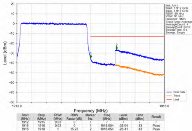
Band25_3MHz_256QAM_HCH_1913.5MHz_RB_15_0_NTNV
