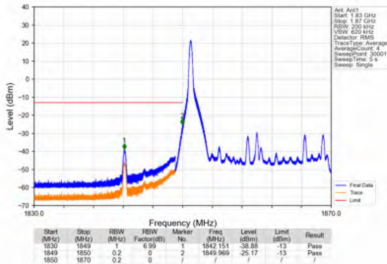
Band25_20MHz_16QAM_LCH_1860MHz_RB_100_0_NTNV
