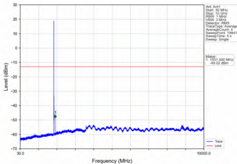
Band25_10MHz_256QAM_LCH_1855MHz_RB_1_0_NTNV
