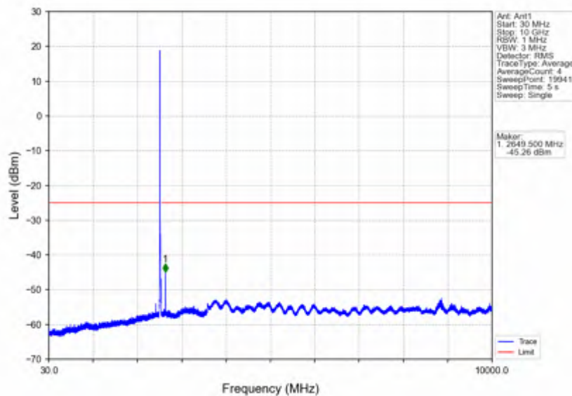
Band7_15MHz_256QAM_MCH_2535MHz_RB_1_0_NTNV
