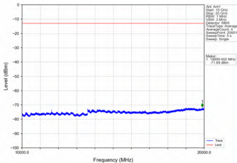
Band25_20MHz_16QAM_HCH_1905MHz_RB_1_0_NTV
