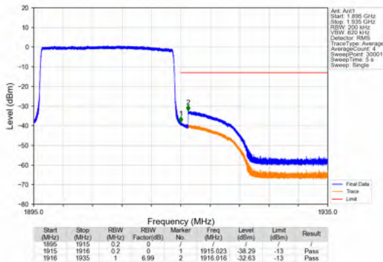
Band25_20MHz_256QAM_HCH_1905MHz_RB_100_0_NTNV
