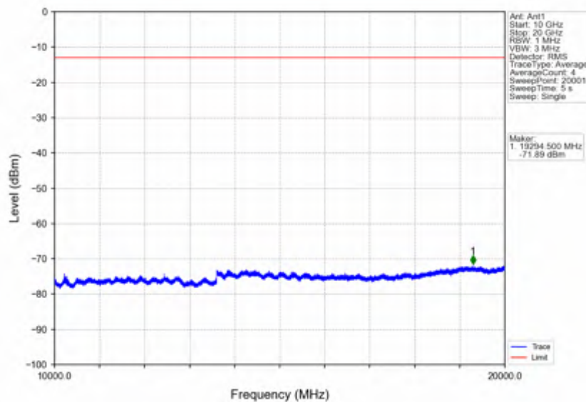
Band25_15MHz_256QAM_MCH_1882.5MHz_RB_1_0_NTNV
