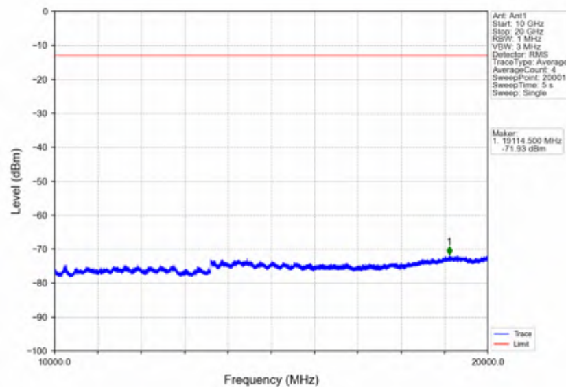
Band25_10MHz_256QAM_LCH_1855MHz_RB_50_0_NTNV
