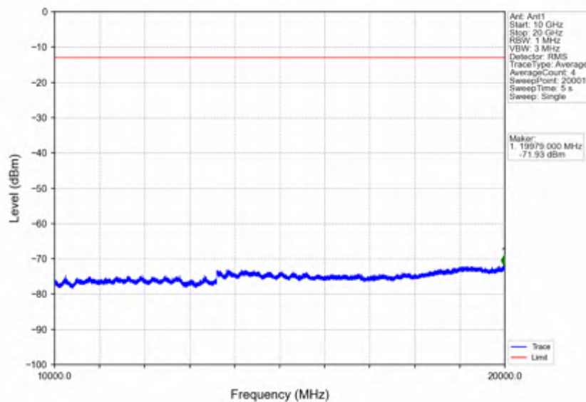
Band25 15MHz 64QAM HCH 1907.5MHz RB 1 0 NTNV
