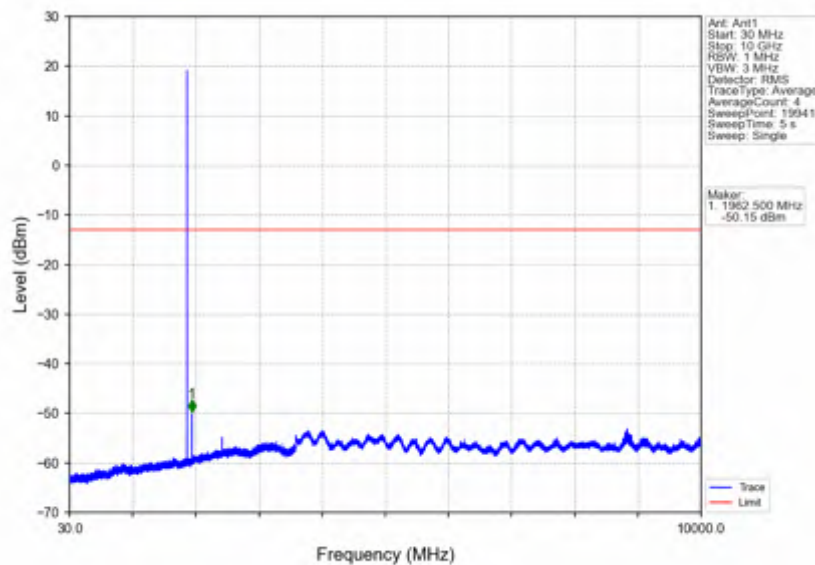
Band25_1.4MHz_256QAM_MCH_1882.5MHz_RB_1_0_NTNV
