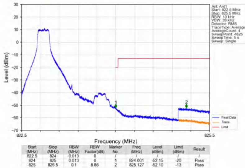
Band26a_1.4MHz_16QAM_HCH_823.3MHz_RB_6_0_NTNV
