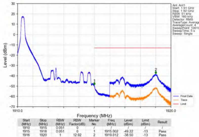
Band25_5MHz_64QAM_HCH_1912.5MHz_RB_1_24_NTNV
