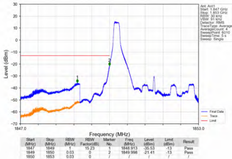
Band25_3MHz_QPSK_LCH_1851.5MHz_RB_15_0_NTNV
