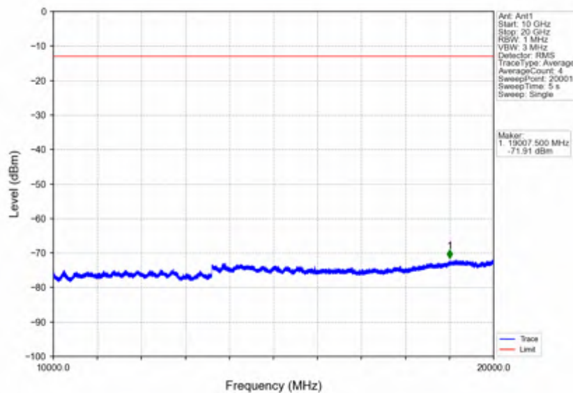
Band25_3MHz_256QAM_MCH_1882.5MHz_RB_1_0_NTNV
