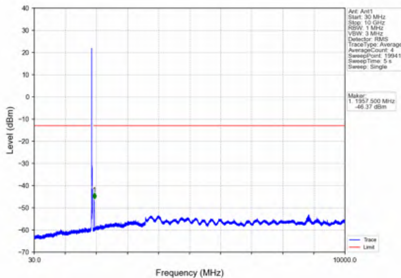
Band25 20MHz 16QAM MCH 1882.5MHz RB 1 0 NTNV
