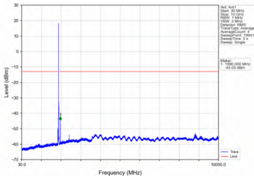
Band25_20MHz_256QAM_HCH_1905MHz_RB_1_0_NTNV
