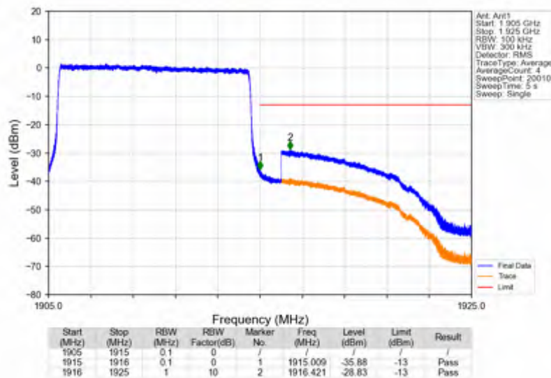
Band25 10MHz 256QAM HCH 1910MHz RB 50 0 NTNV
