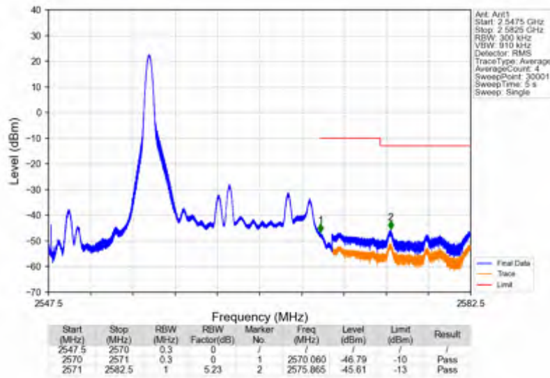
Band7_15MHz_16QAM_HCH_2562.5MHz_RB_1_74_NTNV
