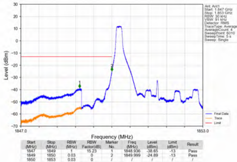
Band25_3MHz_256QAM_LCH_1851.5MHz_RB_1_0_NTNV
