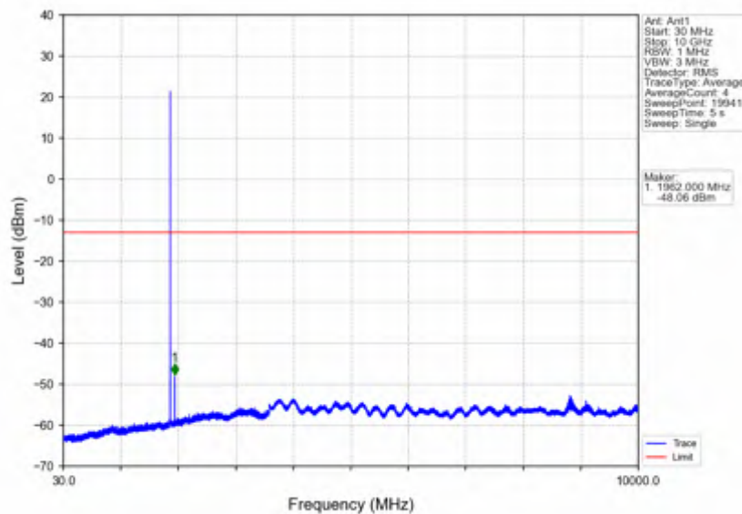
Band25_3MHz_16QAM_MCH_1882.5MHz_RB_1_0_NTNV
