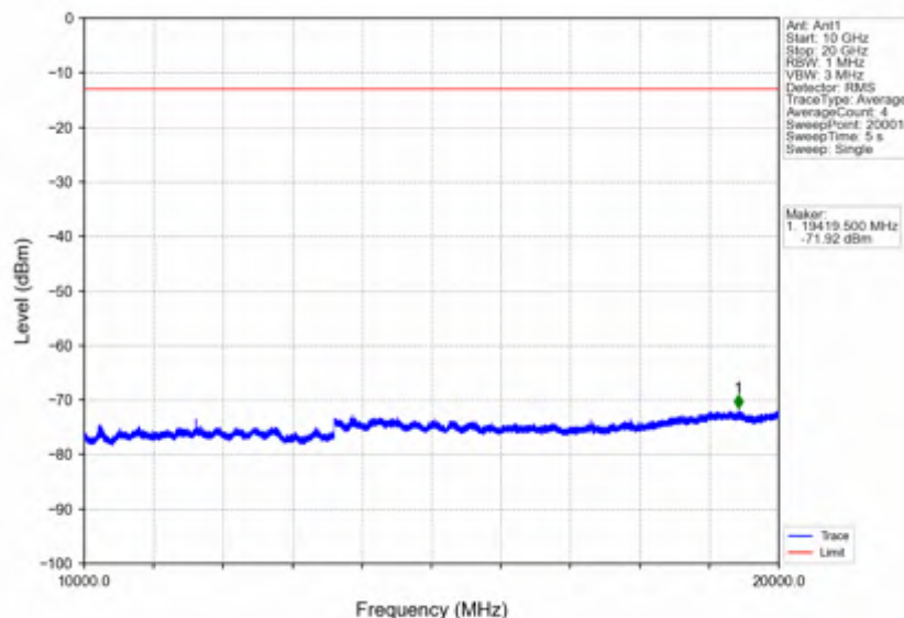
Band25_3MHz_256QAM_HCH_1913.5MHz_RB_1_0_NTNV
