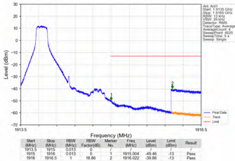
Band25_1.4MHz_16QAM_HCH_1914.3MHz_RB_1_5_NTNV
