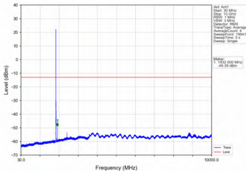
Band25_10MHz_16QAM_LCH_1855MHz_RB_1_0_NTV
