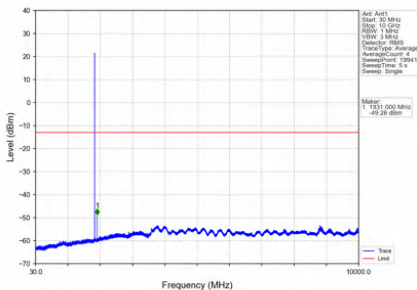
Band25_3MHz_QPSK_LCH_1851.5MHz_RB_1_0_NTNV
