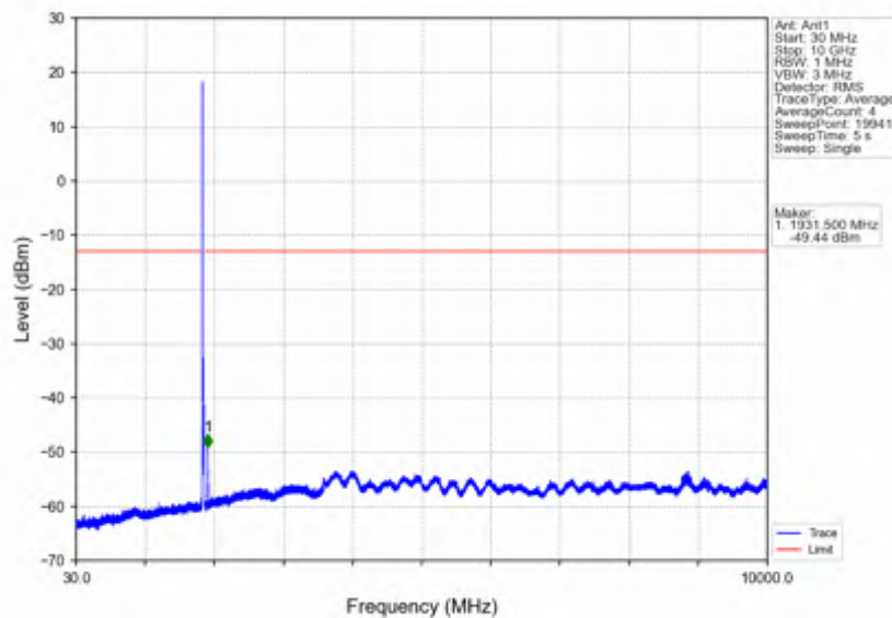
Band25 15MHz 256QAM LCH 1857.5MHz RB 1 0 NTNV
