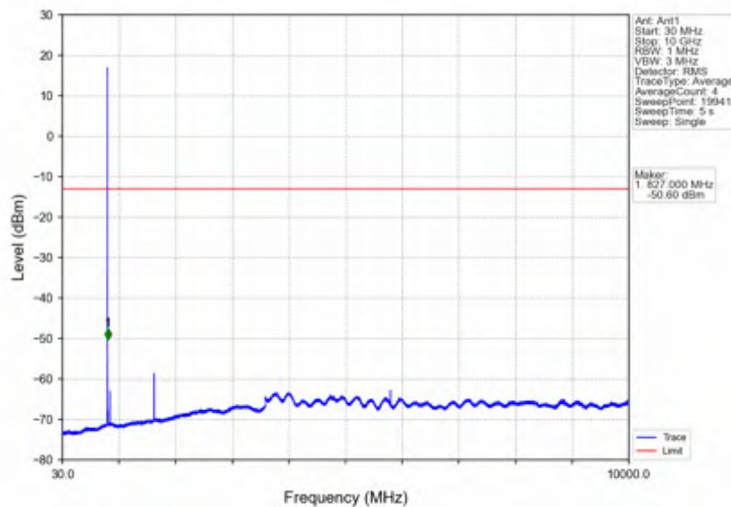
Band26a_1.4MHz_256QAM_HCH_823.3MHz_RB_1_0_NTNV
