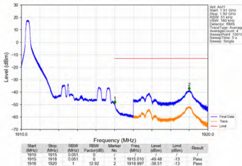
Band25_5MHz_64QAM_HCH_1912.5MHz_RB_25_0_NTNV
