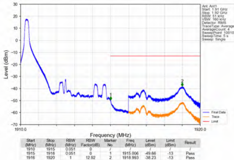
Band25 5MHz 16QAM HCH 1912.5MHz RB 1 24 NTNv
