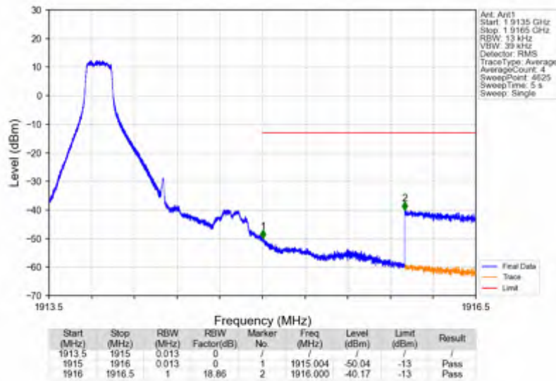
Band25_1.4MHz_64QAM_HCH_1914.3MHz_RB_1_5_NTNV
