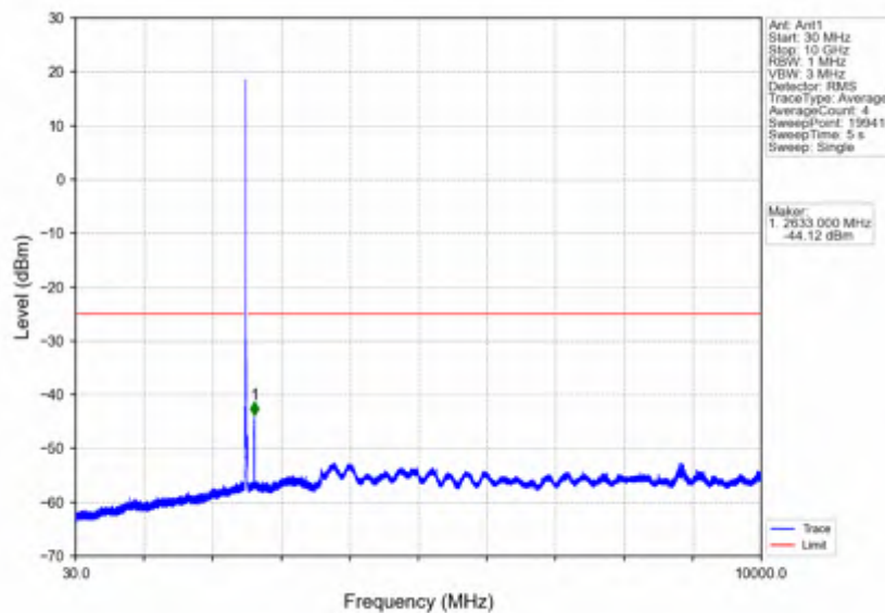
Band7_15MHz_256QAM_LCH_2507.5MHz_RB_1_0_NTNV
