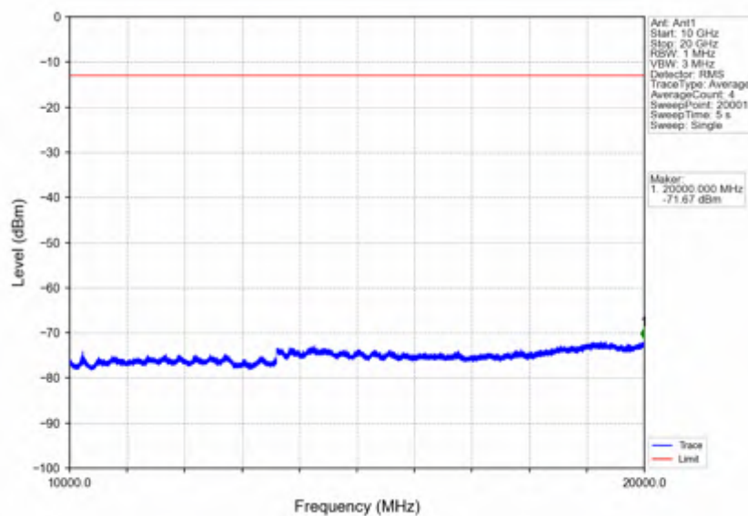
Band25_3MHz_64QAM_HCH_1913.5MHz_RB_1_0_NTNV
