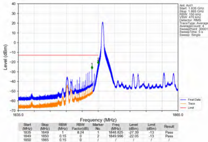
Band25_15MHz_64QAM_LCH_1857.5MHz_RB_1_0_NTNV
