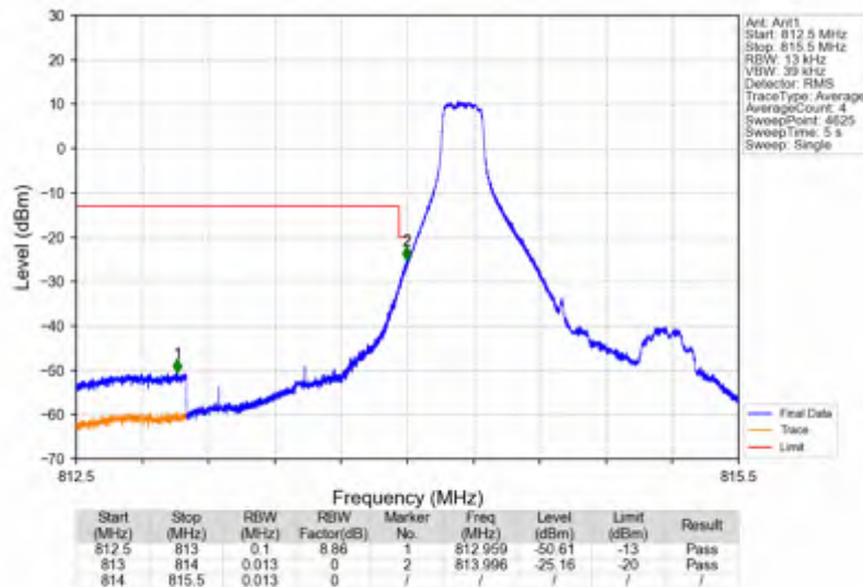
Band26a_1.4MHz_16QAM_LCH_814.7MHz_RB_6_0_NTNV
