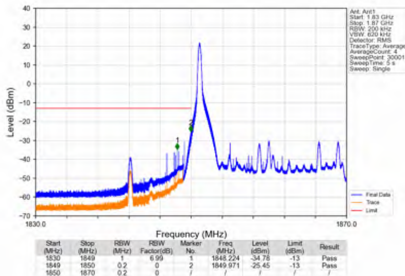
Band25_20MHz_64QAM_LCH_1860MHz_RB_100_0_NTNV
