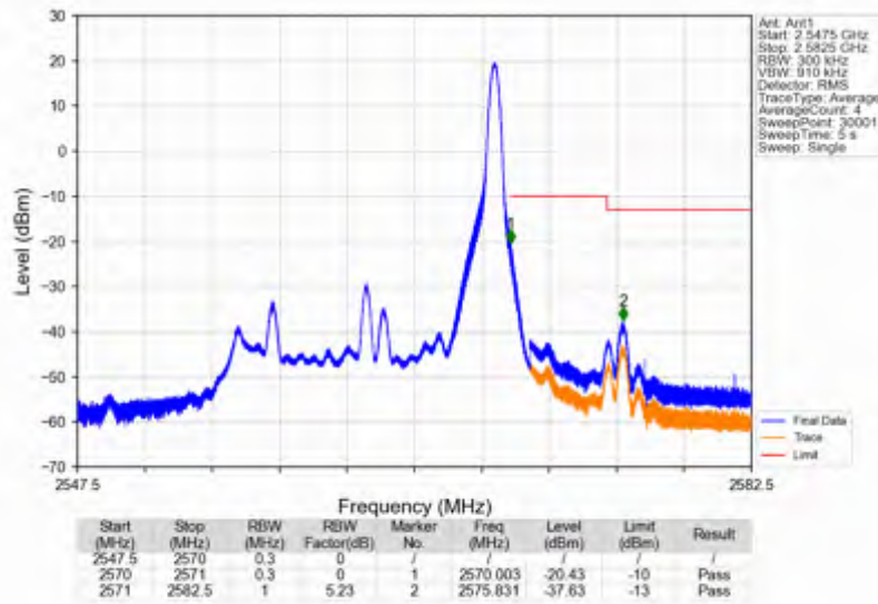
Band7_15MHz_256QAM_HCH_2562.5MHz_RB_1_74_NTNV
