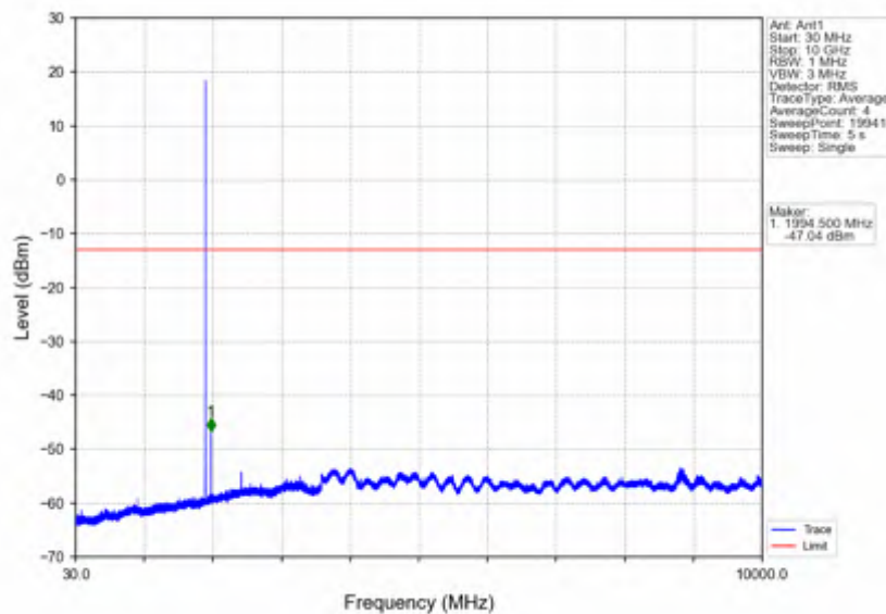
Band25_1.4MHz_256QAM_HCH_1914.3MHz_RB_1_0_NTNV
