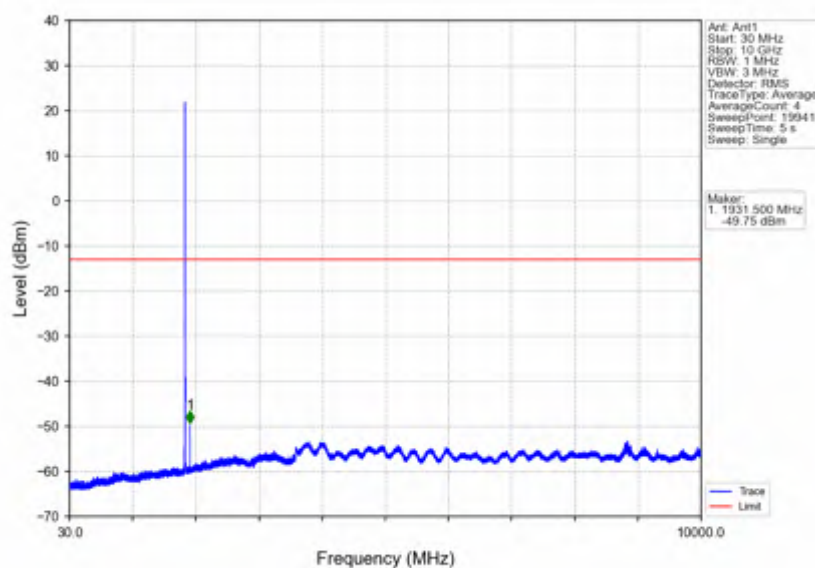
Band25_5MHz_QPSK_LCH_1852.5MHz_RB_1_0_NTNV
