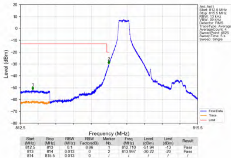
Band26a_1.4MHz_256QAM_LCH_814.7MHz_RB_1_0_NTNV
