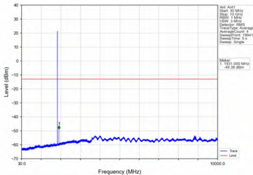
Band25 3MHz 64QAM LCH 1851.5MHz RB 1 0 NTNV
