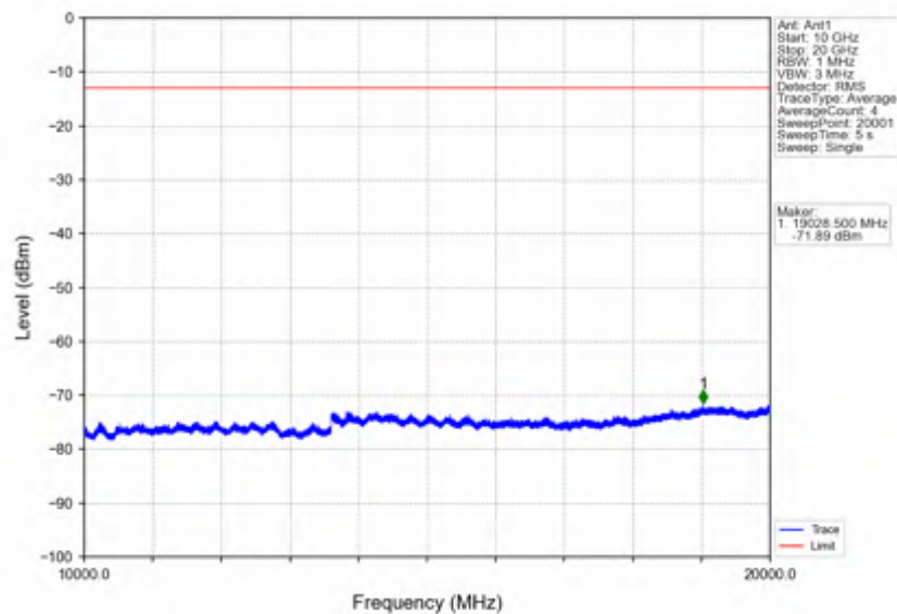
Band25_20MHz_16QAM_LCH_1860MHz_RB_100_0_NTNV
