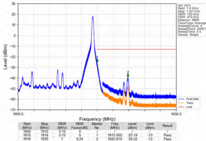
Band25_15MHz_256QAM_HCH_1907.5MHz_RB_1_74_NTNV
