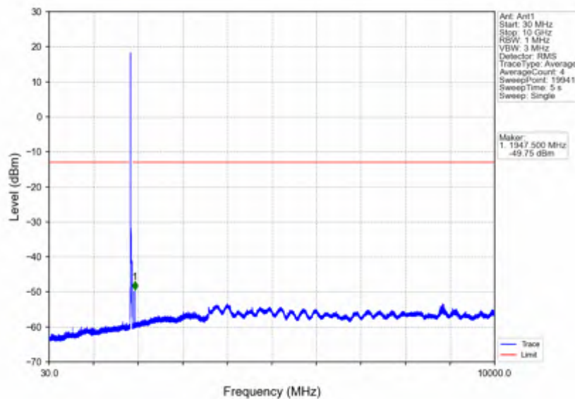
Band25 20MHz 256QAM LCH 1860MHz RB 1 0 NTV
