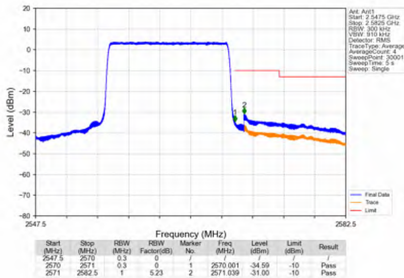
Band7_15MHz_256QAM_HCH_2562.5MHz_RB_75_0_NTNV
