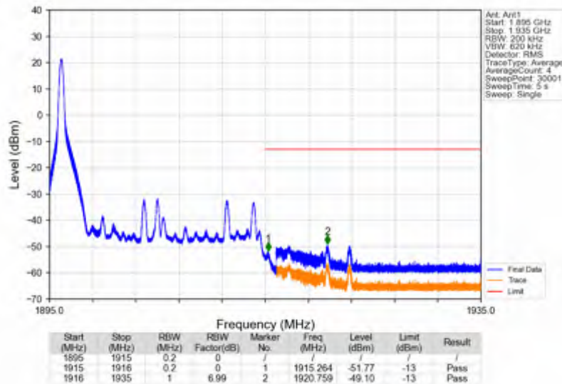
Band25_20MHz_16QAM_HCH_1905MHz_RB_1_99_NTNV
