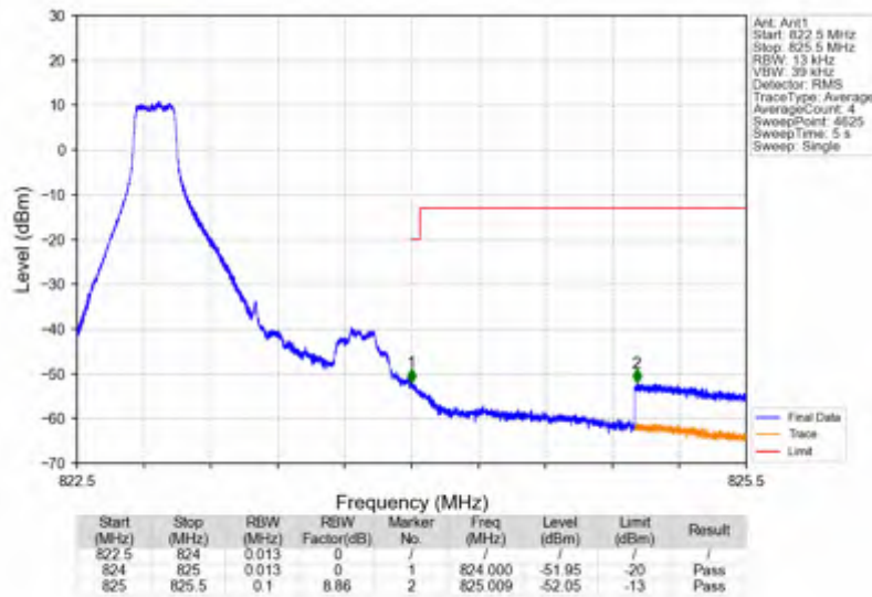
Band26a_1.4MHz_16QAM_HCH_823.3MHz_RB_1_5_NTNV
