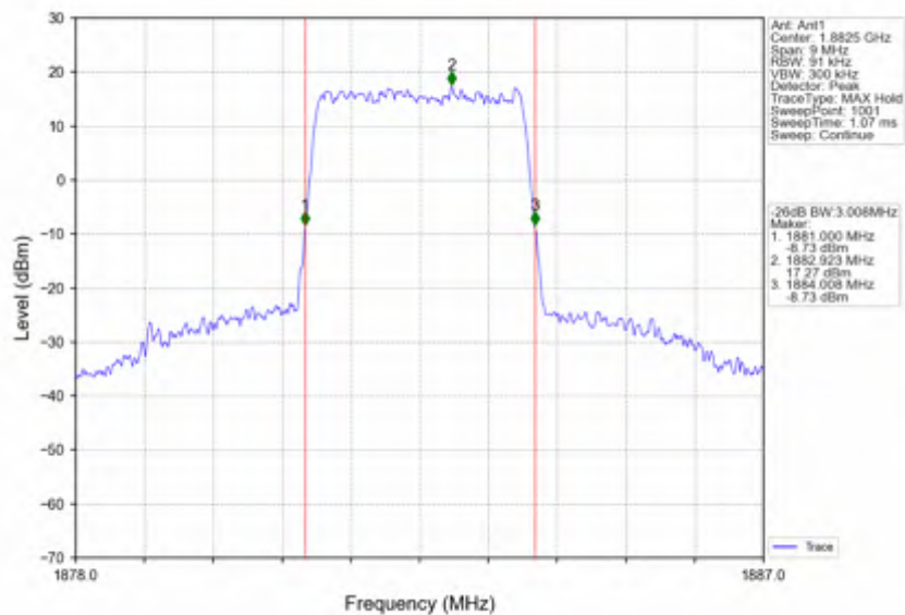
Band25 3MHz 64QAM MCH 1882.5MHz RB 15 0 NTN
