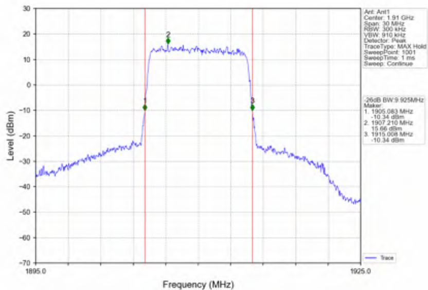
Band25 10MHz 256QAM HCH 1910MHz RB 50 0 NTNV
