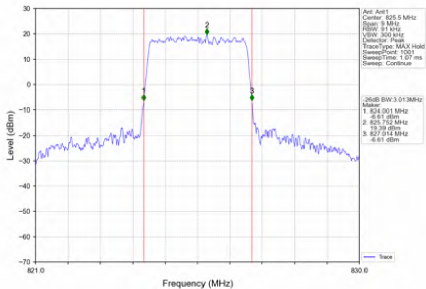
Band5 3MHz 16QAM LCH 825.5MHz RB 15 0 NTNV
