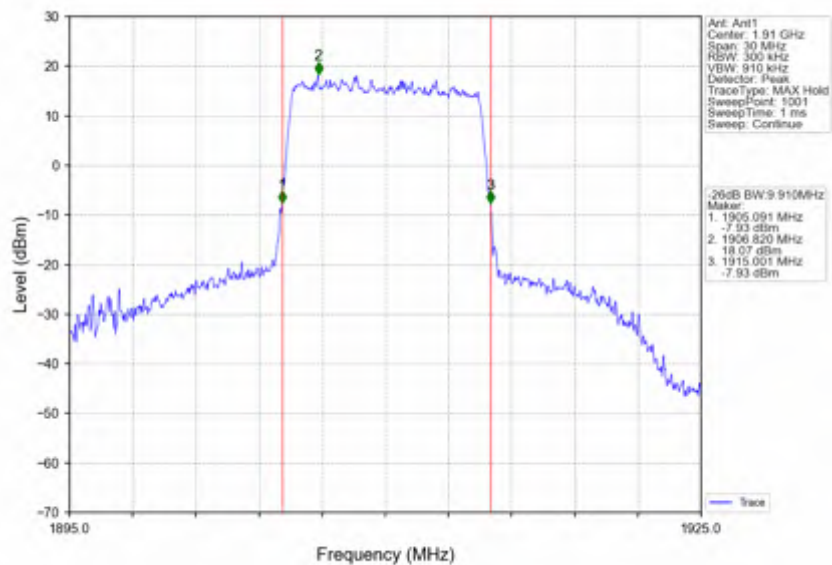
Band25 10MHz 16QAM HCH 1910MHz RB 50 0 NTNV
