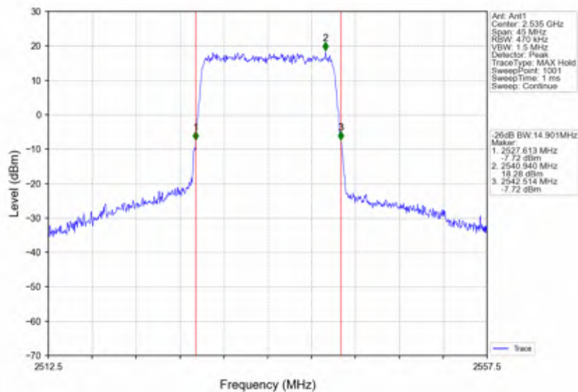
Band7 15MHz 64QAM MCH 2535MHz RB 75 0 NTN
