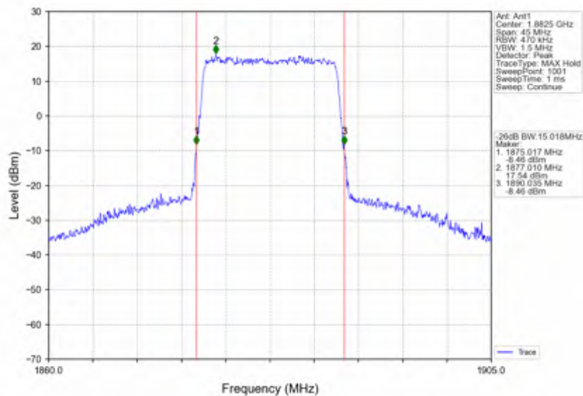
Band25 15MHz 64QAM MCH 1882.5MHz RB 75 0 NTNv
