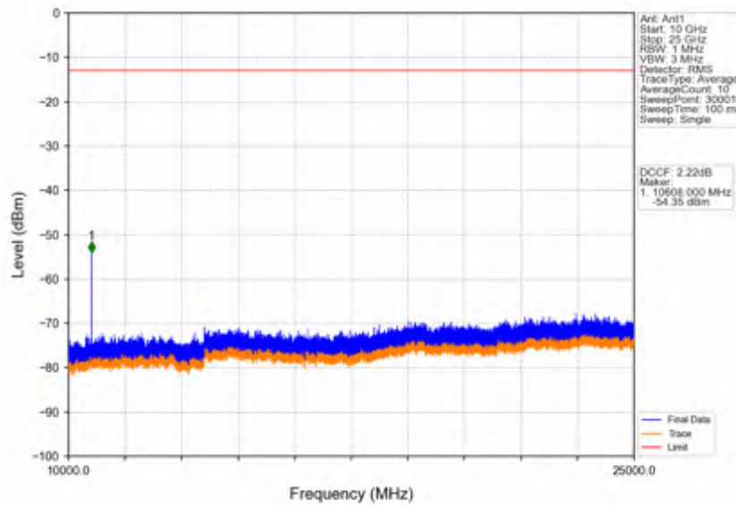
Band42a_15MHz_QPSK_HCH_3542.5MHz_RB_1_0_NTNV
