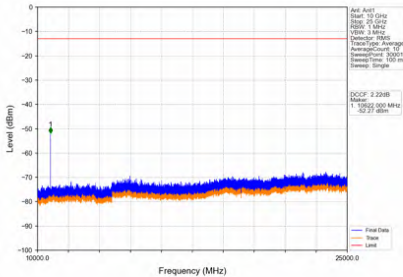
Band42a_10MHz_64QAM_HCH_3545MHz_RB_1_0_NTNV
