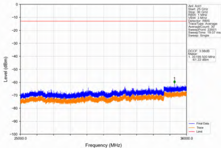
Band42c_20MHz_64QAM_LCH_3560MHz_RB_1_0_NTNV
