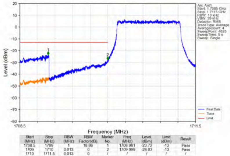
Band66_1.4MHz_16QAM_LCH_1710.7MHz_RB_6_0_NTNV
