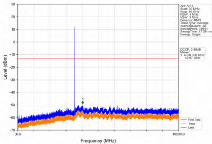
Band42c_5MHz_64QAM_LCH_3552.5MHz_RB_1_0_NTNV
