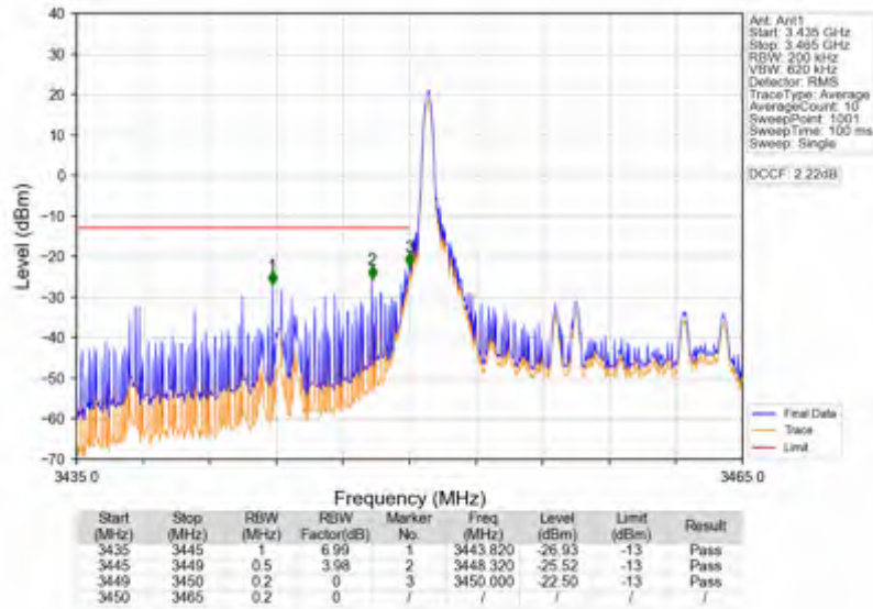
Band42a_15MHz_64QAM_LCH_3457.5MHz_RB_1_0_NTNV
