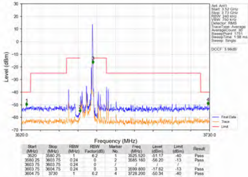
Band42c_15MHz_256QAM_HCH_3592.5MHz_RB_75_0_NTNV
