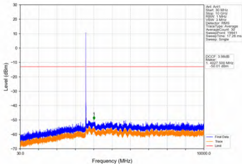
Band42c_15MHz_16QAM_HCH_3592.5MHz_RB_1_0_NTNV
