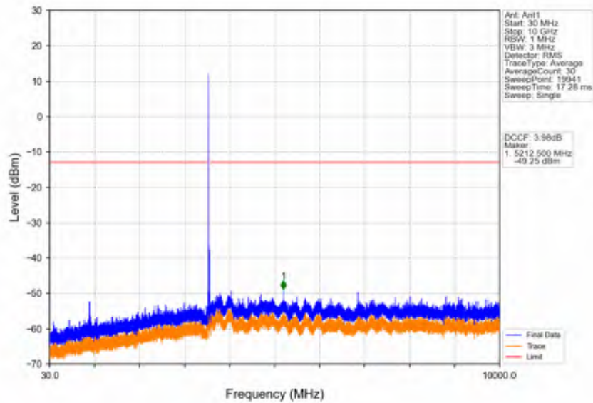
Band42c_15MHz_64QAM_LCH_3557.5MHz_RB_1_0_NTNV
