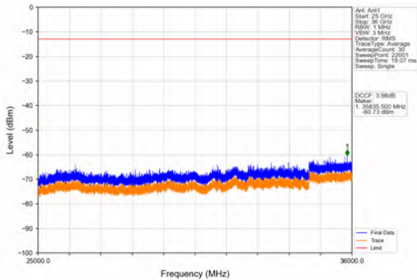
Band42c_5MHz_16QAM_LCH_3552.5MHz_RB_25_0_NTNV
