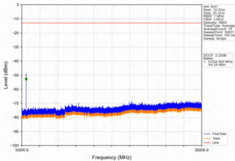
Band42a_15MHz_16QAM_LCH_3457.5MHz_RB_1_0_NTNV
