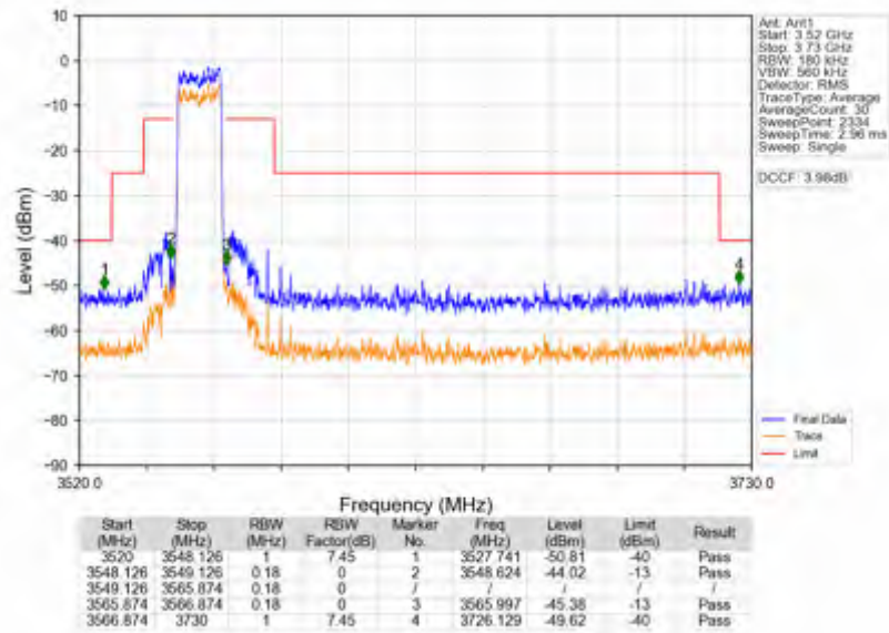
Band42c_15MHz_16QAM_LCH_3557.5MHz_RB_75_0_NTNV
