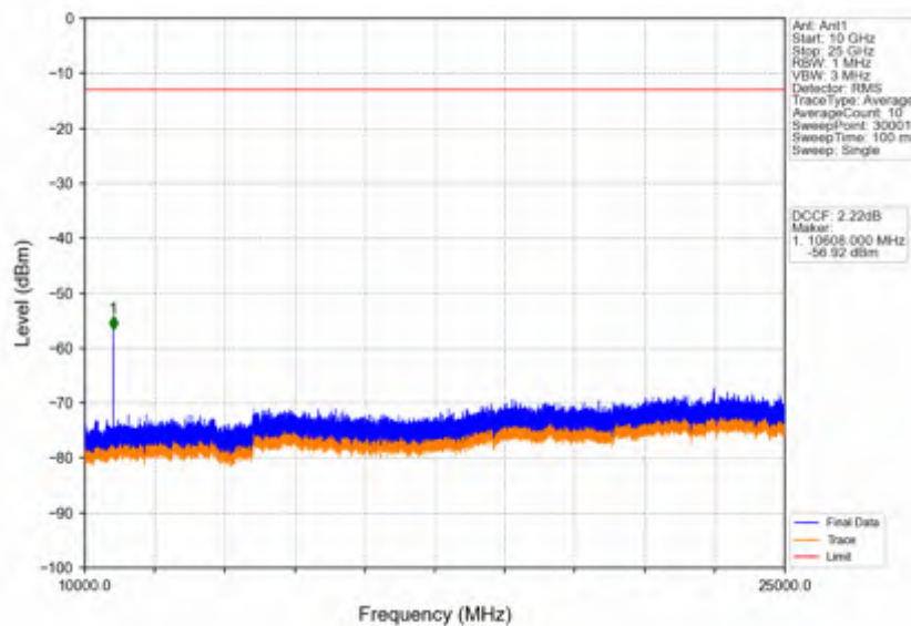
Band42a_15MHz_64QAM_HCH_3542.5MHz_RB_1_0_NTNV
