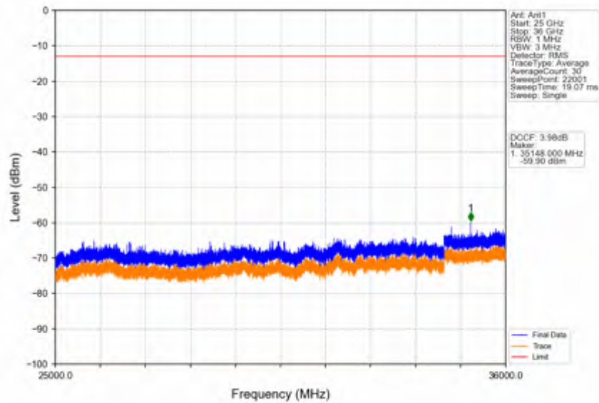
Band42c_10MHz_16QAM_LCH_3555MHz_RB_50_0_NTNV
