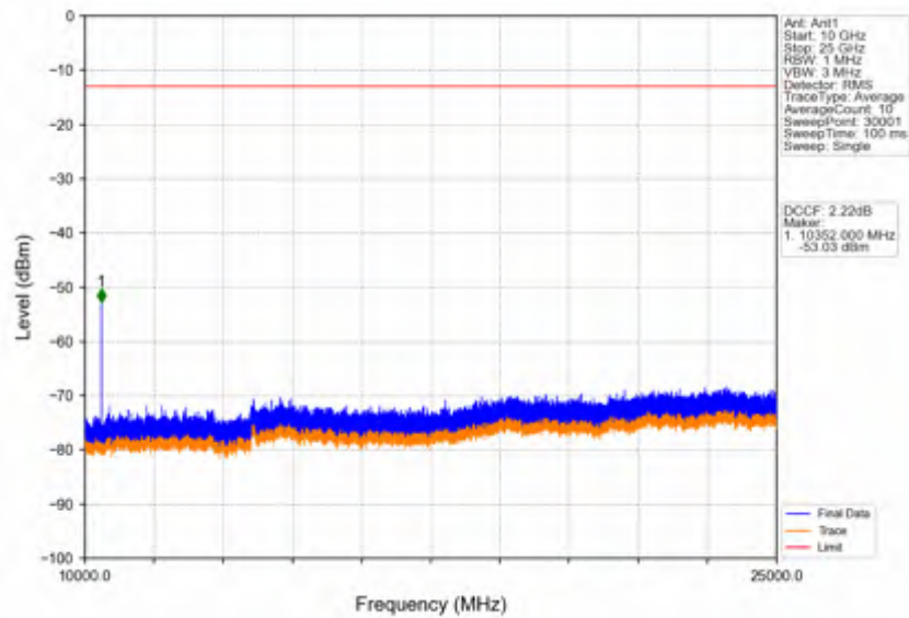
Band42a_15MHz_64QAM_LCH_3457.5MHz_RB_1_0_NTNV
