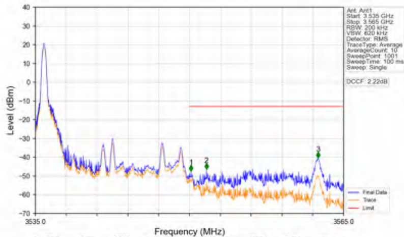
Band42a_15MHz_QPSK_HCH_3542.5MHz_RB_1_74_NTNV
