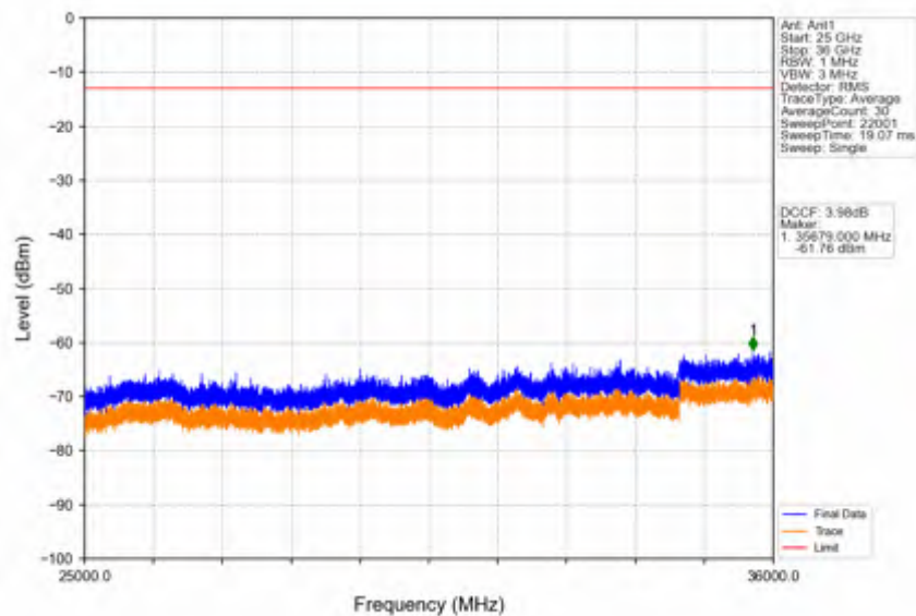
Band42c_5MHz_64QAM_LCH_3552.5MHz_RB_1_0_NTNV
