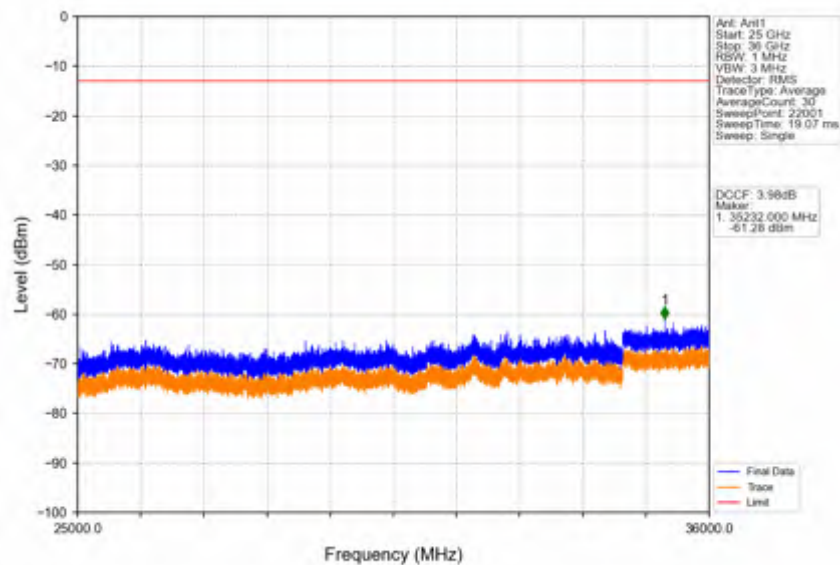
Band42c_20MHz_256QAM_HCH_3590MHz_RB_1_0_NTNV
