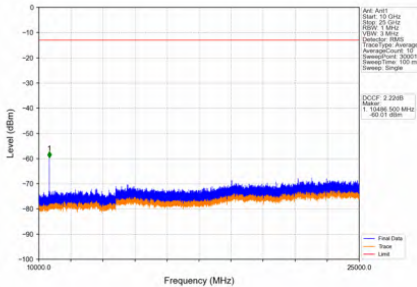
Band42a_10MHz_256QAM_MCH_3500MHz_RB_1_0_NTNV
