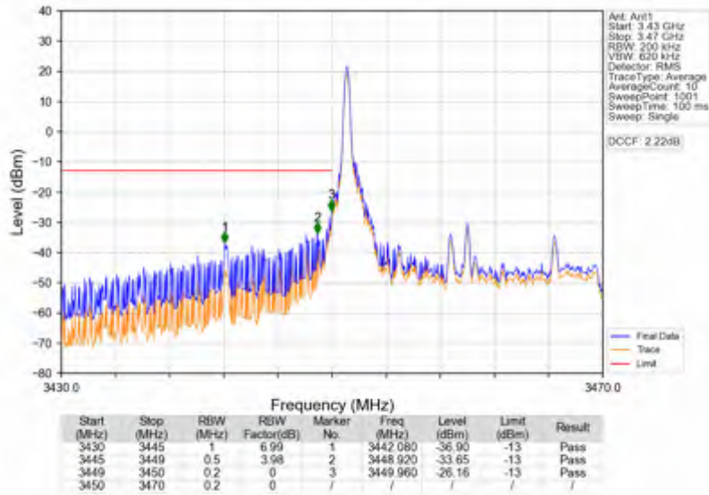
Band42a_20MHz_64QAM_LCH_3460MHz_RB_1_0_NTNV
