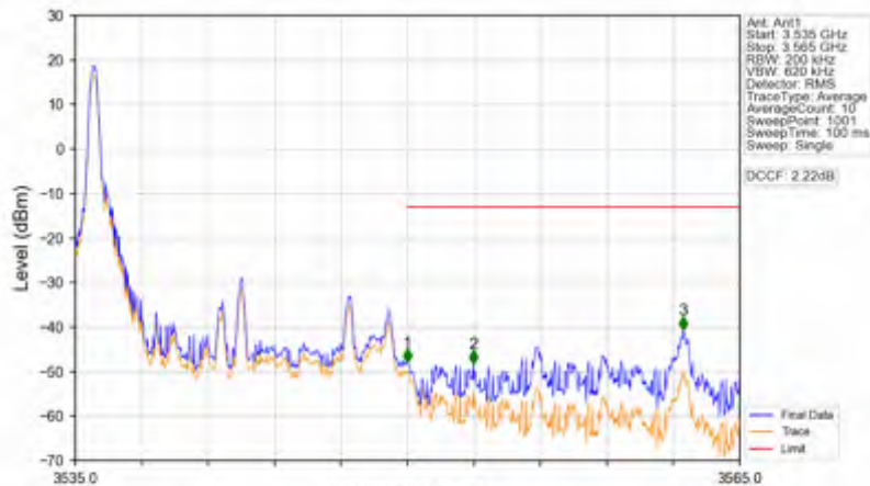
Band42a_15MHz_64QAM_HCH_3542.5MHz_RB_1_74_NTNV
