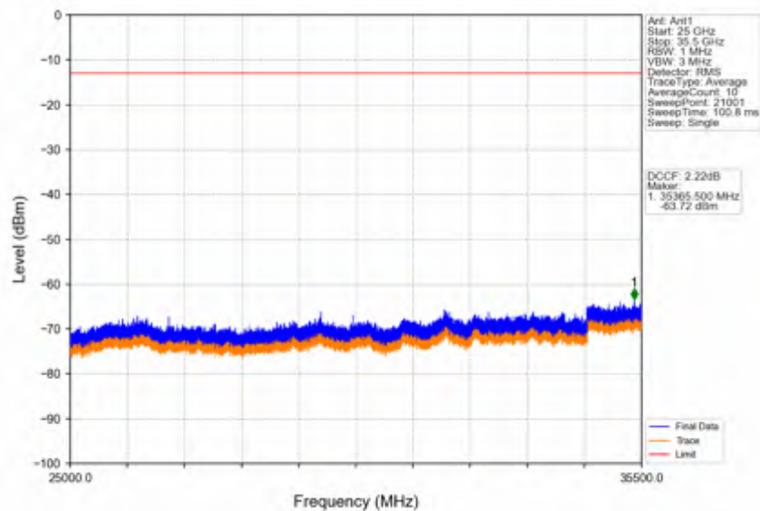
Band42a_15MHz_64QAM_MCH_3500MHz_RB_1_0_NTNV
