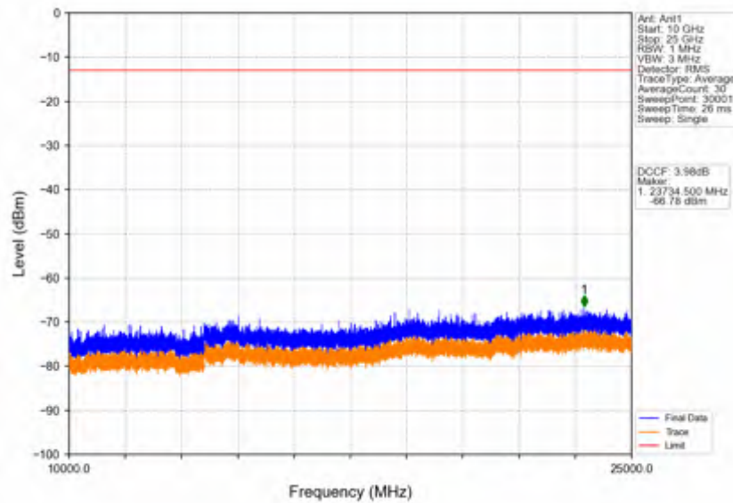
Band42c_10MHz_QPSK_MCH_3575MHz_RB_1_0_NTV
