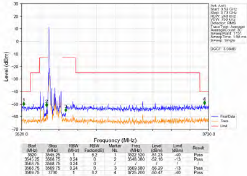
Band42c_15MHz_64QAM_LCH_3557.5MHz_RB_1_0_NTNV
