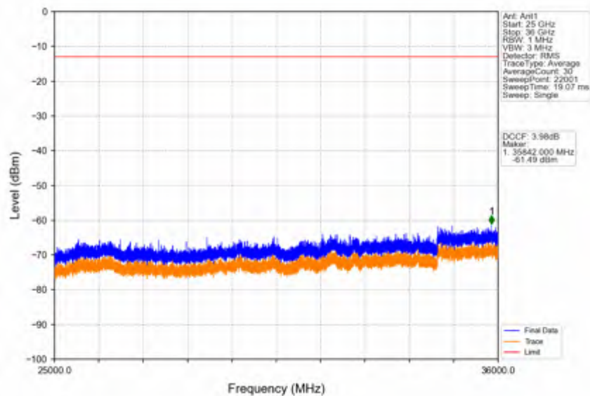
Band42c_10MHz_16QAM_HCH_3595MHz_RB_1_0_NTNV
