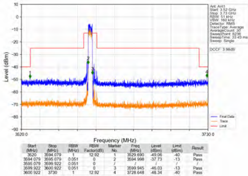
Band42c_5MHz_256QAM_HCH_3597.5MHz_RB_25_0_NTNV
