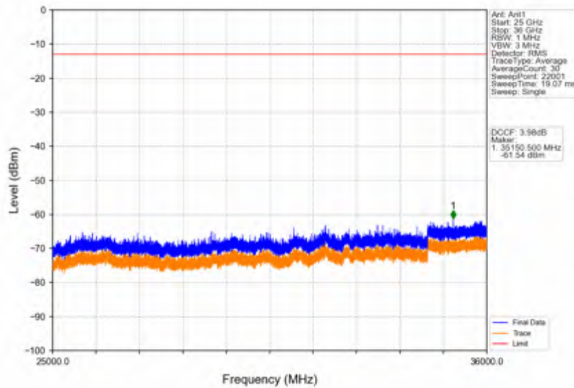
Band42c_5MHz_QPSK_HCH_3597.5MHz_RB_1_24_NTNV
