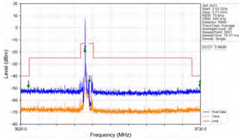
Band42c_5MHz_64QAM_HCH_3597.5MHz_RB_1_24_NTNV
