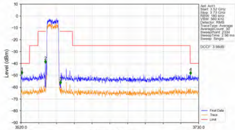
Band42c_15MHz_256QAM_LCH_3557.5MHz_RB_75_0_NTNV
