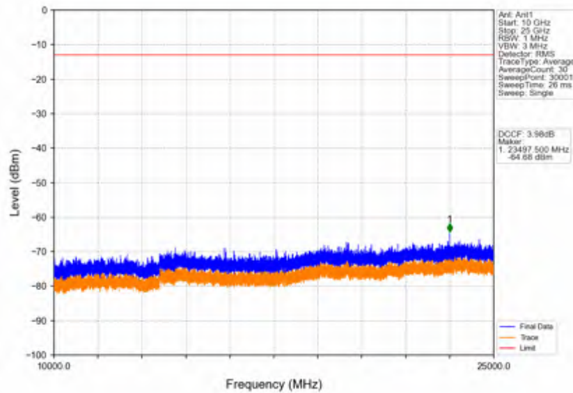
Band42c_5MHz_QPSK_LCH_3552.5MHz_RB_1_0_NTV
