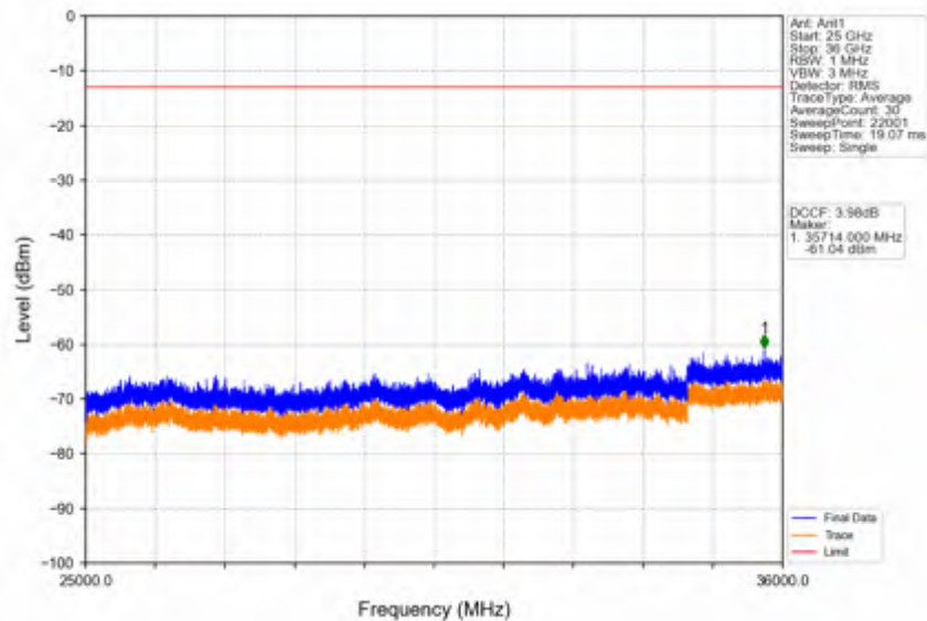
Band42c_15MHz_QPSK_MCH_3575MHz_RB_1_0_NTV
