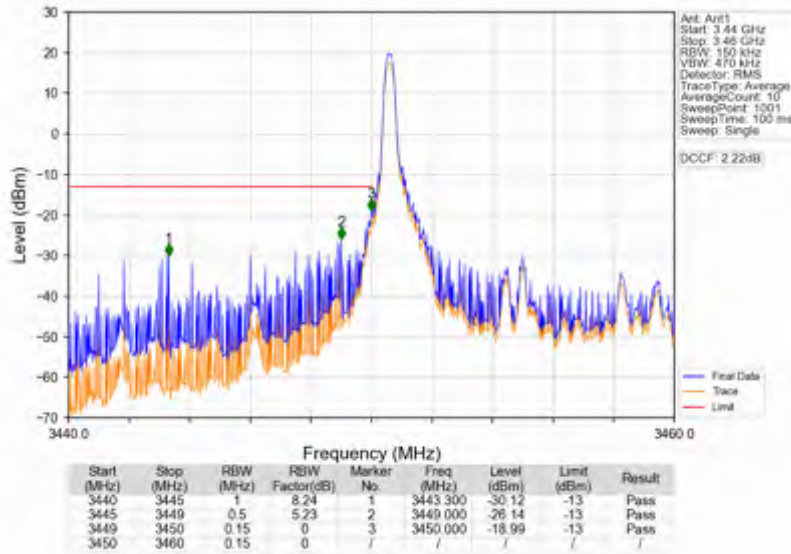
Band42a_10MHz_64QAM_LCH_3455MHz_RB_1_0_NTNV
