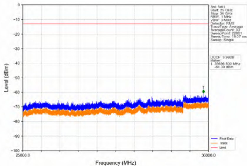
Band42c_15MHz_64QAM_MCH_3575MHz_RB_1_0_NTNV
