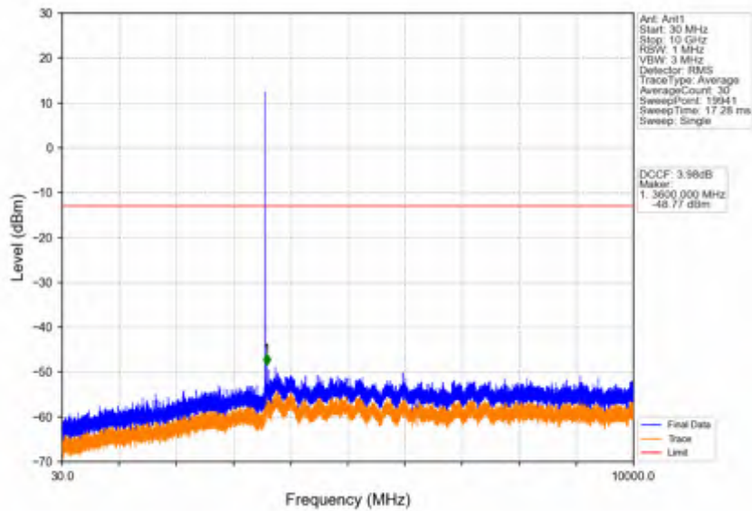
Band42c_5MHz_16QAM_MCH_3575MHz_RB_1_0_NTV
