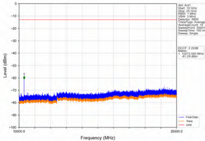
Band42a_20MHz_256QAM_MCH_3500MHz_RB_1_0_NTNV
