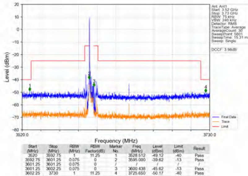
Band42c_5MHz_QPSK_HCH_3597.5MHz_RB_1_24_NTNV
