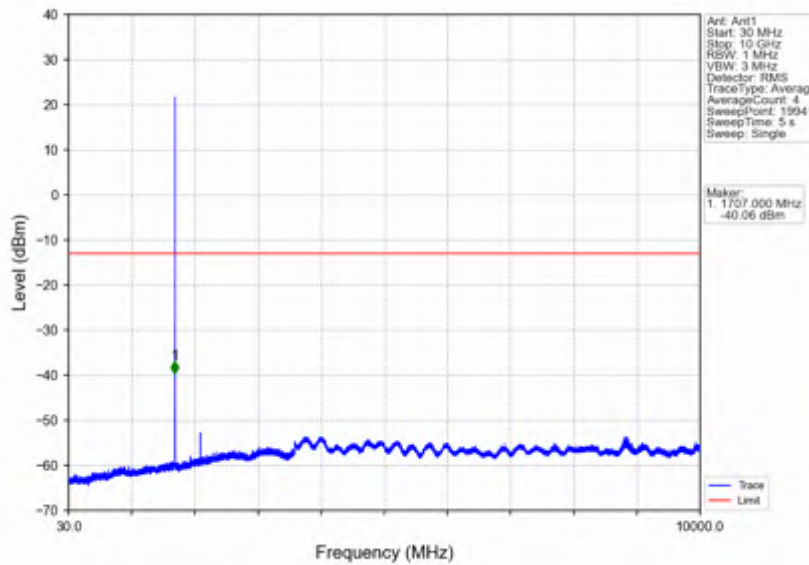
Band66_1.4MHz_16QAM_LCH_1710.7MHz_RB_1_0_NTNV
