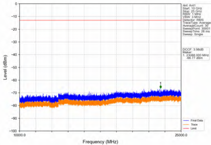
Band42c_5MHz_64QAM_MCH_3575MHz_RB_1_0_NTV
