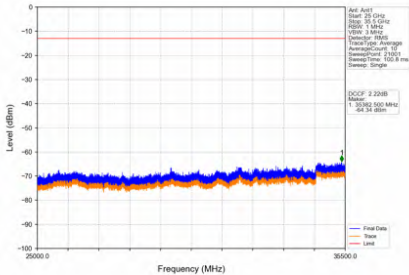
Band42a_15MHz_256QAM_LCH_3457.5MHz_RB_75_0_NTNV
