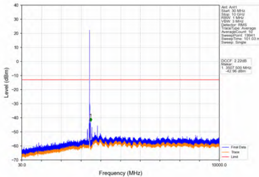
Band42a_15MHz_64QAM_LCH_3457.5MHz_RB_1_0_NTNV
