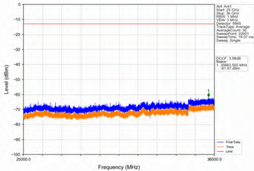
Band42c_10MHz_256QAM_LCH_3555MHz_RB_50_0_NTNV
