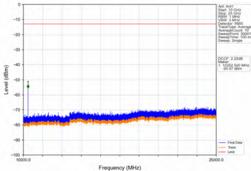
Band42a_15MHz_256QAM_LCH_3457.5MHz_RB_1_0_NTNV
