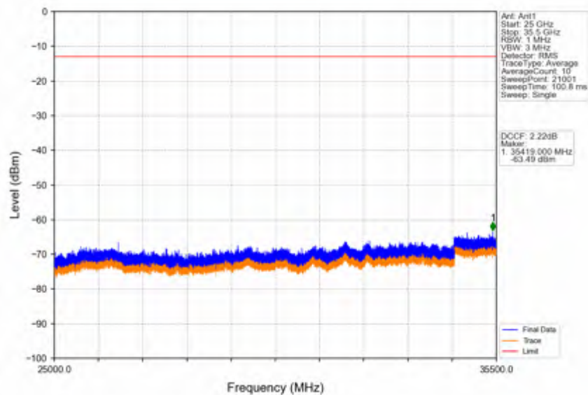
Band42a_20MHz_64QAM_LCH_3460MHz_RB_1_0_NTNV
