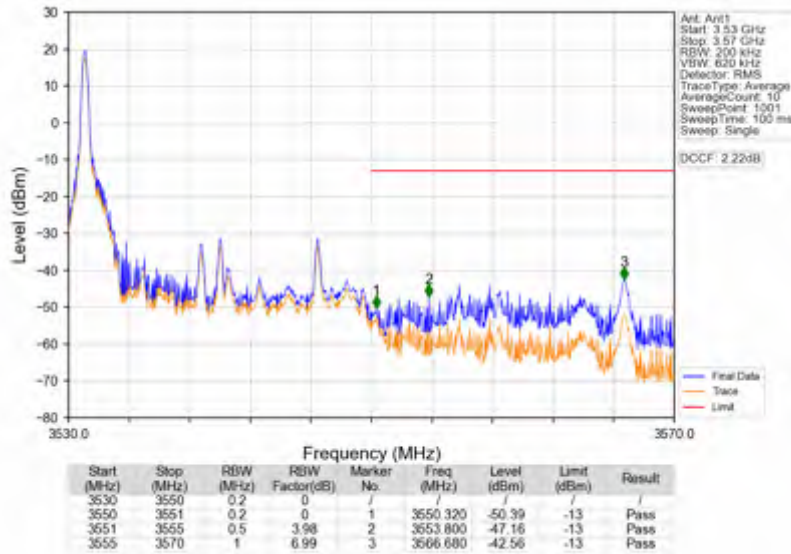
Band42a_20MHz_16QAM_HCH_3540MHz_RB_100_0_NTNV
