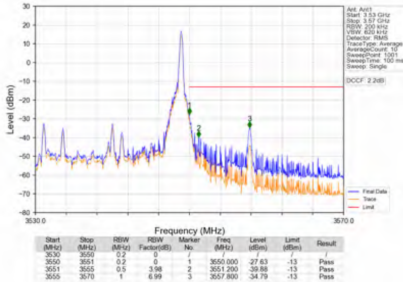
Band42a_20MHz_256QAM_HCH_3540MHz_RB_100_0_NTNV
