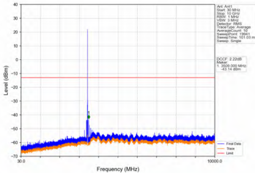
Band42a_10MHz_64QAM_LCH_3455MHz_RB_1_0_NTNV
