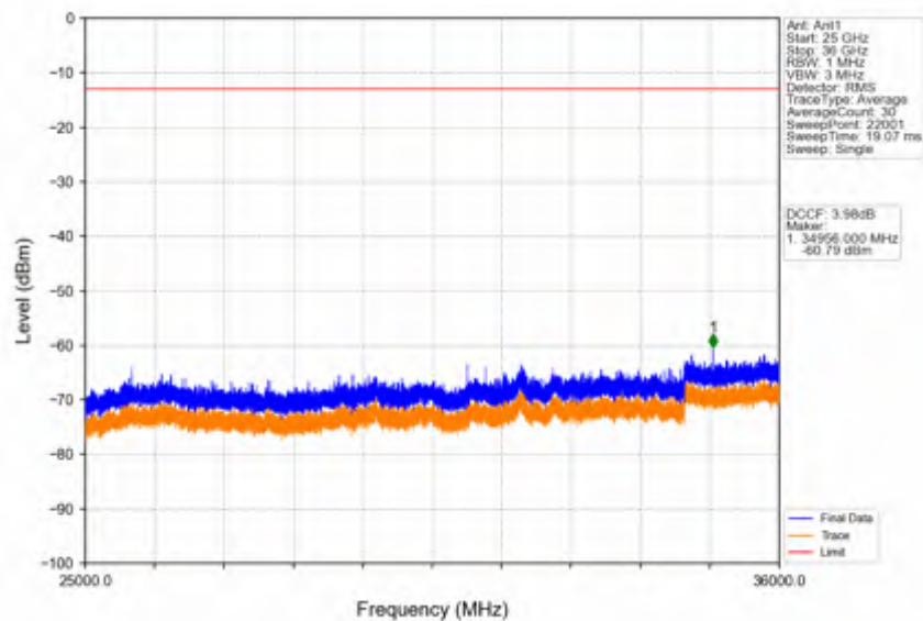
Band42c_15MHz_QPSK_LCH_3557.5MHz_RB_1_0_NTNV
