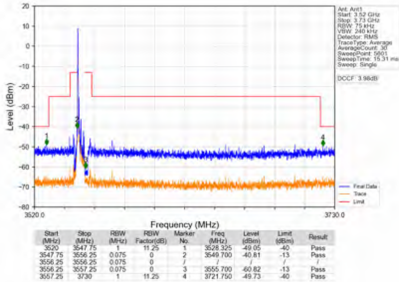
Band42c_5MHz_64QAM_LCH_3552.5MHz_RB_1_0_NTNV
