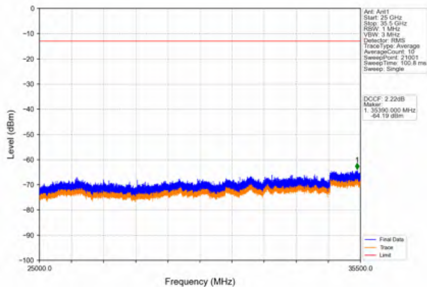
Band42a_10MHz_64QAM_LCH_3455MHz_RB_1_0_NTNV
