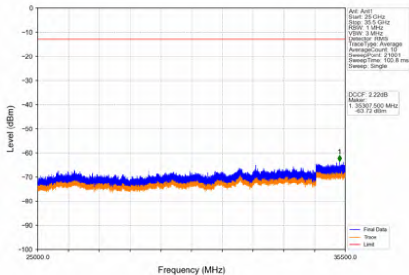
Band42a_20MHz_64QAM_MCH_3500MHz_RB_1_0_NTNV
