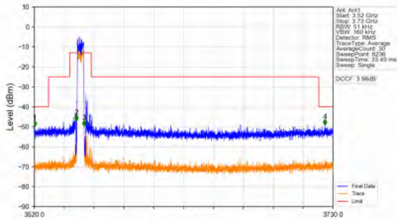
Band42c_5MHz_256QAM_LCH_3552.5MHz_RB_25_0_NTNV
