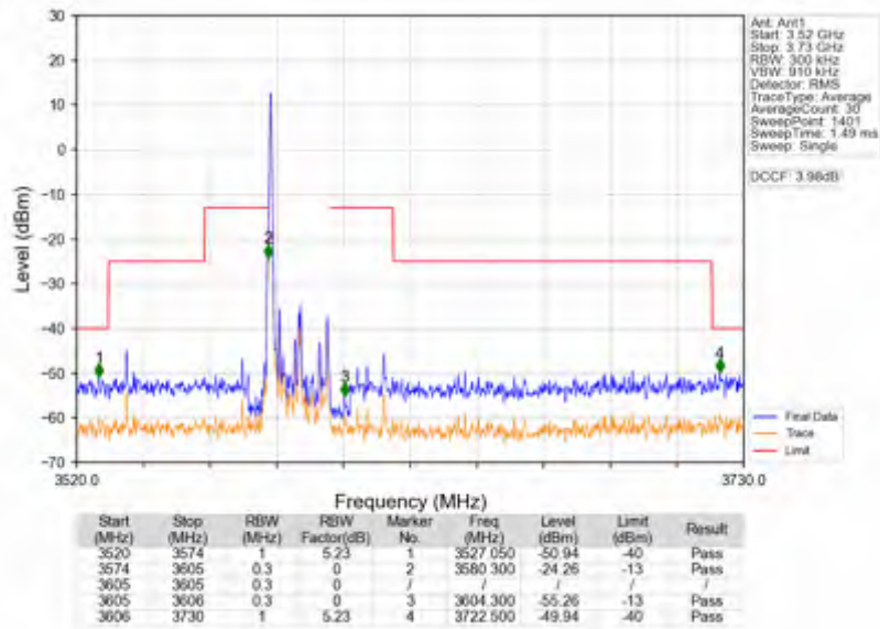
Band42c_20MHz_64QAM_HCH_3590MHz_RB_1_99_NTNV
