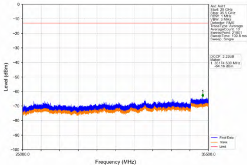
Band42a_10MHz_64QAM_MCH_3500MHz_RB_1_0_NTNV
