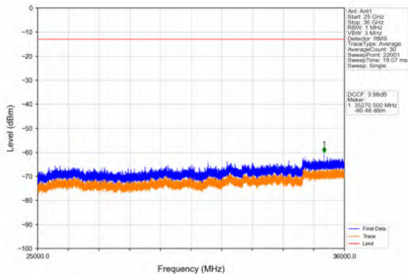
Band42c_20MHz_64QAM_MCH_3575MHz_RB_1_0_NTNV
