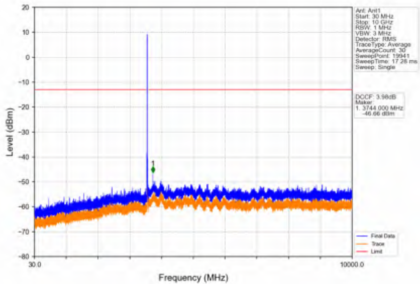
Band42c_15MHz_256QAM_MCH_3575MHz_RB_1_0_NTNV
