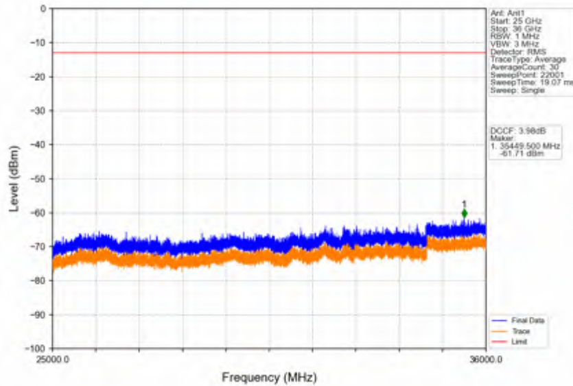
Band42c_15MHz_64QAM_HCH_3592.5MHz_RB_1_74_NTNV
