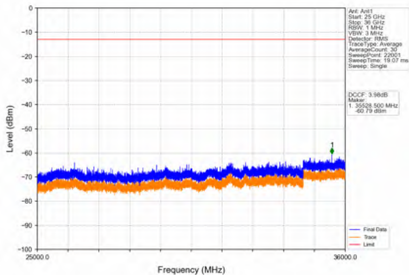
Band42c_5MHz_64QAM_MCH_3575MHz_RB_1_0_NTV
