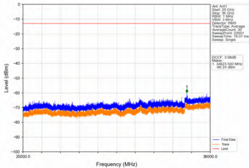
Band42c_15MHz_16QAM_HCH_3592.5MHz_RB_1_0_NTNV
