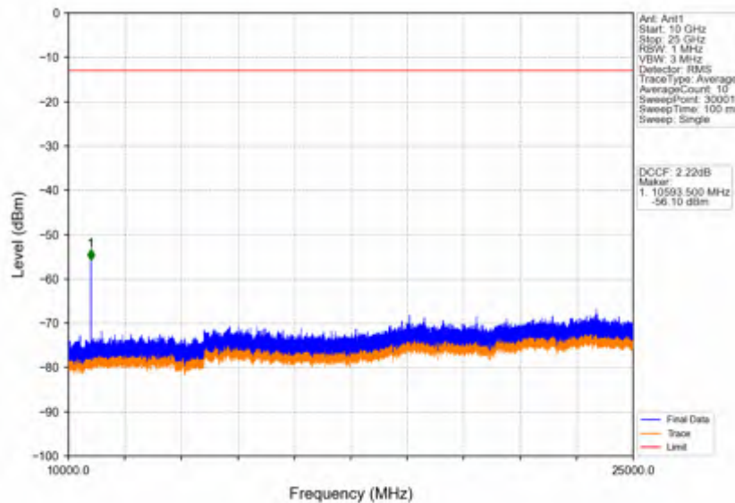
Band42a_20MHz_QPSK_HCH_3540MHz_RB_1_0_NTV
