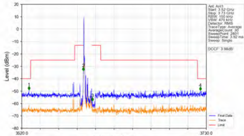
Band42c_10MHz_64QAM_HCH_3595MHz_RB_1_49_NTNV
