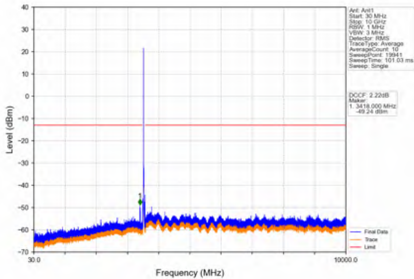
Band42a_20MHz_QPSK_HCH_3540MHz_RB_1_0_NTV
