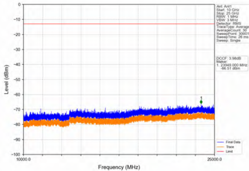
Band42c_15MHz_QPSK_MCH_3575MHz_RB_1_0_NTV
