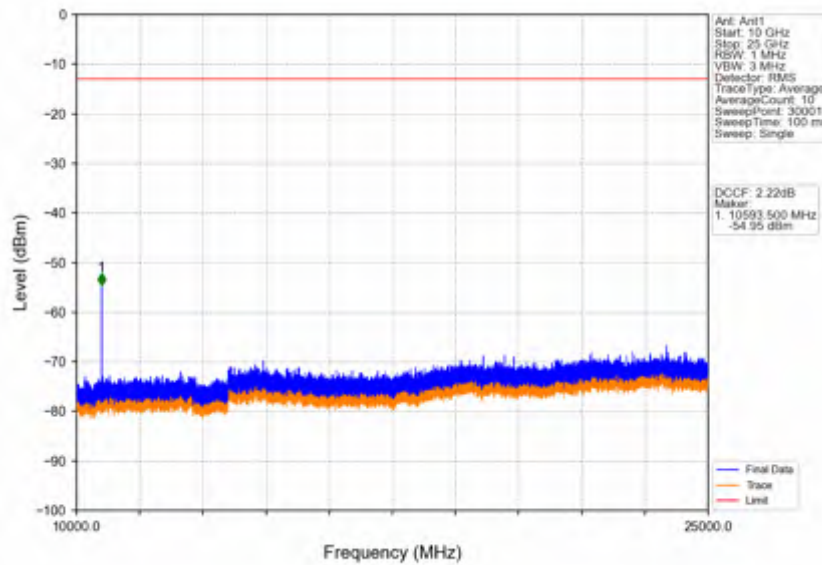
Band42a_20MHz_64QAM_HCH_3540MHz_RB_1_0_NTNV
