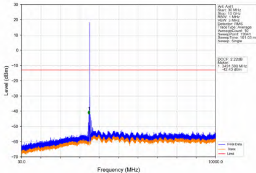
Band42a_15MHz_256QAM_HCH_3542.5MHz_RB_1_0_NTNV
