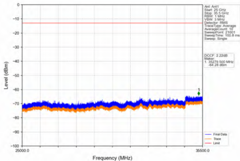
Band42a_20MHz_256QAM_HCH_3540MHz_RB_1_0_NTNV
