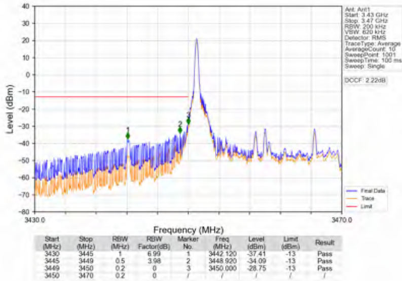
Band42a_20MHz_64QAM_LCH_3460MHz_RB_100_0_NTNV
