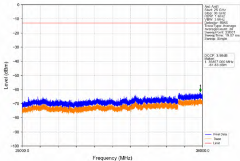
Band42c_15MHz_256QAM_HCH_3592.5MHz_RB_1_0_NTNV
