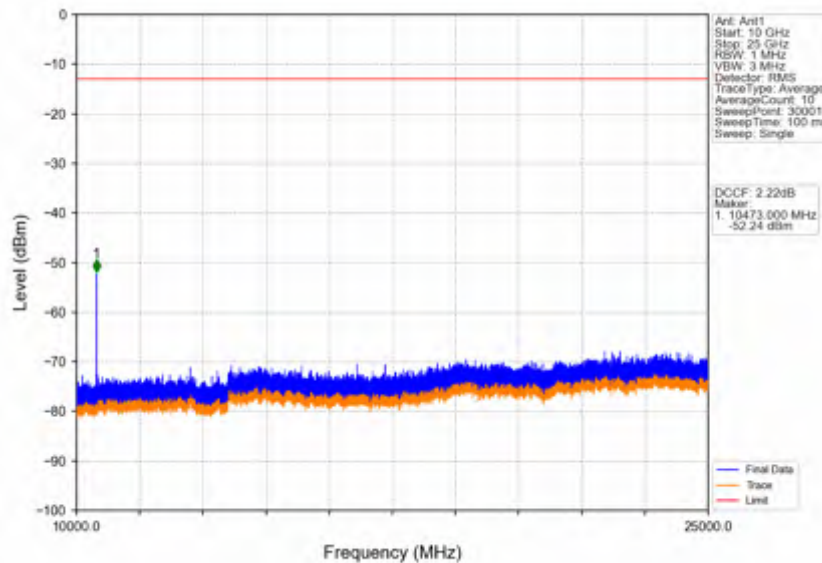
Band42a_20MHz_16QAM_MCH_3500MHz_RB_1_0_NTNV
