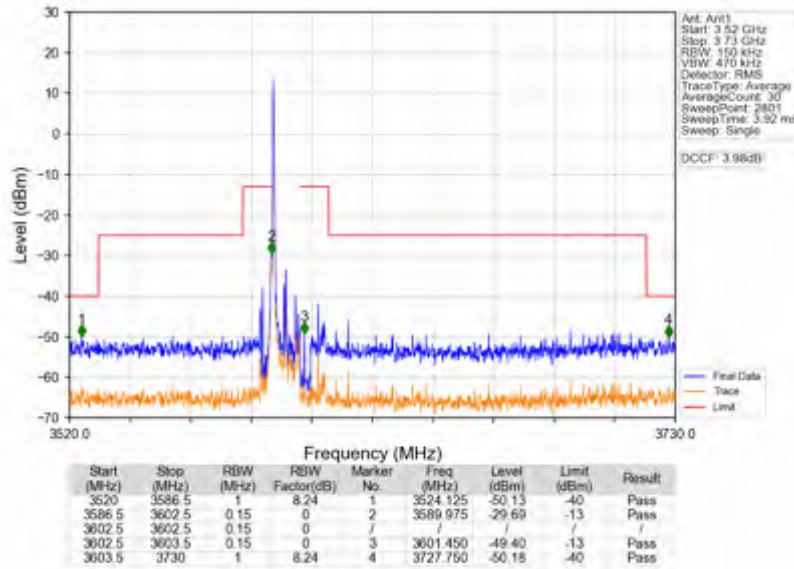
Band42c_10MHz_16QAM_HCH_3595MHz_RB_50_0_NTNV
