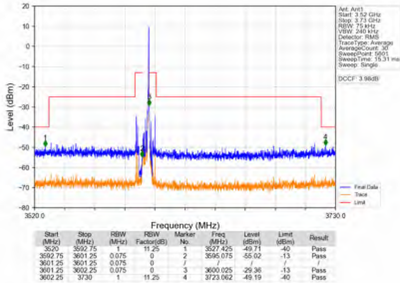
Band42c_5MHz_256QAM_HCH_3597.5MHz_RB_25_0_NTNV
