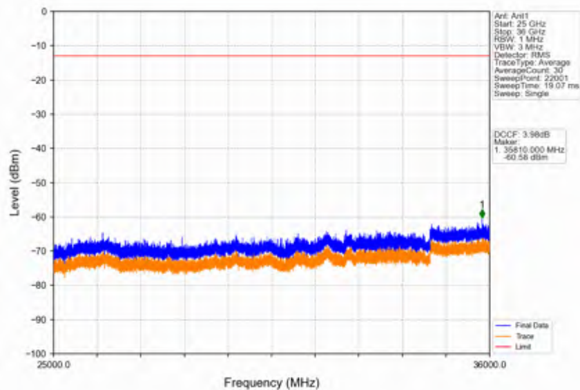
Band42c_10MHz_256QAM_HCH_3595MHz_RB_1_0_NTNV
