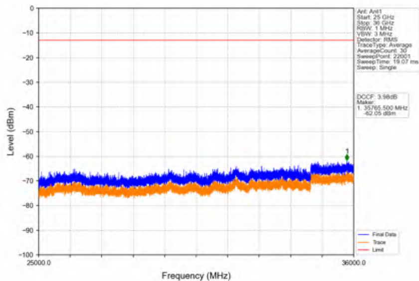
Band42c_15MHz_64QAM_LCH_3557.5MHz_RB_1_0_NTNV
