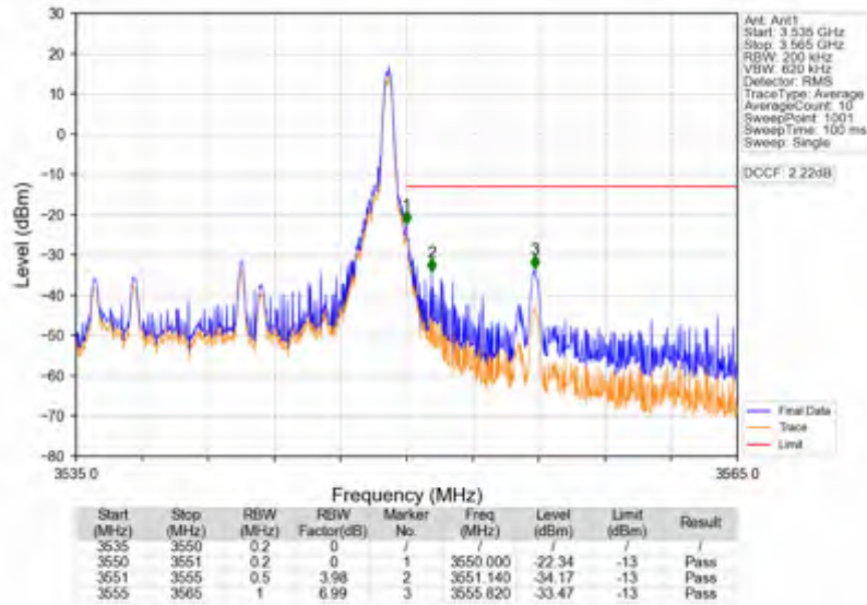
Band42a_15MHz_256QAM_HCH_3542.5MHz_RB_75_0_NTNV
