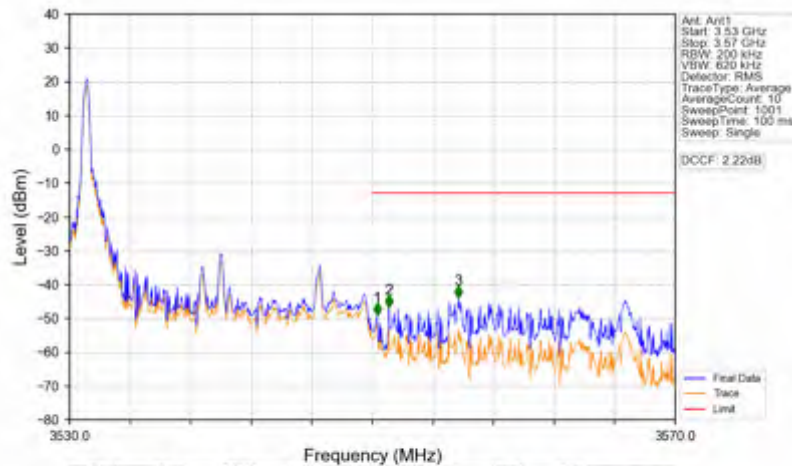
Band42a_20MHz_64QAM_HCH_3540MHz_RB_1_99_NTNV
