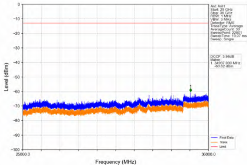
Band42c_10MHz_64QAM_LCH_3555MHz_RB_1_0_NTNV
