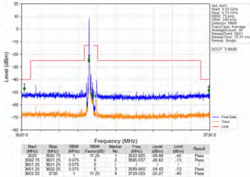
Band42c_5MHz_16QAM_HCH_3597.5MHz_RB_25_0_NTNV
