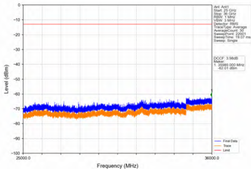
Band42c_5MHz_QPSK_MCH_3575MHz_RB_1_0_NTNV
