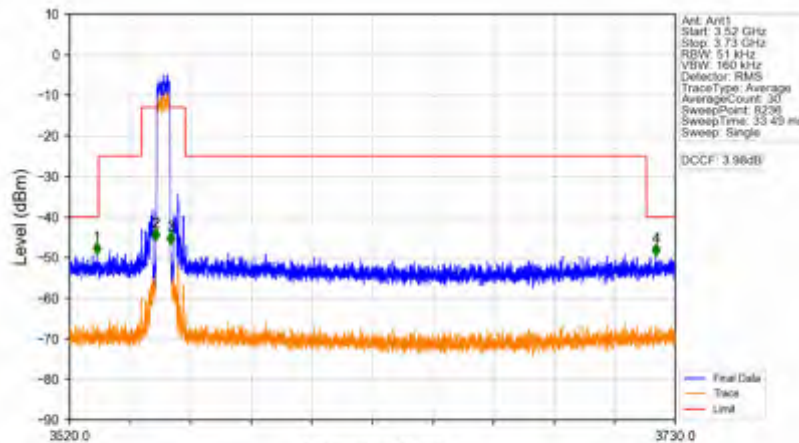
Band42c_5MHz_16QAM_LCH_3552.5MHz_RB_25_0_NTNV
