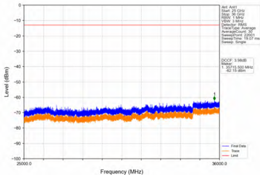
Band42c_5MHz_QPSK_LCH_3552.5MHz_RB_1_0_NTV
