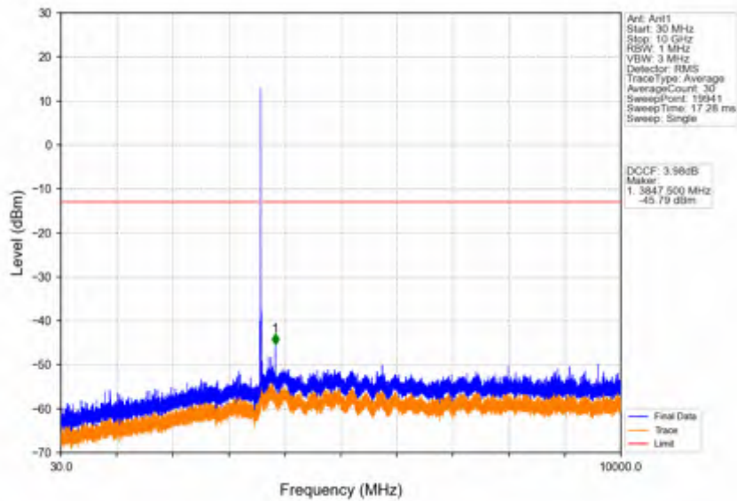
Band42c_15MHz_256QAM_HCH_3592.5MHz_RB_1_0_NTNV
