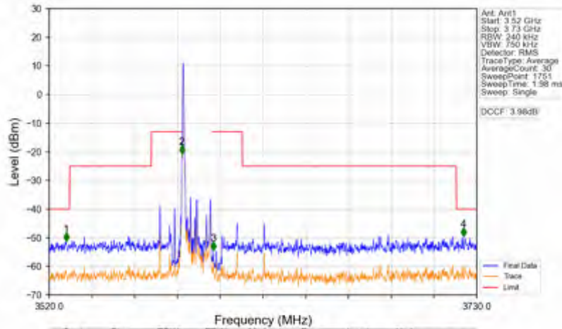
Band42c_15MHz_64QAM_HCH_3592.5MHz_RB_1_74_NTNV
