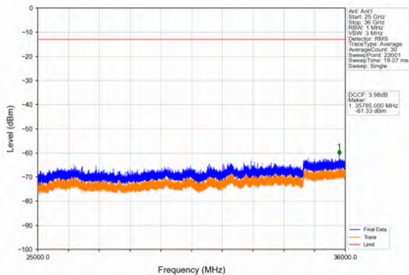
Band42c_10MHz_QPSK_MCH_3575MHz_RB_1_0_NTV
