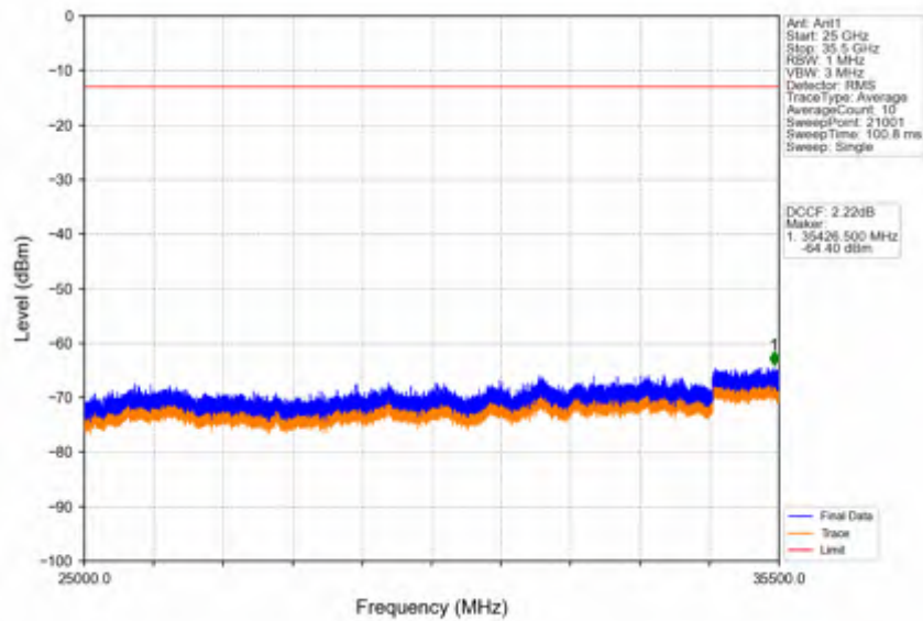
Band42a_20MHz_16QAM_HCH_3540MHz_RB_1_0_NTNV
