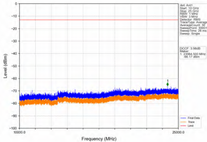
Band42c_20MHz_256QAM_HCH_3590MHz_RB_1_0_NTNV
