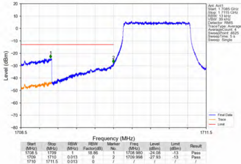
Band66_1.4MHz_QPSK_LCH_1710.7MHz_RB_6_0_NTNV
