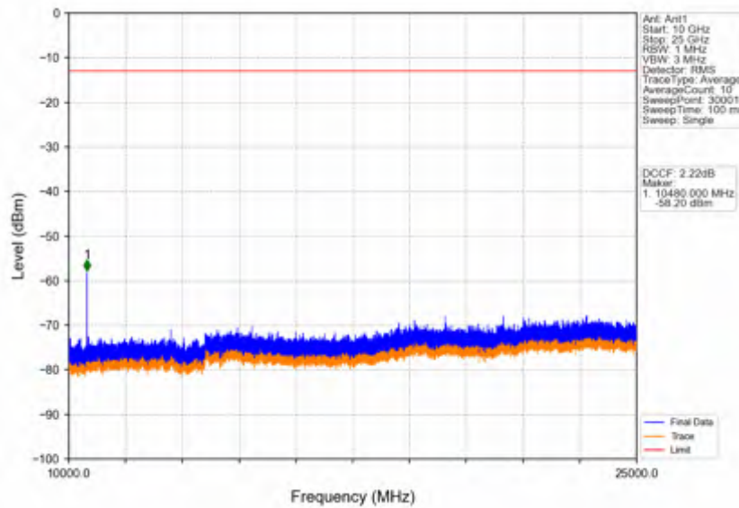
Band42a_15MHz_256QAM_MCH_3500MHz_RB_1_0_NTNV
