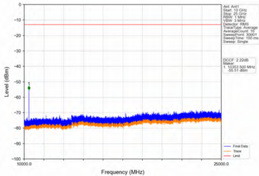
Band42a_20MHz_64QAM_LCH_3460MHz_RB_1_0_NTNV
