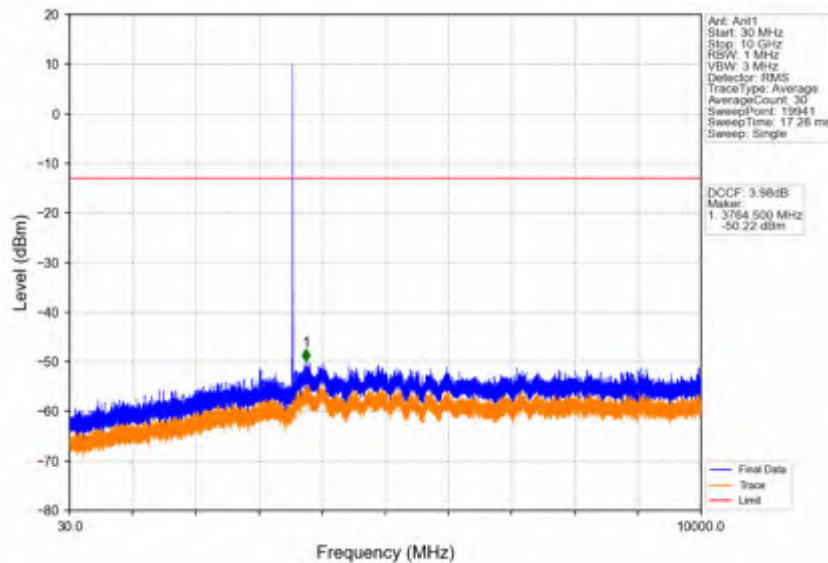
Band42c_10MHz_64QAM_LCH_3555MHz_RB_1_0_NTNV
