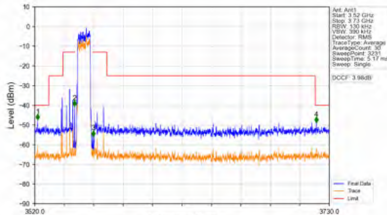
Band42c_10MHz_256QAM_LCH_3555MHz_RB_50_0_NTNV
