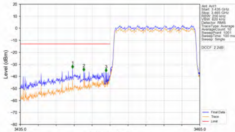
Band42a_15MHz_256QAM_LCH_3457.5MHz_RB_75_0_NTNV
