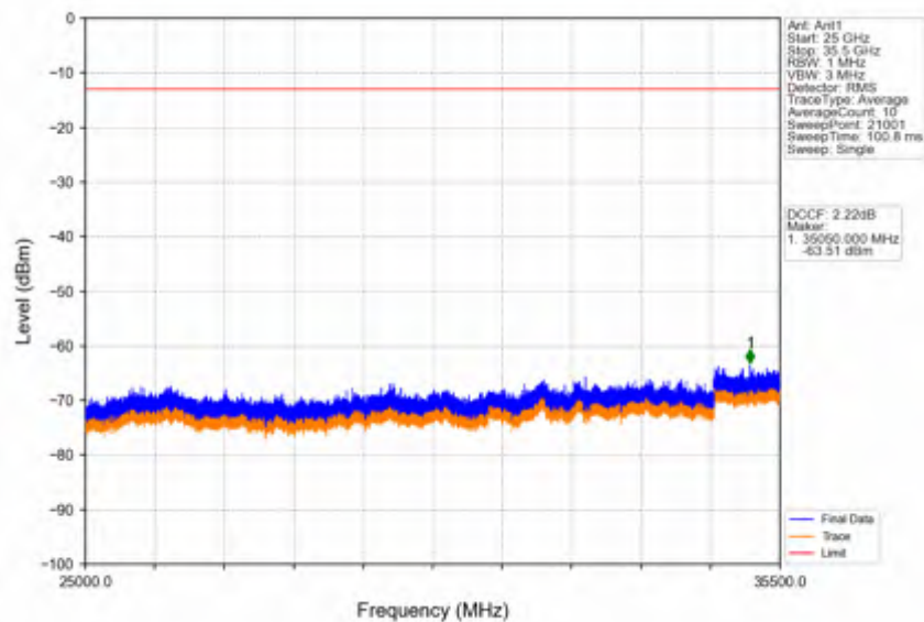
Band42a_15MHz_QPSK_LCH_3457.5MHz_RB_1_0_NTNV
