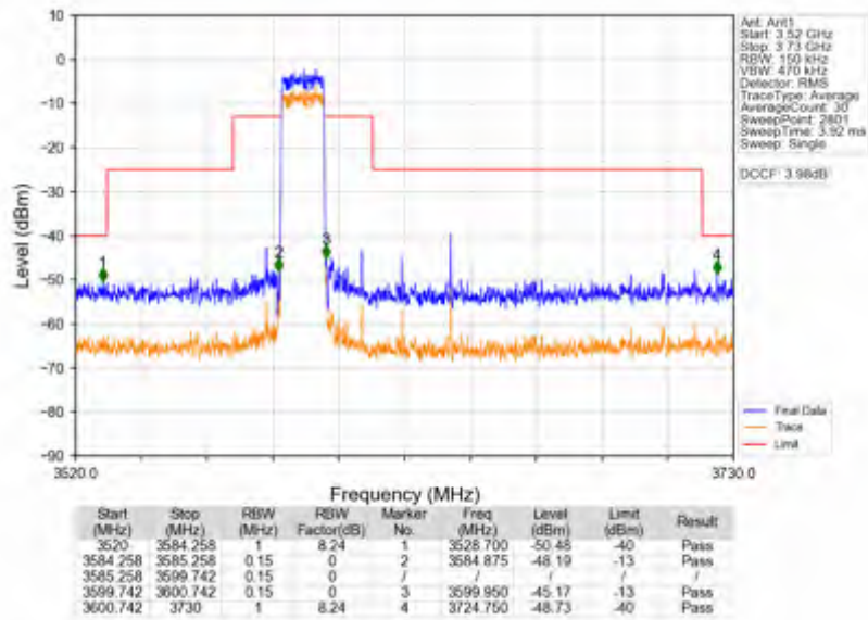
Band42c_15MHz_256QAM_HCH_3592.5MHz_RB_75_0_NTNV
