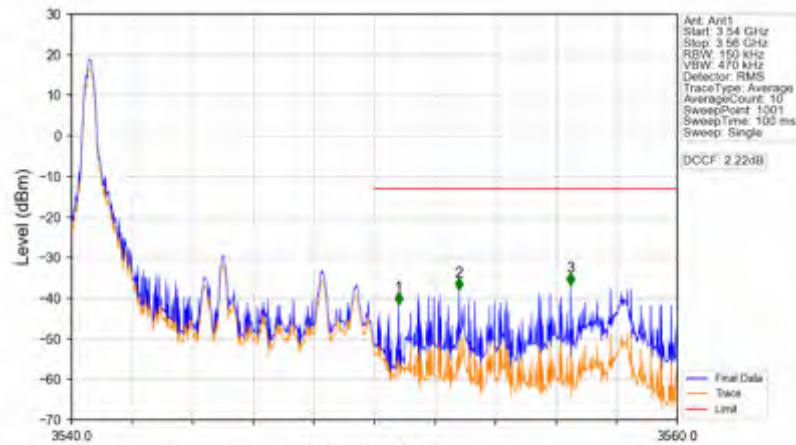
Band42a_10MHz_64QAM_HCH_3545MHz_RB_1_49_NTNV
