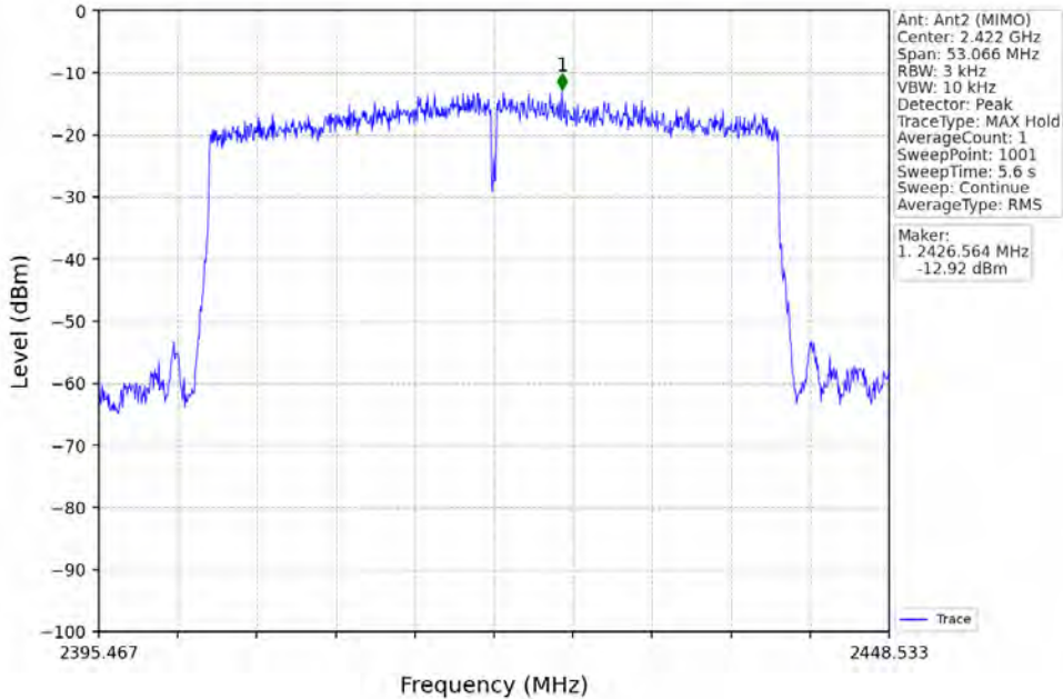
802.11ax(HEW40)_LCH_2422MHz_RU484_Left_MIMO_NTNV
