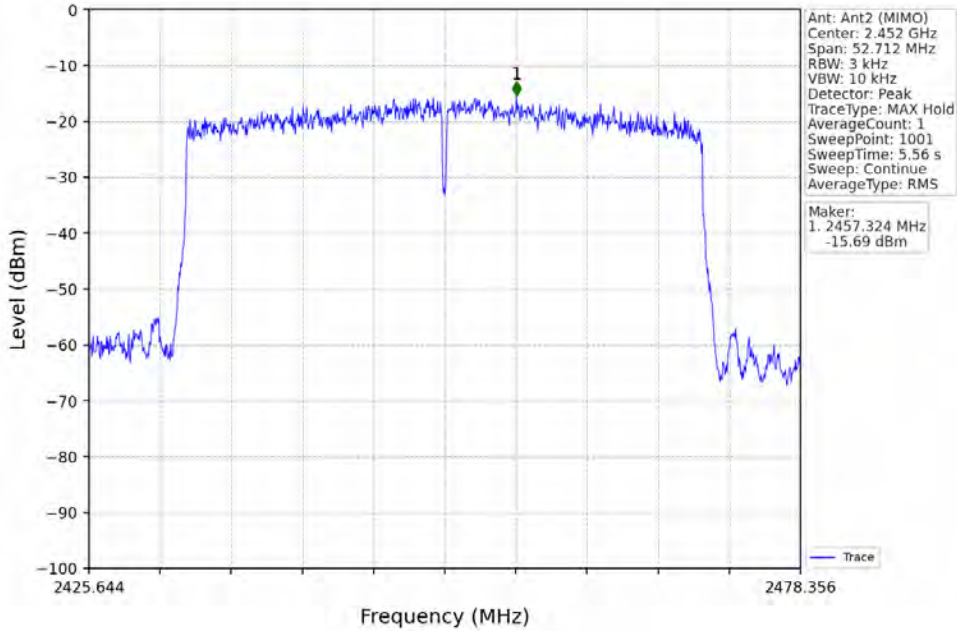
802.11ax(HEW40)_HCH_2452MHz_RU484_Left_MIMO_NTNV
