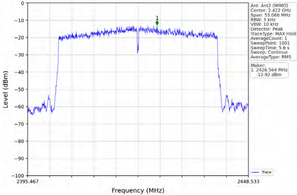
802.11ax(HEW40)_LCH_2422MHz_RU484_Left_MIMO_NTNV
