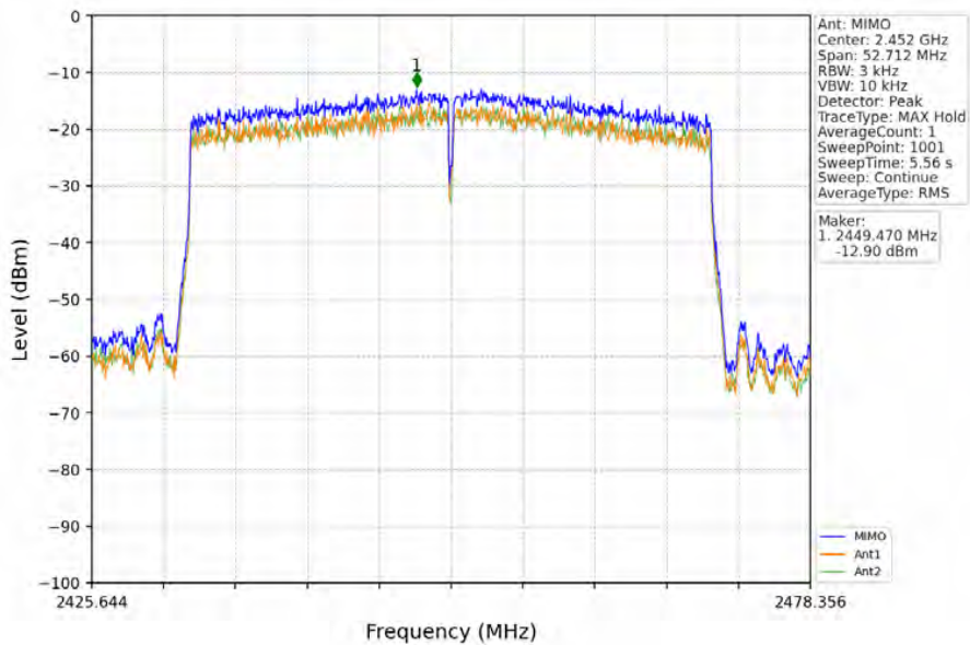
802.11ax(HEW40)_HCH_2452MHz_RU484_Left_MIMO_NTNV
