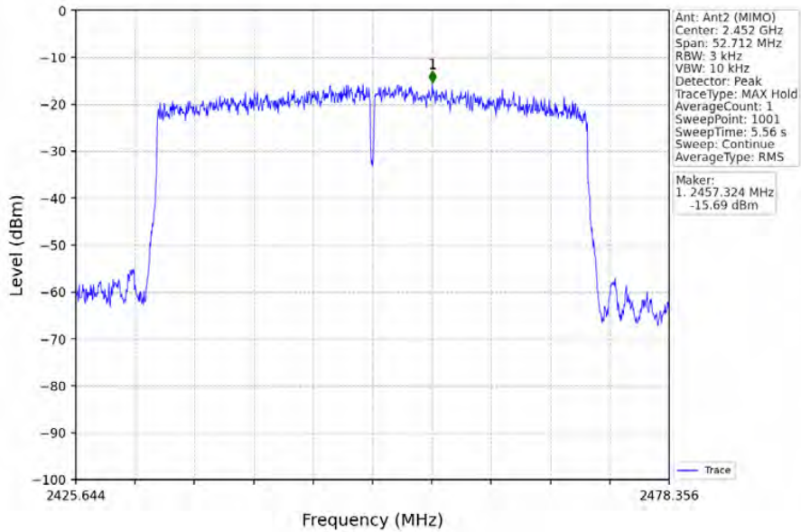
802.11ax(HEW40)_HCH_2452MHz_RU484_Left_MIMO_NTNV
