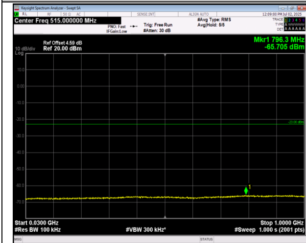
66-66-20MHz-5MHz-16QAM-16QAM-132072-132189-1R B#0-1RB#24-30~1000MHz-PASS
