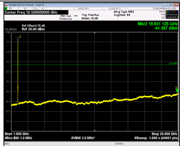
66-66-20MHz-5MHz-16QAM-16QAM-132522-132639-1RB# #0-ORB#0-1000~20000MHz-PASS
