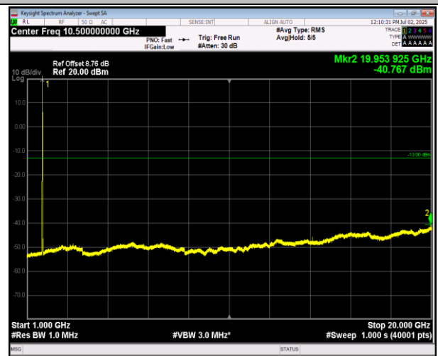
66-66-20MHz-5MHz-16QAM-16QAM-132072-132189-100R B#0-25RB#0-1000~20000MHz-PASS
