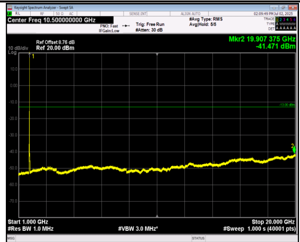
66-66-20MHz-20MHz-16QAM-16QAM-132323-132521-100RB#0-100RB#0-1000~20000MHz-PASS
