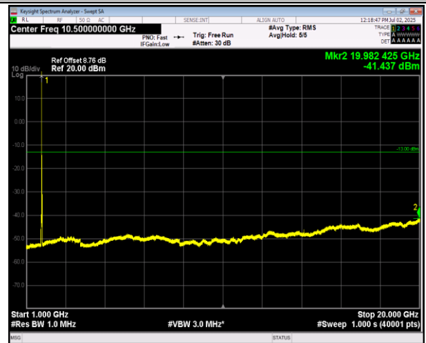
66-66-20MHz-5MHz-16QAM-16QAM-132397-132514-1RB #99-ORB#0-1000~20000MHz-PASS
