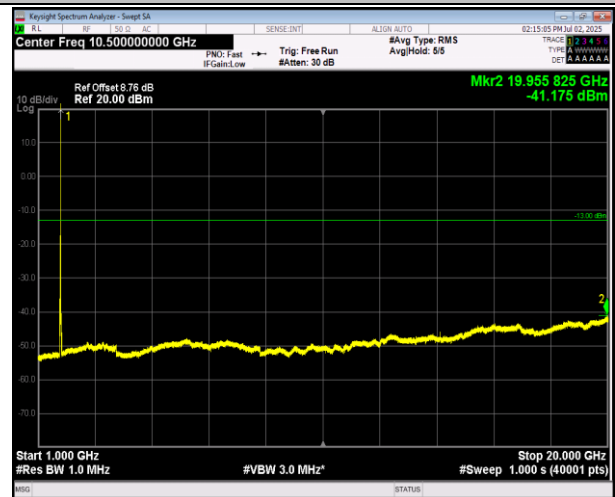
66-66-20MHz-20MHz-16QAM-16QAM-132374-132572-100 RB#0-100RB#0-1000~20000MHz-PASS
