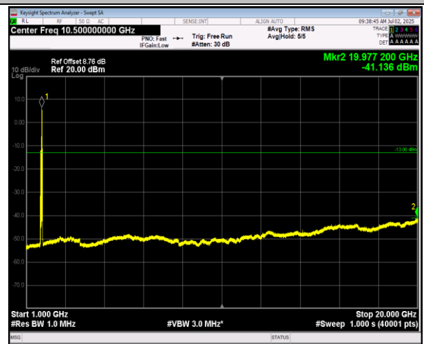
66-66-5MHz-20MHz-16QAM-16QAM-132455-132572-1RB #24-0RB#0-1000~20000MHz-PASS
