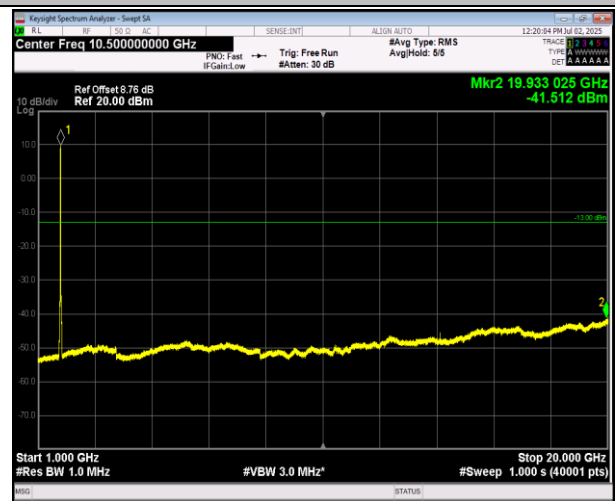
66-66-20MHz-5MHz-QPSK-QPSK-132522-132639-1RB#0- ORB#0-1000~20000MHz-PASS
