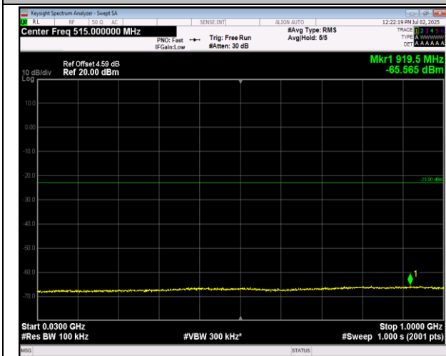
66-66-20MHz-5MHz-QPSK-QPSK-132522-132639-1RB# 0-1RB#24-30~1000MHz-PASS
