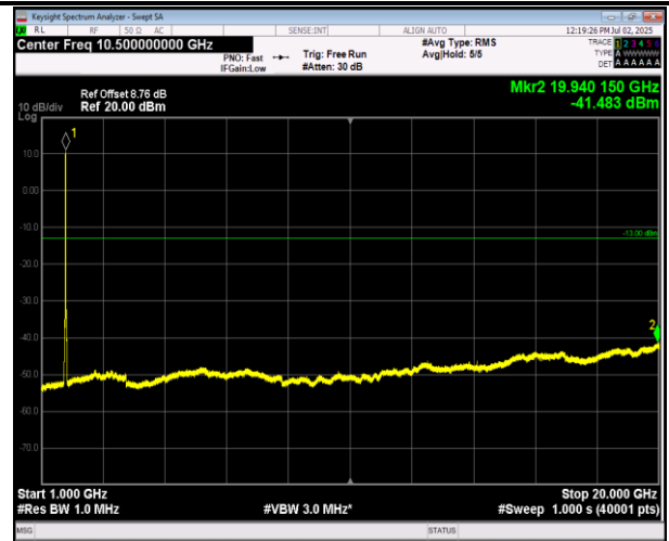
66-66-20MHz-5MHz-16QAM-16QAM-132397-132514-1RB #0-ORB#0-1000~20000MHz-PASS
