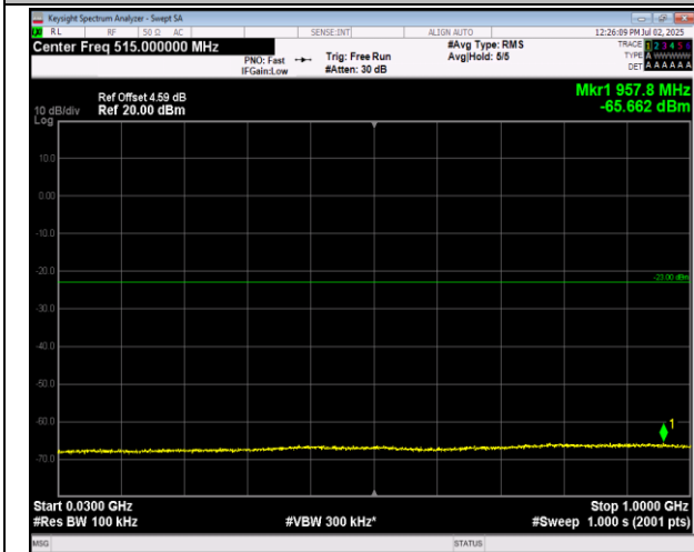
66-66-20MHz-5MHz-16QAM-16QAM-132522-132639-1RB# B#0-ORB#0-30~1000MHz-PASS
