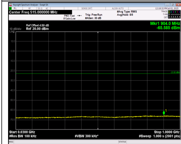
66-66-20MHz-5MHz-16QAM-16QAM-132397-132514-1R B#99-ORB#0-30~1000MHz-PASS
