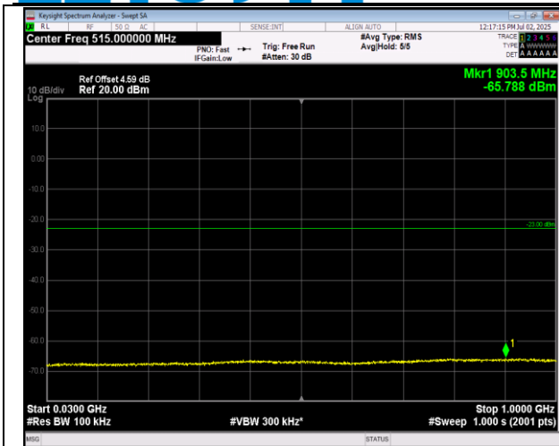
66-66-20MHz-5MHz-16QAM-16QAM-132397-132514-10 ORB#0-25RB#0-30~1000MHz-PASS
