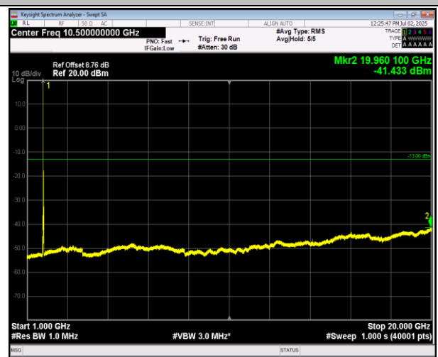
66-66-20MHz-5MHz-16QAM-16QAM-132522-132639-1RB #99-0RB#0-1000~20000MHz-PASS
