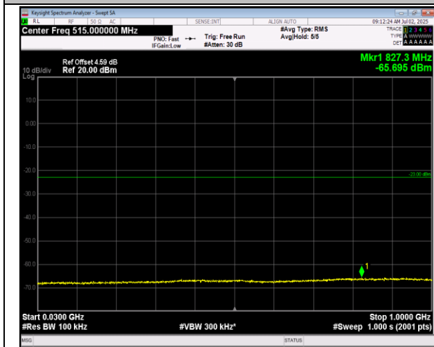
66-66-5MHz-20MHz-16QAM-16QAM-132005-132122-1RB B#0-0RB#0-30~1000MHz-PASS
