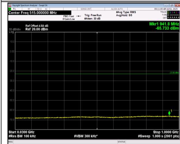
66-66-5MHz-20MHz-QPSK-QPSK-132005-132122-1RB# 24-0RB#0-30~1000MHz-PASS
