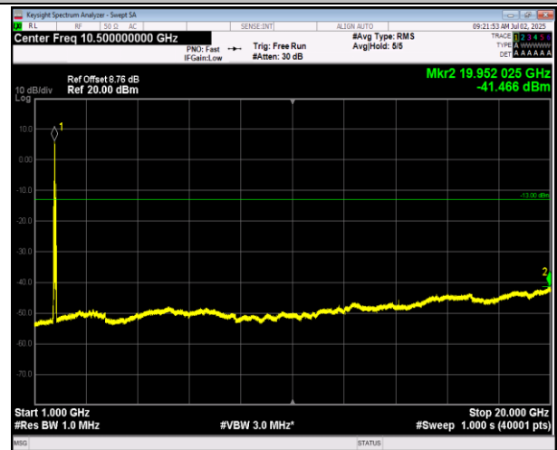
66-66-5MHz-20MHz-16QAM-16QAM-132330-132447-1RB #24-ORB#0-1000~20000MHz-PASS
