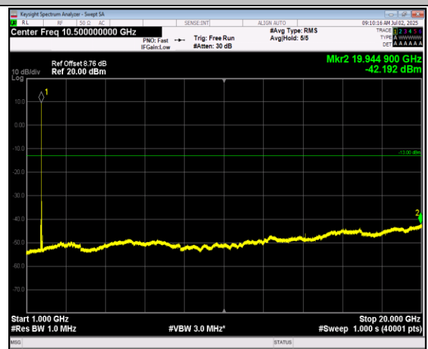
66-66-5MHz-20MHz-16QAM-16QAM-132005-132122-25R B#0-100RB#0-1000~20000MHz-PASS
