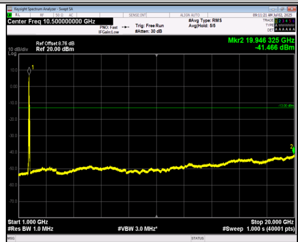
66-66-5MHz-20MHz-QPSK-QPSK-132005-132122-1RB#24 -0RB#0-1000~20000MHz-PASS
