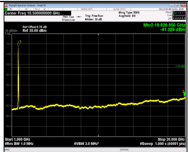
66-66-5MHz-20MHz-16QAM-16QAM-132005-132122-1RB #24-ORB#0-1000~20000MHz-PASS
