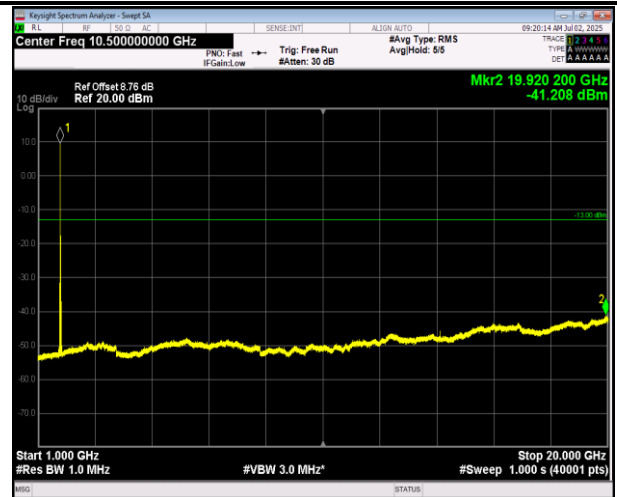
66-66-5MHz-20MHz-16QAM-16QAM-132330-132447-25R B#0-100RB#0-1000~20000MHz-PASS
