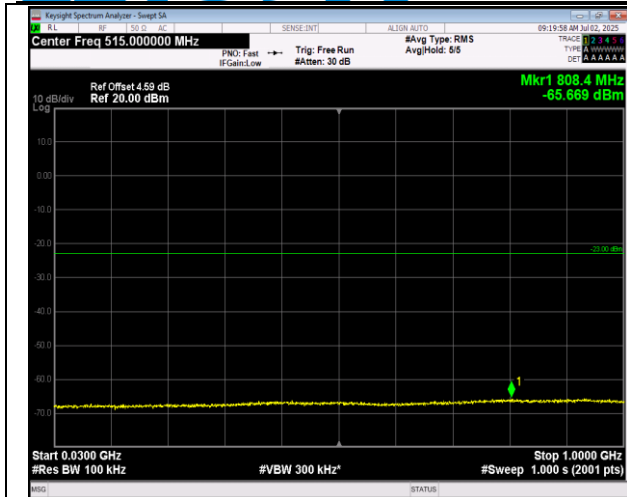
66-66-5MHz-20MHz-16QAM-16QAM-132330-132447-25 RB#0-100RB#0-30~1000MHz-PASS
