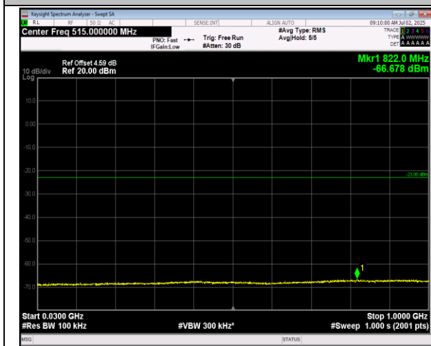
66-66-5MHz-20MHz-16QAM-16QAM-132005-132122-25 RB#0-100RB#0-30~1000MHz-PASS
