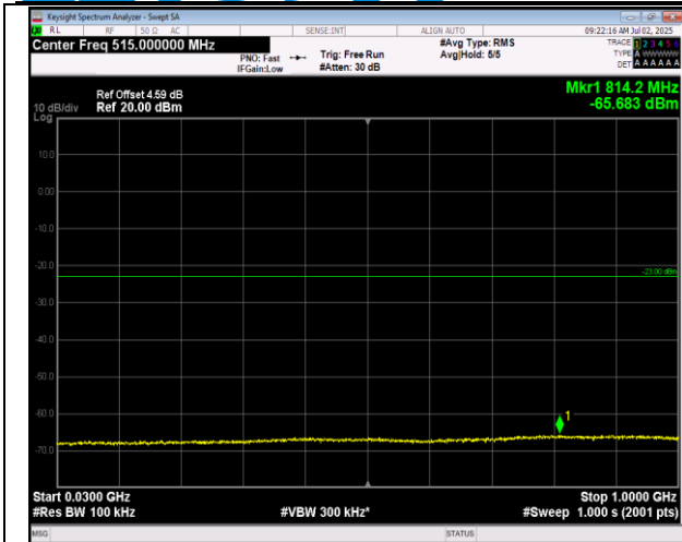
66-66-5MHz-20MHz-16QAM-16QAM-132330-132447-1R B#0-ORB#0-30~1000MHz-PASS
