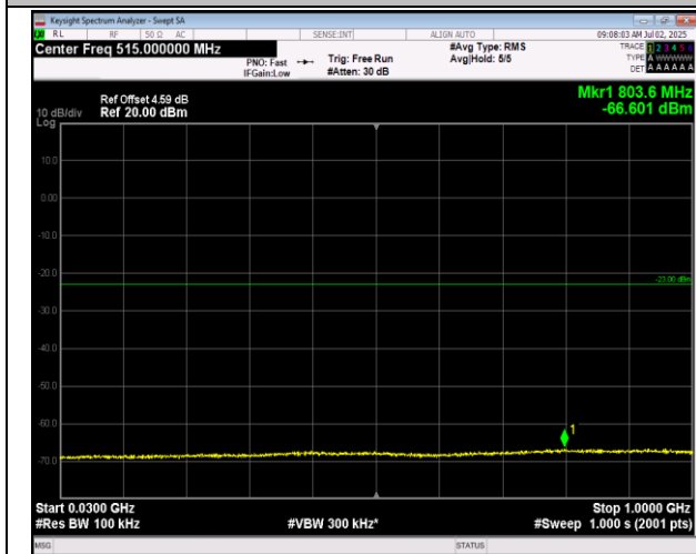
66-66-5MHz-20MHz-16QAM-16QAM-132005-132122-1RB B#0-1RB#99-30~1000MHz-PASS
