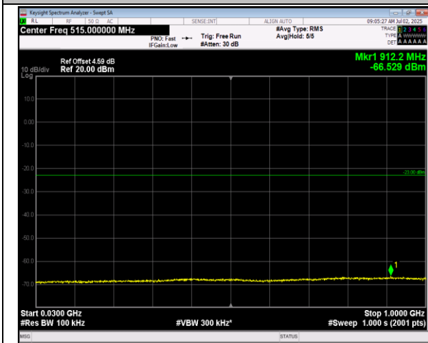
66-66-5MHz-20MHz-QPSK-QPSK-132005-132122-1RB# 0-1RB#99-30~1000MHz-PASS
