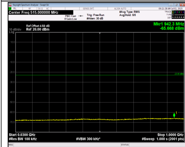
66-66-5MHz-20MHz-16QAM-16QAM-132330-132447-1R B#24-ORB#0-30~1000MHz-PASS
