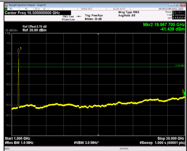
66-66-5MHz-20MHz-16QAM-16QAM-132455-132572-1RB #0-ORB#0-1000~20000MHz-PASS
