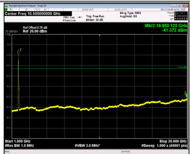
66-66-5MHz-20MHz-QPSK-QPSK-132330-132447-1RB#0- ORB#0-1000~20000MHz-PASS
