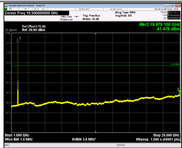
66-66-5MHz-20MHz-16QAM-16QAM-132330-132447-1RB #0-1RB#99-1000~20000MHz-PASS
