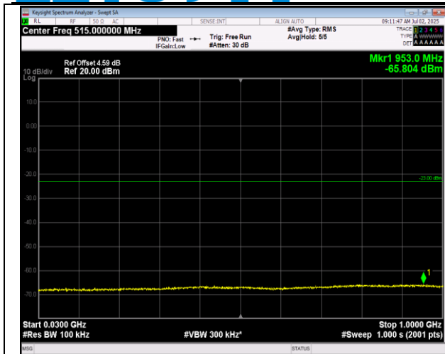
66-66-5MHz-20MHz-16QAM-16QAM-132005-132122-1R B#24-ORB#0-30~1000MHz-PASS
