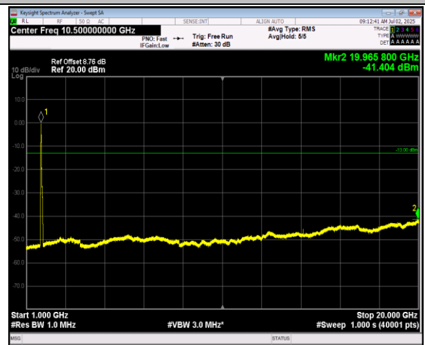
66-66-5MHz-20MHz-16QAM-16QAM-132005-132122-1RB #0-0RB#0-1000~20000MHz-PASS
