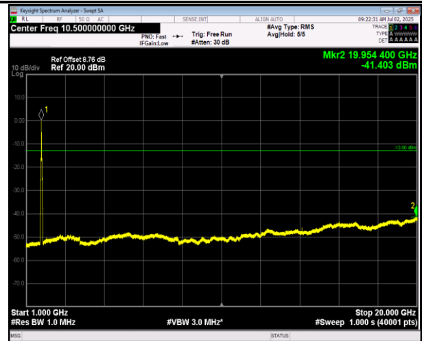
66-66-5MHz-20MHz-16QAM-16QAM-132330-132447-1RB #0-ORB#0-1000~20000MHz-PASS
