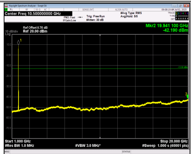
66-66-5MHz-20MHz-16QAM-16QAM-132005-132122-1RB #0-1RB#99-1000~20000MHz-PASS
