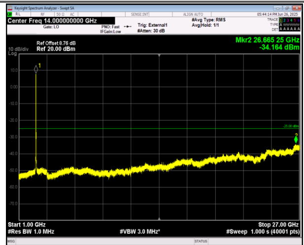
38-38-20MHz-20MHz-16QAM-16QAM-37952-38150-1RB# 0-0RB#0-1000~27000MHz-PASS
