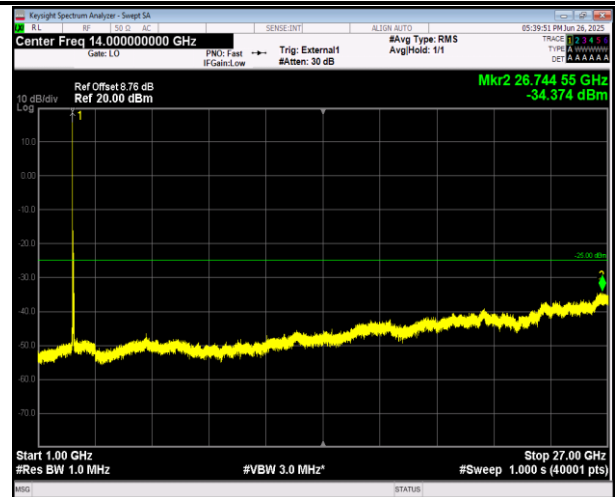
38-38-20MHz-20MHz-16QAM-16QAM-37952-38150-1RB# 0-1RB#99-1000~27000MHz-PASS
