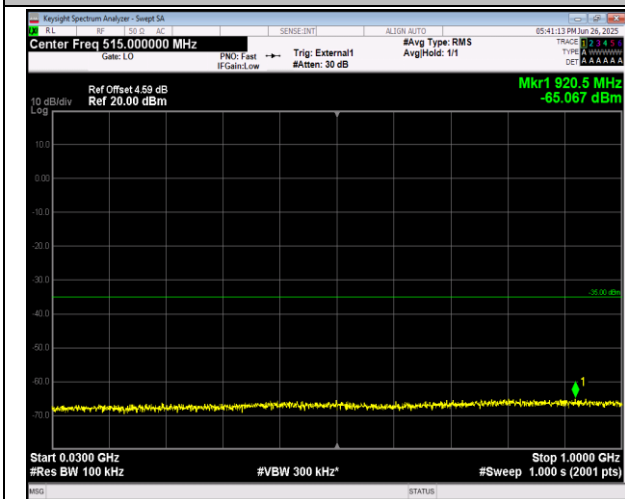
38-38-20MHz-20MHz-16QAM-16QAM-37952-38150-100 RB#0-100RB#0-30~1000MHz-PASS
