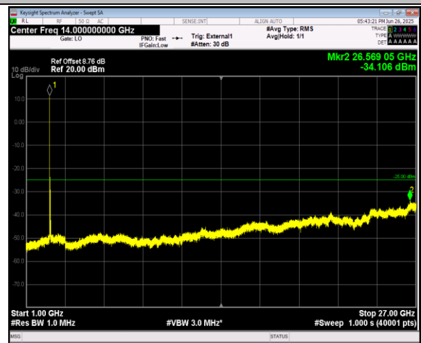
38-38-20MHz-20MHz-16QAM-16QAM-37952-38150-1RB# 99-0RB#0-1000~27000MHz-PASS
