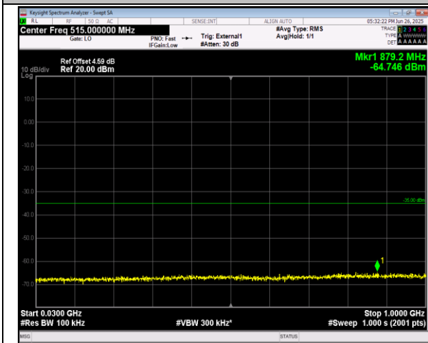
38-38-20MHz-20MHz-16QAM-16QAM-37901-38099-1RB #0-1RB#99-30~1000MHz-PASS
