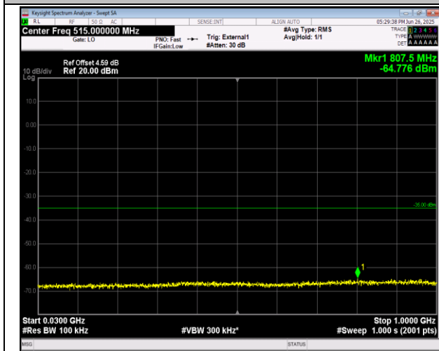
38-38-20MHz-20MHz-16QAM-16QAM-37850-38048-1RB #0-0RB#0-30~1000MHz-PASS
