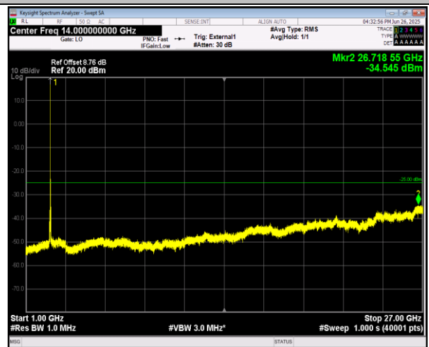
38-38-15MHz-15MHz-QPSK-QPSK-38025-38175-1RB#0-1 RB#74-1000~27000MHz-PASS
