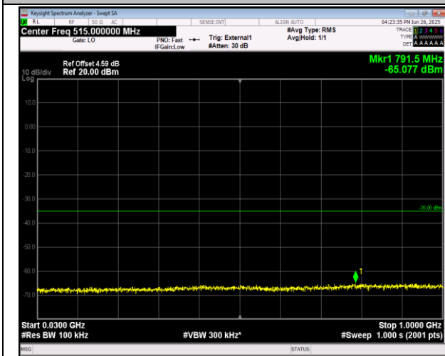
38-38-15MHz-15MHz-16QAM-16QAM-37825-37975-1RB #0-0RB#0-30~1000MHz-PASS
