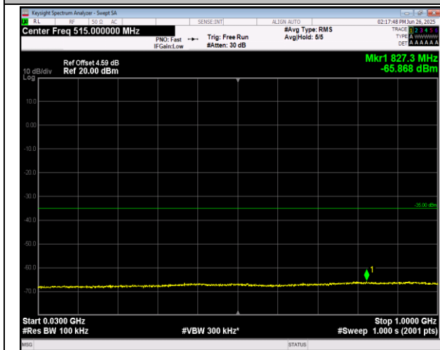
7-7-20MHz-20MHz-16QAM-16QAM-21152-21350-100RB #0-100RB#0-30~1000MHz-PASS
