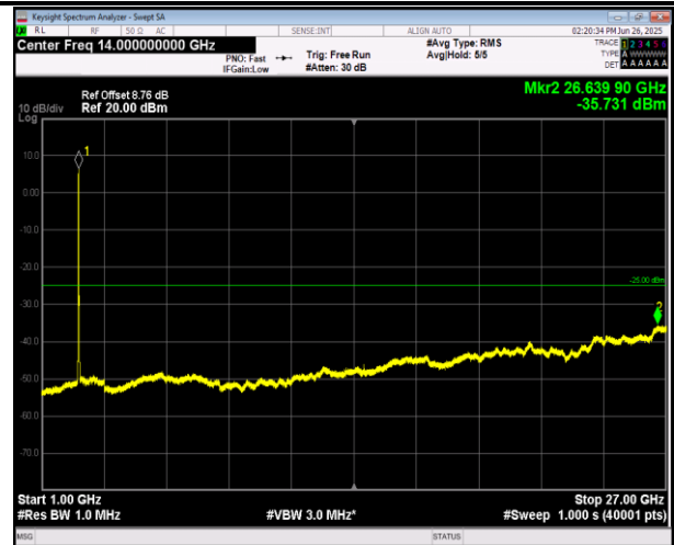
38-38-15MHz-15MHz-QPSK-QPSK-37825-37975-1RB#0-0 RB#0-1000~27000MHz-PASS
