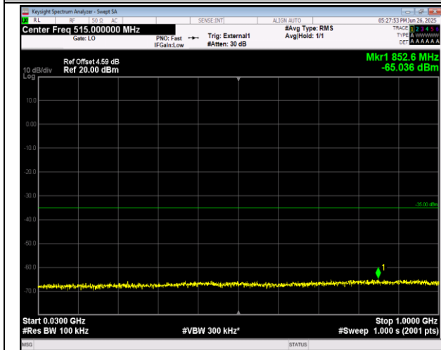
38-38-20MHz-20MHz-QPSK-QPSK-37850-38048-1RB#9-9-ORB#0-30~1000MHz-PASS
