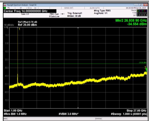
38-38-15MHz-15MHz-QPSK-QPSK-38025-38175-75RB#0- 75RB#0-1000~27000MHz-PASS
