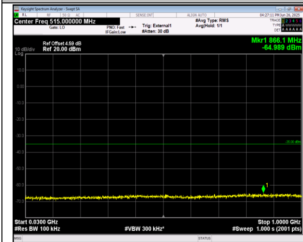
38-38-15MHz-15MHz-QPSK-QPSK-37925-38075-75RB#0-75RB#0-30~1000MHz-PASS
