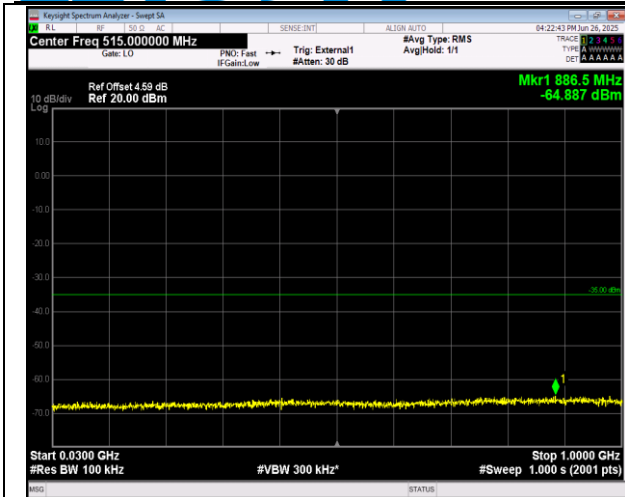
38-38-15MHz-15MHz-16QAM-16QAM-37825-37975-1RB #74-ORB#0-30~1000MHz-PASS
