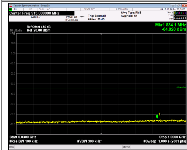
38-38-15MHz-15MHz-QPSK-QPSK-37825-37975-1RB#0- 1RB#74-30~1000MHz-PASS
