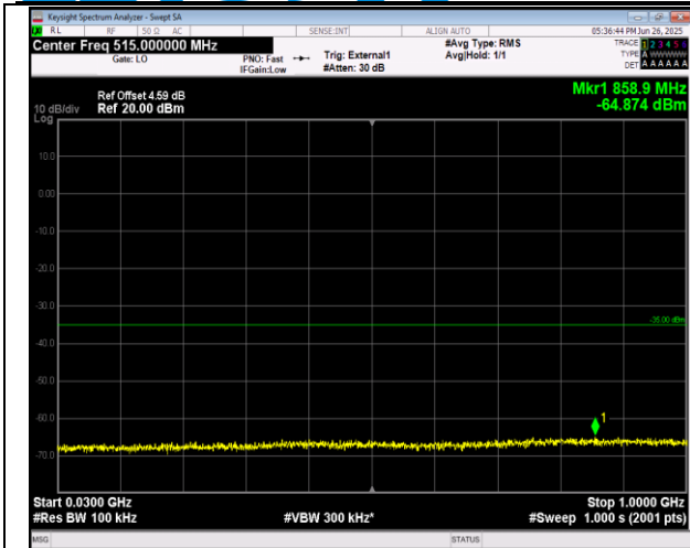
38-38-20MHz-20MHz-16QAM-16QAM-37901-38099-1RB #0-ORB#0-30~1000MHz-PASS
