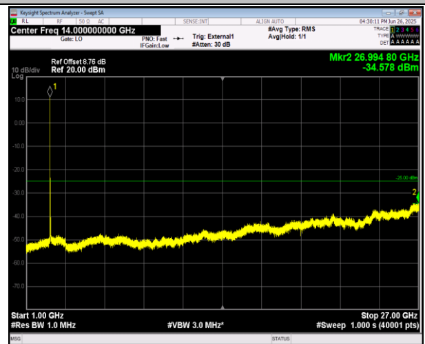
38-38-15MHz-15MHz-16QAM-16QAM-37925-38075-1RB# 74-ORB#0-1000~27000MHz-PASS
