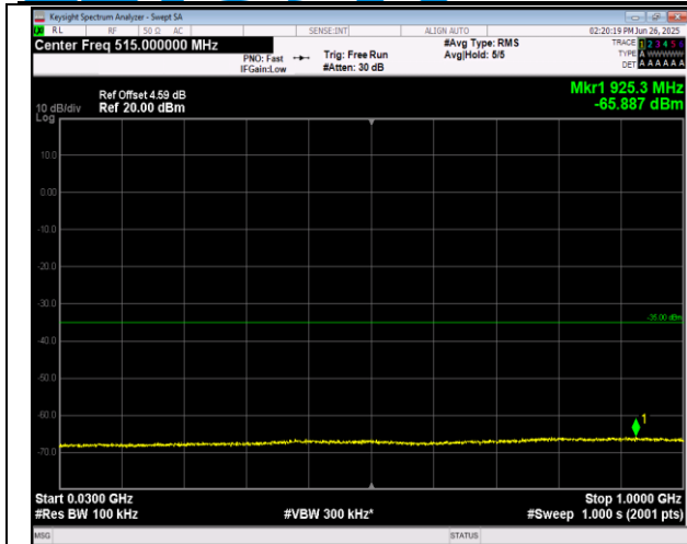
38-38-15MHz-15MHz-QPSK-QPSK-37825-37975-1RB#0- ORB#0-30~1000MHz-PASS
