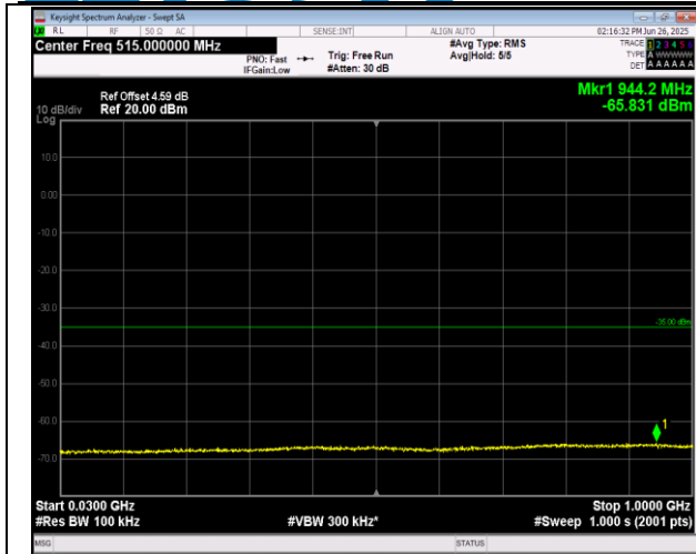
7-7-20MHz-20MHz-16QAM-16QAM-21152-21350-1RB#0 -1RB#99-30~1000MHz-PASS
