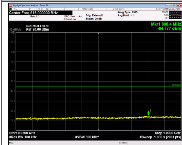
38-38-15MHz-15MHz-16QAM-16QAM-38025-38175-1RB #0-ORB#0-30~1000MHz-PASS
