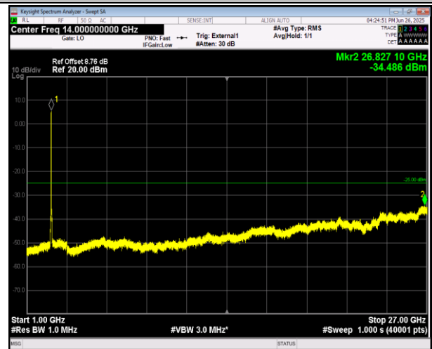
38-38-15MHz-15MHz-QPSK-QPSK-37925-38075-1RB#0-0 RB#0-1000~27000MHz-PASS
