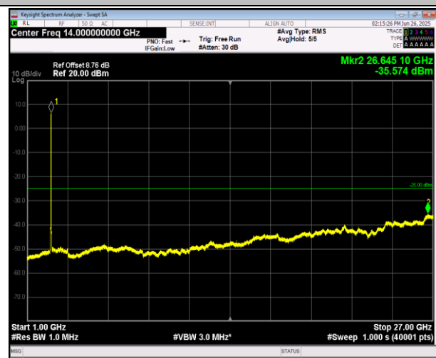
7-7-20MHz-20MHz-QPSK-QPSK-21152-21350-1RB#0-0RB #0-1000~27000MHz-PASS
