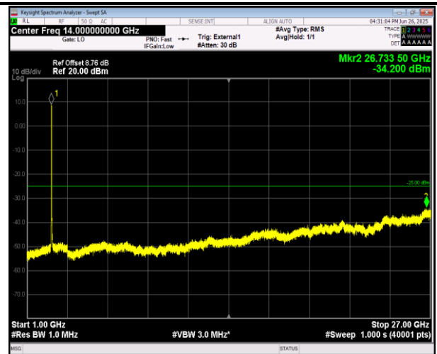
38-38-15MHz-15MHz-16QAM-16QAM-37925-38075-1RB# 0-ORB#0-1000~27000MHz-PASS
