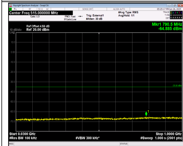
38-38-20MHz-20MHz-16QAM-16QAM-37850-38048-1RB #0-1RB#99-30~1000MHz-PASS
