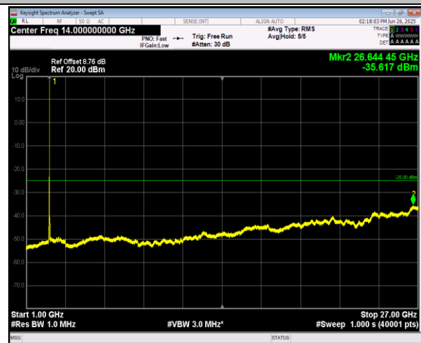
7-7-20MHz-20MHz-16QAM-16QAM-21152-21350-100RB#0 -100RB#0-1000~27000MHz-PASS
