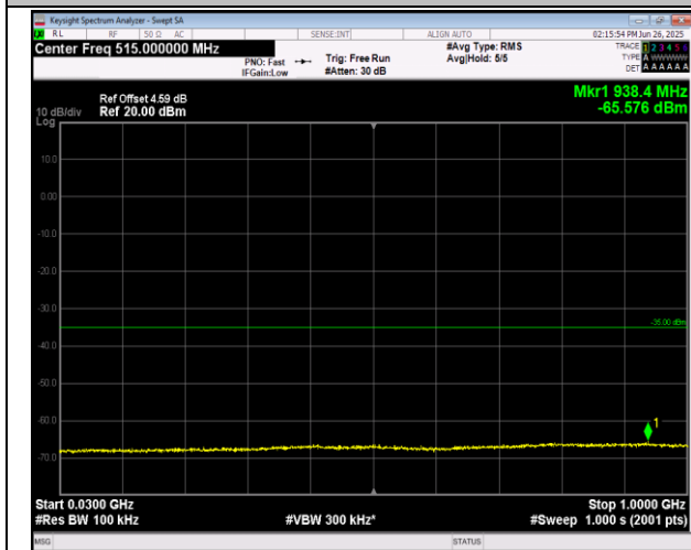
7-7-20MHz-20MHz-QPSK-QPSK-21152-21350-1RB#0-1 RB#99-30~1000MHz-PASS
