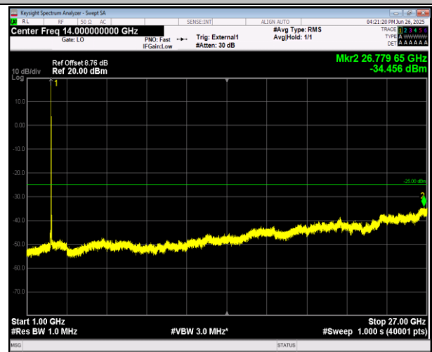
38-38-15MHz-15MHz-16QAM-16QAM-37825-37975-75RB #0-75RB#0-1000~27000MHz-PASS
