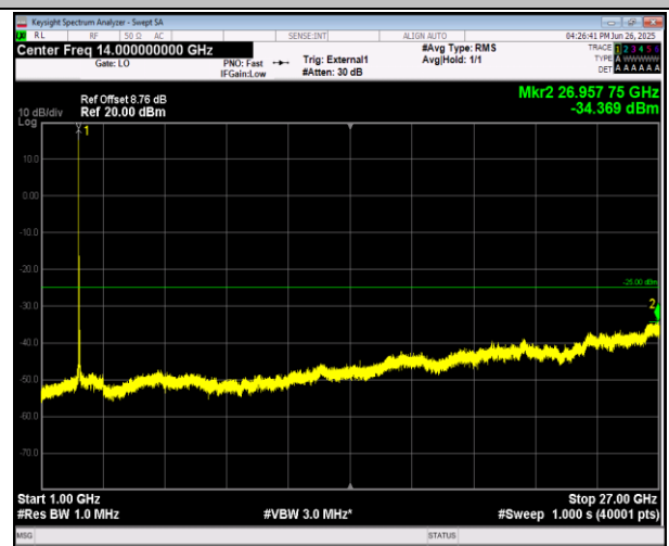
38-38-15MHz-15MHz-16QAM-16QAM-37925-38075-1RB# 0-1RB#74-1000~27000MHz-PASS
