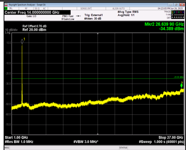
38-38-15MHz-15MHz-16QAM-16QAM-37825-37975-1RB# 74-ORB#0-1000~27000MHz-PASS
