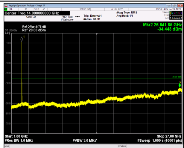
38-38-20MHz-20MHz-16QAM-16QAM-37901-38099-1RB# 99-ORB#0-1000~27000MHz-PASS
