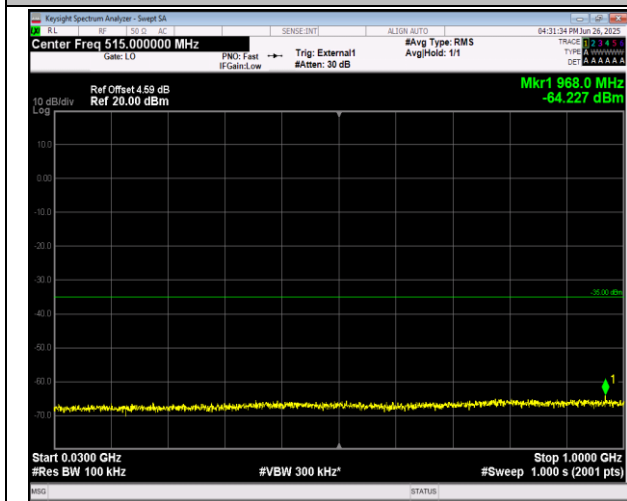
38-38-15MHz-15MHz-QPSK-QPSK-38025-38175-1RB#0- ORB#0-30~1000MHz-PASS
