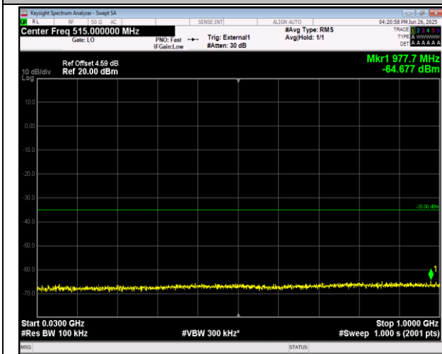
38-38-15MHz-15MHz-16QAM-16QAM-37825-37975-75R B#0-75RB#0-30~1000MHz-PASS
