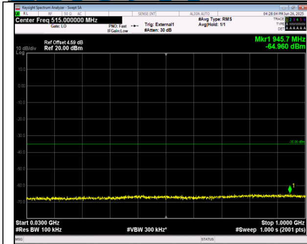
38-38-15MHz-15MHz-16QAM-16QAM-37925-38075-75R B#0-75RB#0-30~1000MHz-PASS
