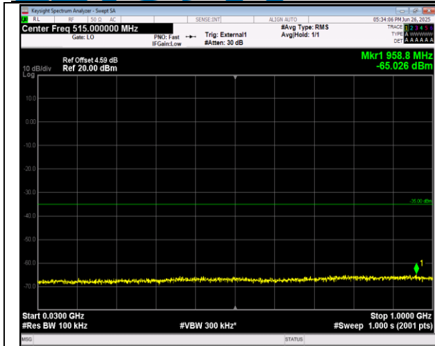
38-38-20MHz-20MHz-16QAM-16QAM-37901-38099-100 RB#0-100RB#0-30~1000MHz-PASS
