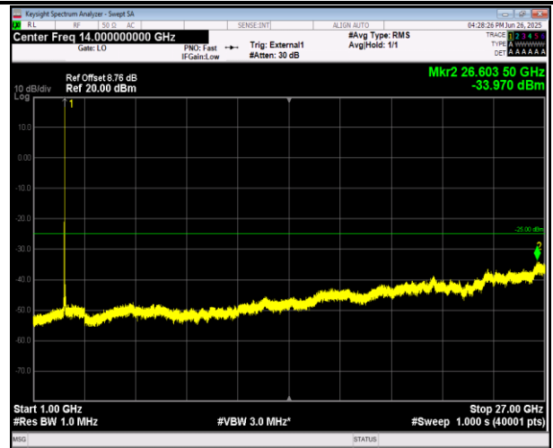
38-38-15MHz-15MHz-16QAM-16QAM-37925-38075-75RB #0-75RB#0-1000~27000MHz-PASS
