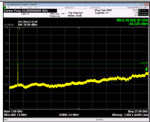
38-38-15MHz-15MHz-QPSK-QPSK-37825-37975-1RB#0-1 RB#74-1000~27000MHz-PASS
