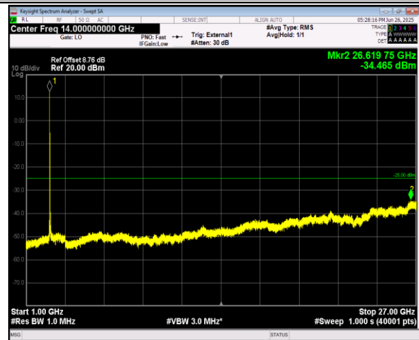
38-38-20MHz-20MHz-QPSK-QPSK-37850-38048-1RB#99-ORB#0-1000~27000MHz-PASS
