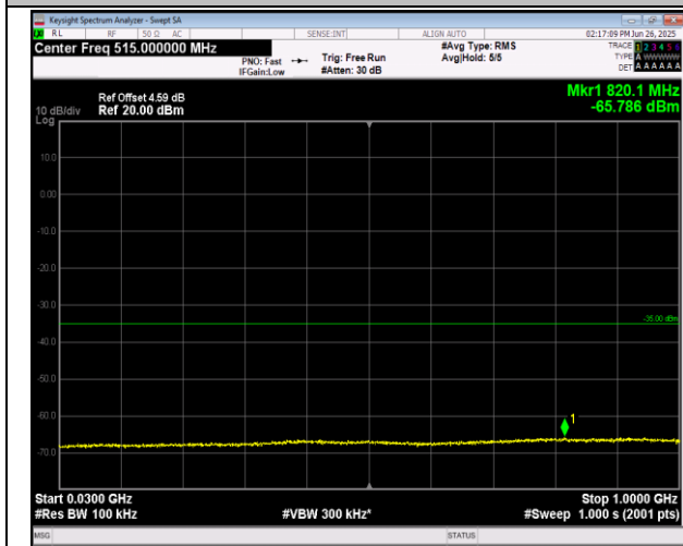
7-7-20MHz-20MHz-QPSK-QPSK-21152-21350-100RB#0- 100RB#0-30~1000MHz-PASS
