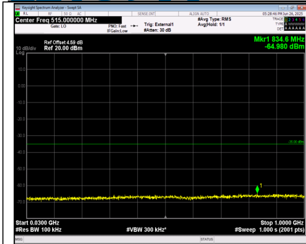
38-38-20MHz-20MHz-16QAM-16QAM-37850-38048-1RB #99-ORB#0-30~1000MHz-PASS
