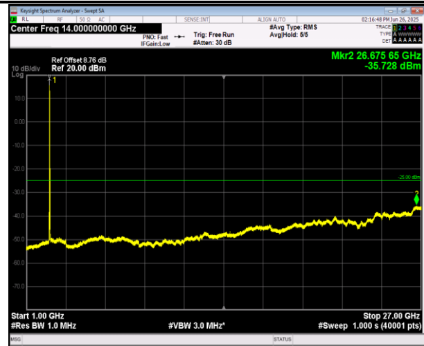
7-7-20MHz-20MHz-16QAM-16QAM-21152-21350-1RB#0-1 RB#99-1000~27000MHz-PASS
