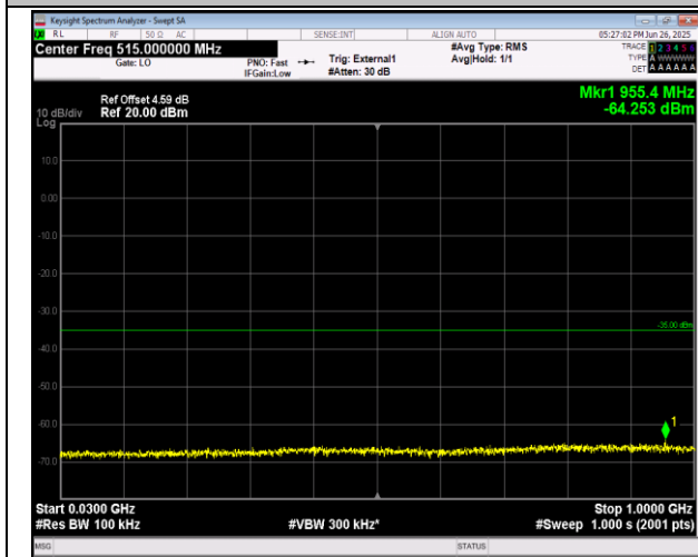
38-38-20MHz-20MHz-16QAM-16QAM-37850-38048-100 RB#0-100RB#0-30~1000MHz-PASS
