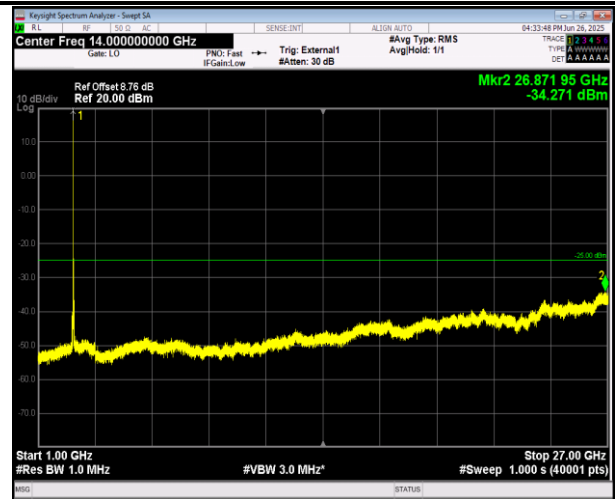
38-38-15MHz-15MHz-16QAM-16QAM-38025-38175-1RB# 0-1RB#74-1000~27000MHz-PASS
