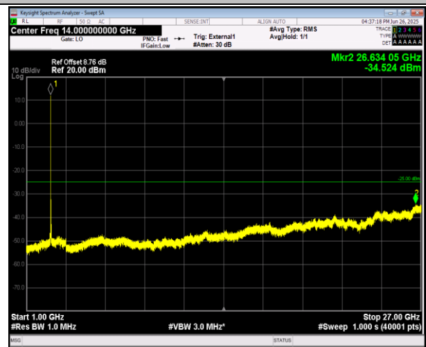
38-38-15MHz-15MHz-16QAM-16QAM-38025-38175-1RB# 74-0RB#0-1000~27000MHz-PASS
