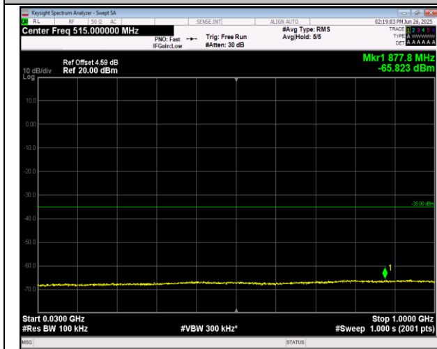
7-7-20MHz-20MHz-16QAM-16QAM-21152-21350-1RB#9 9-0RB#0-30~1000MHz-PASS
