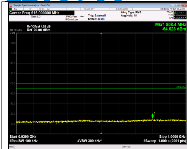
38-38-15MHz-15MHz-QPSK-QPSK-38025-38175-1RB#7 4-ORB#0-30~1000MHz-PASS
