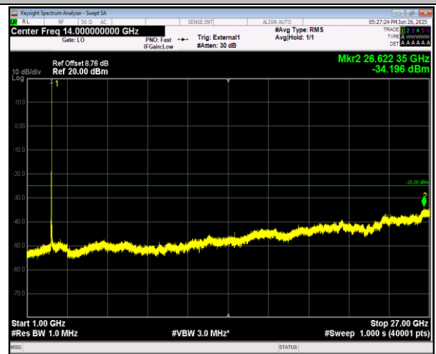
38-38-20MHz-20MHz-16QAM-16QAM-37850-38048-100R B#0-100RB#0-1000~27000MHz-PASS
