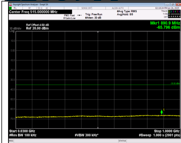
7-7-20MHz-20MHz-QPSK-QPSK-21152-21350-1RB#99-0 RB#0-30~1000MHz-PASS
