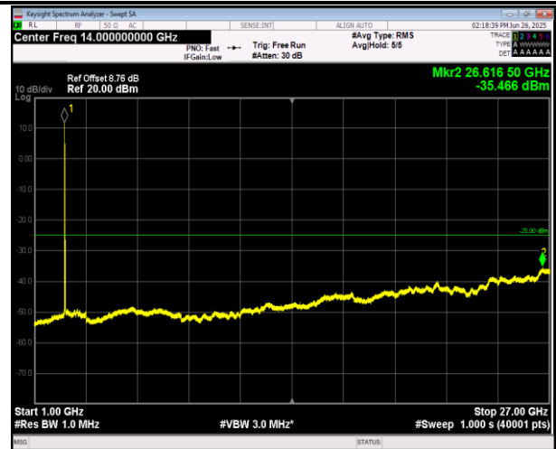
7-7-20MHz-20MHz-QPSK-QPSK-21152-21350-1RB#99-0R B#0-1000~27000MHz-PASS
