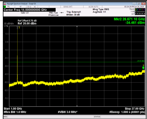
38-38-20MHz-20MHz-16QAM-16QAM-37901-38099-100R B#0-100RB#0-1000~27000MHz-PASS
