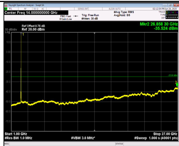
7-7-20MHz-20MHz-16QAM-16QAM-21001-21199-100RB#0 -100RB#0-1000~27000MHz-PASS
