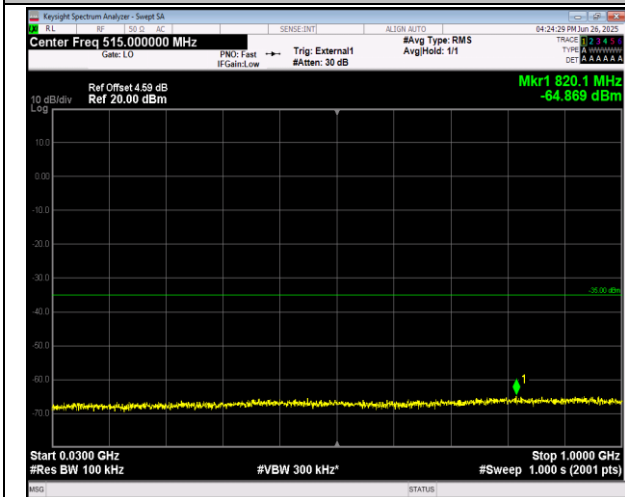
38-38-15MHz-15MHz-QPSK-QPSK-37925-38075-1RB#0- ORB#0-30~1000MHz-PASS
