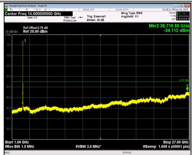
38-38-15MHz-15MHz-16QAM-16QAM-38025-38175-1RB# 0-ORB#0-1000~27000MHz-PASS
