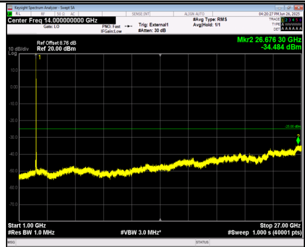
38-38-15MHz-15MHz-QPSK-QPSK-37825-37975-75RB#0- 75RB#0-1000~27000MHz-PASS
