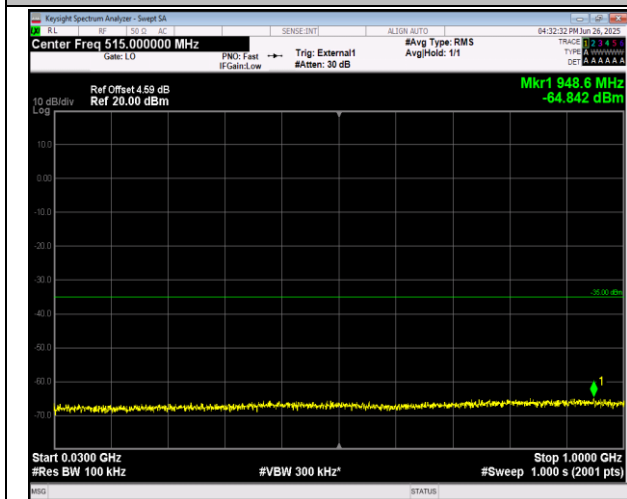
38-38-15MHz-15MHz-QPSK-QPSK-38025-38175-1RB#0- 1RB#74-30~1000MHz-PASS
