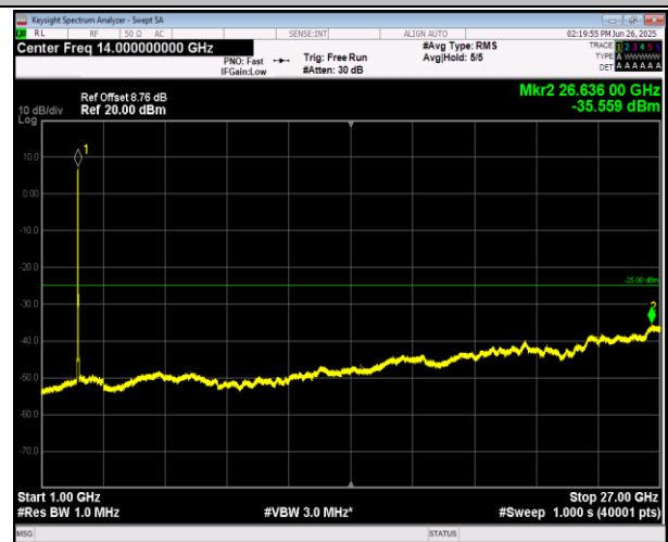
7-7-20MHz-20MHz-16QAM-16QAM-21152-21350-1RB#0-0 RB#0-1000~27000MHz-PASS
