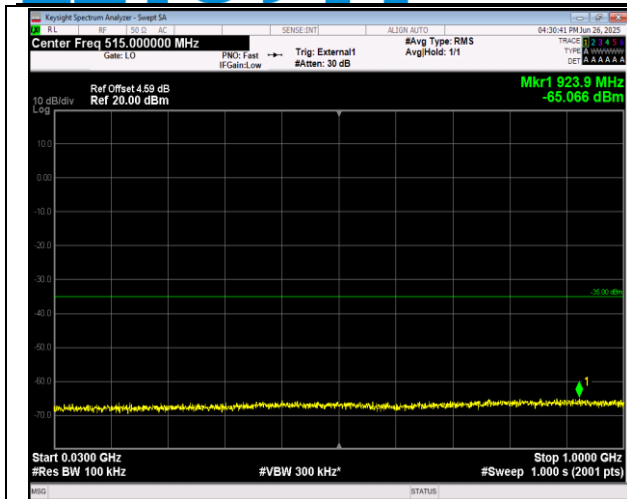
38-38-15MHz-15MHz-16QAM-16QAM-37925-38075-1RB #0-ORB#0-30~1000MHz-PASS
