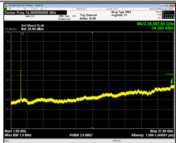
38-38-15MHz-15MHz-QPSK-QPSK-37925-38075-75RB#0-75RB#0-1000~27000MHz-PASS
