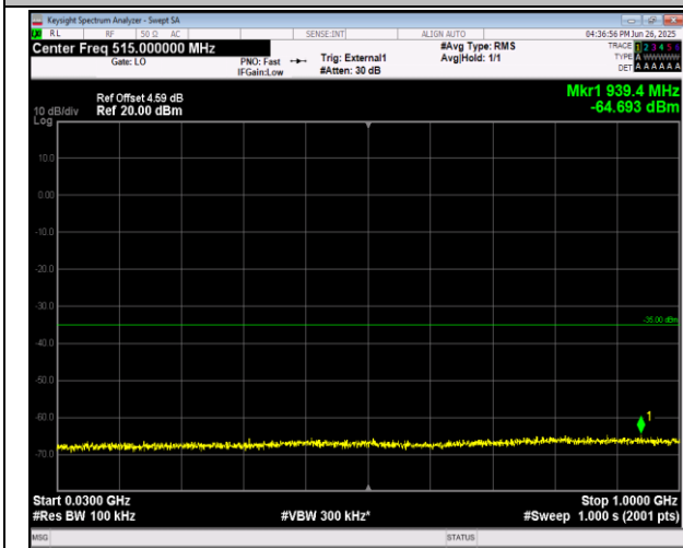
38-38-15MHz-15MHz-16QAM-16QAM-38025-38175-1RB #74-0RB#0-30~1000MHz-PASS
