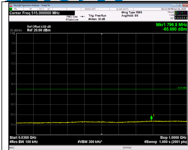
7-7-20MHz-20MHz-16QAM-16QAM-21001-21199-100RB #0-100RB#0-30~1000MHz-PASS
