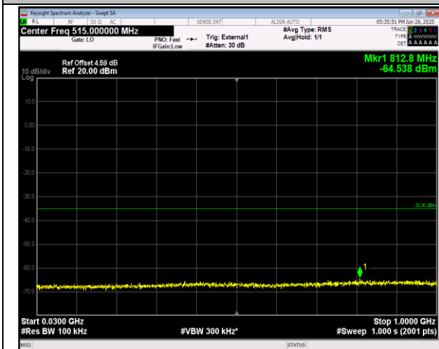
38-38-20MHz-20MHz-16QAM-16QAM-37901-38099-1RB #99-ORB#0-30~1000MHz-PASS
