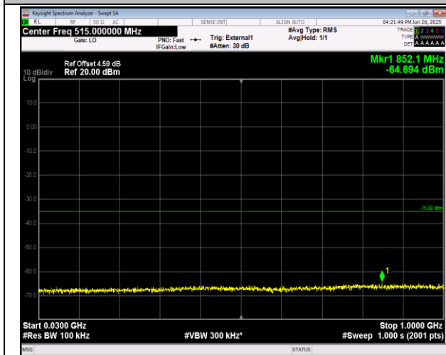
38-38-15MHz-15MHz-QPSK-QPSK-37825-37975-1RB#7 4-ORB#0-30~1000MHz-PASS
