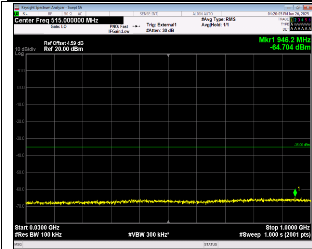
38-38-15MHz-15MHz-QPSK-QPSK-37825-37975-75RB# 0-75RB#0-30~1000MHz-PASS
