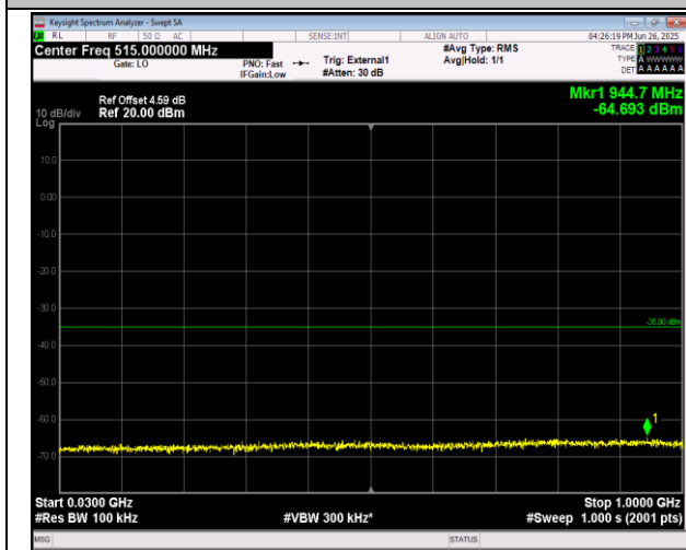
38-38-15MHz-15MHz-16QAM-16QAM-37925-38075-1RB #0-1RB#74-30~1000MHz-PASS
