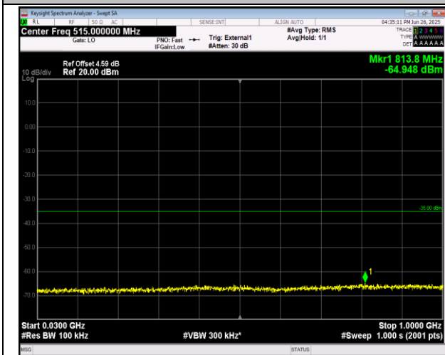
38-38-15MHz-15MHz-16QAM-16QAM-38025-38175-75R B#0-75RB#0-30~1000MHz-PASS
