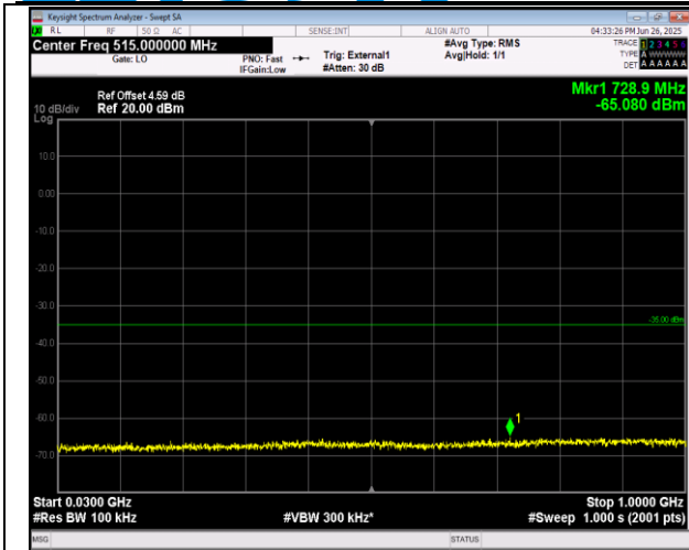
38-38-15MHz-15MHz-16QAM-16QAM-38025-38175-1RB #0-1RB#74-30~1000MHz-PASS
