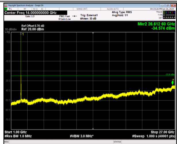
38-38-15MHz-15MHz-16QAM-16QAM-37825-37975-1RB# 0-1RB#74-1000~27000MHz-PASS
