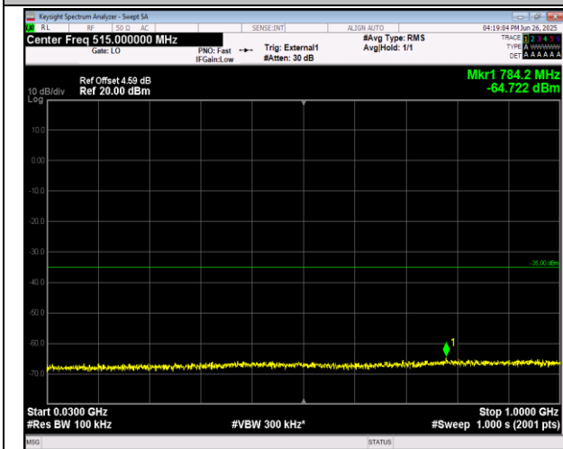
38-38-15MHz-15MHz-16QAM-16QAM-37825-37975-1RB #0-1RB#74-30~1000MHz-PASS
