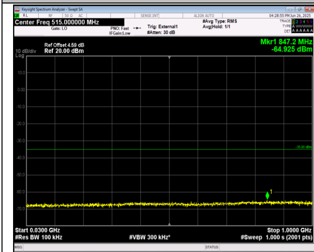
38-38-15MHz-15MHz-QPSK-QPSK-37925-38075-1RB#7-4-0RB#0-30~1000MHz-PASS
