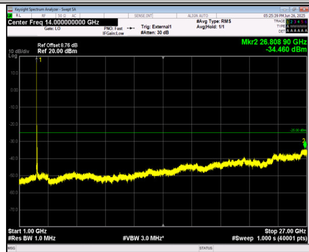
38-38-20MHz-20MHz-16QAM-16QAM-37850-38048-1RB# 0-1RB#99-1000~27000MHz-PASS
