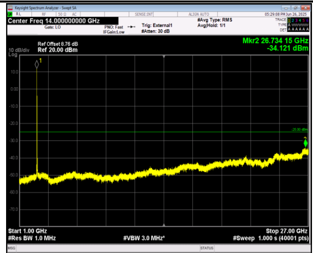
38-38-20MHz-20MHz-16QAM-16QAM-37850-38048-1RB# 99-ORB#0-1000~27000MHz-PASS
