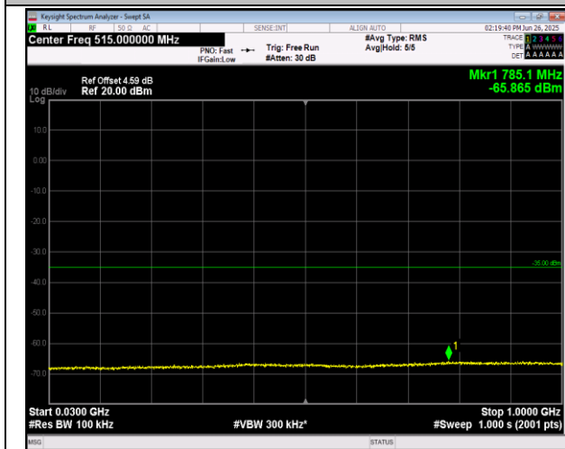
7-7-20MHz-20MHz-16QAM-16QAM-21152-21350-1RB#0- -0RB#0-30~1000MHz-PASS
