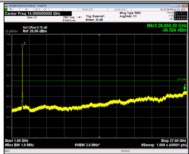
38-38-15MHz-15MHz-16QAM-16QAM-37825-37975-1RB# 0-0RB#0-1000~27000MHz-PASS
