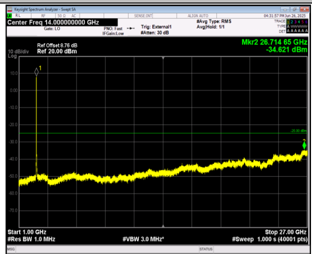
38-38-15MHz-15MHz-QPSK-QPSK-38025-38175-1RB#0-0 RB#0-1000~27000MHz-PASS
