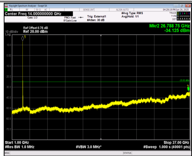
38-38-15MHz-15MHz-QPSK-QPSK-37925-38075-1RB#74-0RB#0-1000~27000MHz-PASS
