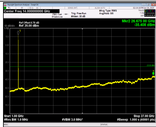
7-7-20MHz-20MHz-16QAM-16QAM-21152-21350-1RB#99- 0RB#0-1000~27000MHz-PASS
