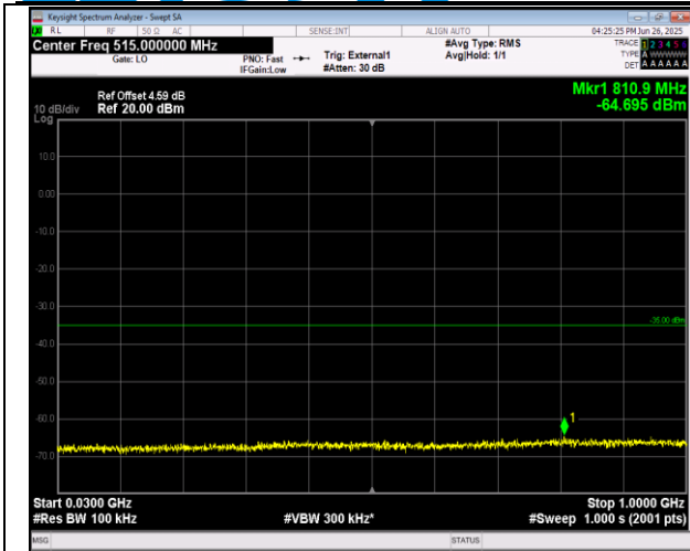
38-38-15MHz-15MHz-QPSK-QPSK-37925-38075-1RB#0-1RB#74-30~1000MHz-PASS
