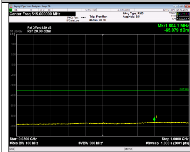
7-7-20MHz-20MHz-QPSK-QPSK-21152-21350-1RB#0-0 RB#0-30~1000MHz-PASS
