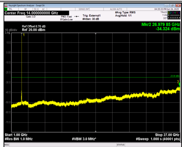
38-38-15MHz-15MHz-16QAM-16QAM-38025-38175-75RB #0-75RB#0-1000~27000MHz-PASS
