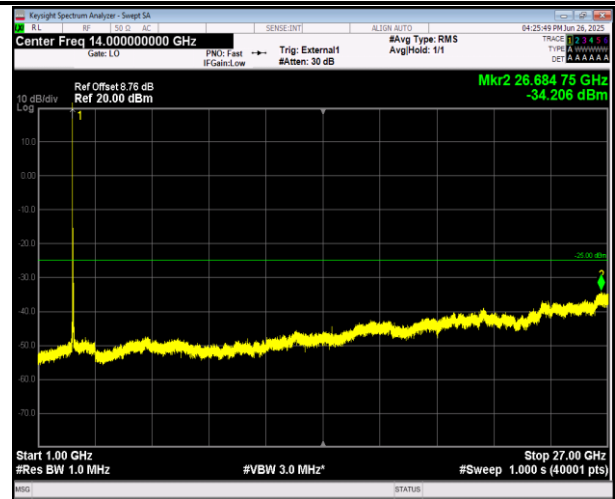
38-38-15MHz-15MHz-QPSK-QPSK-37925-38075-1RB#0-1RB#74-1000~27000MHz-PASS
