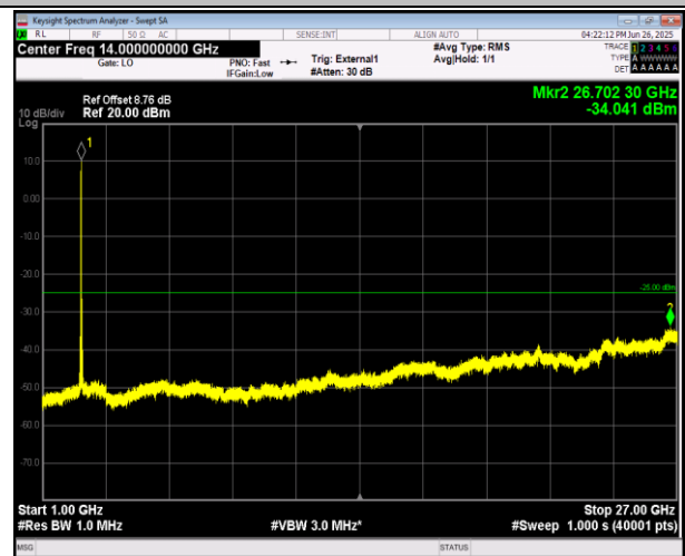
38-38-15MHz-15MHz-QPSK-QPSK-37825-37975-1RB#74- ORB#0-1000~27000MHz-PASS
