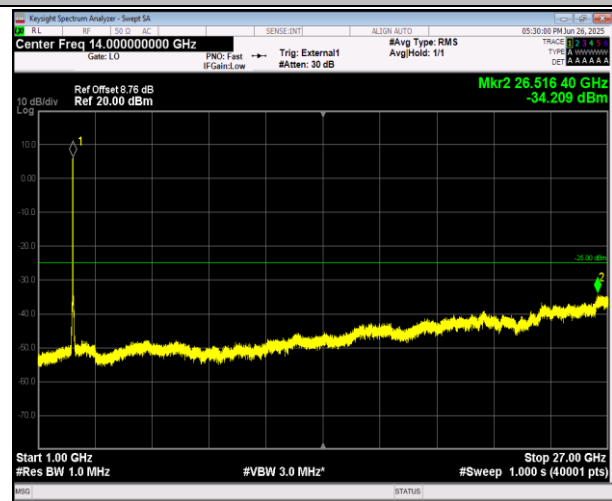
38-38-20MHz-20MHz-16QAM-16QAM-37850-38048-1RB# 0-0RB#0-1000~27000MHz-PASS
