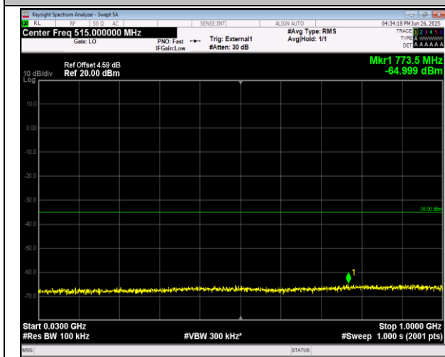
38-38-15MHz-15MHz-QPSK-QPSK-38025-38175-75RB#- 0-75RB#0-30~1000MHz-PASS
