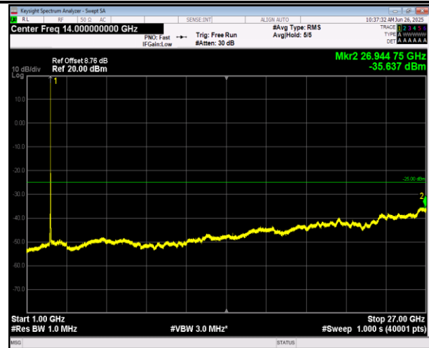
7-7-20MHz-10MHz-16QAM-16QAM-21251-21395-1RB#0-1 RB#49-1000~27000MHz-PASS
