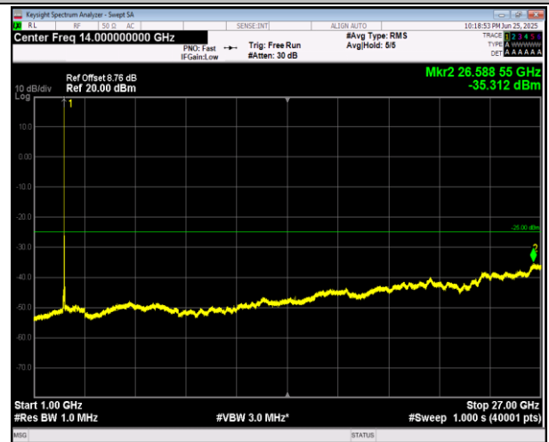
7-7-10MHz-20MHz-16QAM-16QAM-21206-21350-50RB#0- 100RB#0-1000~27000MHz-PASS
