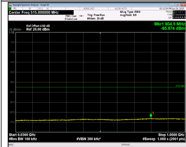
7-7-20MHz-20MHz-16QAM-16QAM-21001-21199-1RB#9 9-0RB#0-30~1000MHz-PASS
