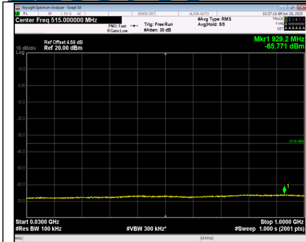
7-7-20MHz-10MHz-16QAM-16QAM-21251-21395-1RB#0 -1RB#49-30~1000MHz-PASS
