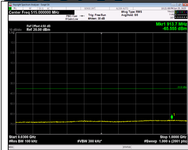
7-7-20MHz-10MHz-QPSK-QPSK-20850-20994-1RB#0-0 RB#0-30~1000MHz-PASS
