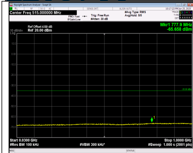
7-7-10MHz-20MHz-16QAM-16QAM-21206-21350-1RB#0 -1RB#99-30~1000MHz-PASS
