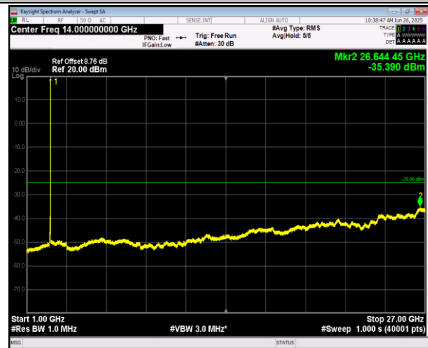
7-7-20MHz-10MHz-16QAM-16QAM-21251-21395-100RB# 0-50RB#0-1000~27000MHz-PASS
