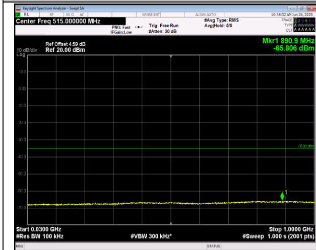
7-7-20MHz-10MHz-16QAM-16QAM-21251-21395-100RB #0-50RB#0-30~1000MHz-PASS
