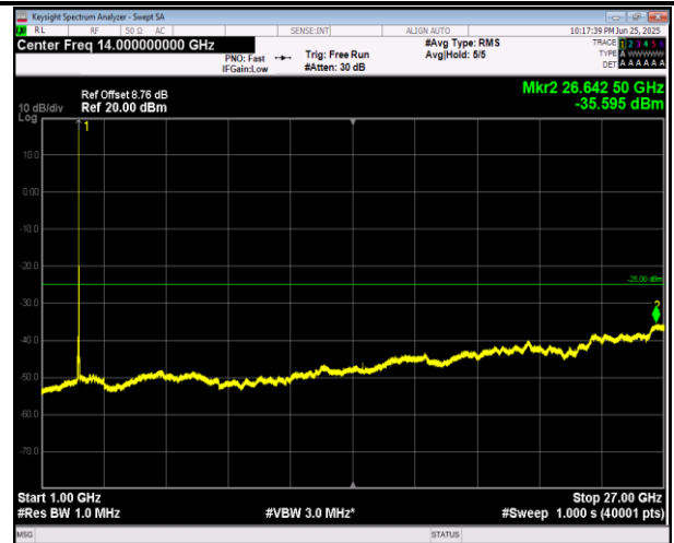
7-7-10MHz-20MHz-16QAM-16QAM-21206-21350-1RB#0-1 RB#99-1000~27000MHz-PASS
