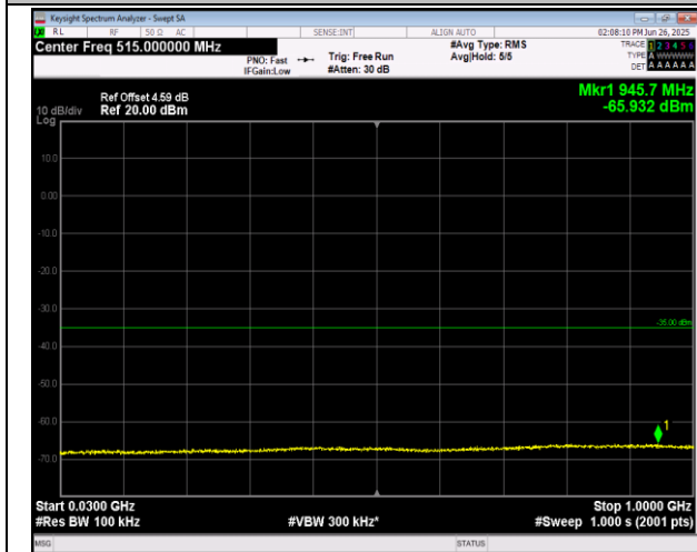
7-7-20MHz-20MHz-QPSK-QPSK-20850-21048-1RB#99-0 RB#0-30~1000MHz-PASS
