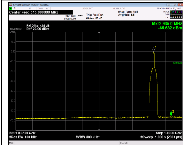
5-5-10MHz-10MHz-16QAM-16QAM-20501-20600-1RB#0 -ORB#0-30~1000MHz-PASS
