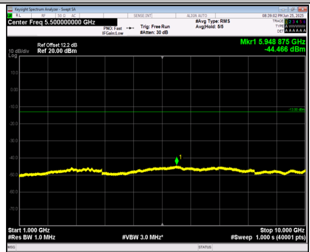
5-5-10MHz-10MHz-QPSK-QPSK-20476-20575-1RB#49-0R B#0-1000~10000MHz-PASS
