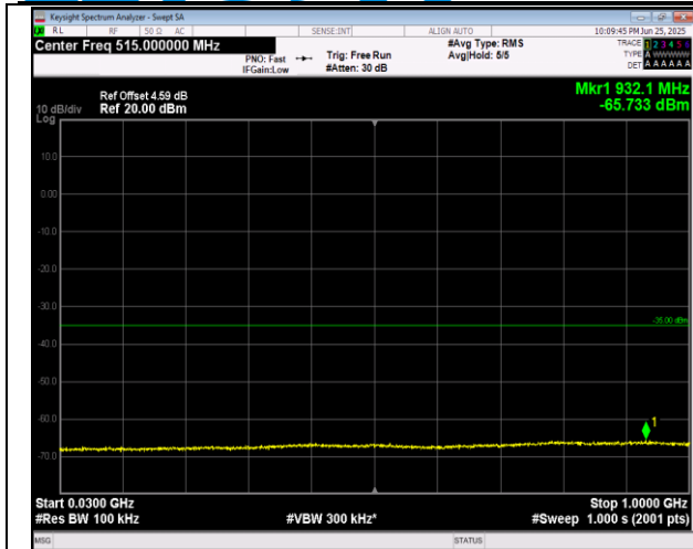
7-7-10MHz-20MHz-16QAM-16QAM-20805-20949-1RB#4 9-0RB#0-30~1000MHz-PASS
