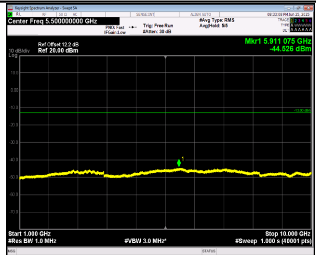
5-5-10MHz-10MHz-QPSK-QPSK-20450-20549-50RB#0-50 RB#0-1000~10000MHz-PASS
