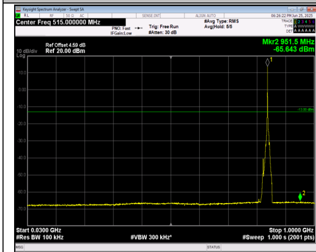
5-5-5MHz-3MHz-16QAM-16QAM-20595-20634-1RB#24- 0RB#0-30~1000MHz-PASS
