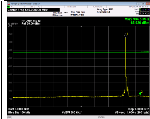
5-5-10MHz-10MHz-QPSK-QPSK-20501-20600-1RB#49-0 RB#0-30~1000MHz-PASS
