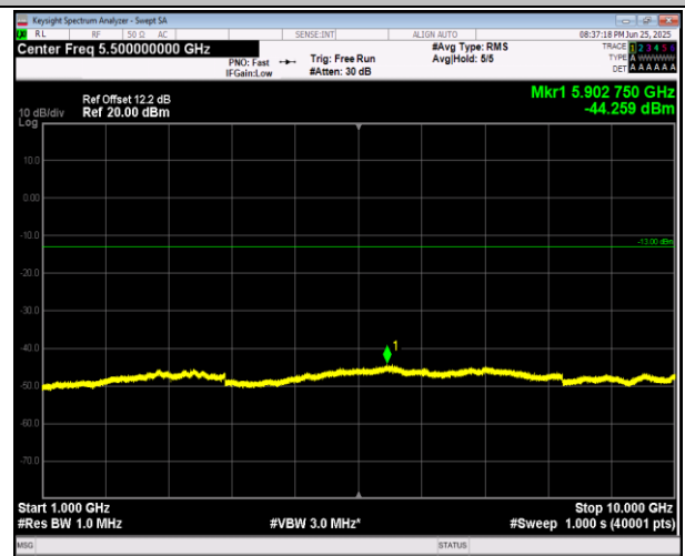
5-5-10MHz-10MHz-16QAM-16QAM-20476-20575-1RB#0-1 RB#49-1000~10000MHz-PASS
