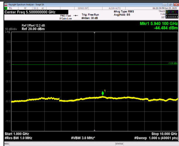
5-5-5MHz-3MHz-16QAM-16QAM-20510-20549-25RB#0-15RB#0-1000~10000MHz-PASS
