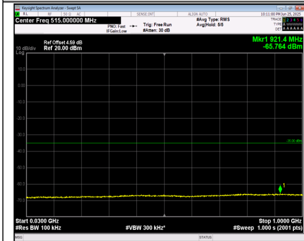
7-7-10MHz-20MHz-QPSK-QPSK-21006-21150-1RB#0-0 RB#0-30~1000MHz-PASS
