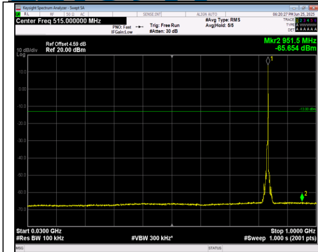
5-5-5MHz-3MHz-16QAM-16QAM-20510-20549-25RB#0-15RB#0-30~1000MHz-PASS
