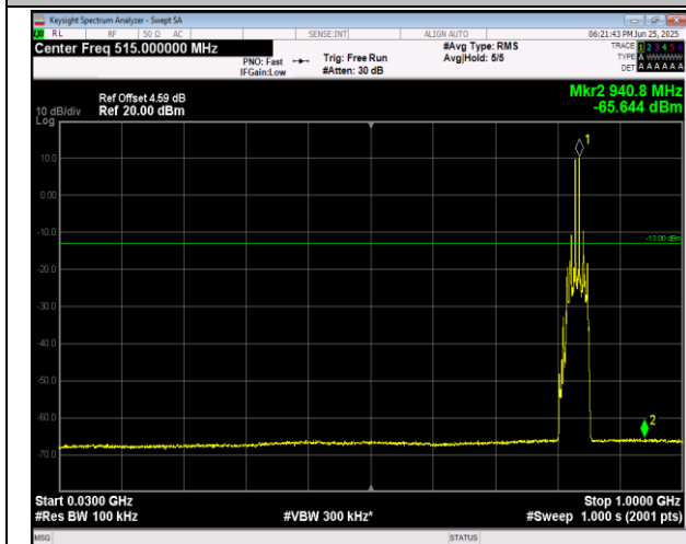
5-5-5MHz-3MHz-16QAM-16QAM-20510-20549-1RB#24- ORB#0-30~1000MHz-PASS
