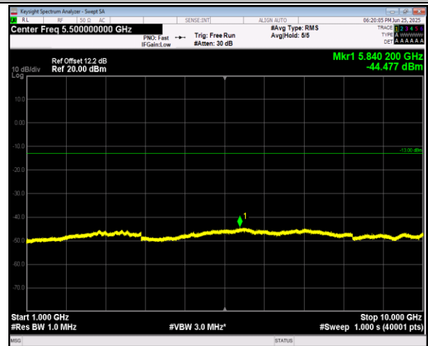
5-5-5MHz-3MHz-QPSK-QPSK-20510-20549-25RB#0-15RB #0-1000~10000MHz-PASS
