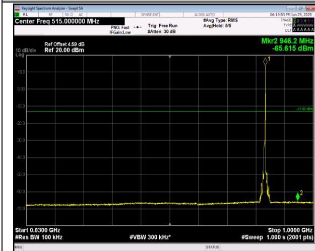
5-5-5MHz-3MHz-QPSK-QPSK-20510-20549-25RB#0-15 RB#0-30~1000MHz-PASS
