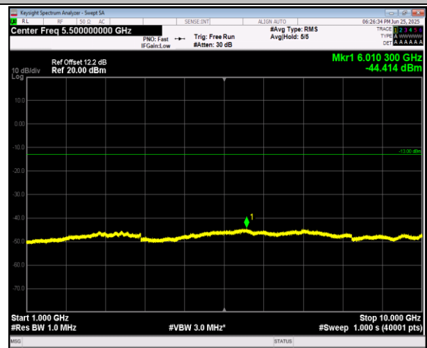
5-5-5MHz-3MHz-16QAM-16QAM-20595-20634-1RB#24-0R B#0-1000~10000MHz-PASS
