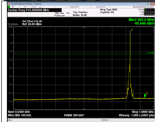
5-5-10MHz-10MHz-QPSK-QPSK-20450-20549-50RB#0-5 ORB#0-30~1000MHz-PASS
