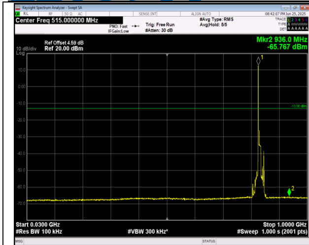
5-5-10MHz-10MHz-16QAM-16QAM-20501-20600-1RB#0 -1RB#49-30~1000MHz-PASS
