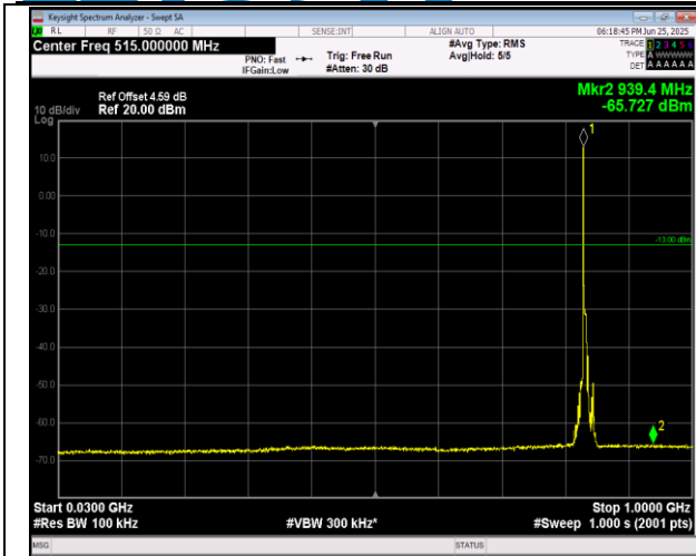
5-5-5MHz-3MHz-QPSK-QPSK-20510-20549-1RB#0-1RB #15-30~1000MHz-PASS
