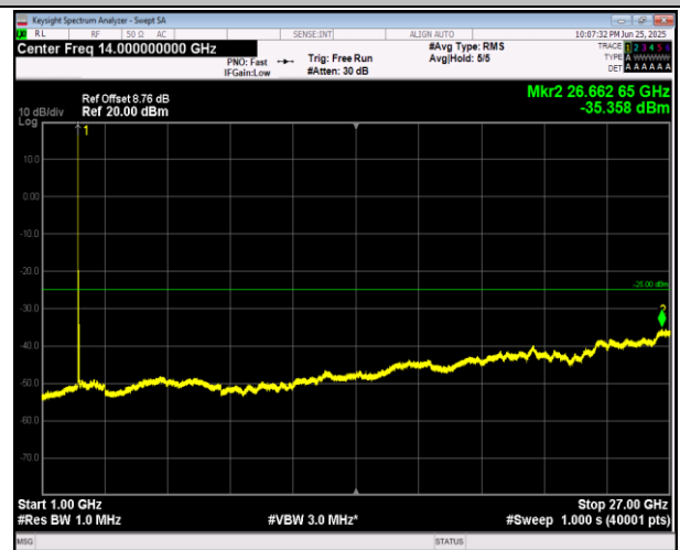
7-7-10MHz-20MHz-16QAM-16QAM-20805-20949-1RB#0-1 RB#99-1000~27000MHz-PASS
