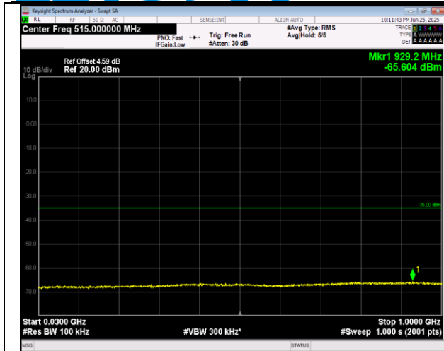
7-7-10MHz-20MHz-QPSK-QPSK-21006-21150-1RB#0-1 RB#99-30~1000MHz-PASS
