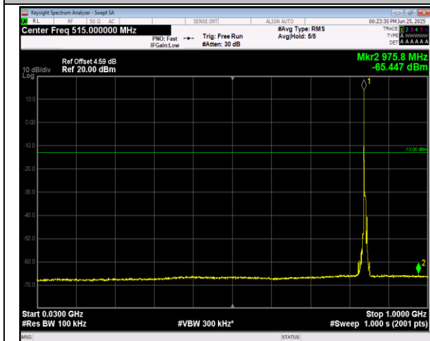
5-5-5MHz-3MHz-QPSK-QPSK-20595-20634-1RB#0-1RB#15-30~1000MHz-PASS
