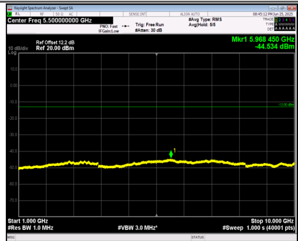
5-5-10MHz-10MHz-16QAM-16QAM-20501-20600-1RB#0-0 RB#0-1000~10000MHz-PASS
