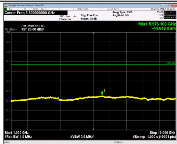
5-5-5MHz-3MHz-QPSK-QPSK-20595-20634-1RB#0-1RB#15-1000~10000MHz-PASS
