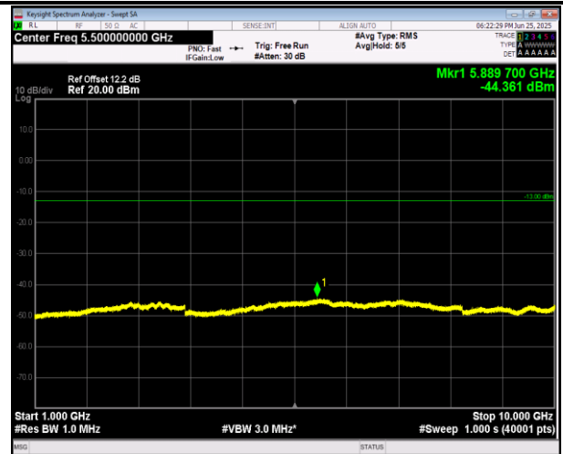
5-5-5MHz-3MHz-16QAM-16QAM-20510-20549-1RB#0-0R B#0-1000~10000MHz-PASS
