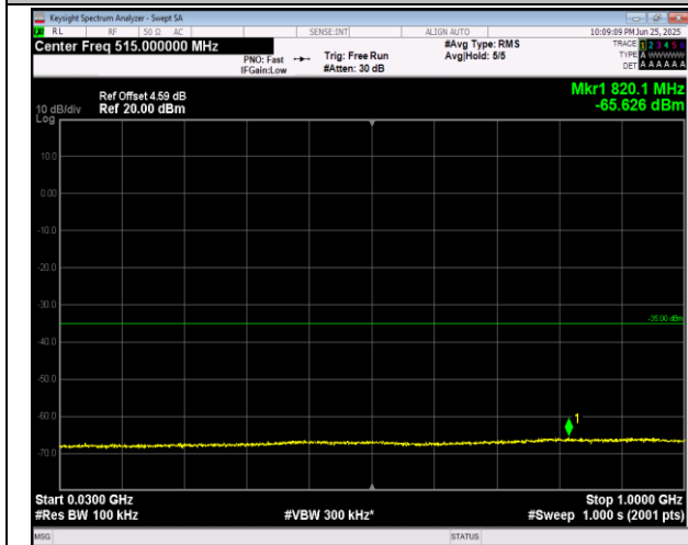
7-7-10MHz-20MHz-QPSK-QPSK-20805-20949-1RB#49-0 RB#0-30~1000MHz-PASS
