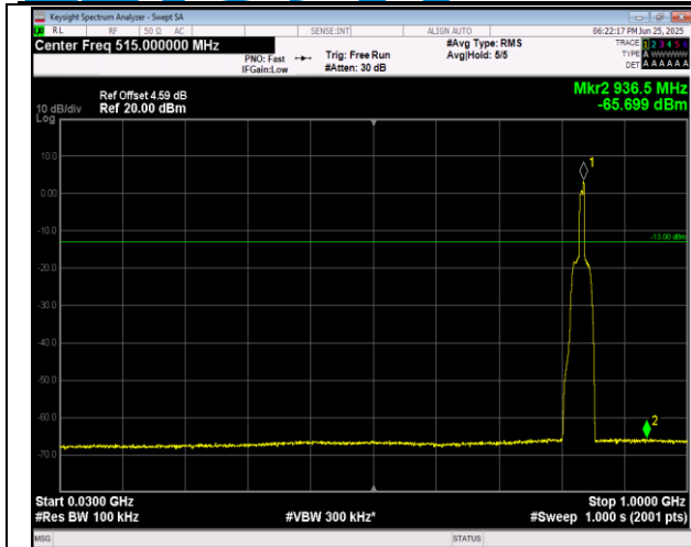
5-5-5MHz-3MHz-16QAM-16QAM-20510-20549-1RB#0-0 RB#0-30~1000MHz-PASS
