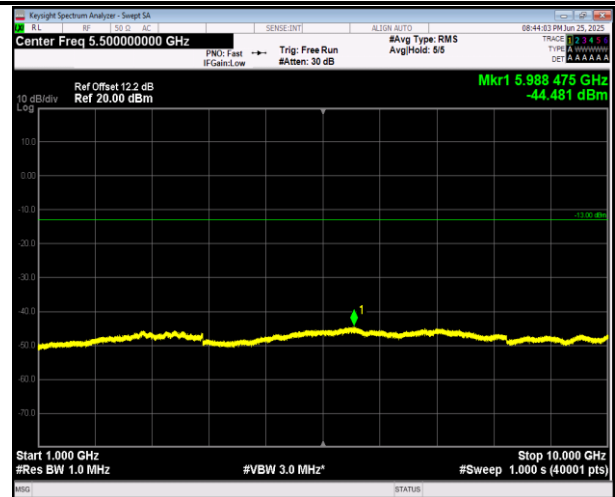
5-5-10MHz-10MHz-QPSK-QPSK-20501-20600-1RB#49-0R B#0-1000~10000MHz-PASS
