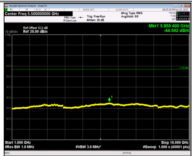
5-5-10MHz-10MHz-16QAM-16QAM-20450-20549-1RB#0-0 RB#0-1000~10000MHz-PASS
