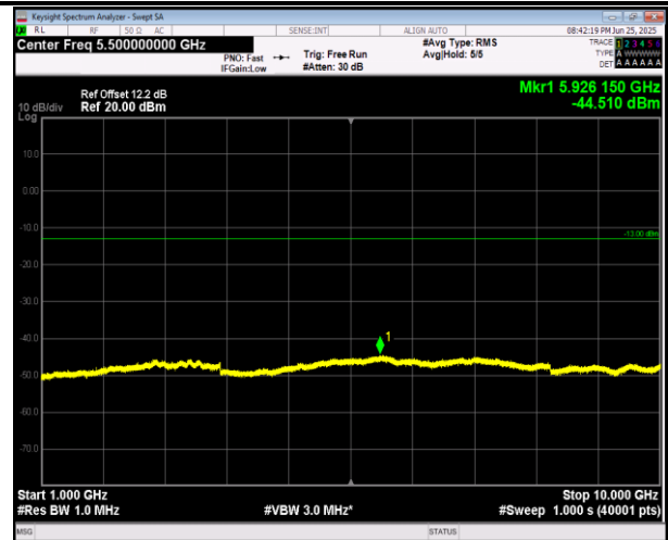
5-5-10MHz-10MHz-16QAM-16QAM-20501-20600-1RB#0-1 RB#49-1000~10000MHz-PASS
