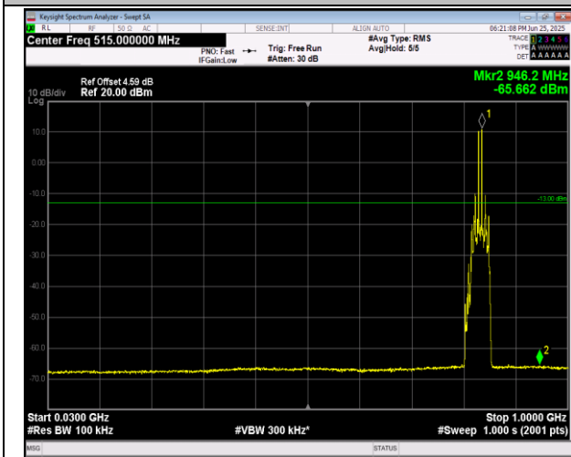
5-5-5MHz-3MHz-QPSK-QPSK-20510-20549-1RB#24-0R B#0-30~1000MHz-PASS
