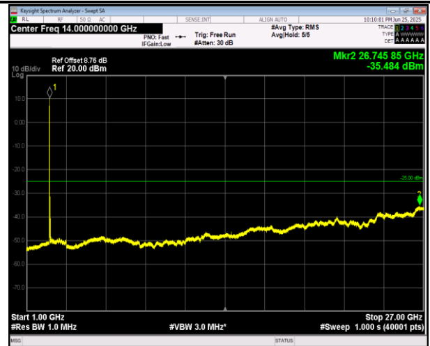
7-7-10MHz-20MHz-16QAM-16QAM-20805-20949-1RB#49- 0RB#0-1000~27000MHz-PASS
