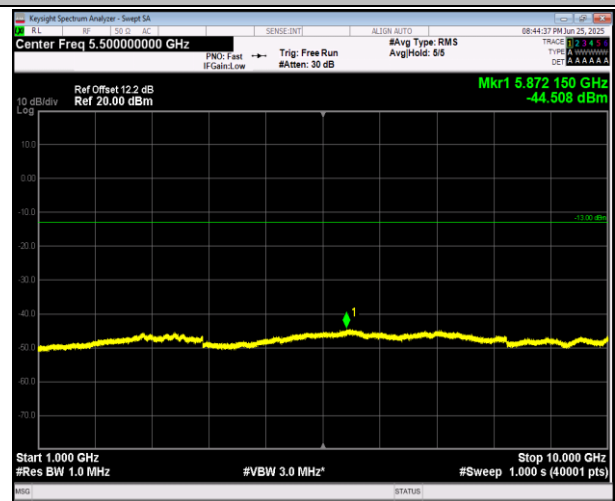
5-5-10MHz-10MHz-16QAM-16QAM-20501-20600-1RB#49- 0RB#0-1000~10000MHz-PASS
