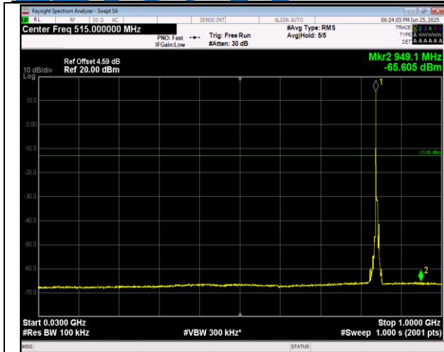
5-5-5MHz-3MHz-16QAM-16QAM-20595-20634-1RB#0-1 RB#15-30~1000MHz-PASS
