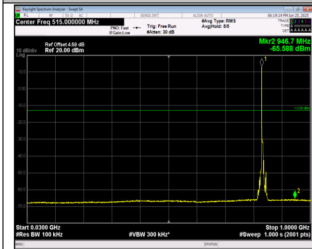
5-5-5MHz-3MHz-16QAM-16QAM-20510-20549-1RB#0-1 RB#15-30~1000MHz-PASS
