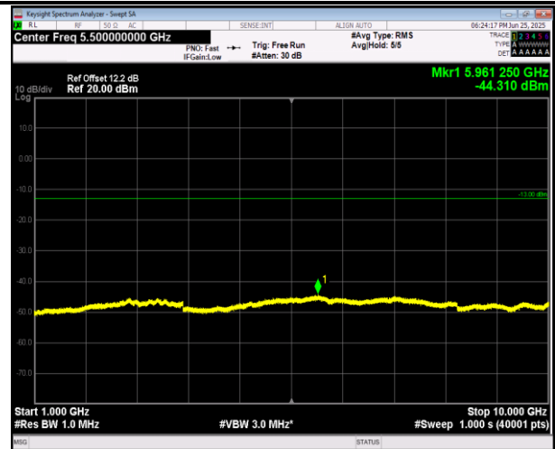
5-5-5MHz-3MHz-16QAM-16QAM-20595-20634-1RB#0-1R B#15-1000~10000MHz-PASS
