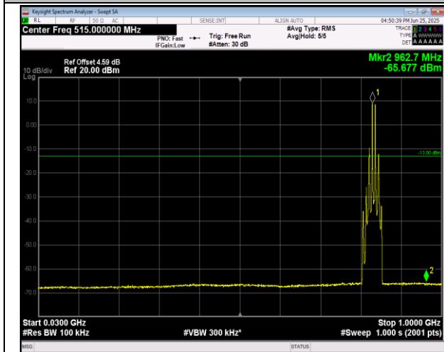
5-5-3MHz-5MHz-16QAM-16QAM-20501-20540-1RB#14- ORB#0-30~1000MHz-PASS
