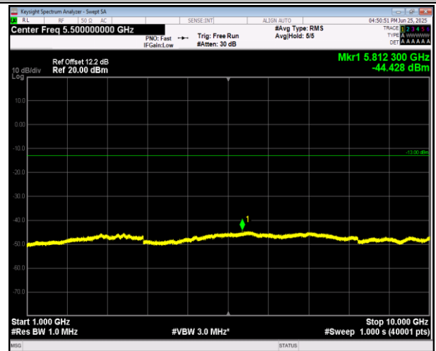
5-5-3MHz-5MHz-16QAM-16QAM-20501-20540-1RB#14-0R B#0-1000~10000MHz-PASS
