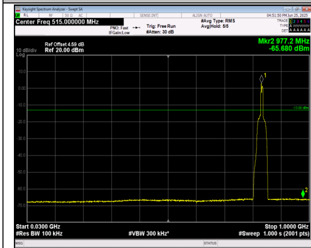
5-5-3MHz-5MHz-QPSK-QPSK-20586-20625-1RB#0-0RB#0-30~1000MHz-PASS
