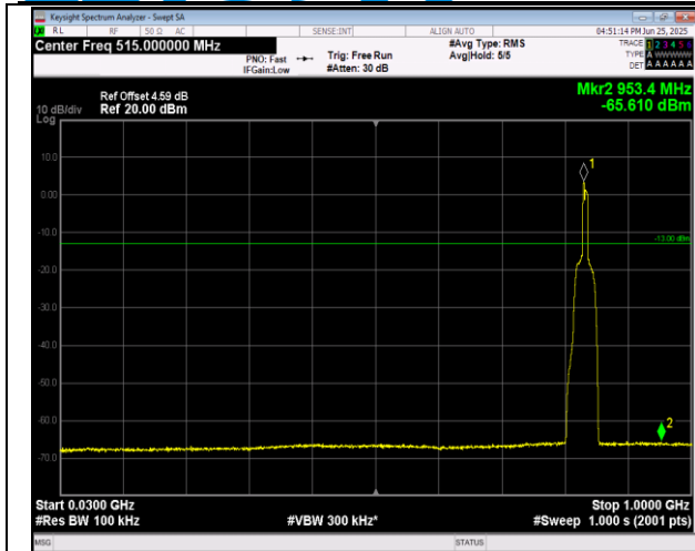
5-5-3MHz-5MHz-16QAM-16QAM-20501-20540-1RB#0-0 RB#0-30~1000MHz-PASS
