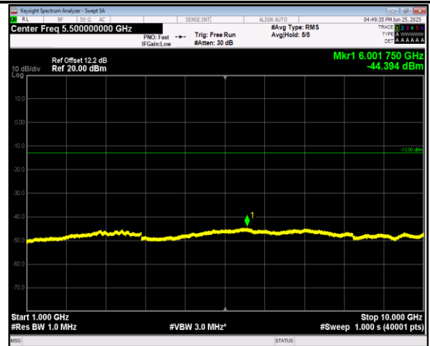
5-5-3MHz-5MHz-16QAM-16QAM-20501-20540-15RB#0-25RB#0-1000~10000MHz-PASS
