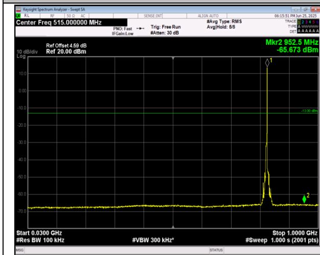
5-5-5MHz-3MHz-16QAM-16QAM-20425-20464-25RB#0-15RB#0-30~1000MHz-PASS
