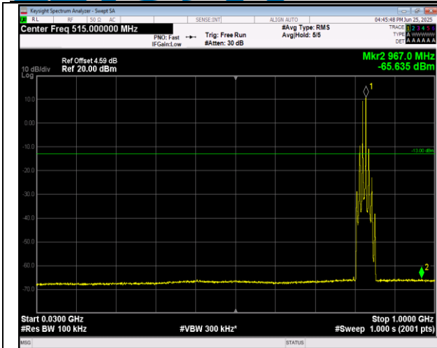
5-5-3MHz-5MHz-16QAM-16QAM-20416-20455-1RB#14- ORB#0-30~1000MHz-PASS
