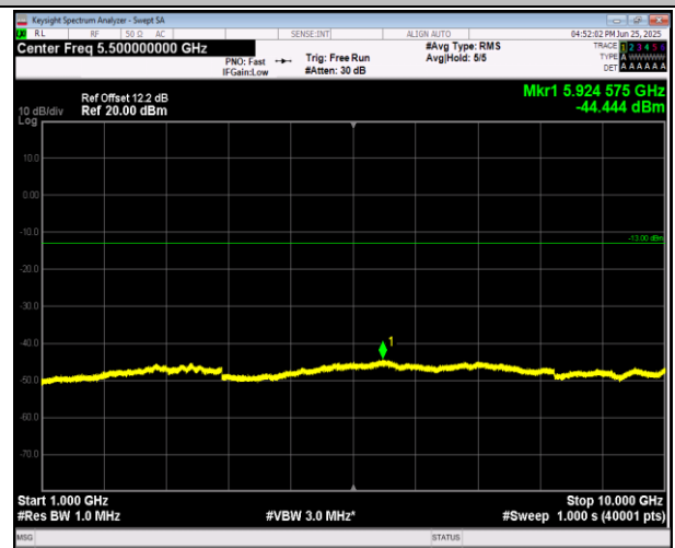
5-5-3MHz-5MHz-QPSK-QPSK-20586-20625-1RB#0-0RB#0-1000~10000MHz-PASS
