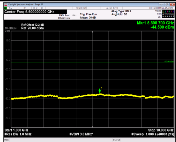
5-5-3MHz-5MHz-16QAM-16QAM-20416-20455-1RB#14-0R B#0-1000~10000MHz-PASS
