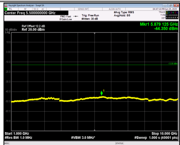
5-5-3MHz-5MHz-QPSK-QPSK-20501-20540-1RB#0-0RB#0 -1000~10000MHz-PASS
