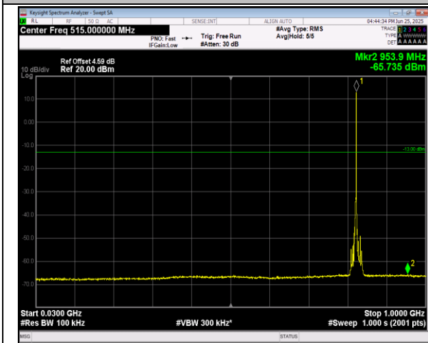
5-5-3MHz-5MHz-16QAM-16QAM-20416-20455-15RB#0- 25RB#0-30~1000MHz-PASS
