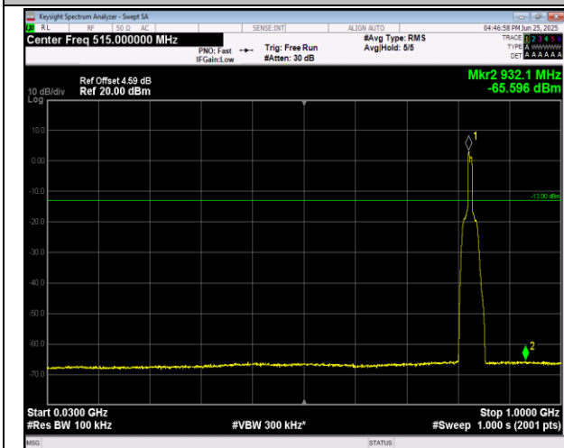
5-5-3MHz-5MHz-QPSK-QPSK-20501-20540-1RB#0-0RB #0-30~1000MHz-PASS
