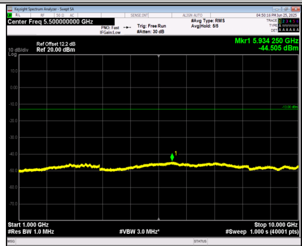
5-5-3MHz-5MHz-QPSK-QPSK-20501-20540-1RB#14-0RB# 0-1000~10000MHz-PASS
