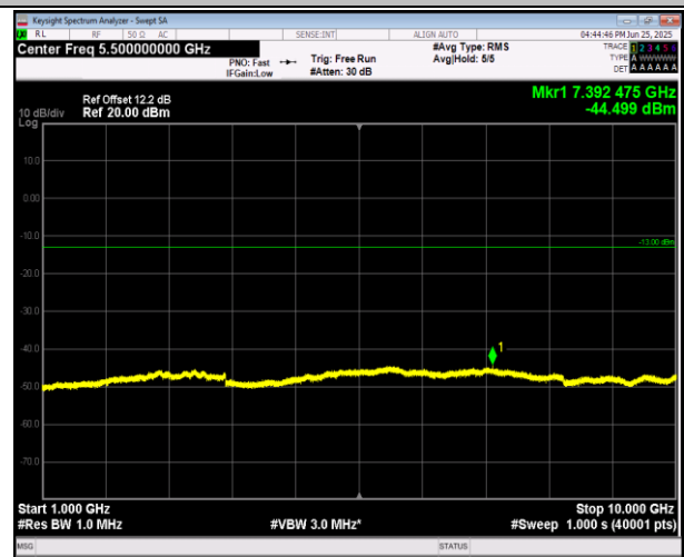
5-5-3MHz-5MHz-16QAM-16QAM-20416-20455-15RB#0-25 RB#0-1000~10000MHz-PASS
