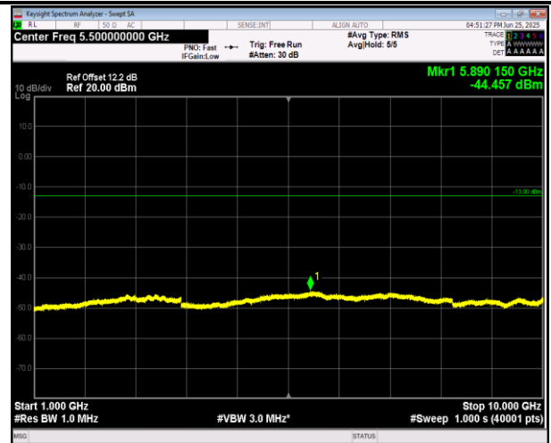
5-5-3MHz-5MHz-16QAM-16QAM-20501-20540-1RB#0-0R B#0-1000~10000MHz-PASS
