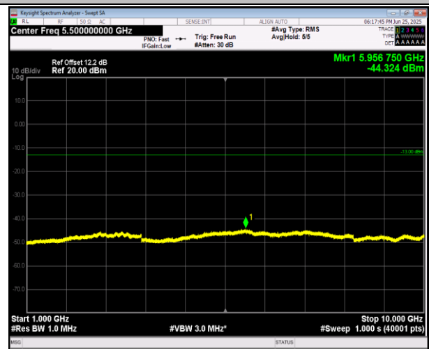
5-5-5MHz-3MHz-16QAM-16QAM-20425-20464-1RB#0-0R B#0-1000~10000MHz-PASS
