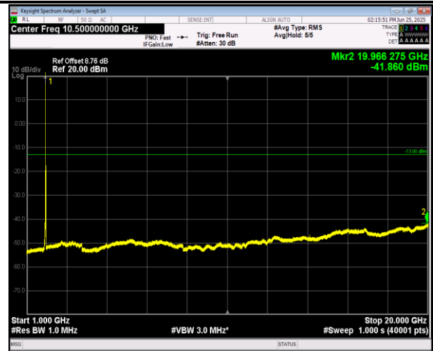
2-2-20MHz-20MHz-16QAM-16QAM-18902-19100-1RB#0-1 RB#99-1000~20000MHz-PASS
