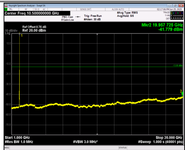
2-2-20MHz-20MHz-16QAM-16QAM-18902-19100-100RB# 0-100RB#0-1000~20000MHz-PASS
