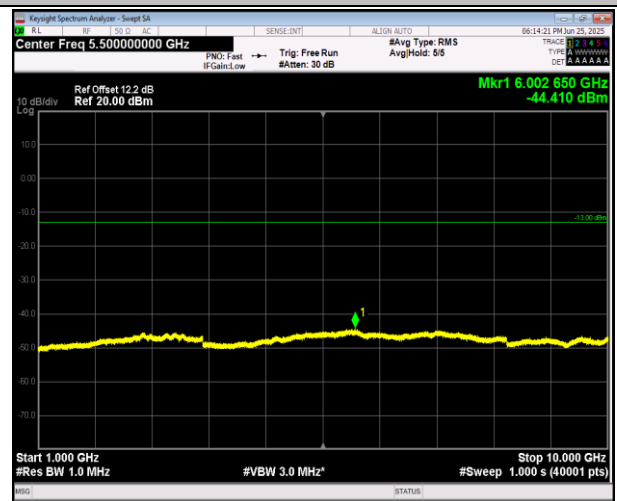
5-5-5MHz-3MHz-QPSK-QPSK-20425-20464-1RB#0-1RB#1 5-1000~10000MHz-PASS
