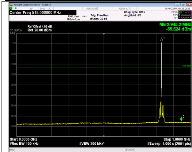
5-5-3MHz-5MHz-16QAM-16QAM-20501-20540-15RB#0-25RB#0-30~1000MHz-PASS
