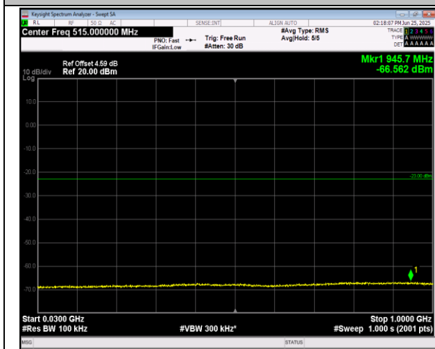
2-2-20MHz-20MHz-16QAM-16QAM-18902-19100-1RB#9 9-0RB#0-30~1000MHz-PASS
