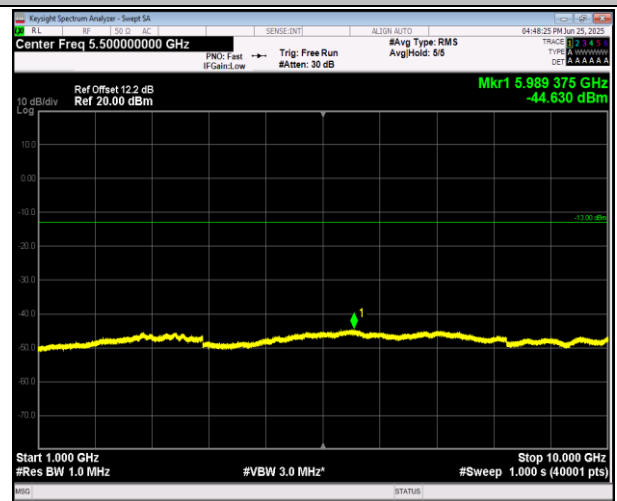
5-5-3MHz-5MHz-16QAM-16QAM-20501-20540-1RB#0-1R B#24-1000~10000MHz-PASS
