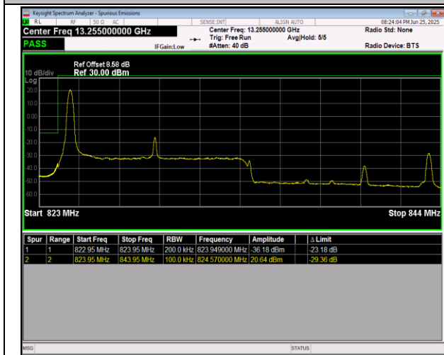
5-5-10MHz-10MHz-QPSK@QPSK-QPSK@QPSK-20450-20549-1RB#49@50RB#0-0RB#0@50RB#0-PASS
