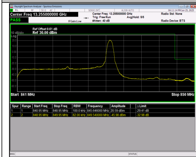
5-5-5MHz-3MHz-16QAM@16QAM-16QAM@16QAM-20595-20634-1RB#0@25RB#0-0RB#0@15RB#0-PASS
