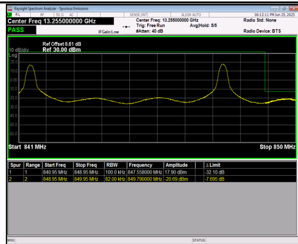
5-5-5MHz-3MHz-QPSK@QPSK-QPSK@QPSK-20595-206 34-25RB#0@25RB#0-15RB#0@15RB#0-PASS
