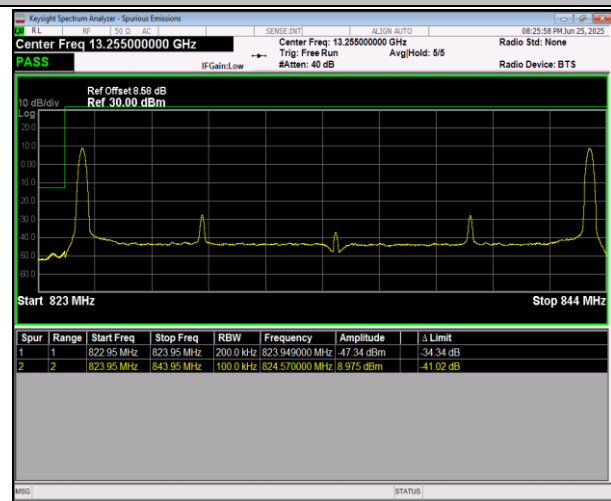
5-5-10MHz-10MHz-QPSK@QPSK-QPSK@QPSK-20450-20549-50RB#0@50RB#0-50RB#0@50RB#0-PASS
