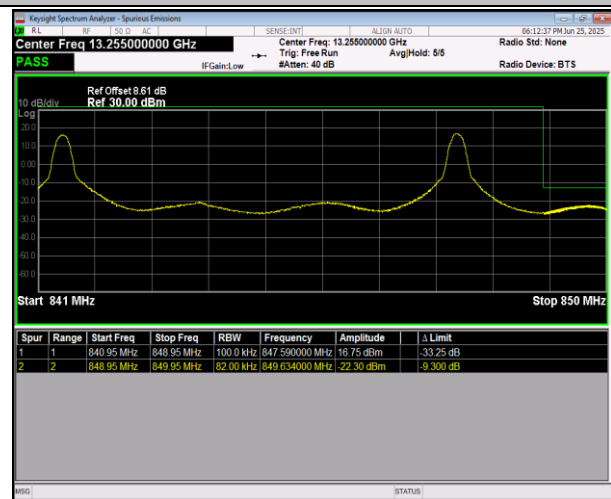
5-5-5MHz-3MHz-16QAM@16QAM-16QAM@16QAM-20595-20634-25RB#0@25RB#0-15RB#0@15RB#0-PASS
