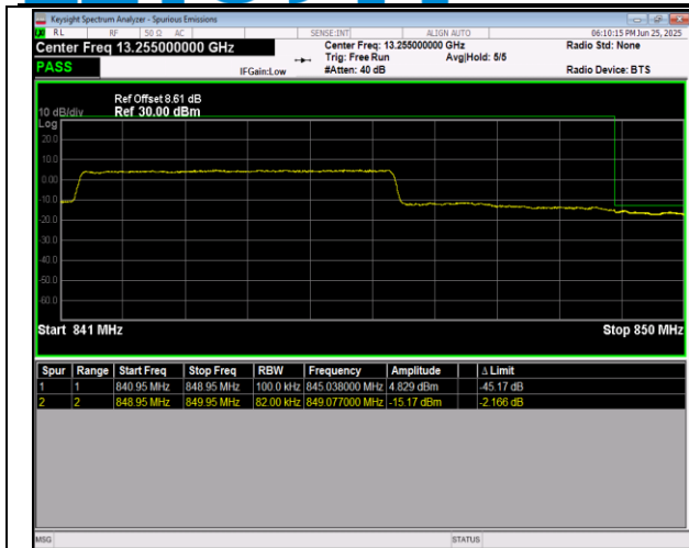
5-5-5MHz-3MHz-QPSK@QPSK-QPSK@QPSK-20595-20 634-1RB#24@25RB#0-0RB#0@15RB#0-PASS
