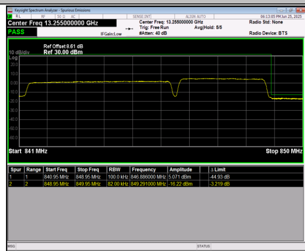
5-5-5MHz-3MHz-16QAM@16QAM-16QAM@16QAM-20595-20634-1RB#0@25RB#0-1RB#15@15RB#0-PASS
