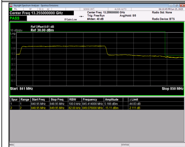
5-5-5MHz-3MHz-16QAM@16QAM-16QAM@16QAM-20595-20634-1RB#24@25RB#0-0RB#0@15RB#0-PASS
