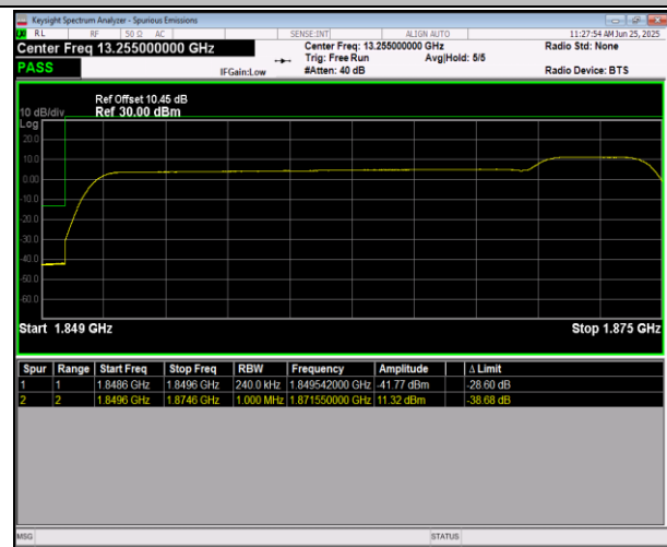
2-2-20MHz-5MHz-16QAM@16QAM-16QAM@16QAM-18700-18817-1RB#0@100RB#0-1RB#24@25RB#0-PASS
