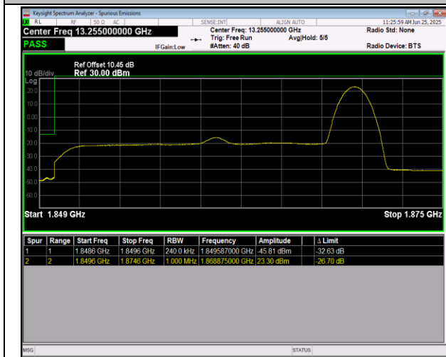
2-2-20MHz-5MHz-16QAM@16QAM-16QAM@16QAM-18700-18817-1RB#0@100RB#0-0RB#0@25RB#0-PASS
