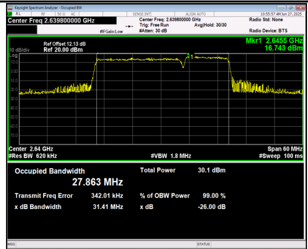
41(2555-2655)-41(2555-2655)-20MHz-15MHz-16QAM-16Q AM-40340-40511-100RB#0-75RB#0-PASS
