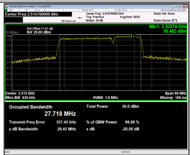
7-7-20MHz-10MHz-16QAM-16QAM-21051-21195-100RB#0-50RB#0-PASS
