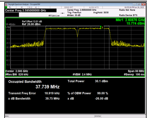
38-38-20MHz-20MHz-16QAM-16QAM-37952-38150-100RB B#0-100RB#0-PASS
