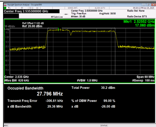
7-7-10MHz-20MHz-16QAM-16QAM-21206-21350-50RB#0- 100RB#0-PASS
