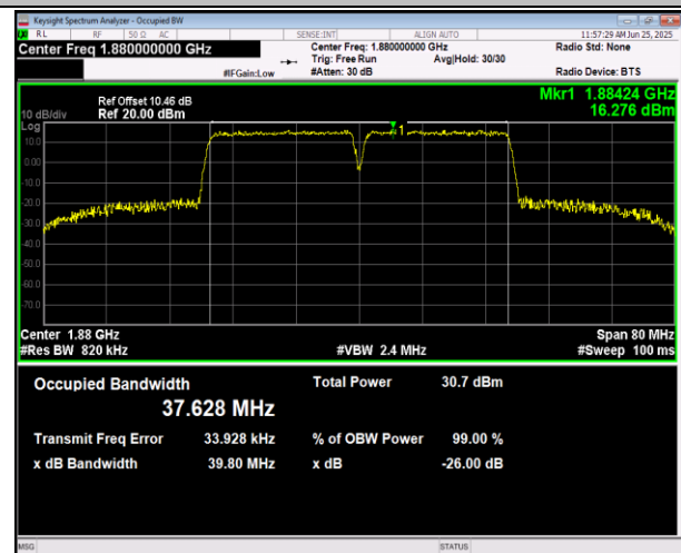
2-2-20MHz-20MHz-16QAM-16QAM-18902-19100-100RB#0-100RB#0-PASS
