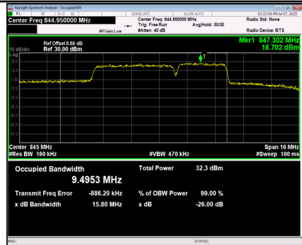
5-5-5MHz-10MHz-16QAM-16QAM-20428-20500-25RB#0-5 ORB#0-PASS
