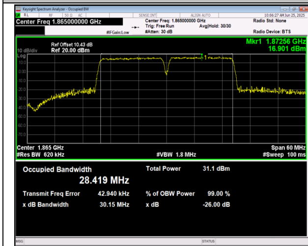
2-2-15MHz-15MHz-QPSK-QPSK-18825-18975-75RB#0-7 5RB#0-PASS
