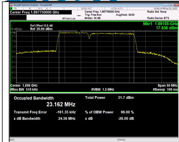
2-2-10MHz-20MHz-QPSK-QPSK-18655-18799-50RB#0-1 00RB#0-PASS
