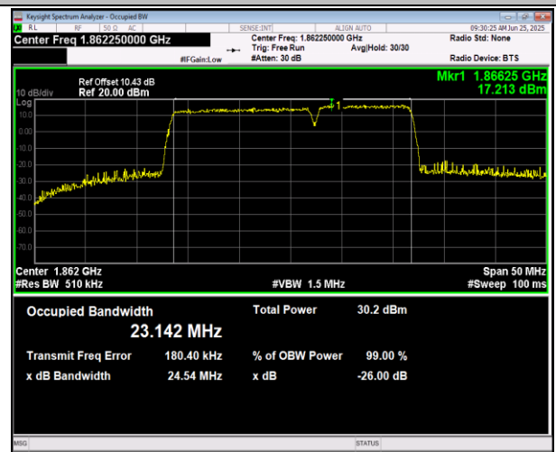
2-2-15MHz-10MHz-16QAM-16QAM-18851-18971-75RB#0-5 50RB#0-PASS
