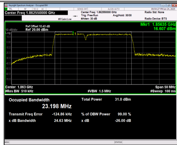
2-2-10MHz-15MHz-QPSK-QPSK-18829-18949-50RB#0-7 5RB#0-PASS
