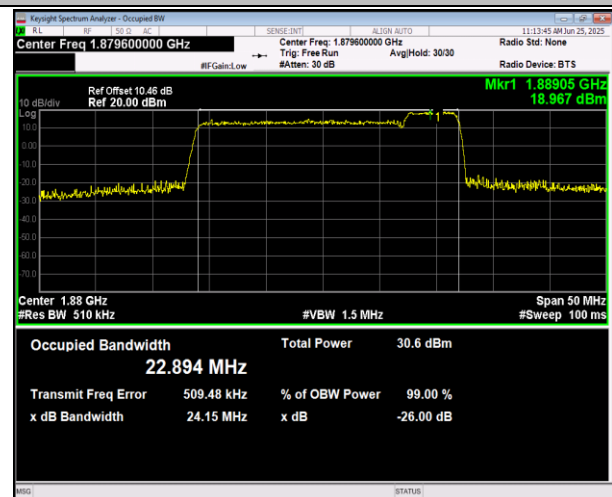
2-2-20MHz-5MHz-16QAM-16QAM-19050-19167-100RB#0- 25RB#0-PASS
