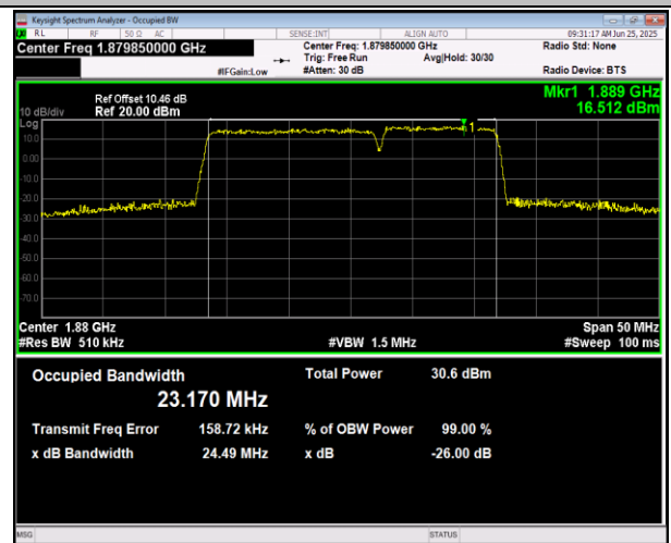
2-2-15MHz-10MHz-16QAM-16QAM-19027-19147-75RB#0-5 50RB#0-PASS
