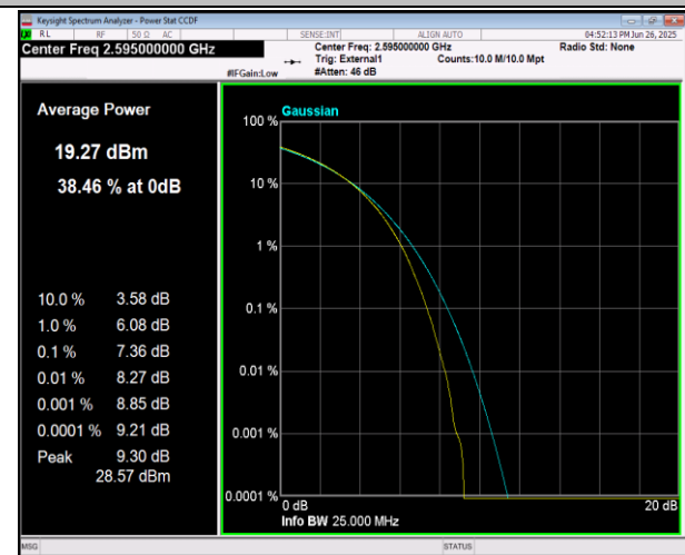
38-38-20MHz-20MHz-16QAM-16QAM-37952-38150-100R B#0-100RB#0-PASS
