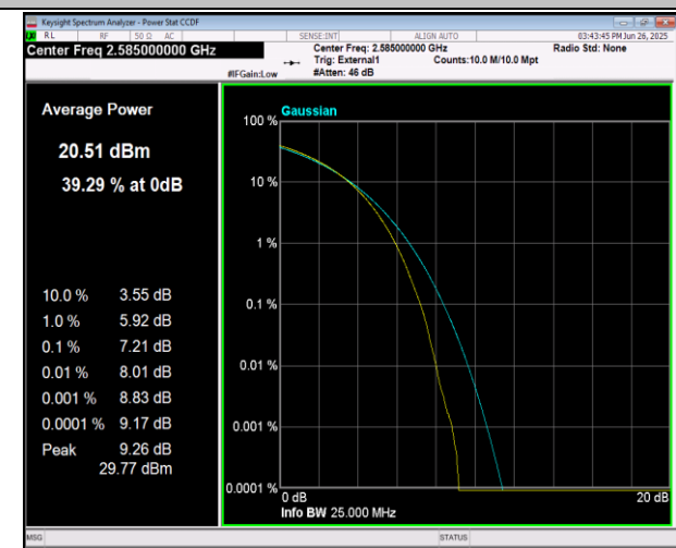
38-38-15MHz-15MHz-16QAM-16QAM-37925-38075-75RB #0-75RB#0-PASS
