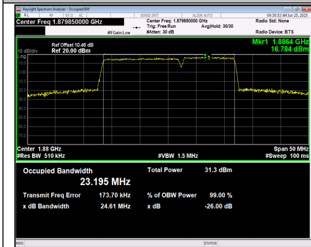
2-2-15MHz-10MHz-QPSK-QPSK-19027-19147-75RB#0-5 ORB#0-PASS
