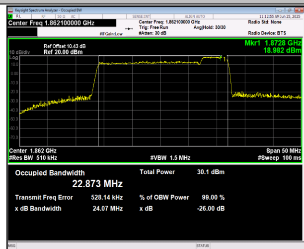
2-2-20MHz-5MHz-16QAM-16QAM-18875-18992-100RB#0- 25RB#0-PASS
