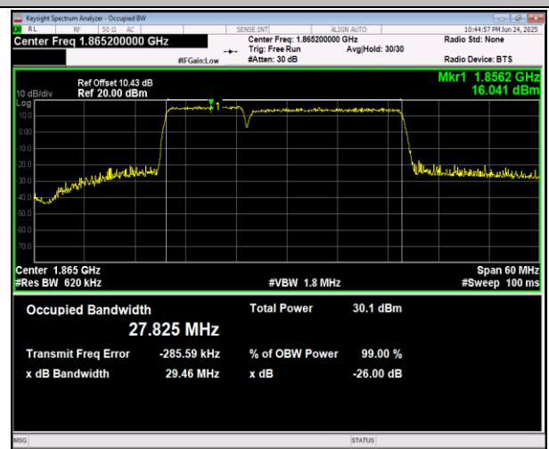
2-2-10MHz-20MHz-16QAM-16QAM-18806-18950-50RB#0- 100RB#0-PASS
