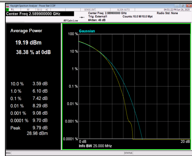
38-38-20MHz-20MHz-16QAM-16QAM-37901-38099-100R B#0-100RB#0-PASS
