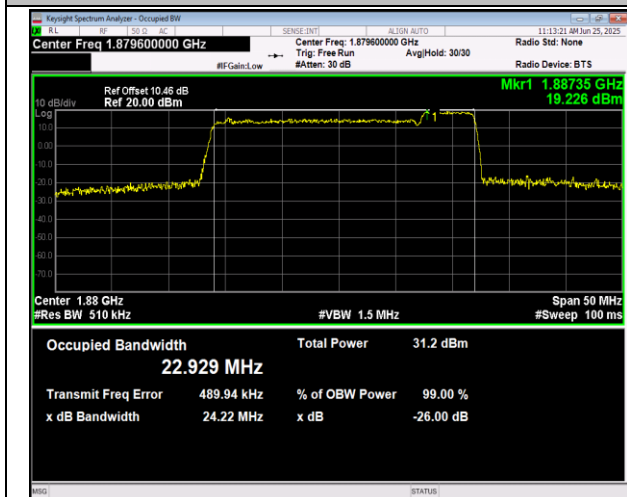
2-2-20MHz-5MHz-QPSK-QPSK-19050-19167-100RB#0-2 5RB#0-PASS
