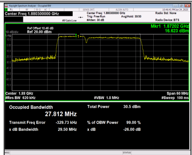
2-2-10MHz-20MHz-16QAM-16QAM-18956-19100-50RB#0- 100RB#0-PASS
