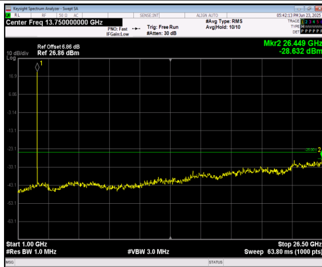
Band38-5MHz-64QAM-37775-1RB#0-Range2:1000~26500MHz
