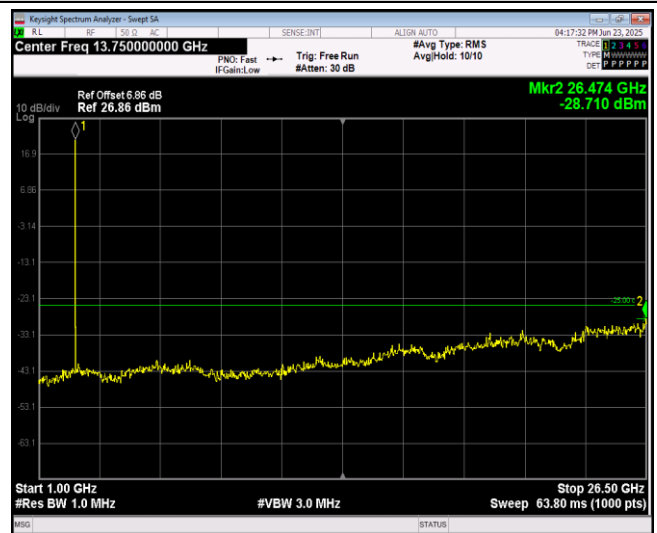
Band41-5MHz-16QAM-40640-1RB#0-Range2:1000~ 26500MHz
