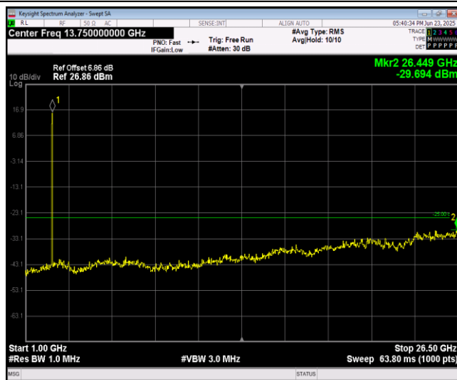
Band38-5MHz-64QAM-38000-1RB#0-Range2:1000~26500MHz
