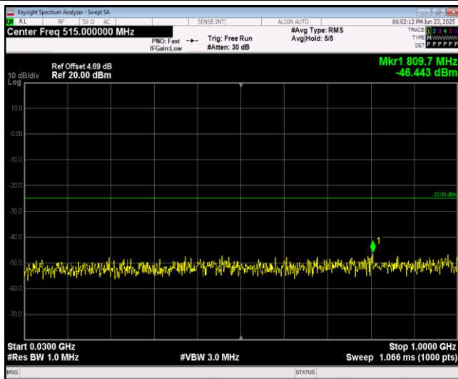
Band38-20MHz-QPSK-38150-1RB#0-Range1:30~1000MHz
