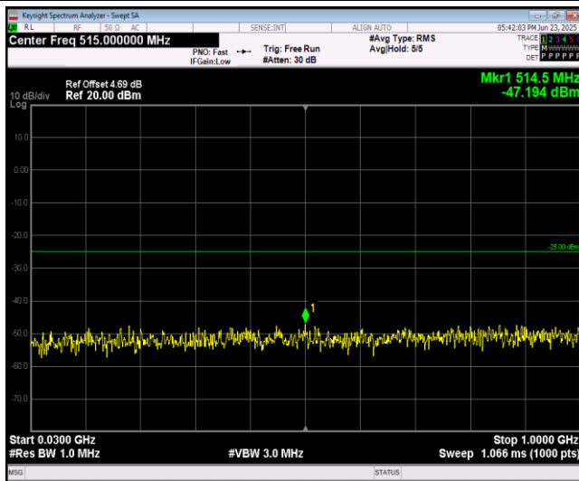
Band38-5MHz-64QAM-37775-1RB#0-Range1:30~1000MHz
