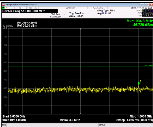
Band38-20MHz-16QAM-37850-1RB#0-Range1:30~1000MHz
