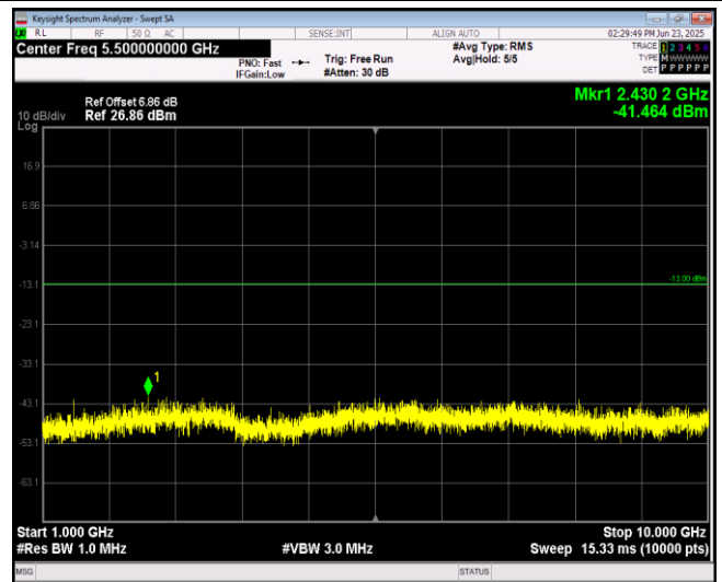
Band17-10MHz-QPSK-23780-1RB#0-Range2:1000~10000MHz
