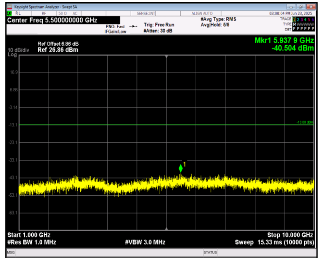
Band26-1.4MHz-16QAM-27033-1RB#0-Range2:1000 ~10000MHz
