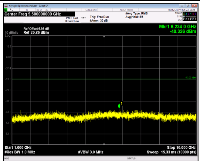
Band17-10MHz-QPSK-23790-1RB#0-Range2:1000~10000MHz
