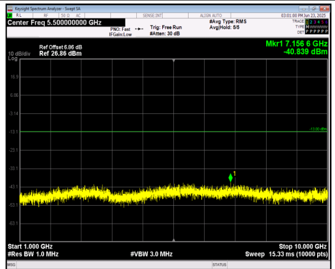
Band26-1.4MHz-64QAM-26697-1RB#0-Range2:1000 ~10000MHz
