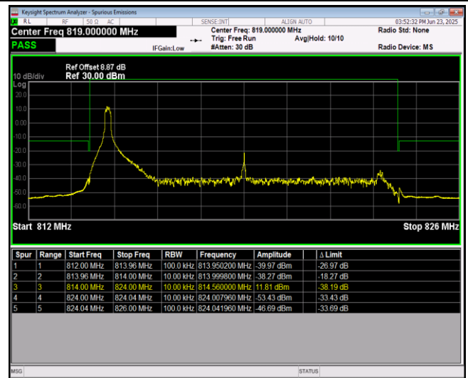
Band26-10MHz-64QAM-26740-50RB#0
