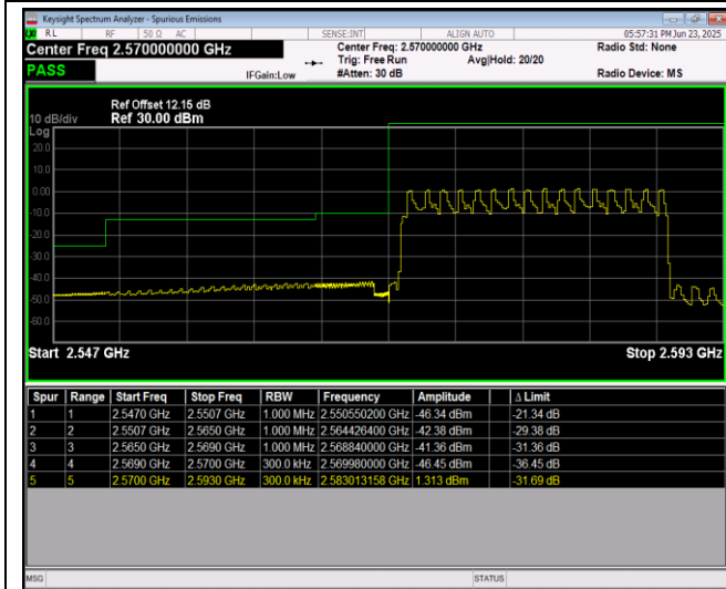
Band38-20MHz-16QAM-38150-1RB#99
