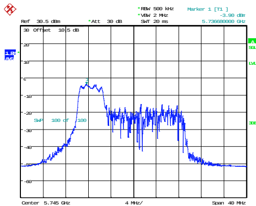
802.11ax20_5745MHz_RU_52/37_Chain 0
