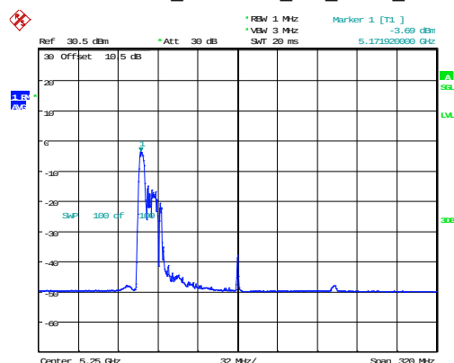
802.11ax160_5250MHz_RU_52/37_Chain 1
