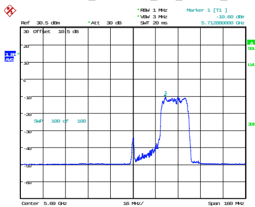
802.11ax80_5690MHz_RU_242/64_Chain 0
