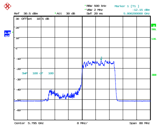
802.11ax40_5795MHz_RU_242/62_Chain 1
