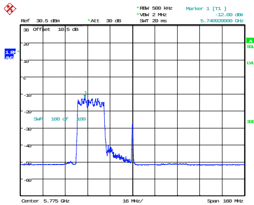
802.11ax80_5775MHz_RU_242/61_Chain 0
