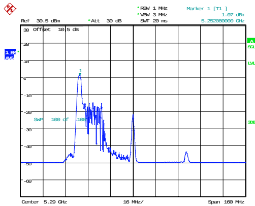
802.11ax80_5290MHz_RU_26/0_Chain 0
