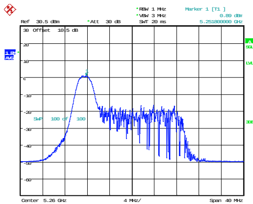
802.11ax20_5260MHz_RU_26/0_Chain 1
