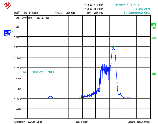
802.11ax80_5690MHz_RU_52/52_Chain 1
