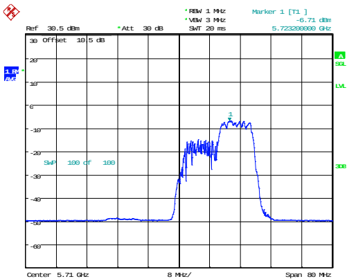
802.11ax40_5710MHz_RU_106/56_Chain 0
