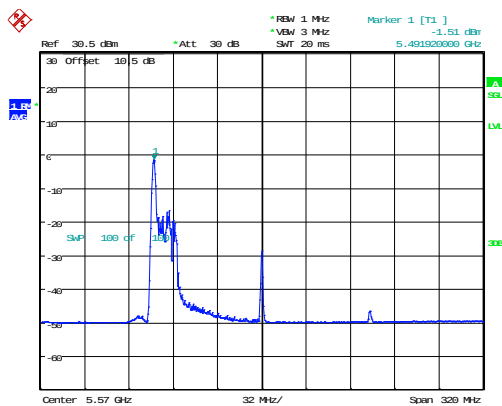
802.11ax160_5570MHz_RU_26/0_Chain 0
