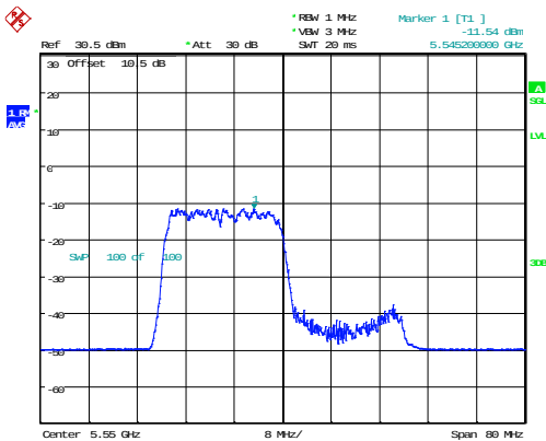
802.11ax40_5550MHz_RU_242/61_Chain 1
