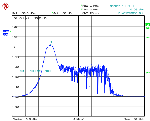
802.11ax20_5500MHz_RU_26/0_Chain 0
