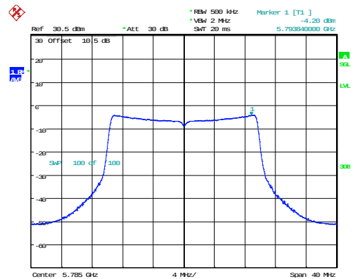
802.11ax20_5785MHz_RU_Full_Chain 0
