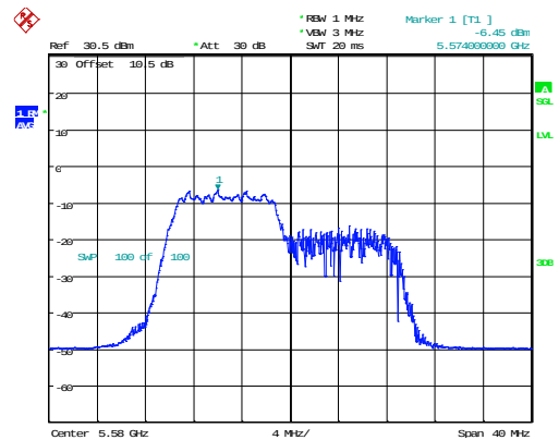
802.11ax20_5580MHz_RU_106/53_Chain 1
