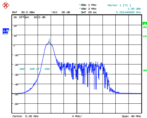
802.11ax20_5260MHz_RU_26/0_Chain 0
