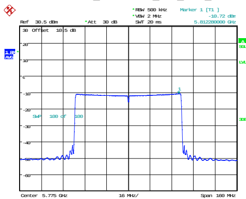
802.11ax80_5775MHz_RU_Full_Chain 0
