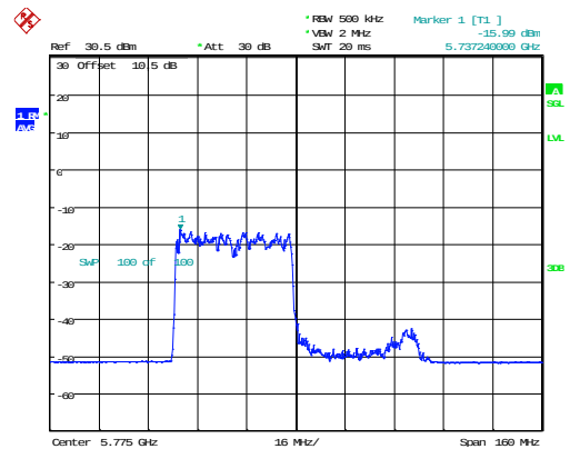
802.11ax80_5775MHz_RU_484/65_Chain 1
