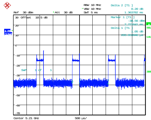
802.11ax80_5210MHz_RU_52/37_Chain 0
