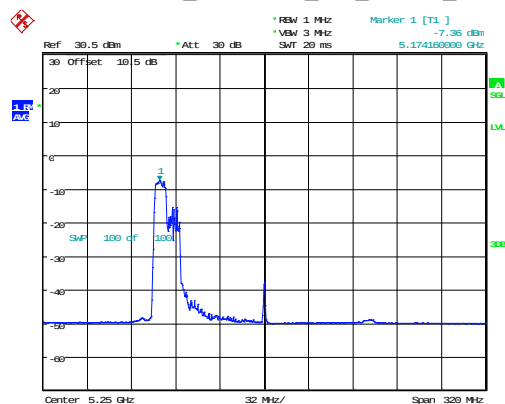
802.11ax160_5250MHz_RU_106/53_Chain 1
