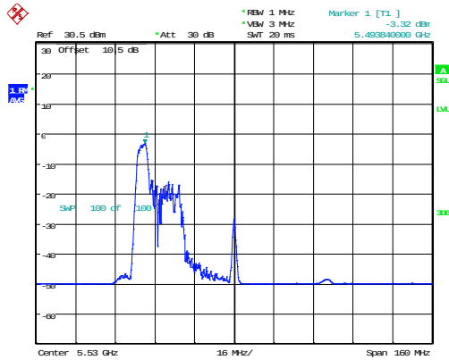
802.11ax80_5530MHz_RU_52/37_Chain 0
