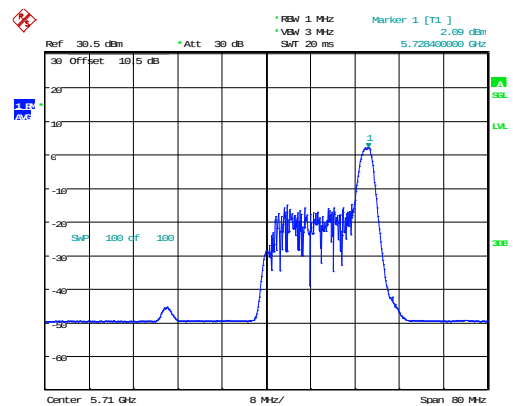
802.11ax40_5710MHz_RU_26/17_Chain 0
