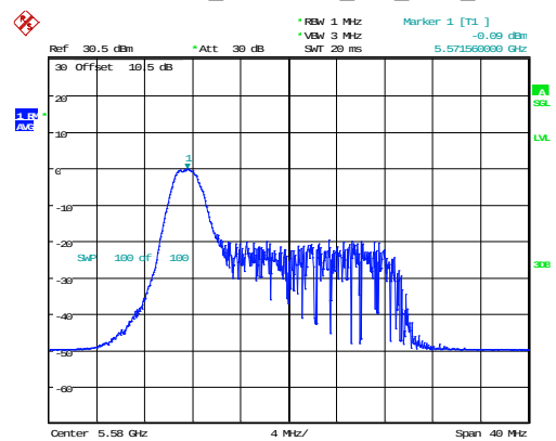
802.11ax20_5580MHz_RU_26/0_Chain 1
