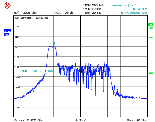
802.11ax20_5785MHz_RU_26/0_Chain 0
