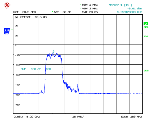
802.11ax80_5290MHz_RU_242/61_Chain 1
