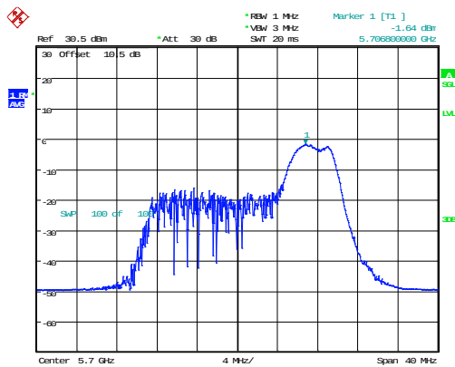
802.11ax20_5700MHz_RU_52/40_Chain 1
