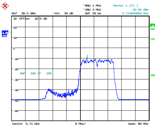
802.11ax40_5710MHz_RU_242/62_Chain 1
