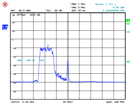
802.11ax80_5290MHz_RU_242/61_Chain 0
