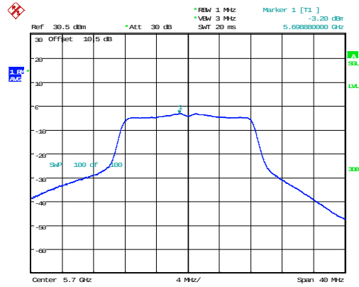
802.11a_5700MHz_Chain 0
