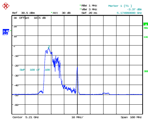
802.11ax80_5210MHz_RU_106/53_Chain 0
