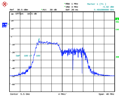
802.11ax20_5500MHz_RU_106/53_Chain 0
