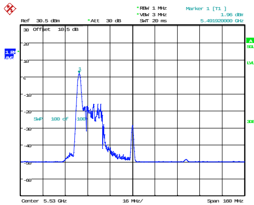
802.11ax80_5530MHz_RU_26/0_Chain 0
