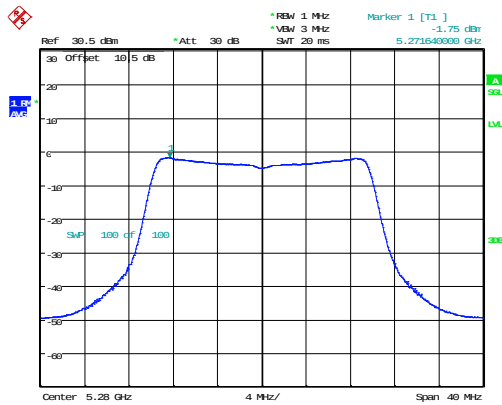
802.11ax20_5280MHz_RU_Full_Chain 1
