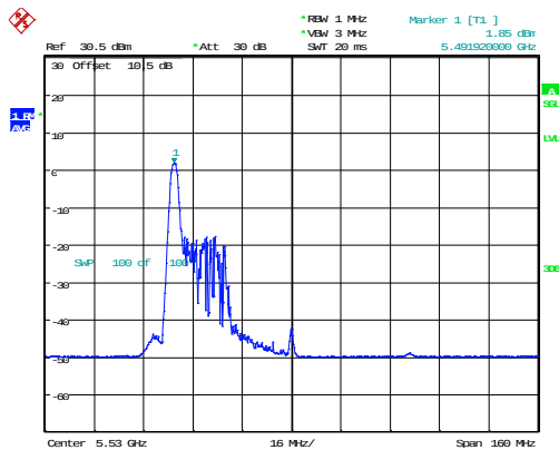
802.11ax80_5530MHz_RU_26/0_Chain 1
