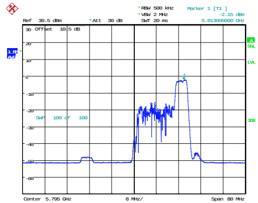
802.11ax40_5795MHz_RU_52/44_Chain 1
