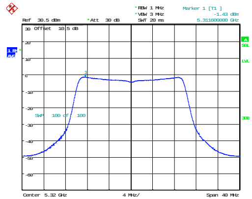
802.11ax20_5320MHz_RU_Full_Chain 1
