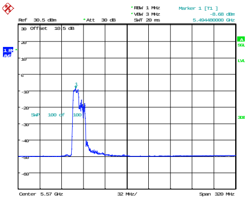
802.11ax160_5570MHz_RU_106/53_Chain 1
