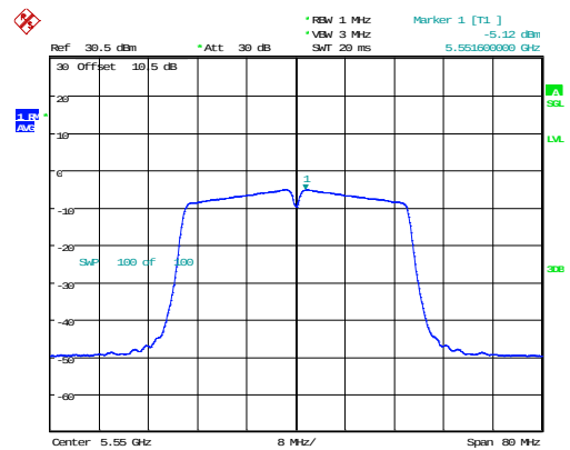
802.11n40_5550MHz_Chain 0
