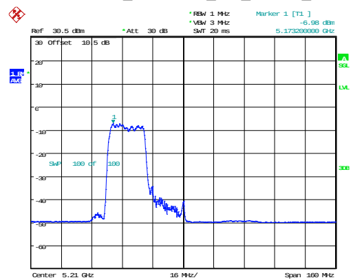
802.11ax80_5210MHz_RU_242/61_Chain 1
