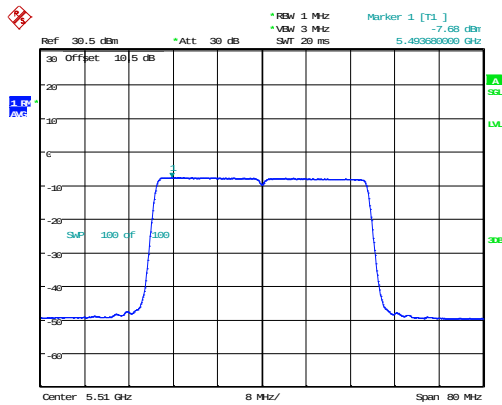
802.11ax40_5510MHz_RU_Full_Chain 1
