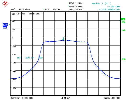
802.11a_5580MHz_Chain 1
