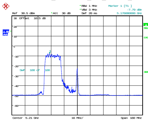
802.11ax80_5210MHz_RU_242/61_Chain 0
