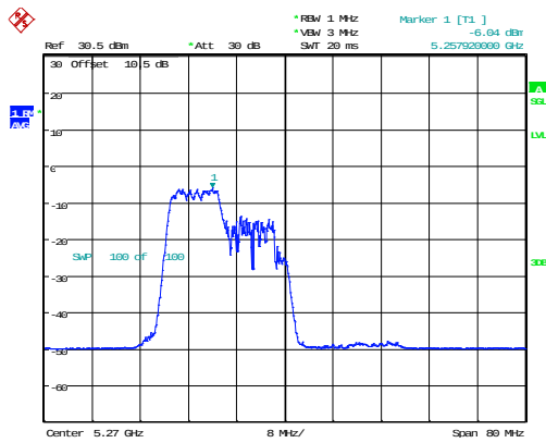
802.11ax40_5270MHz_RU_106/53_Chain 0
