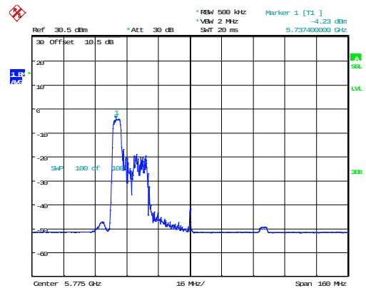
802.11ax80_5775MHz_RU_52/37_Chain 1
