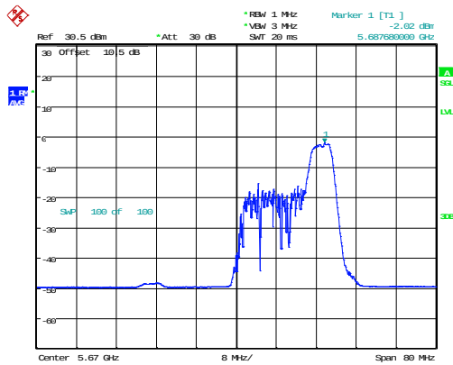
802.11ax40_5670MHz_RU_52/44_Chain 1
