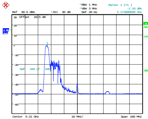
802.11ax80_5210MHz_RU_52/37_Chain 0
