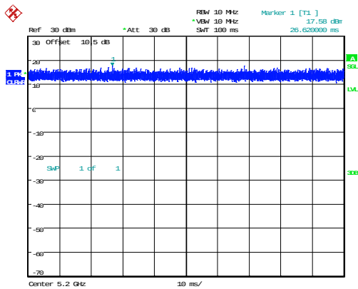
802.11ax20_5200MHz_RU_Full_Chain 0
