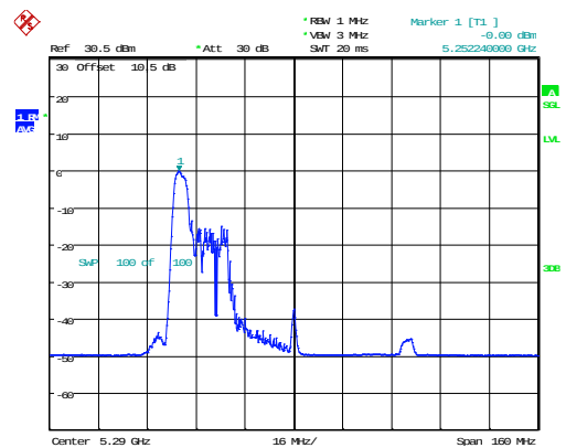
802.11ax80_5290MHz_RU_52/37_Chain 1
