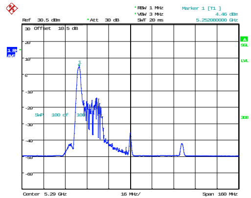
802.11ax80_5290MHz_RU_26/0_Chain 1
