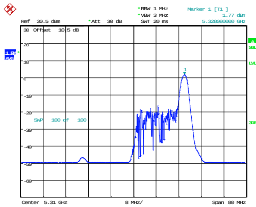
802.11ax40_5310MHz_RU_26/17_Chain 0
