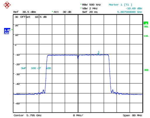
802.11ax40_5795MHz_RU_Full_Chain 1
