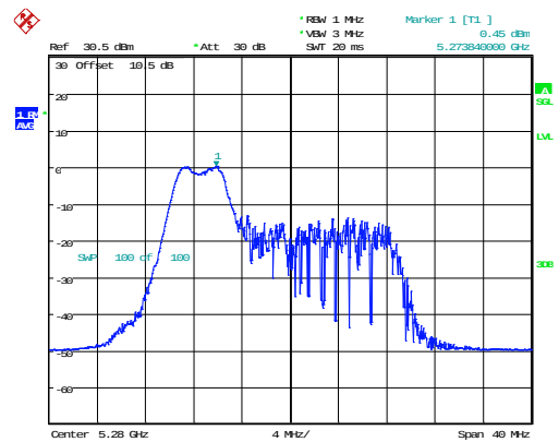
802.11ax20_5280MHz_RU_52/37_Chain 1
