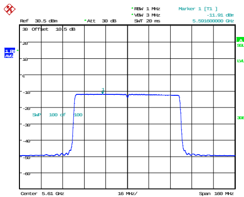
802.11ax80_5610MHz_RU_Full_Chain 1
