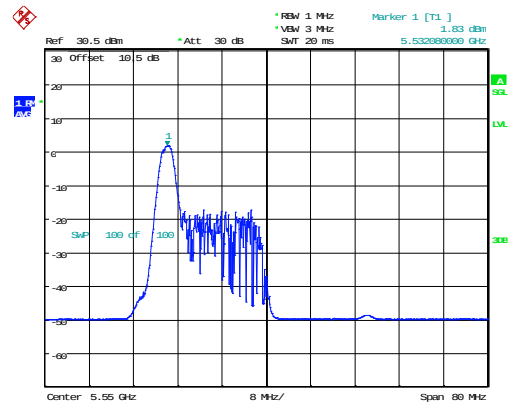
802.11ax40_5550MHz_RU_26/0_Chain 1
