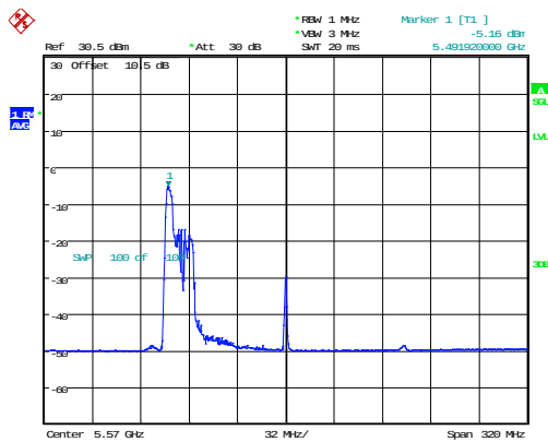
802.11ax160_5570MHz_RU_52/37_Chain 0
