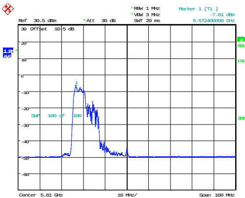
802.11ax80_5610MHz_RU_106/53_Chain 1
