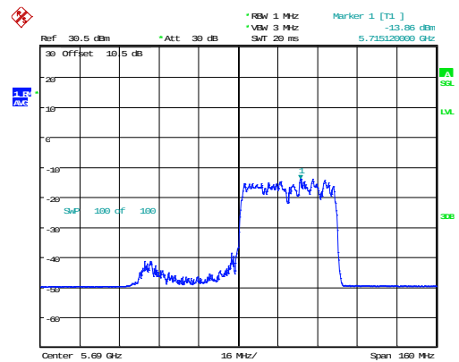
802.11ax80_5690MHz_RU_484/66_Chain 1
