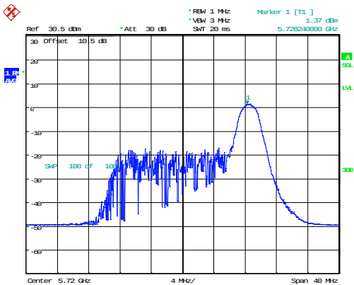
802.11ax20_5720MHz_RU_26/8_Chain 0
