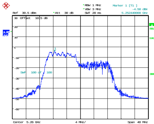
802.11ax20_5260MHz_RU_106/53_Chain 0
