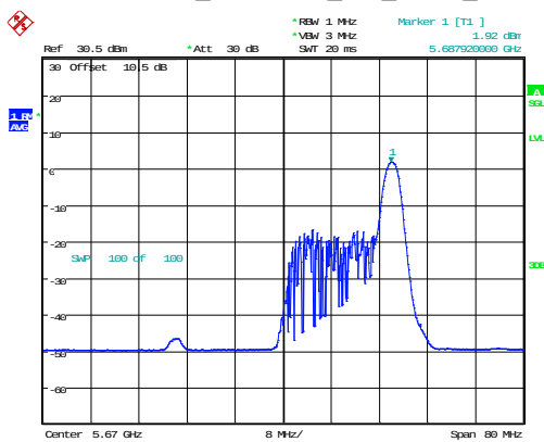
802.11ax40_5670MHz_RU_26/17_Chain 1
