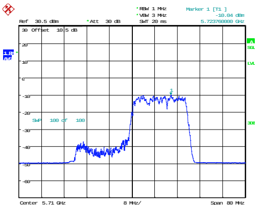
802.11ax40_5710MHz_RU_242/62_Chain 0
