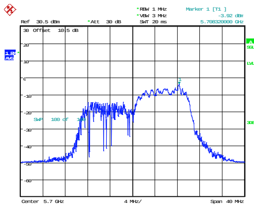
802.11ax20_5700MHz_RU_106/54_Chain 0
