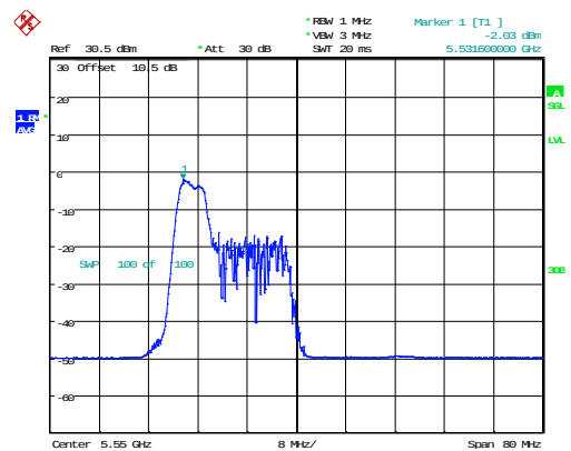
802.11ax40_5550MHz_RU_52/37_Chain 1
