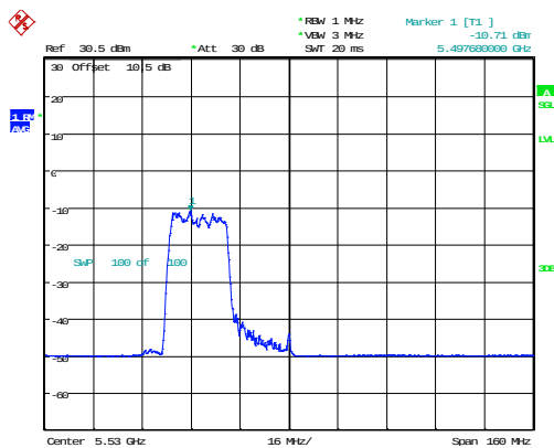
802.11ax80_5530MHz_RU_242/61_Chain 1
