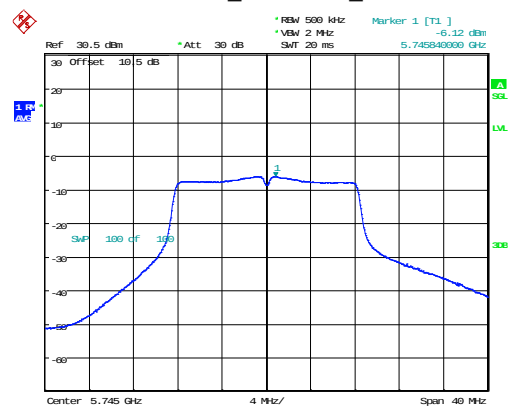
802.11a_5745MHz_Chain 1
