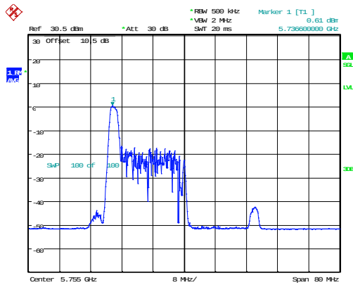
802.11ax40_5755MHz_RU_26/0_Chain 0
