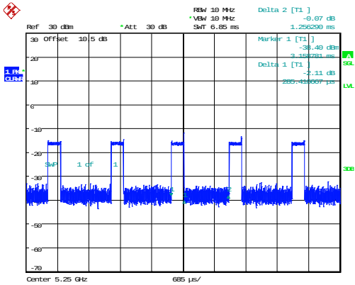
802.11ax160_5250MHz_RU_52/37_Chain 0
