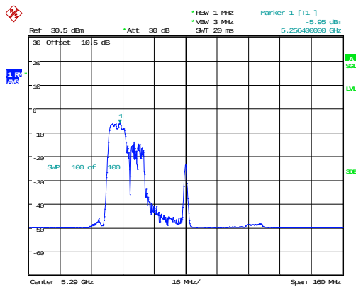
802.11ax80_5290MHz_RU_106/53_Chain 0
