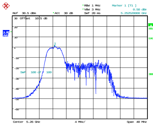
802.11ax20_5260MHz_RU_52/37_Chain 1
