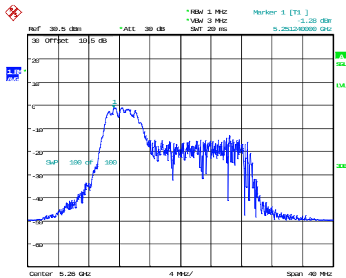
802.11ax20_5260MHz_RU_52/37_Chain 0
