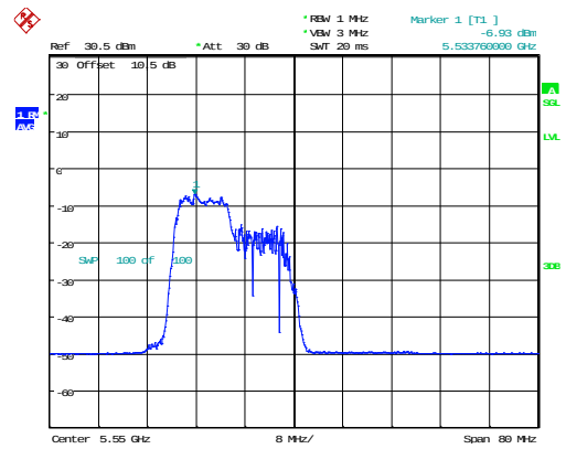
802.11ax40_5550MHz_RU_106/53_Chain 0
