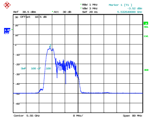
802.11ax40_5550MHz_RU_52/37_Chain 0
