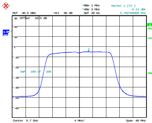
802.11ax20_5700MHz_RU_Full_Chain 1
