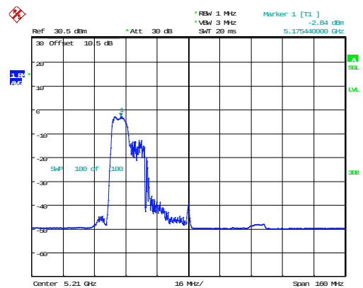
802.11ax80_5210MHz_RU_106/53_Chain 1
