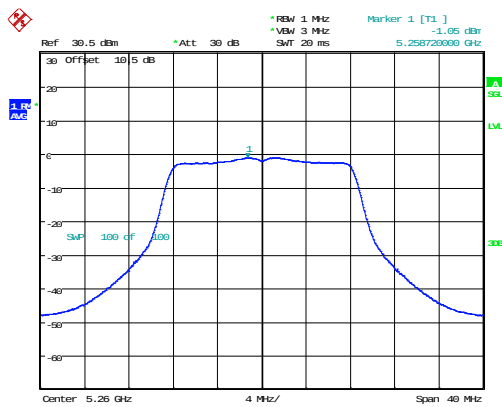
802.11a_5260MHz_Chain 0
