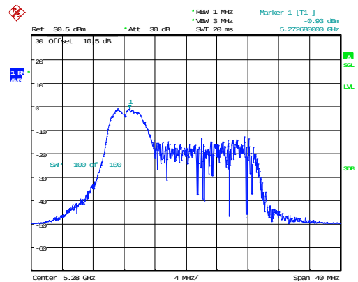
802.11ax20_5280MHz_RU_52/37_Chain 0
