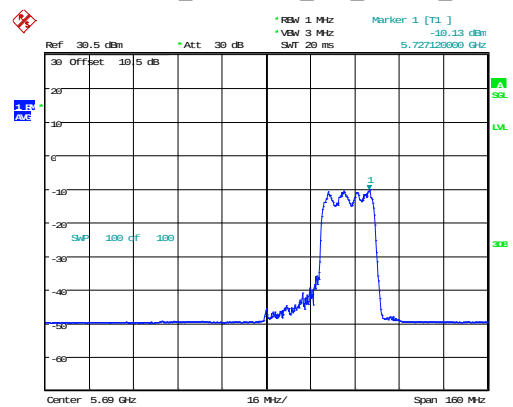
802.11ax80_5690MHz_RU_242/64_Chain 1
