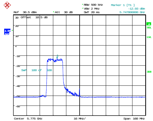
802.11ax80_5775MHz_RU_242/61_Chain 1
