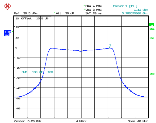
802.11ax20_5280MHz_RU_Full_Chain 0
