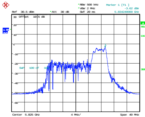
802.11ax20_5825MHz_RU_52/40_Chain 0
