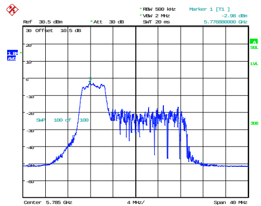
802.11ax20_5785MHz_RU_52/37_Chain 1
