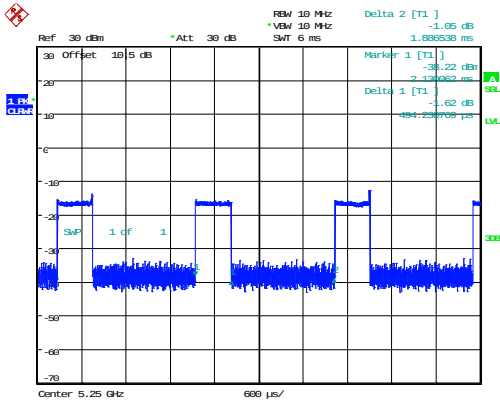
802.11ax160_5250MHz_RU_26/0_Chain 0
