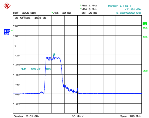
802.11ax80_5610MHz_RU_242/61_Chain 1
