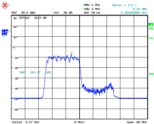
802.11ax40_5270MHz_RU_242/61_Chain 1
