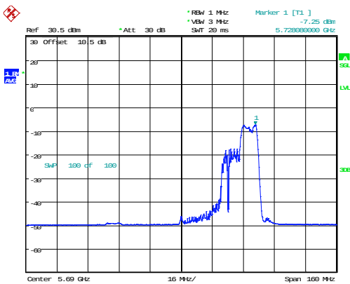
802.11ax80_5690MHz_RU_106/60_Chain 1
