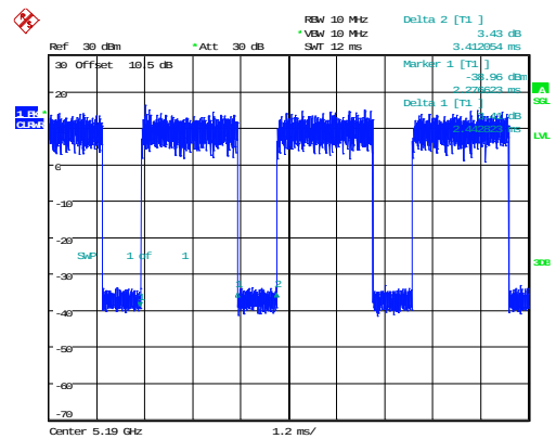
802.11ax40_5190MHz_RU_106/53_Chain 0
