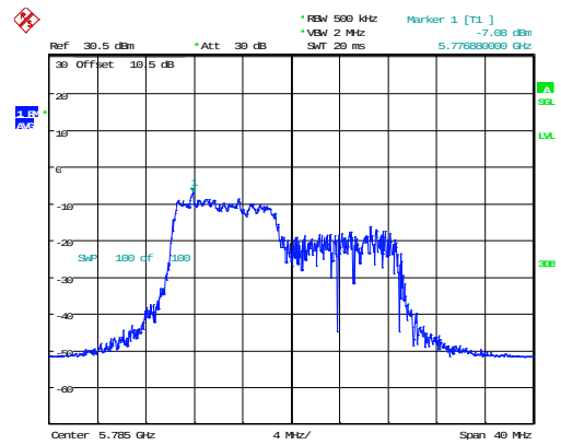
802.11ax20_5785MHz_RU_106/53_Chain 0
