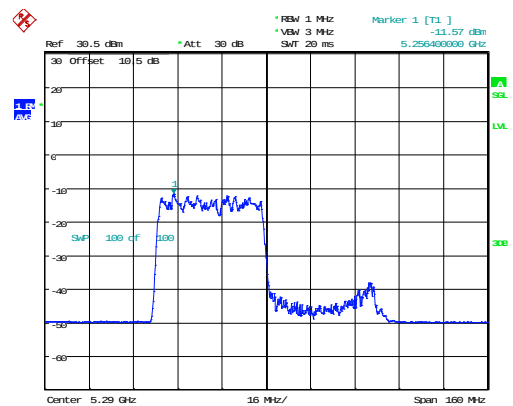
802.11ax80_5290MHz_RU_484/65_Chain 1
