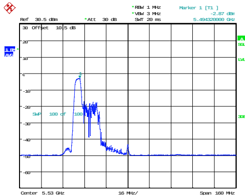
802.11ax80_5530MHz_RU_52/37_Chain 1
