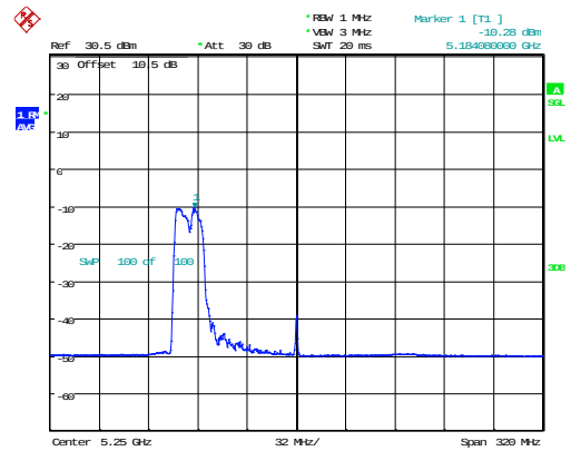
802.11ax160_5250MHz_RU_242/61_Chain 1
