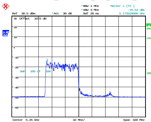
802.11ax160_5250MHz_RU_996/67_Chain 0
