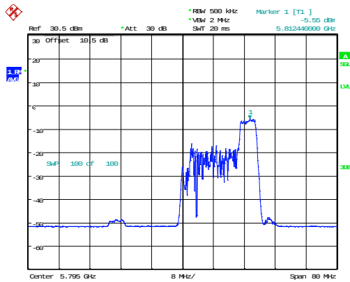
802.11ax40_5795MHz_RU_52/44_Chain 0
