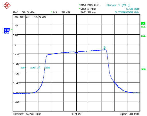
802.11ax20_5745MHz_RU_Full_Chain 1
