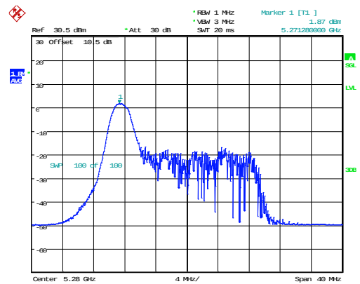
802.11ax20_5280MHz_RU_26/0_Chain 1
