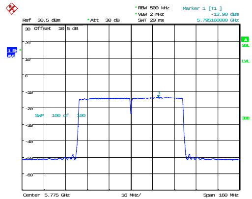
802.11ac80_5775MHz_Chain 1
