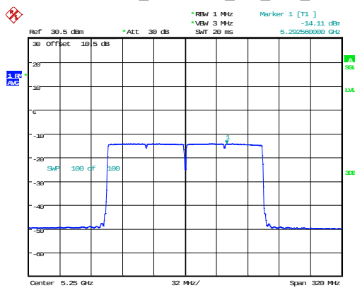
802.11ax160_5250MHz_RU_Full_Chain 0
