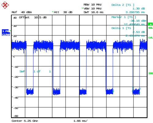
802.11ax160_5250MHz_RU_106/53_Chain 0
