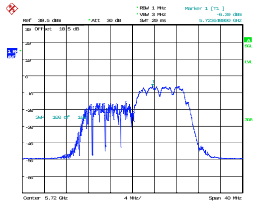
802.11ax20_5720MHz_RU_106/54_Chain 1
