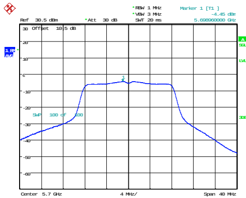
802.11a_5700MHz_Chain 1
