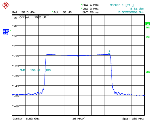
802.11ax80_5530MHz_RU_Full_Chain 0
