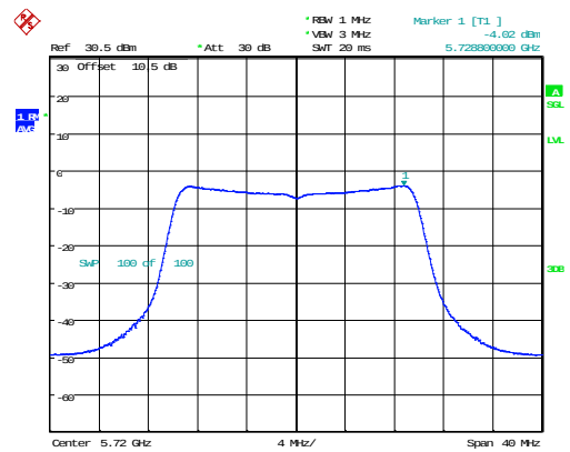
802.11ax20_5720MHz_RU_Full_Chain 1
