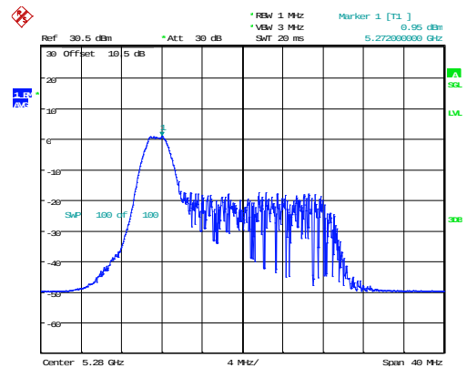
802.11ax20_5280MHz_RU_26/0_Chain 0
