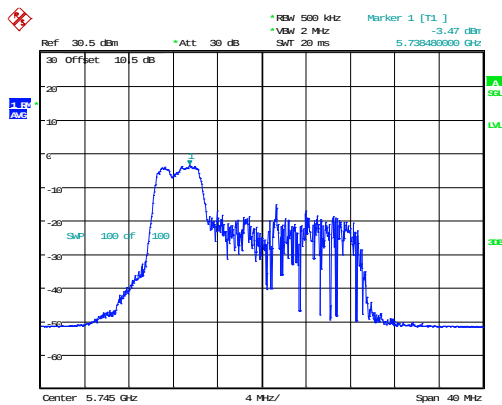
802.11ax20_5745MHz_RU_52/37_Chain 1
