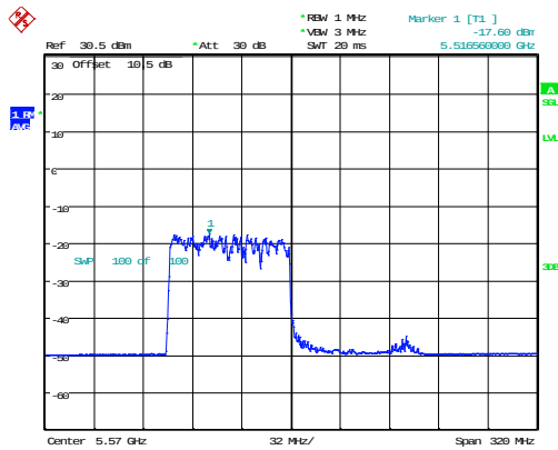
802.11ax160_5570MHz_RU_996/67_Chain 0
