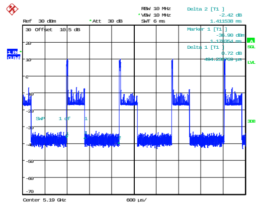
802.11ax40_5190MHz_RU_26/0_Chain 0
