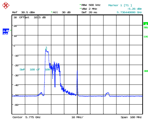
802.11ax80_5775MHz_RU_52/37_Chain 0
