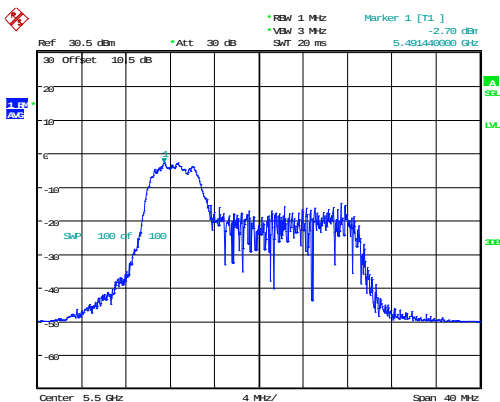
802.11ax20_5500MHz_RU_52/37_Chain 0
