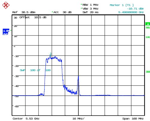
802.11ax80_5530MHz_RU_242/61_Chain 0
