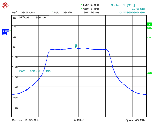
802.11n20_5280MHz_Chain 1
