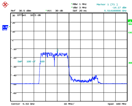
802.11ax80_5530MHz_RU_484/65_Chain 0
