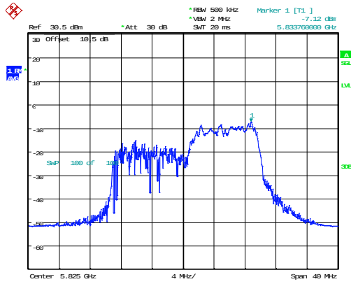
802.11ax20_5825MHz_RU_106/54_Chain 0
