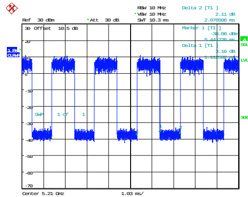
802.11ax80_5210MHz_RU_242/61_Chain 0
