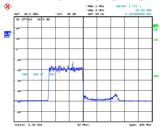
802.11ax160_5250MHz_RU_996/67_Chain 1
