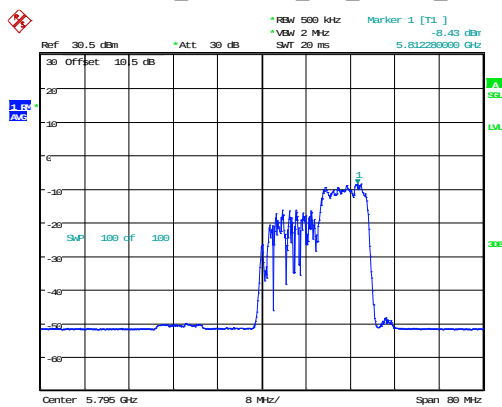
802.11ax40_5795MHz_RU_106/56_Chain 0
