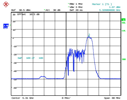
802.11ax40_5310MHz_RU_52/44_Chain 1
