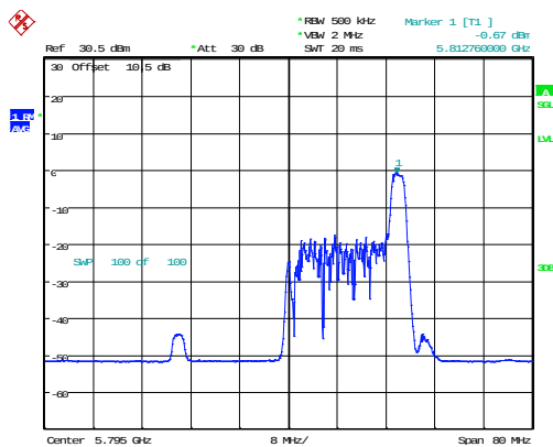
802.11ax40_5795MHz_RU_26/17_Chain 0
