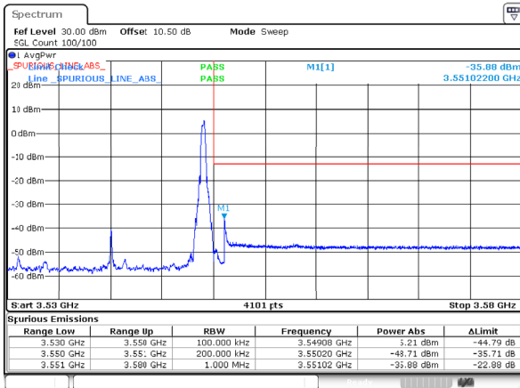
n77_1_20MHz_30kHz_3540MHz_DFT-s-OFDM QPSK_RB1@0
