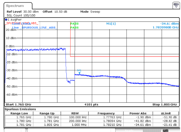
n66_15MHz_15kHz_1772.5MHz_DFT-s-OFDM QPSK_RB75@0
