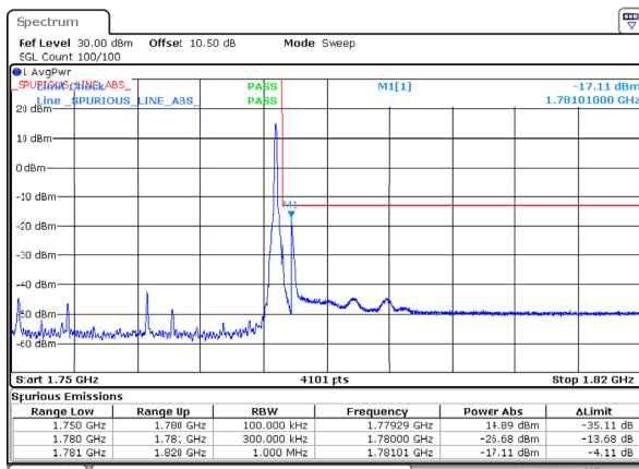
n66_30MHz_15kHz_1765MHz_DFT-s-OFDM QPSK_RB1@159
