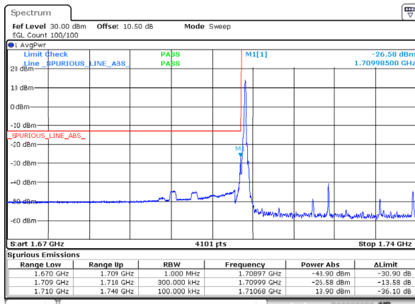
n66_30MHz_15kHz_1725MHz_DFT-s-OFDM QPSK_RB1@0
