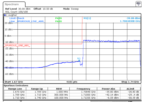
n66_30MHz_15kHz_1725MHz_DFT-s-OFDM QPSK_RB160@0
