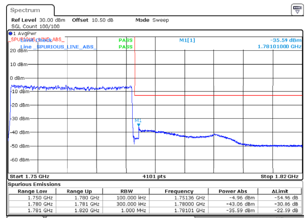
n66_30MHz_15kHz_1765MHz_DFT-s-OFDM QPSK_RB160@0
