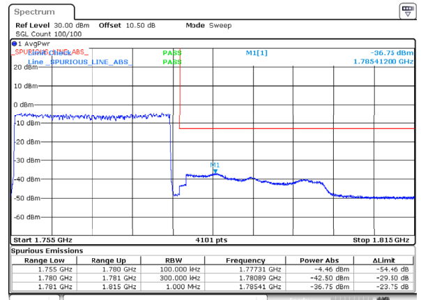
n66_25MHz_15kHz_1767.5MHz_DFT-s-OFDM QPSK_RB128@0
