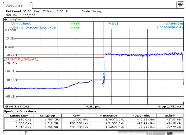
n66_40MHz_15kHz_1730MHz_DFT-s-OFDM QPSK_RB216@0
