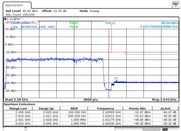
n38_40MHz_30kHz_2600MHz_DFT-s-OFDM QPSK_RB100@0
