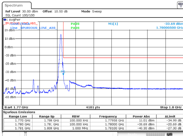
n66_10MHz_15kHz_1775MHz_DFT-s-OFDM QPSK_RB1@51
