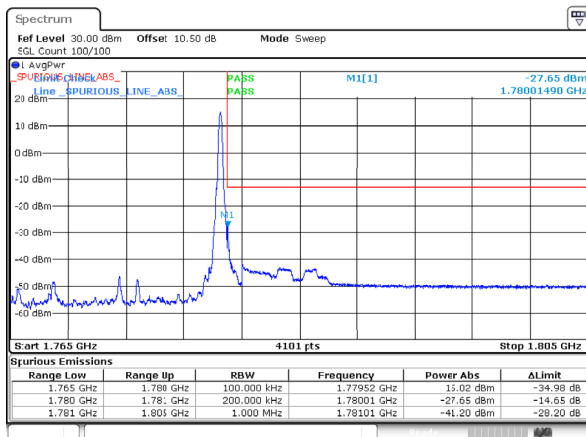
n66_15MHz_15kHz_1772.5MHz_DFT-s-OFDM QPSK_RB1@78
