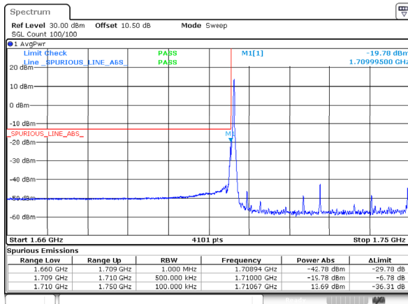
n66_40MHz_15kHz_1730MHz_DFT-s-OFDM QPSK_RB1@0
