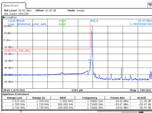
n66_25MHz_15kHz_1722.5MHz_DFT-s-OFDM QPSK_RB1@0
