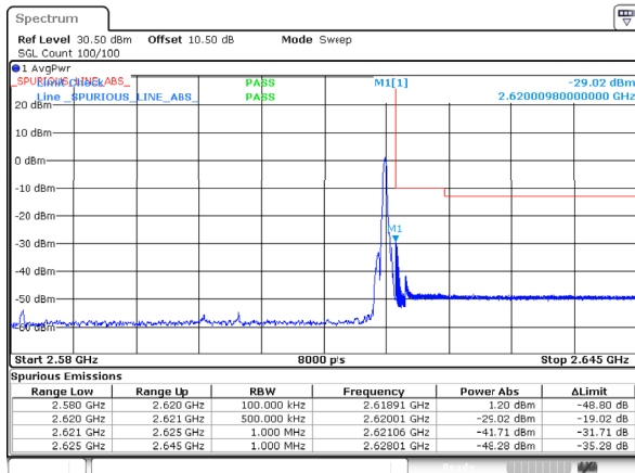
n38_40MHz_30kHz_2600MHz_DFT-s-OFDM QPSK_RB1@105
