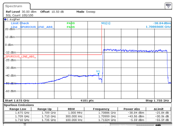
n66_25MHz_15kHz_1722.5MHz_DFT-s-OFDM QPSK_RB128@0
