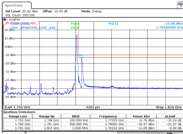
n66_25MHz_15kHz_1767.5MHz_DFT-s-OFDM QPSK_RB1@132
