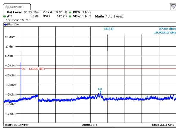
n78_1_80MHz_30kHz_3500MHz_DFT-s-OFDM QPSK_RB216@0 -37.82dBm
