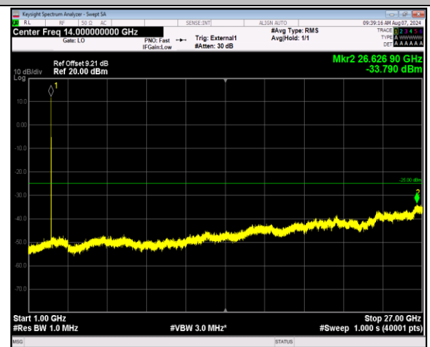
41-41-20MHz-10MHz-16QAM-16QAM-39750-39894-1RB#0 -1RB#49-1000~27000MHz-PASS
