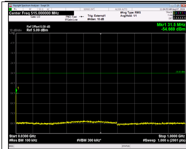
41-41-20MHz-20MHz-QPSK-QPSK-40521-40719-1RB#9 9-ORB#0-30~1000MHz-PASS
