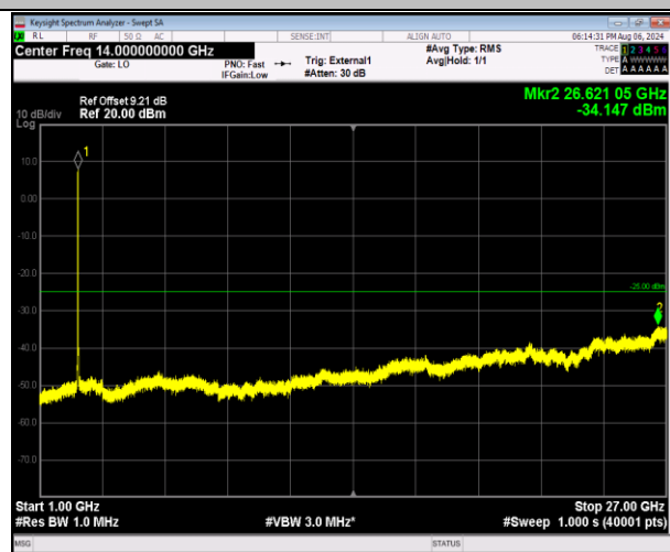
41-41-20MHz-5MHz-16QAM-16QAM-40595-40712-100RB# 0-25RB#0-1000~27000MHz-PASS
