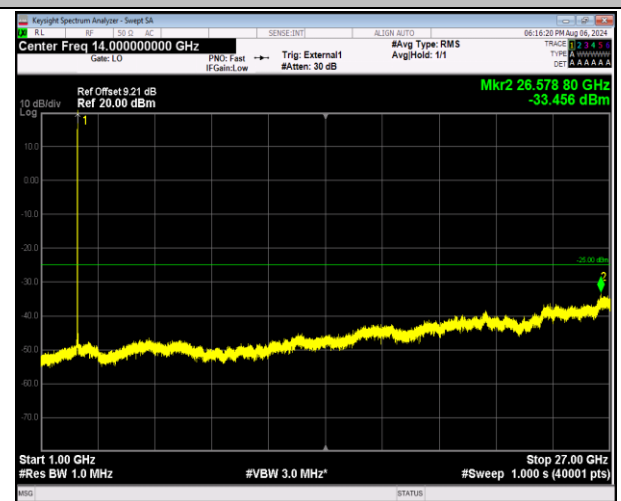
41-41-20MHz-5MHz-16QAM-16QAM-41440-41557-1RB#0-ORB#0-1000~27000MHz-PASS
