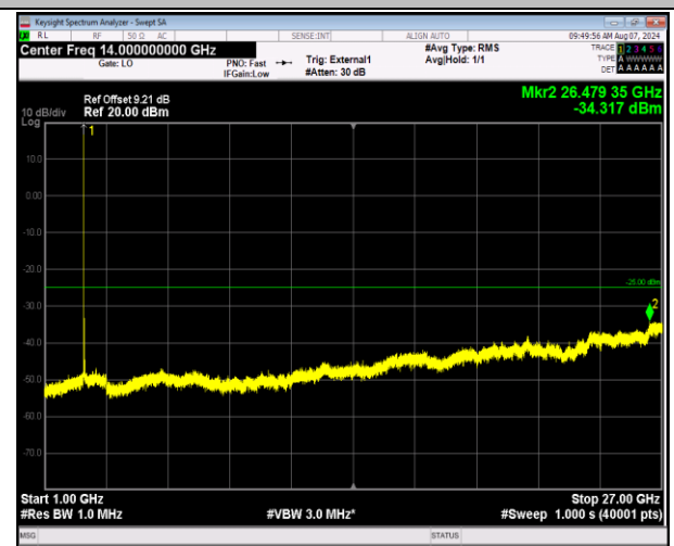
41-41-20MHz-10MHz-16QAM-16QAM-41391-41535-1RB#0 -ORB#0-1000~27000MHz-PASS
