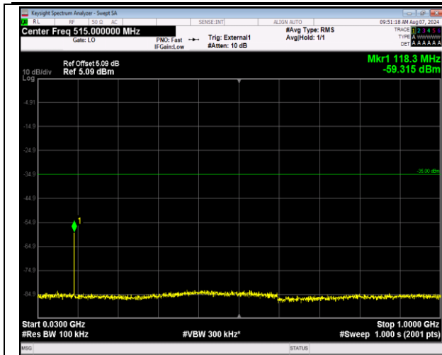
41-41-20MHz-10MHz-16QAM-16QAM-41391-41535-1RB #99-ORB#0-30~1000MHz-PASS
