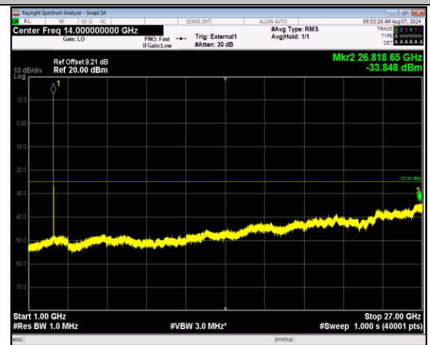
41-41-20MHz-10MHz-16QAM-16QAM-41391-41535-1RB#0 -1RB#49-1000~27000MHz-PASS
