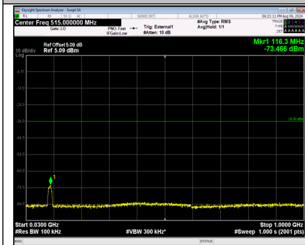
41-41-20MHz-5MHz-16QAM-16QAM-41440-41557-100RB# 0-25RB#0-30~1000MHz-PASS
