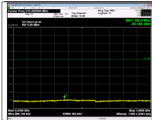
41-41-20MHz-20MHz-16QAM-16QAM-39750-39948-100 RB#0-100RB#0-30~1000MHz-PASS
