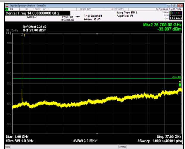
41-41-20MHz-20MHz-16QAM-16QAM-39750-39948-1RB#9 9-ORB#0-1000~27000MHz-PASS
