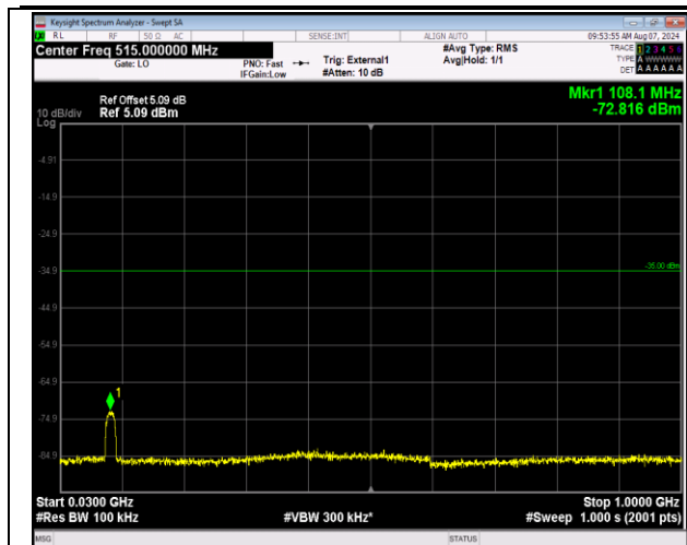
41-41-20MHz-10MHz-QPSK-QPSK-41391-41535-100RB #0-50RB#0-30~1000MHz-PASS
