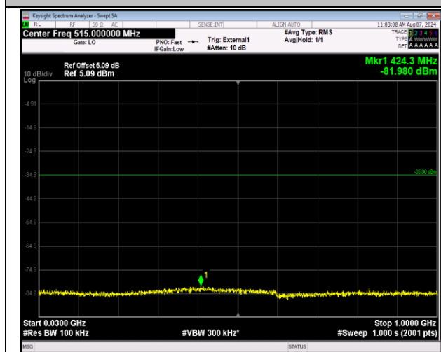
41-41-20MHz-20MHz-QPSK-QPSK-40521-40719-1RB#0-0RB#0-30~1000MHz-PASS
