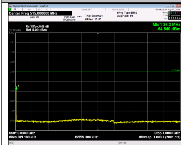
41-41-20MHz-10MHz-16QAM-16QAM-40571-40715-1RB #99-ORB#0-30~1000MHz-PASS
