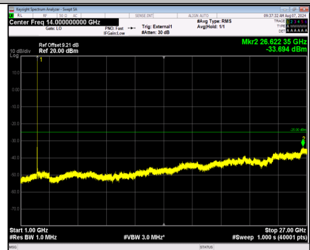
41-41-20MHz-10MHz-16QAM-16QAM-39750-39894-1RB#9 9-ORB#0-1000~27000MHz-PASS
