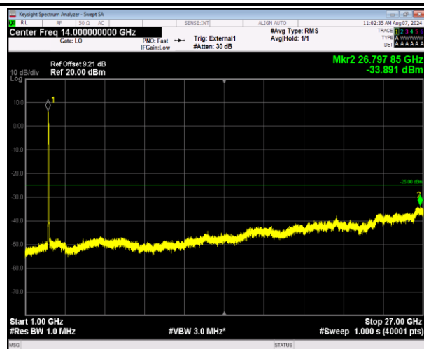
41-41-20MHz-20MHz-16QAM-16QAM-39750-39948-100RB #0-100RB#0-1000~27000MHz-PASS
