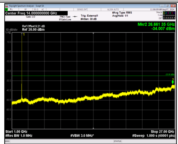
41-41-20MHz-20MHz-16QAM-16QAM-40521-40719-1RB#9 9-ORB#0-1000~27000MHz-PASS
