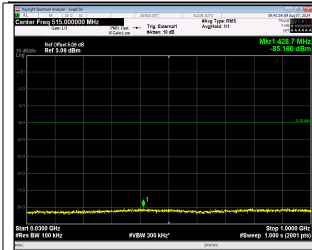
41-41-20MHz-10MHz-16QAM-16QAM-40571-40715-1RB #0-1RB#49-30~1000MHz-PASS
