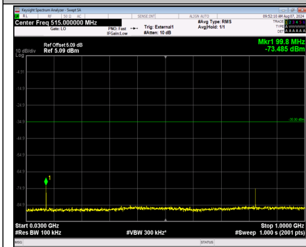
41-41-20MHz-10MHz-QPSK-QPSK-41391-41535-1RB#0 -1RB#49-30~1000MHz-PASS
