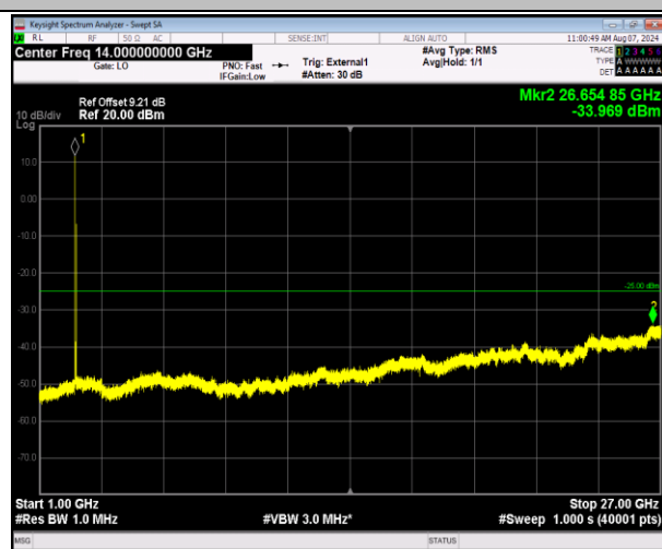
41-41-20MHz-20MHz-16QAM-16QAM-39750-39948-1RB#0-1RB#99-1000~27000MHz-PASS
