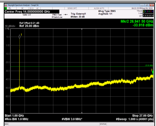
41-41-20MHz-5MHz-16QAM-16QAM-41440-41557-100RB# 0-25RB#0-1000~27000MHz-PASS
