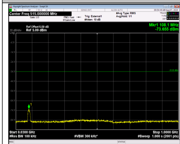
41-41-20MHz-10MHz-16QAM-16QAM-41391-41535-100 RB#0-50RB#0-30~1000MHz-PASS
