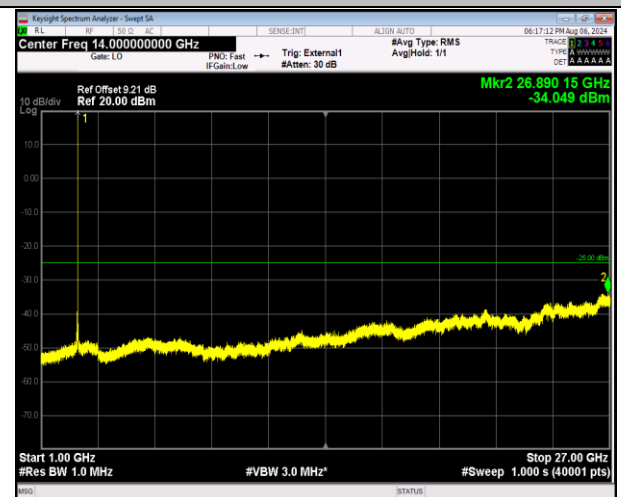
41-41-20MHz-5MHz-QPSK-QPSK-41440-41557-1RB#99-ORB#0-1000~27000MHz-PASS
