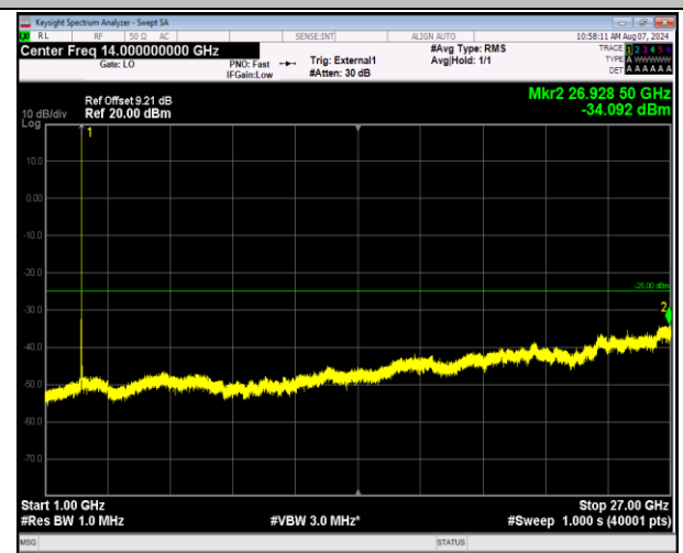
41-41-20MHz-20MHz-QPSK-QPSK-39750-39948-1RB#99- ORB#0-1000~27000MHz-PASS
