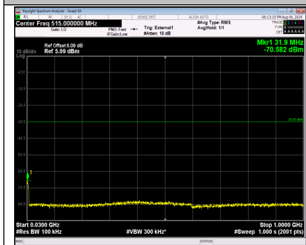
41-41-20MHz-5MHz-QPSK-QPSK-40595-40712-100RB# 0-25RB#0-30~1000MHz-PASS
