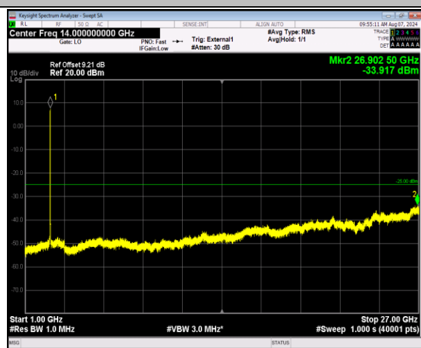
41-41-20MHz-10MHz-16QAM-16QAM-41391-41535-100RB #0-50RB#0-1000~27000MHz-PASS
