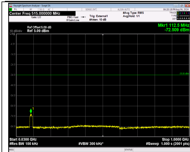
41-41-20MHz-5MHz-QPSK-QPSK-41440-41557-100RB# 0-25RB#0-30~1000MHz-PASS
