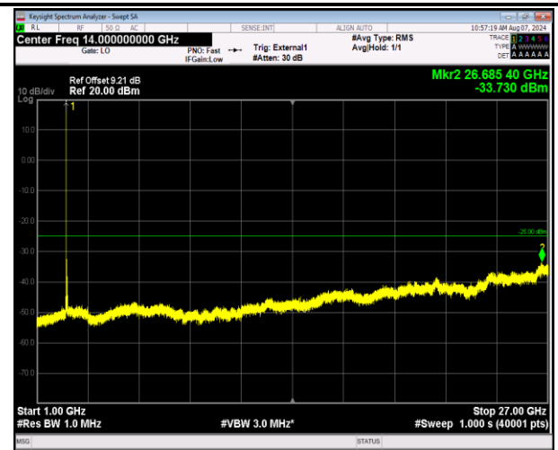
41-41-20MHz-20MHz-16QAM-16QAM-39750-39948-1RB#0 -ORB#0-1000~27000MHz-PASS
