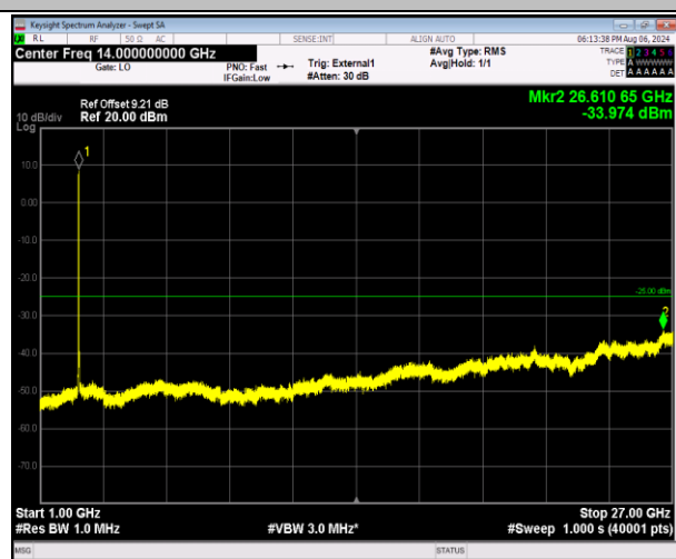
41-41-20MHz-5MHz-QPSK-QPSK-40595-40712-100RB#0- 25RB#0-1000~27000MHz-PASS
