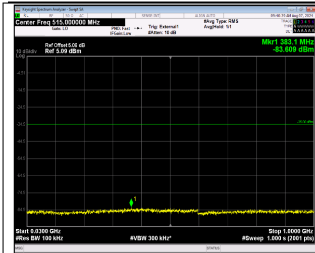
41-41-20MHz-10MHz-16QAM-16QAM-39750-39894-100 RB#0-50RB#0-30~1000MHz-PASS
