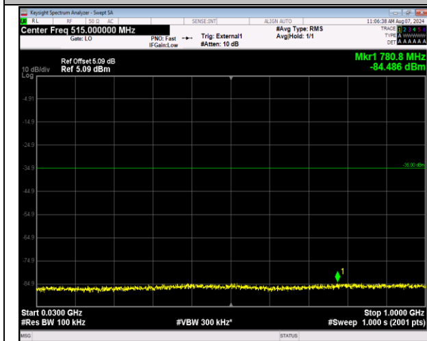
41-41-20MHz-20MHz-QPSK-QPSK-40521-40719-1RB#0 -1RB#99-30~1000MHz-PASS
