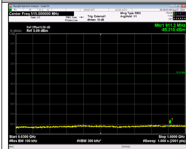
41-41-20MHz-10MHz-16QAM-16QAM-39750-39894-1RB #0-1RB#49-30~1000MHz-PASS
