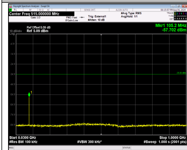
41-41-20MHz-5MHz-16QAM-16QAM-41440-41557-1RB#0-ORB#0-30~1000MHz-PASS
