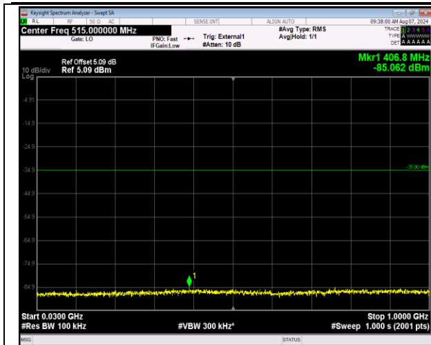
41-41-20MHz-10MHz-QPSK-QPSK-39750-39894-1RB#0 -1RB#49-30~1000MHz-PASS
