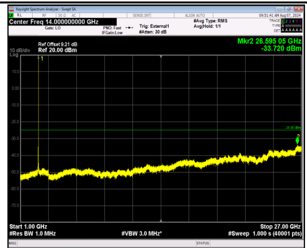
41-41-20MHz-10MHz-16QAM-16QAM-41391-41535-1RB#9 9-ORB#0-1000~27000MHz-PASS
