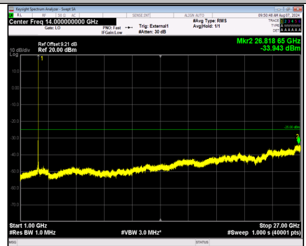
41-41-20MHz-10MHz-QPSK-QPSK-41391-41535-1RB#99- ORB#0-1000~27000MHz-PASS
