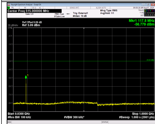
41-41-20MHz-10MHz-QPSK-QPSK-41391-41535-1RB#9 9-ORB#0-30~1000MHz-PASS
