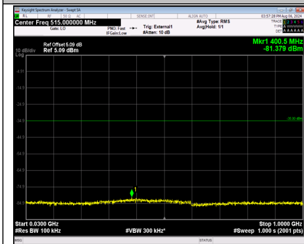
41-41-5MHz-20MHz-QPSK-QPSK-40528-40645-1RB#0-0RB#0-30~1000MHz-PASS
