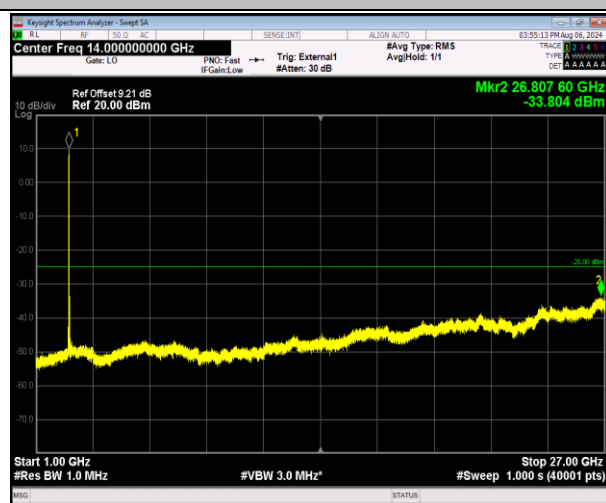
41-41-5MHz-20MHz-16QAM-16QAM-39683-39800-1RB#0-1RB#99-1000~27000MHz-PASS
