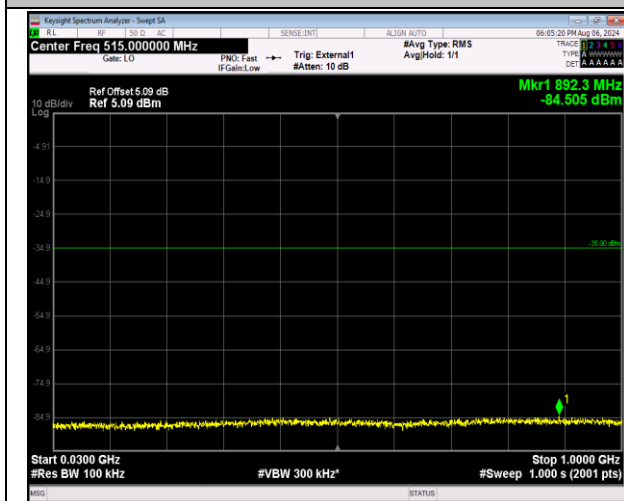
41-41-20MHz-5MHz-16QAM-16QAM-39750-39867-1RB#0-1RB#24-30~1000MHz-PASS
