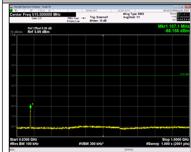
41-41-5MHz-20MHz-16QAM-16QAM-41373-41490-25RB#0 #0-100RB#0-30~1000MHz-PASS
