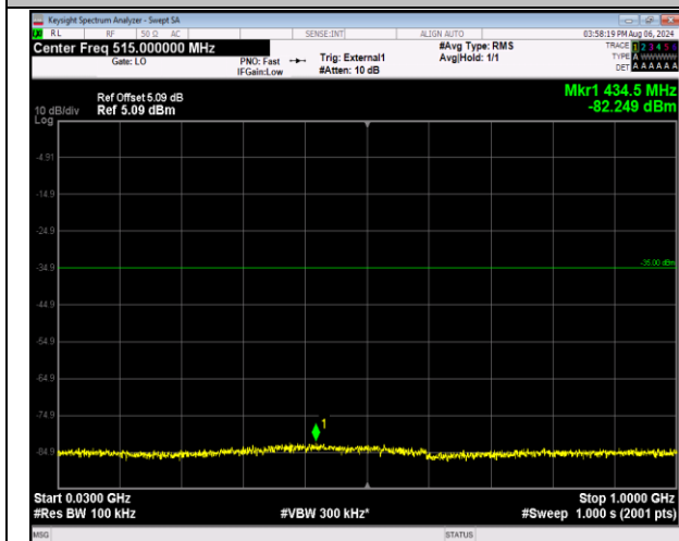
41-41-5MHz-20MHz-16QAM-16QAM-40528-40645-1RB#0-0RB#0-30~1000MHz-PASS
