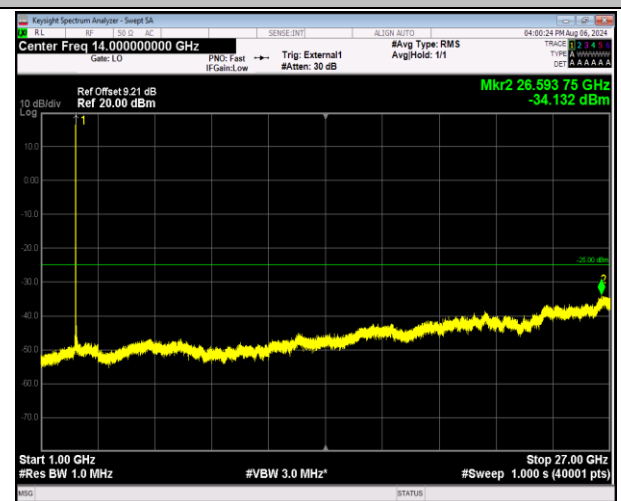
41-41-5MHz-20MHz-16QAM-16QAM-40528-40645-1RB#24 -ORB#0-1000~27000MHz-PASS
