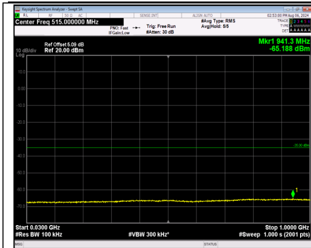
7-7-20MHz-20MHz-16QAM-16QAM-21152-21350-1RB#9 9-ORB#0-30~1000MHz-PASS
