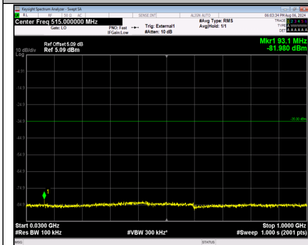
41-41-20MHz-5MHz-16QAM-16QAM-39750-39867-1RB# 99-ORB#0-30~1000MHz-PASS
