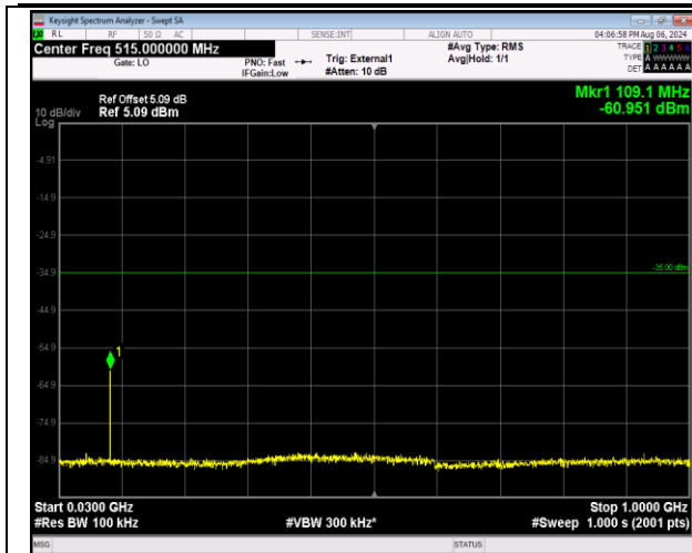
41-41-5MHz-20MHz-16QAM-16QAM-41373-41490-1RB# 24-ORB#0-30~1000MHz-PASS
