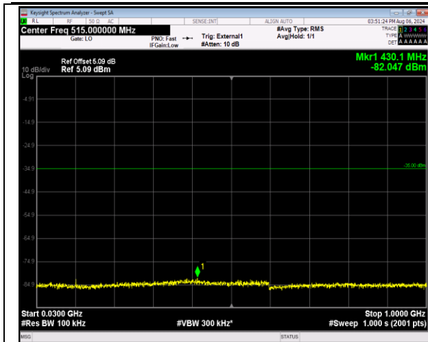
41-41-5MHz-20MHz-16QAM-16QAM-39683-39800-1RB# 0-ORB#0-30~1000MHz-PASS
