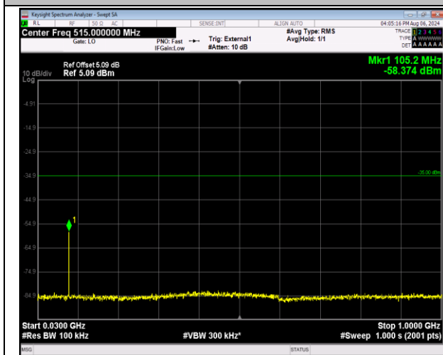
41-41-5MHz-20MHz-16QAM-16QAM-41373-41490-1RB#- 0-ORB#0-30~1000MHz-PASS
