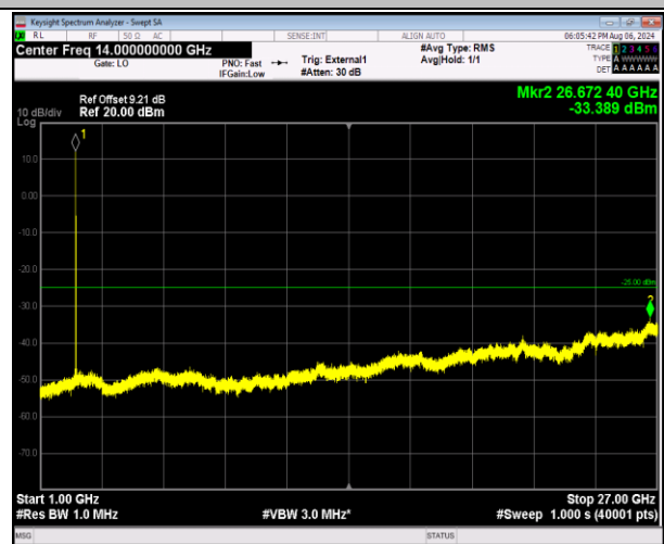
41-41-20MHz-5MHz-16QAM-16QAM-39750-39867-1RB#0-1RB#24-1000~27000MHz-PASS
