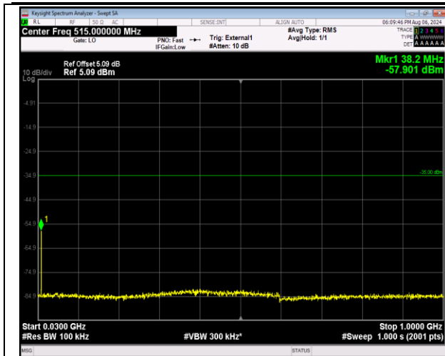
41-41-20MHz-5MHz-QPSK-QPSK-40595-40712-1RB#99 -ORB#0-30~1000MHz-PASS
