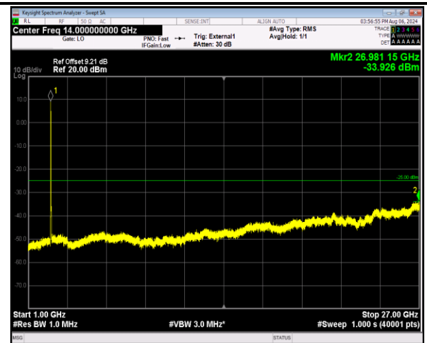
41-41-5MHz-20MHz-16QAM-16QAM-39683-39800-25RB#0-100RB#0-1000~27000MHz-PASS
