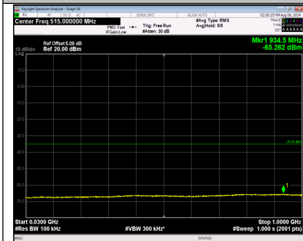
7-7-20MHz-20MHz-16QAM-16QAM-21001-21199-100RB #0-100RB#0-30~1000MHz-PASS
