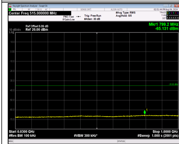
7-7-20MHz-20MHz-16QAM-16QAM-21152-21350-1RB#0 -ORB#0-30~1000MHz-PASS
