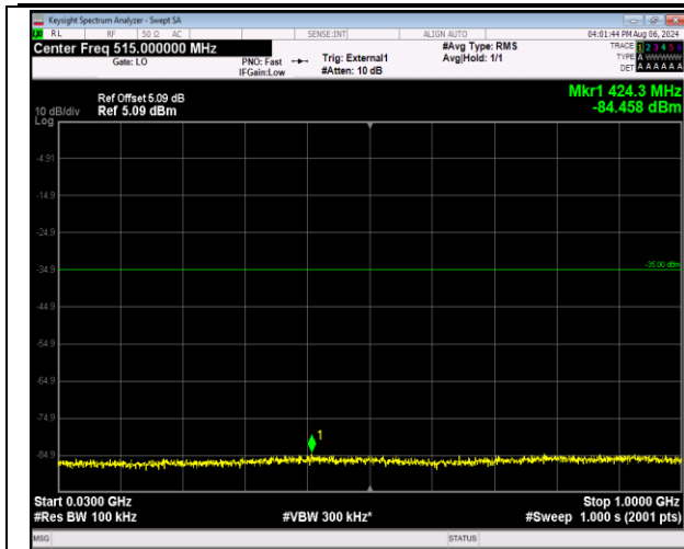
41-41-5MHz-20MHz-16QAM-16QAM-40528-40645-1RB# 0-1RB#99-30~1000MHz-PASS
