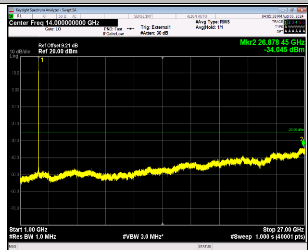
41-41-5MHz-20MHz-16QAM-16QAM-41373-41490-1RB#0- ORB#0-1000~27000MHz-PASS
