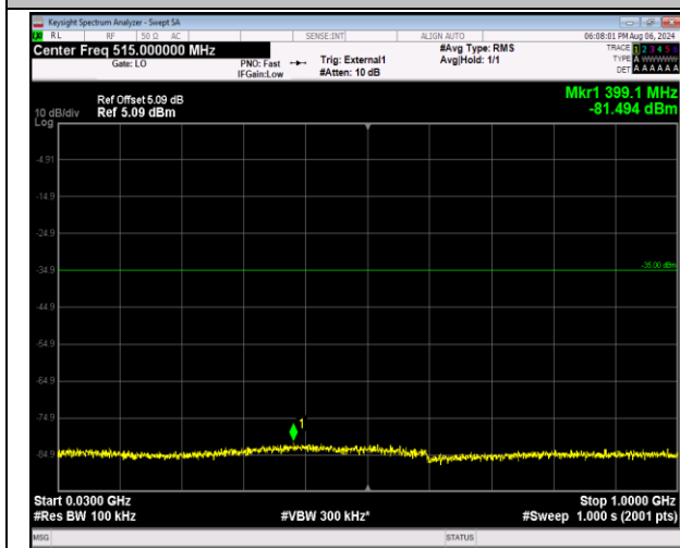
41-41-20MHz-5MHz-QPSK-QPSK-40595-40712-1RB#0-0RB#0-30~1000MHz-PASS
