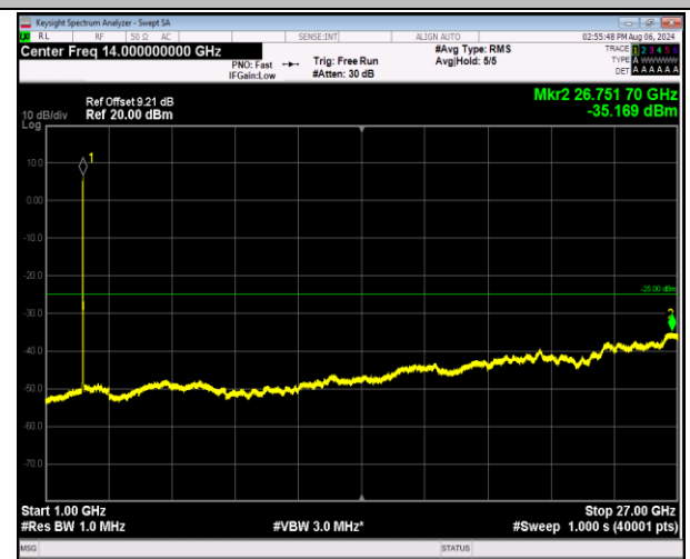
7-7-20MHz-20MHz-16QAM-16QAM-21152-21350-100RB#0 -100RB#0-1000~27000MHz-PASS
