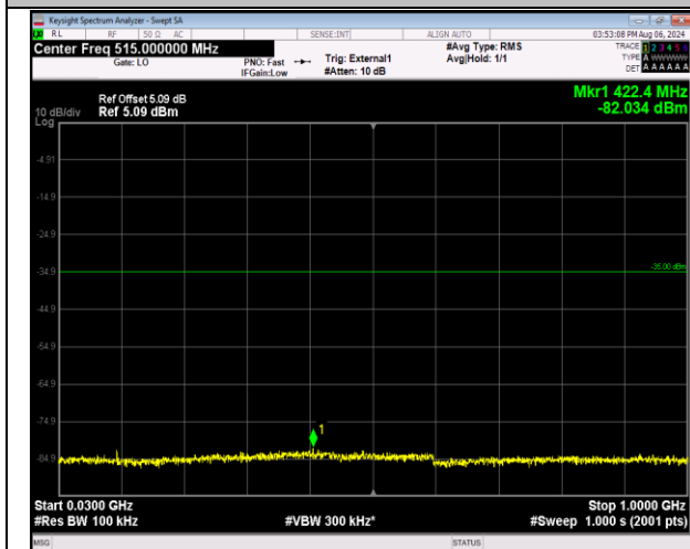
41-41-5MHz-20MHz-16QAM-16QAM-39683-39800-1RB# 24-ORB#0-30~1000MHz-PASS
