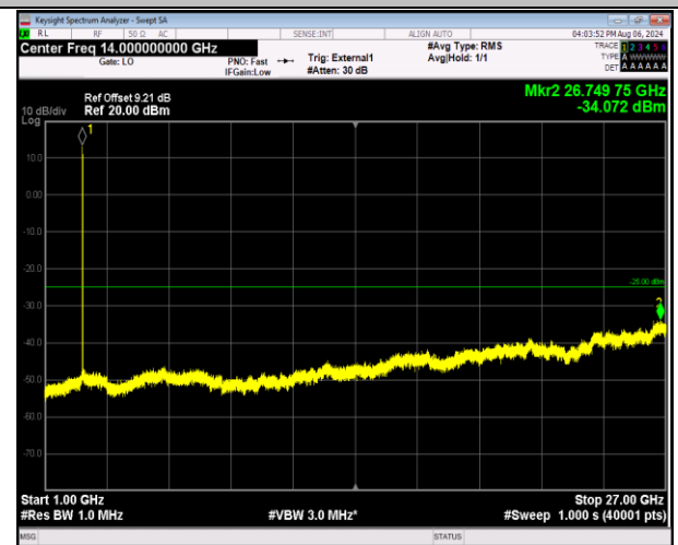
41-41-5MHz-20MHz-16QAM-16QAM-40528-40645-25RB#0 -100RB#0-1000~27000MHz-PASS
