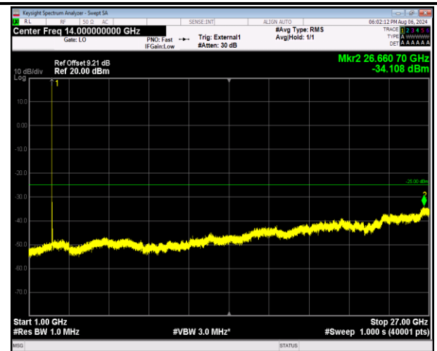
41-41-20MHz-5MHz-16QAM-16QAM-39750-39867-1RB#0- ORB#0-1000~27000MHz-PASS
