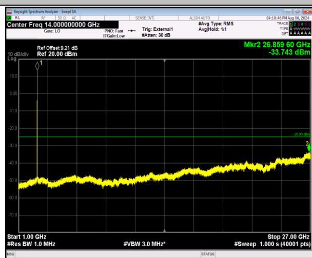
41-41-5MHz-20MHz-16QAM-16QAM-41373-41490-25RB#0 -100RB#0-1000~27000MHz-PASS
