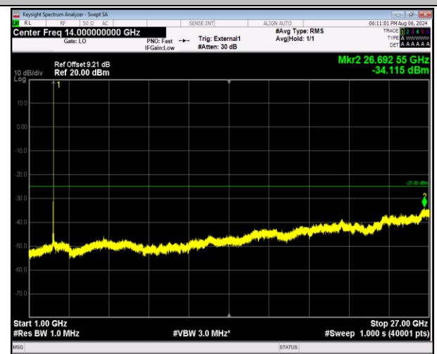
41-41-20MHz-5MHz-16QAM-16QAM-40595-40712-1RB#99-0RB#0-1000~27000MHz-PASS
