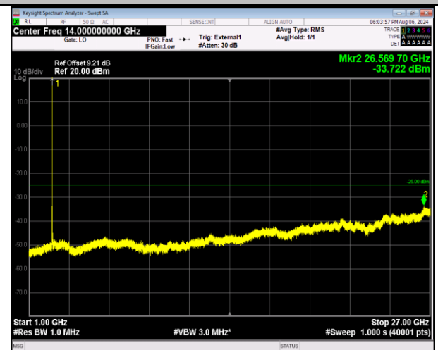
41-41-20MHz-5MHz-16QAM-16QAM-39750-39867-1RB#99 -ORB#0-1000~27000MHz-PASS
