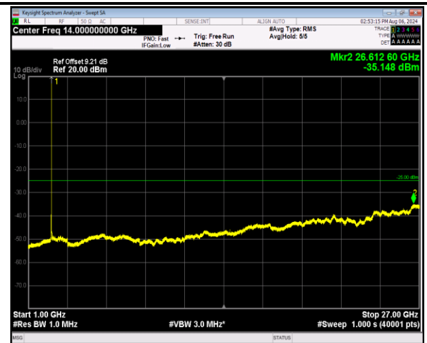
7-7-20MHz-20MHz-16QAM-16QAM-21152-21350-1RB#99- ORB#0-1000~27000MHz-PASS
