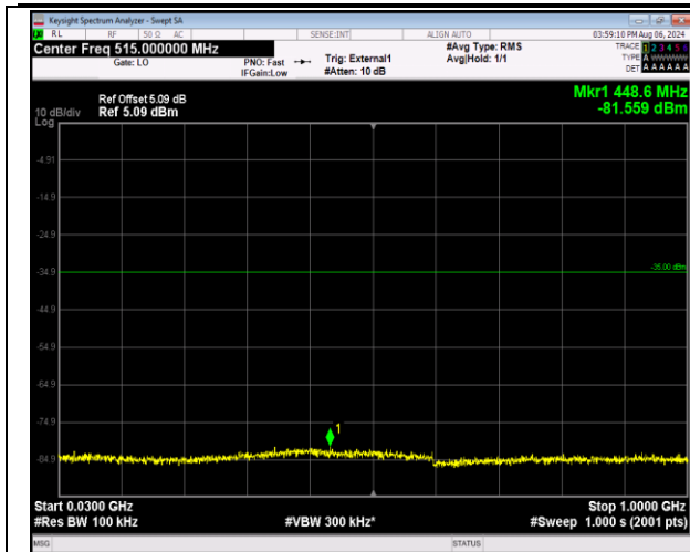
41-41-5MHz-20MHz-QPSK-QPSK-40528-40645-1RB#24 -ORB#0-30~1000MHz-PASS
