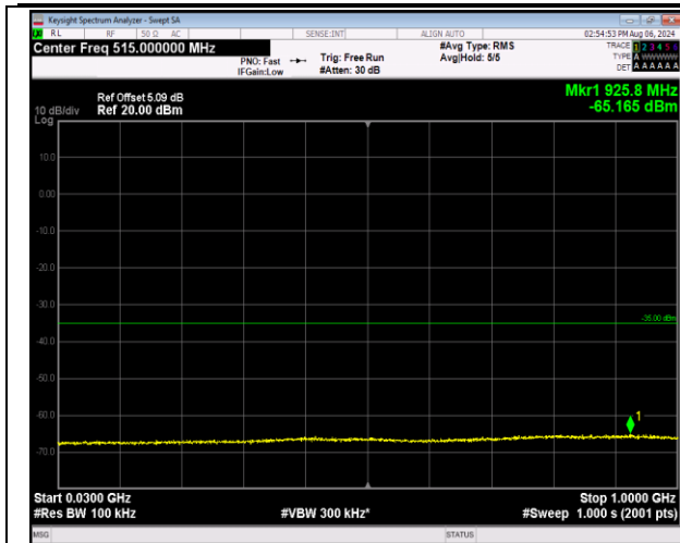
7-7-20MHz-20MHz-QPSK-QPSK-21152-21350-100RB#0 -100RB#0-30~1000MHz-PASS
