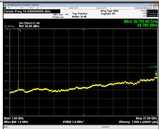
7-7-20MHz-20MHz-QPSK-QPSK-21152-21350-1RB#99-0R B#0-1000~27000MHz-PASS
