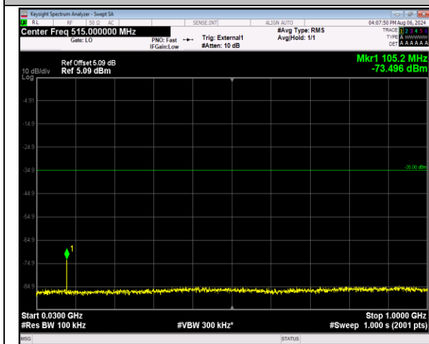
41-41-5MHz-20MHz-QPSK-QPSK-41373-41490-1RB#0-1RB#99-30~1000MHz-PASS
