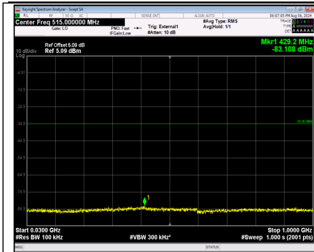
41-41-20MHz-5MHz-16QAM-16QAM-39750-39867-100R B#0-25RB#0-30~1000MHz-PASS
