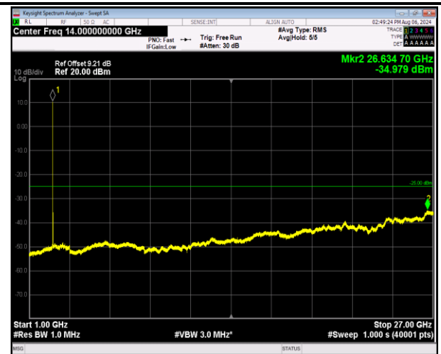
7-7-20MHz-20MHz-16QAM-16QAM-21001-21199-1RB#0-1 RB#99-1000~27000MHz-PASS
