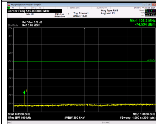
41-41-5MHz-20MHz-16QAM-16QAM-41373-41490-1RB#0-1RB#99-30~1000MHz-PASS
