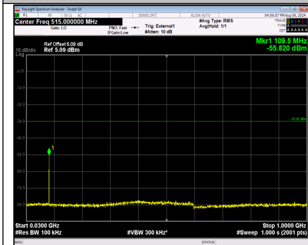
41-41-5MHz-20MHz-QPSK-QPSK-41373-41490-1RB#24 -ORB#0-30~1000MHz-PASS
