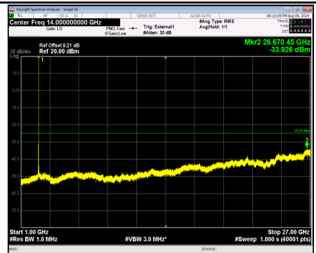
41-41-20MHz-5MHz-QPSK-QPSK-40595-40712-1RB#99-0 RB#0-1000~27000MHz-PASS
