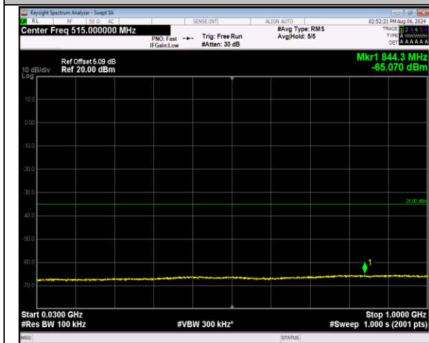
7-7-20MHz-20MHz-QPSK-QPSK-21152-21350-1RB#99-99 ORB#0-30~1000MHz-PASS
