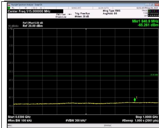
7-7-20MHz-20MHz-QPSK-QPSK-21152-21350-1RB#0-0 RB#0-30~1000MHz-PASS
