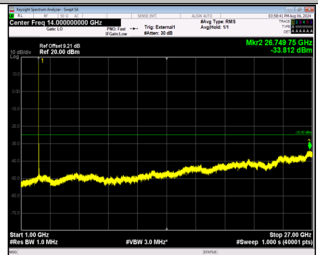
41-41-5MHz-20MHz-16QAM-16QAM-40528-40645-1RB#0-0RB#0-1000~27000MHz-PASS
