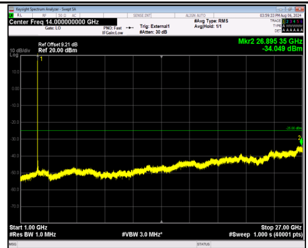
41-41-5MHz-20MHz-QPSK-QPSK-40528-40645-1RB#24-0 RB#0-1000~27000MHz-PASS
