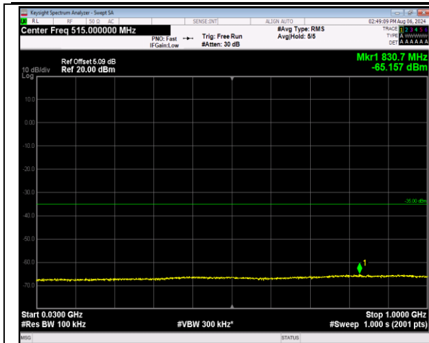
7-7-20MHz-20MHz-16QAM-16QAM-21001-21199-1RB#0 -1RB#99-30~1000MHz-PASS
