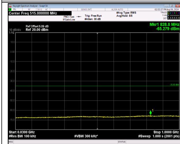
7-7-20MHz-20MHz-QPSK-QPSK-21152-21350-1RB#0-1 RB#99-30~1000MHz-PASS
