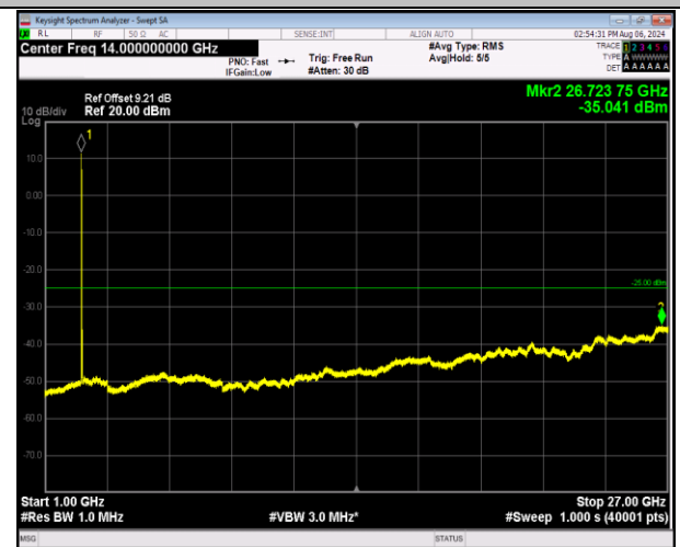
7-7-20MHz-20MHz-16QAM-16QAM-21152-21350-1RB#0-1 RB#99-1000~27000MHz-PASS
