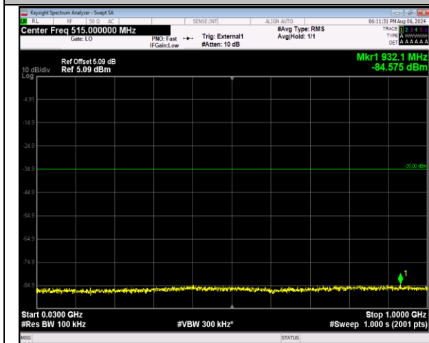
41-41-20MHz-5MHz-QPSK-QPSK-40595-40712-1RB#0-1RB#24-30~1000MHz-PASS
