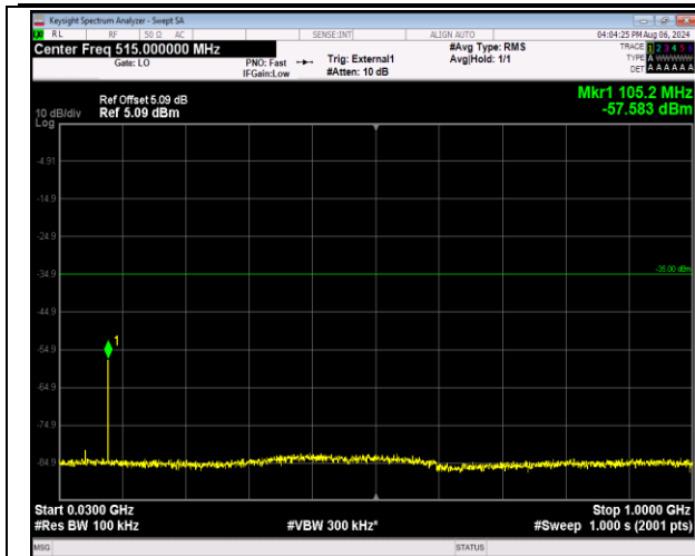
41-41-5MHz-20MHz-QPSK-QPSK-41373-41490-1RB#0- ORB#0-30~1000MHz-PASS
