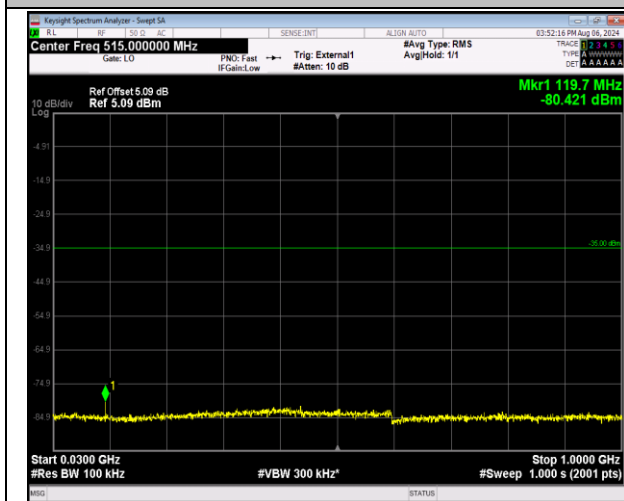
41-41-5MHz-20MHz-QPSK-QPSK-39683-39800-1RB#24 -ORB#0-30~1000MHz-PASS
