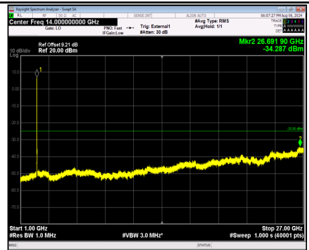
41-41-20MHz-5MHz-16QAM-16QAM-39750-39867-100RB# 0-25RB#0-1000~27000MHz-PASS
