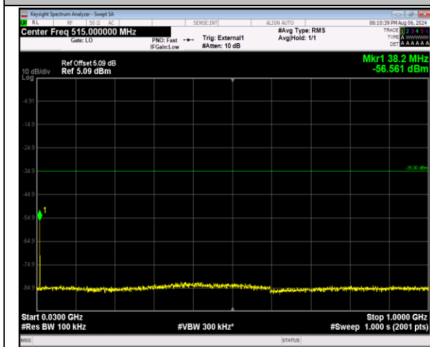
41-41-20MHz-5MHz-16QAM-16QAM-40595-40712-1RB#99-0RB#0-30~1000MHz-PASS
