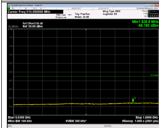
7-7-20MHz-20MHz-QPSK-QPSK-21001-21199-100RB#0 -100RB#0-30~1000MHz-PASS
