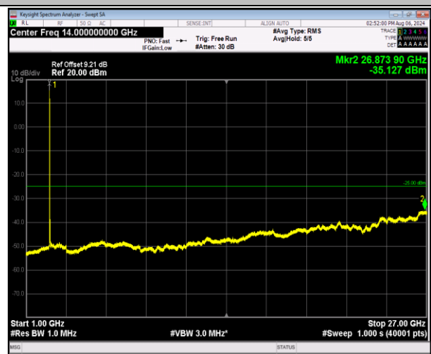
7-7-20MHz-20MHz-16QAM-16QAM-21152-21350-1RB#0-0 RB#0-1000~27000MHz-PASS
