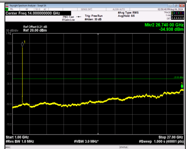
7-7-20MHz-20MHz-16QAM-16QAM-21001-21199-100RB#0 -100RB#0-1000~27000MHz-PASS
