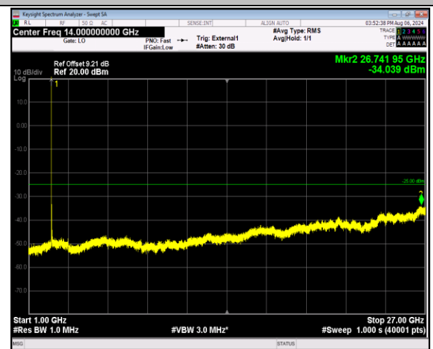
41-41-5MHz-20MHz-QPSK-QPSK-39683-39800-1RB#24-0 RB#0-1000~27000MHz-PASS
