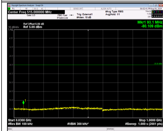
41-41-20MHz-5MHz-QPSK-QPSK-39750-39867-1RB#99 -ORB#0-30~1000MHz-PASS
