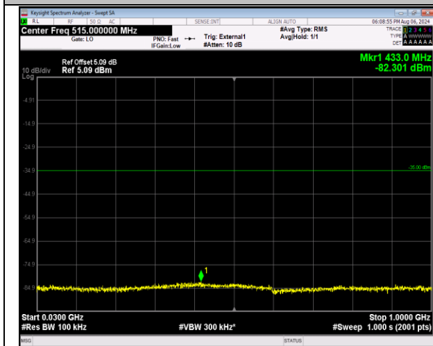
41-41-20MHz-5MHz-16QAM-16QAM-40595-40712-1RB# 0-0RB#0-30~1000MHz-PASS
