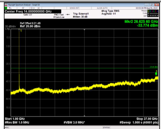
41-41-5MHz-20MHz-16QAM-16QAM-39683-39800-1RB#24 -ORB#0-1000~27000MHz-PASS
