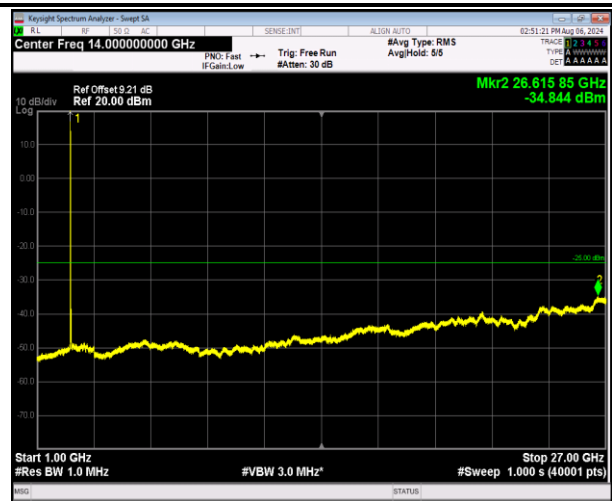
7-7-20MHz-20MHz-QPSK-QPSK-21152-21350-1RB#0-0RB #0-1000~27000MHz-PASS
