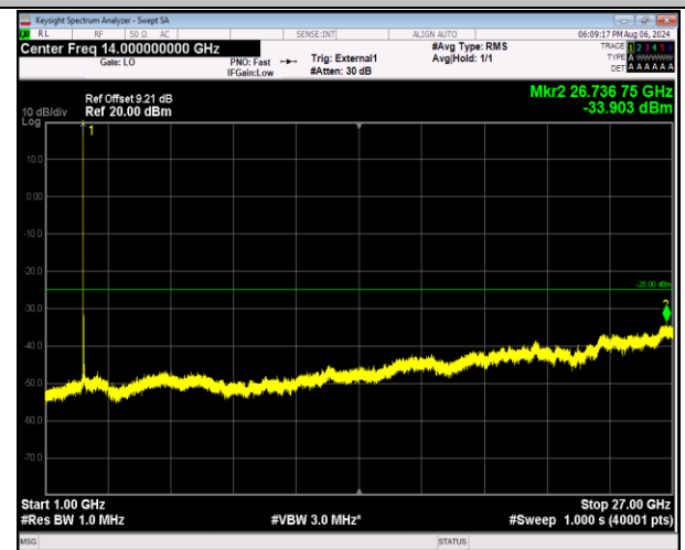
41-41-20MHz-5MHz-16QAM-16QAM-40595-40712-1RB#0-0RB#0-1000~27000MHz-PASS
