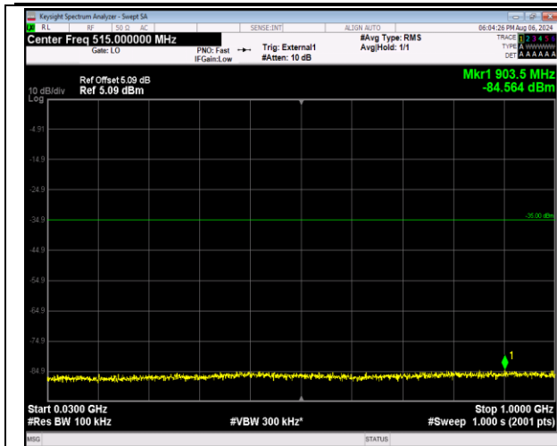
41-41-20MHz-5MHz-QPSK-QPSK-39750-39867-1RB#0-1RB#24-30~1000MHz-PASS
