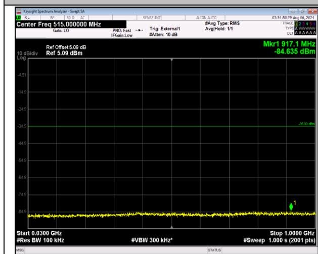
41-41-5MHz-20MHz-16QAM-16QAM-39683-39800-1RB#0-1RB#99-30~1000MHz-PASS
