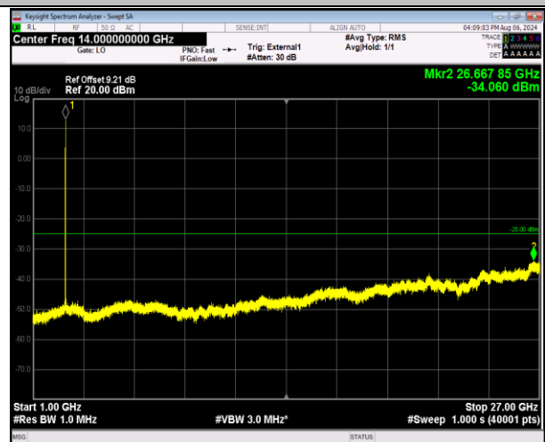
41-41-5MHz-20MHz-16QAM-16QAM-41373-41490-1RB#0-1RB#99-1000~27000MHz-PASS
