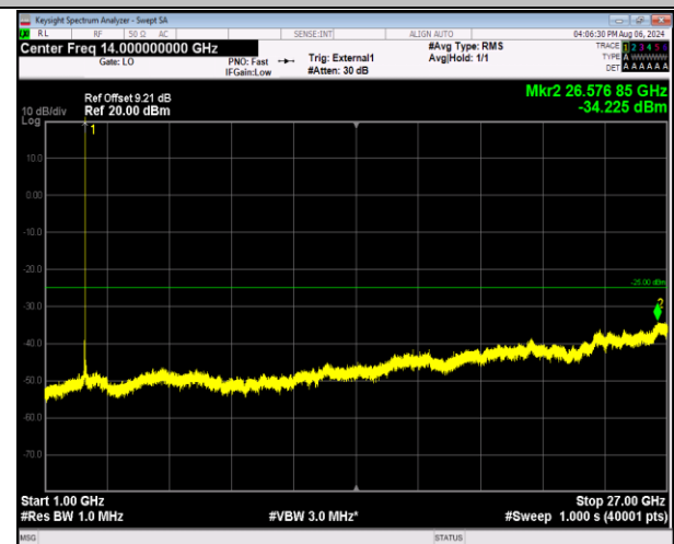
41-41-5MHz-20MHz-QPSK-QPSK-41373-41490-1RB#24-0 RB#0-1000~27000MHz-PASS
