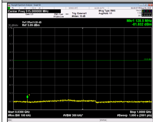
41-41-20MHz-5MHz-QPSK-QPSK-39750-39867-1RB#0-0 ORB#0-30~1000MHz-PASS
