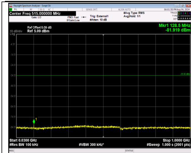
41-41-20MHz-5MHz-16QAM-16QAM-39750-39867-1RB# 0-ORB#0-30~1000MHz-PASS
