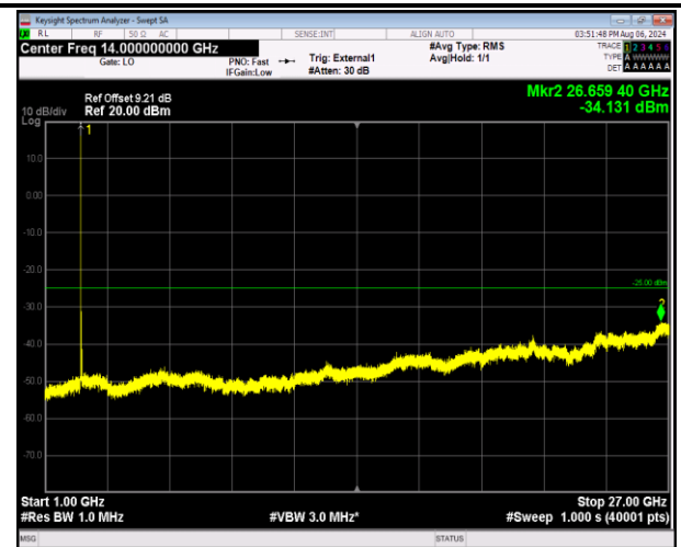
41-41-5MHz-20MHz-16QAM-16QAM-39683-39800-1RB#0- ORB#0-1000~27000MHz-PASS
