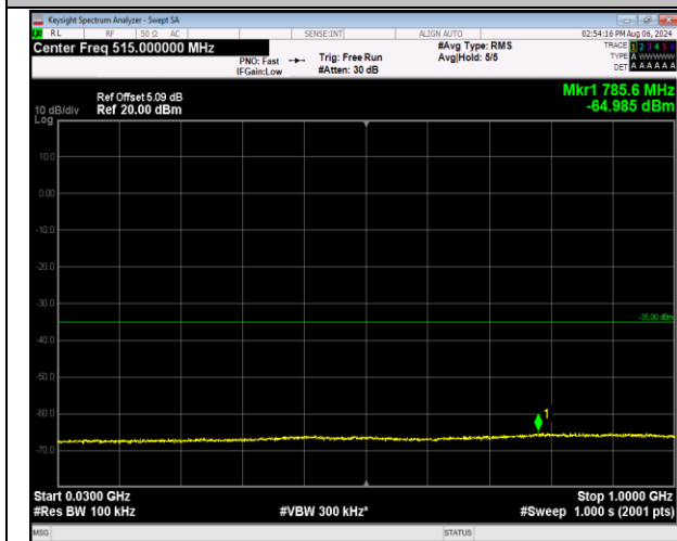
7-7-20MHz-20MHz-16QAM-16QAM-21152-21350-1RB#0 -1RB#99-30~1000MHz-PASS
