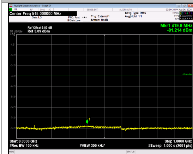
41-41-5MHz-20MHz-QPSK-QPSK-39683-39800-1RB#0-0 ORB#0-30~1000MHz-PASS
