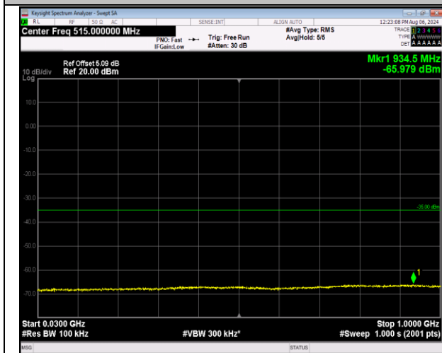
7-7-10MHz-20MHz-QPSK-QPSK-21006-21150-1RB#0-1RB#99-30~1000MHz-PASS
