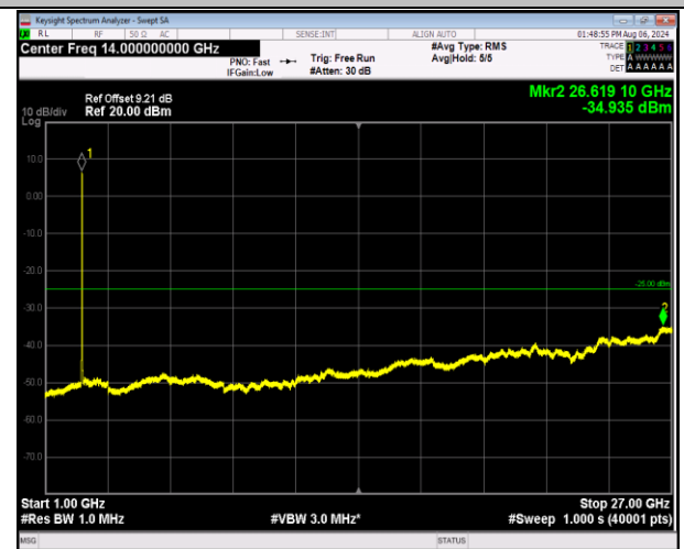
7-7-20MHz-10MHz-16QAM-16QAM-21051-21195-100RB#0 -50RB#0-1000~27000MHz-PASS
