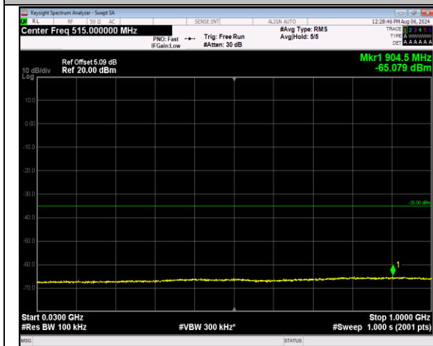
7-7-10MHz-20MHz-16QAM-16QAM-21206-21350-1RB#0 -1RB#99-30~1000MHz-PASS
