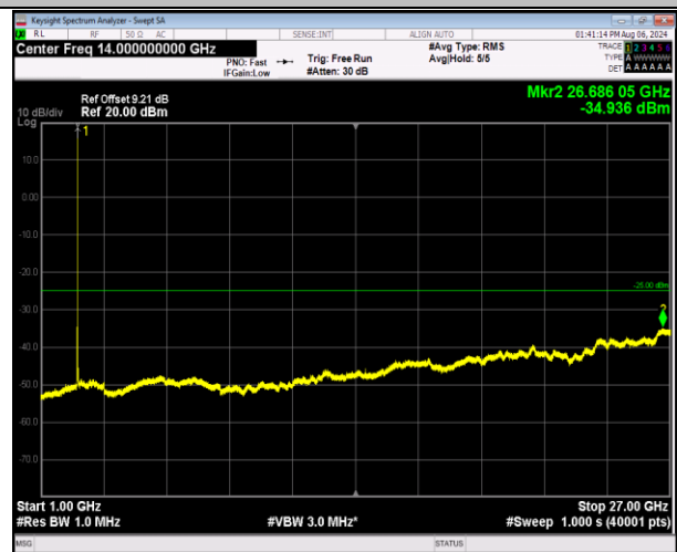
7-7-20MHz-10MHz-16QAM-16QAM-20850-20994-1RB#99-0 ORB#0-1000~27000MHz-PASS
