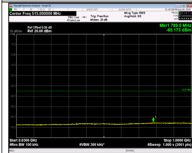
7-7-20MHz-10MHz-16QAM-16QAM-20850-20994-1RB#9 9-ORB#0-30~1000MHz-PASS
