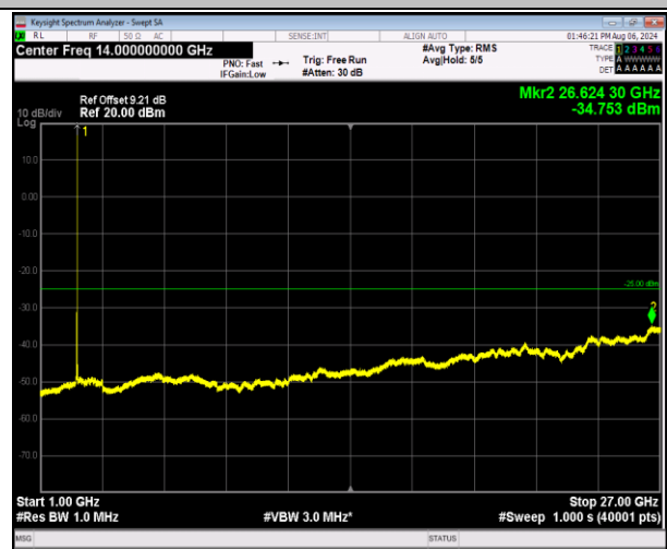
7-7-20MHz-10MHz-16QAM-16QAM-21051-21195-1RB#99-ORB#0-1000~27000MHz-PASS
