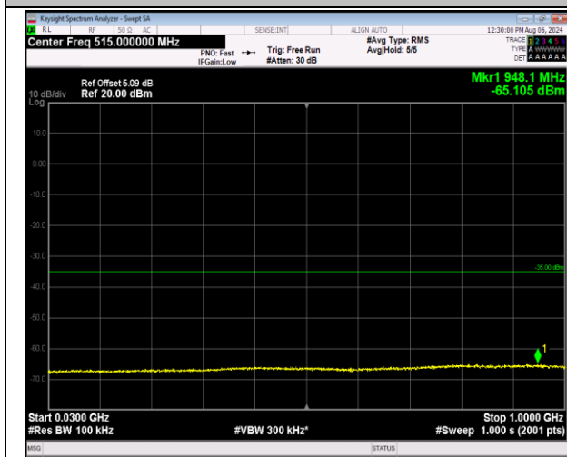
7-7-10MHz-20MHz-16QAM-16QAM-21206-21350-50RB#0-100RB#0-30~1000MHz-PASS
