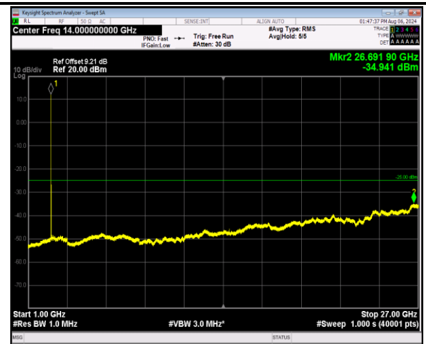
7-7-20MHz-10MHz-16QAM-16QAM-21051-21195-1RB#0-1 RB#49-1000~27000MHz-PASS
