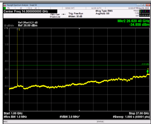
7-7-10MHz-20MHz-16QAM-16QAM-21006-21150-1RB#49-ORB#0-1000~27000MHz-PASS
