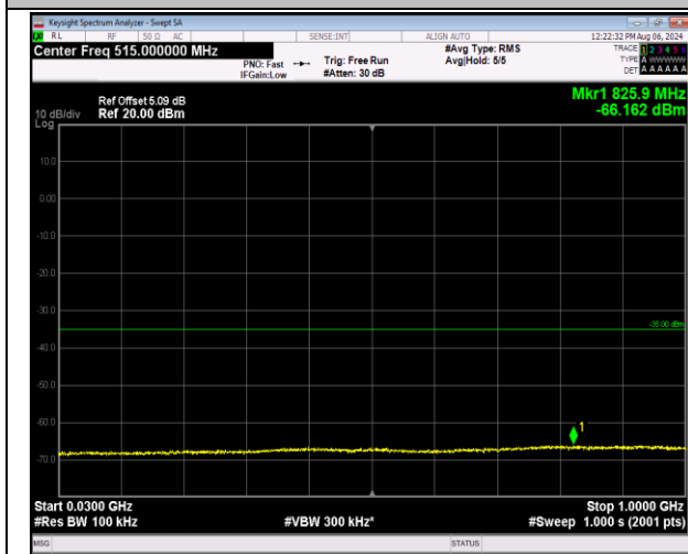
7-7-10MHz-20MHz-16QAM-16QAM-21006-21150-1RB#49-ORB#0-30~1000MHz-PASS
