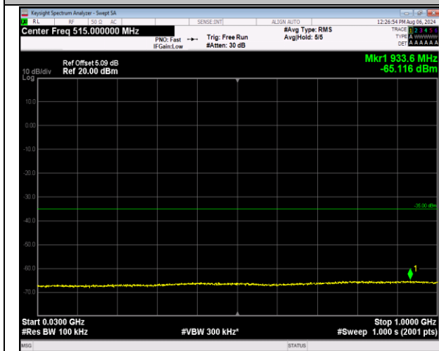
7-7-10MHz-20MHz-QPSK-QPSK-21206-21350-1RB#49-0RB#0-30~1000MHz-PASS
