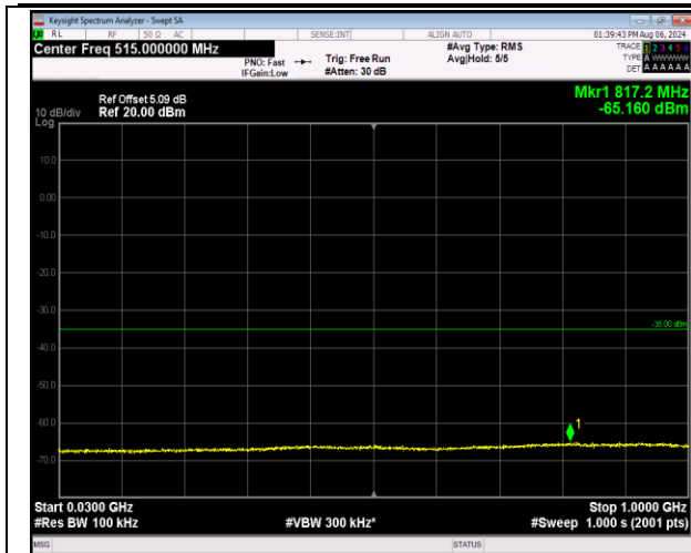
7-7-20MHz-10MHz-16QAM-16QAM-20850-20994-1RB#0 -ORB#0-30~1000MHz-PASS
