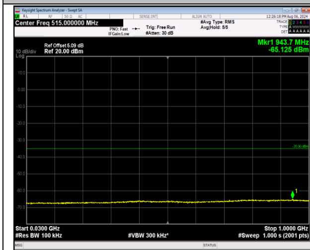
7-7-10MHz-20MHz-16QAM-16QAM-21206-21350-1RB#0-0RB#0-0-30~1000MHz-PASS
