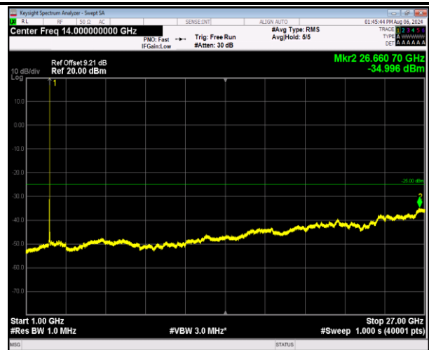
7-7-20MHz-10MHz-QPSK-QPSK-21051-21195-1RB#99-ORB#0-1000~27000MHz-PASS
