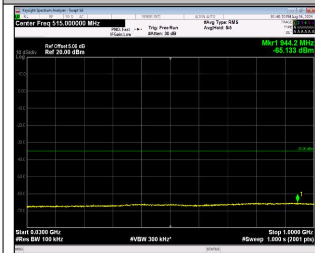
7-7-20MHz-10MHz-QPSK-QPSK-20850-20994-1RB#99-0 ORB#0-30~1000MHz-PASS
