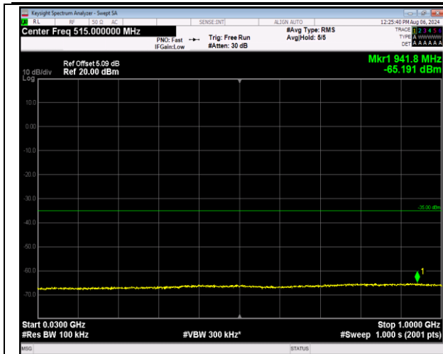
7-7-10MHz-20MHz-QPSK-QPSK-21206-21350-1RB#0-0 RB#0-30~1000MHz-PASS
