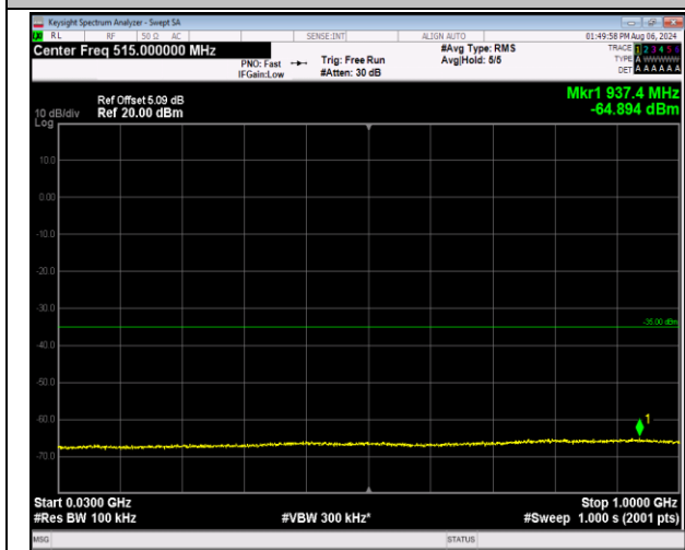
7-7-20MHz-10MHz-16QAM-16QAM-21251-21395-1RB#0-0RB #0-30~1000MHz-PASS
