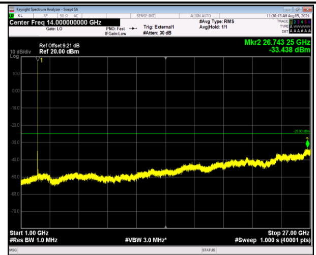
41-41-20MHz-10MHz-64QAM-64QAM-39750-39894-1RB#9 9-0RB#0-1000~27000MHz-PASS
