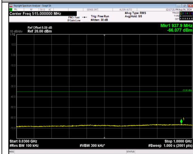
7-7-10MHz-20MHz-16QAM-16QAM-20805-20949-1RB#4 9-ORB#0-30~1000MHz-PASS
