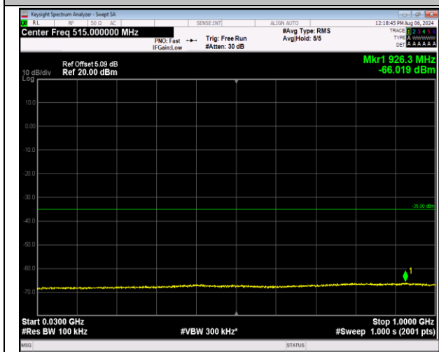
7-7-10MHz-20MHz-16QAM-16QAM-20805-20949-1RB#0 -1RB#99-30~1000MHz-PASS
