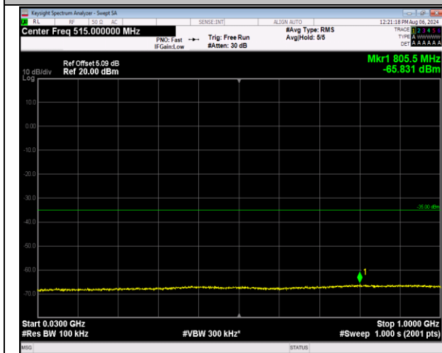
7-7-10MHz-20MHz-16QAM-16QAM-21006-21150-1RB#0 -0RB#0-30~1000MHz-PASS
