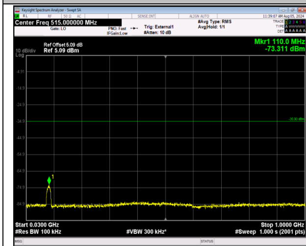
41-41-20MHz-10MHz-64QAM-64QAM-41391-41535-100RB RB#0-50RB#0-30~1000MHz-PASS
