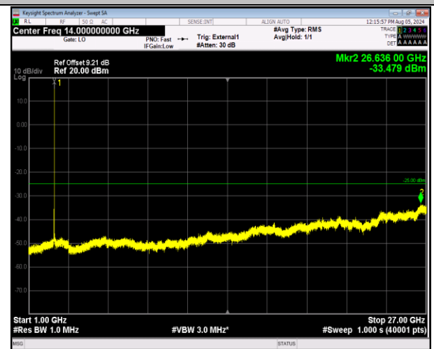
41-41-20MHz-20MHz-64QAM-64QAM-41292-41490-1RB#9 9-0RB#0-1000~27000MHz-PASS
