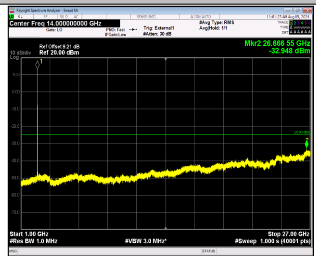
41-41-20MHz-5MHz-64QAM-64QAM-39750-39867-1RB#0- 1RB#24-1000~27000MHz-PASS
