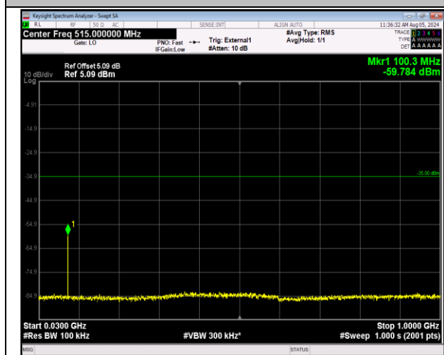
41-41-20MHz-10MHz-64QAM-64QAM-41391-41535-1RB #0-0RB#0-30~1000MHz-PASS
