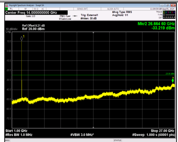
41-41-20MHz-5MHz-64QAM-64QAM-40595-40712-1RB#0- 1RB#24-1000~27000MHz-PASS
