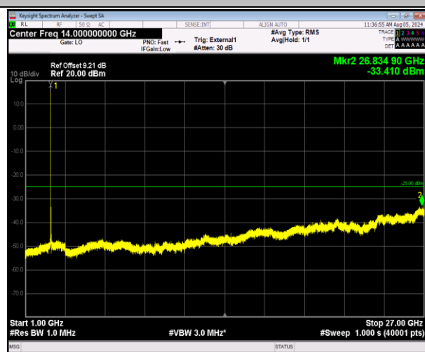
41-41-20MHz-10MHz-64QAM-64QAM-41391-41535-1RB#0 -0RB#0-1000~27000MHz-PASS
