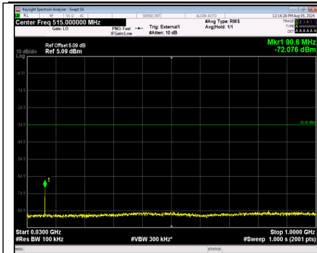
41-41-20MHz-20MHz-64QAM-64QAM-41292-41490-1RB #0-1RB#99-30~1000MHz-PASS
