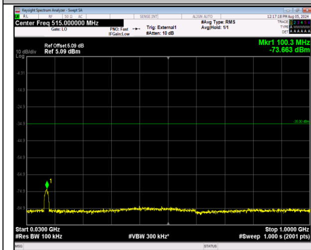
41-41-20MHz-20MHz-64QAM-64QAM-41292-41490-100RB RB#0-100RB#0-30~1000MHz-PASS
