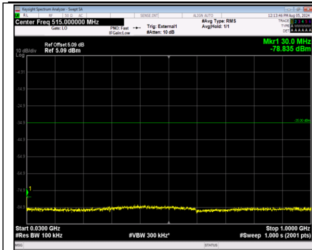
41-41-20MHz-20MHz-64QAM-64QAM-40521-40719-100 RB#0-100RB#0-30~1000MHz-PASS
