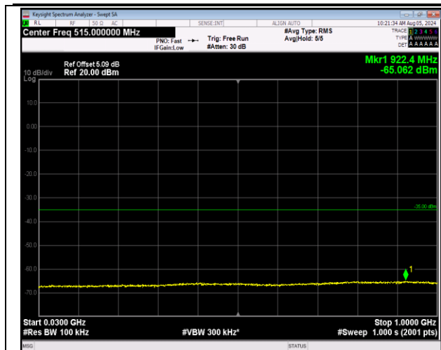
7-7-20MHz-20MHz-64QAM-64QAM-21152-21350-1RB#0 -1RB#99-30~1000MHz-PASS
