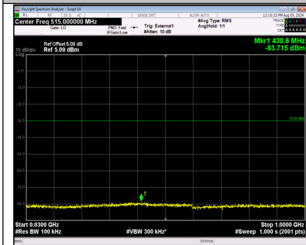
41-41-20MHz-20MHz-64QAM-64QAM-39750-39948-100 RB#0-100RB#0-30~1000MHz-PASS
