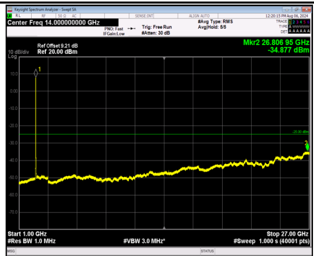
7-7-10MHz-20MHz-16QAM-16QAM-20805-20949-50RB#0- 100RB#0-1000~27000MHz-PASS
