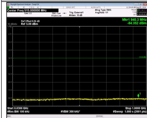
41-41-20MHz-10MHz-64QAM-64QAM-40571-40715-1RB #0-1RB#49-30~1000MHz-PASS
