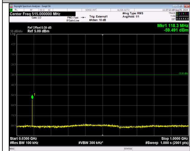
41-41-20MHz-10MHz-64QAM-64QAM-41391-41535-1RB #99-0RB#0-30~1000MHz-PASS
