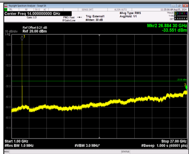
41-41-20MHz-10MHz-64QAM-64QAM-40571-40715-1RB#0 -1RB#49-1000~27000MHz-PASS
