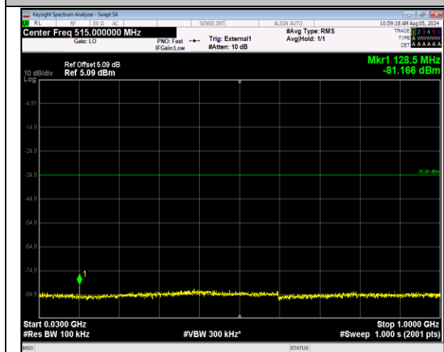
41-41-20MHz-5MHz-64QAM-64QAM-39750-39867-1RB# 0-0RB#0-30~1000MHz-PASS
