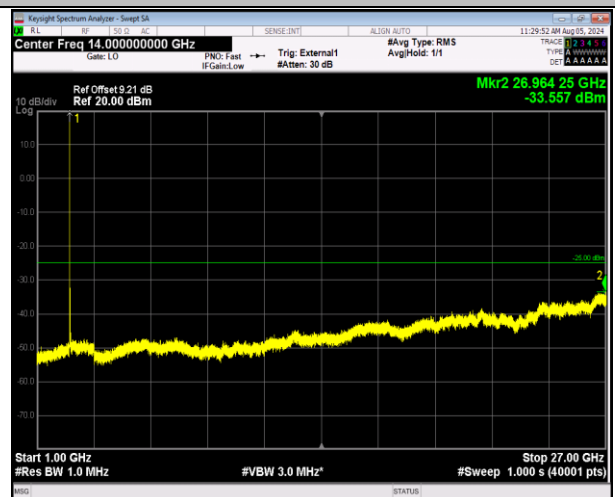
41-41-20MHz-10MHz-64QAM-64QAM-39750-39894-1RB#0 -ORB#0-1000~27000MHz-PASS
