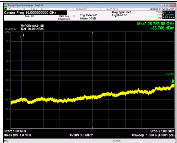
41-41-20MHz-5MHz-64QAM-64QAM-41440-41557-1RB#0- 1RB#24-1000~27000MHz-PASS
