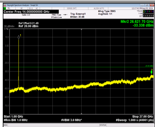
41-41-20MHz-20MHz-64QAM-64QAM-41292-41490-100RB #0-100RB#0-1000~27000MHz-PASS
