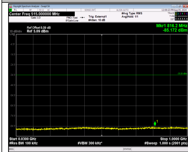
41-41-20MHz-20MHz-64QAM-64QAM-39750-39948-1RB #0-1RB#99-30~1000MHz-PASS
