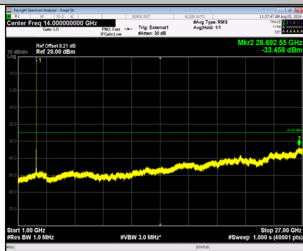
41-41-20MHz-10MHz-64QAM-64QAM-41391-41535-1RB#9 9-0RB#0-1000~27000MHz-PASS
