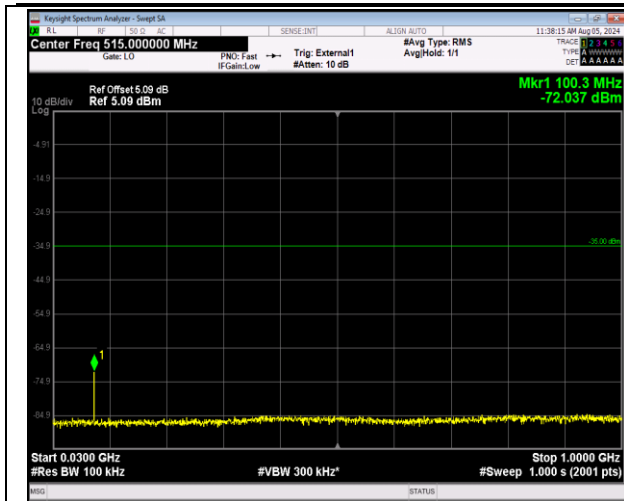
41-41-20MHz-10MHz-64QAM-64QAM-41391-41535-1RB #0-1RB#49-30~1000MHz-PASS
