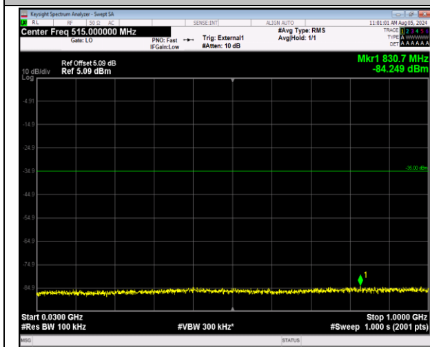
41-41-20MHz-5MHz-64QAM-64QAM-39750-39867-1RB# 0-1RB#24-30~1000MHz-PASS
