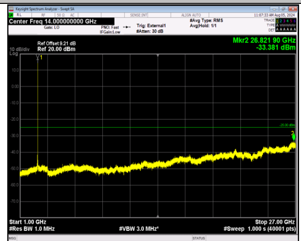
41-41-20MHz-5MHz-64QAM-64QAM-41440-41557-1RB#99 -0RB#0-1000~27000MHz-PASS
