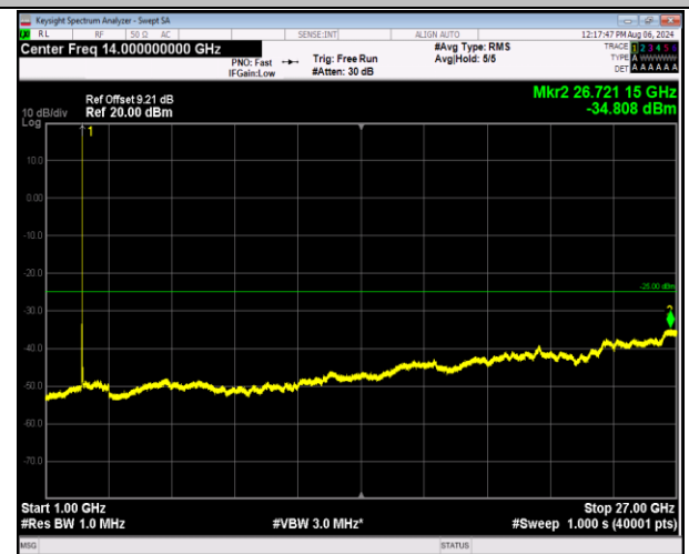
7-7-10MHz-20MHz-16QAM-16QAM-20805-20949-1RB#49-0 ORB#0-1000~27000MHz-PASS
