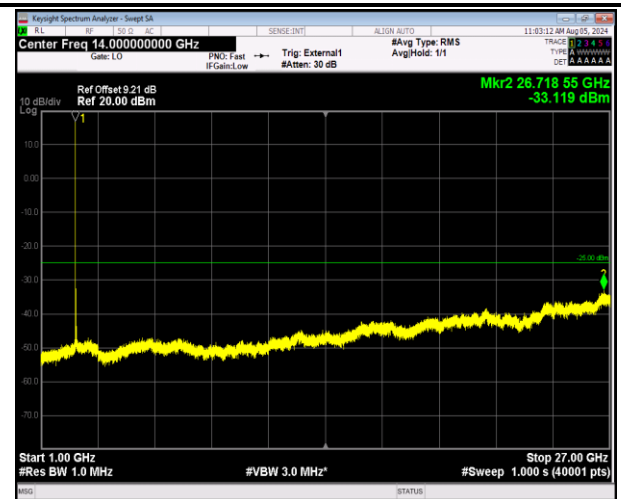
41-41-20MHz-5MHz-64QAM-64QAM-40595-40712-1RB#0- ORB#0-1000~27000MHz-PASS
