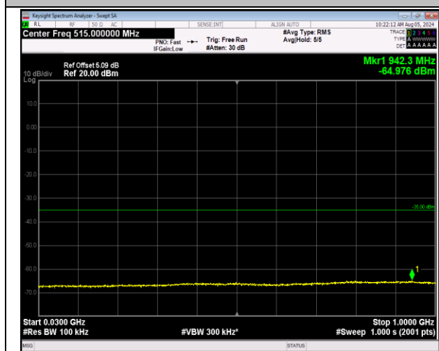
7-7-20MHz-20MHz-64QAM-64QAM-21152-21350-100RB #0-100RB#0-30~1000MHz-PASS
