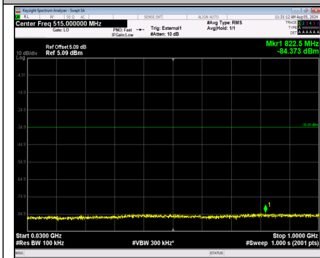
41-41-20MHz-10MHz-64QAM-64QAM-39750-39894-1RB #0-1RB#49-30~1000MHz-PASS
