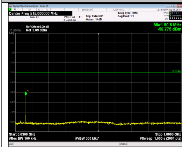
41-41-20MHz-20MHz-64QAM-64QAM-41292-41490-1RB #0-0RB#0-30~1000MHz-PASS
