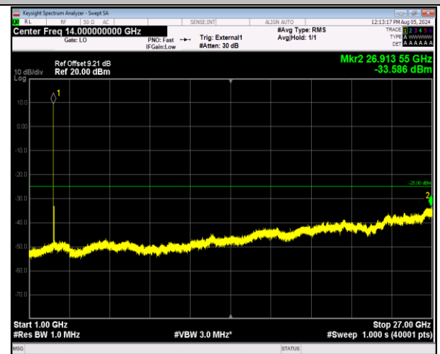
41-41-20MHz-20MHz-64QAM-64QAM-40521-40719-1RB#0 -1RB#99-1000~27000MHz-PASS
