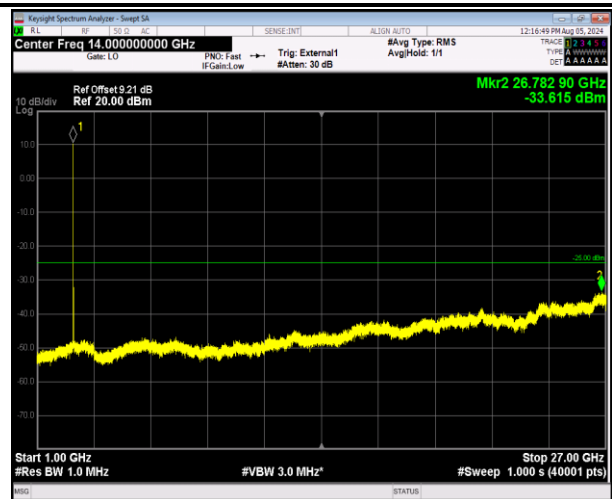
41-41-20MHz-20MHz-64QAM-64QAM-41292-41490-1RB#0 -1RB#99-1000~27000MHz-PASS
