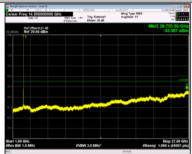
41-41-20MHz-5MHz-64QAM-64QAM-40595-40712-1RB#99 -ORB#0-1000~27000MHz-PASS
