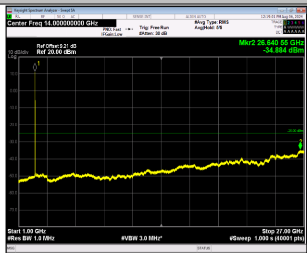
7-7-10MHz-20MHz-16QAM-16QAM-20805-20949-1RB#0-1 RB#99-1000~27000MHz-PASS
