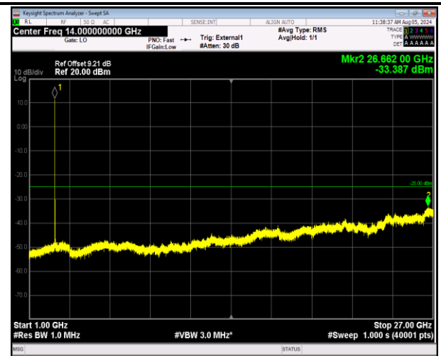
41-41-20MHz-10MHz-64QAM-64QAM-41391-41535-1RB#0 -1RB#49-1000~27000MHz-PASS
