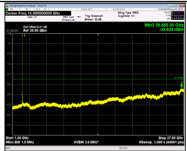
41-41-20MHz-20MHz-64QAM-64QAM-39750-39948-1RB#9 9-0RB#0-1000~27000MHz-PASS
