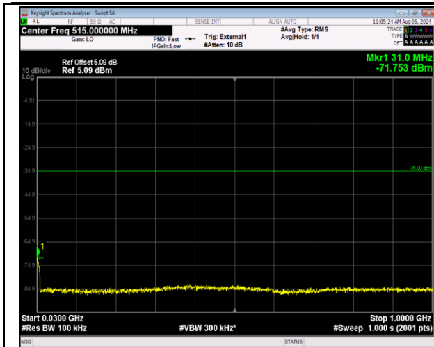
41-41-20MHz-5MHz-64QAM-64QAM-40595-40712-100R B#0-25RB#0-30~1000MHz-PASS
