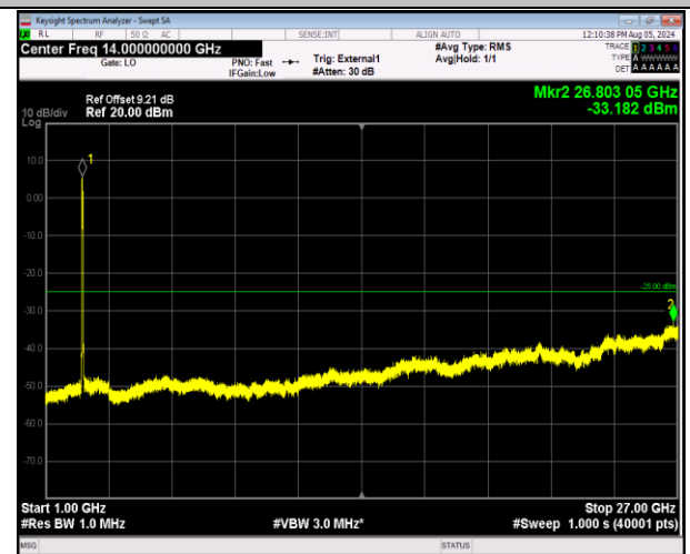
41-41-20MHz-20MHz-64QAM-64QAM-39750-39948-100RB #0-100RB#0-1000~27000MHz-PASS
