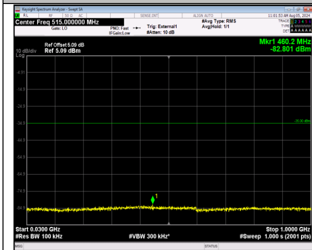
41-41-20MHz-5MHz-64QAM-64QAM-39750-39867-100R B#0-25RB#0-30~1000MHz-PASS
