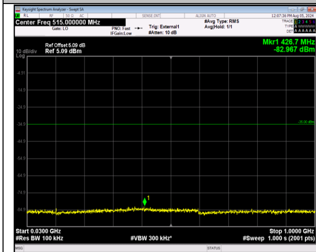
41-41-20MHz-20MHz-64QAM-64QAM-39750-39948-1RB #0-ORB#0-30~1000MHz-PASS
