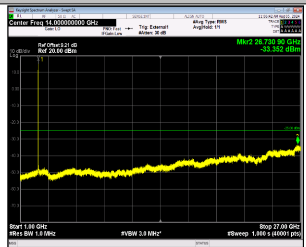
41-41-20MHz-5MHz-64QAM-64QAM-41440-41557-1RB#0- 0RB#0-1000~27000MHz-PASS
