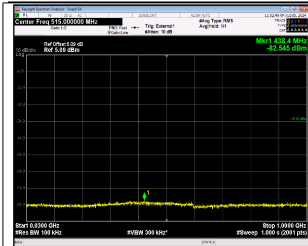
41-41-20MHz-5MHz-64QAM-64QAM-40595-40712-1RB# 0-ORB#0-30~1000MHz-PASS
