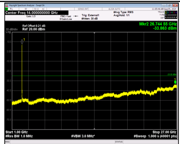
41-41-20MHz-5MHz-64QAM-64QAM-40595-40712-100RB# 0-25RB#0-1000~27000MHz-PASS
