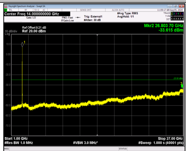
41-41-20MHz-5MHz-64QAM-64QAM-41440-41557-100RB# 0-25RB#0-1000~27000MHz-PASS
