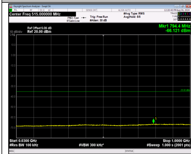
7-7-10MHz-20MHz-QPSK-QPSK-21006-21150-1RB#0-0 RB#0-30~1000MHz-PASS
