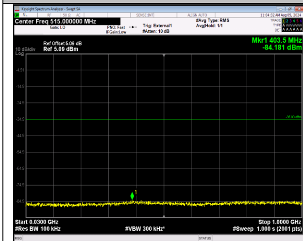
41-41-20MHz-5MHz-64QAM-64QAM-40595-40712-1RB# 0-1RB#24-30~1000MHz-PASS
