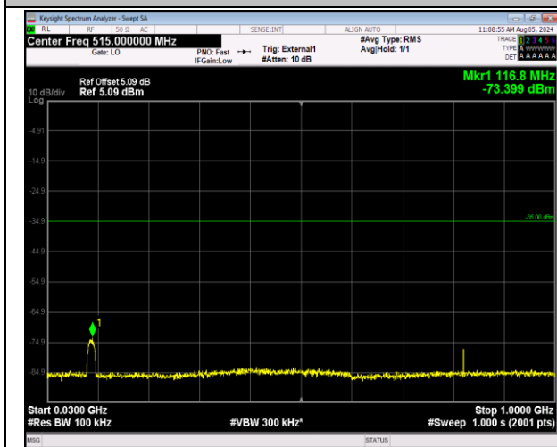
41-41-20MHz-5MHz-64QAM-64QAM-41440-41557-100RB B#0-25RB#0-30~1000MHz-PASS
