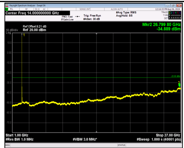
7-7-10MHz-20MHz-16QAM-16QAM-20805-20949-1RB#0-0 RB#0-1000~27000MHz-PASS
