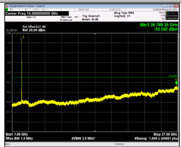
41-41-20MHz-20MHz-64QAM-64QAM-39750-39948-1RB#0 -1RB#99-1000~27000MHz-PASS
