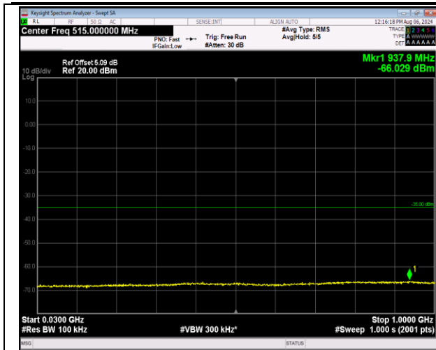
7-7-10MHz-20MHz-16QAM-16QAM-20805-20949-1RB#0 -ORB#0-30~1000MHz-PASS
