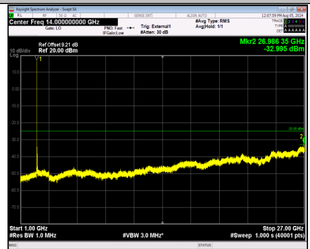
41-41-20MHz-20MHz-64QAM-64QAM-39750-39948-1RB#0 -ORB#0-1000~27000MHz-PASS
