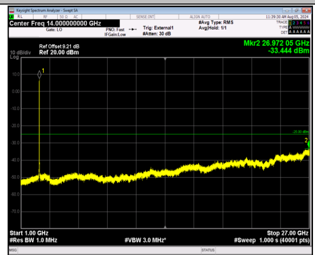
41-41-20MHz-10MHz-64QAM-64QAM-41391-41535-100RB#0 #0-50RB#0-1000~27000MHz-PASS
