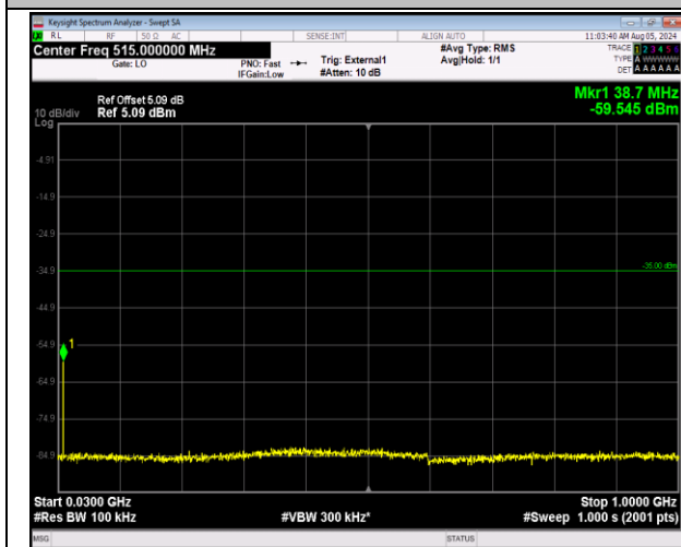
41-41-20MHz-5MHz-64QAM-64QAM-40595-40712-1RB# 99-ORB#0-30~1000MHz-PASS
