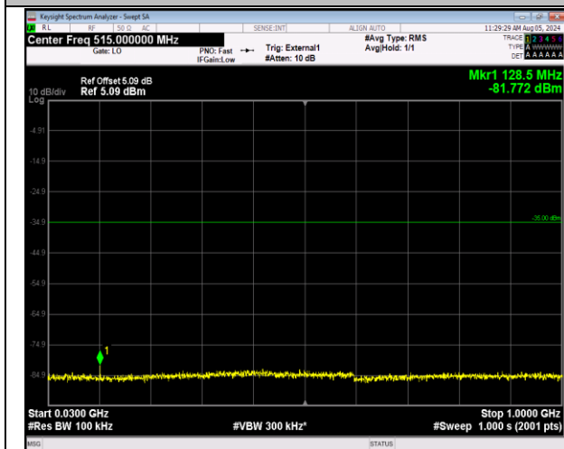
41-41-20MHz-10MHz-64QAM-64QAM-39750-39894-1RB #0-ORB#0-30~1000MHz-PASS
