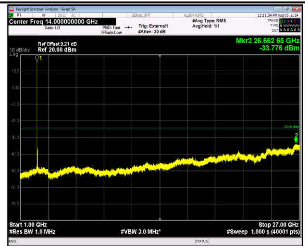
41-41-20MHz-20MHz-64QAM-64QAM-40521-40719-1RB#0 -ORB#0-1000~27000MHz-PASS
