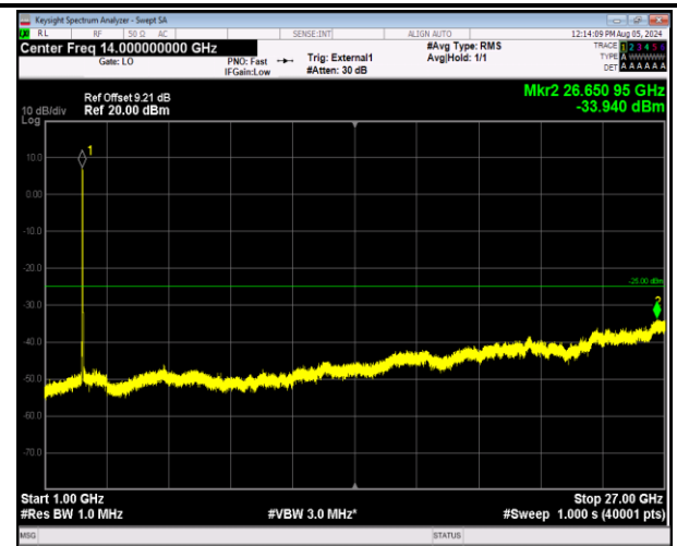
41-41-20MHz-20MHz-64QAM-64QAM-40521-40719-100RB #0-100RB#0-1000~27000MHz-PASS
