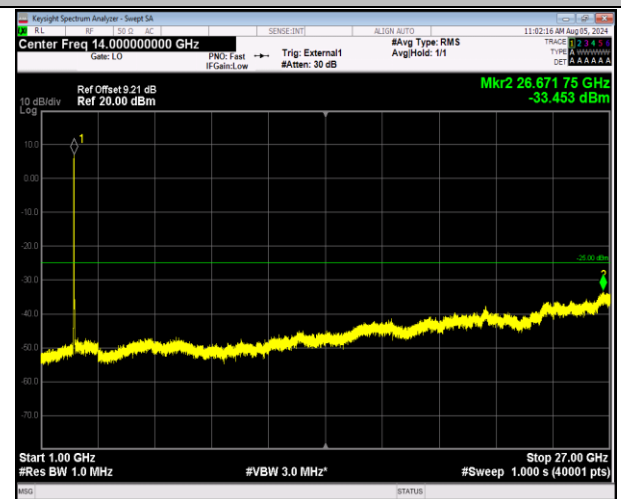
41-41-20MHz-5MHz-64QAM-64QAM-39750-39867-100RB# 0-25RB#0-1000~27000MHz-PASS
