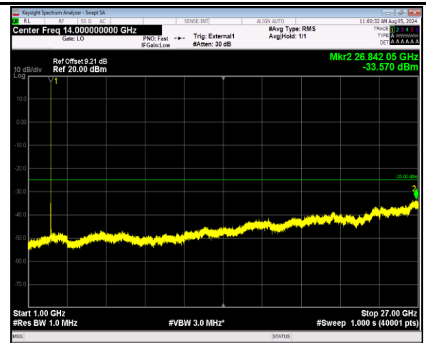
41-41-20MHz-5MHz-64QAM-64QAM-39750-39867-1RB#99 -ORB#0-1000~27000MHz-PASS
