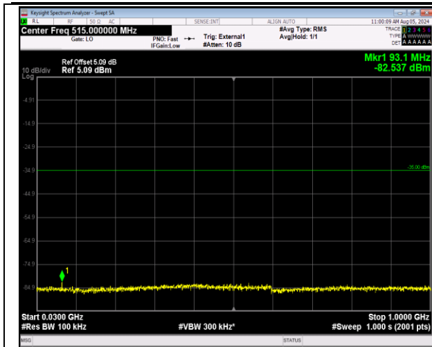
41-41-20MHz-5MHz-64QAM-64QAM-39750-39867-1RB# 99-ORB#0-30~1000MHz-PASS
