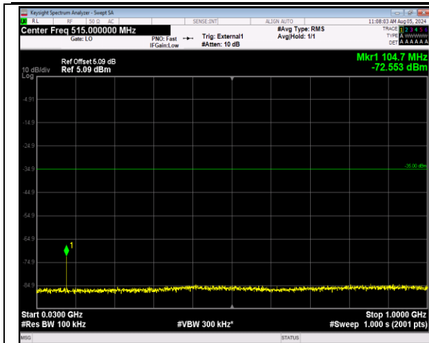
41-41-20MHz-5MHz-64QAM-64QAM-41440-41557-1RB# 0-1RB#24-30~1000MHz-PASS
