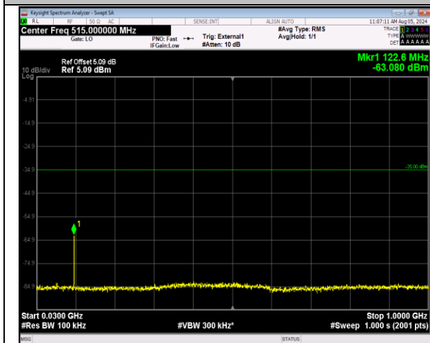
41-41-20MHz-5MHz-64QAM-64QAM-41440-41557-1RB# 99-0RB#0-30~1000MHz-PASS
