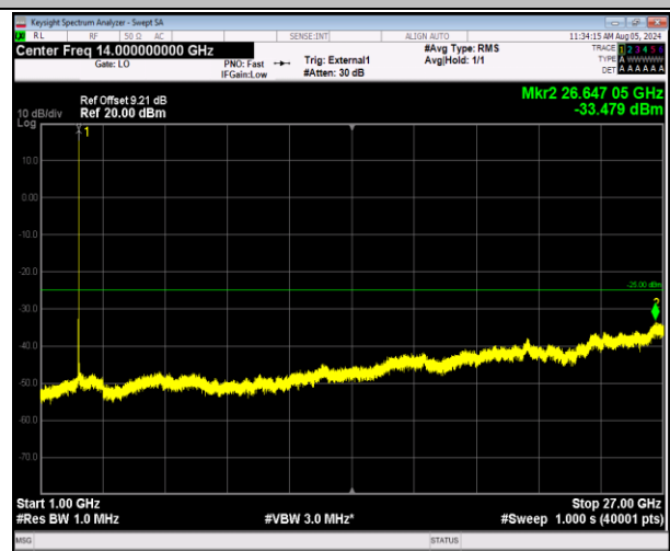
41-41-20MHz-10MHz-64QAM-64QAM-40571-40715-1RB#9 9-ORB#0-1000~27000MHz-PASS
