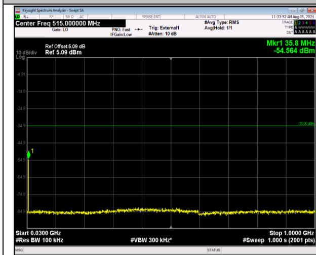
41-41-20MHz-10MHz-64QAM-64QAM-40571-40715-1RB #99-ORB#0-30~1000MHz-PASS
