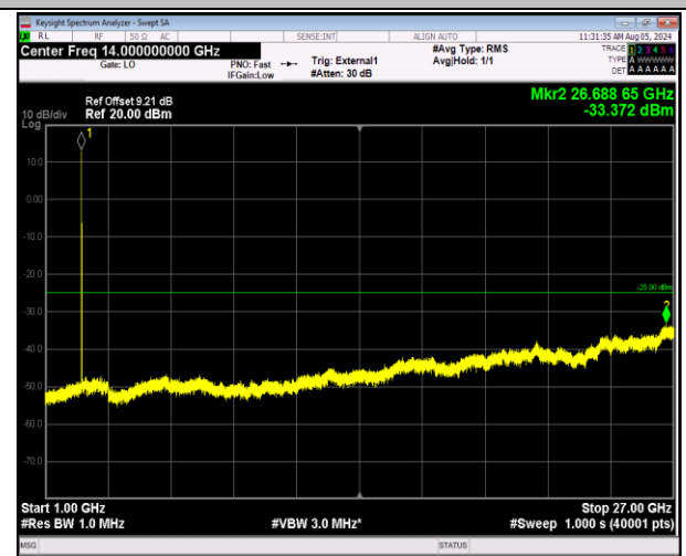
41-41-20MHz-10MHz-64QAM-64QAM-39750-39894-1RB#0 -1RB#49-1000~27000MHz-PASS
