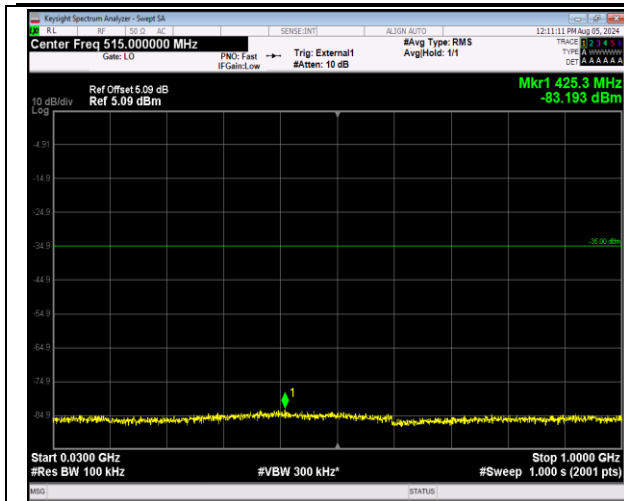
41-41-20MHz-20MHz-64QAM-64QAM-40521-40719-1RB #0-ORB#0-30~1000MHz-PASS
