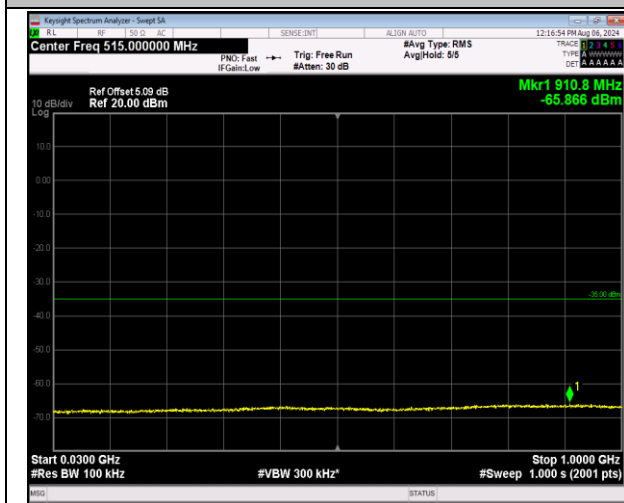
7-7-10MHz-20MHz-QPSK-QPSK-20805-20949-1RB#49-0 ORB#0-30~1000MHz-PASS
