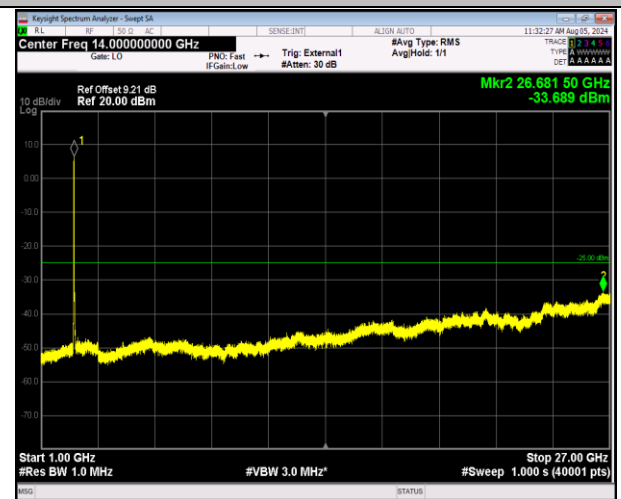
41-41-20MHz-10MHz-64QAM-64QAM-39750-39894-100RB #0-50RB#0-1000~27000MHz-PASS
