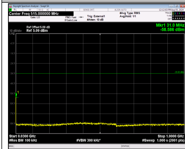
41-41-20MHz-20MHz-64QAM-64QAM-40521-40719-1RB #99-ORB#0-30~1000MHz-PASS
