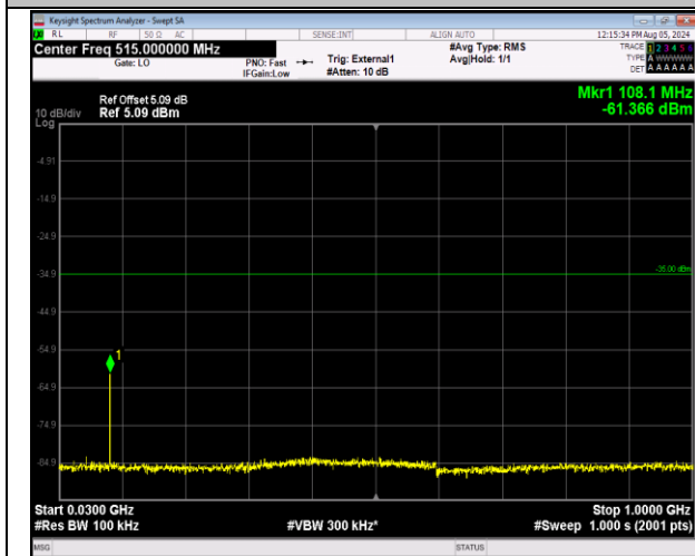
41-41-20MHz-20MHz-64QAM-64QAM-41292-41490-1RB #99-0RB#0-30~1000MHz-PASS
