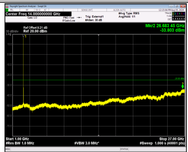
41-41-20MHz-20MHz-64QAM-64QAM-41292-41490-1RB#0 -0RB#0-1000~27000MHz-PASS
