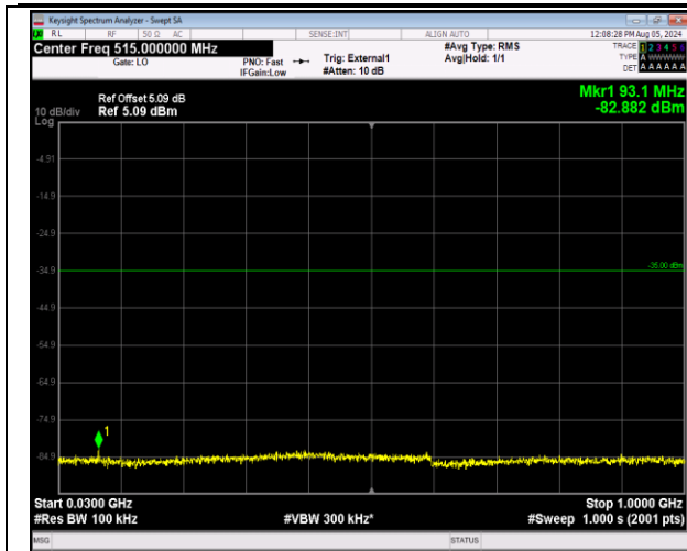
41-41-20MHz-20MHz-64QAM-64QAM-39750-39948-1RB #99-0RB#0-30~1000MHz-PASS
